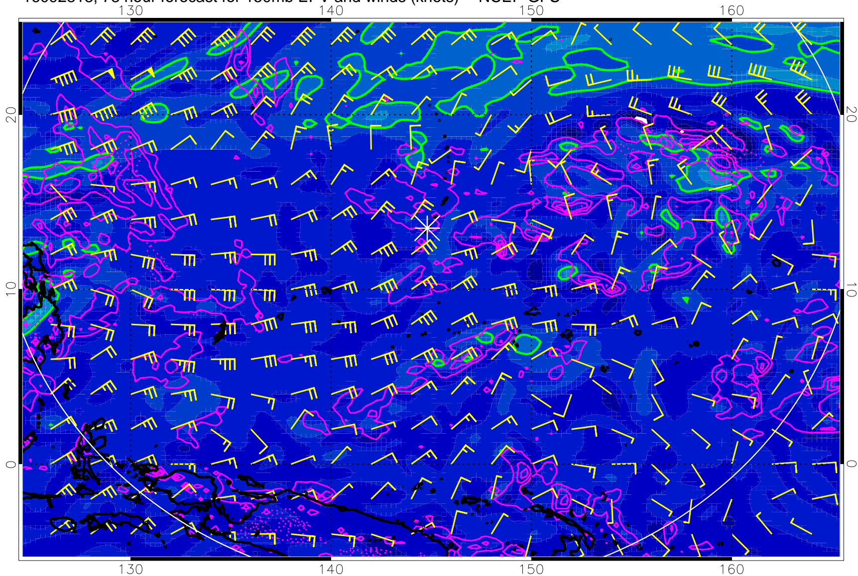
16092818, 78 hour forecast for 150mb EPV and winds (knots) -- NCEP GFS
