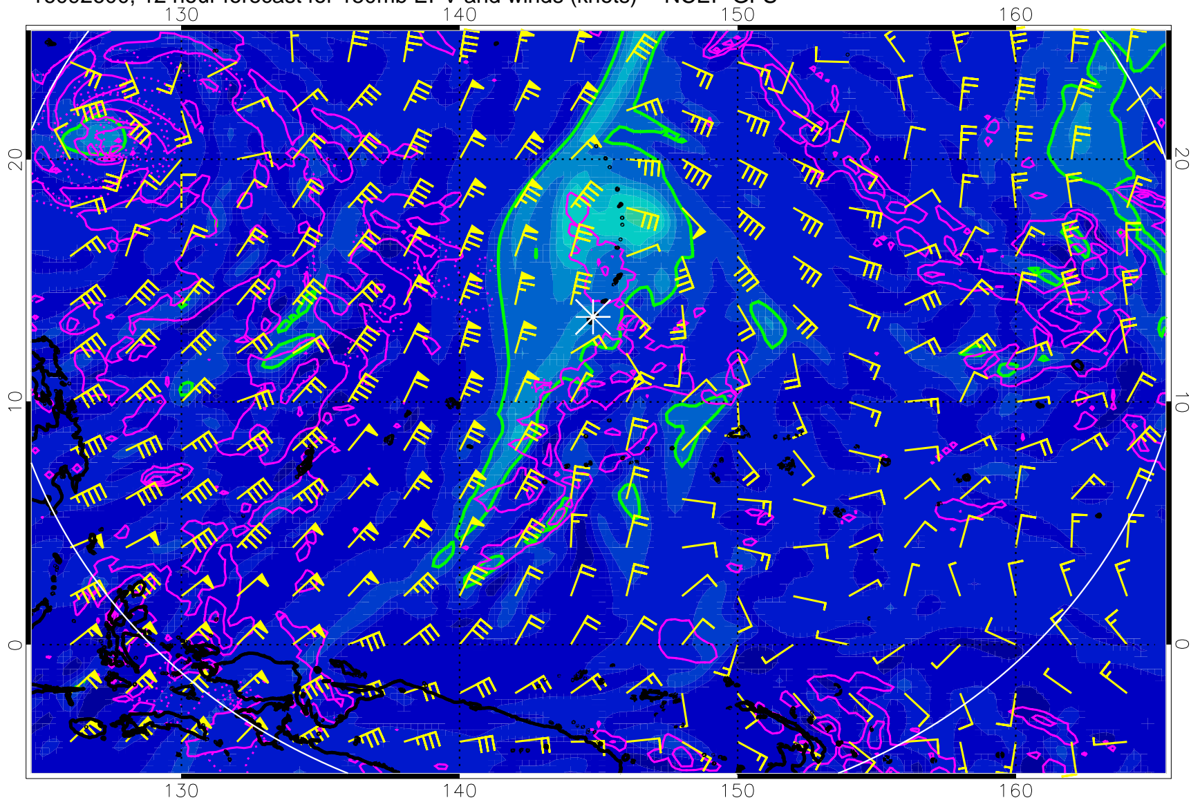
16092600, 12 hour forecast for 150mb EPV and winds (knots) -- NCEP GFS
