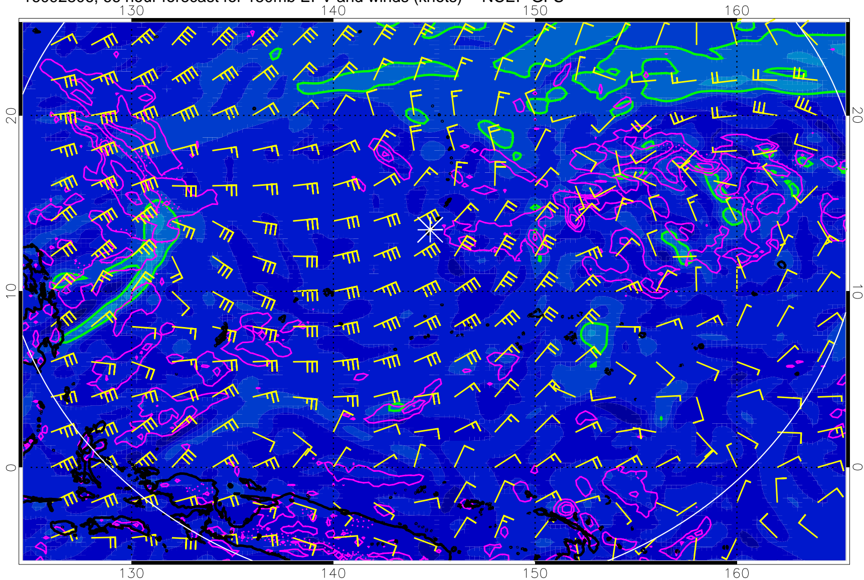
16092806, 66 hour forecast for 150mb EPV and winds (knots) -- NCEP GFS
