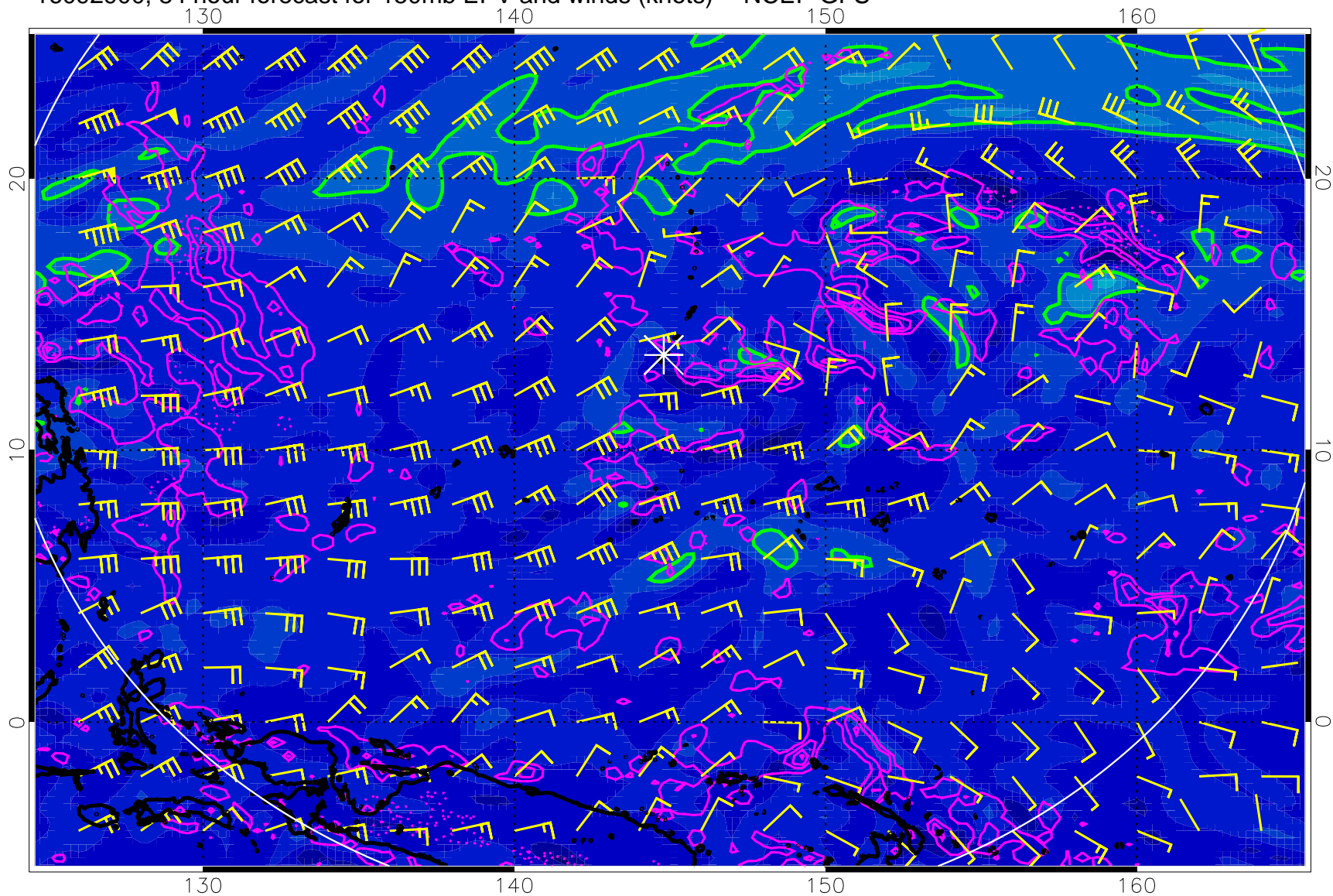
16092900, 84 hour forecast for 150mb EPV and winds (knots) -- NCEP GFS
