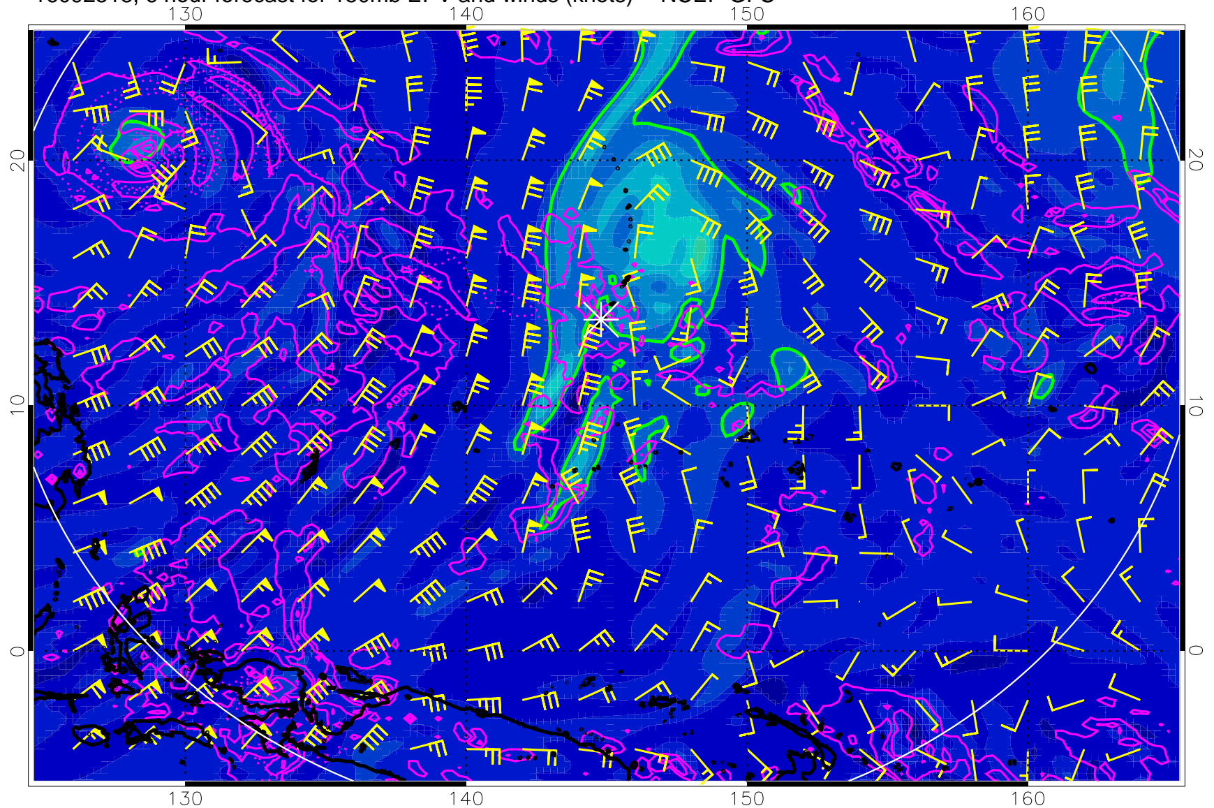
16092518, 6 hour forecast for 150mb EPV and winds (knots) -- NCEP GFS
