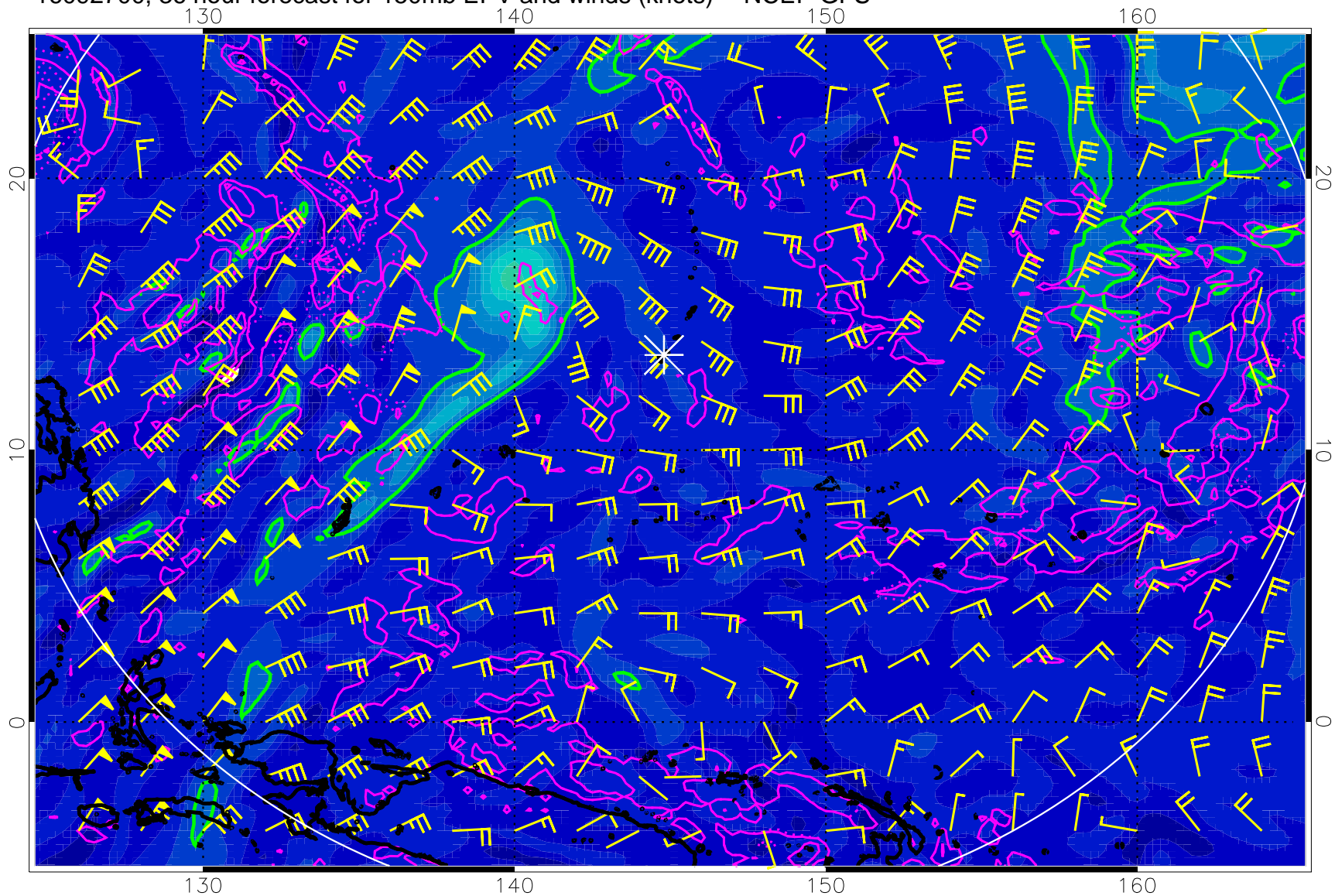
16092700, 36 hour forecast for 150mb EPV and winds (knots) -- NCEP GFS
