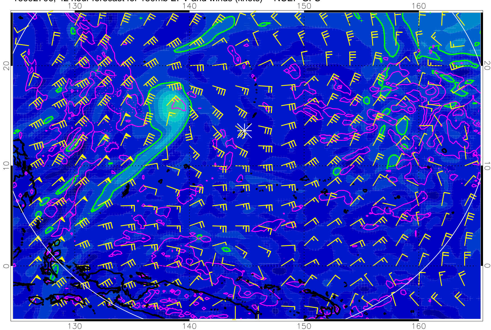
16092706, 42 hour forecast for 150mb EPV and winds (knots) -- NCEP GFS
