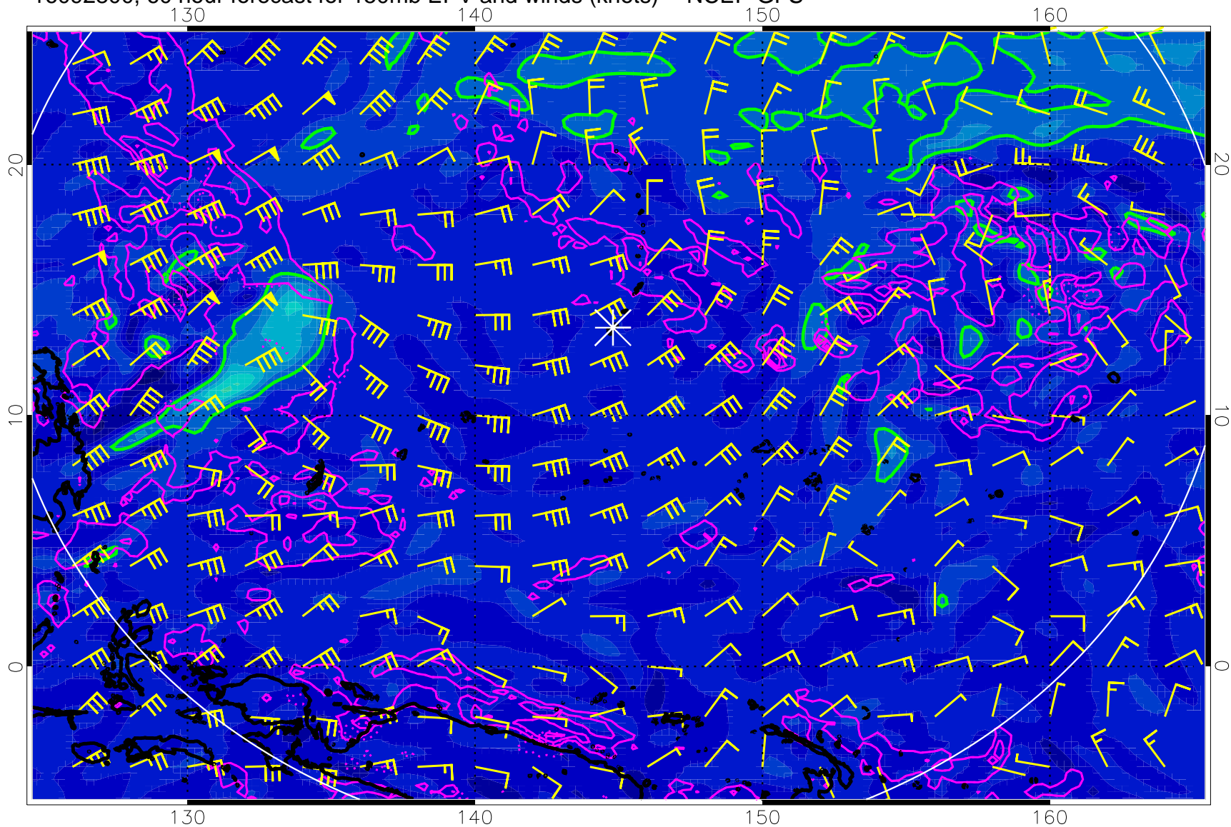
16092800, 60 hour forecast for 150mb EPV and winds (knots) -- NCEP GFS
