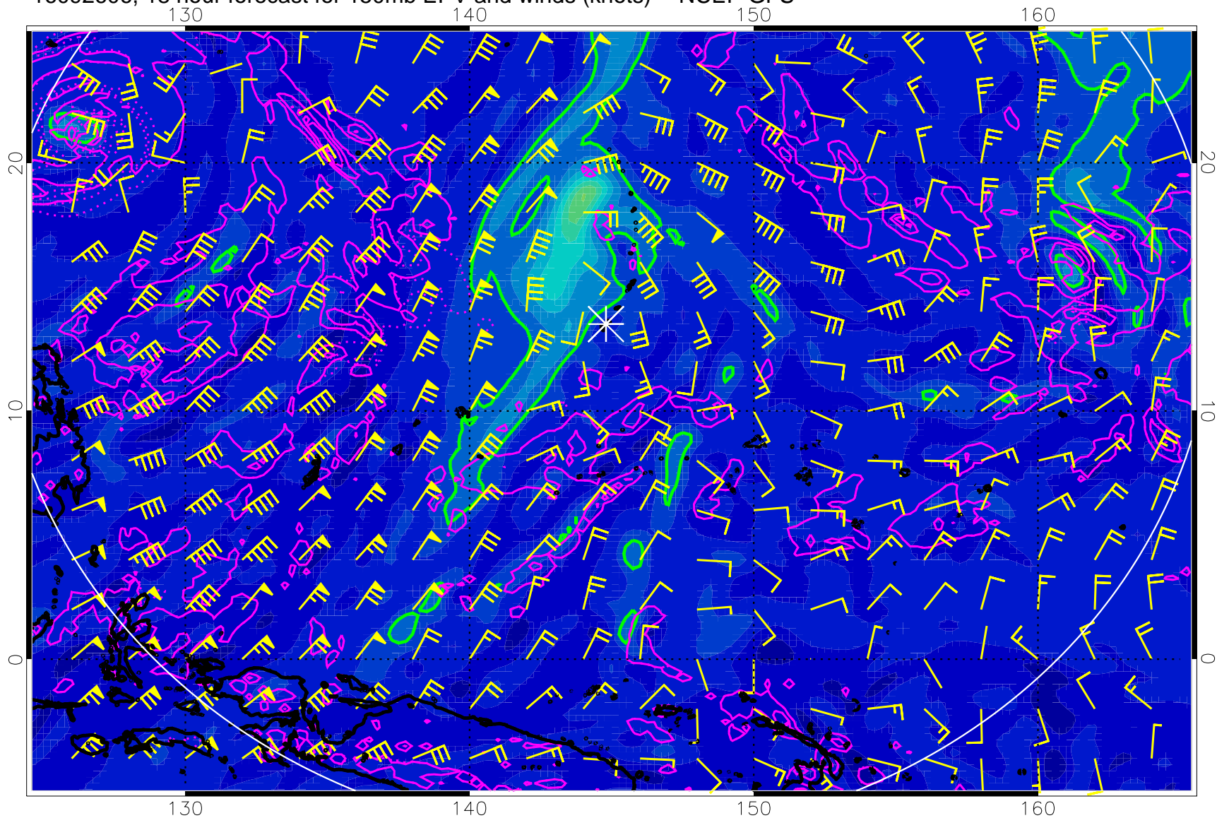
16092606, 18 hour forecast for 150mb EPV and winds (knots) -- NCEP GFS
