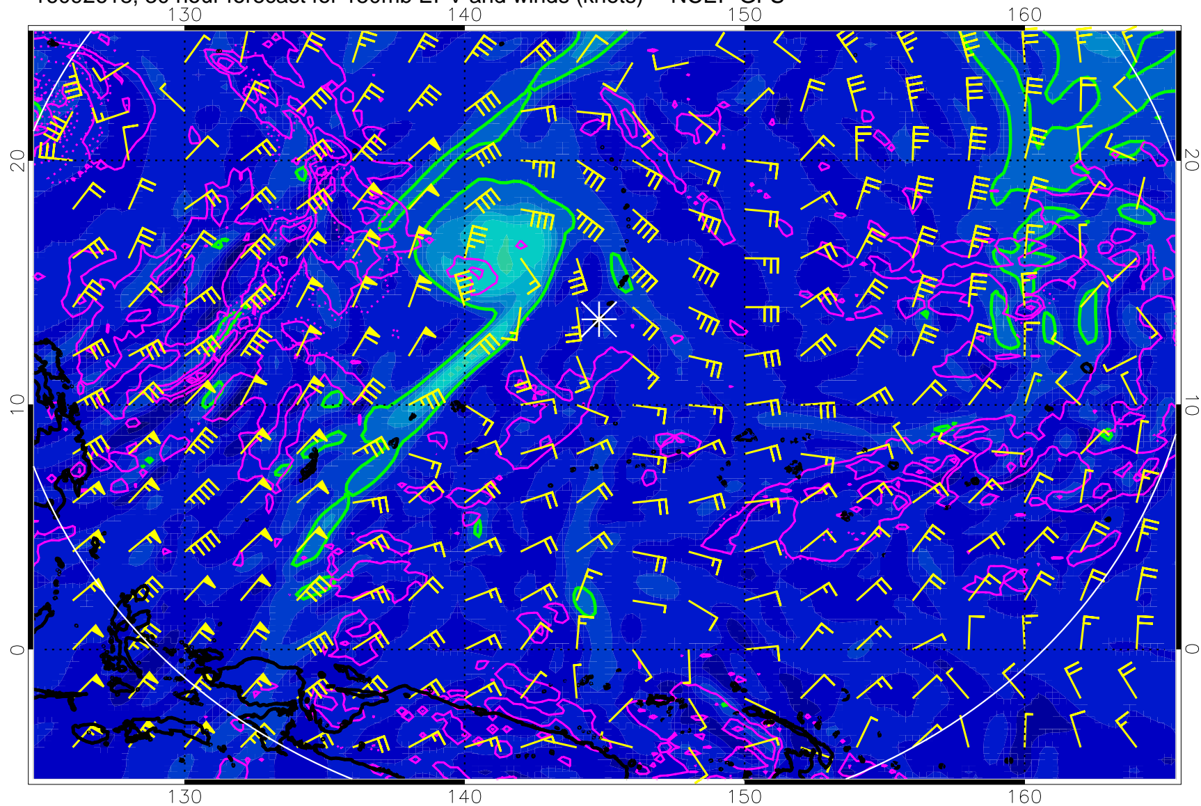
16092618, 30 hour forecast for 150mb EPV and winds (knots) -- NCEP GFS
