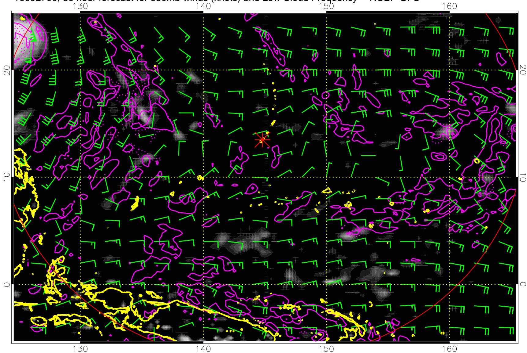
16092700, 36 hour forecast for 850mb winds (knots) and Low Cloud Frequency -- NCEP GFS
