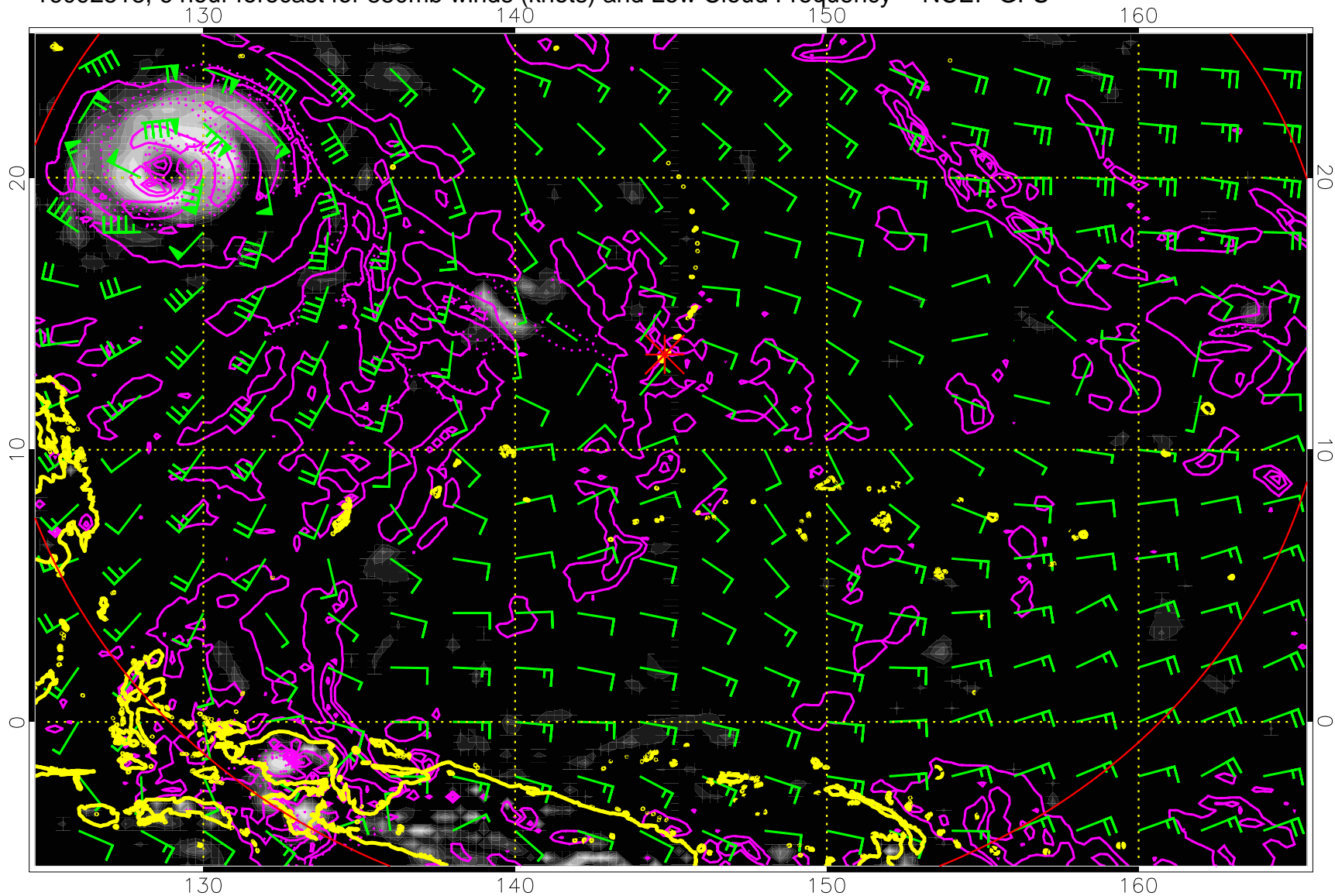
16092518, 6 hour forecast for 850mb winds (knots) and Low Cloud Frequency -- NCEP GFS
