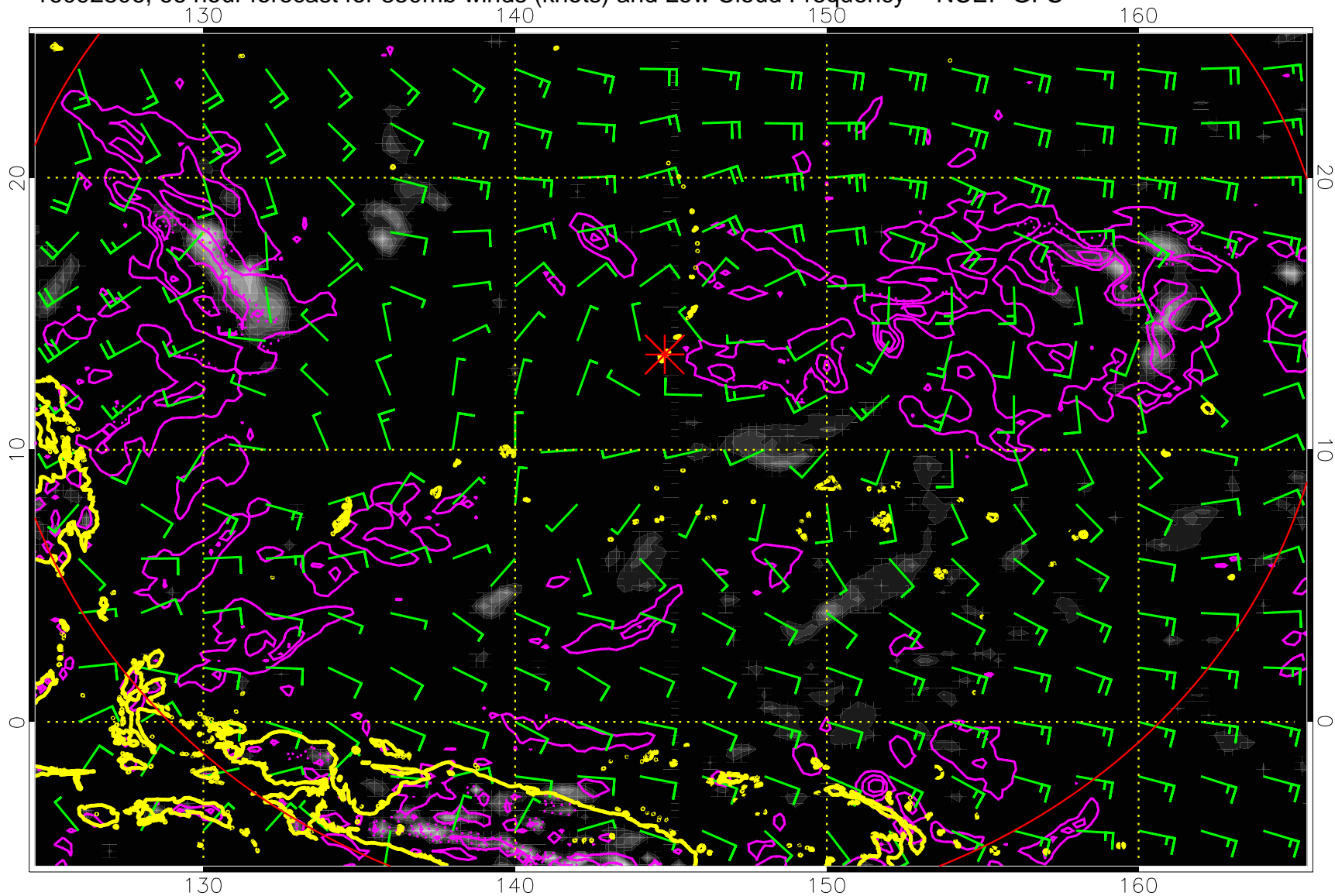
16092806, 66 hour forecast for 850mb winds (knots) and Low Cloud Frequency -- NCEP GFS
