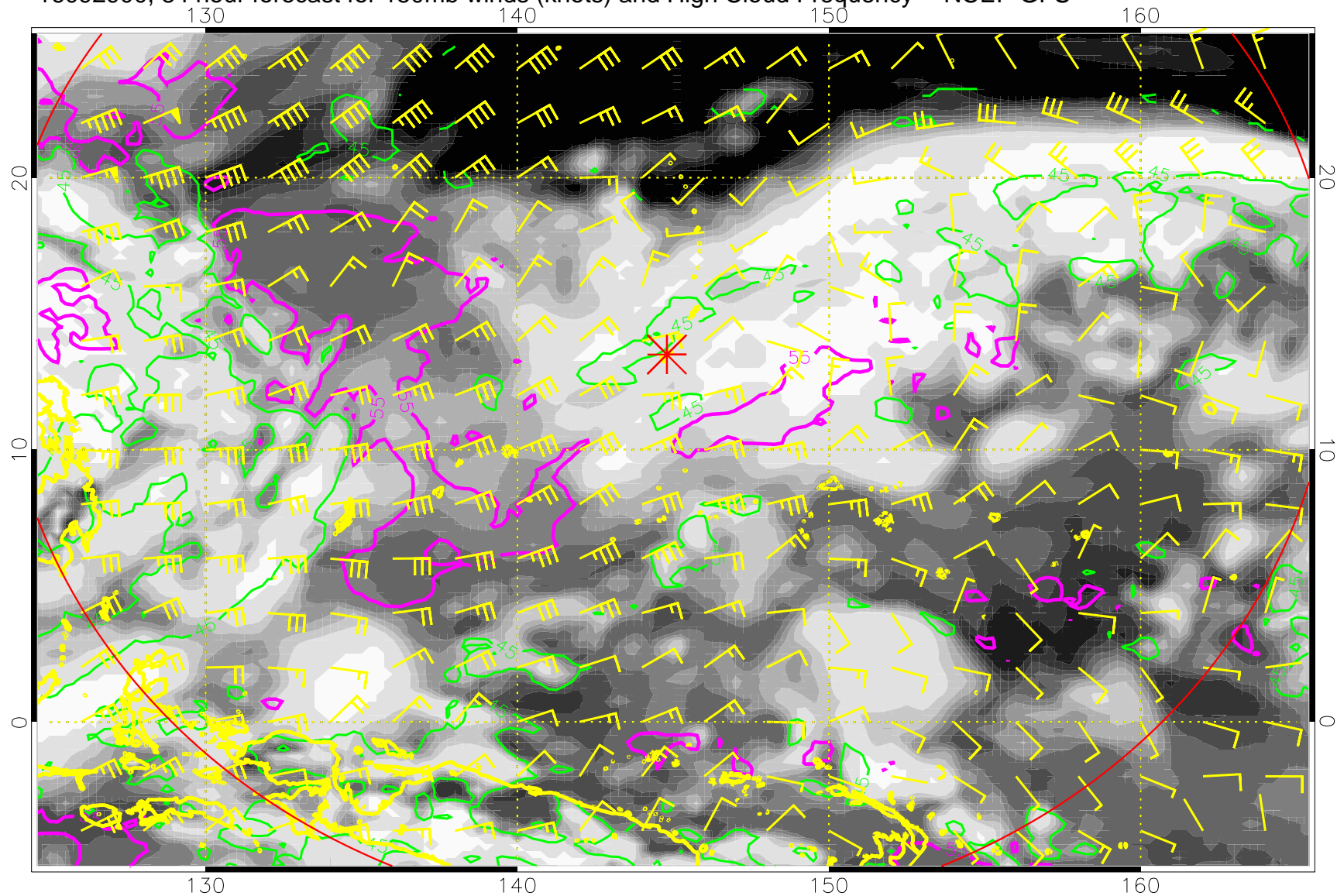
16092900, 84 hour forecast for 150mb winds (knots) and High Cloud Frequency -- NCEP GFS
