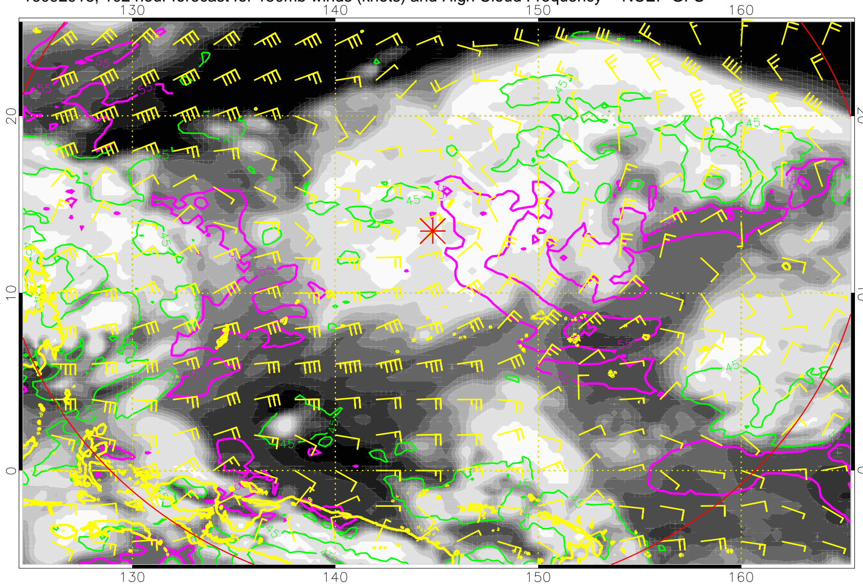
16092918, 102 hour forecast for 150mb winds (knots) and High Cloud Frequency -- NCEP GFS
