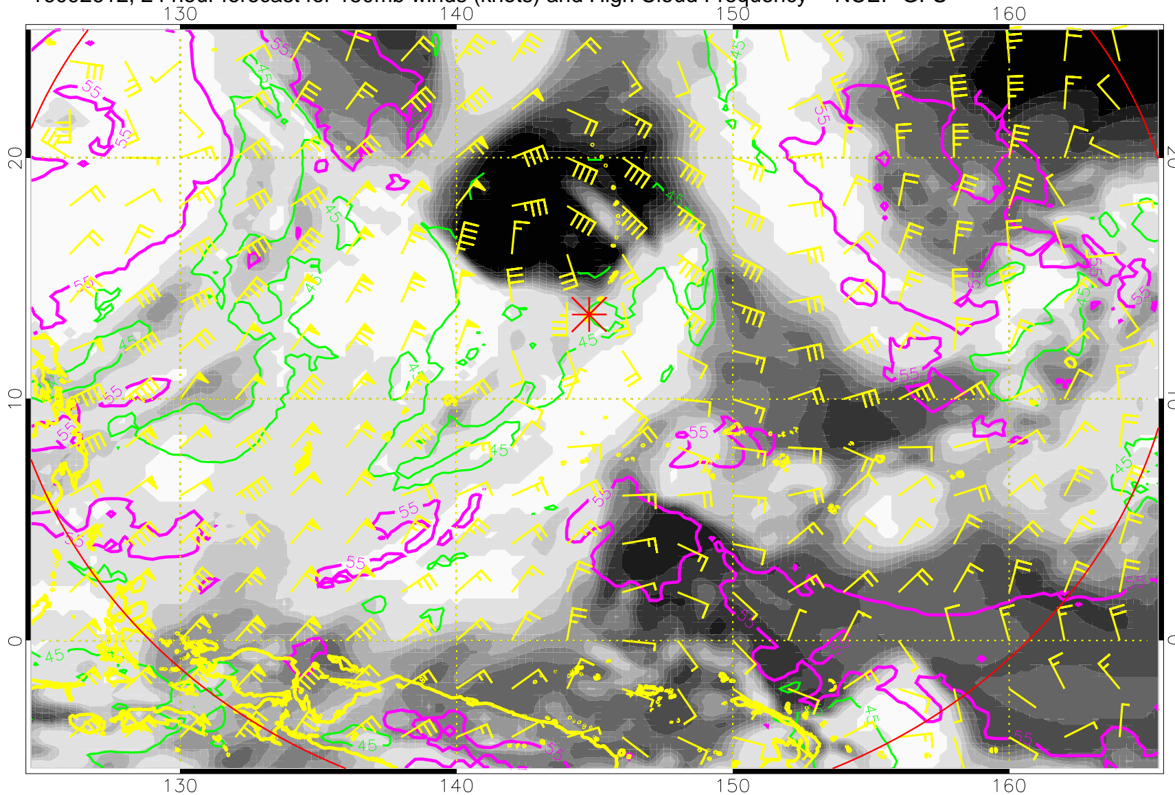
16092612, 24 hour forecast for 150mb winds (knots) and High Cloud Frequency -- NCEP GFS
