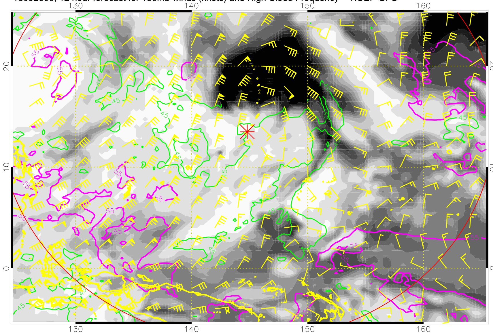
16092600, 12 hour forecast for 150mb winds (knots) and High Cloud Frequency -- NCEP GFS
