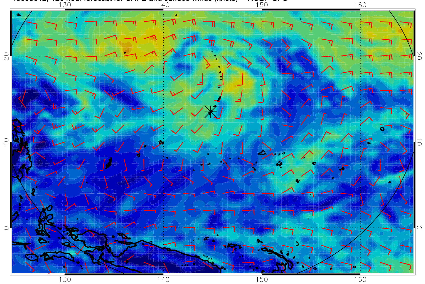
16093012, 120 hour forecast for CAPE and surface winds (knots) -- NCEP GFS
