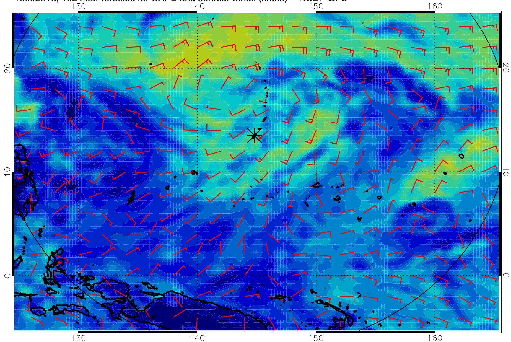
16092918, 102 hour forecast for CAPE and surface winds (knots) -- NCEP GFS
