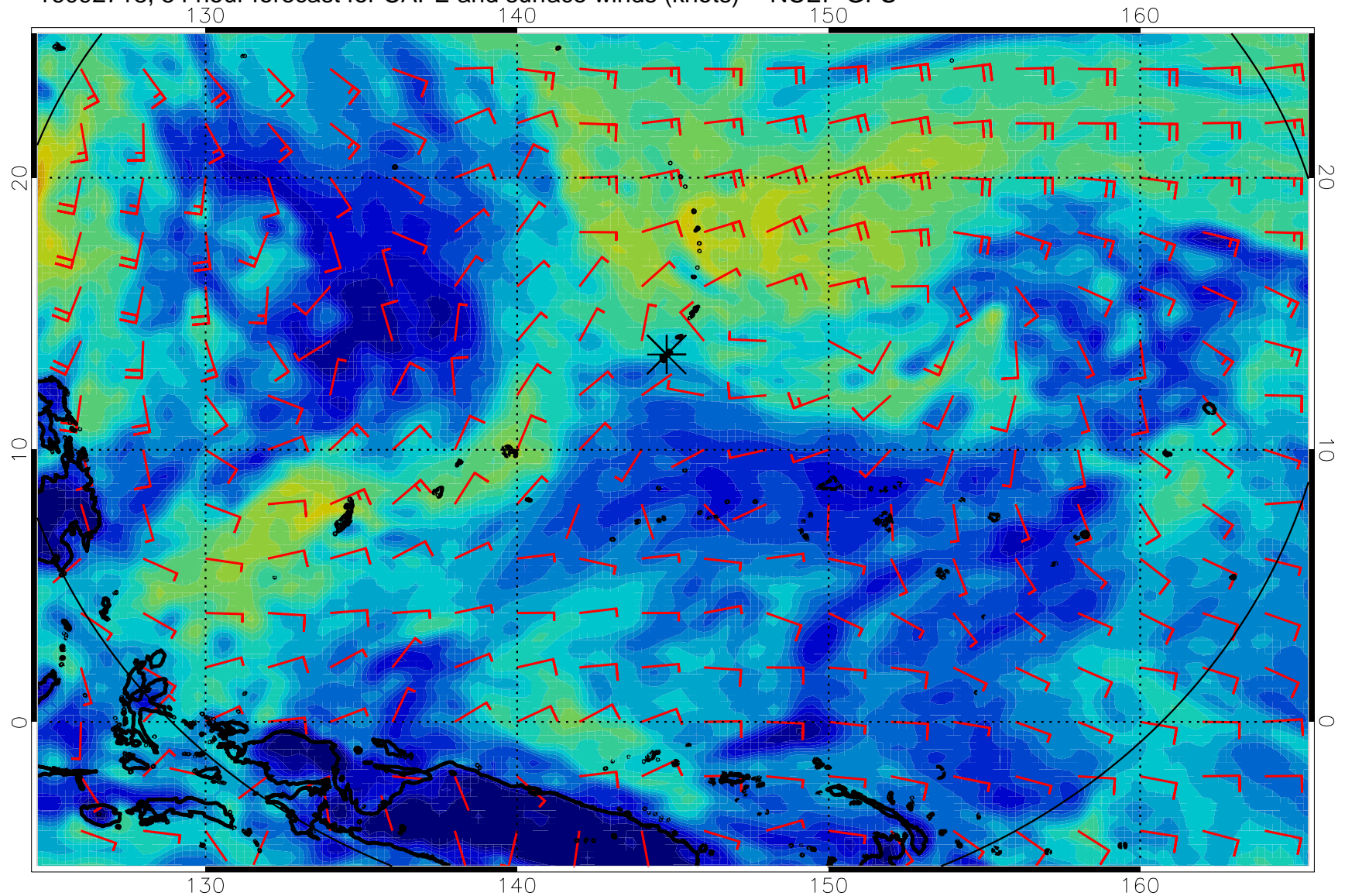
16092718, 54 hour forecast for CAPE and surface winds (knots) -- NCEP GFS
