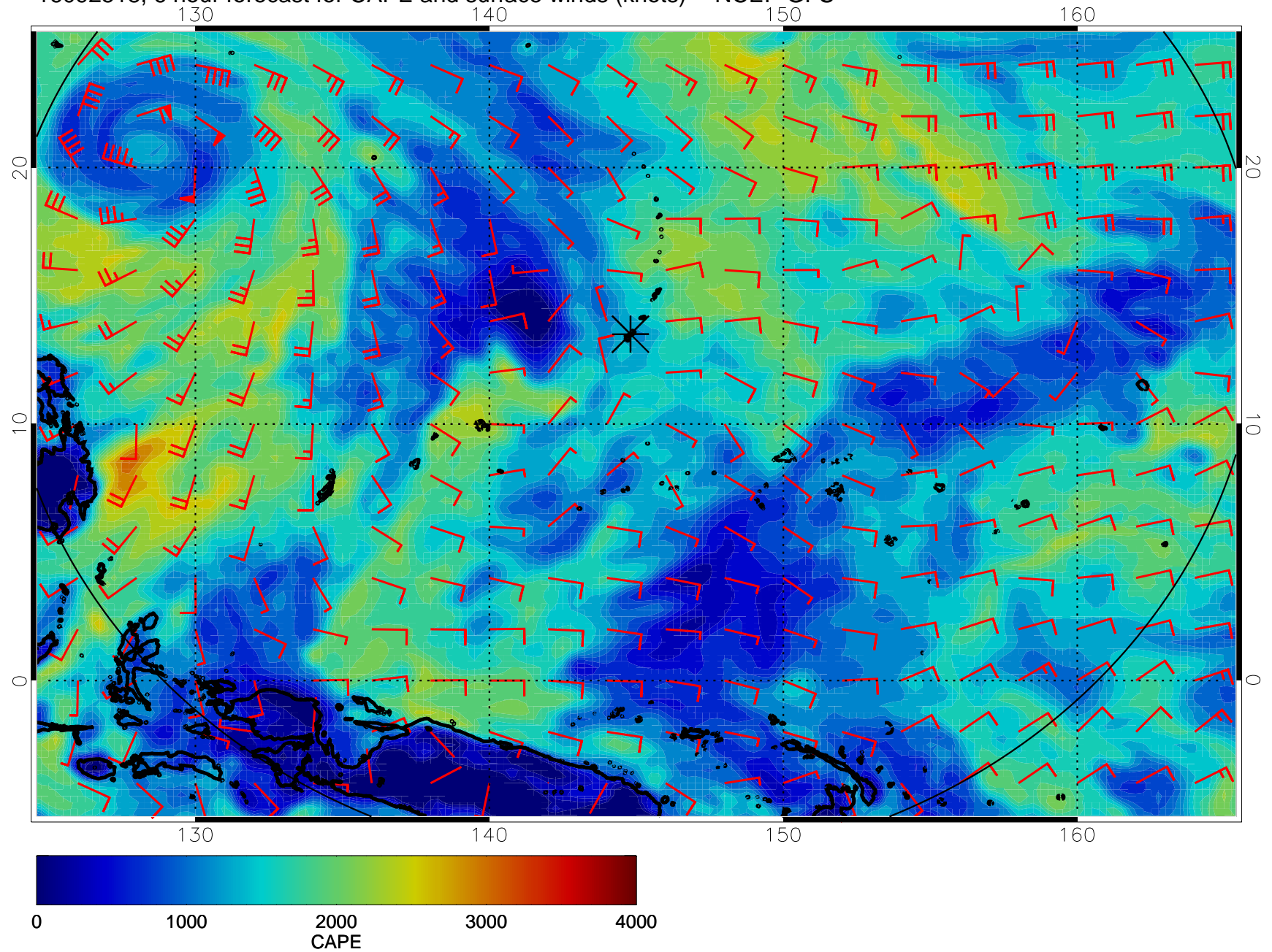
16092518, 6 hour forecast for CAPE and surface winds (knots) -- NCEP GFS
