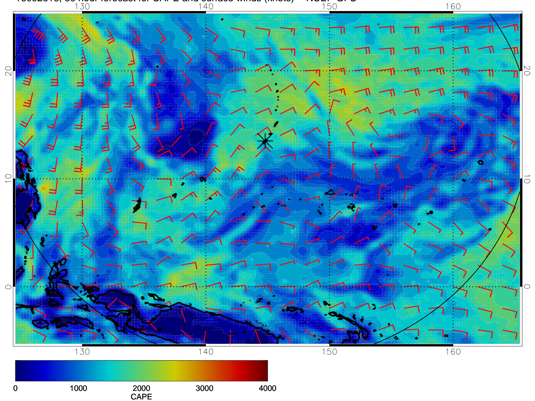
16092618, 30 hour forecast for CAPE and surface winds (knots) -- NCEP GFS
