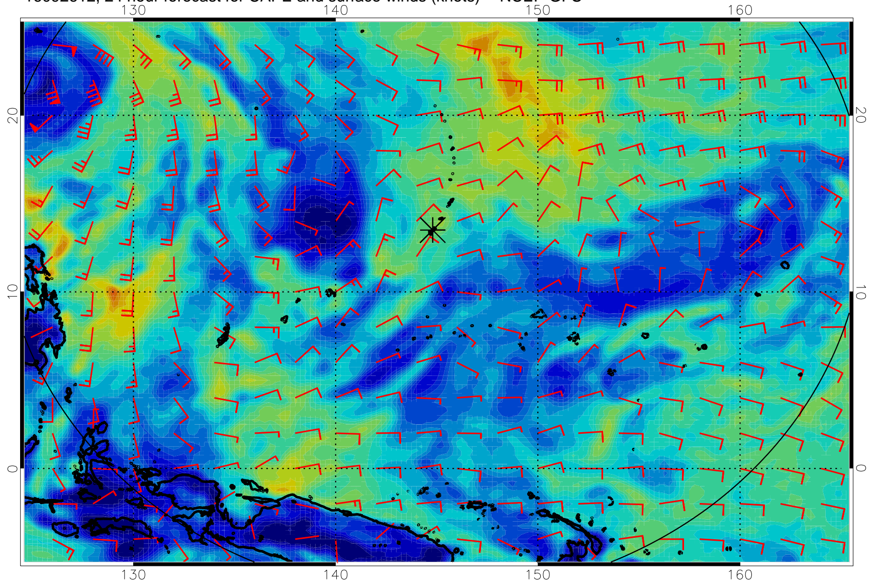
16092612, 24 hour forecast for CAPE and surface winds (knots) -- NCEP GFS
