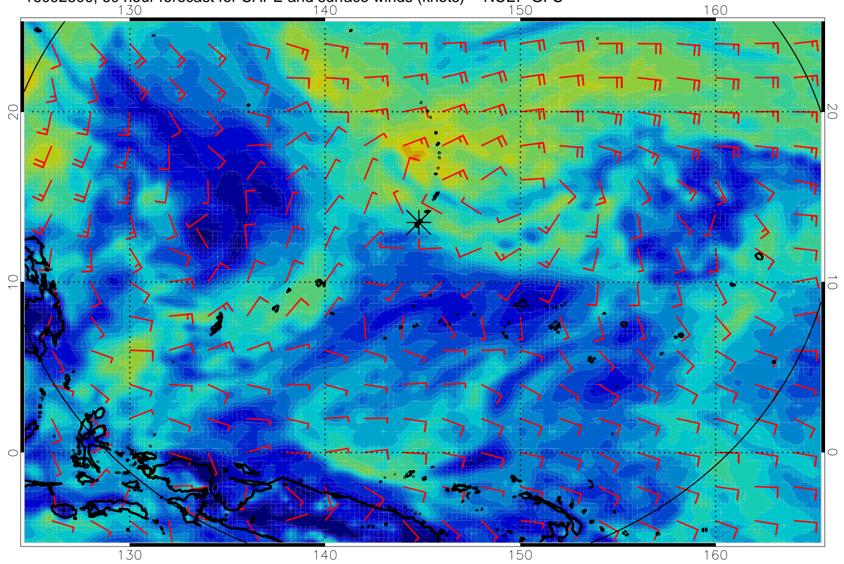
16092800, 60 hour forecast for CAPE and surface winds (knots) -- NCEP GFS
