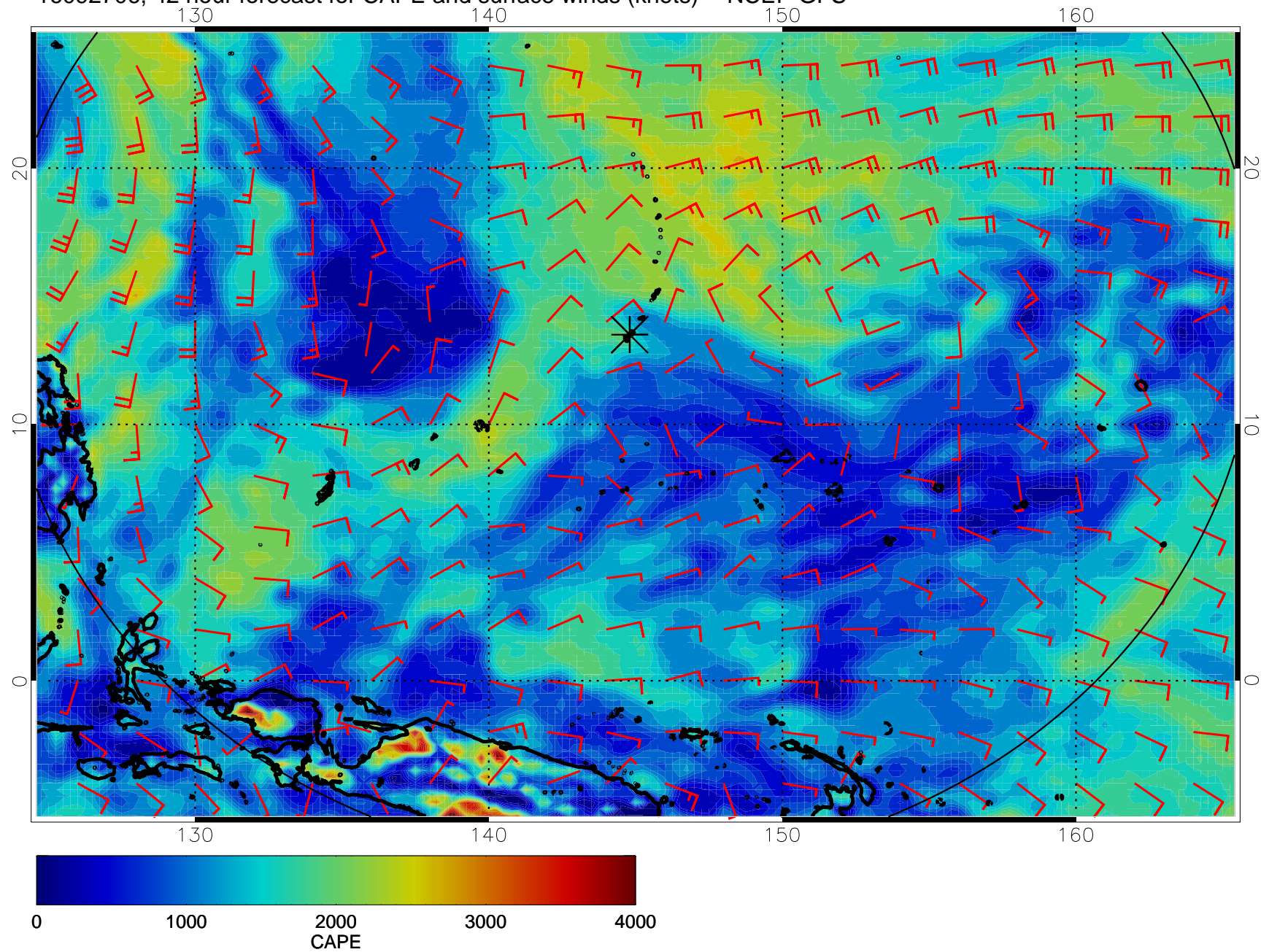
16092706, 42 hour forecast for CAPE and surface winds (knots) -- NCEP GFS
