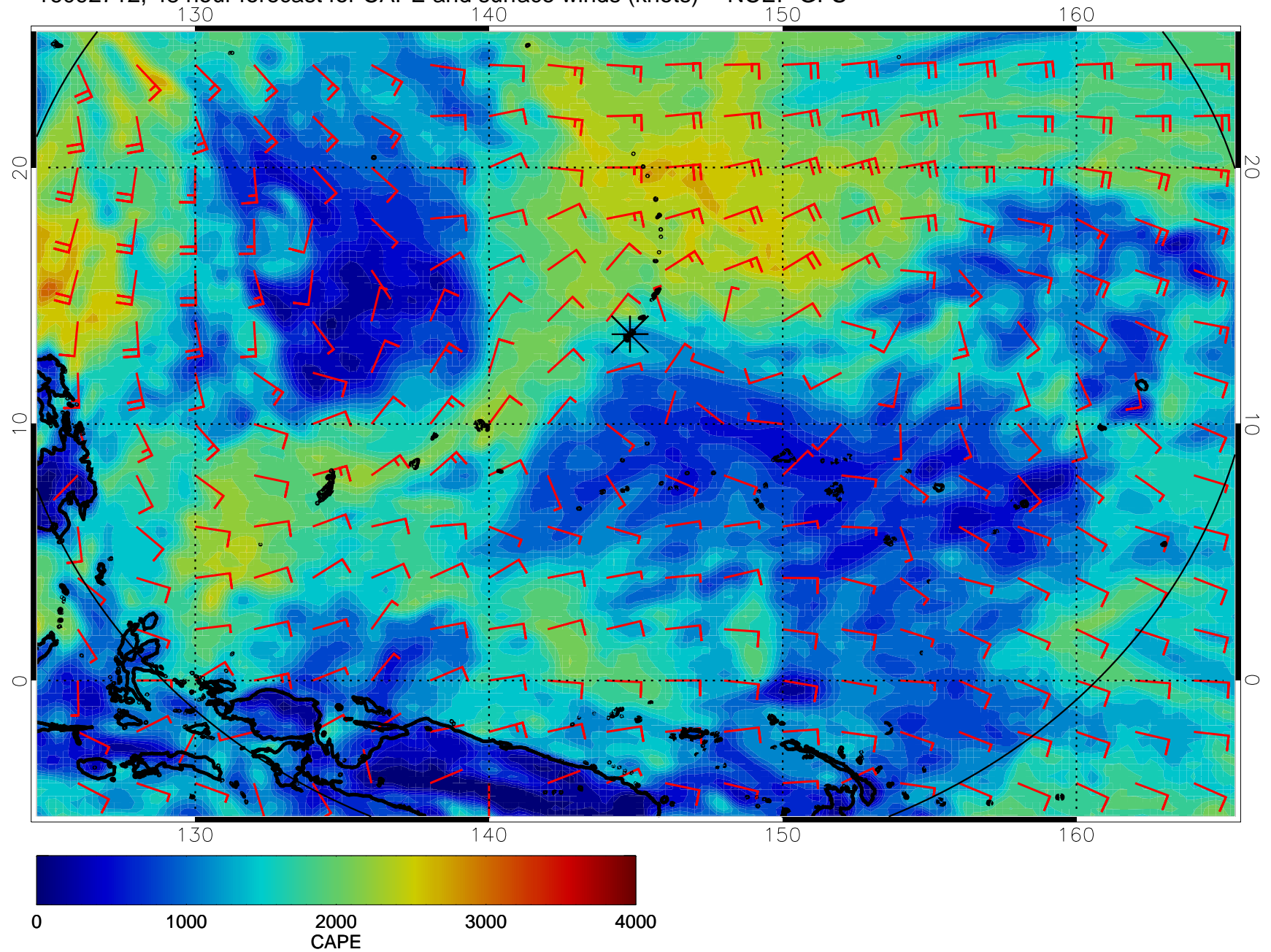
16092712, 48 hour forecast for CAPE and surface winds (knots) -- NCEP GFS
