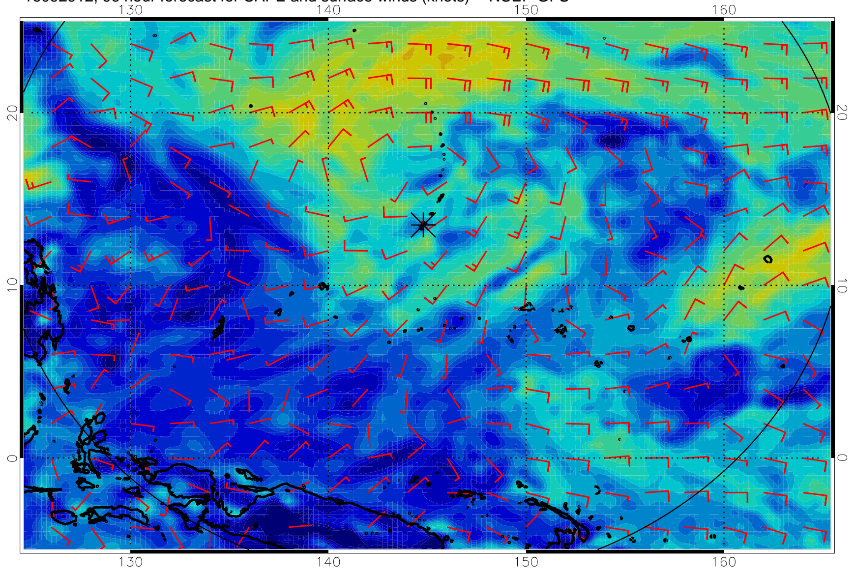
16092912, 96 hour forecast for CAPE and surface winds (knots) -- NCEP GFS
