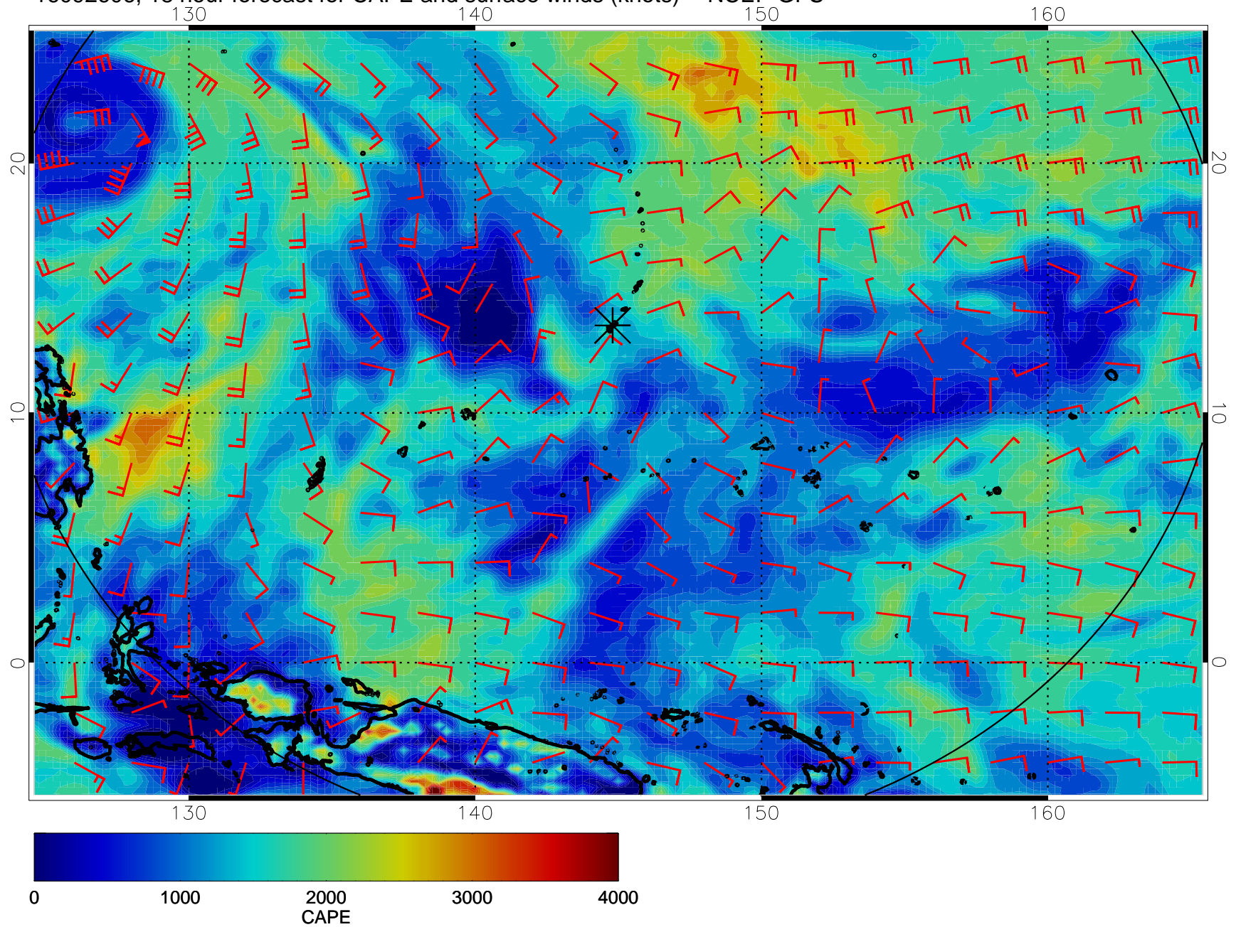
16092606, 18 hour forecast for CAPE and surface winds (knots) -- NCEP GFS
