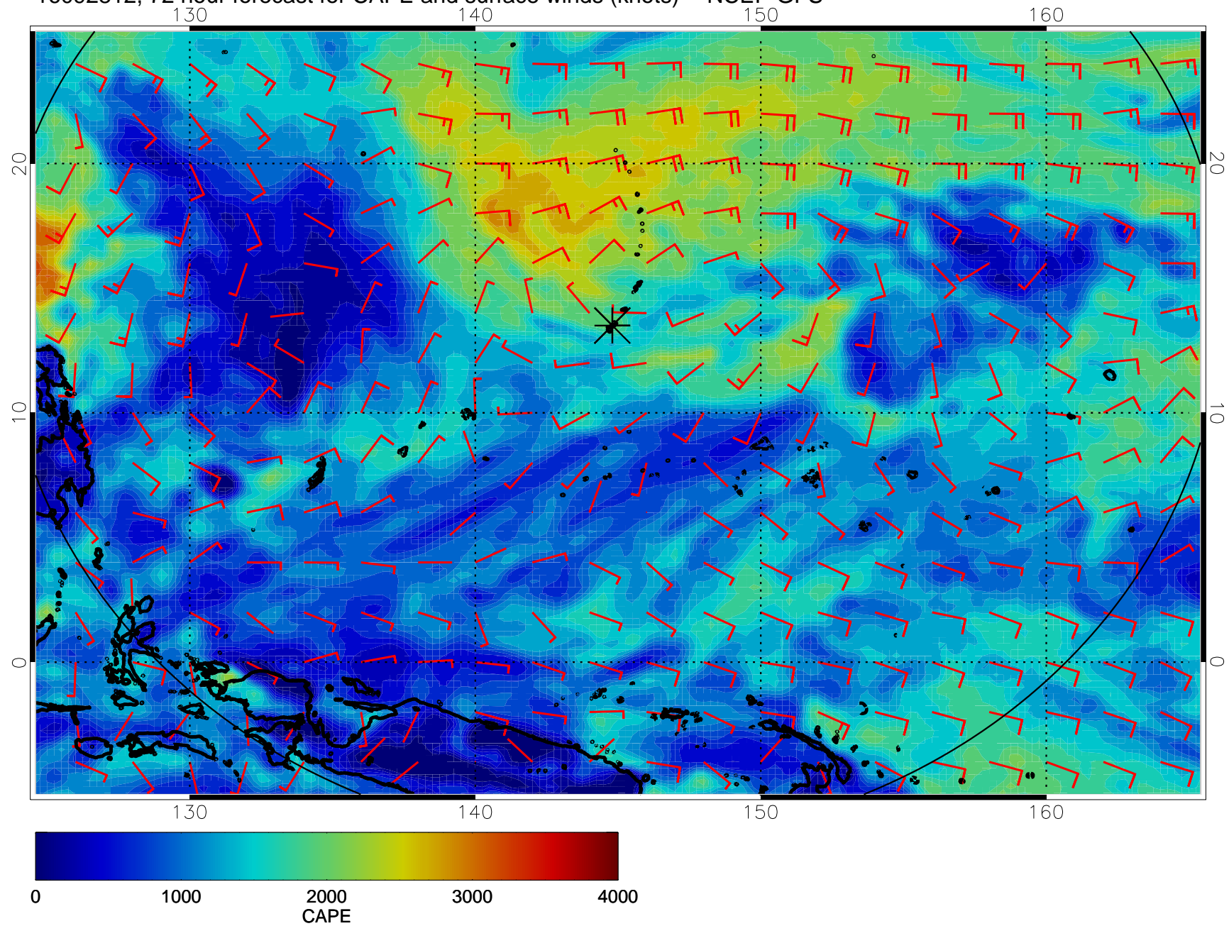
16092812, 72 hour forecast for CAPE and surface winds (knots) -- NCEP GFS
