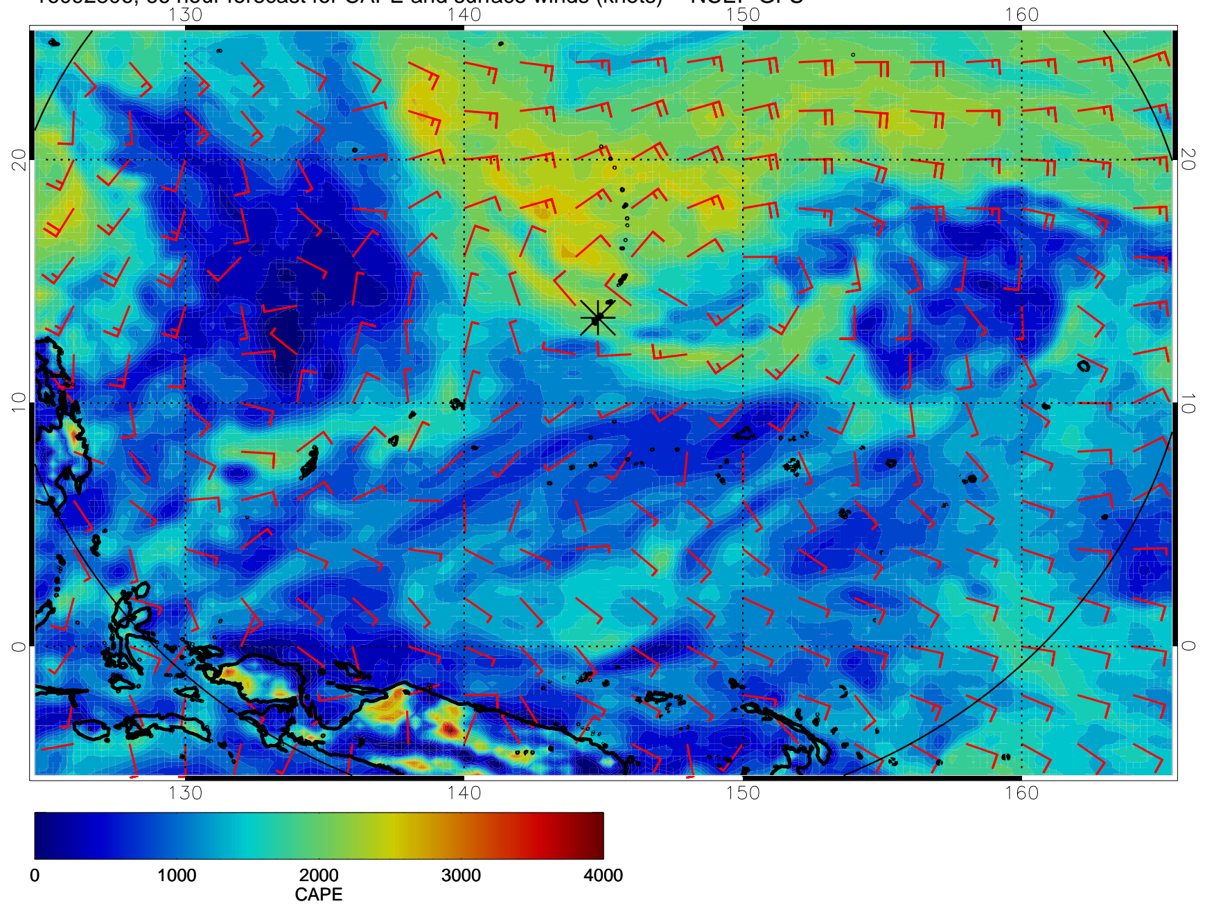
16092806, 66 hour forecast for CAPE and surface winds (knots) -- NCEP GFS
