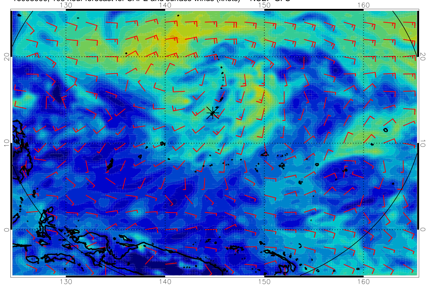
16093000, 108 hour forecast for CAPE and surface winds (knots) -- NCEP GFS
