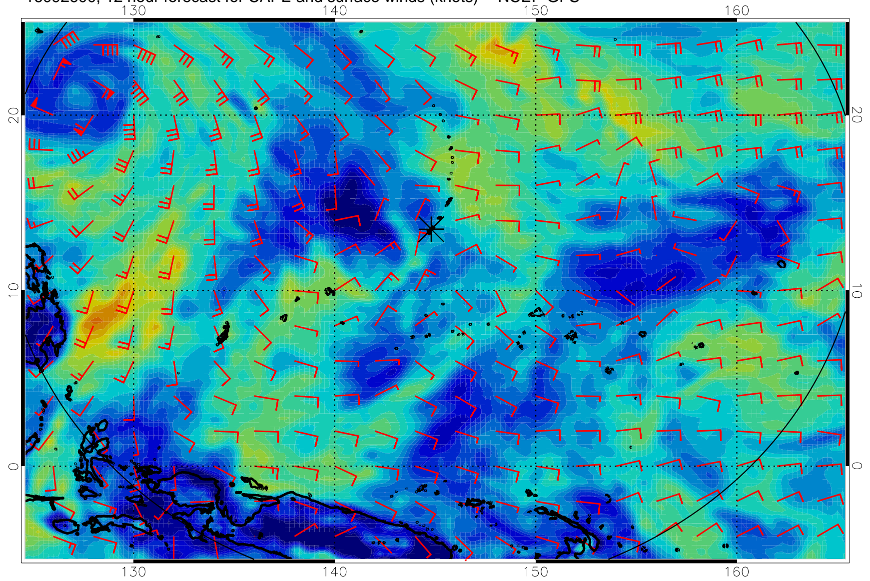
16092600, 12 hour forecast for CAPE and surface winds (knots) -- NCEP GFS
