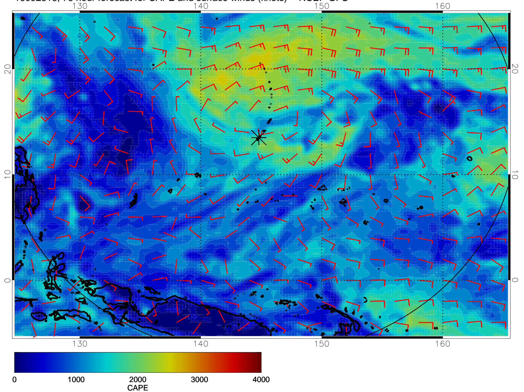
16092818, 78 hour forecast for CAPE and surface winds (knots) -- NCEP GFS
