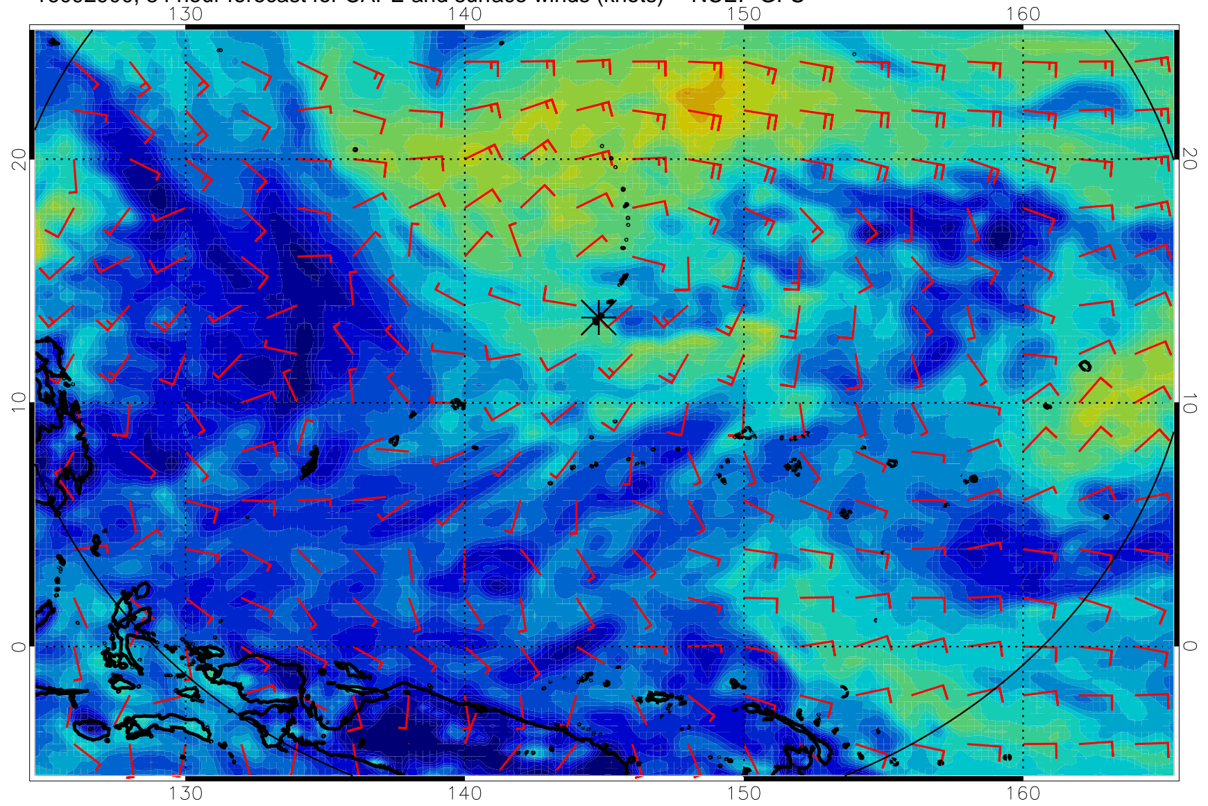
16092900, 84 hour forecast for CAPE and surface winds (knots) -- NCEP GFS
