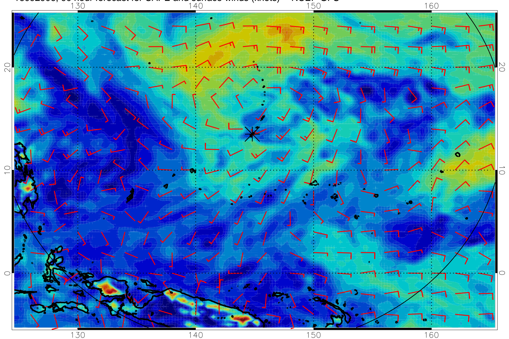
16092906, 90 hour forecast for CAPE and surface winds (knots) -- NCEP GFS
