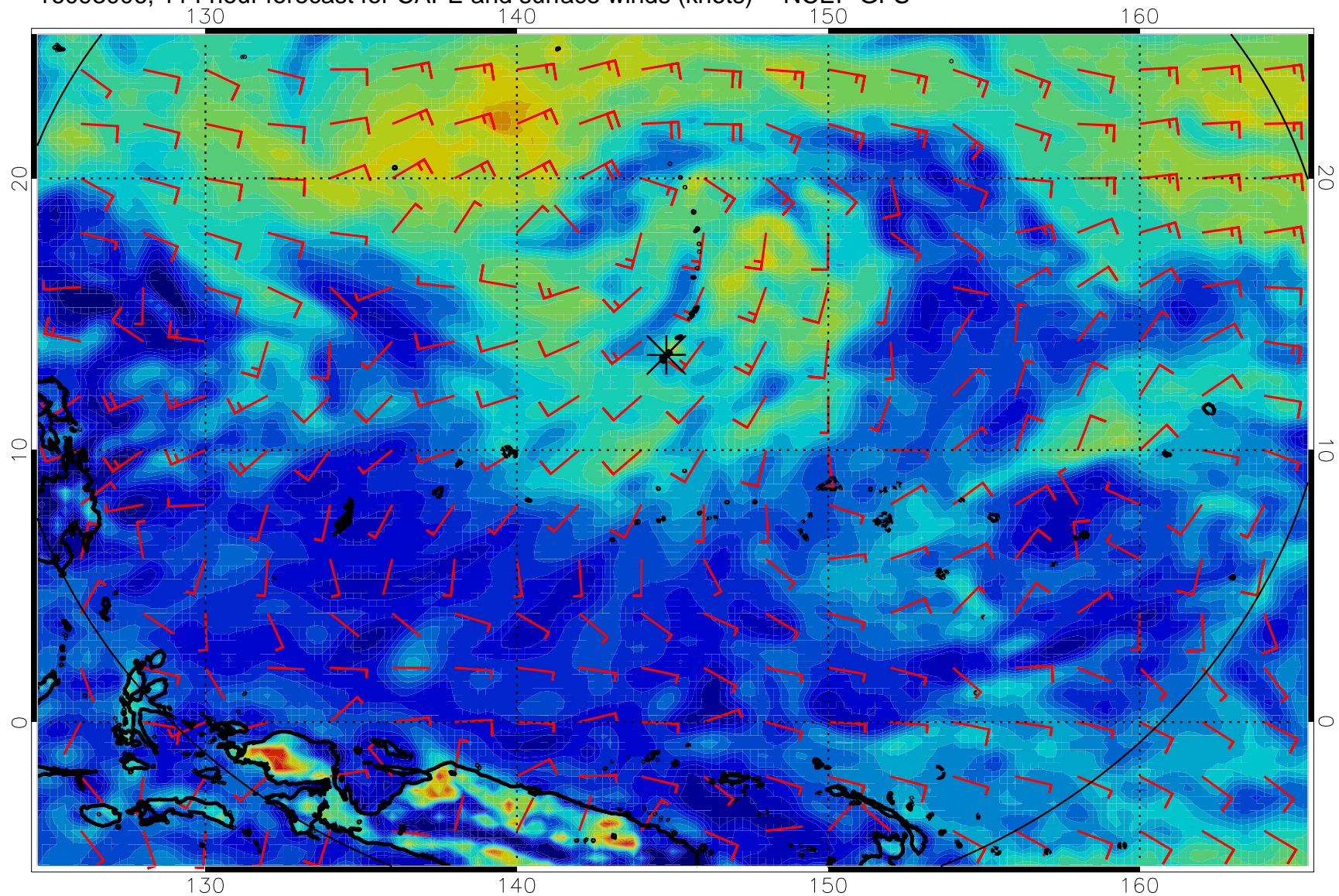
16093006, 114 hour forecast for CAPE and surface winds (knots) -- NCEP GFS
