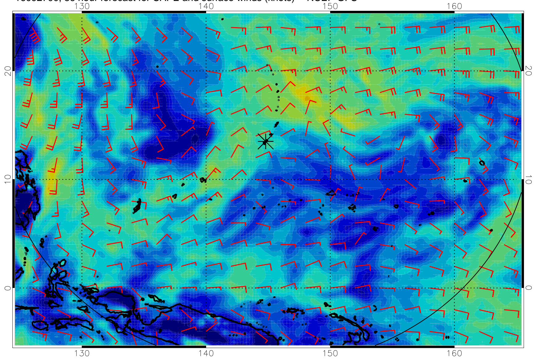
16092700, 36 hour forecast for CAPE and surface winds (knots) -- NCEP GFS
