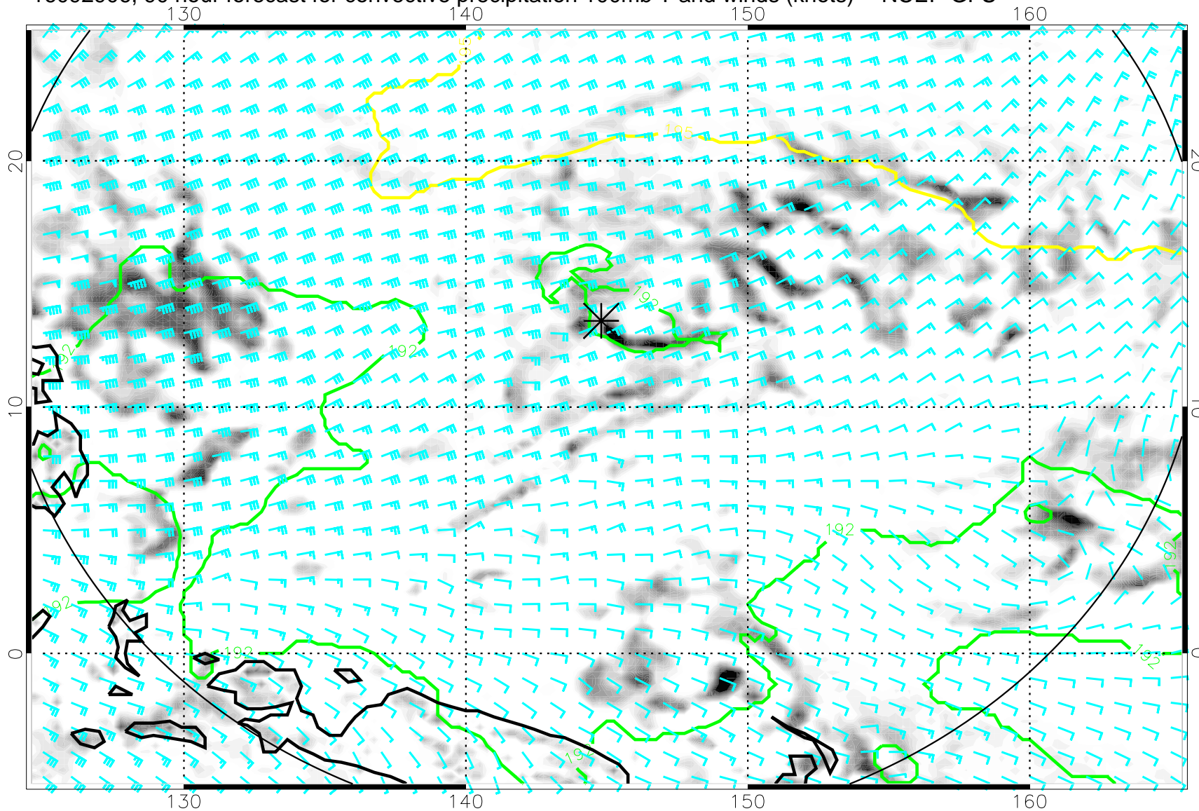
16092906, 90 hour forecast for convective precipitation 100mb T and winds (knots) -- NCEP GFS
