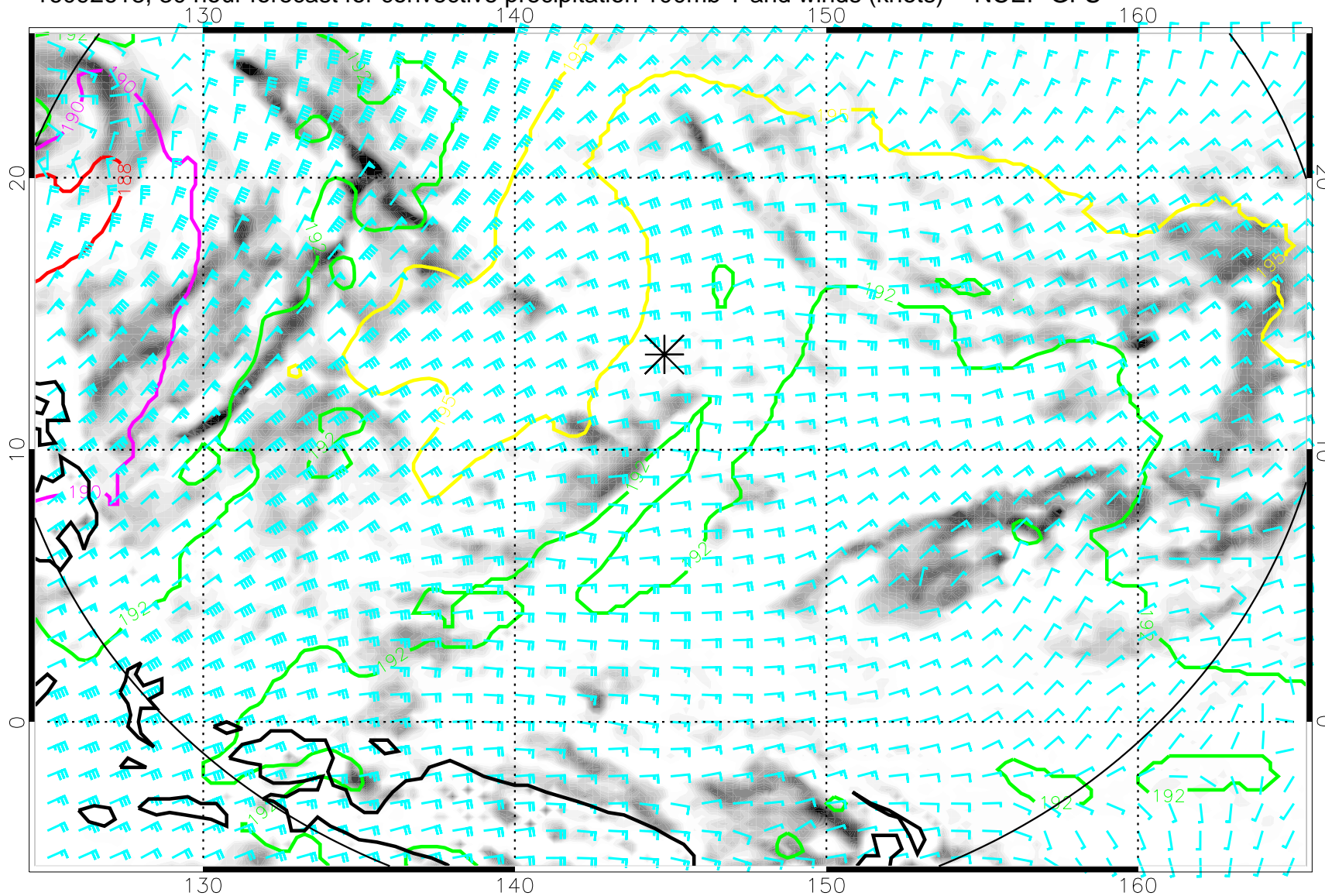
16092618, 30 hour forecast for convective precipitation 100mb T and winds (knots) -- NCEP GFS
