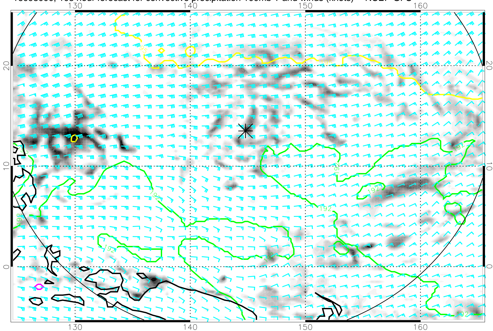
16093000, 108 hour forecast for convective precipitation 100mb T and winds (knots) -- NCEP GFS
