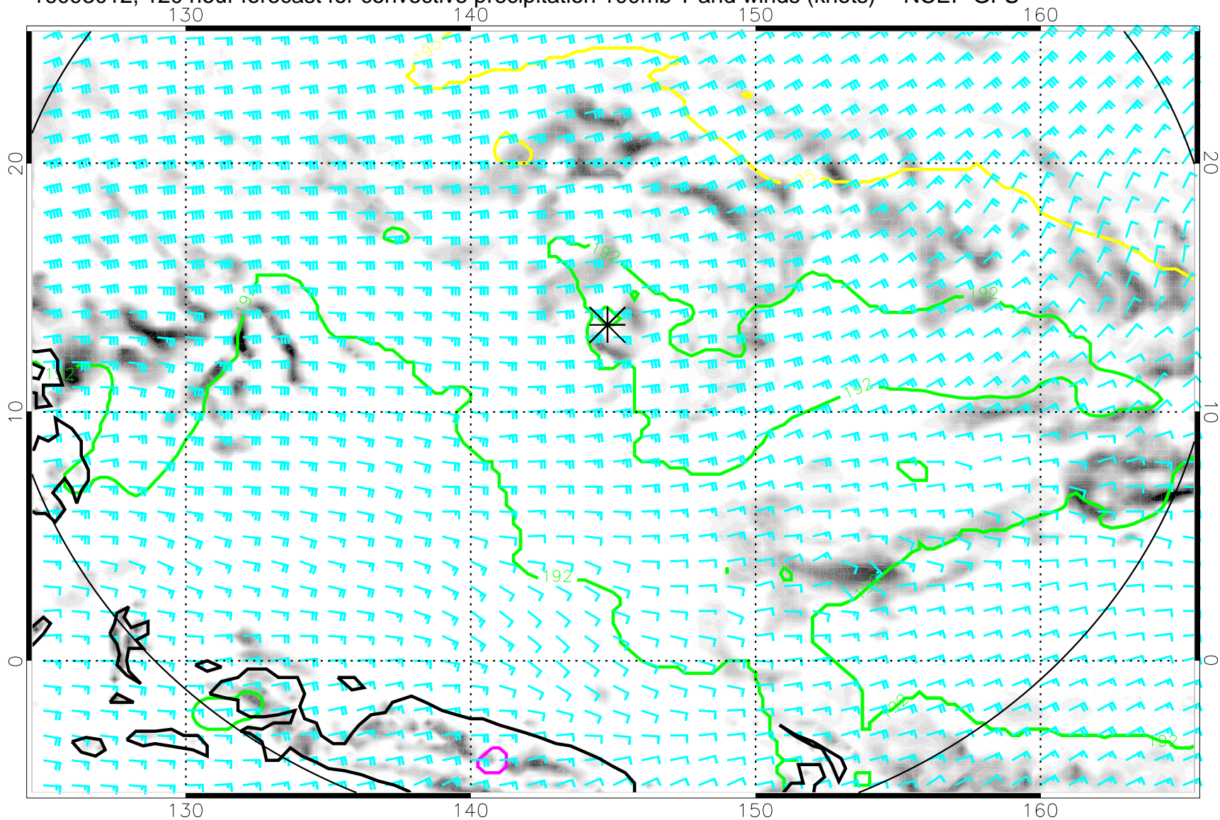
16093012, 120 hour forecast for convective precipitation 100mb T and winds (knots) -- NCEP GFS
