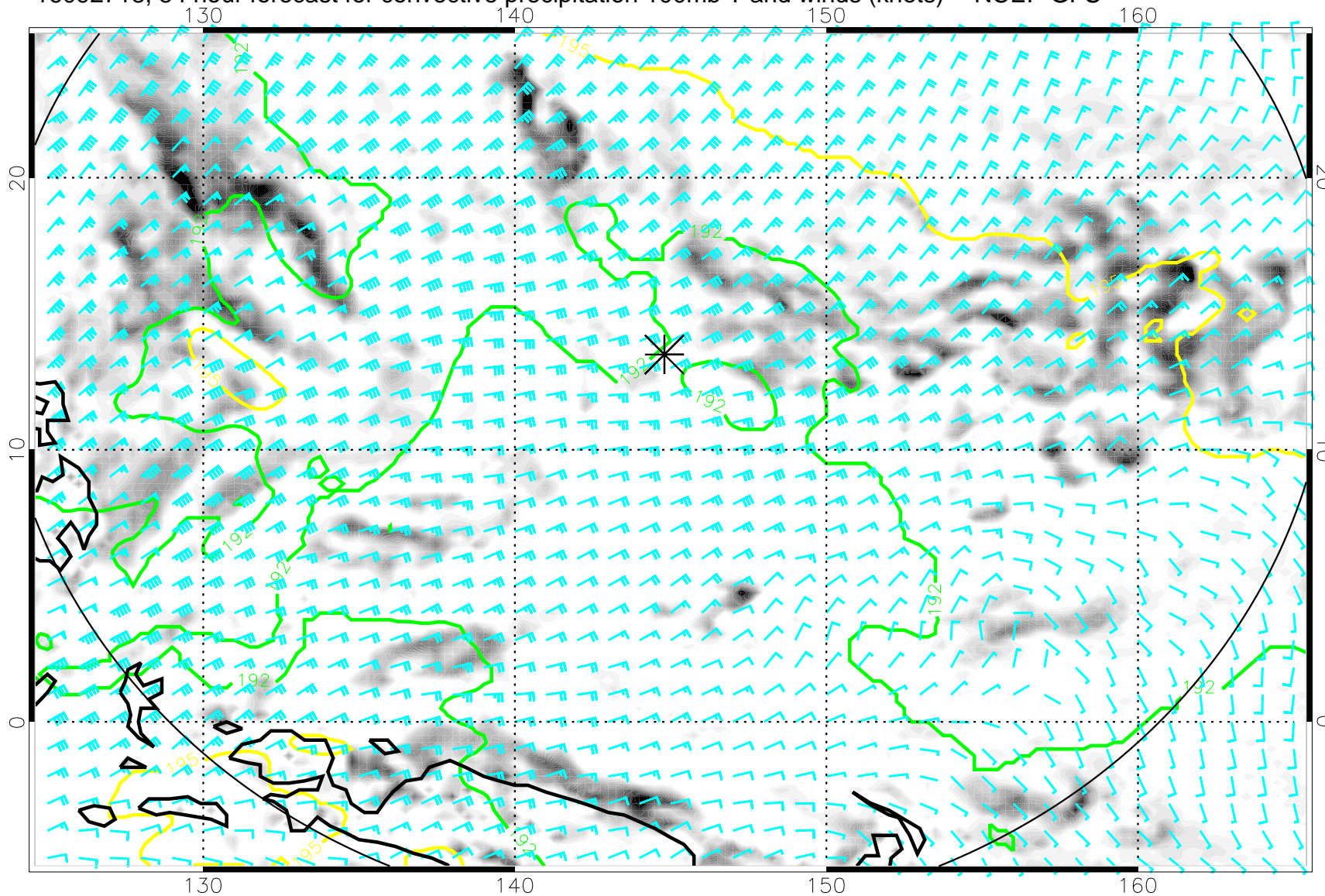
16092718, 54 hour forecast for convective precipitation 100mb T and winds (knots) -- NCEP GFS
