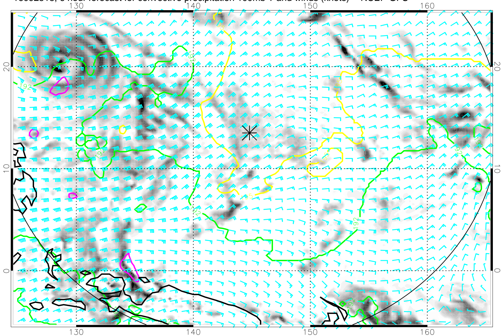
16092518, 6 hour forecast for convective precipitation 100mb T and winds (knots) -- NCEP GFS
