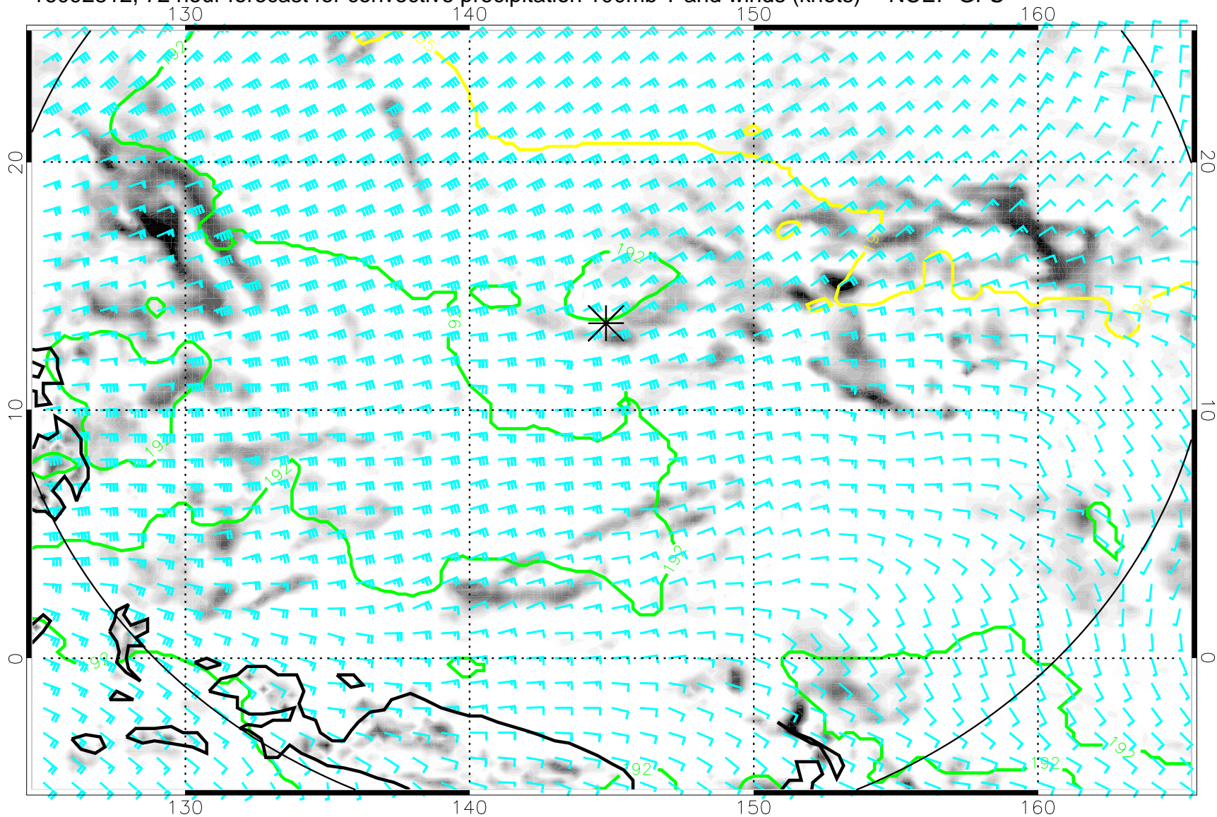
16092812, 72 hour forecast for convective precipitation 100mb T and winds (knots) -- NCEP GFS
