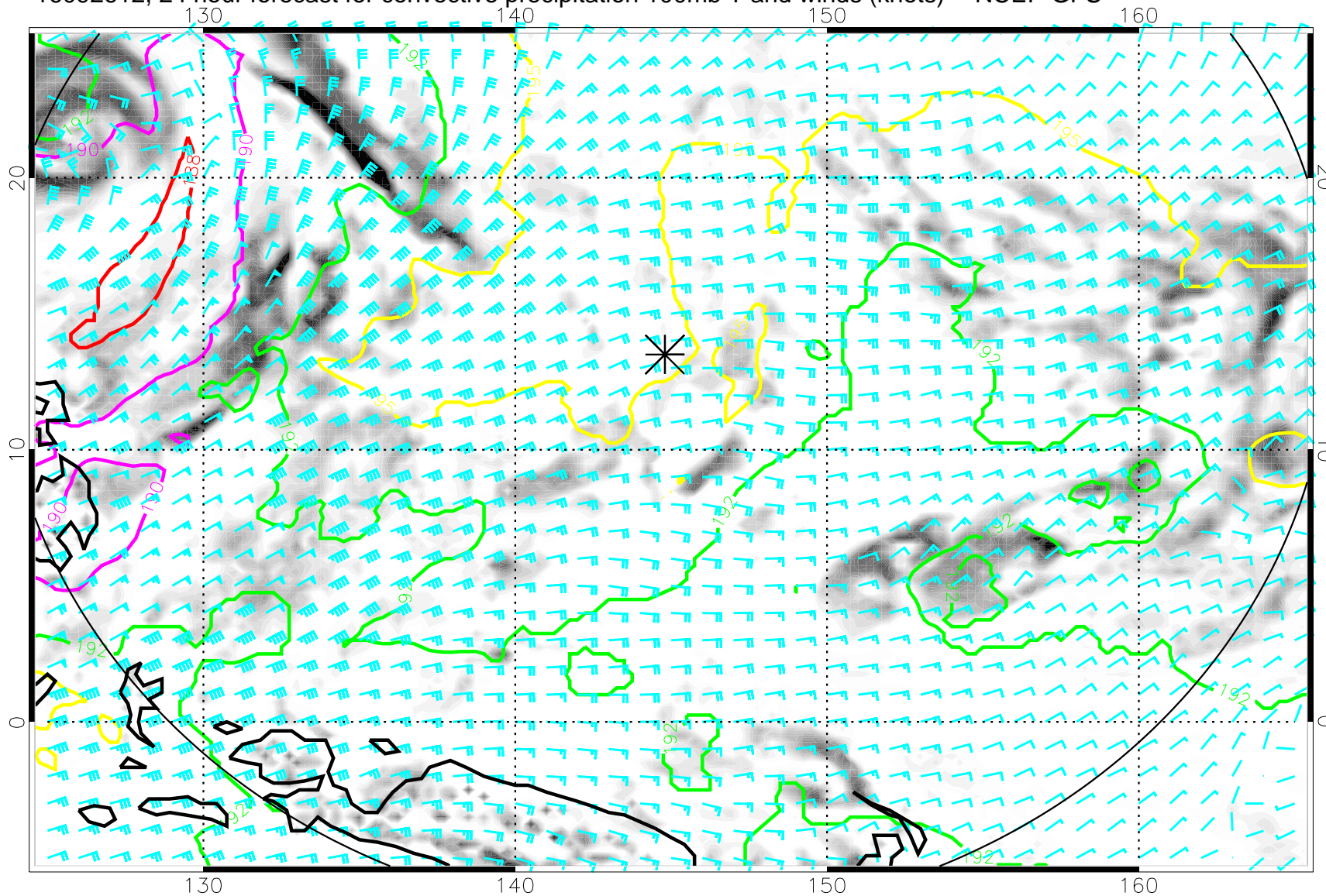
16092612, 24 hour forecast for convective precipitation 100mb T and winds (knots) -- NCEP GFS
