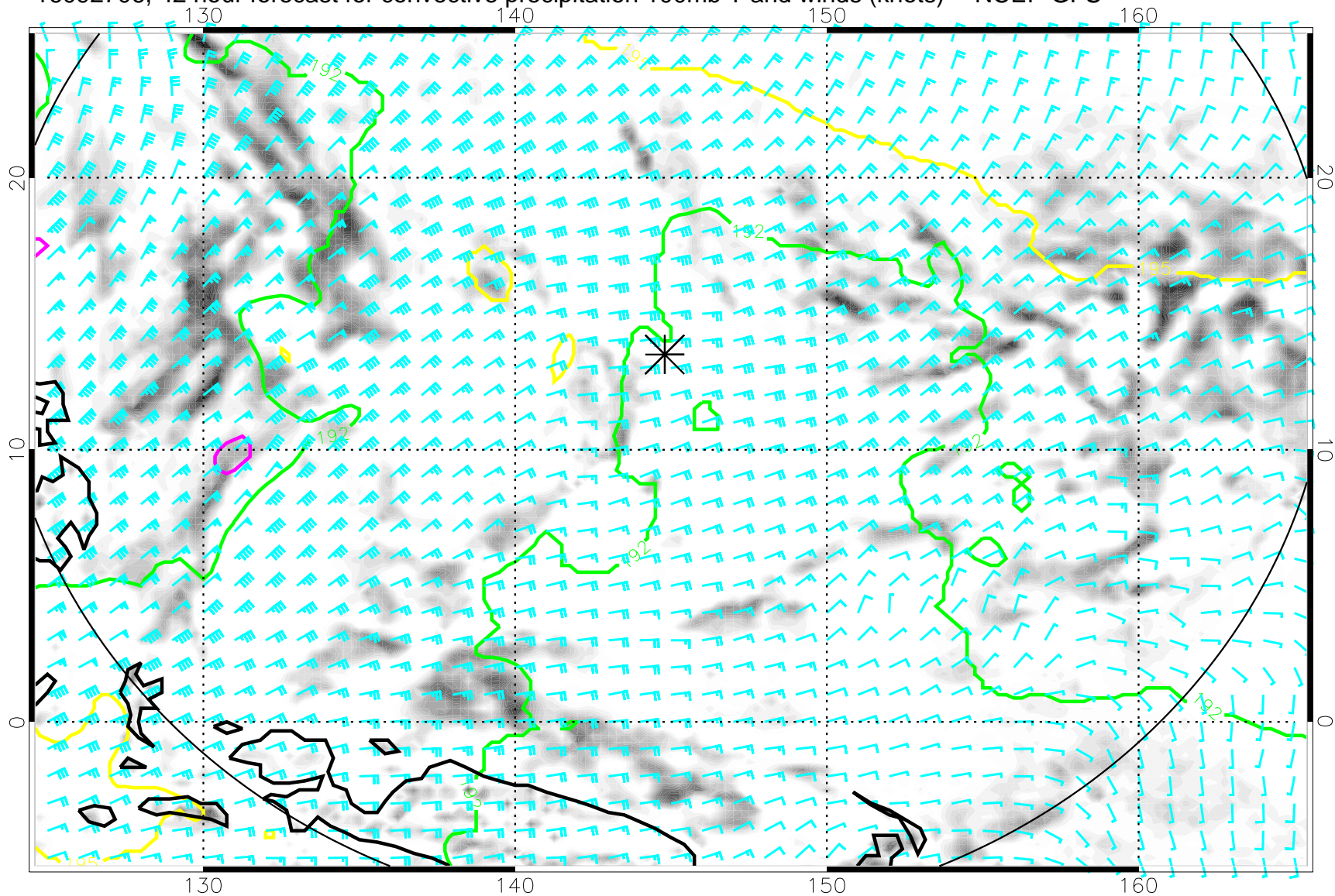
16092706, 42 hour forecast for convective precipitation 100mb T and winds (knots) -- NCEP GFS
