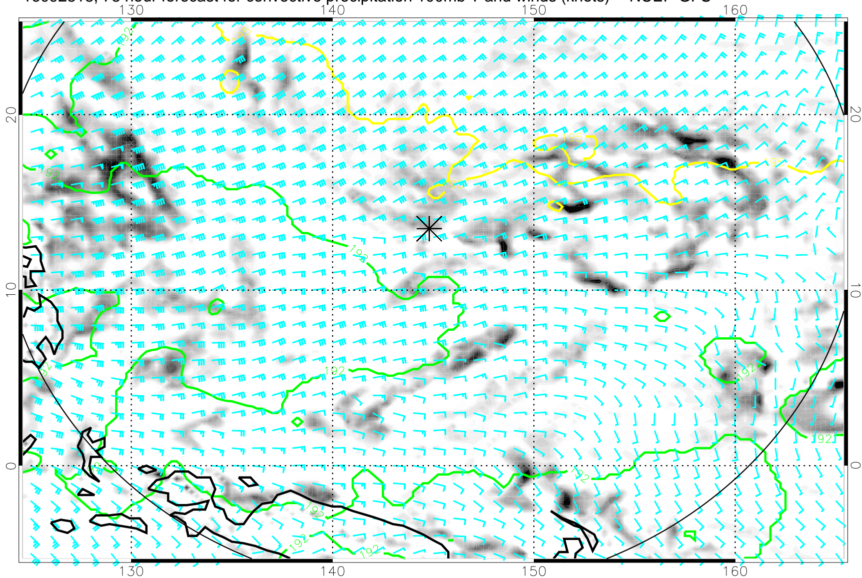
16092818, 78 hour forecast for convective precipitation 100mb T and winds (knots) -- NCEP GFS
