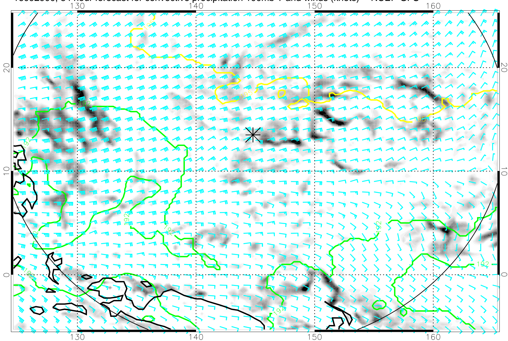
16092900, 84 hour forecast for convective precipitation 100mb T and winds (knots) -- NCEP GFS
