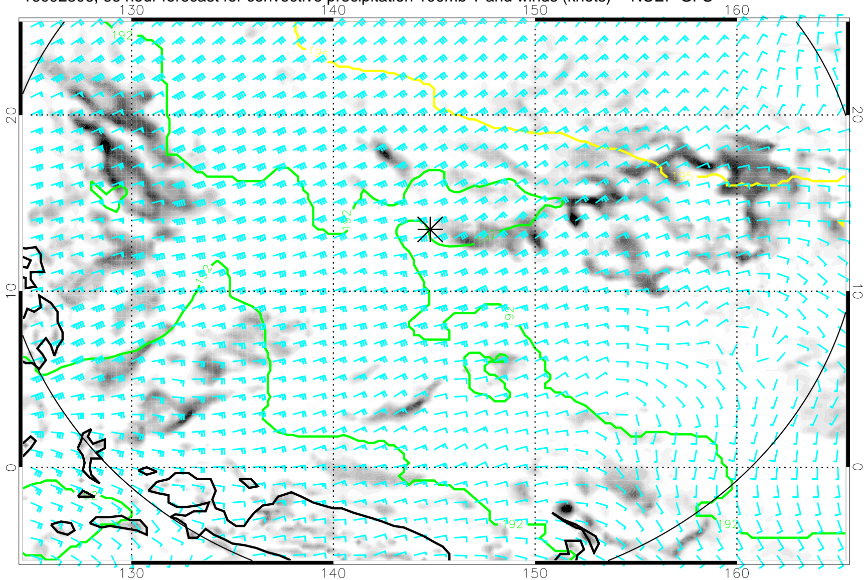
16092806, 66 hour forecast for convective precipitation 100mb T and winds (knots) -- NCEP GFS
