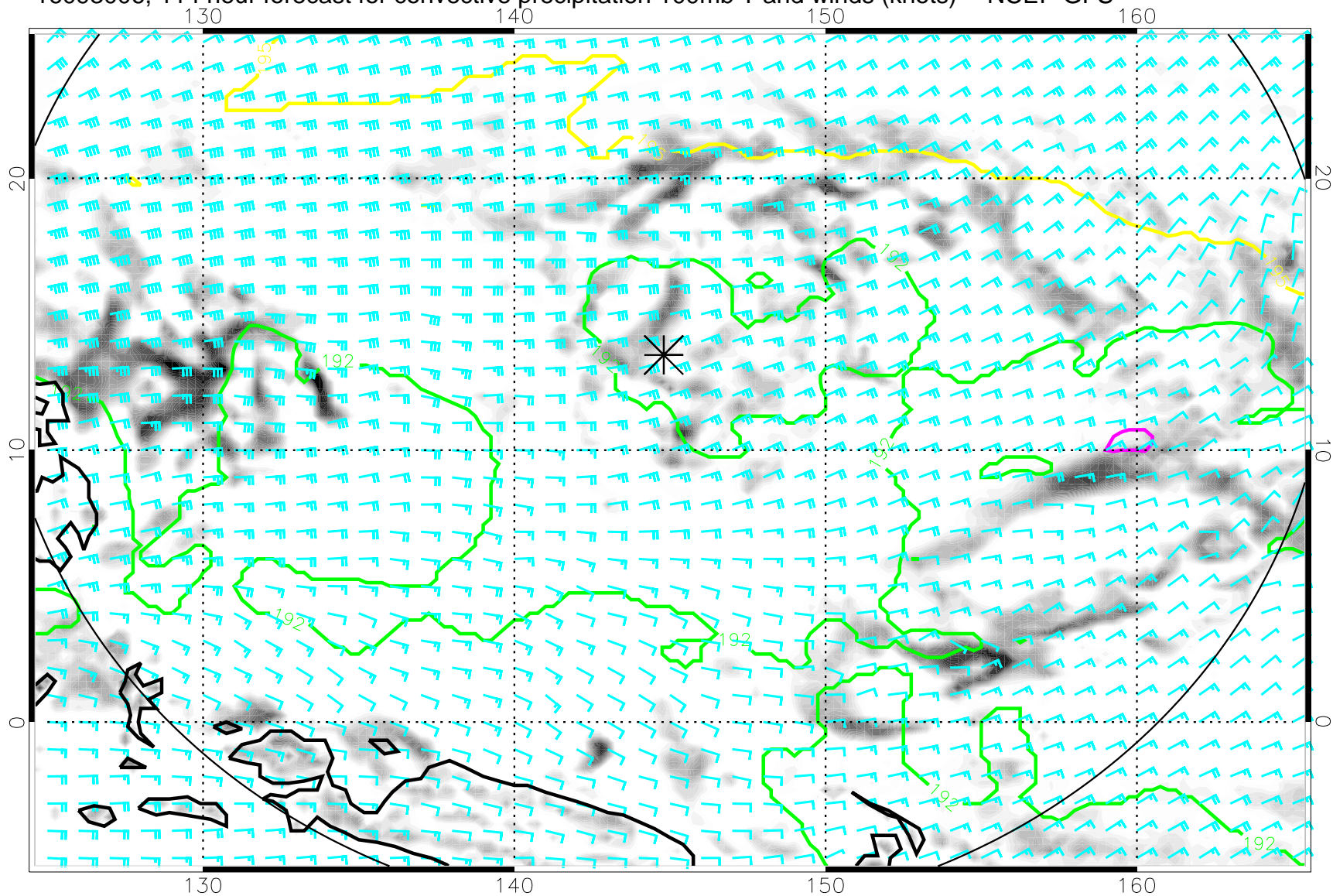
16093006, 114 hour forecast for convective precipitation 100mb T and winds (knots) -- NCEP GFS
