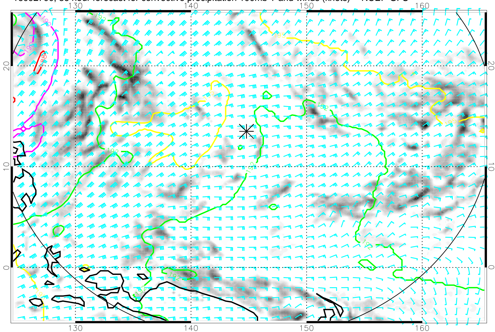
16092700, 36 hour forecast for convective precipitation 100mb T and winds (knots) -- NCEP GFS
