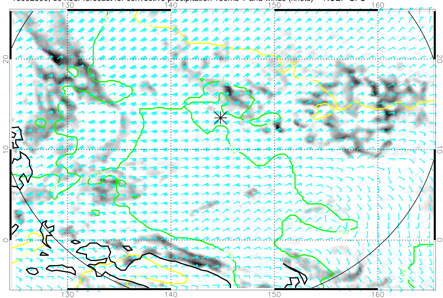
16092800, 60 hour forecast for convective precipitation 100mb T and winds (knots) -- NCEP GFS
