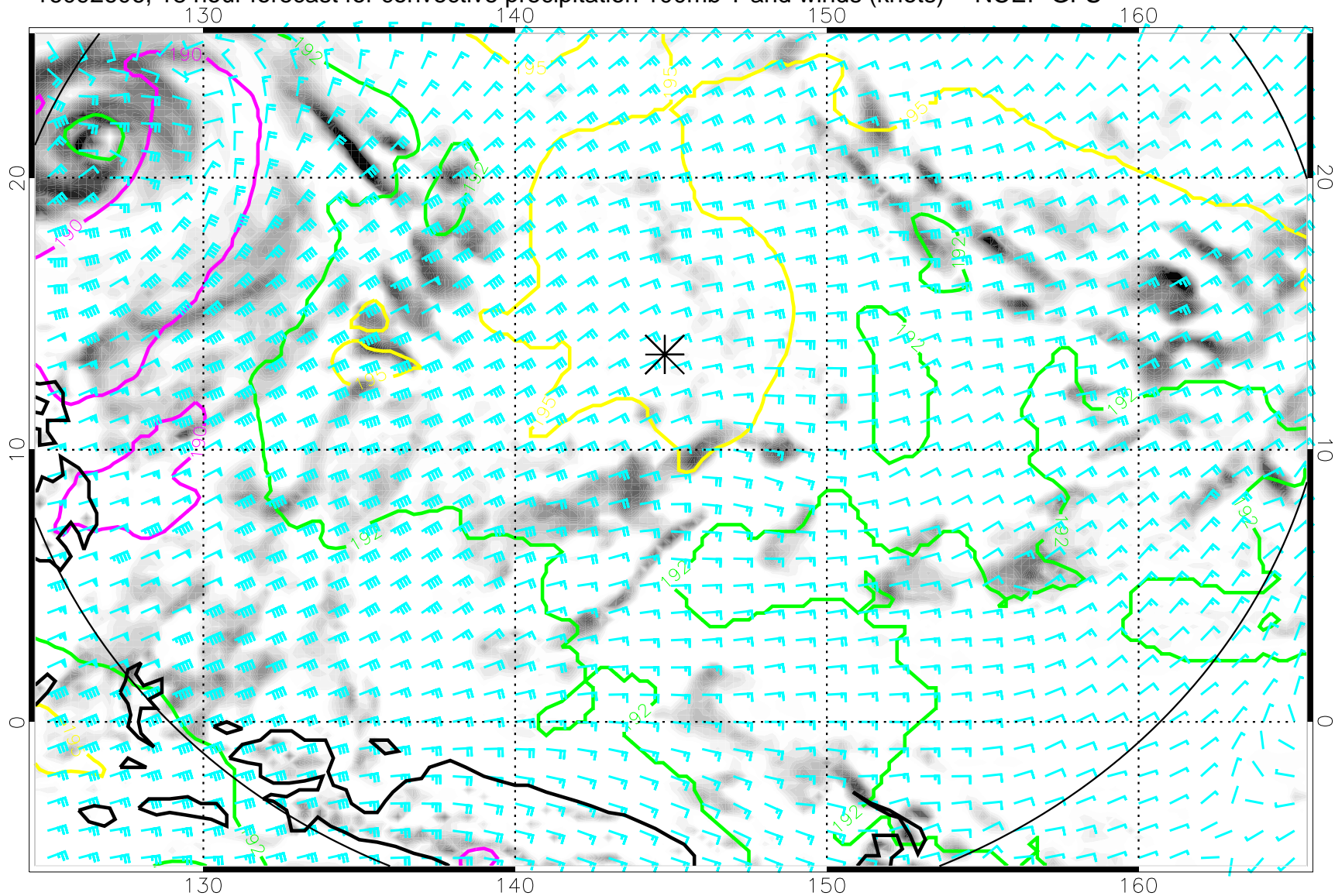
16092606, 18 hour forecast for convective precipitation 100mb T and winds (knots) -- NCEP GFS
