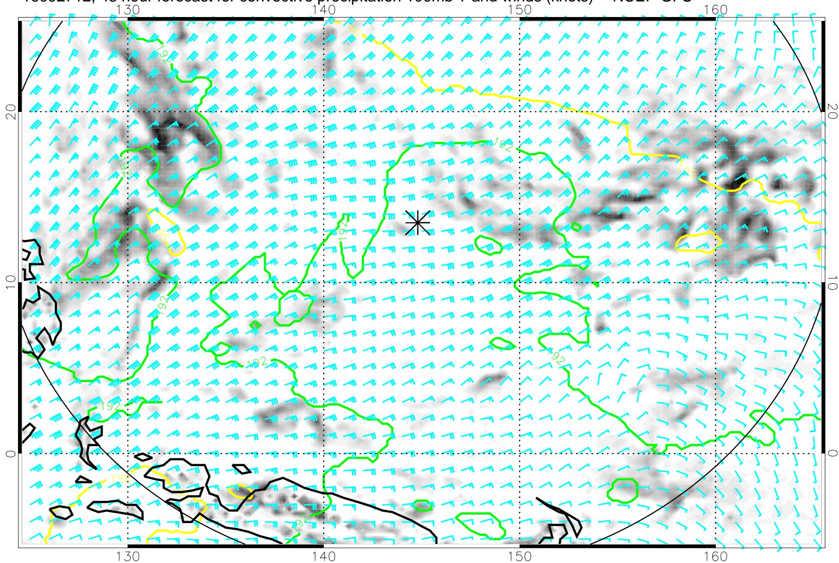
16092712, 48 hour forecast for convective precipitation 100mb T and winds (knots) -- NCEP GFS
