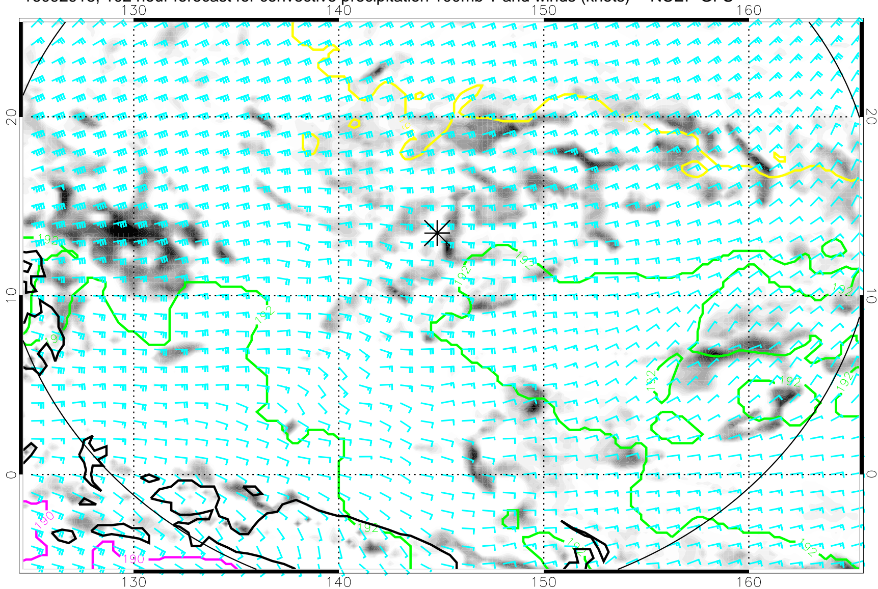
16092918, 102 hour forecast for convective precipitation 100mb T and winds (knots) -- NCEP GFS
