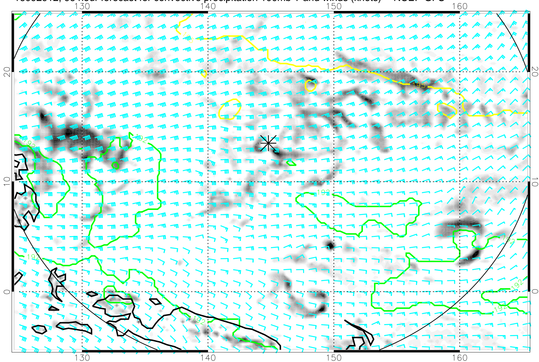
16092912, 96 hour forecast for convective precipitation 100mb T and winds (knots) -- NCEP GFS
