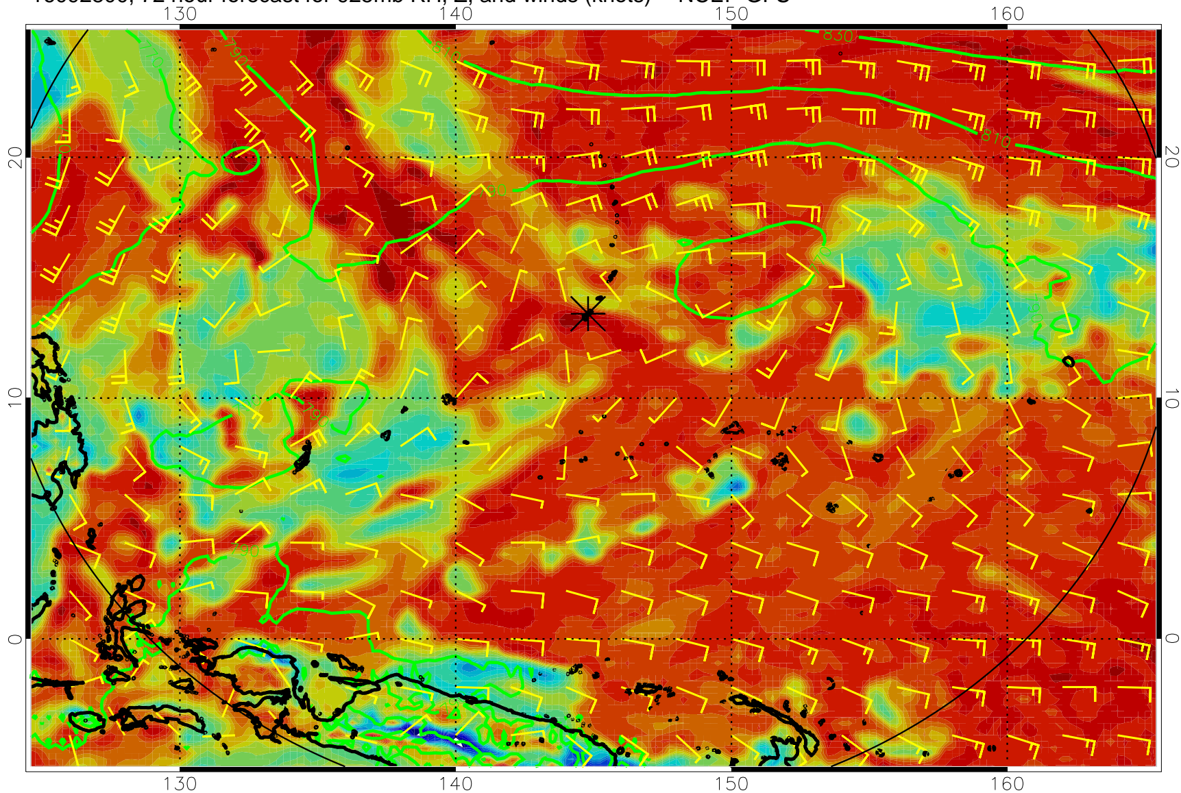
16092800, 72 hour forecast for 925mb RH, Z, and winds (knots) -- NCEP GFS
