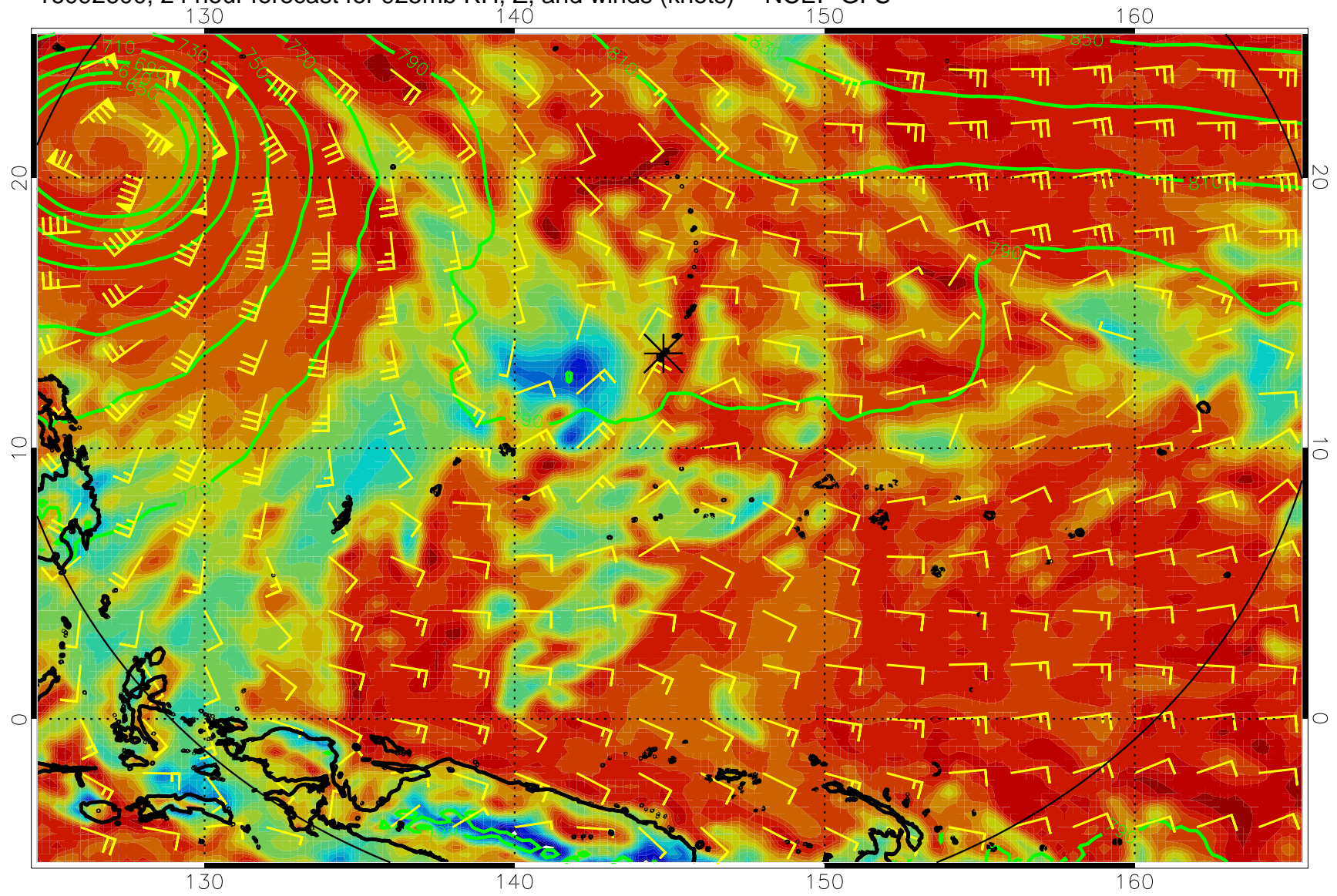
16092600, 24 hour forecast for 925mb RH, Z, and winds (knots) -- NCEP GFS
