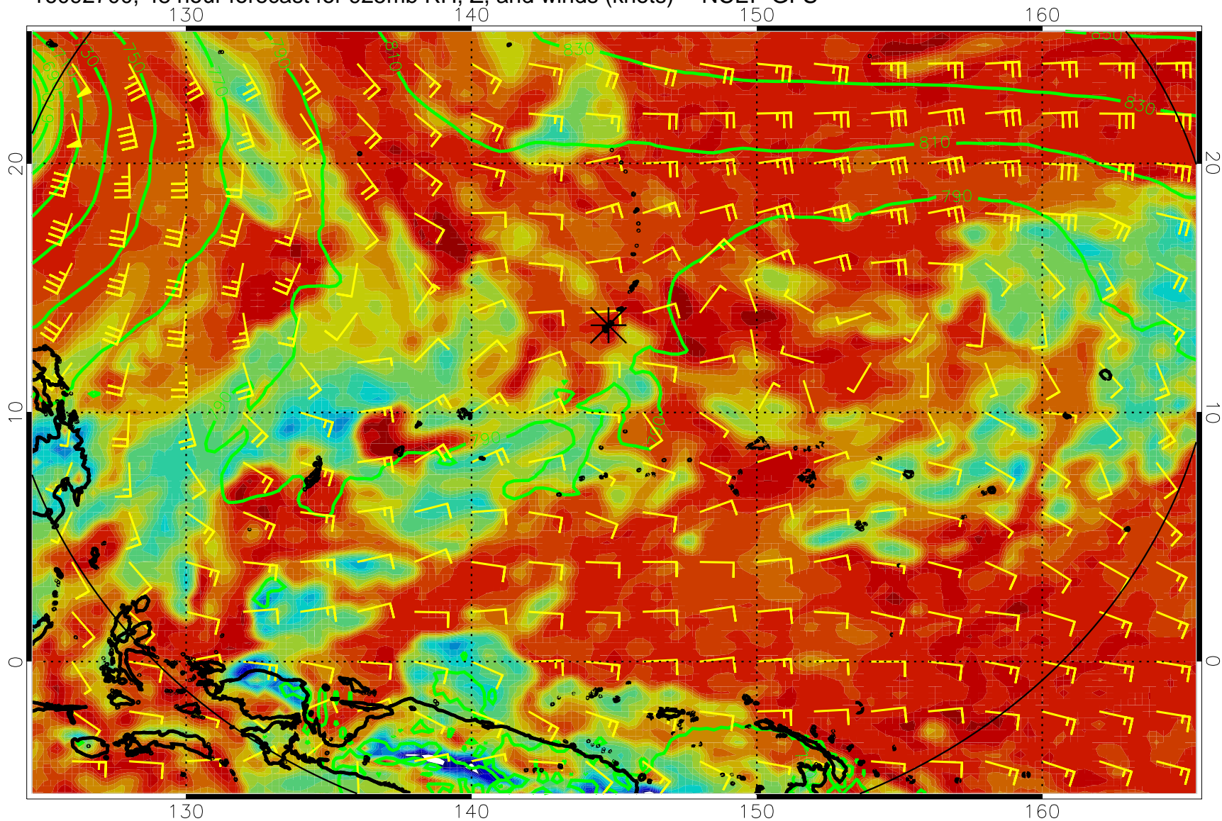
16092700, 48 hour forecast for 925mb RH, Z, and winds (knots) -- NCEP GFS
