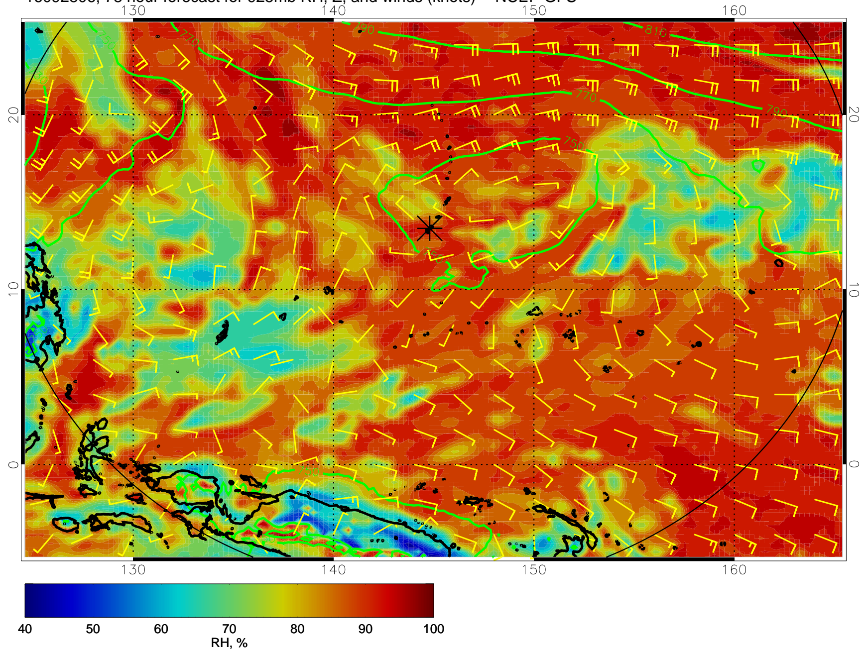
16092806, 78 hour forecast for 925mb RH, Z, and winds (knots) -- NCEP GFS
