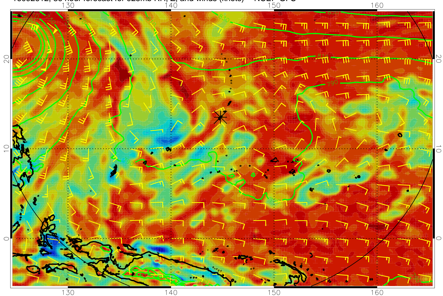
16092612, 36 hour forecast for 925mb RH, Z, and winds (knots) -- NCEP GFS
