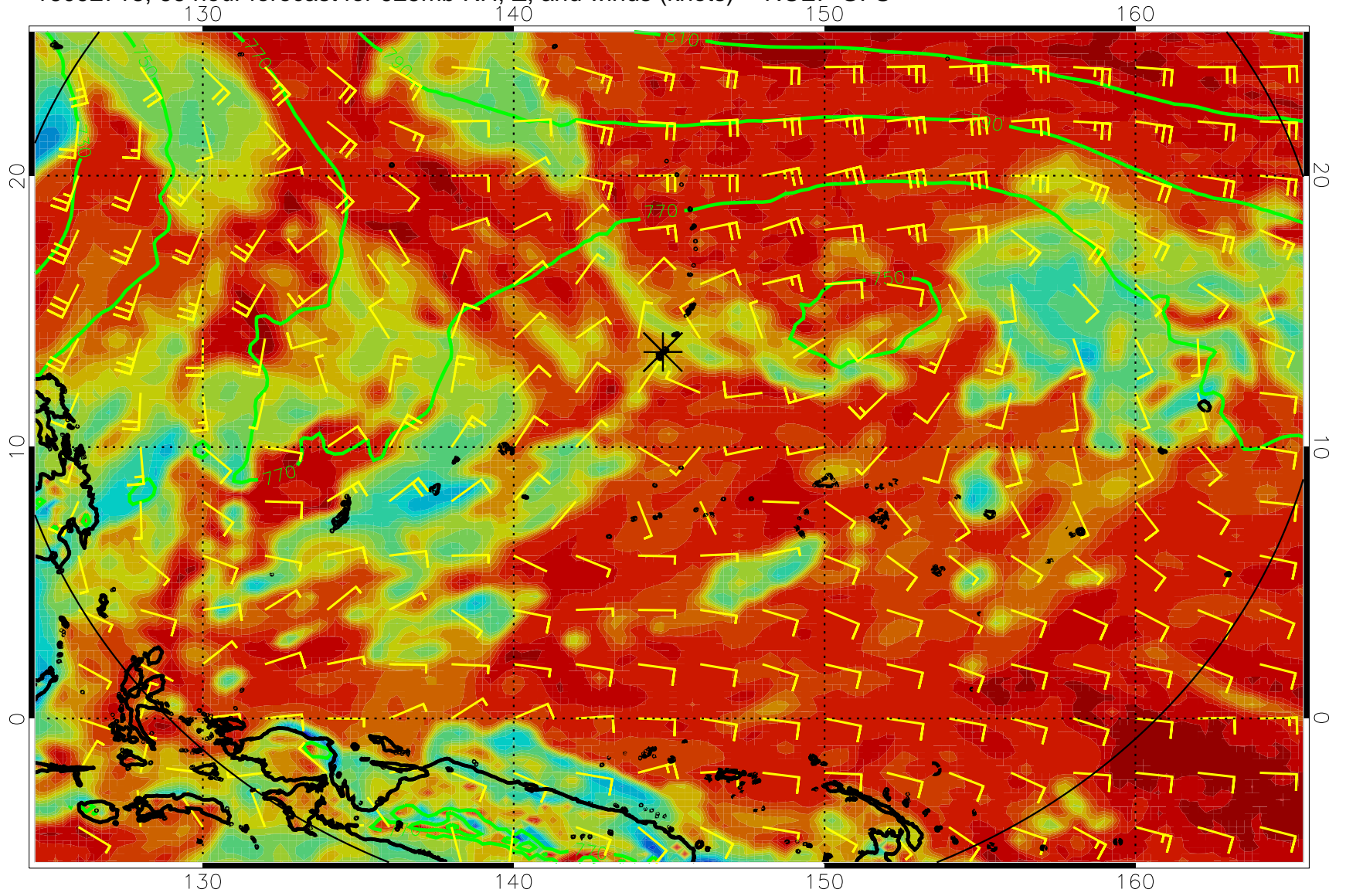
16092718, 66 hour forecast for 925mb RH, Z, and winds (knots) -- NCEP GFS
