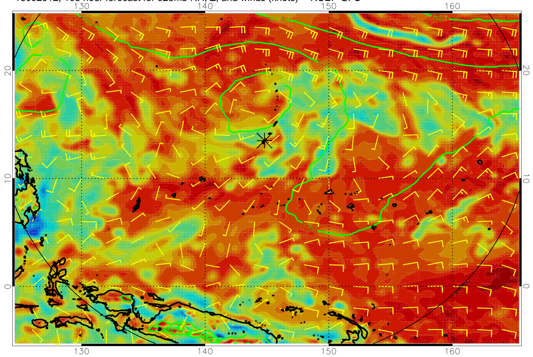
16092912, 108 hour forecast for 925mb RH, Z, and winds (knots) -- NCEP GFS
