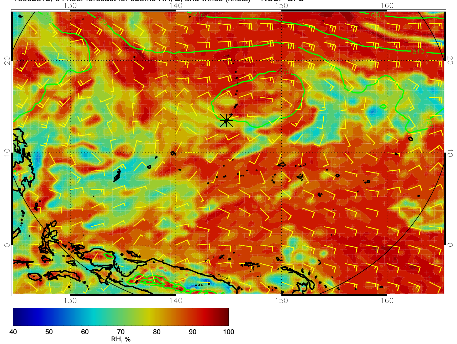
16092812, 84 hour forecast for 925mb RH, Z, and winds (knots) -- NCEP GFS
