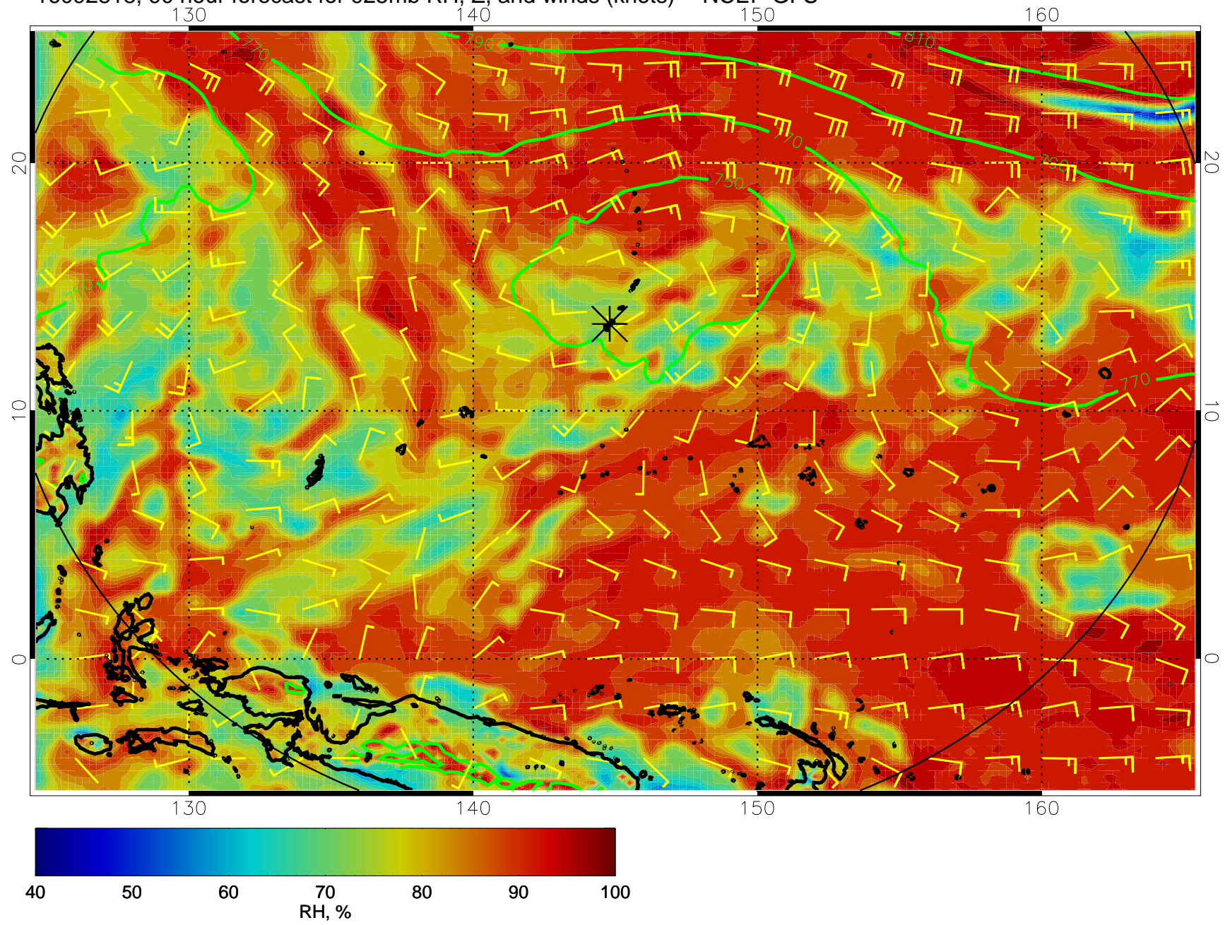
16092818, 90 hour forecast for 925mb RH, Z, and winds (knots) -- NCEP GFS
