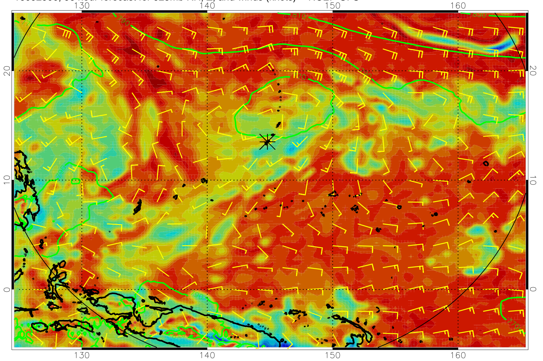
16092900, 96 hour forecast for 925mb RH, Z, and winds (knots) -- NCEP GFS
