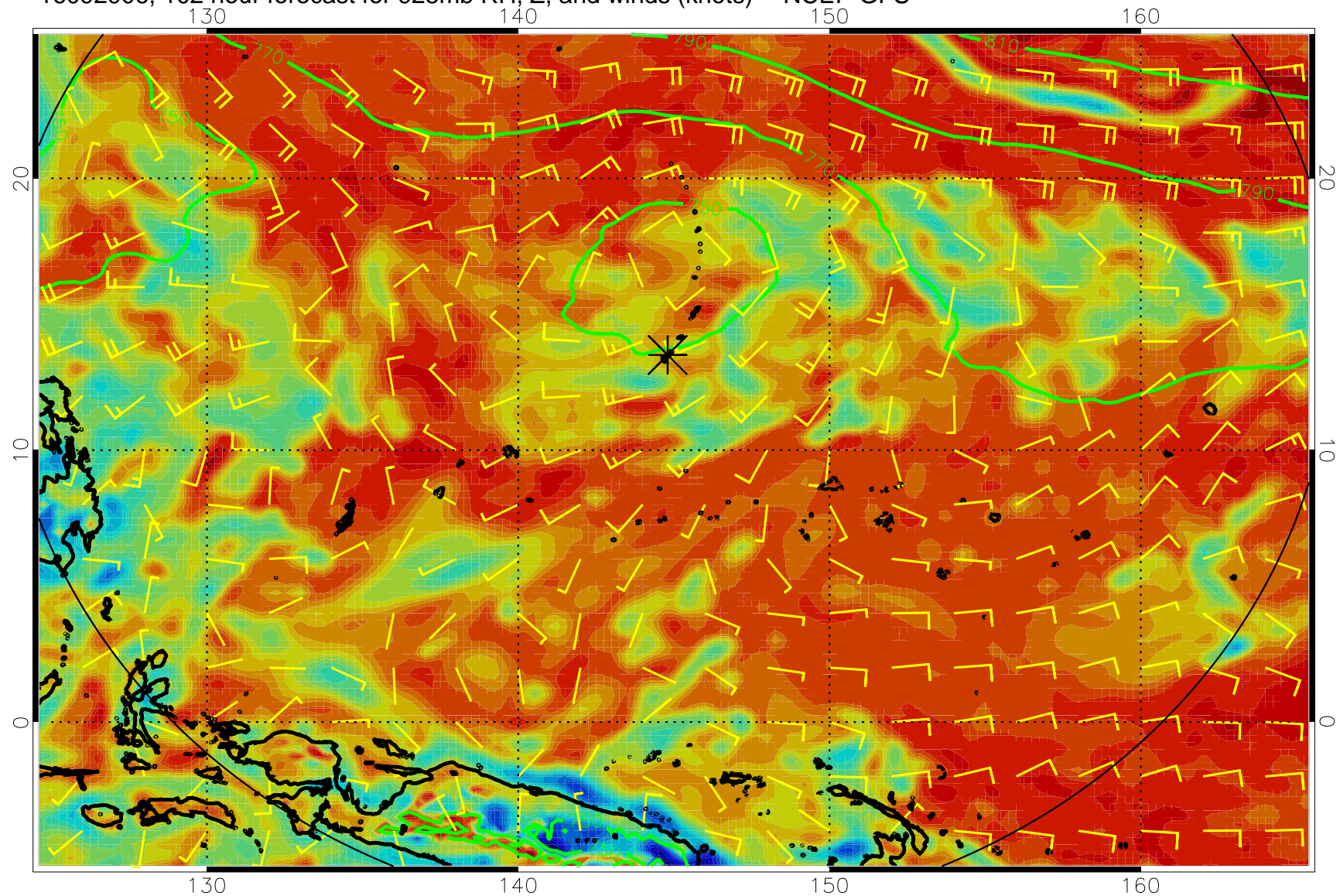
16092906, 102 hour forecast for 925mb RH, Z, and winds (knots) -- NCEP GFS
