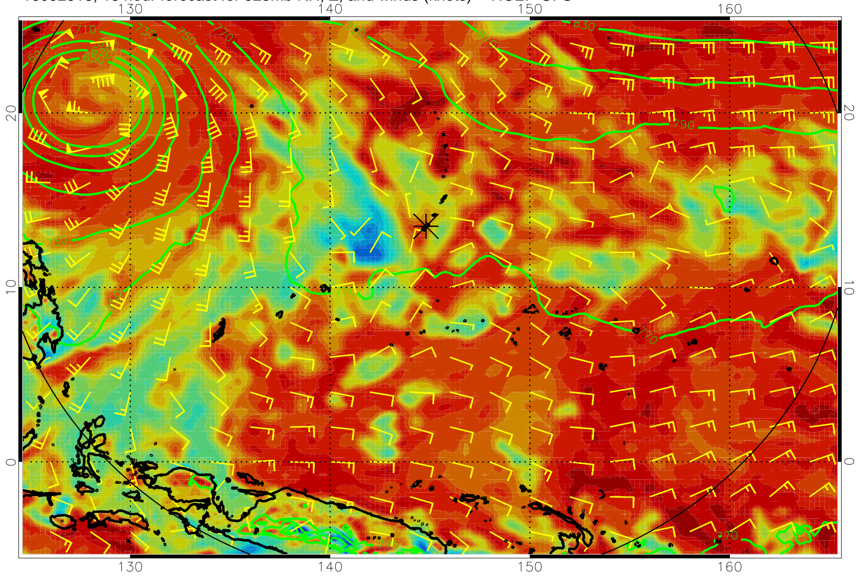
16092518, 18 hour forecast for 925mb RH, Z, and winds (knots) -- NCEP GFS
