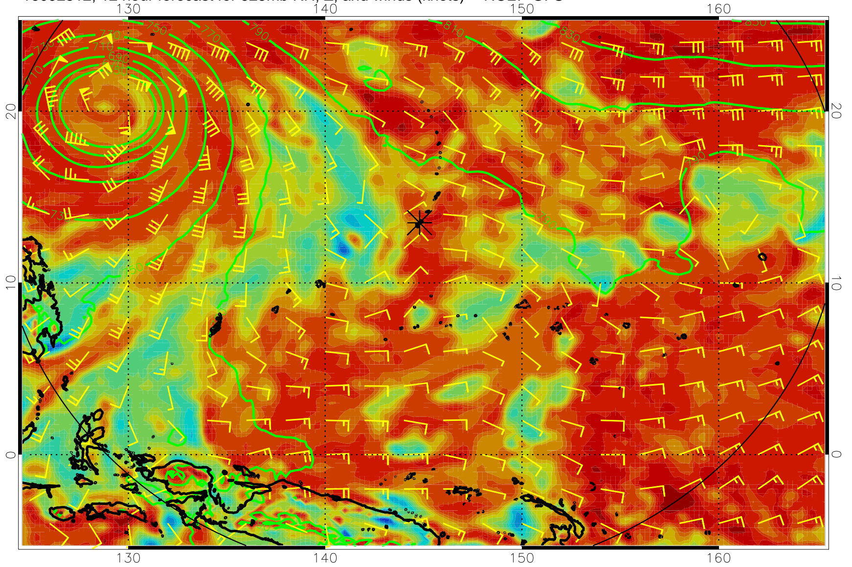
16092512, 12 hour forecast for 925mb RH, Z, and winds (knots) -- NCEP GFS
