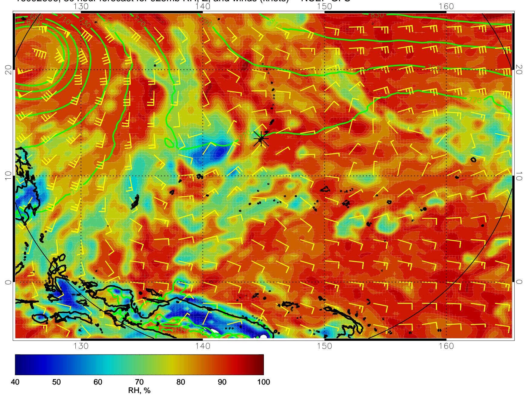
16092606, 30 hour forecast for 925mb RH, Z, and winds (knots) -- NCEP GFS
