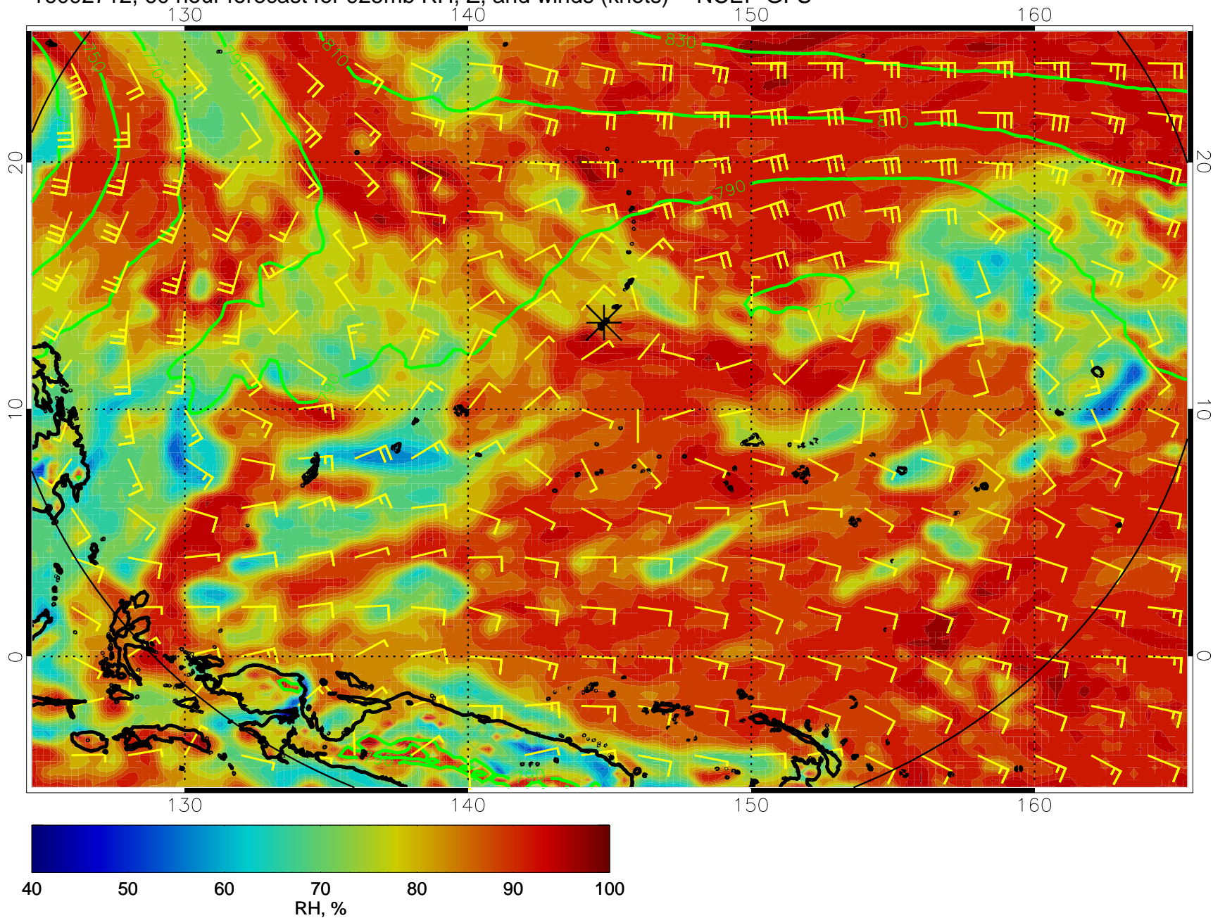
16092712, 60 hour forecast for 925mb RH, Z, and winds (knots) -- NCEP GFS
