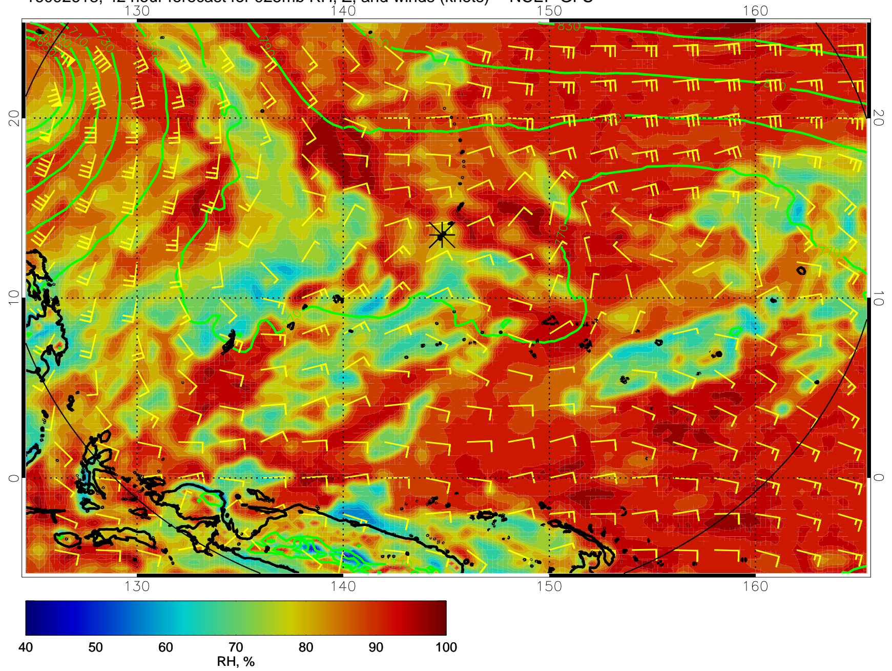
16092618, 42 hour forecast for 925mb RH, Z, and winds (knots) -- NCEP GFS
