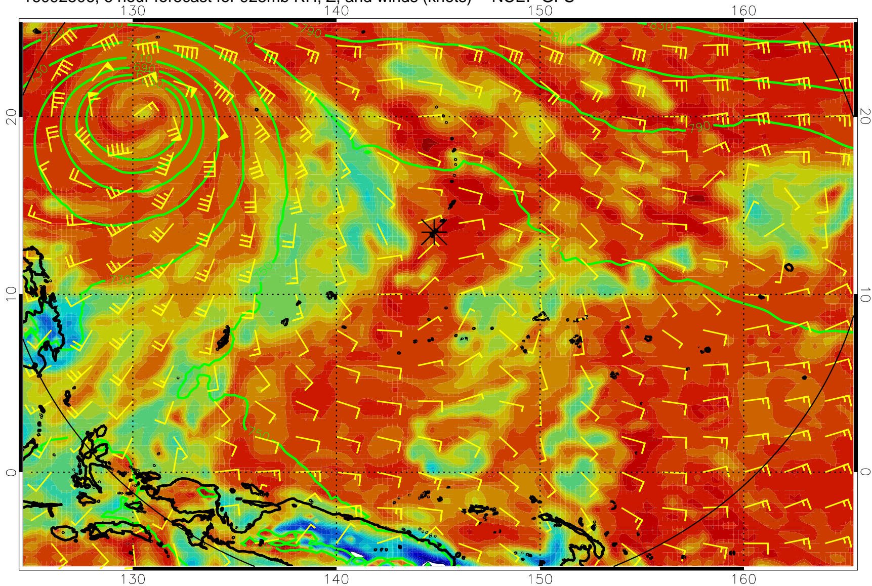
16092506, 6 hour forecast for 925mb RH, Z, and winds (knots) -- NCEP GFS
