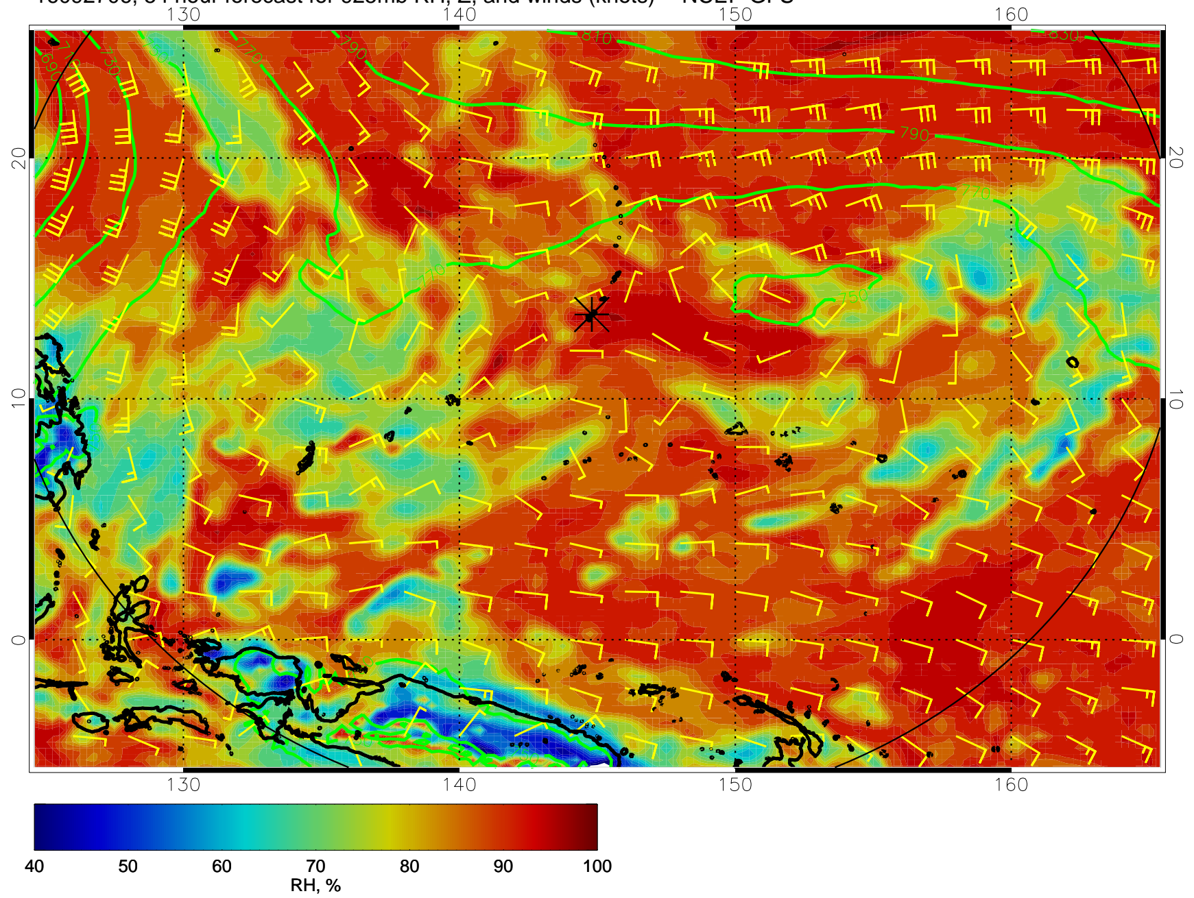
16092706, 54 hour forecast for 925mb RH, Z, and winds (knots) -- NCEP GFS
