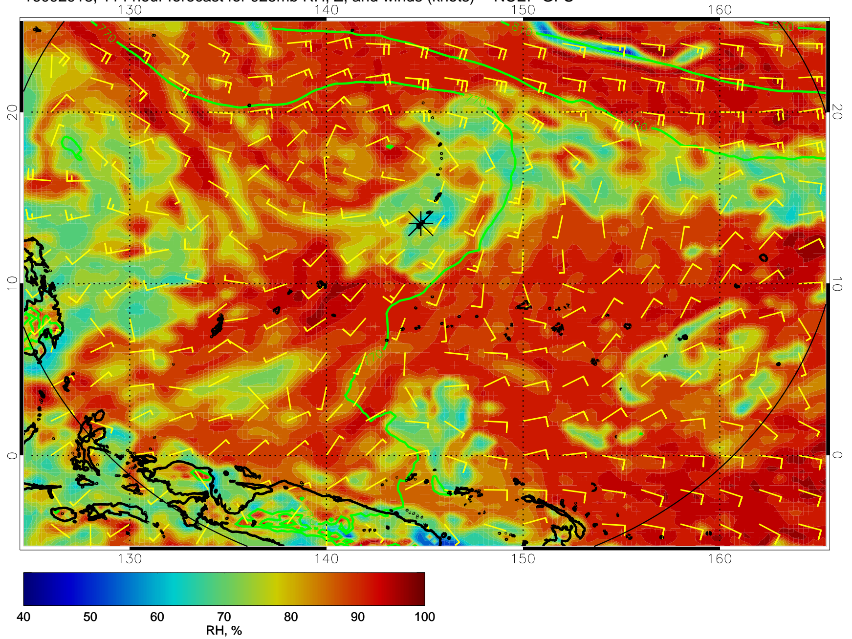
16092918, 114 hour forecast for 925mb RH, Z, and winds (knots) -- NCEP GFS
