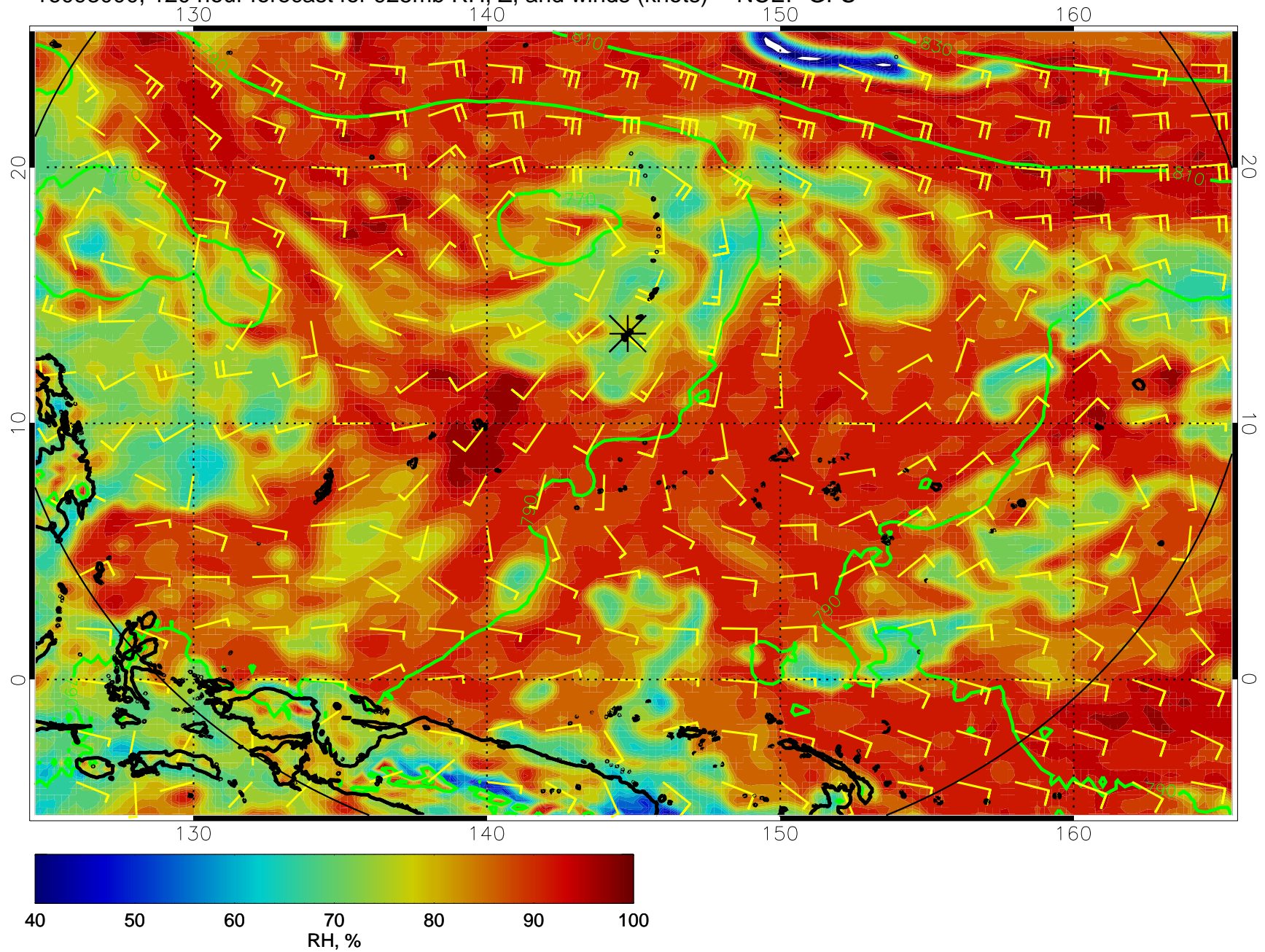
16093000, 120 hour forecast for 925mb RH, Z, and winds (knots) -- NCEP GFS
