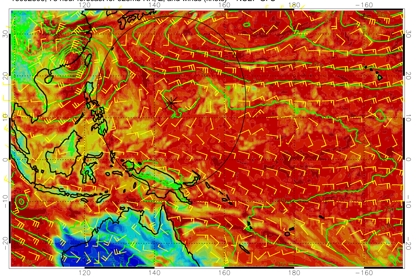
16092806, 78 hour forecast for 925mb RH, Z, and winds (knots) -- NCEP GFS
