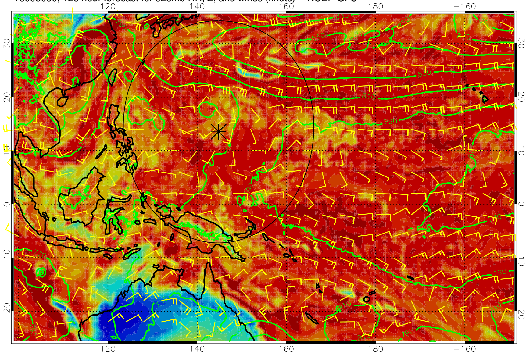
16093000, 120 hour forecast for 925mb RH, Z, and winds (knots) -- NCEP GFS
