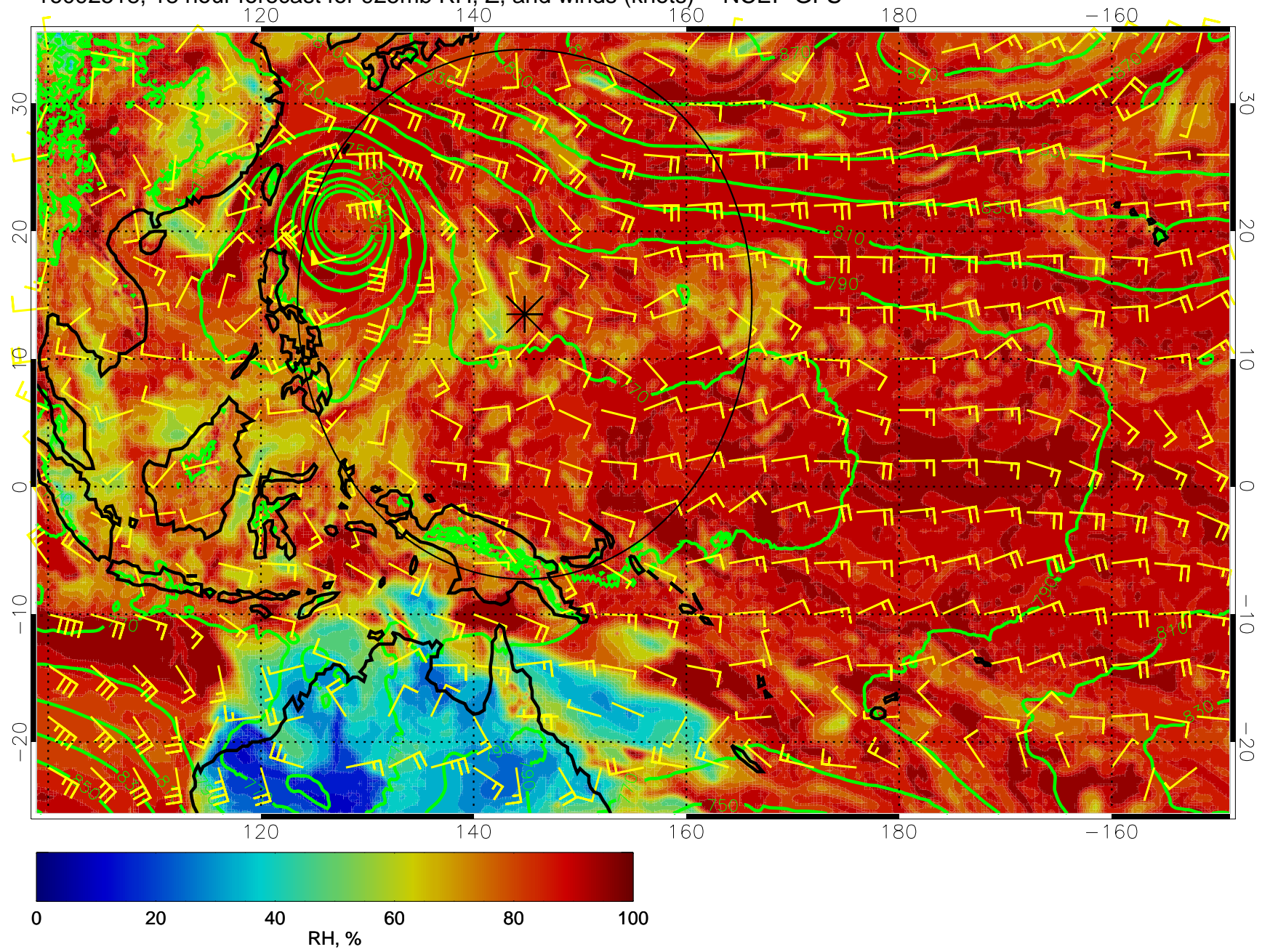
16092518, 18 hour forecast for 925mb RH, Z, and winds (knots) -- NCEP GFS
