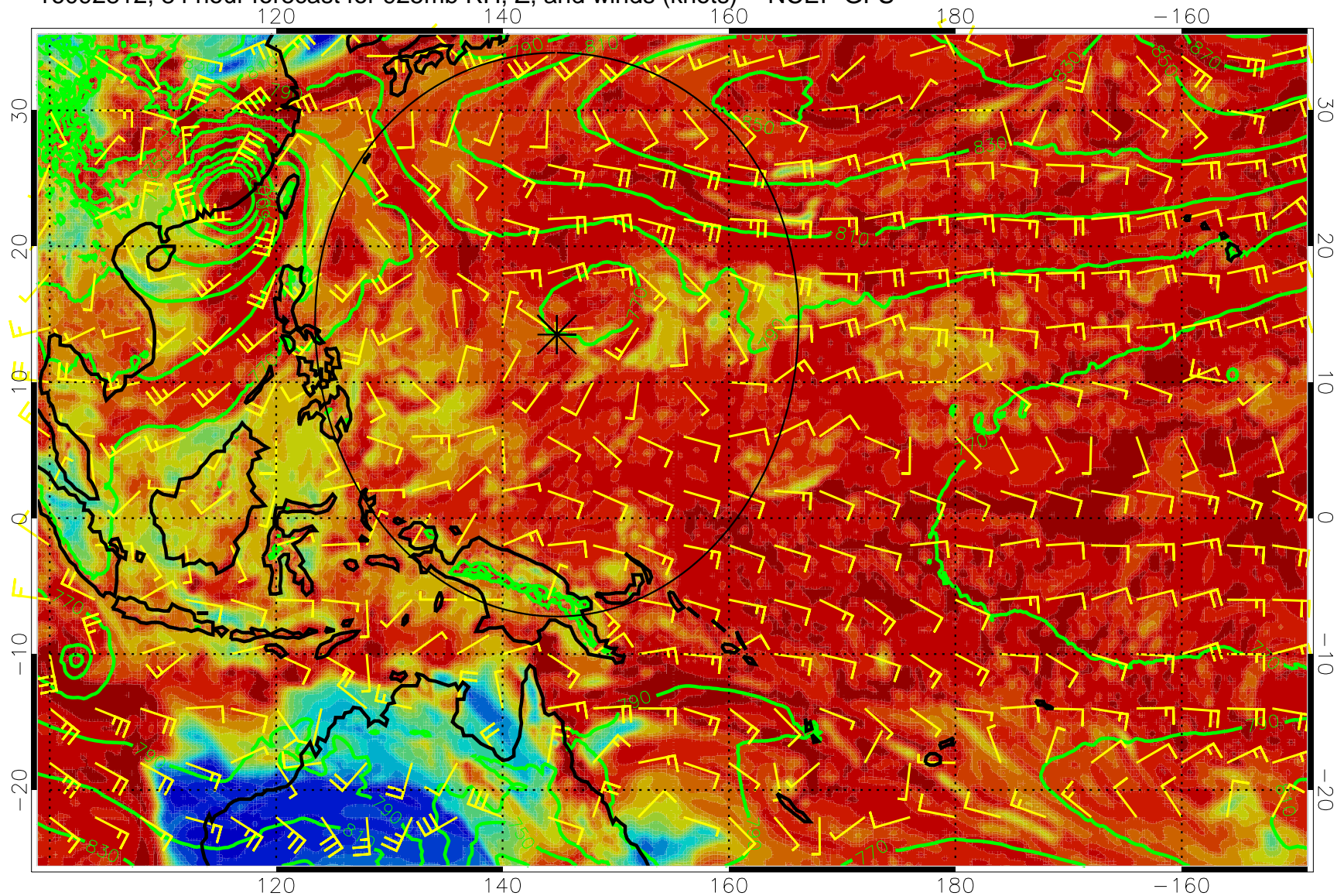
16092812, 84 hour forecast for 925mb RH, Z, and winds (knots) -- NCEP GFS
