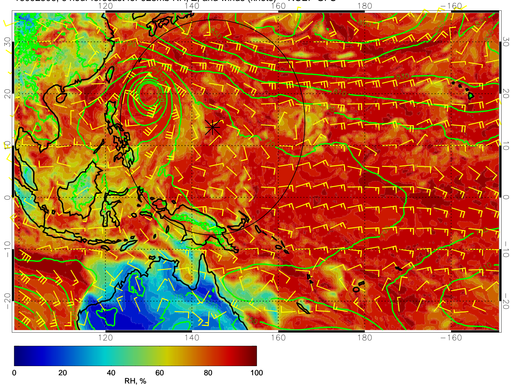
16092506, 6 hour forecast for 925mb RH, Z, and winds (knots) -- NCEP GFS
