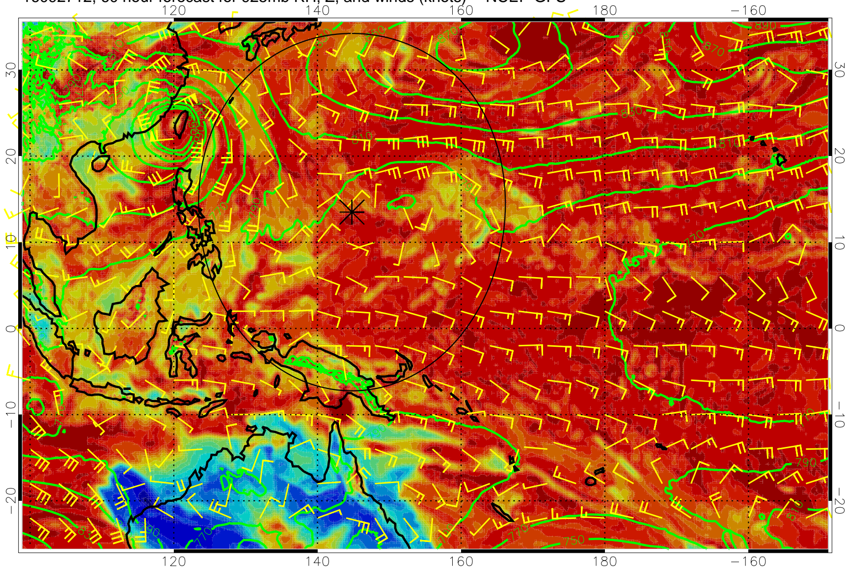
16092712, 60 hour forecast for 925mb RH, Z, and winds (knots) -- NCEP GFS
