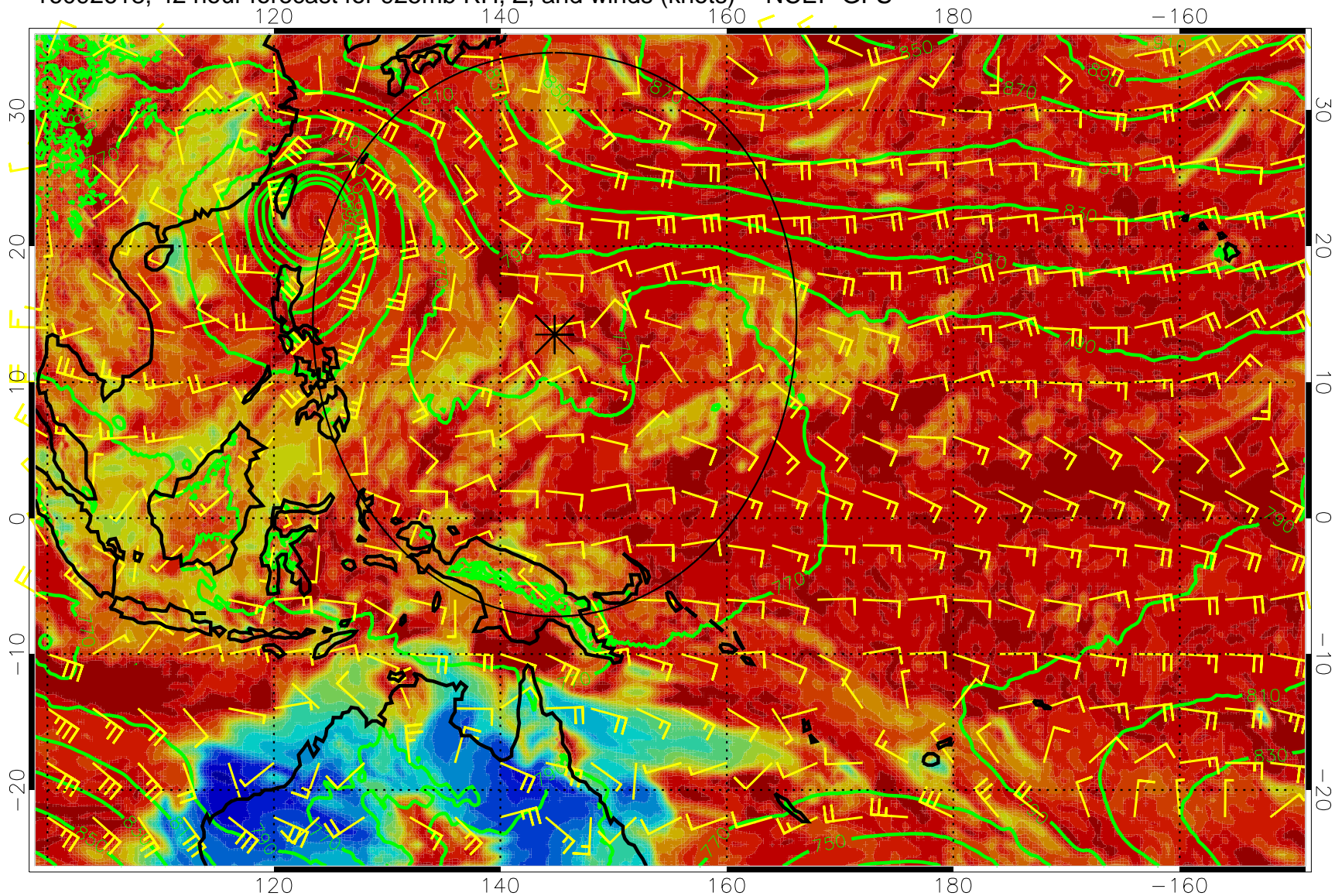
16092618, 42 hour forecast for 925mb RH, Z, and winds (knots) -- NCEP GFS
