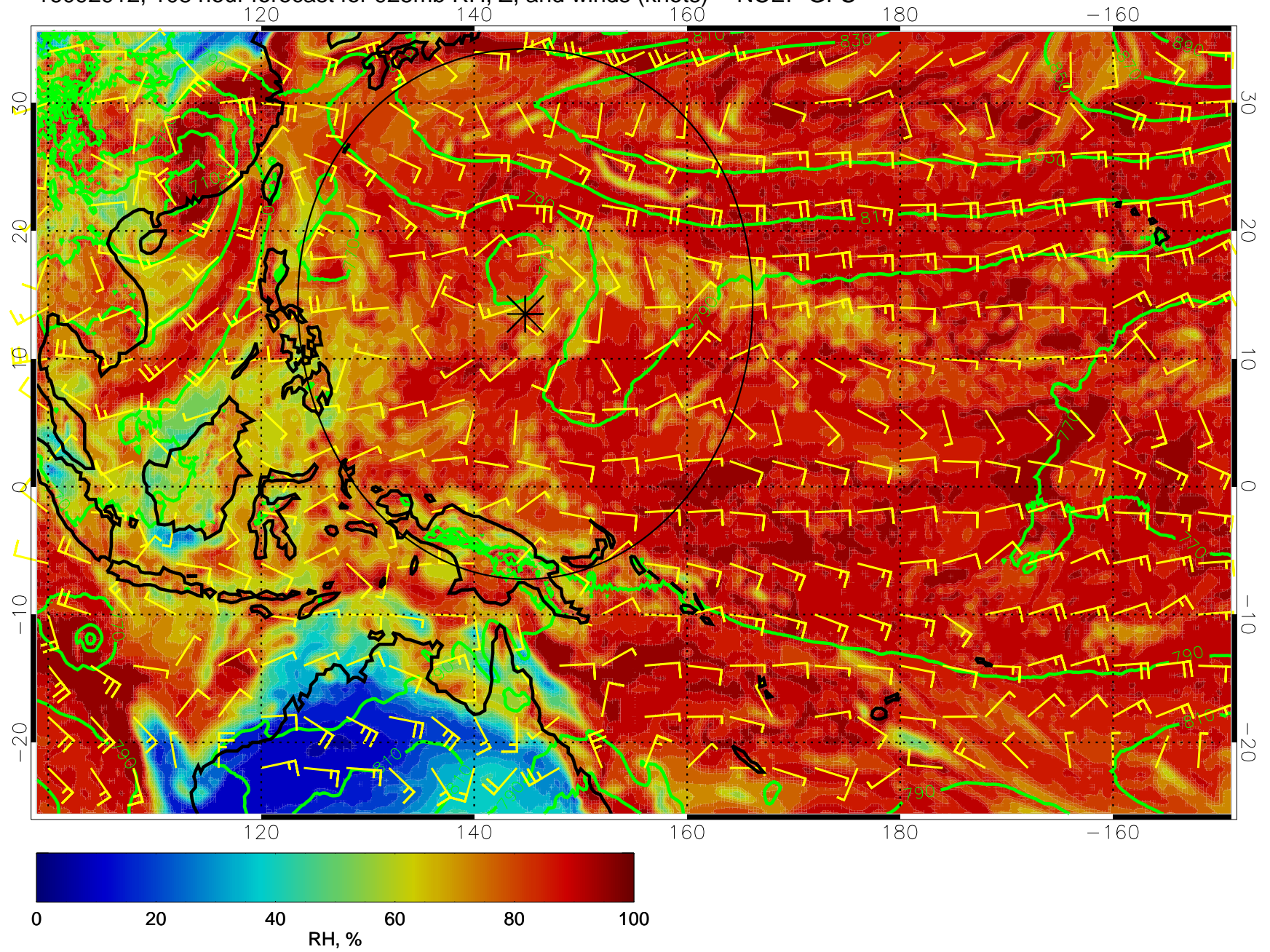
16092912, 108 hour forecast for 925mb RH, Z, and winds (knots) -- NCEP GFS
