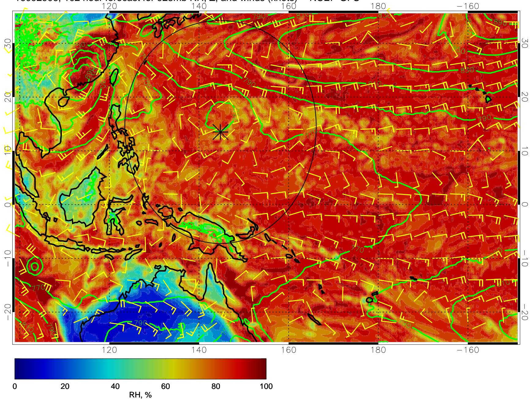
16092906, 102 hour forecast for 925mb RH, Z, and winds (knots) -- NCEP GFS
