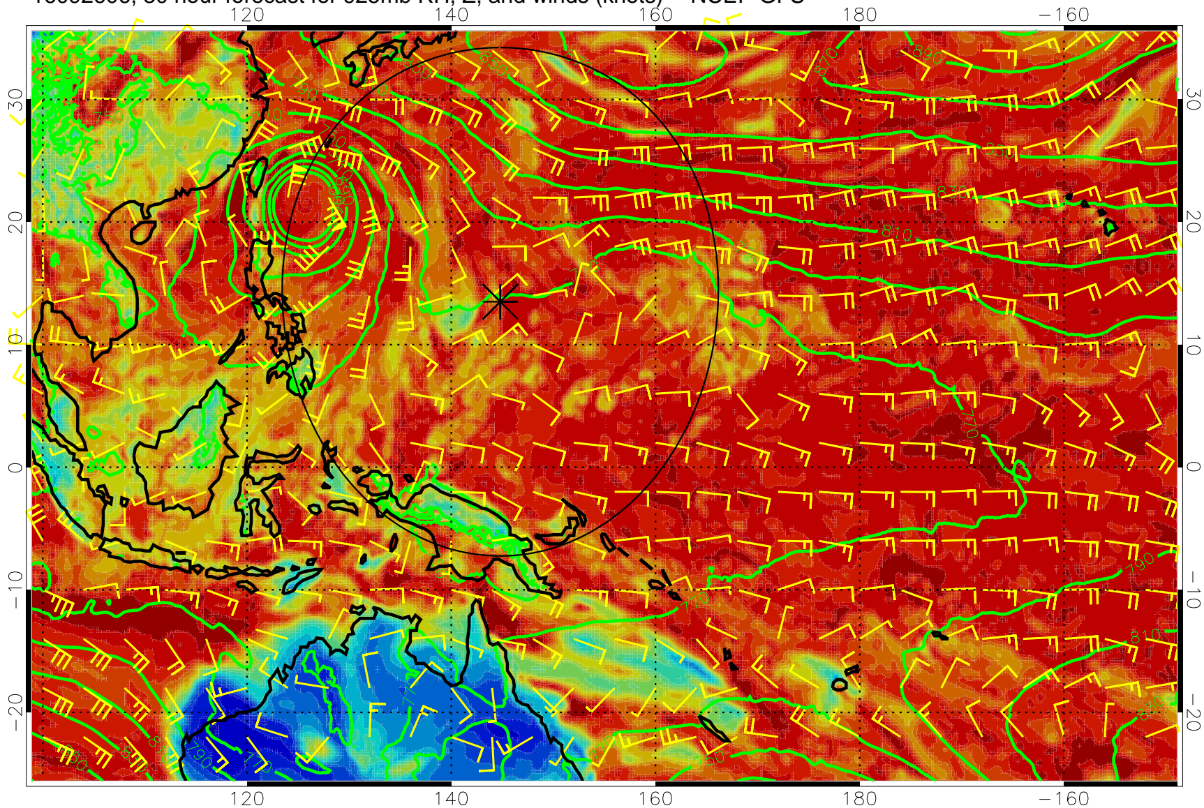
16092606, 30 hour forecast for 925mb RH, Z, and winds (knots) -- NCEP GFS
