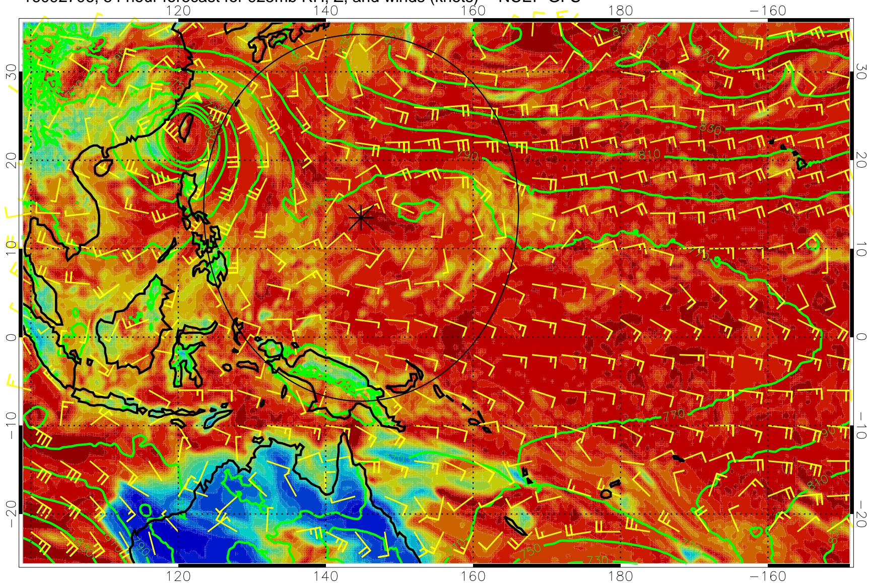
16092706, 54 hour forecast for 925mb RH, Z, and winds (knots) -- NCEP GFS
