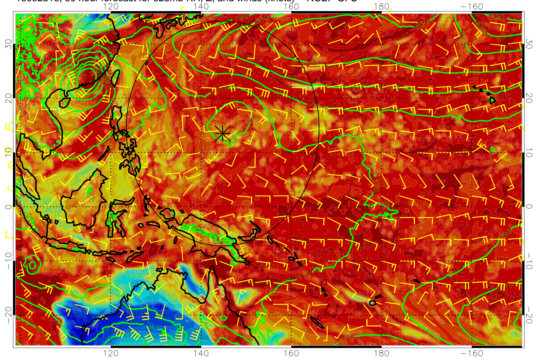
16092818, 90 hour forecast for 925mb RH, Z, and winds (knots) -- NCEP GFS
