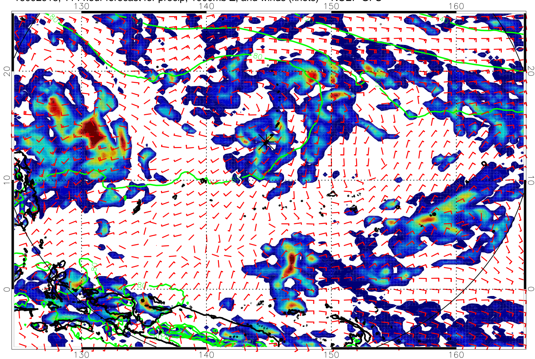
16092918, 114 hour forecast for precip, 1000mb Z, and winds (knots) -- NCEP GFS
