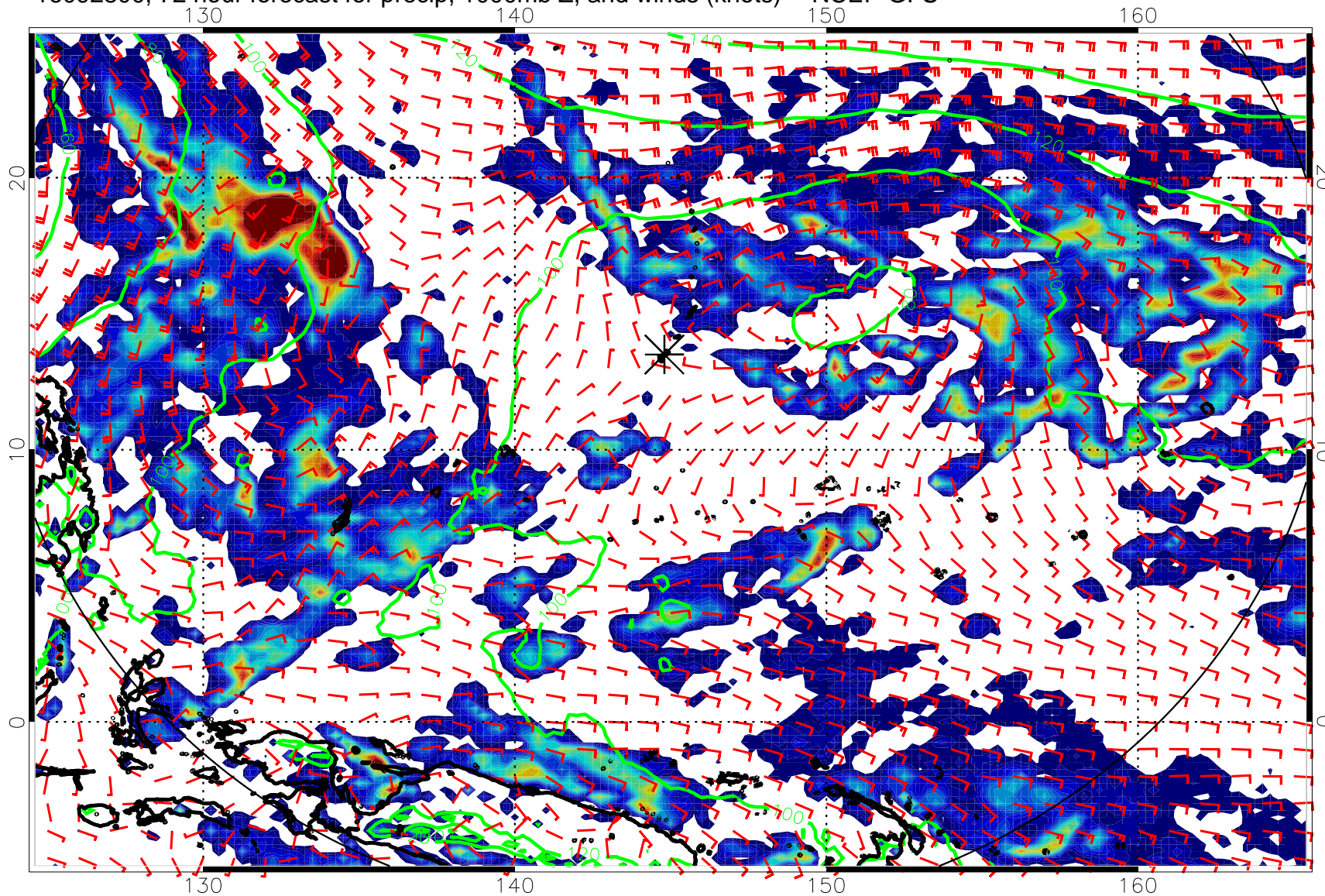
16092800, 72 hour forecast for precip, 1000mb Z, and winds (knots) -- NCEP GFS
