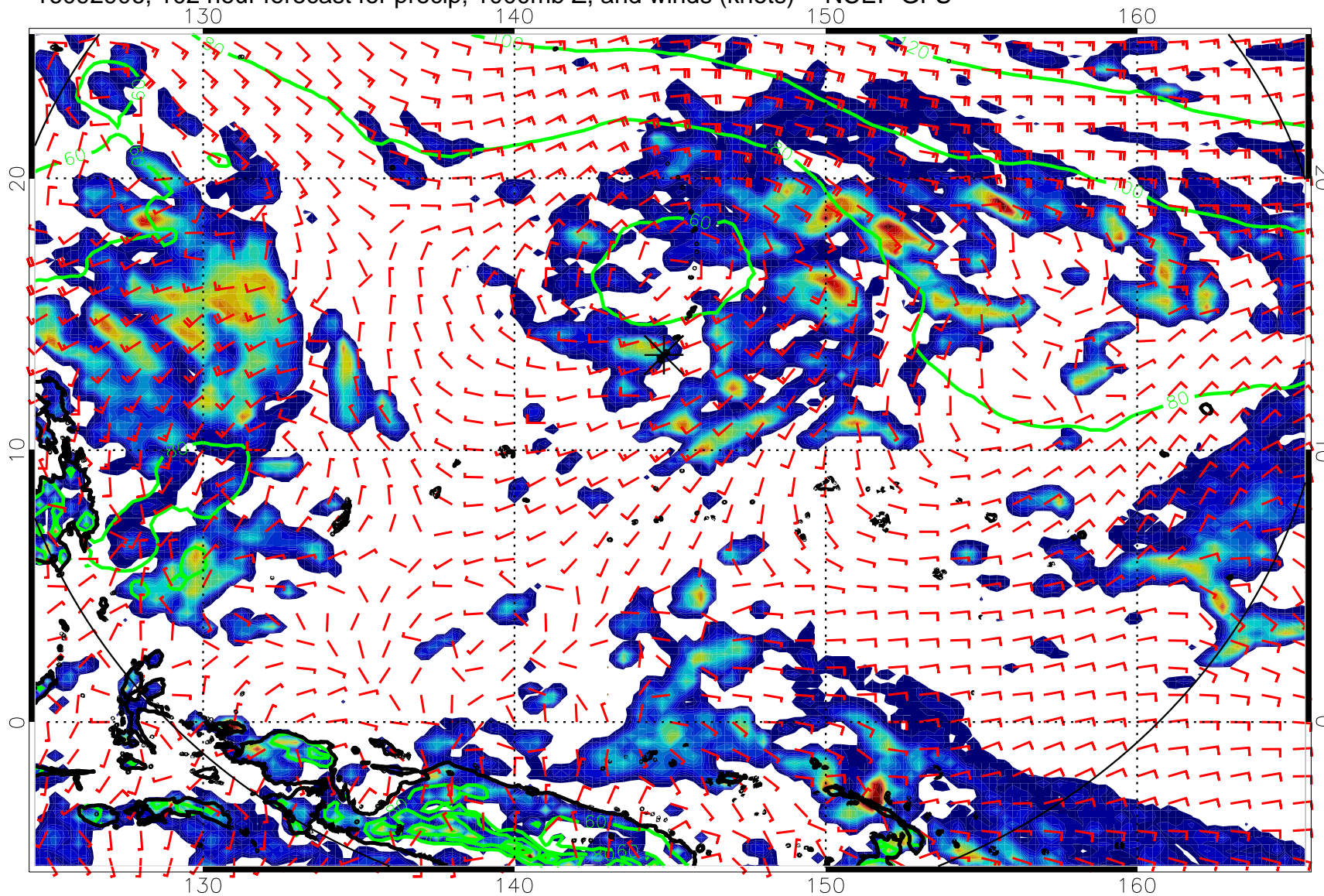
16092906, 102 hour forecast for precip, 1000mb Z, and winds (knots) -- NCEP GFS
