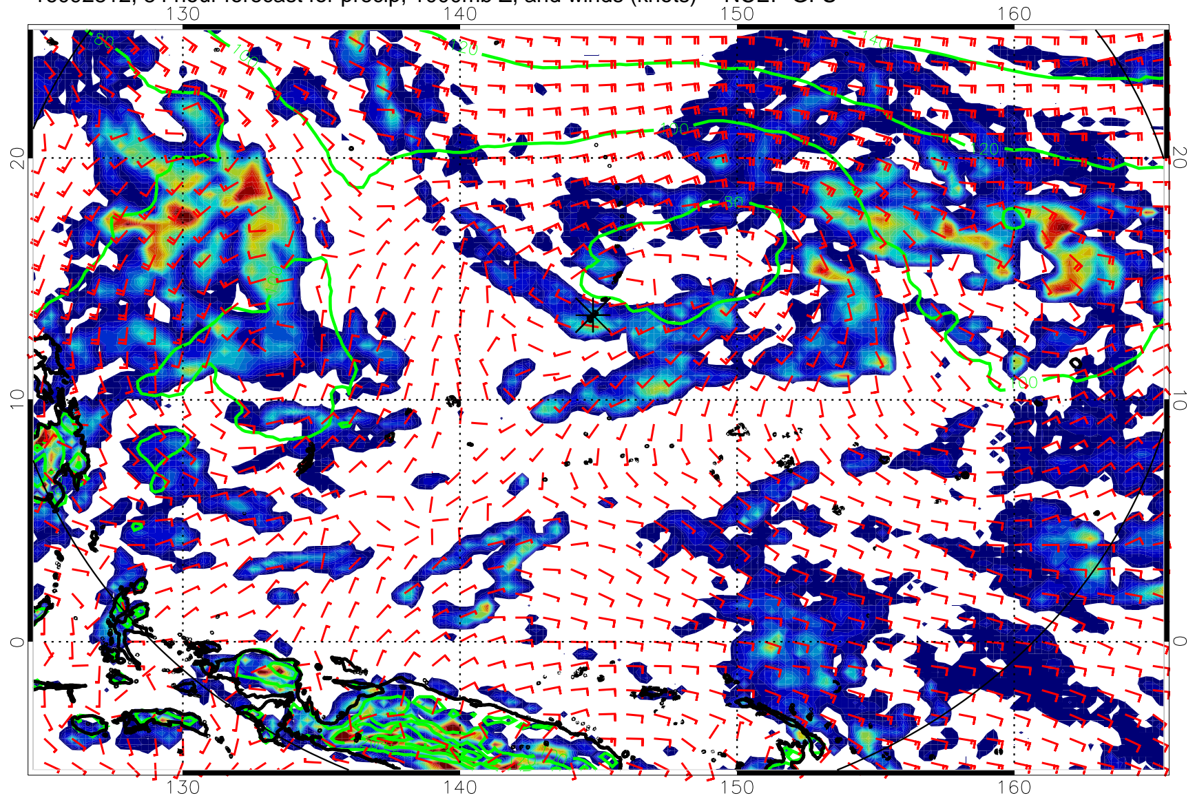
16092812, 84 hour forecast for precip, 1000mb Z, and winds (knots) -- NCEP GFS
