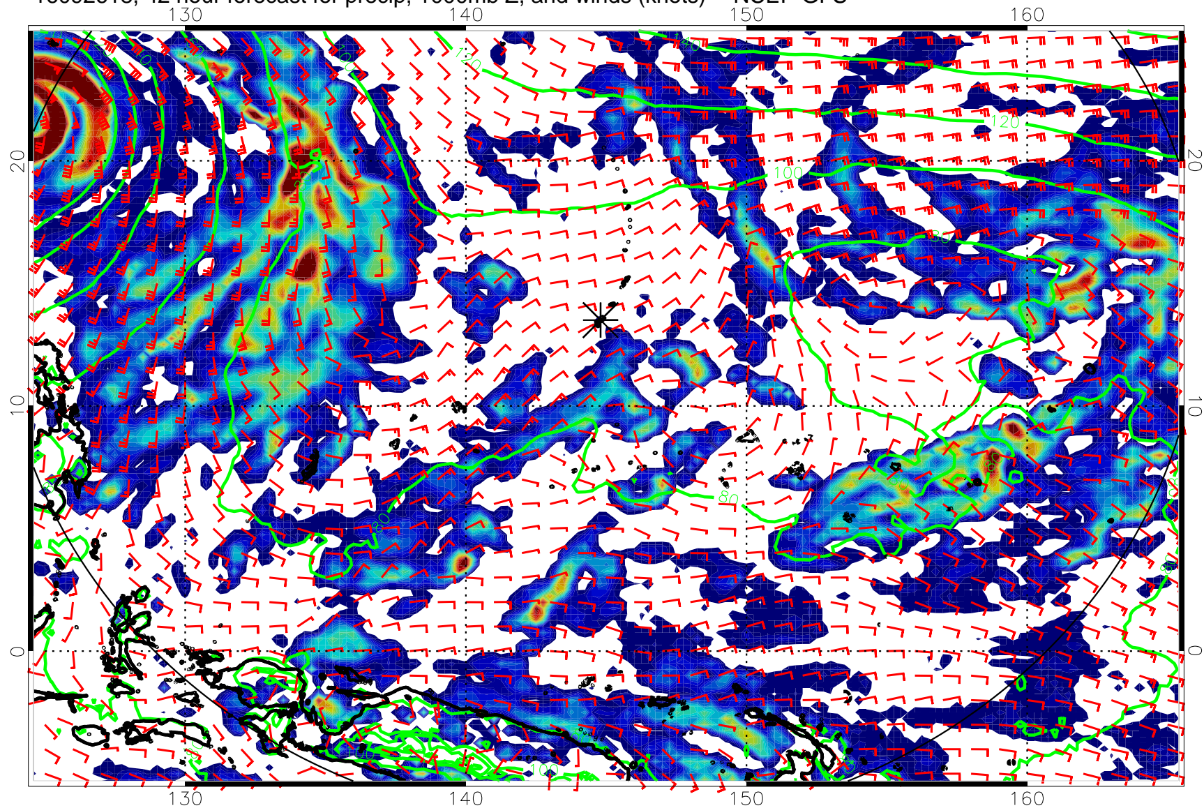
16092618, 42 hour forecast for precip, 1000mb Z, and winds (knots) -- NCEP GFS
