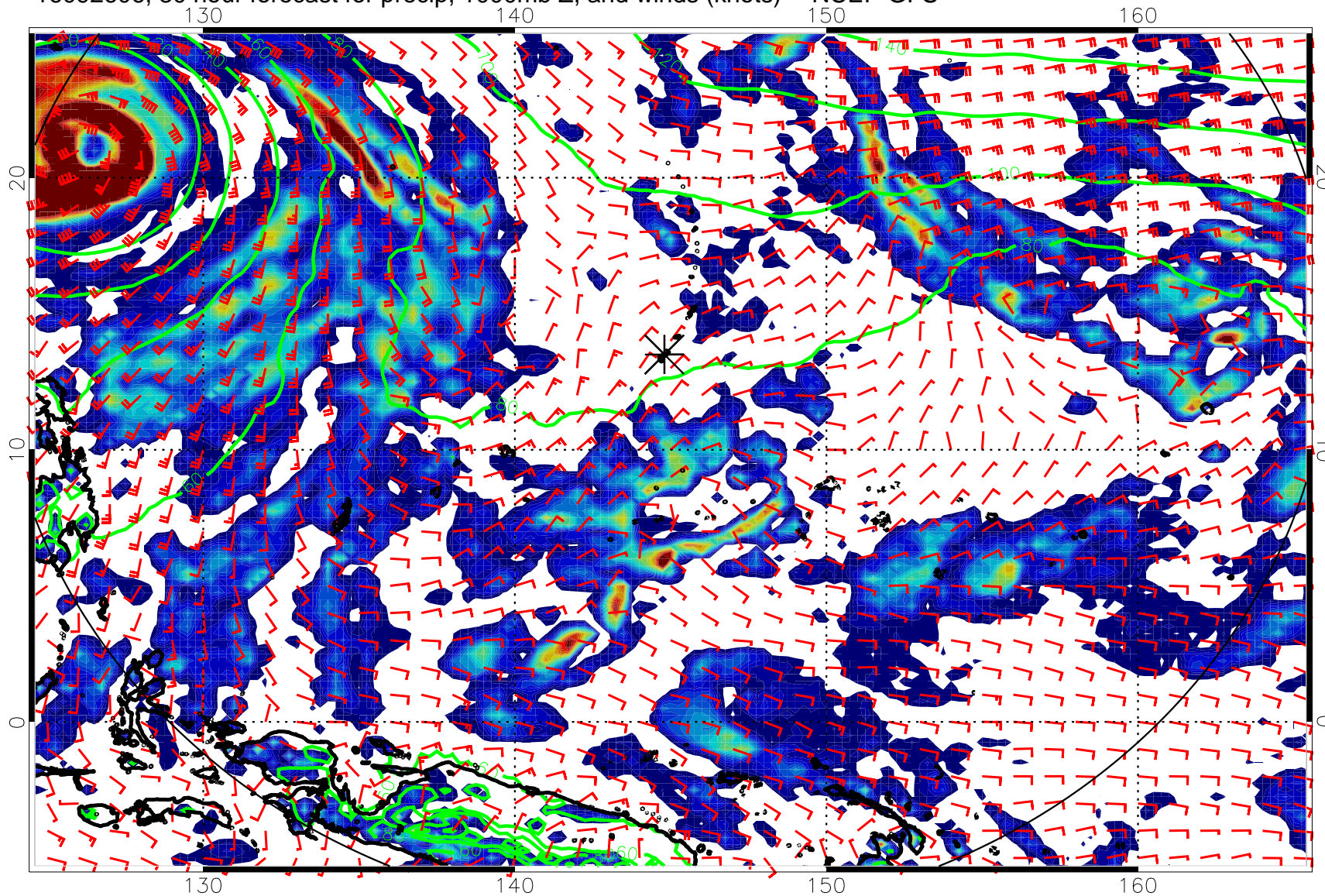
16092606, 30 hour forecast for precip, 1000mb Z, and winds (knots) -- NCEP GFS
