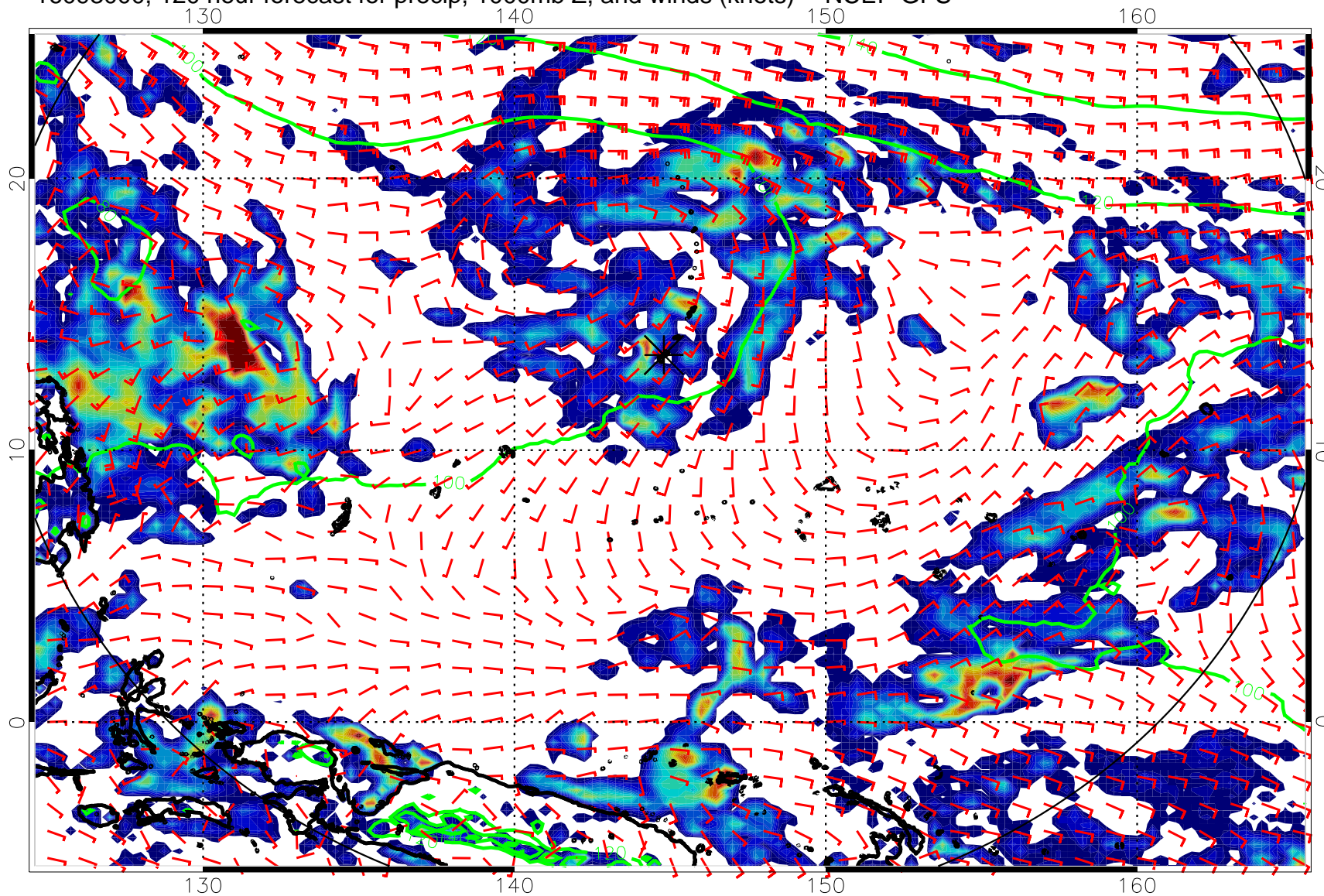
16093000, 120 hour forecast for precip, 1000mb Z, and winds (knots) -- NCEP GFS
