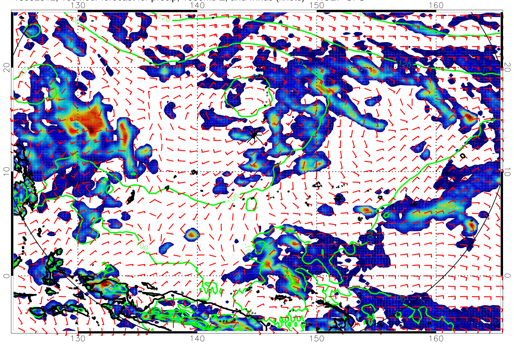
16092912, 108 hour forecast for precip, 1000mb Z, and winds (knots) -- NCEP GFS
