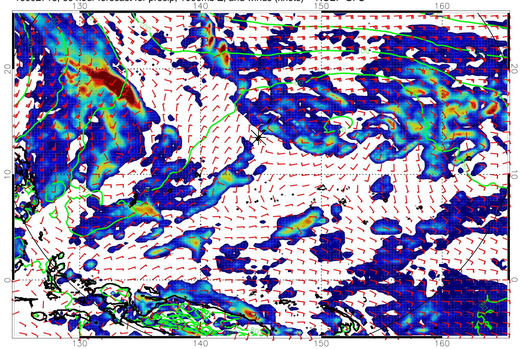
16092718, 66 hour forecast for precip, 1000mb Z, and winds (knots) -- NCEP GFS
