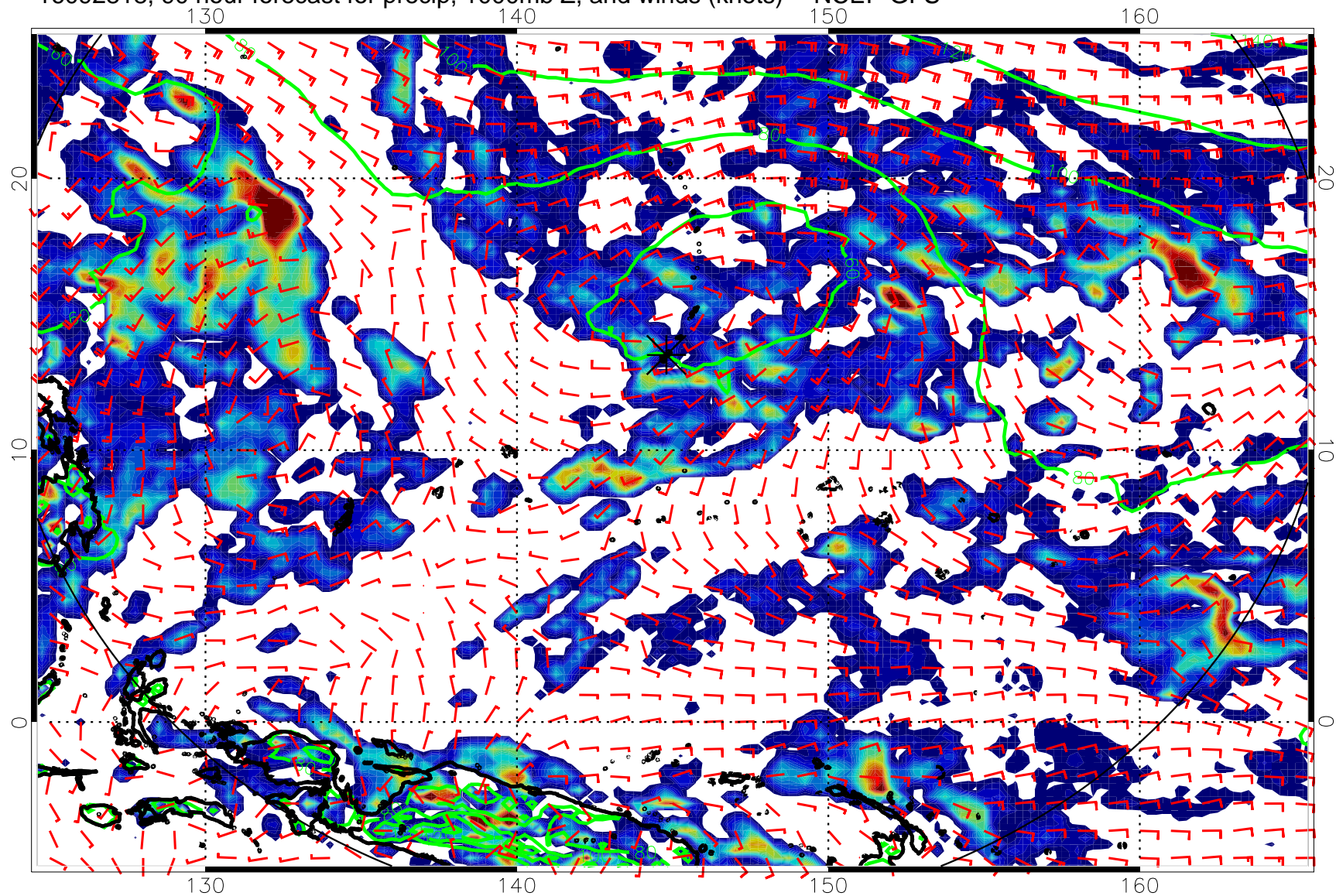
16092818, 90 hour forecast for precip, 1000mb Z, and winds (knots) -- NCEP GFS
