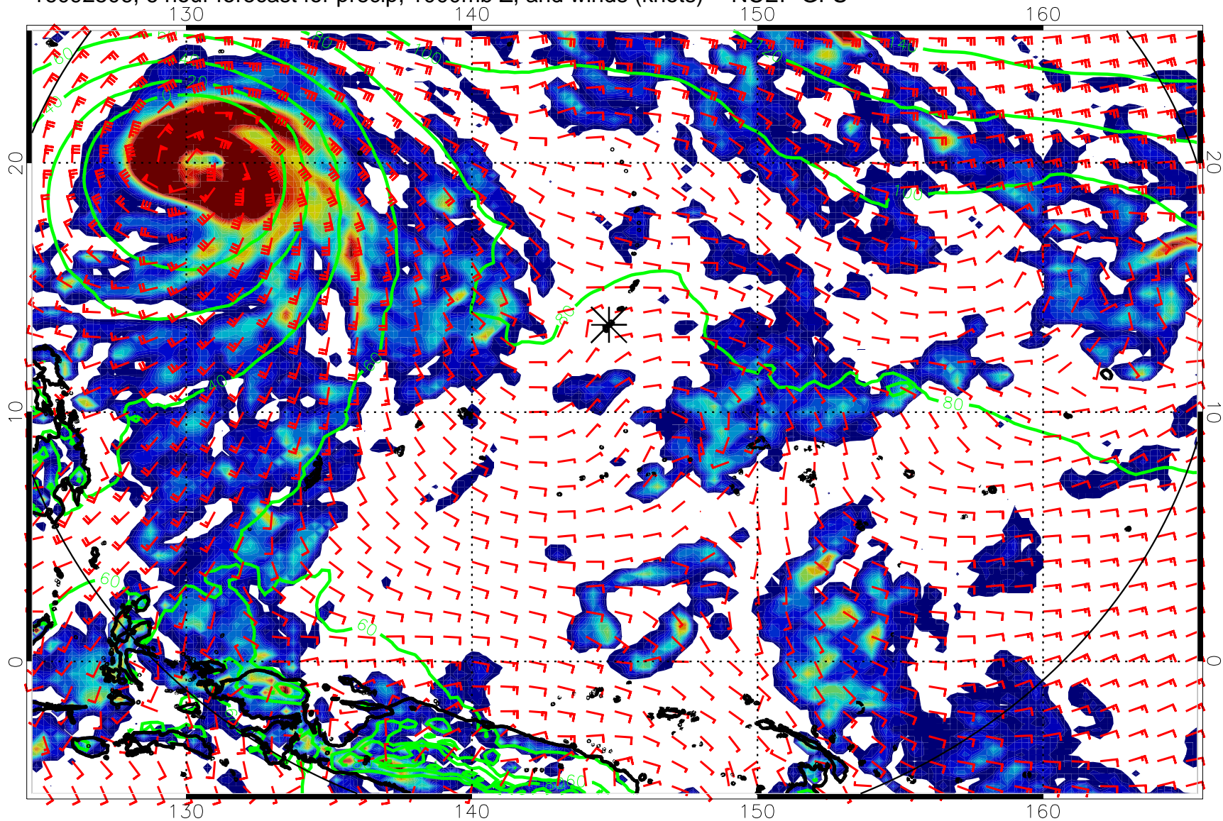
16092506, 6 hour forecast for precip, 1000mb Z, and winds (knots) -- NCEP GFS
