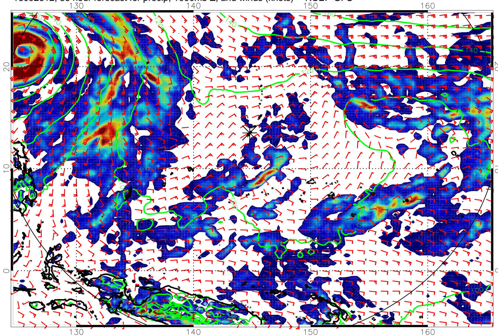
16092612, 36 hour forecast for precip, 1000mb Z, and winds (knots) -- NCEP GFS
