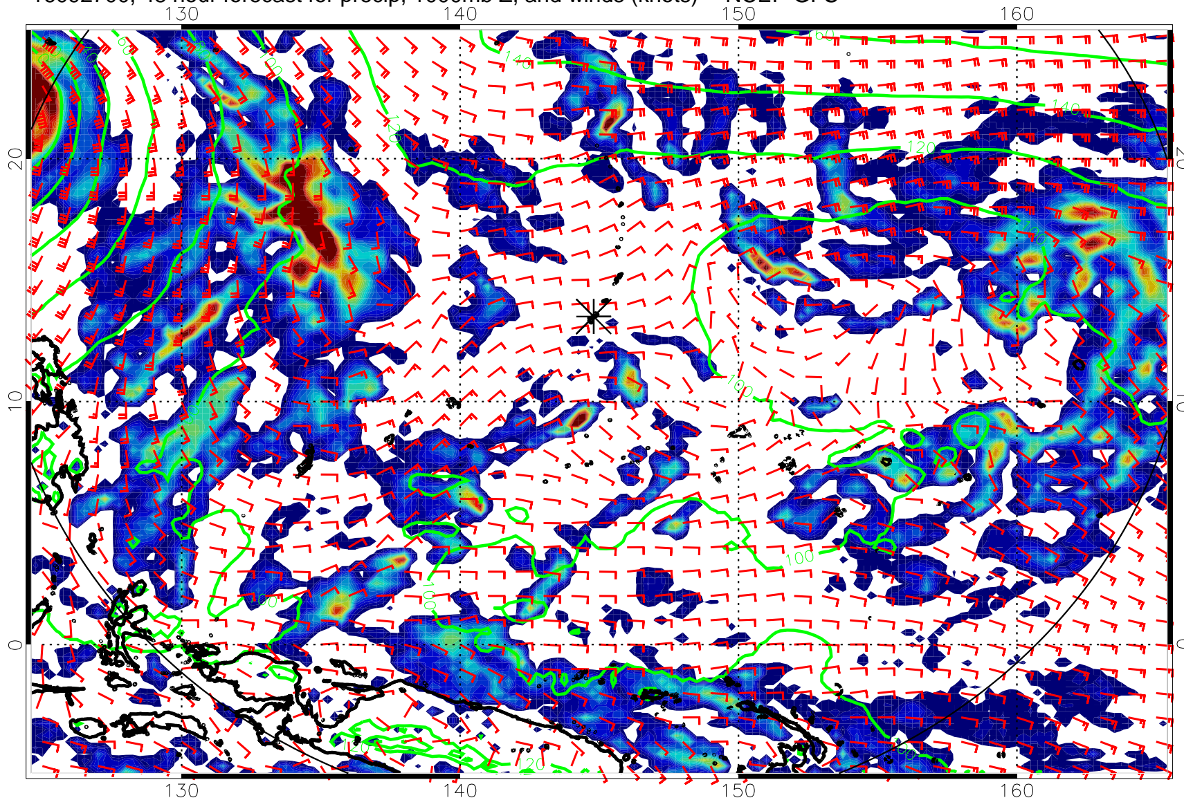
16092700, 48 hour forecast for precip, 1000mb Z, and winds (knots) -- NCEP GFS
