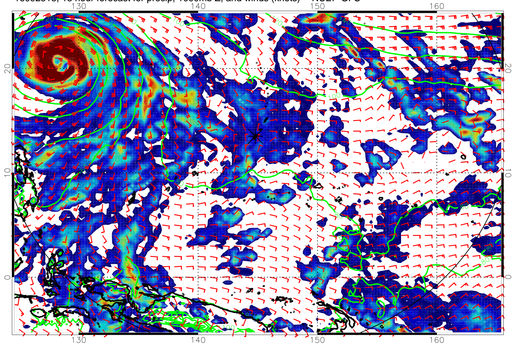
16092518, 18 hour forecast for precip, 1000mb Z, and winds (knots) -- NCEP GFS
