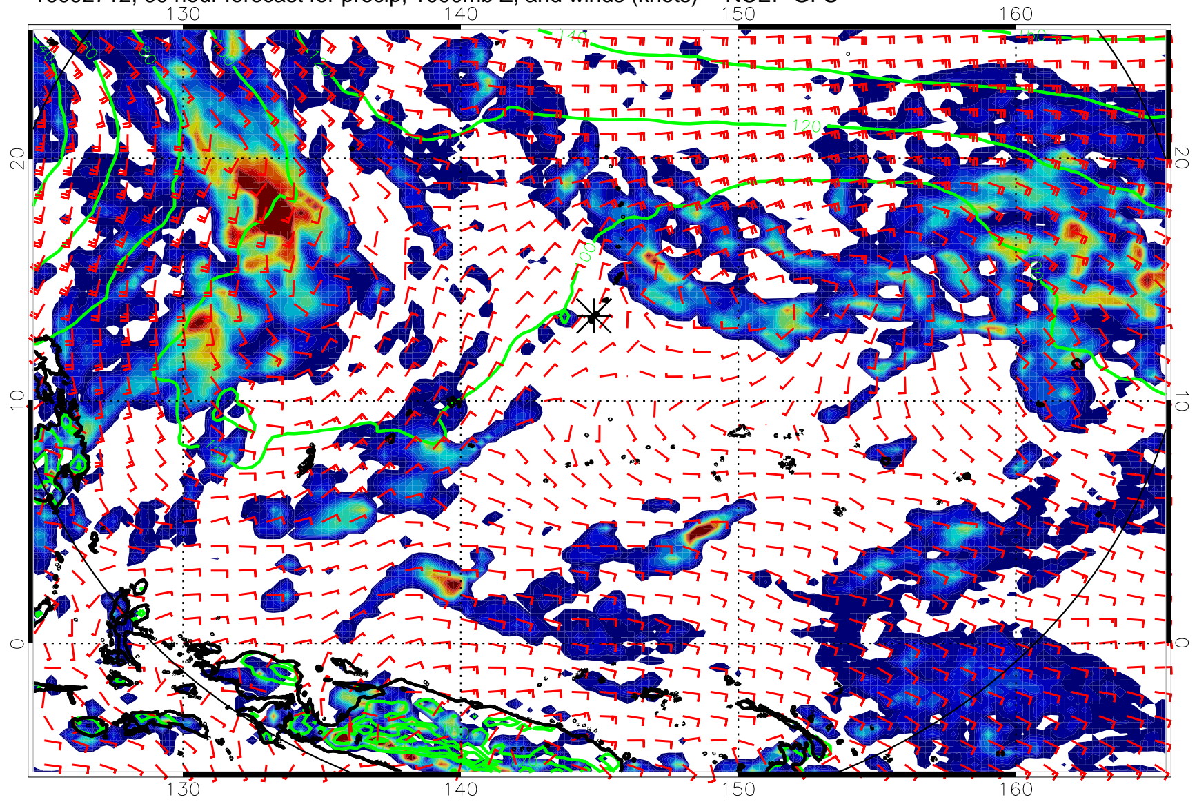
16092712, 60 hour forecast for precip, 1000mb Z, and winds (knots) -- NCEP GFS
