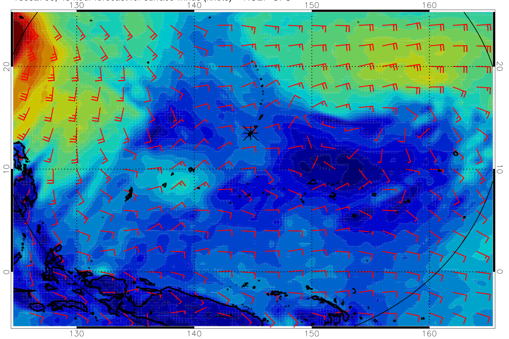
16092700, 48 hour forecast for surface winds (knots) -- NCEP GFS
