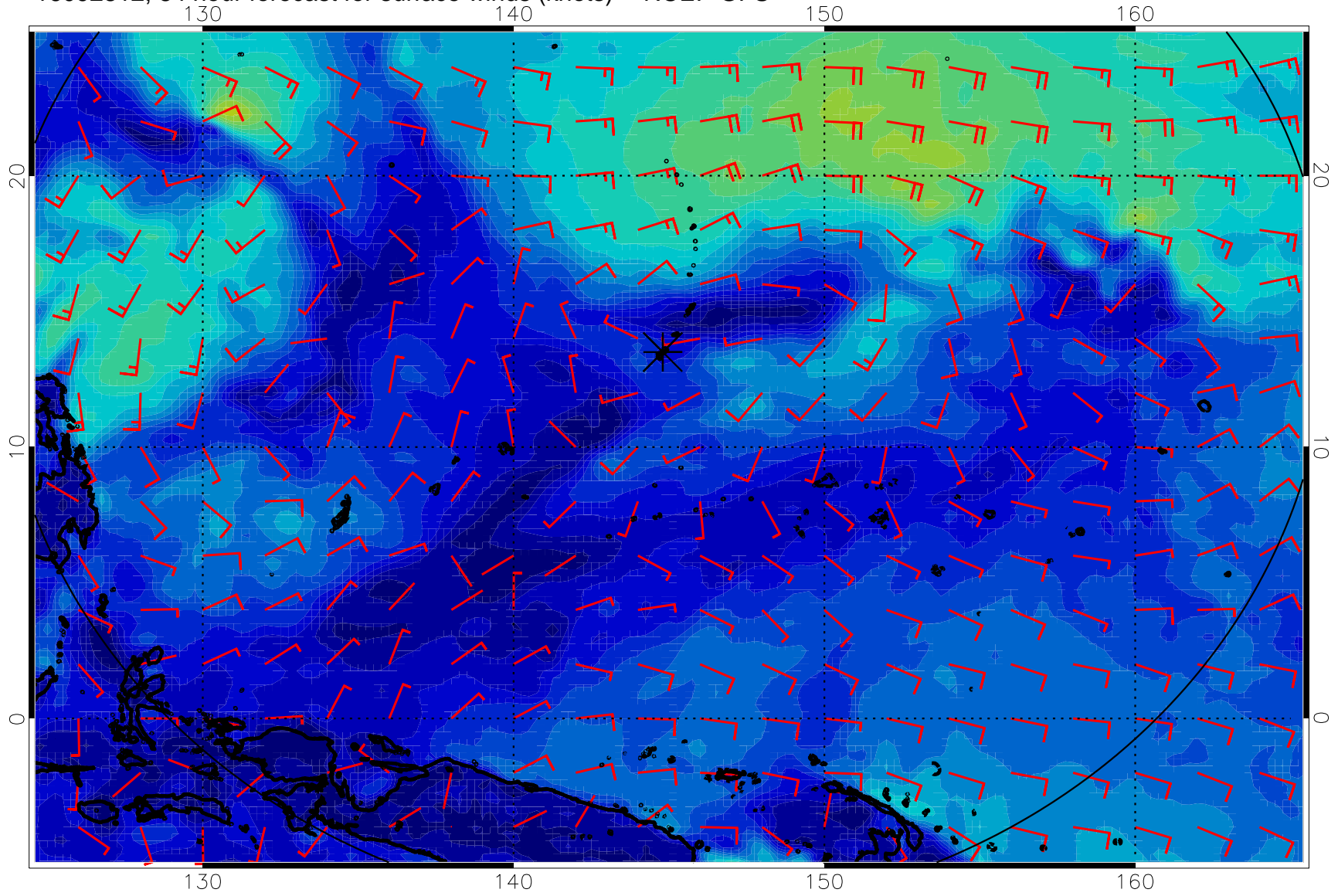
16092812, 84 hour forecast for surface winds (knots) -- NCEP GFS
