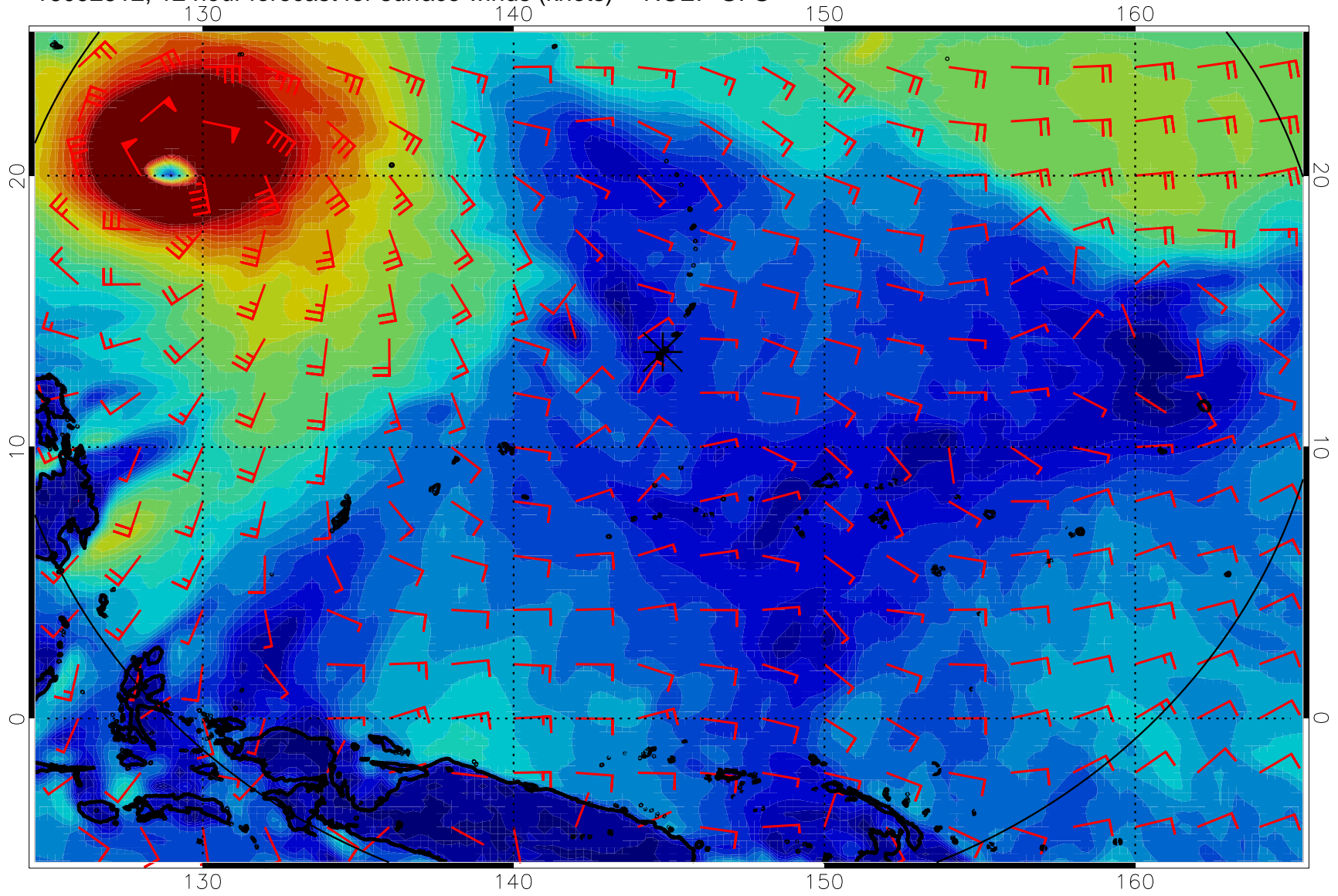
16092512, 12 hour forecast for surface winds (knots) -- NCEP GFS
