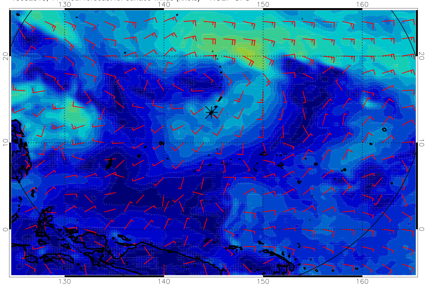
16092918, 114 hour forecast for surface winds (knots) -- NCEP GFS
