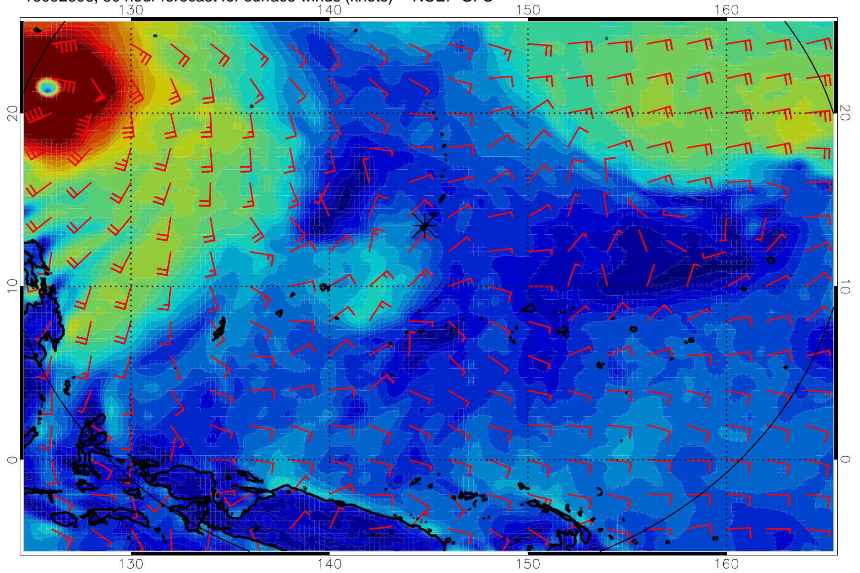
16092606, 30 hour forecast for surface winds (knots) -- NCEP GFS
