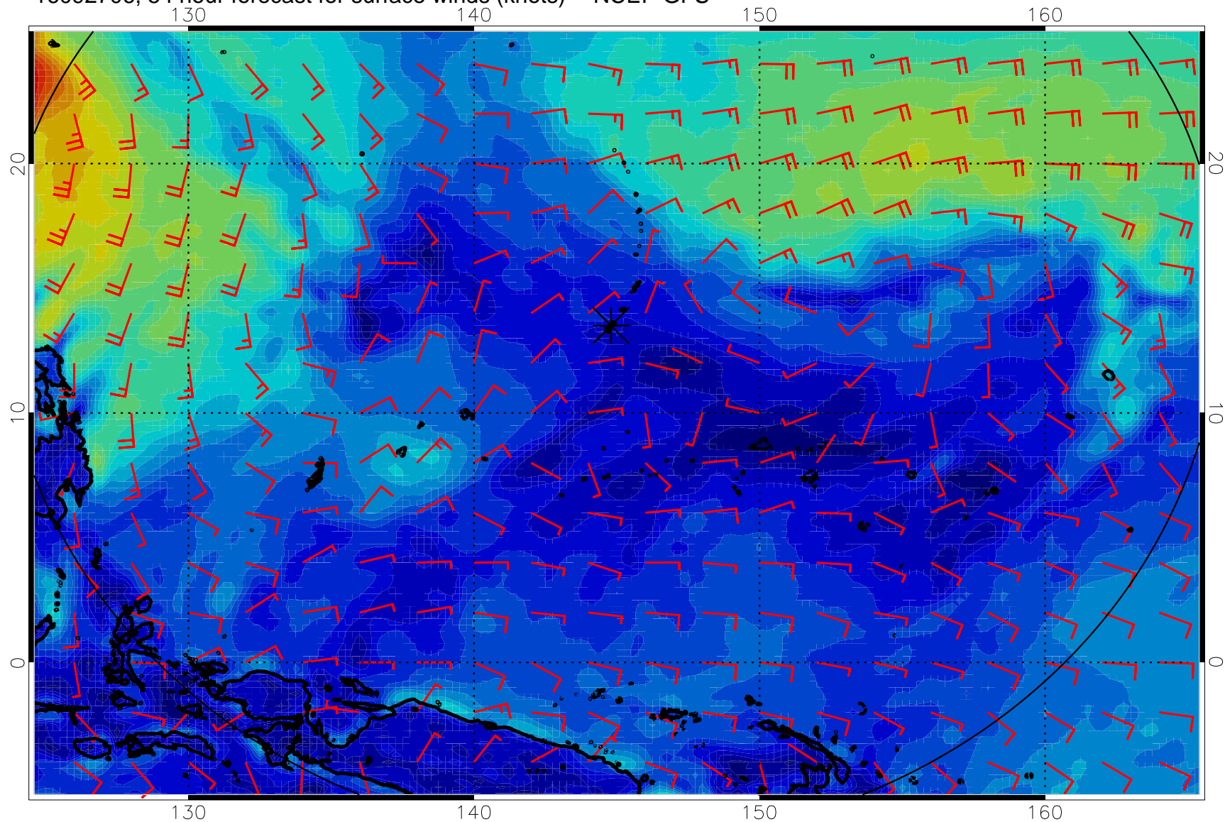
16092706, 54 hour forecast for surface winds (knots) -- NCEP GFS
