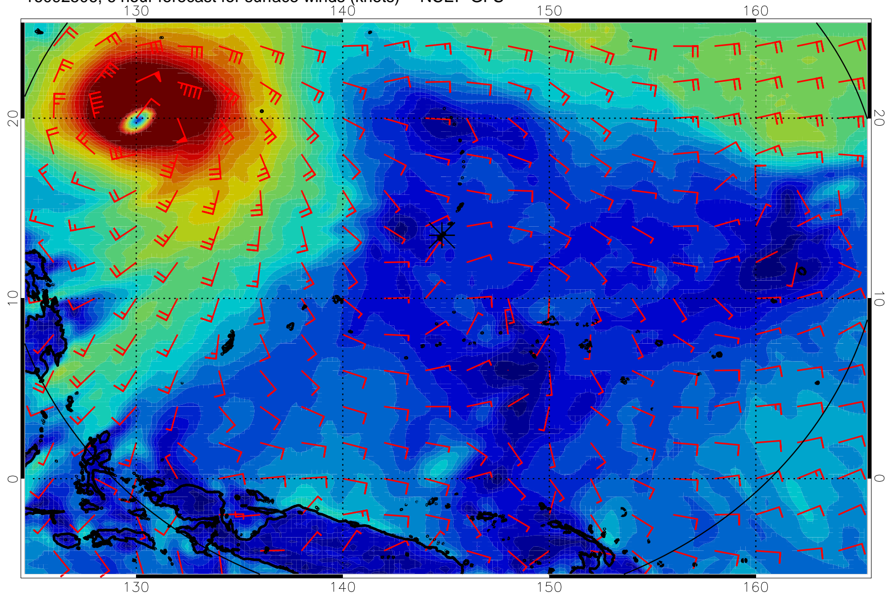
16092506, 6 hour forecast for surface winds (knots) -- NCEP GFS
