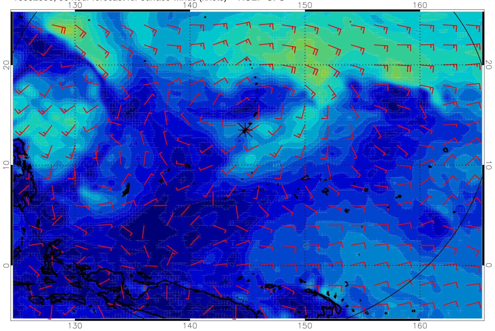
16092900, 96 hour forecast for surface winds (knots) -- NCEP GFS
