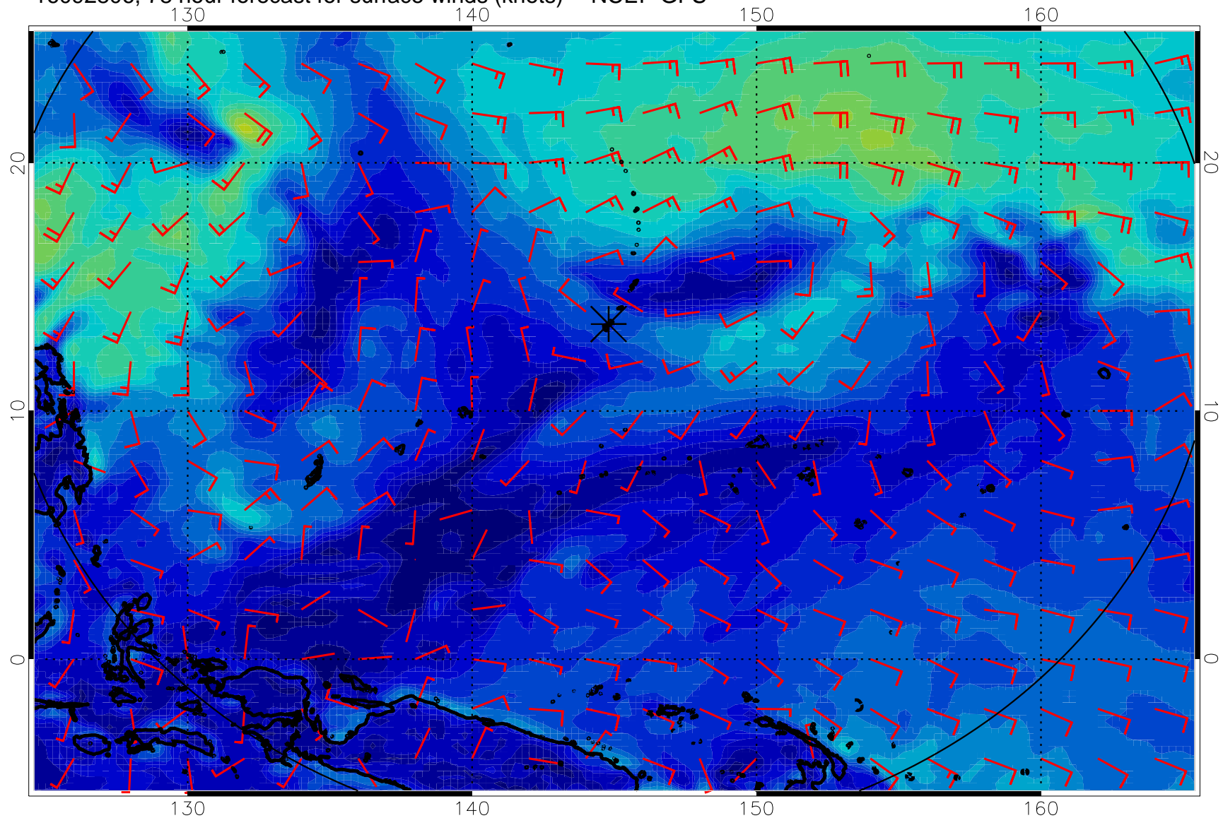
16092806, 78 hour forecast for surface winds (knots) -- NCEP GFS
