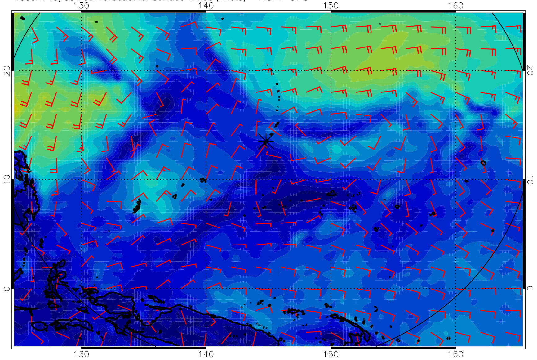
16092718, 66 hour forecast for surface winds (knots) -- NCEP GFS
