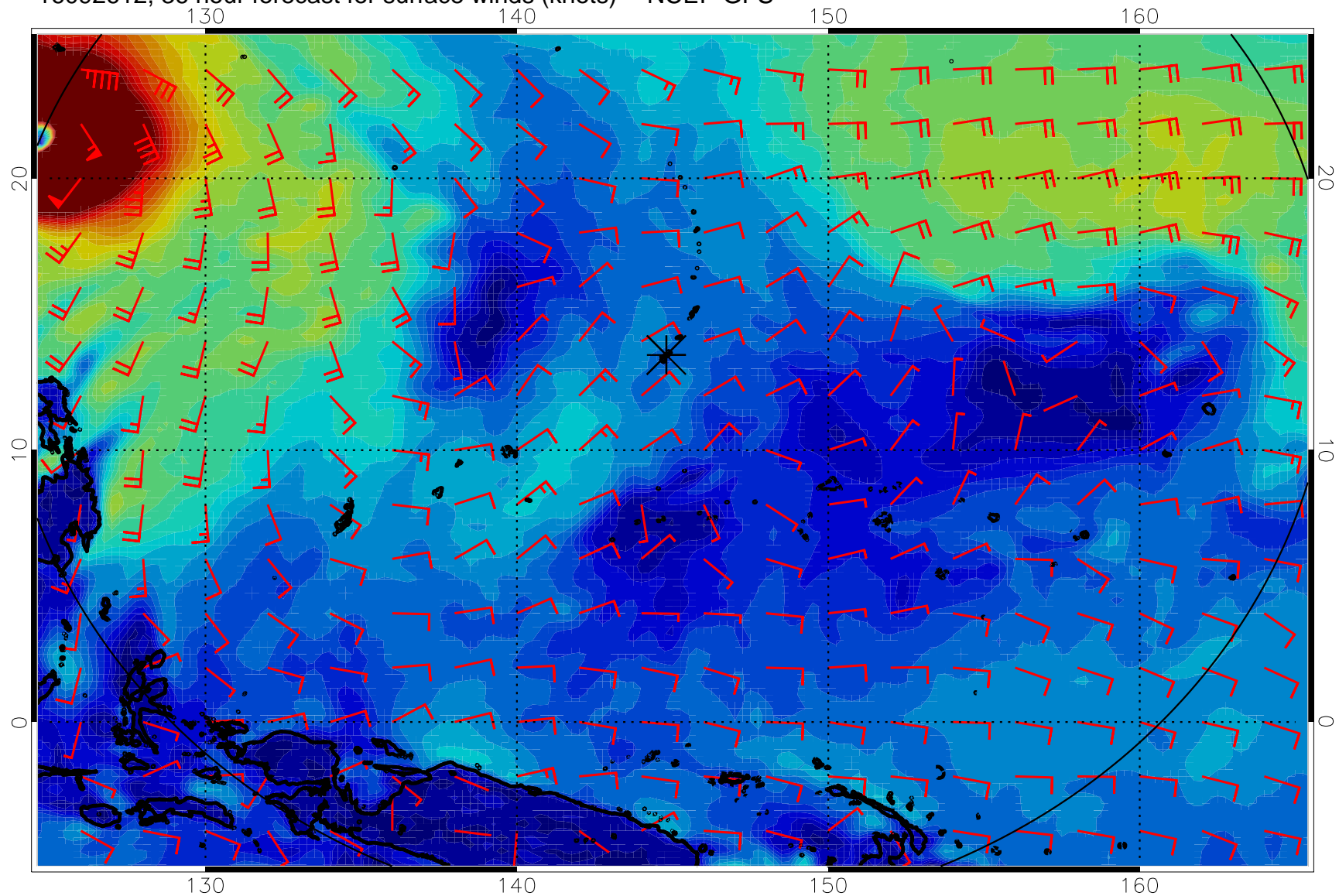
16092612, 36 hour forecast for surface winds (knots) -- NCEP GFS
