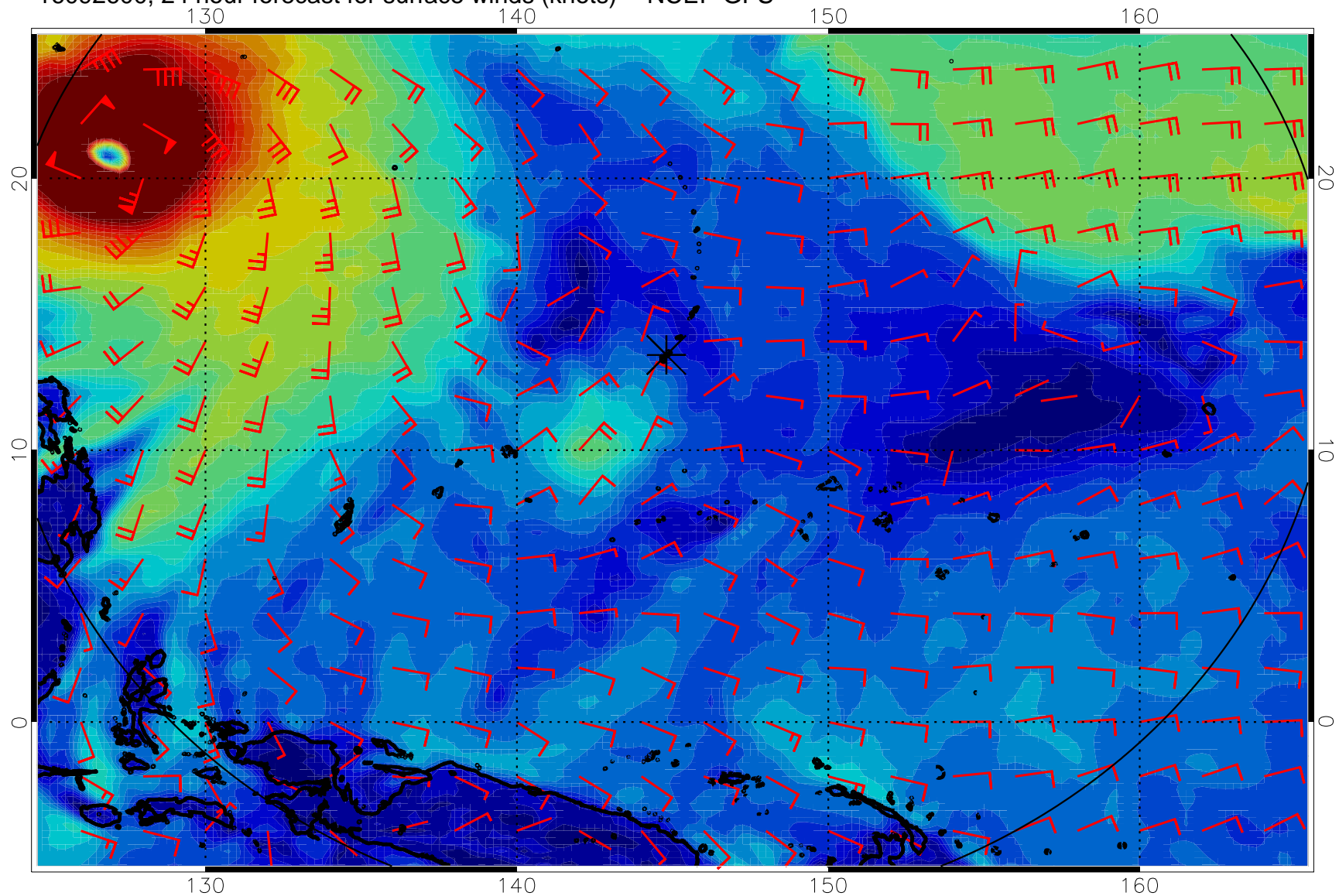
16092600, 24 hour forecast for surface winds (knots) -- NCEP GFS
