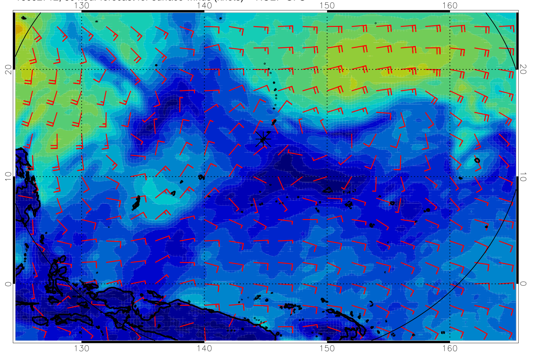
16092712, 60 hour forecast for surface winds (knots) -- NCEP GFS
