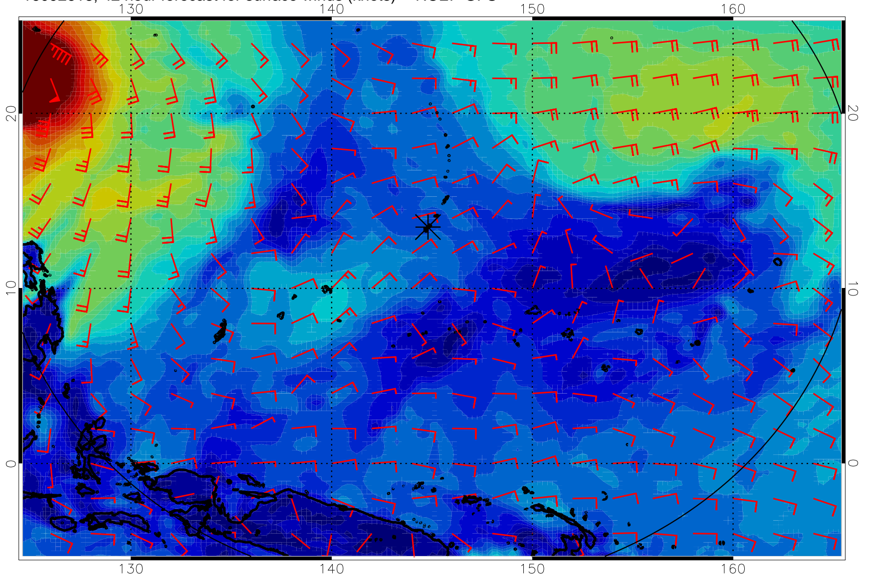
16092618, 42 hour forecast for surface winds (knots) -- NCEP GFS
