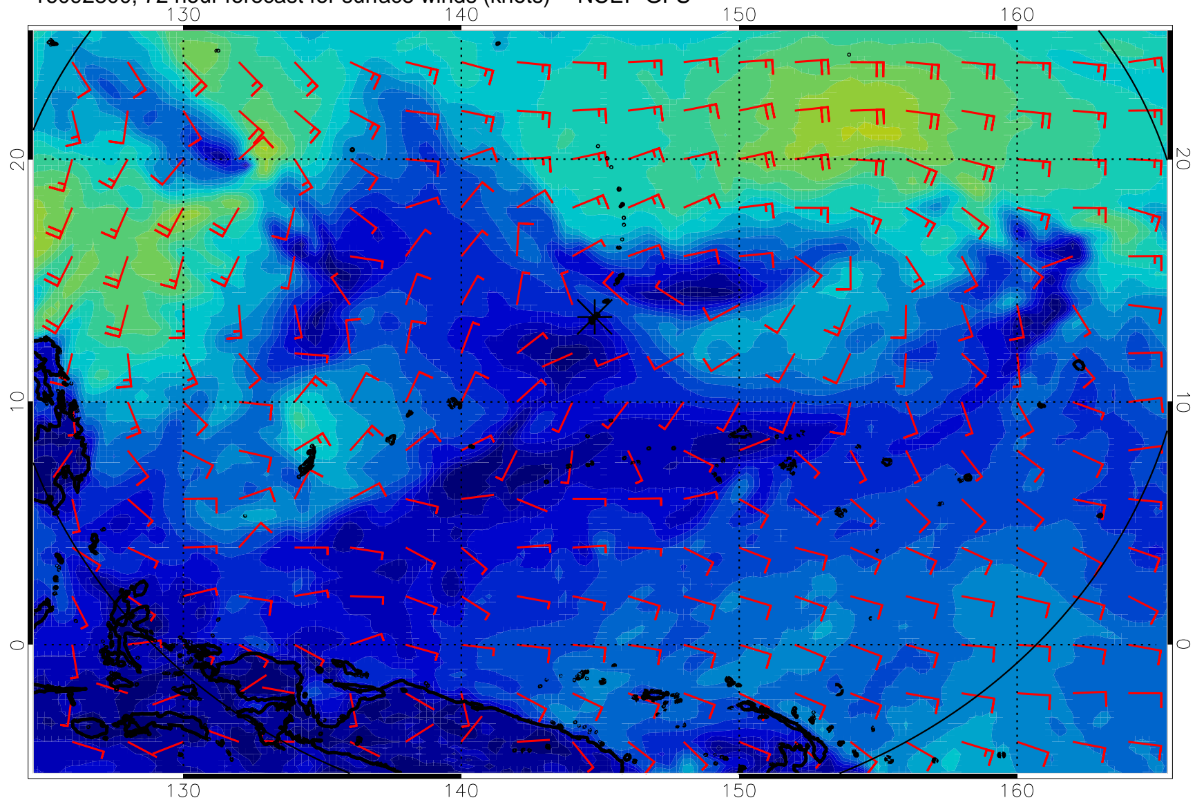
16092800, 72 hour forecast for surface winds (knots) -- NCEP GFS
