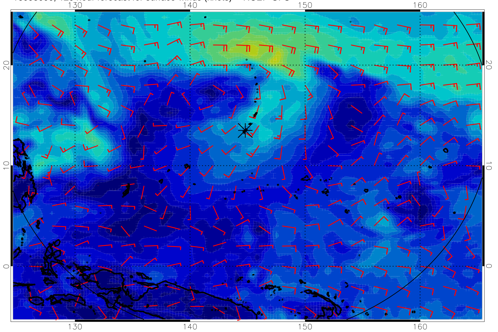
16093000, 120 hour forecast for surface winds (knots) -- NCEP GFS
