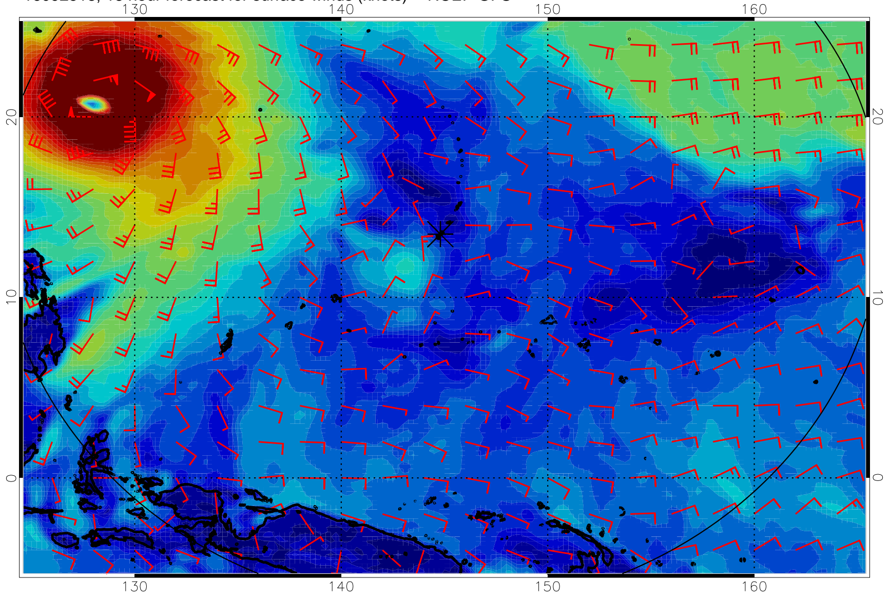
16092518, 18 hour forecast for surface winds (knots) -- NCEP GFS
