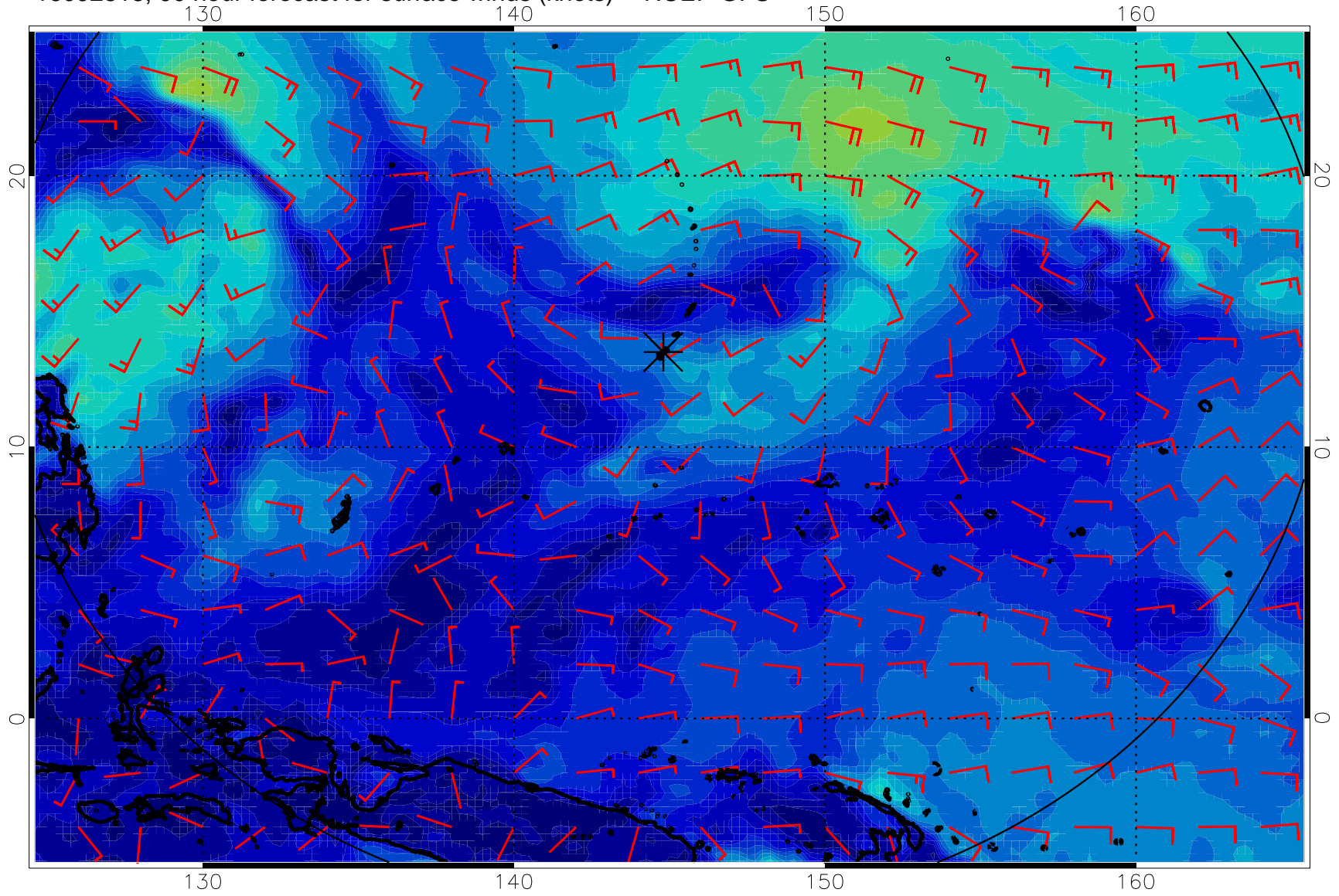
16092818, 90 hour forecast for surface winds (knots) -- NCEP GFS
