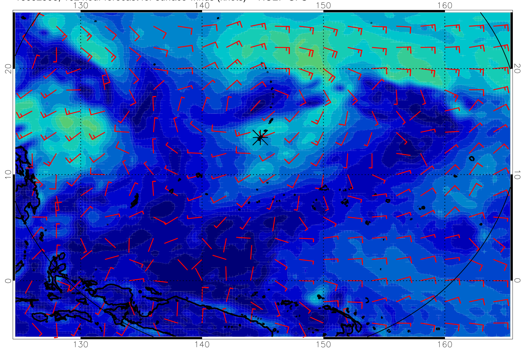
16092906, 102 hour forecast for surface winds (knots) -- NCEP GFS
