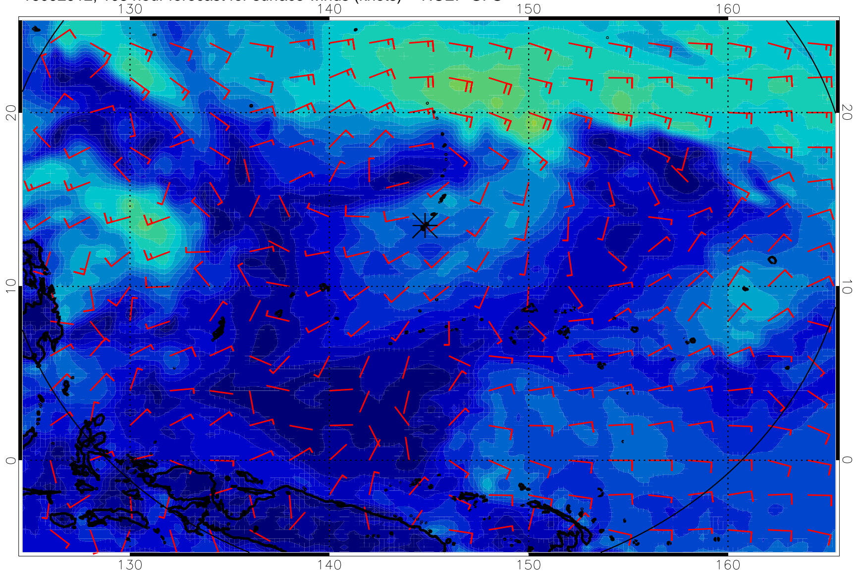
16092912, 108 hour forecast for surface winds (knots) -- NCEP GFS
