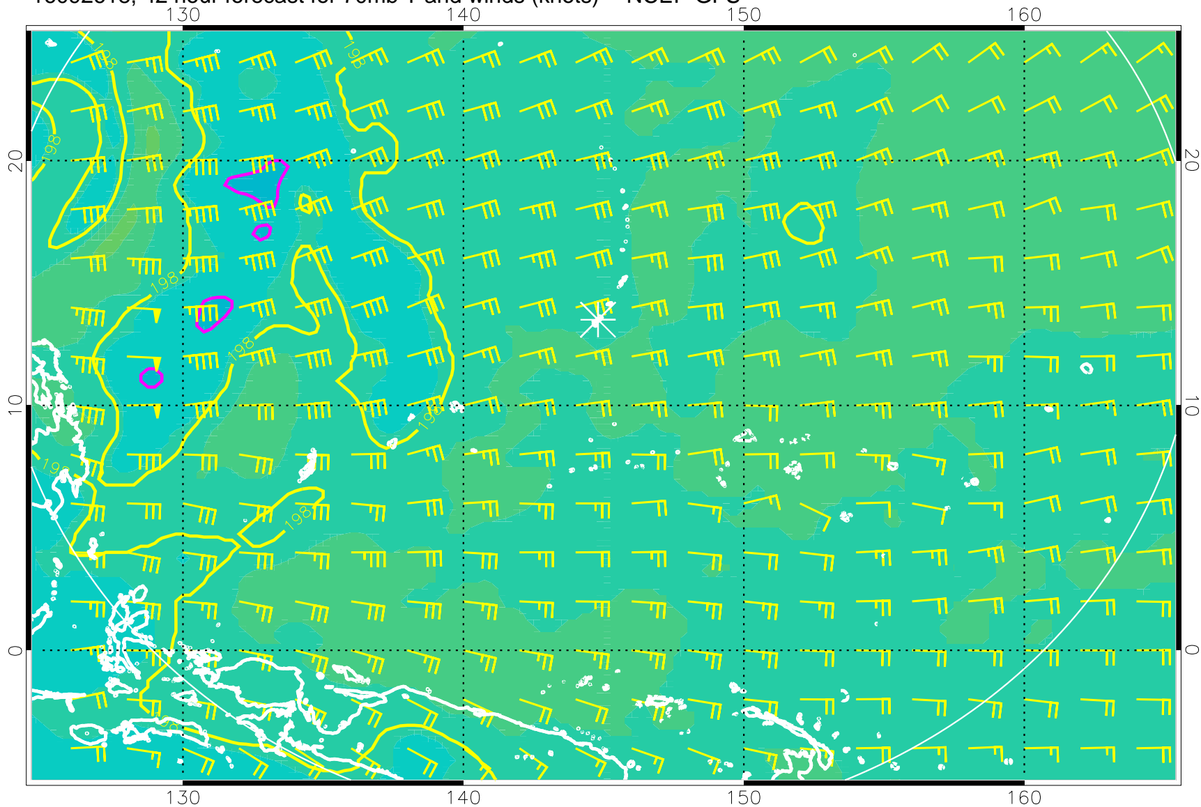
16092618, 42 hour forecast for 70mb T and winds (knots) -- NCEP GFS
