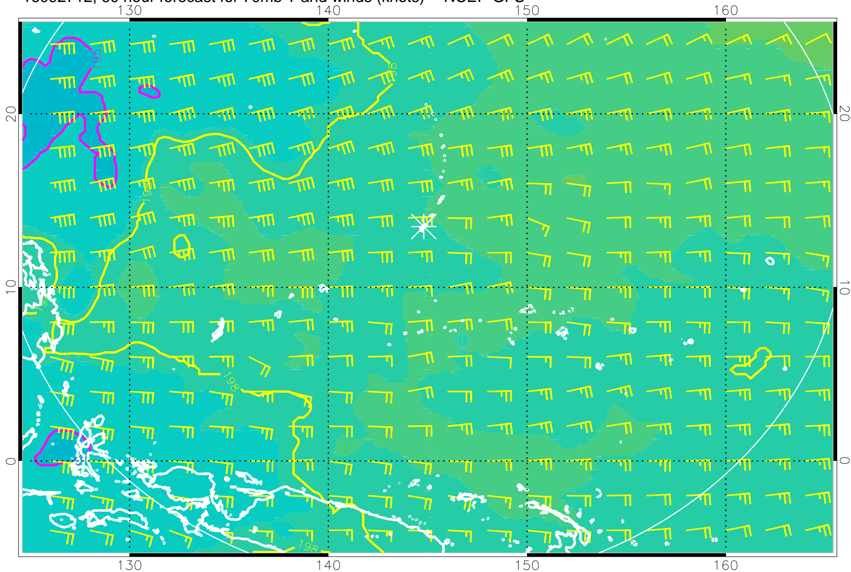
16092712, 60 hour forecast for 70mb T and winds (knots) -- NCEP GFS
