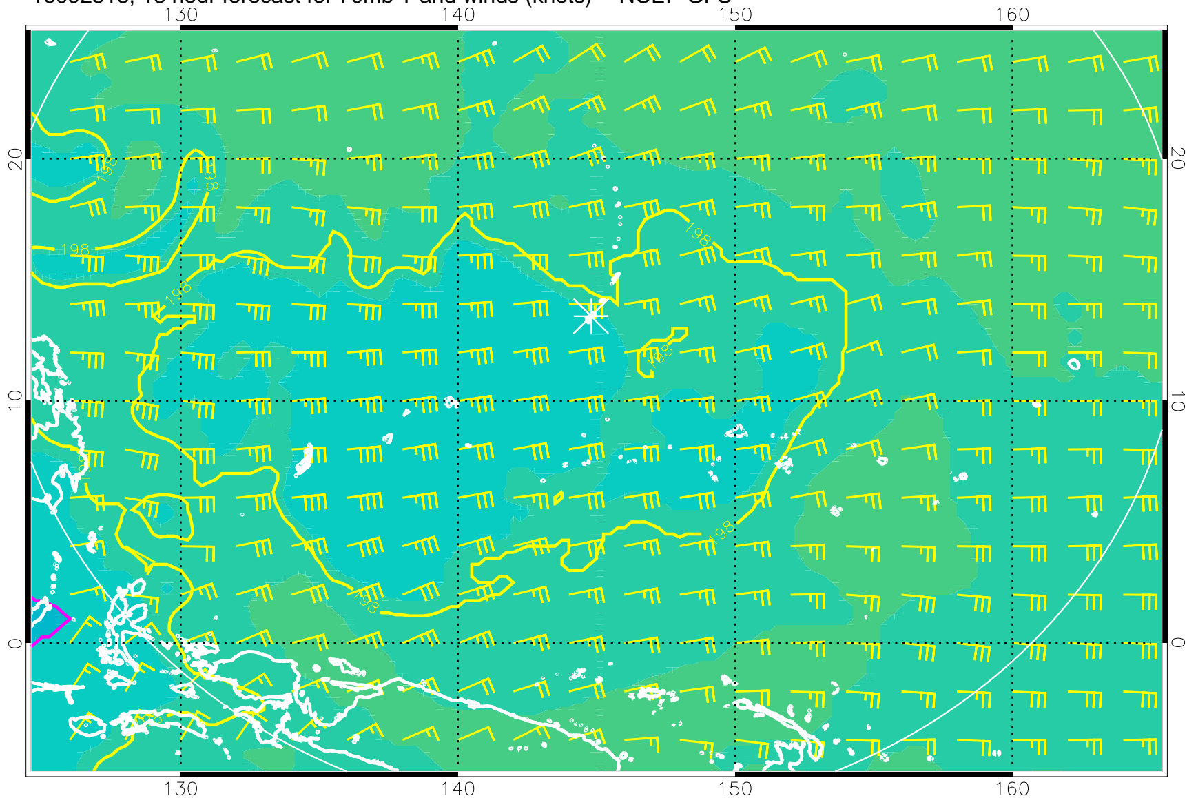
16092518, 18 hour forecast for 70mb T and winds (knots) -- NCEP GFS
