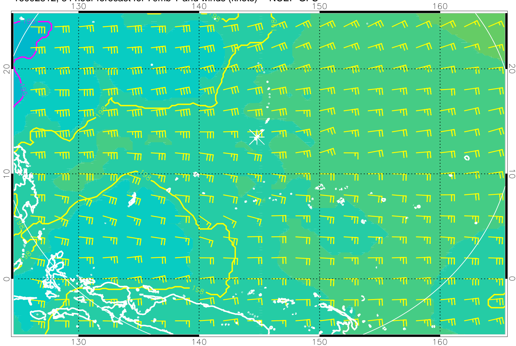
16092812, 84 hour forecast for 70mb T and winds (knots) -- NCEP GFS
