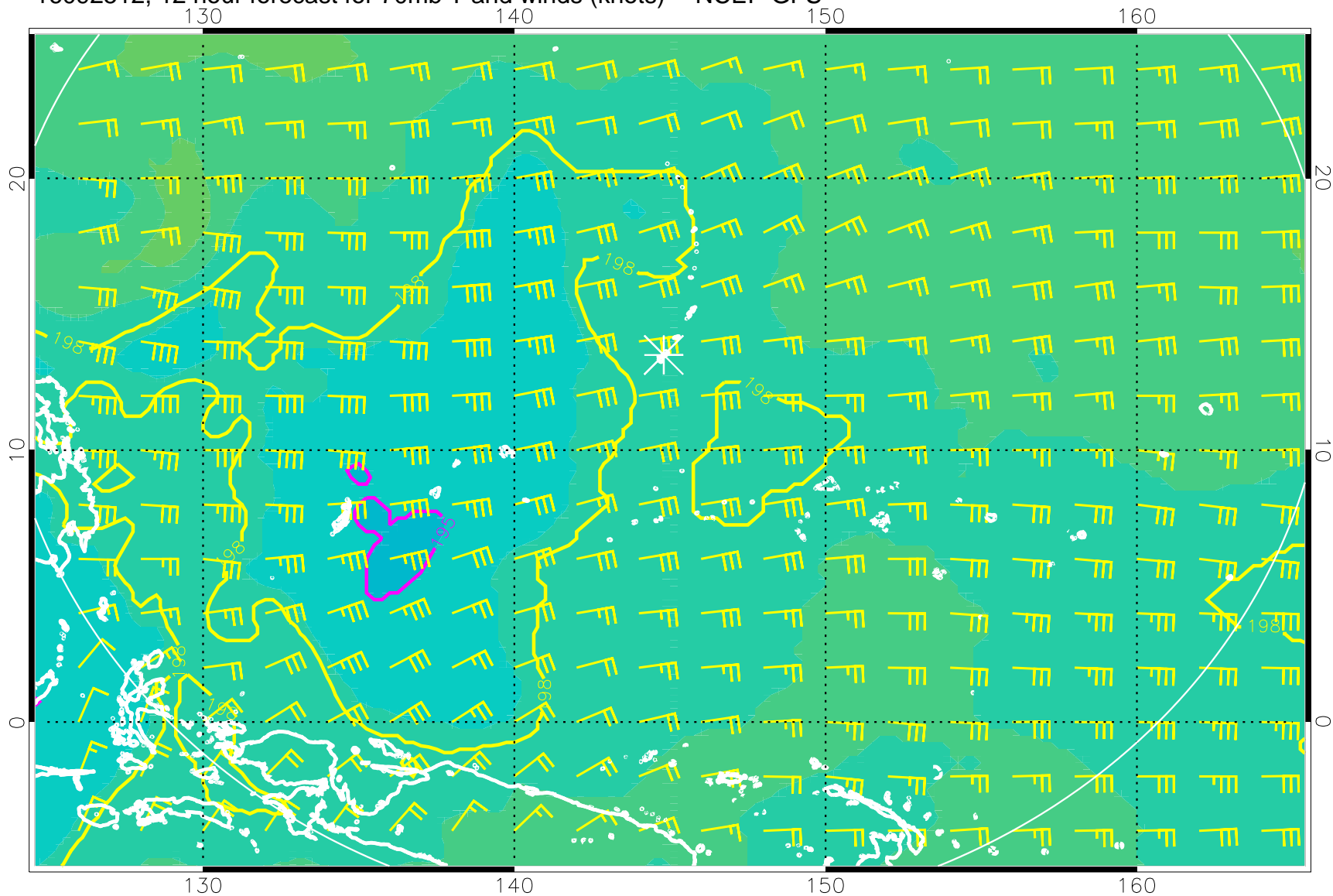
16092512, 12 hour forecast for 70mb T and winds (knots) -- NCEP GFS
