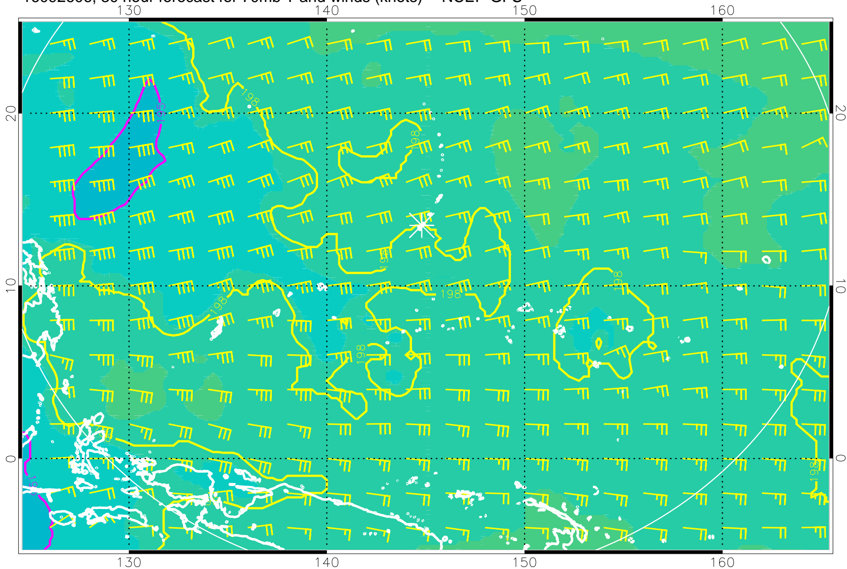
16092606, 30 hour forecast for 70mb T and winds (knots) -- NCEP GFS
