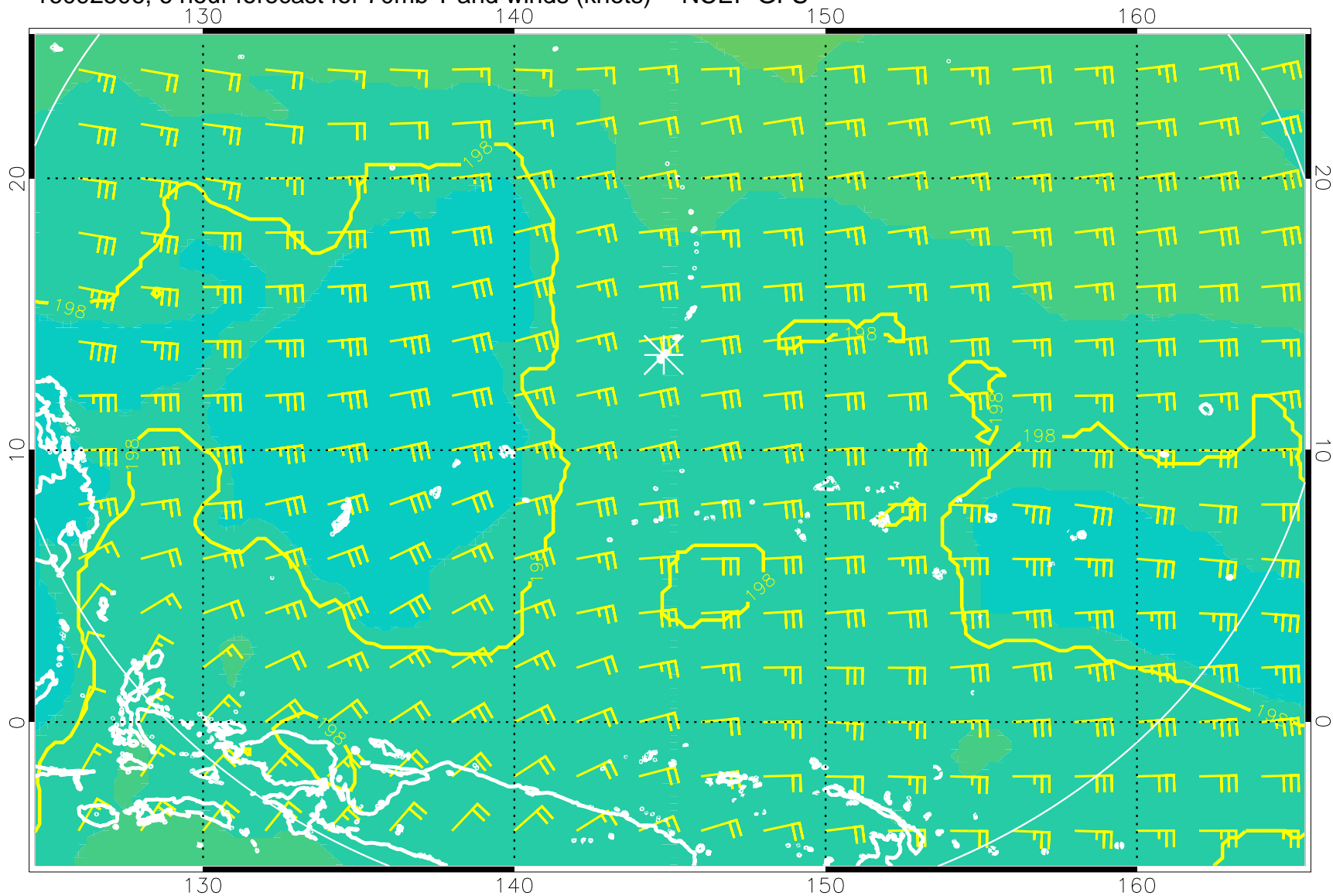
16092506, 6 hour forecast for 70mb T and winds (knots) -- NCEP GFS
