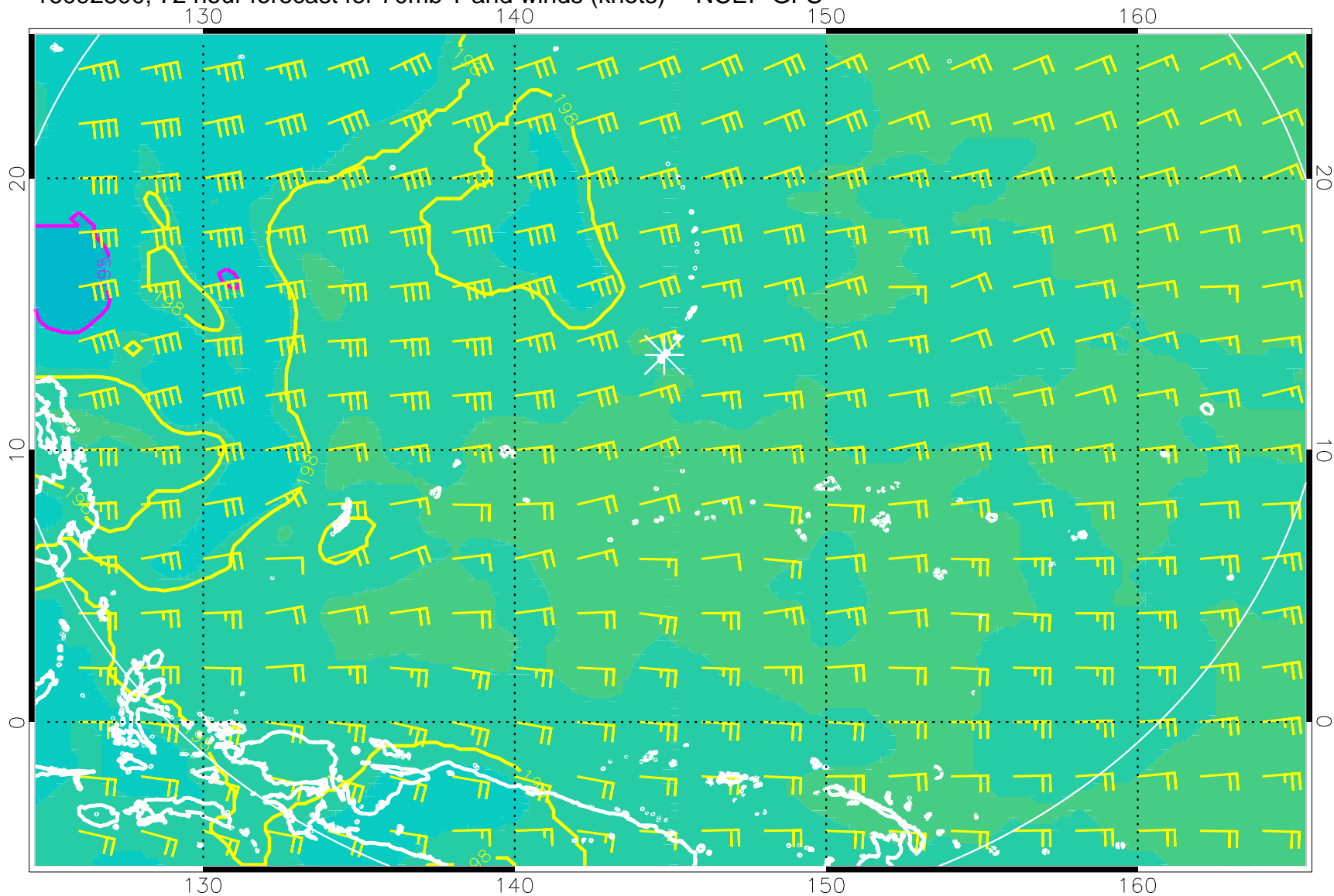
16092800, 72 hour forecast for 70mb T and winds (knots) -- NCEP GFS
