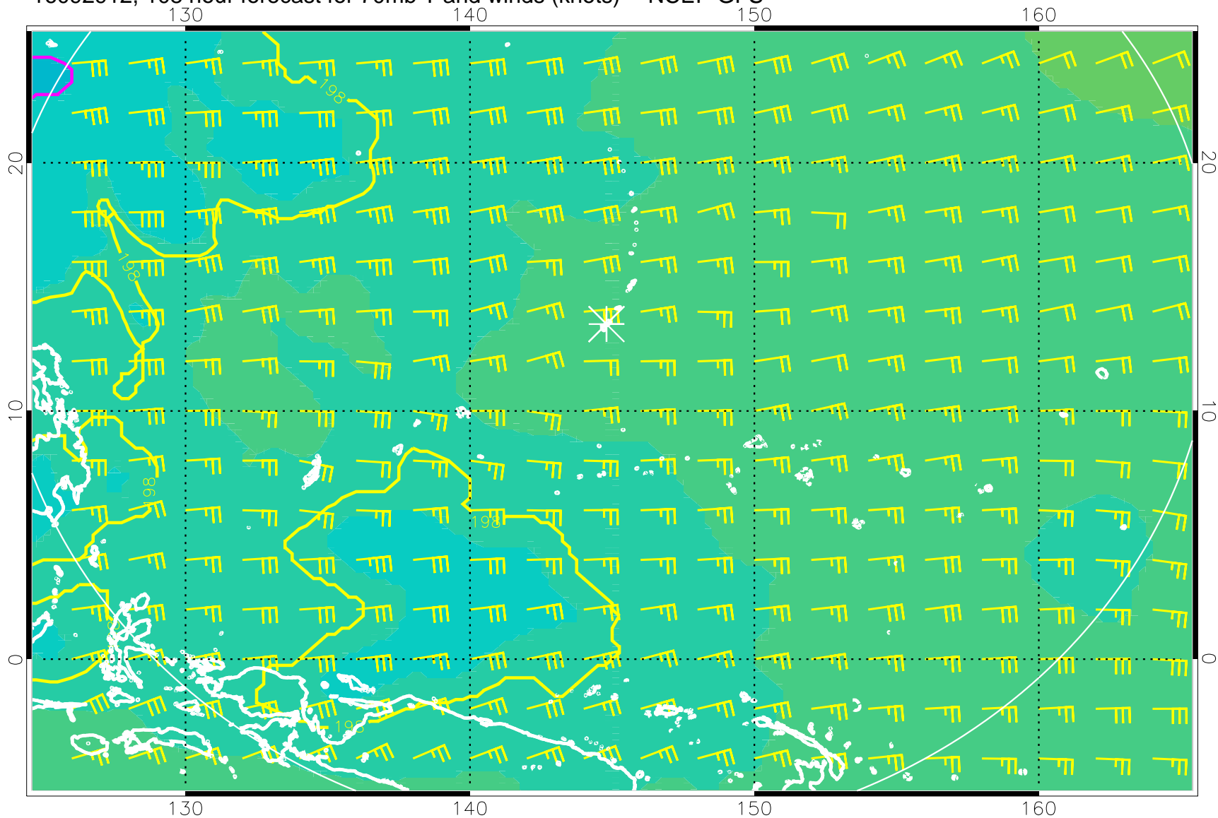
16092912, 108 hour forecast for 70mb T and winds (knots) -- NCEP GFS
