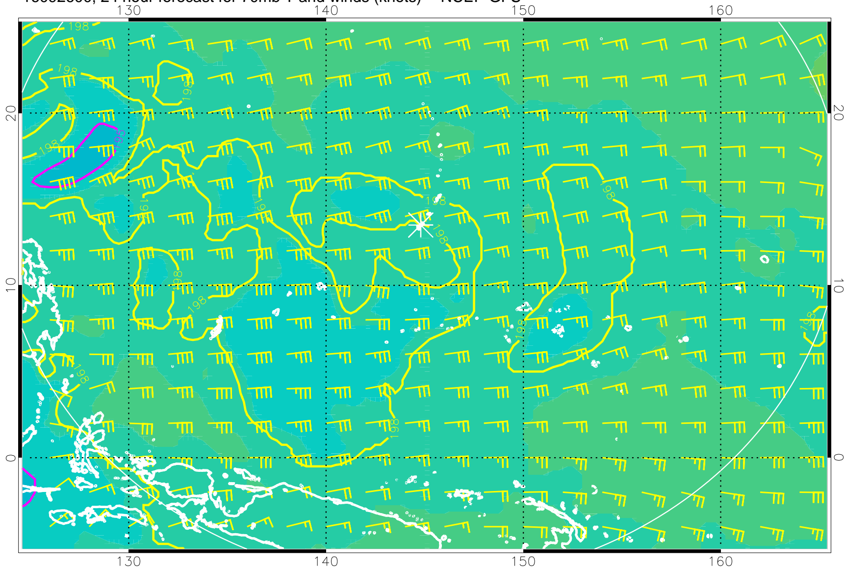
16092600, 24 hour forecast for 70mb T and winds (knots) -- NCEP GFS
