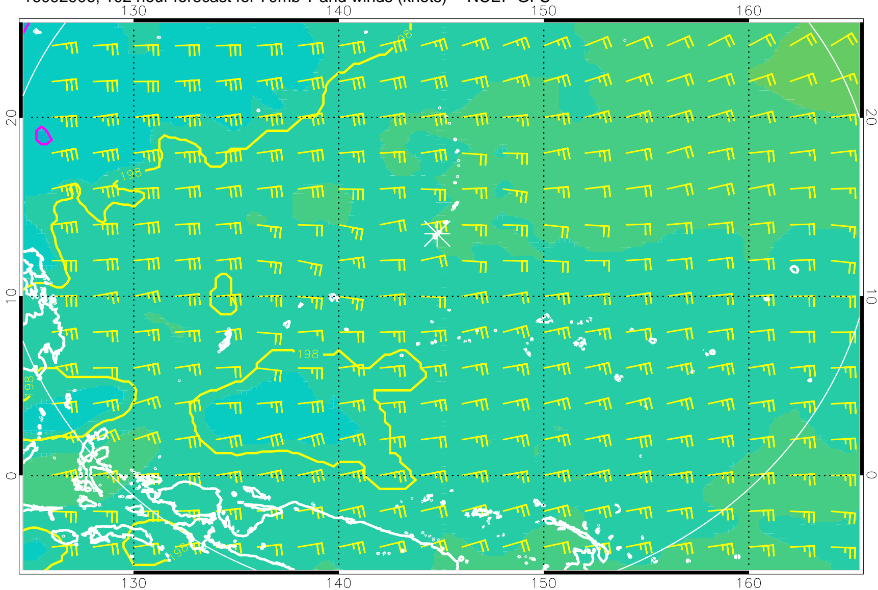
16092906, 102 hour forecast for 70mb T and winds (knots) -- NCEP GFS
