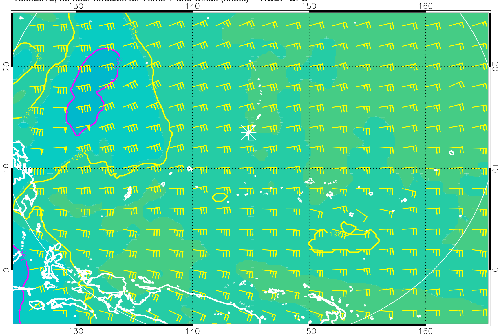
16092612, 36 hour forecast for 70mb T and winds (knots) -- NCEP GFS
