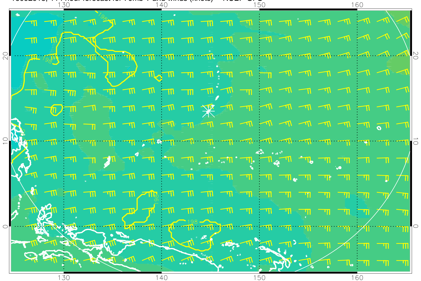
16092918, 114 hour forecast for 70mb T and winds (knots) -- NCEP GFS
