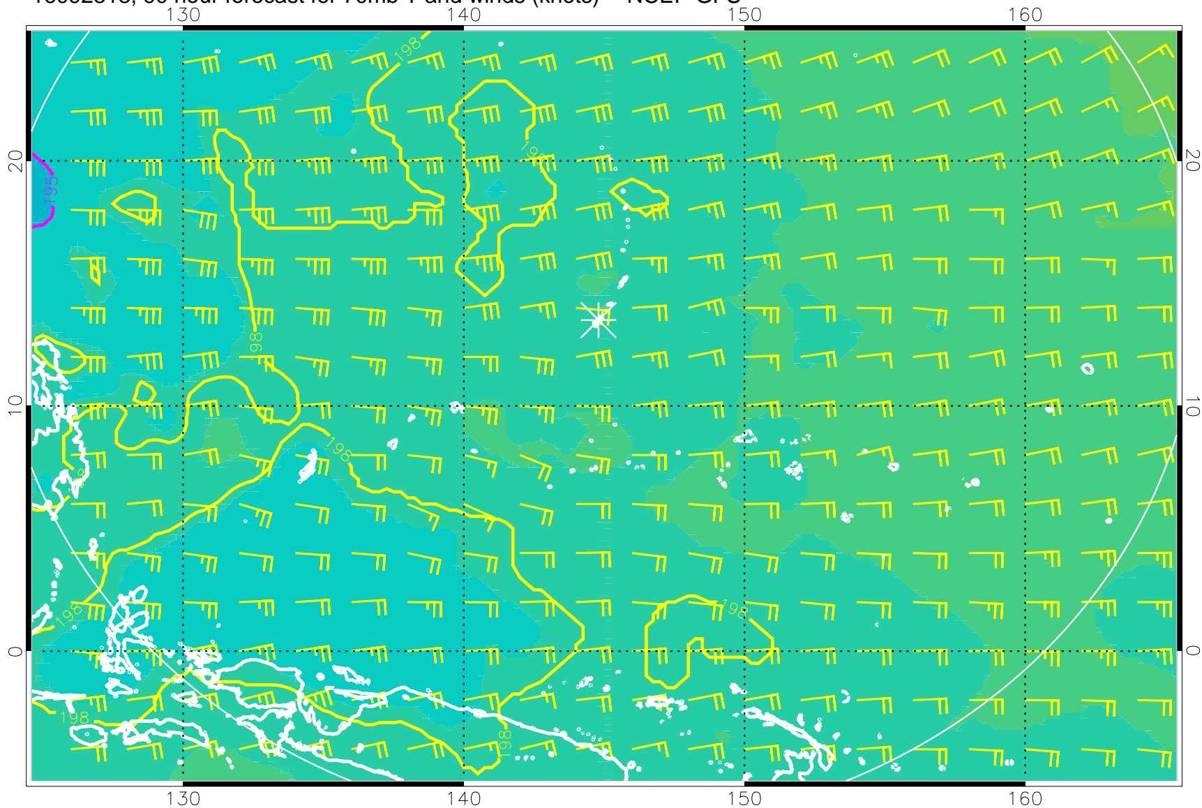
16092818, 90 hour forecast for 70mb T and winds (knots) -- NCEP GFS
