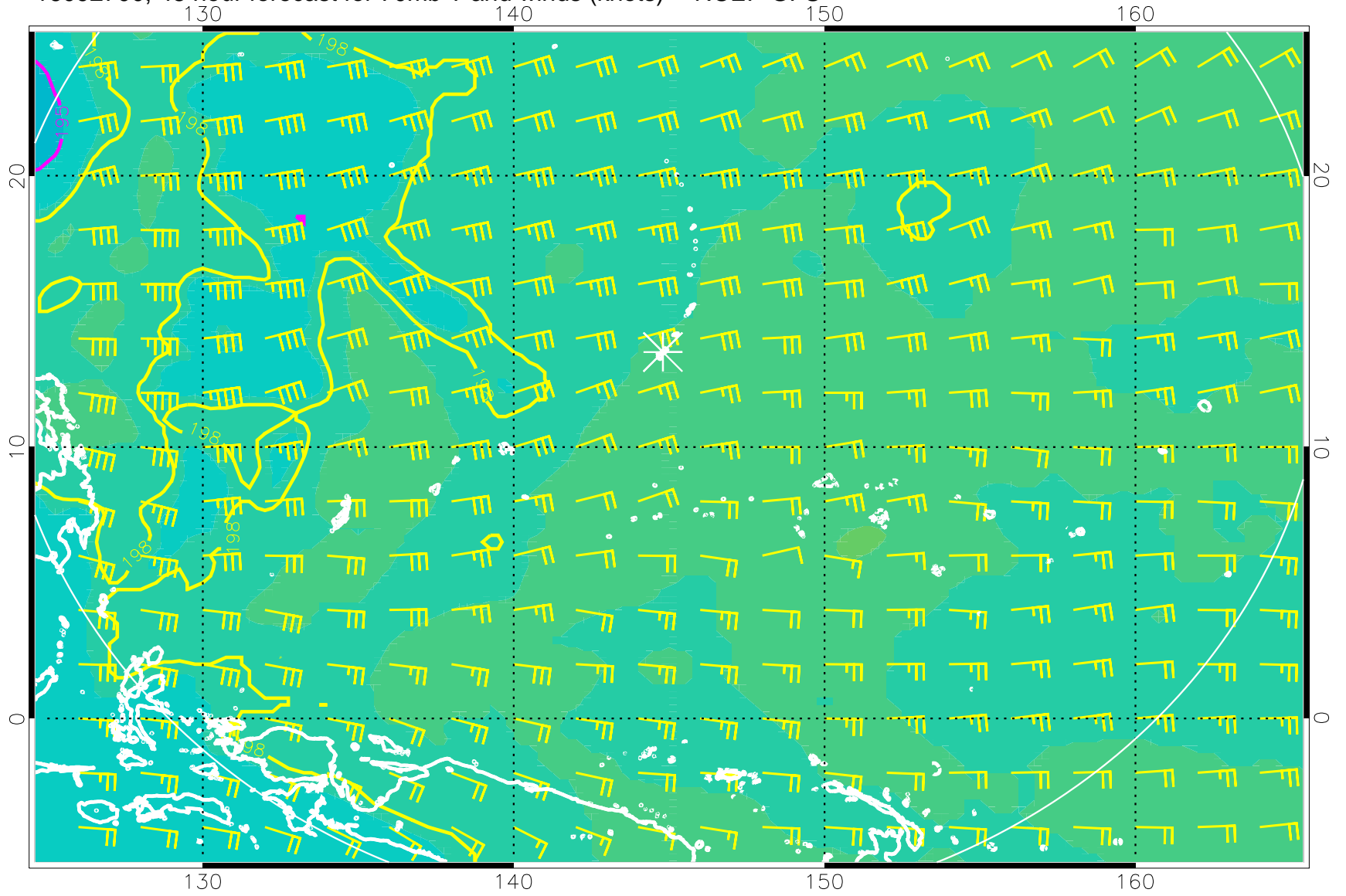
16092700, 48 hour forecast for 70mb T and winds (knots) -- NCEP GFS
