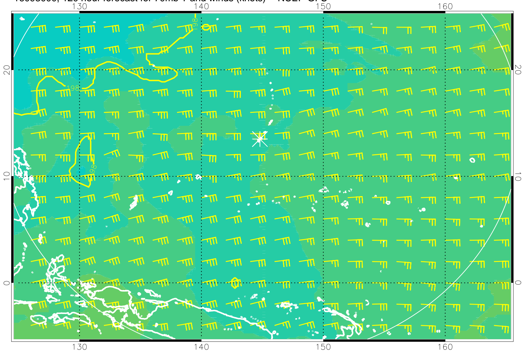
16093000, 120 hour forecast for 70mb T and winds (knots) -- NCEP GFS
