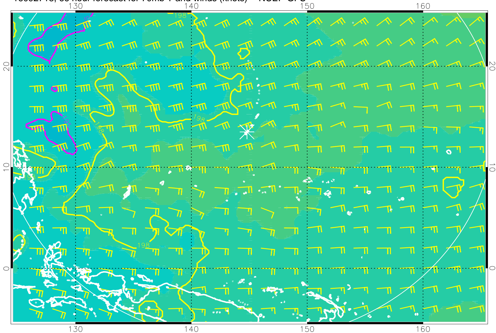
16092718, 66 hour forecast for 70mb T and winds (knots) -- NCEP GFS
