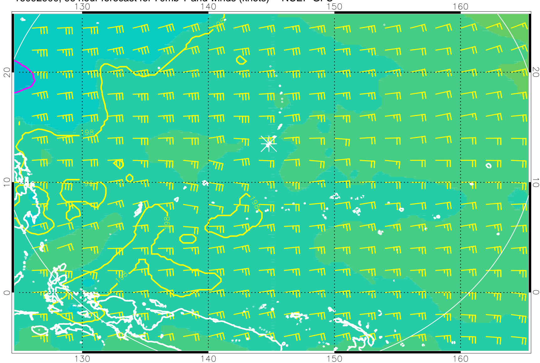
16092900, 96 hour forecast for 70mb T and winds (knots) -- NCEP GFS
