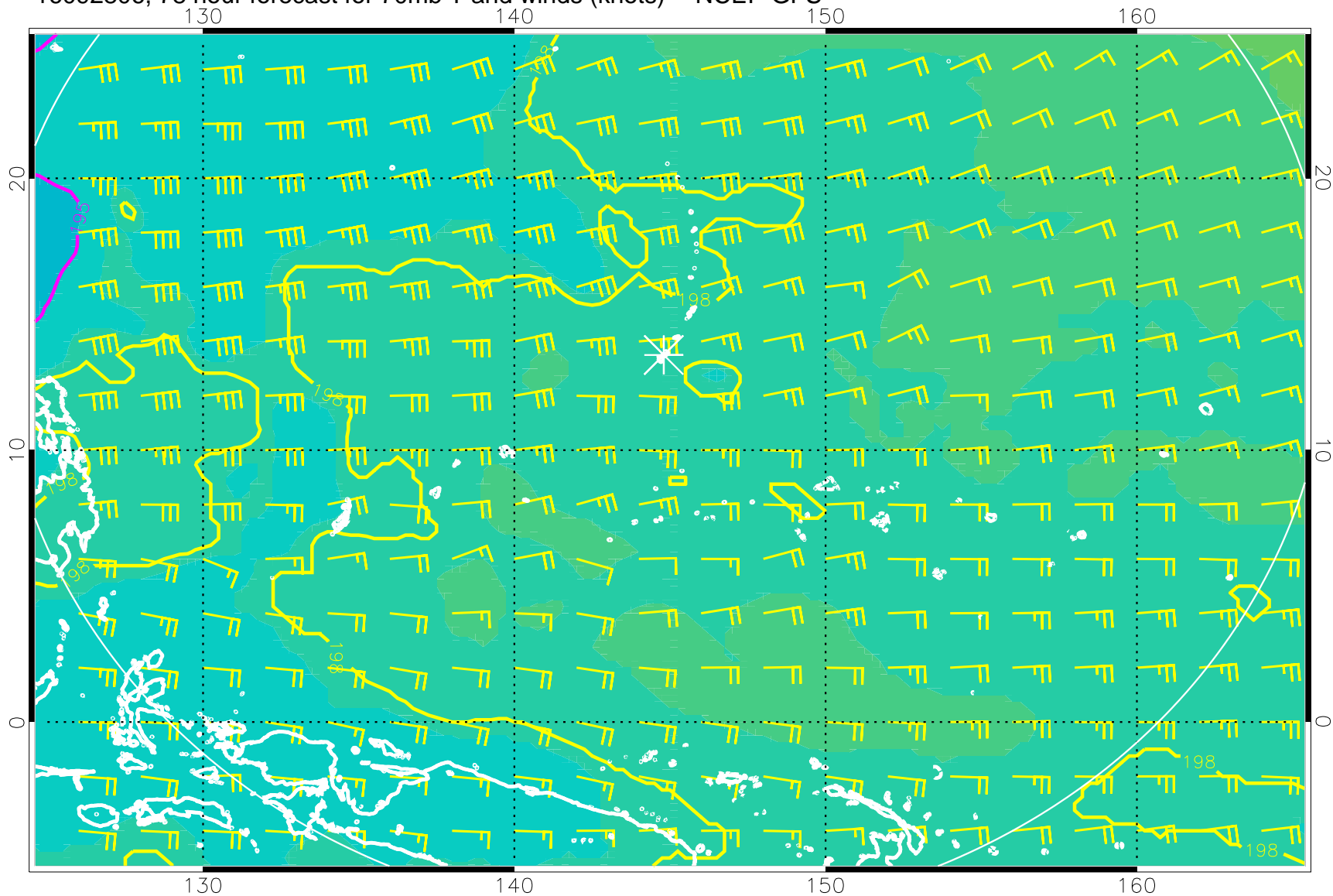
16092806, 78 hour forecast for 70mb T and winds (knots) -- NCEP GFS
