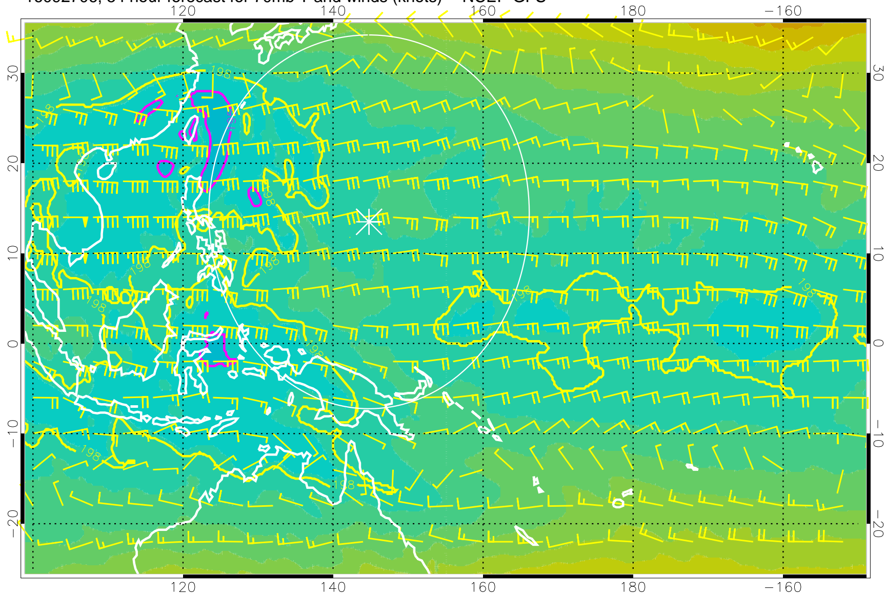
16092706, 54 hour forecast for 70mb T and winds (knots) -- NCEP GFS
