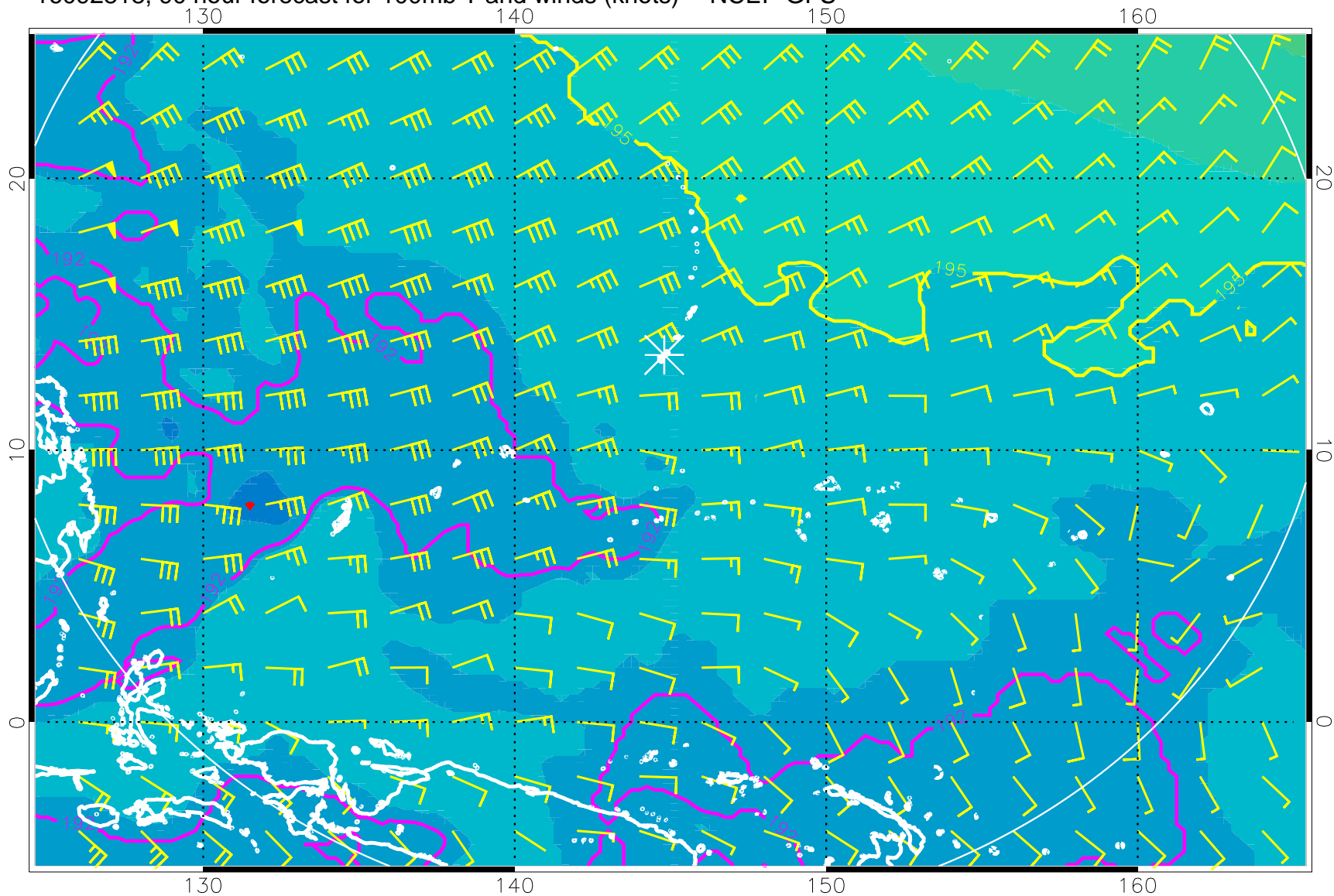
16092818, 90 hour forecast for 100mb T and winds (knots) -- NCEP GFS
