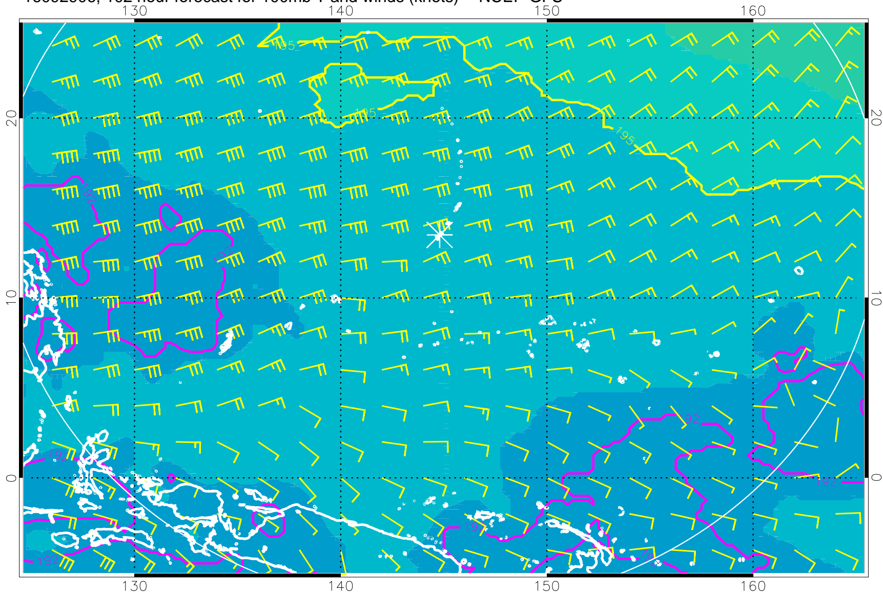
16092906, 102 hour forecast for 100mb T and winds (knots) -- NCEP GFS
