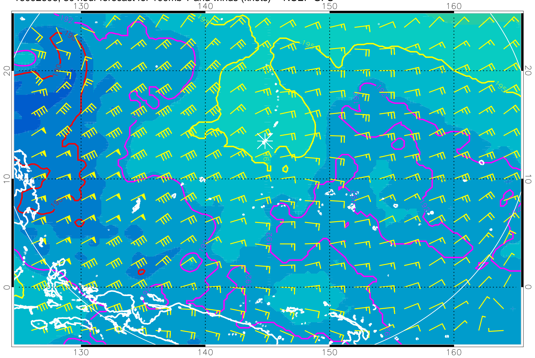
16092606, 30 hour forecast for 100mb T and winds (knots) -- NCEP GFS
