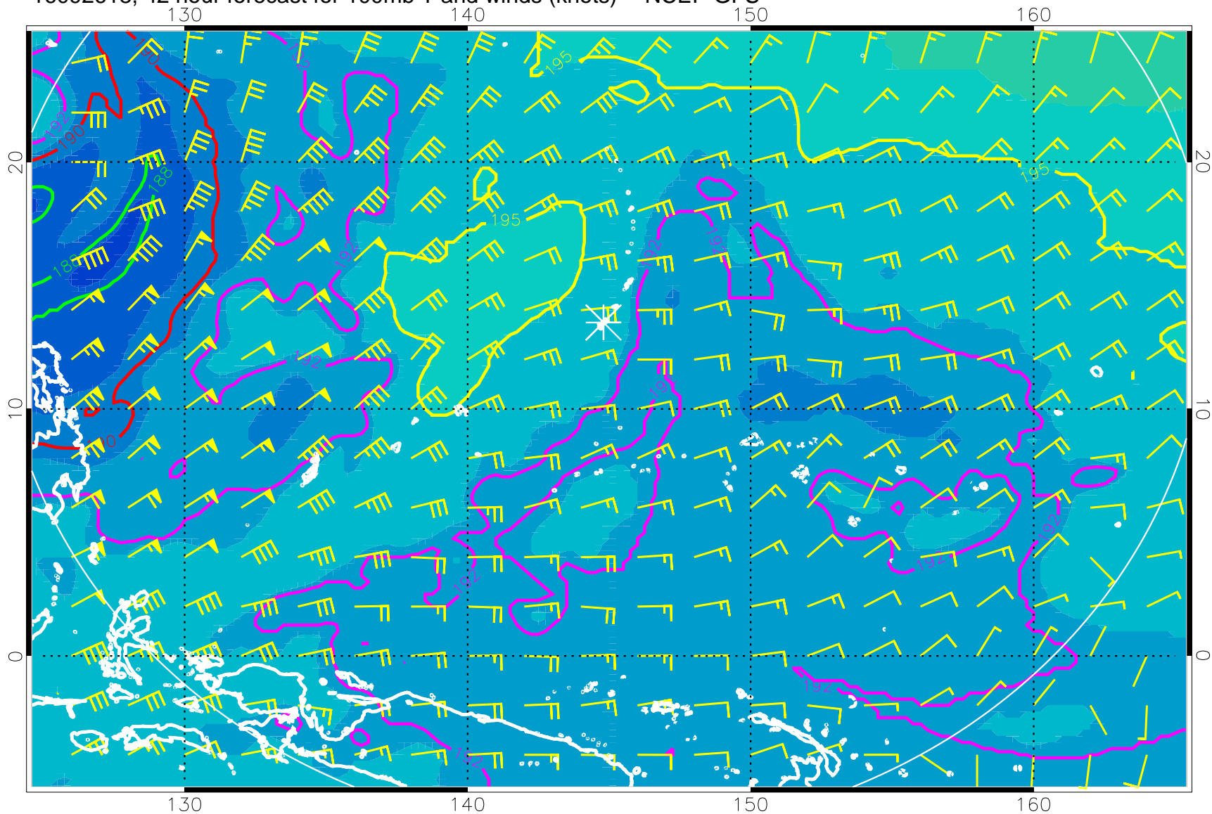
16092618, 42 hour forecast for 100mb T and winds (knots) -- NCEP GFS
