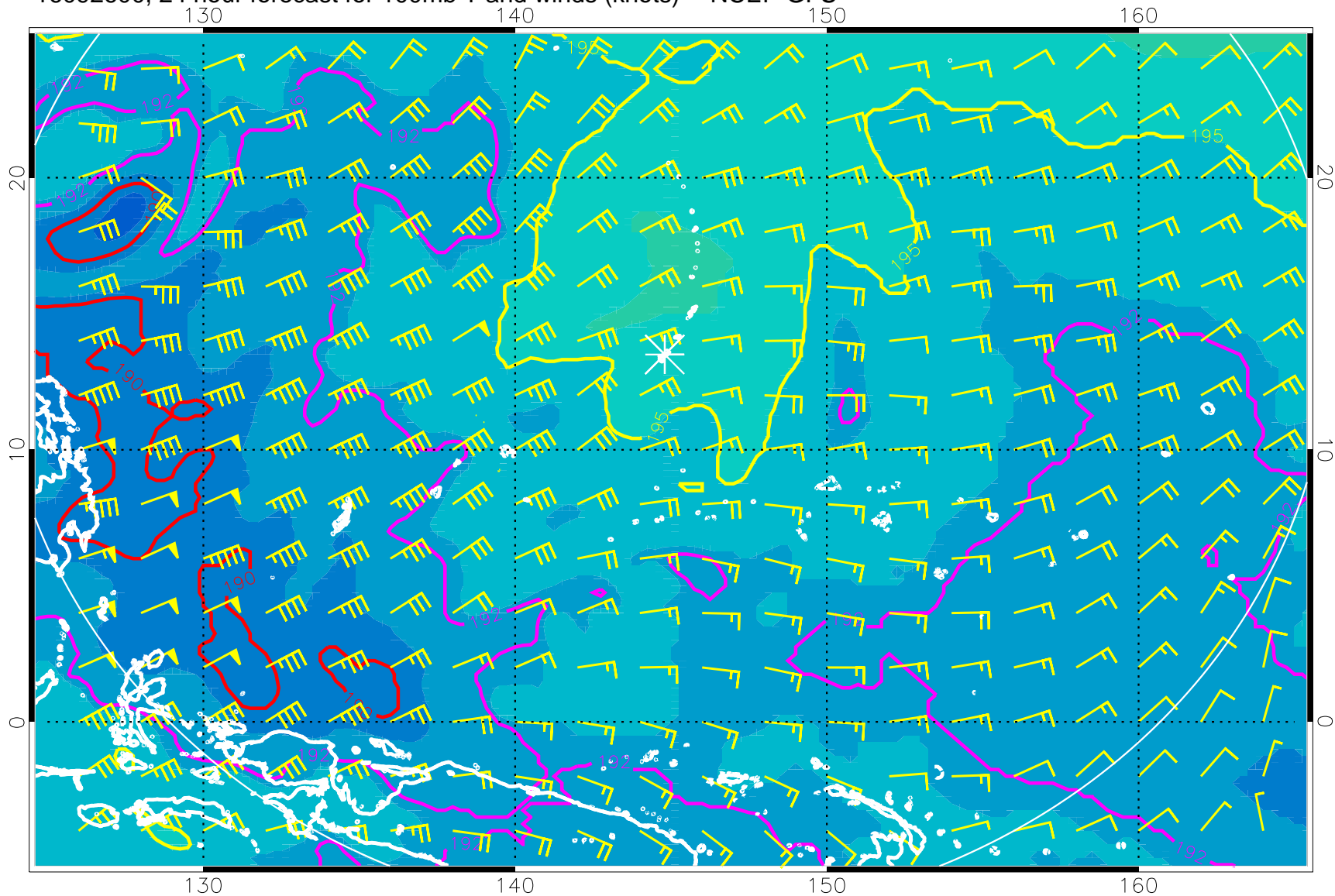
16092600, 24 hour forecast for 100mb T and winds (knots) -- NCEP GFS
