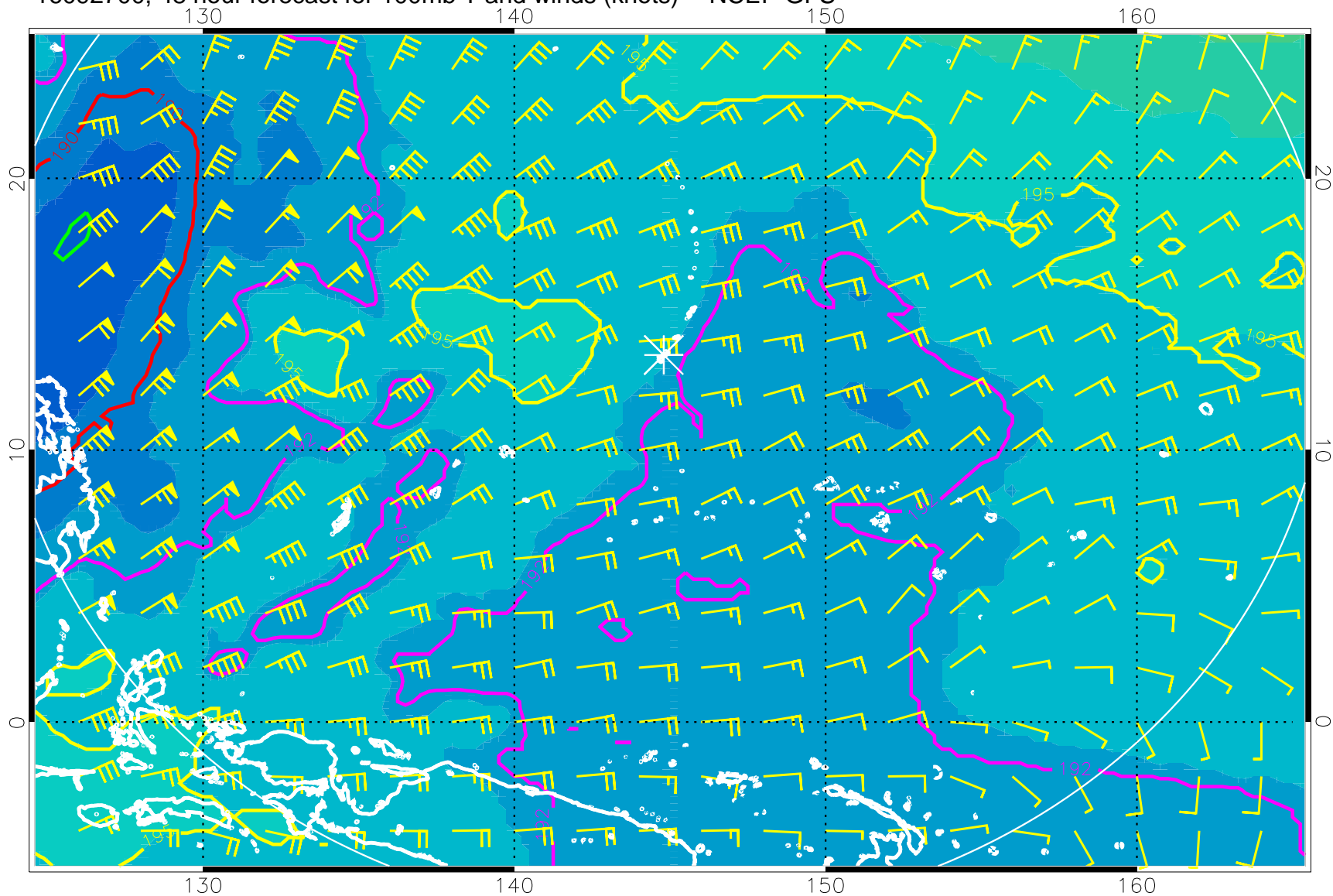
16092700, 48 hour forecast for 100mb T and winds (knots) -- NCEP GFS
