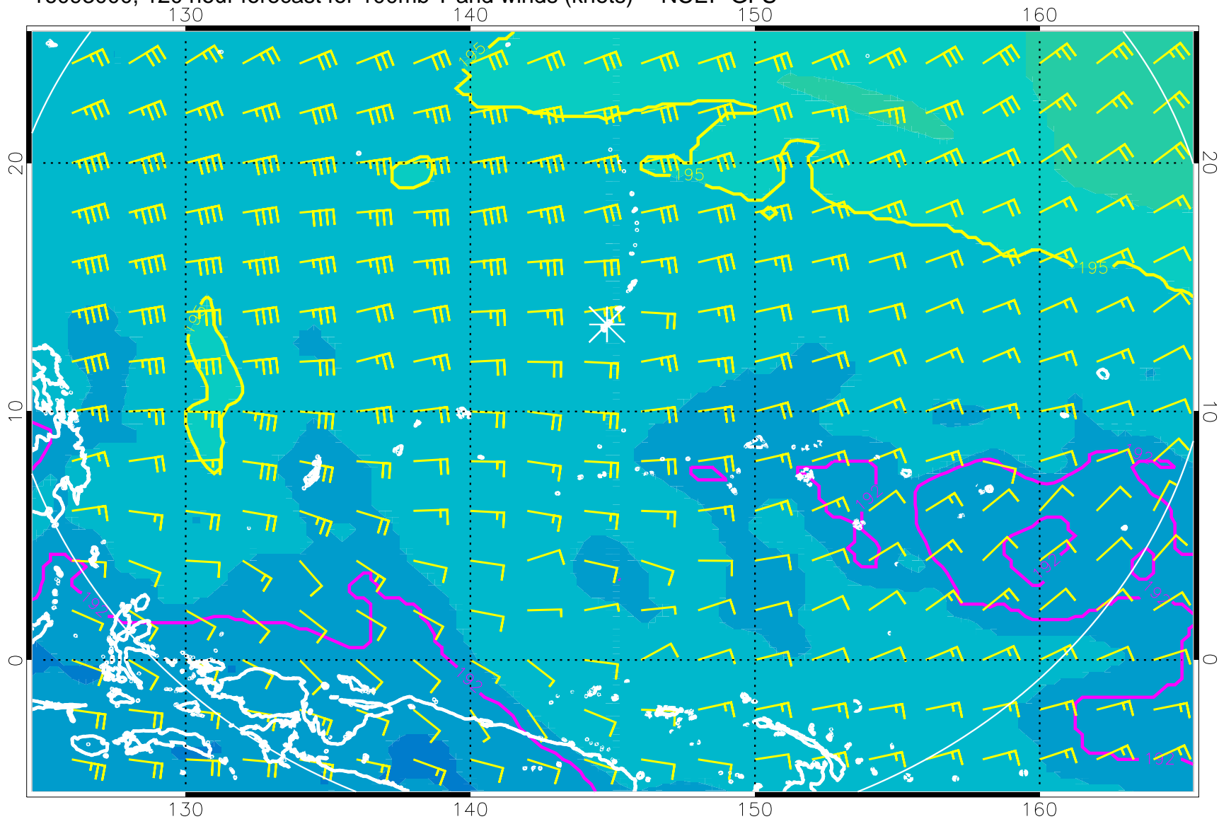
16093000, 120 hour forecast for 100mb T and winds (knots) -- NCEP GFS
