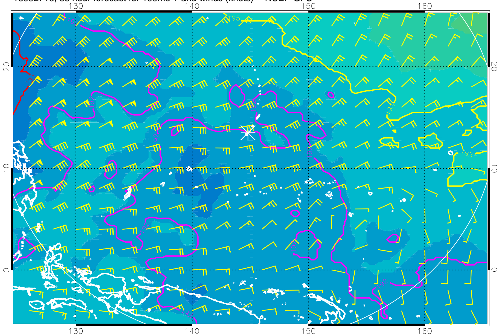
16092718, 66 hour forecast for 100mb T and winds (knots) -- NCEP GFS
