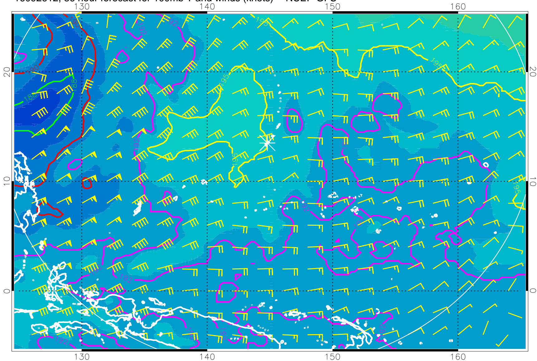
16092612, 36 hour forecast for 100mb T and winds (knots) -- NCEP GFS
