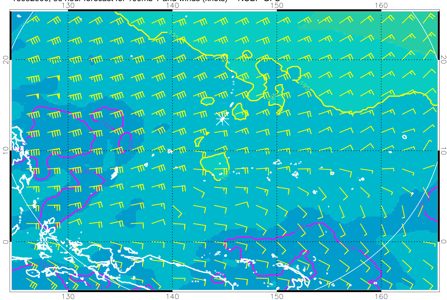
16092900, 96 hour forecast for 100mb T and winds (knots) -- NCEP GFS
