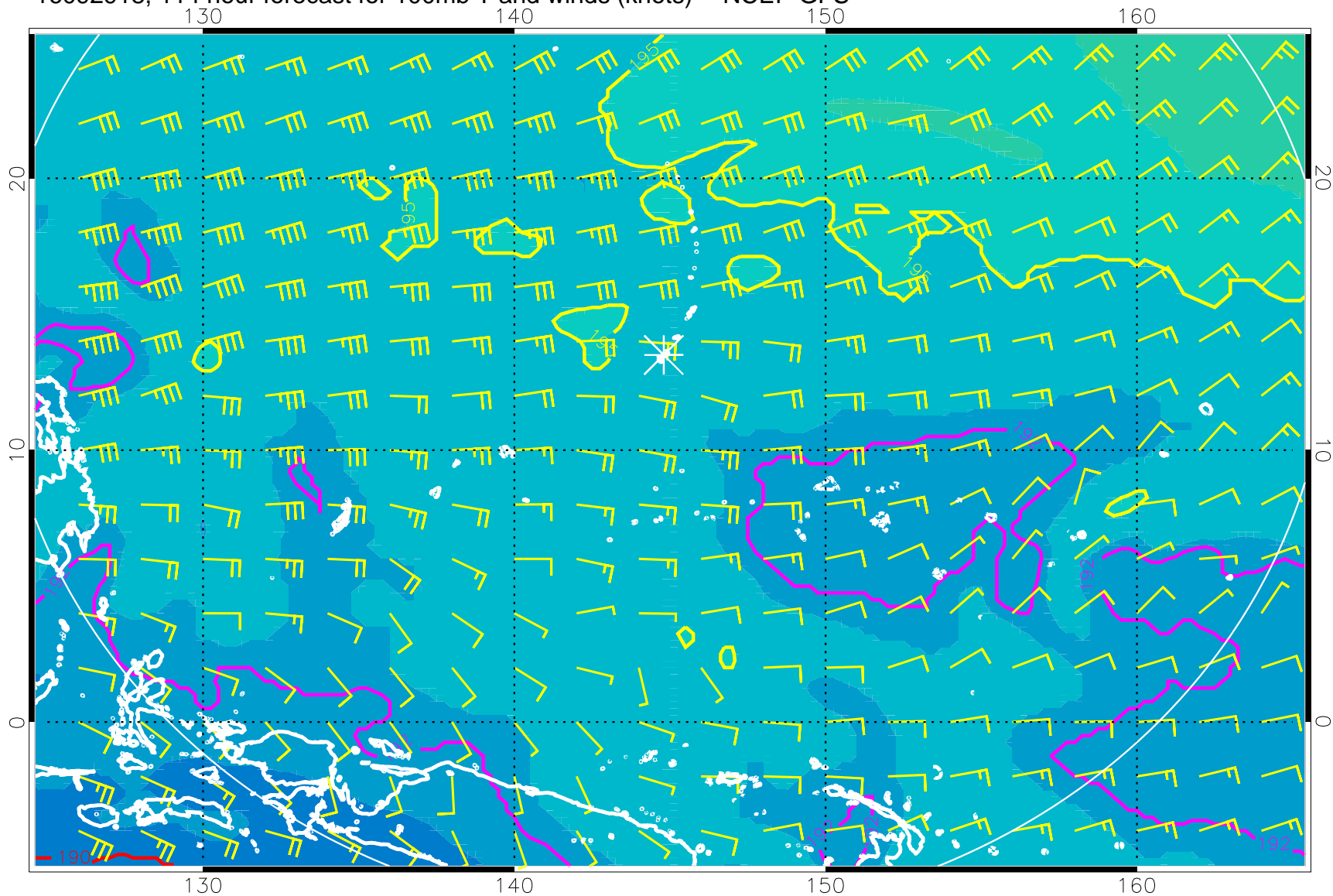
16092918, 114 hour forecast for 100mb T and winds (knots) -- NCEP GFS
