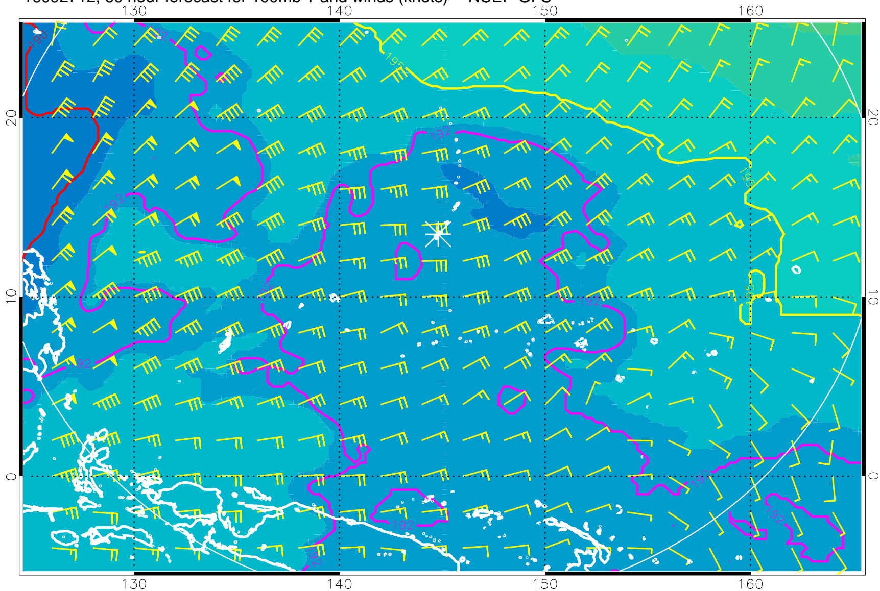
16092712, 60 hour forecast for 100mb T and winds (knots) -- NCEP GFS
