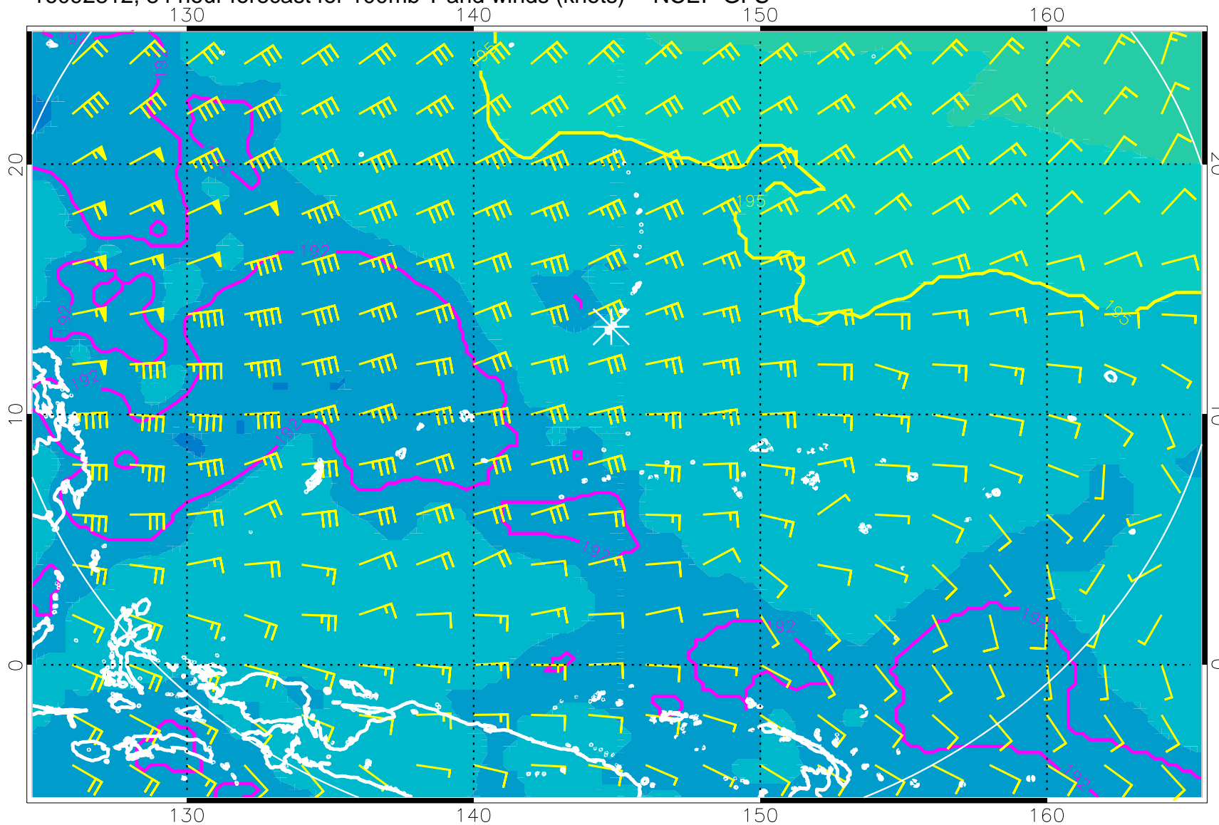
16092812, 84 hour forecast for 100mb T and winds (knots) -- NCEP GFS
