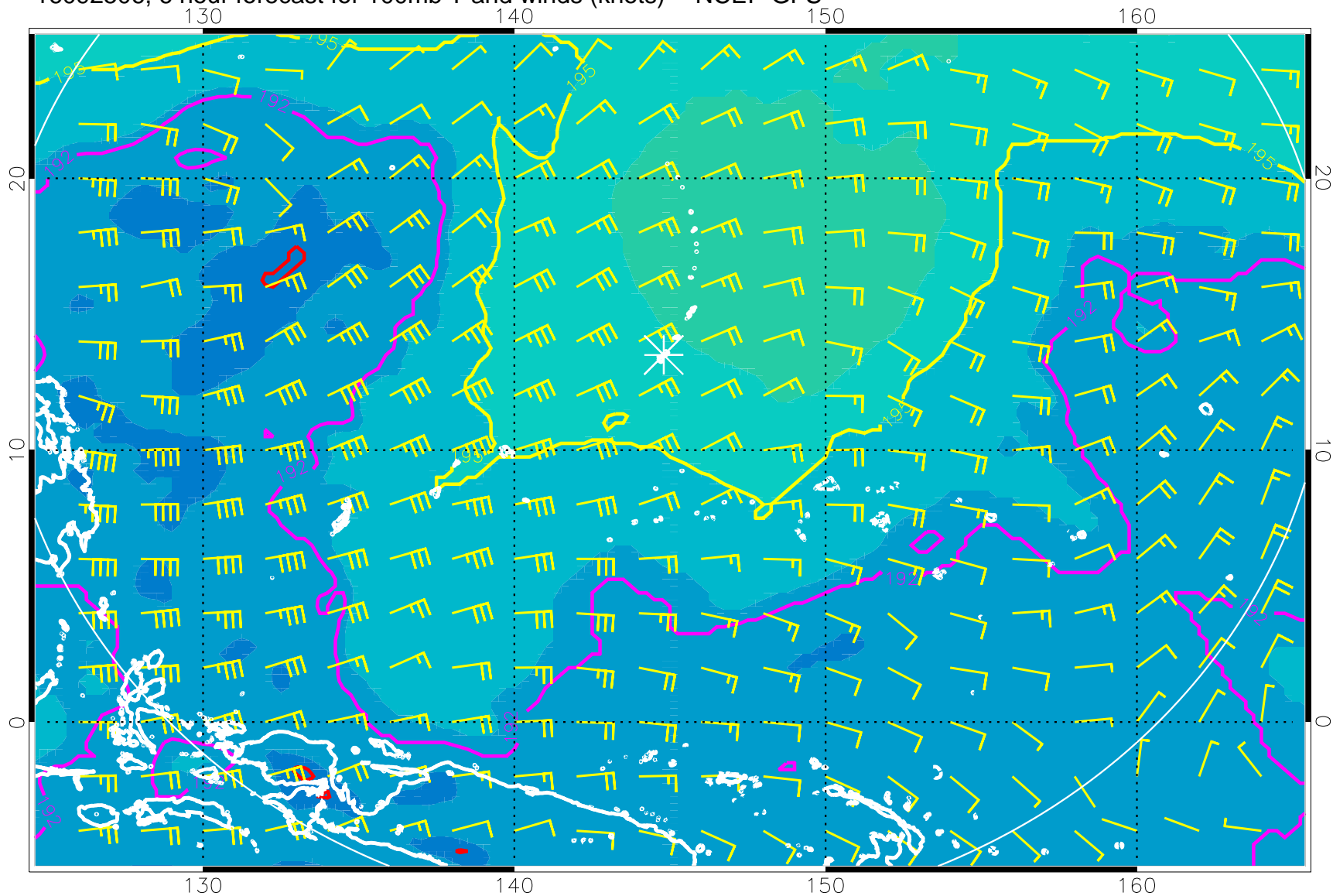
16092506, 6 hour forecast for 100mb T and winds (knots) -- NCEP GFS
