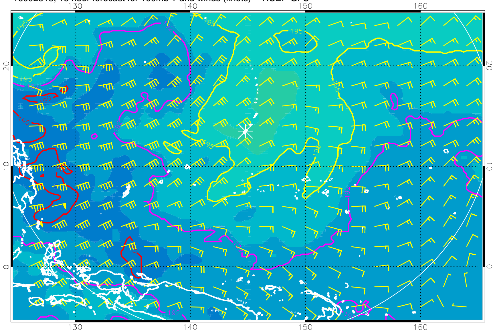
16092518, 18 hour forecast for 100mb T and winds (knots) -- NCEP GFS
