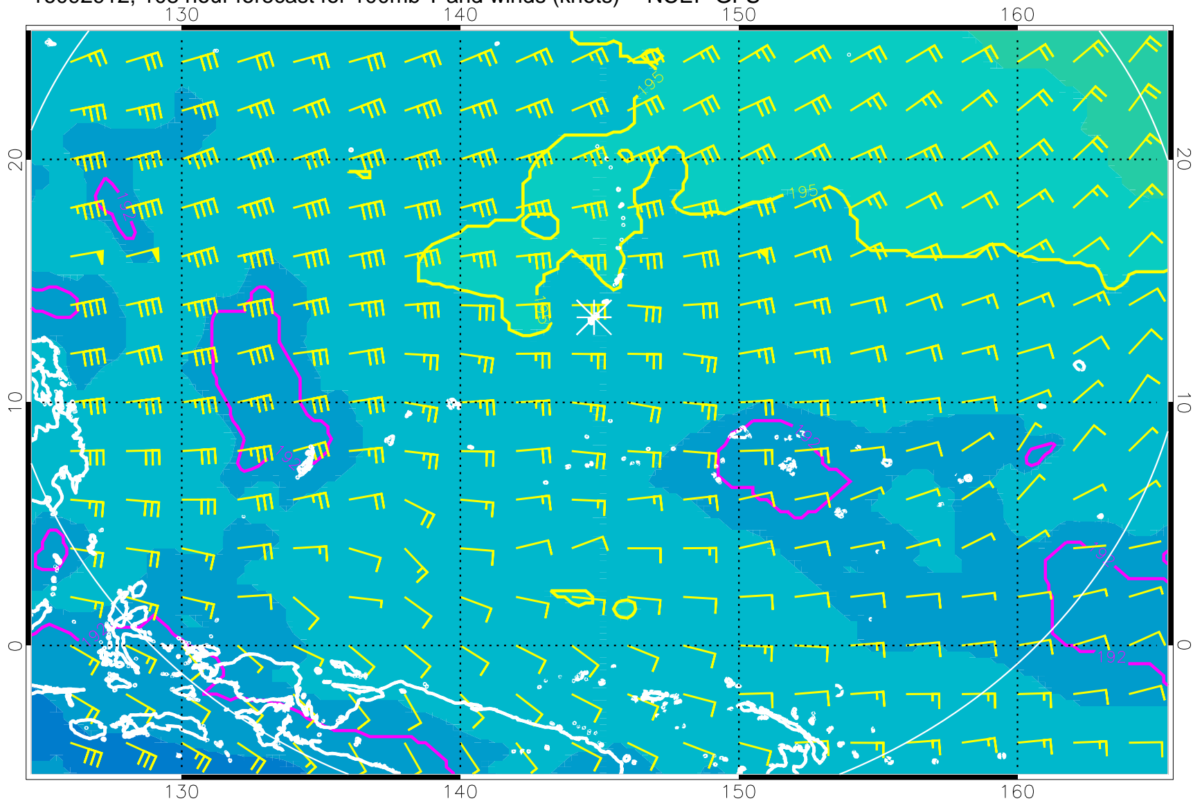
16092912, 108 hour forecast for 100mb T and winds (knots) -- NCEP GFS
