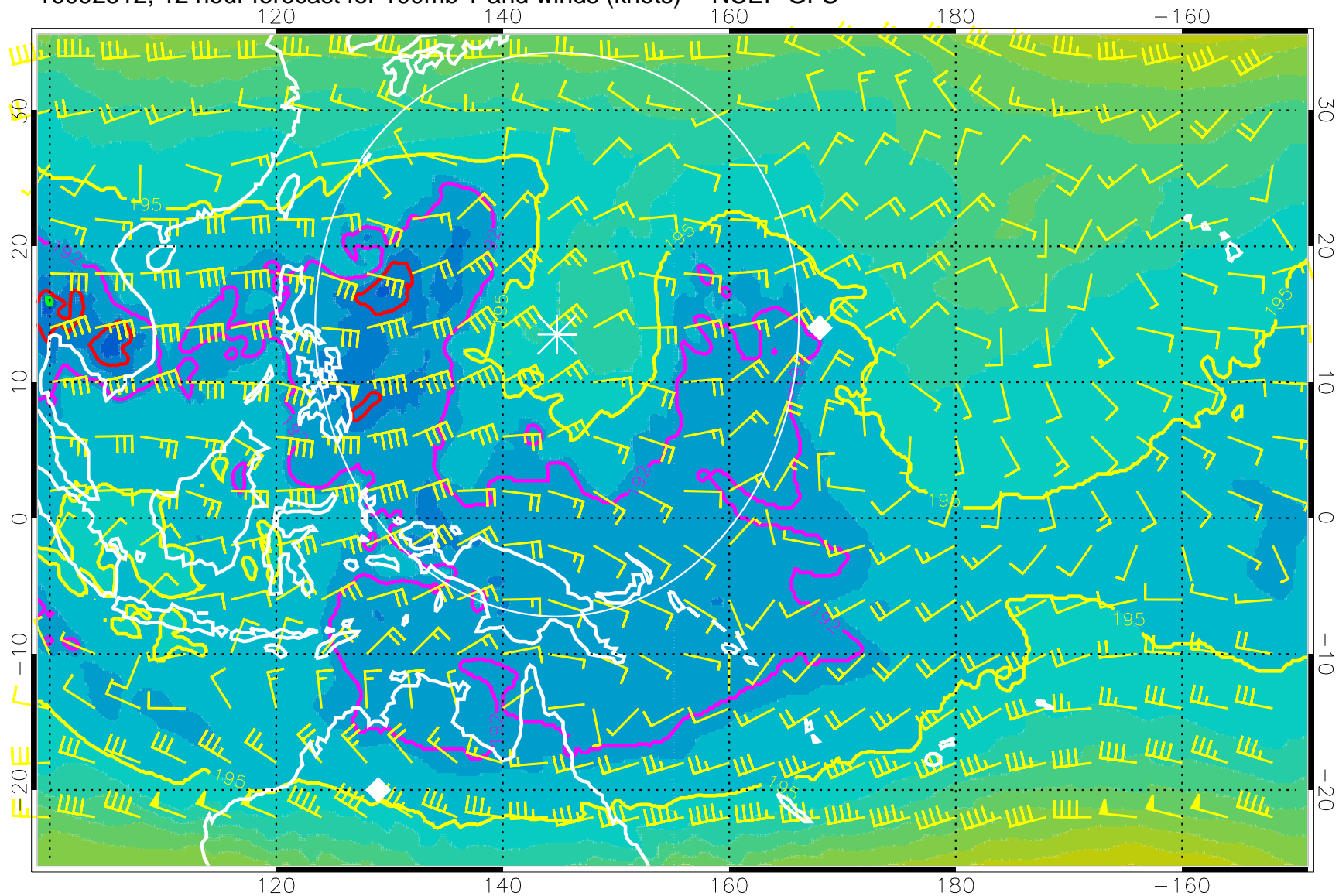
16092512, 12 hour forecast for 100mb T and winds (knots) -- NCEP GFS
