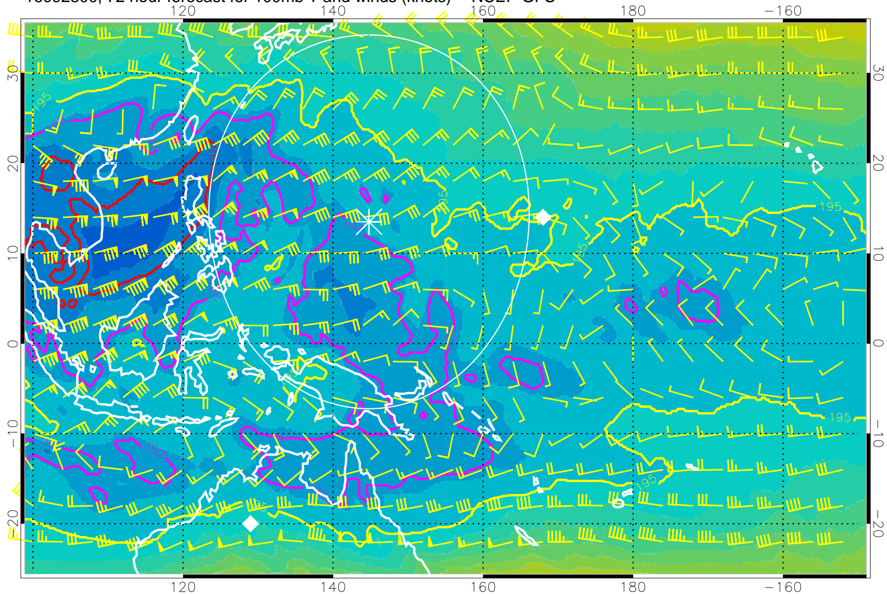
16092800, 72 hour forecast for 100mb T and winds (knots) -- NCEP GFS
