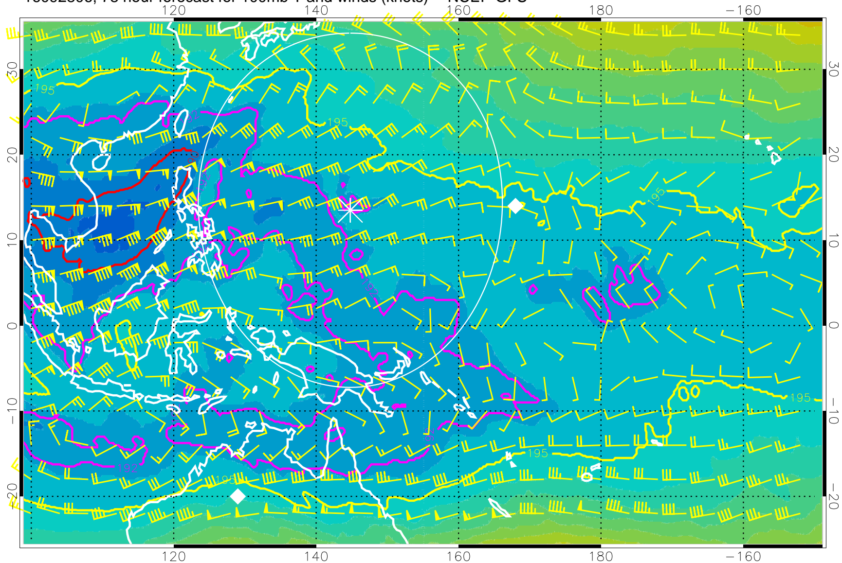
16092806, 78 hour forecast for 100mb T and winds (knots) -- NCEP GFS
