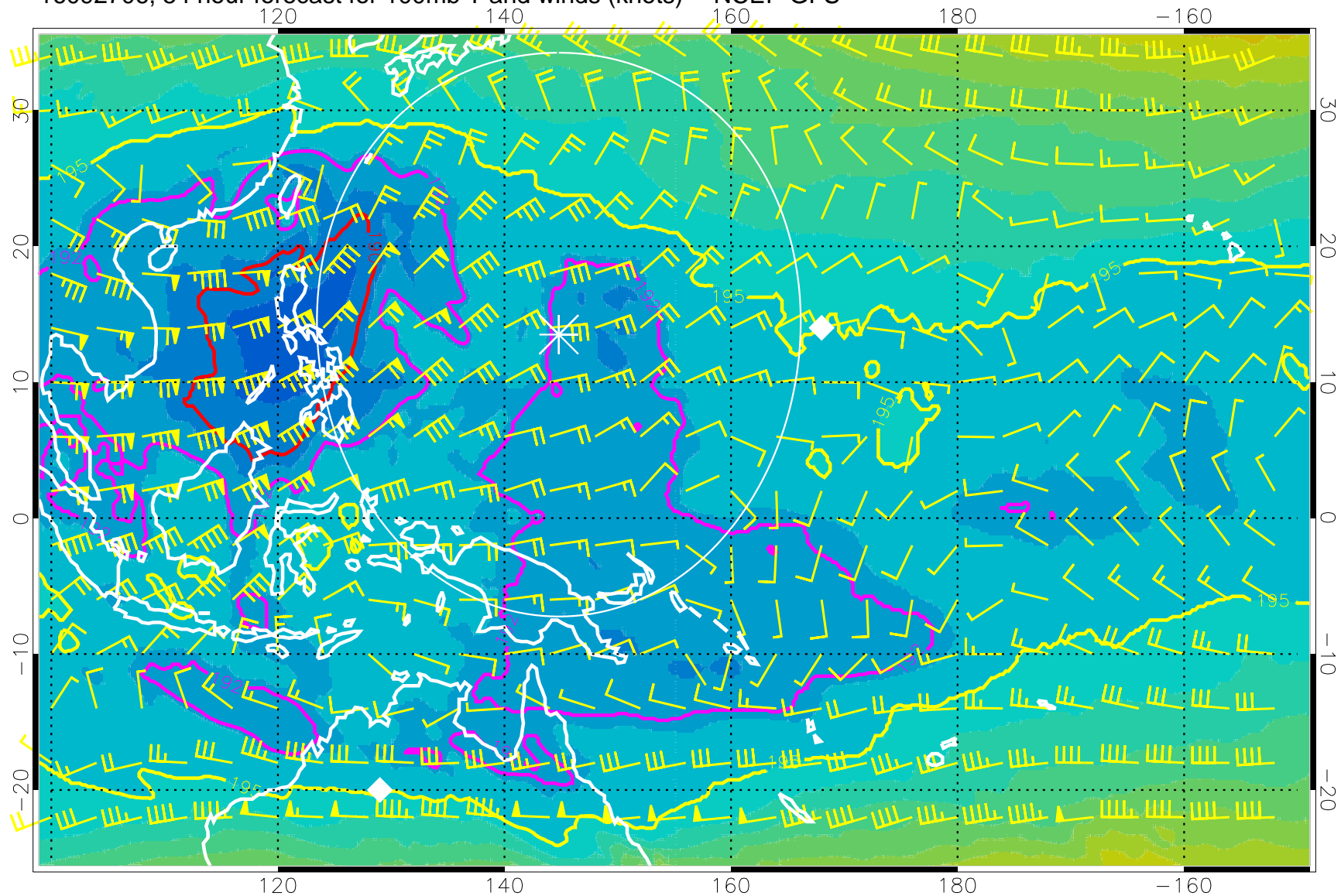
16092706, 54 hour forecast for 100mb T and winds (knots) -- NCEP GFS
