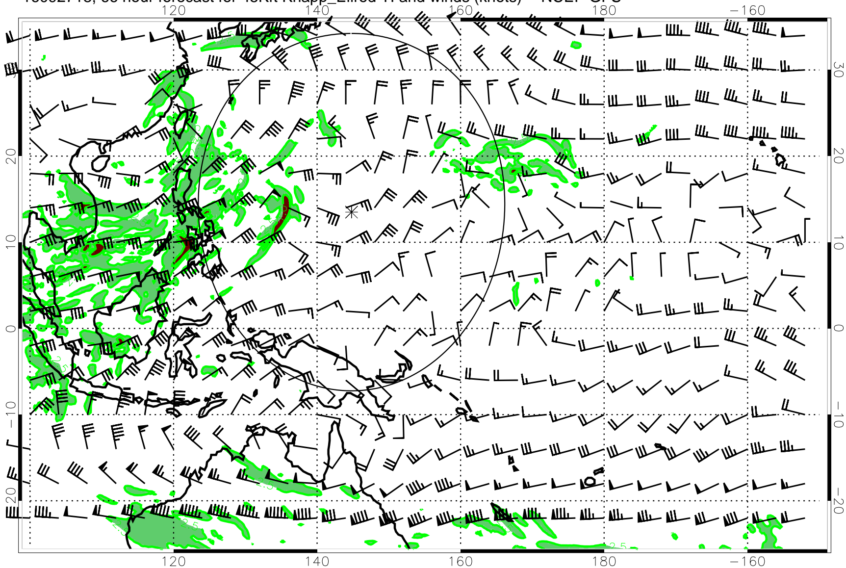
16092718, 66 hour forecast for 45Kft Knapp_Ellrod TI and winds (knots) -- NCEP GFS
