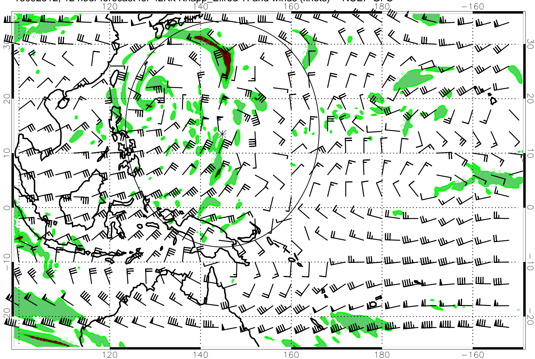
16092512, 12 hour forecast for 42Kft Knapp_Ellrod TI and winds (knots) -- NCEP GFS
