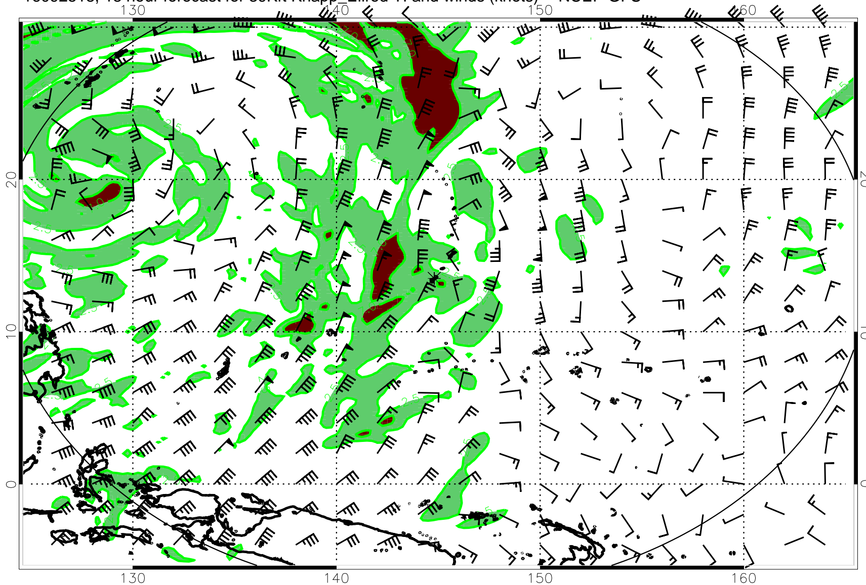
16092518, 18 hour forecast for 39Kft Knapp_Ellrod TI and winds (knots) -- NCEP GFS
