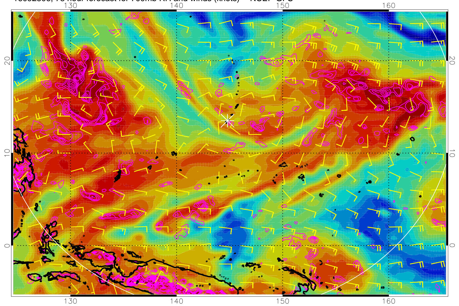
16092806, 78 hour forecast for 700mb RH and winds (knots) -- NCEP GFS
