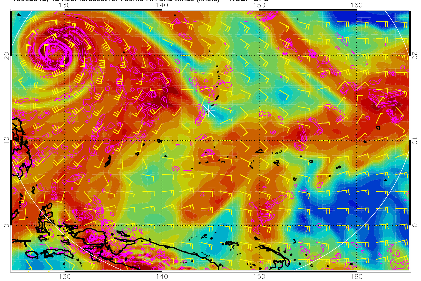
16092512, 12 hour forecast for 700mb RH and winds (knots) -- NCEP GFS
