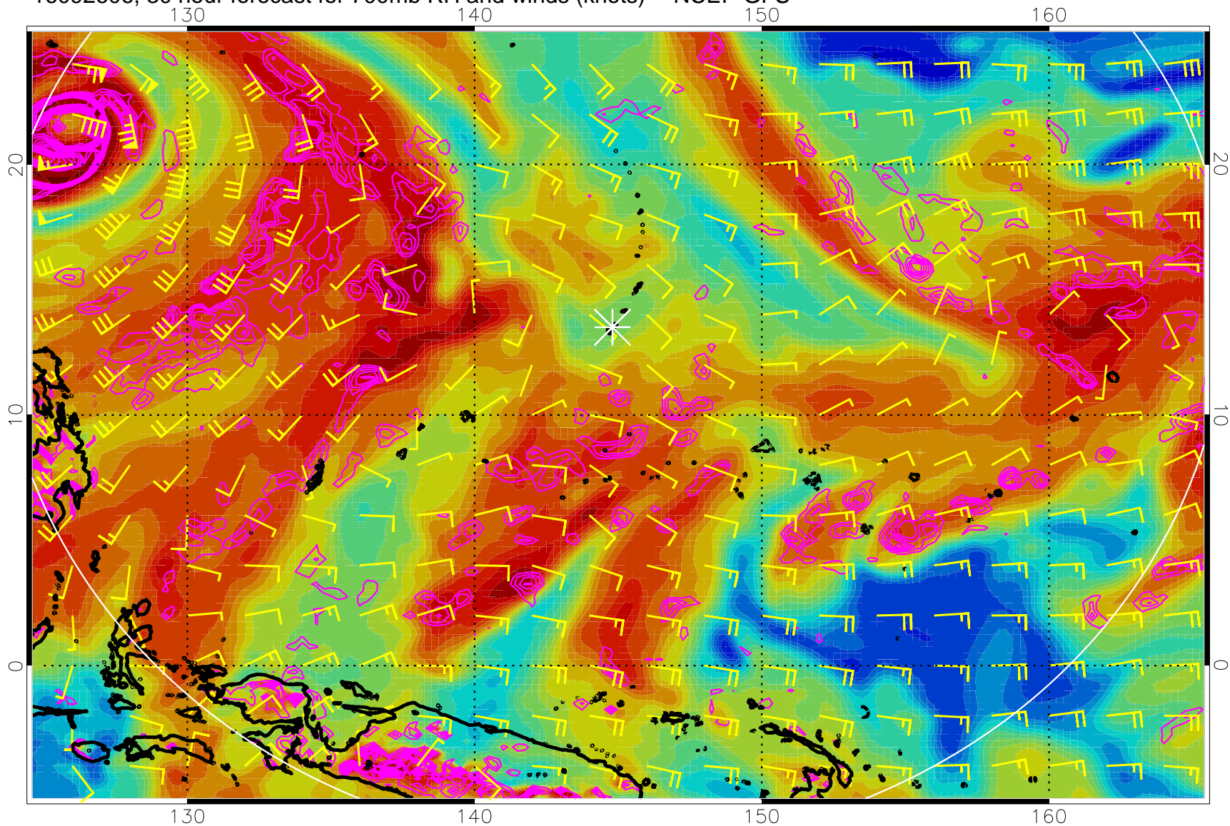
16092606, 30 hour forecast for 700mb RH and winds (knots) -- NCEP GFS
