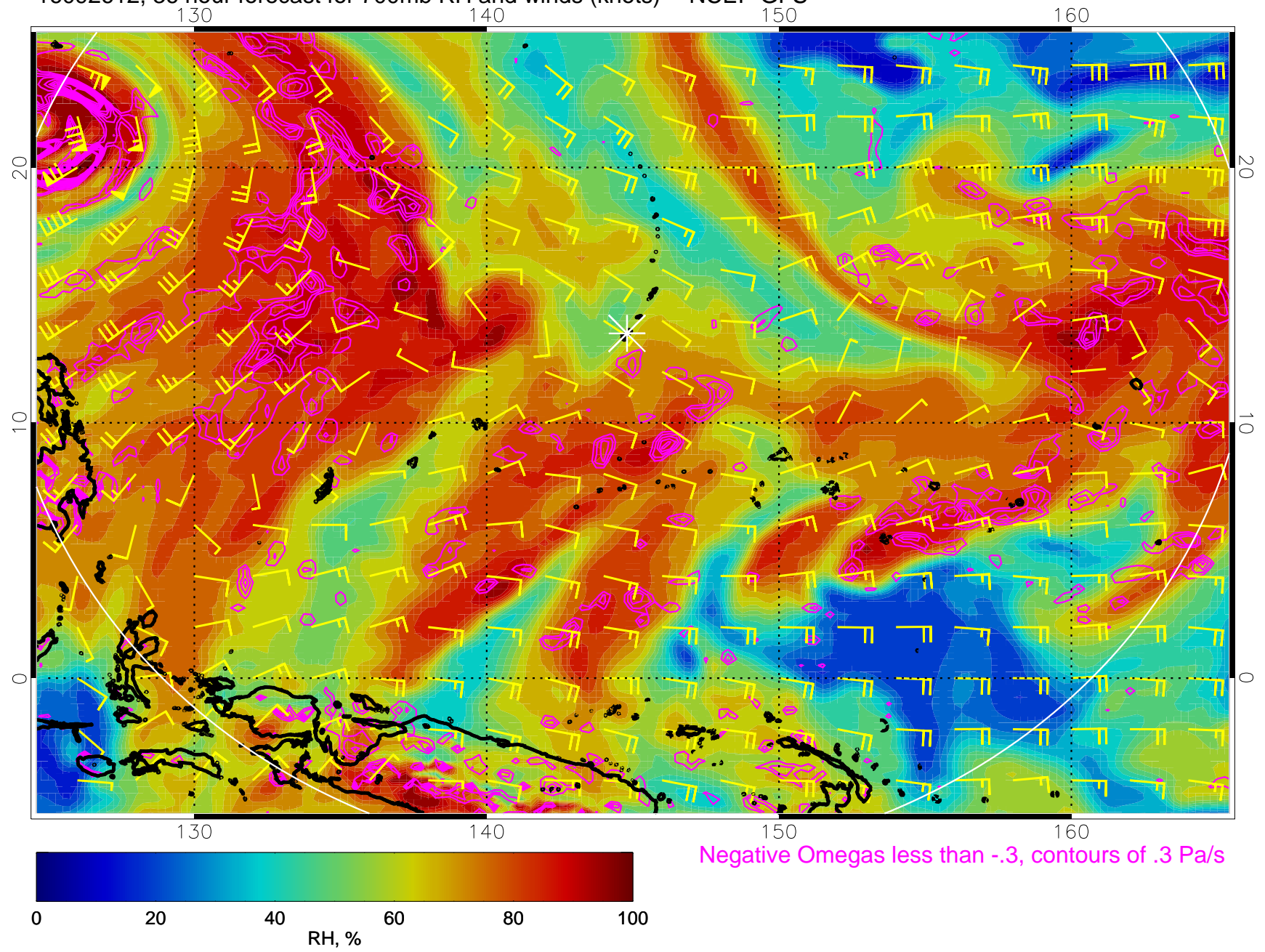
16092612, 36 hour forecast for 700mb RH and winds (knots) -- NCEP GFS
