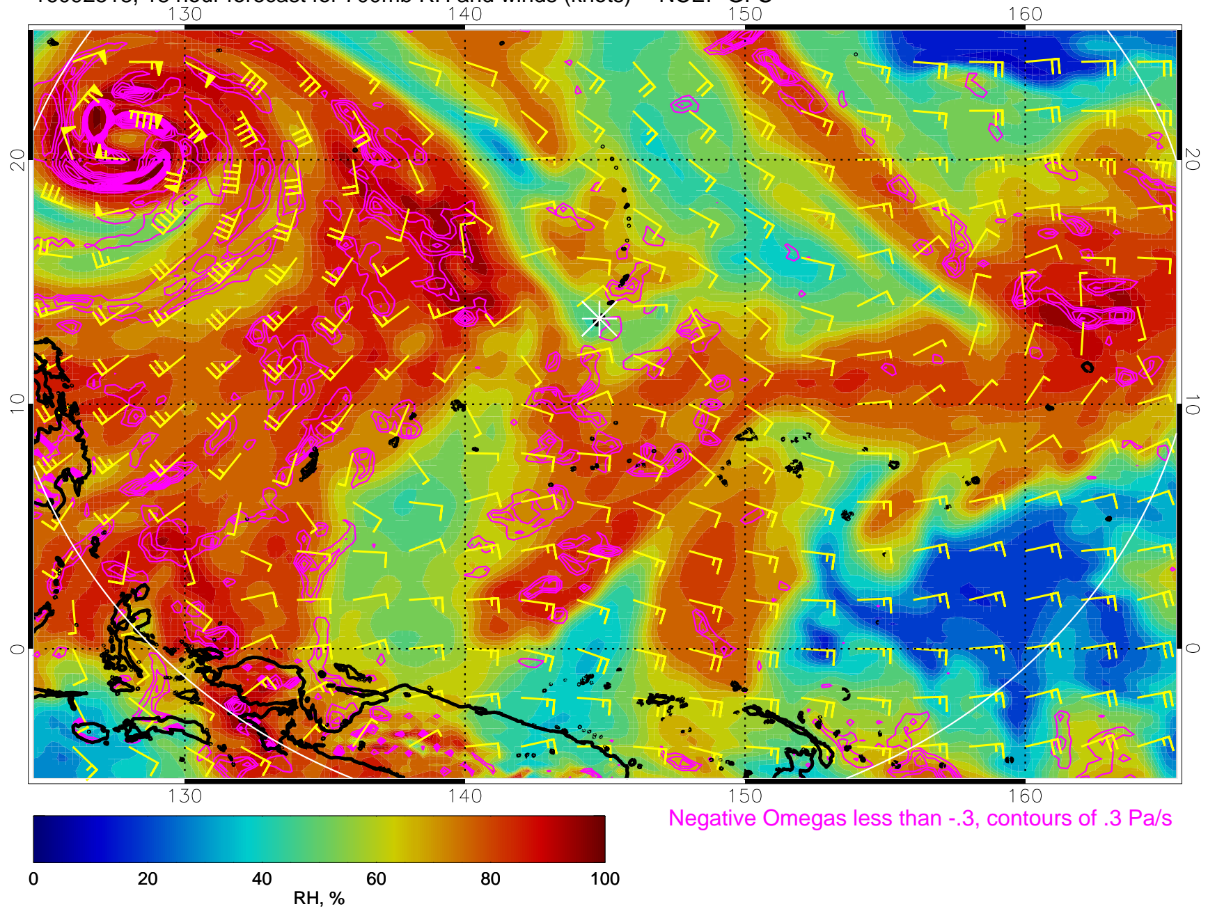
16092518, 18 hour forecast for 700mb RH and winds (knots) -- NCEP GFS
