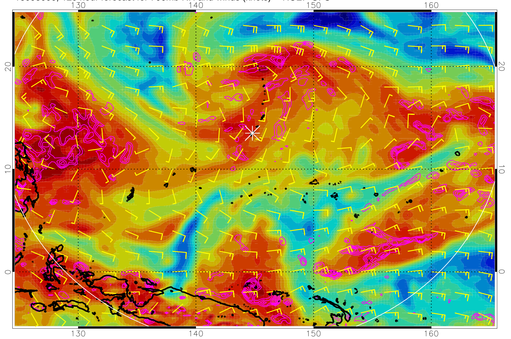
16093000, 120 hour forecast for 700mb RH and winds (knots) -- NCEP GFS
