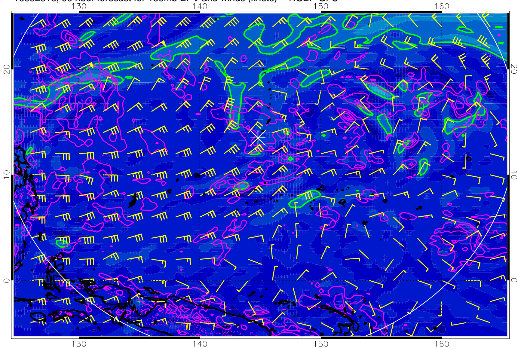
16092818, 90 hour forecast for 150mb EPV and winds (knots) -- NCEP GFS
