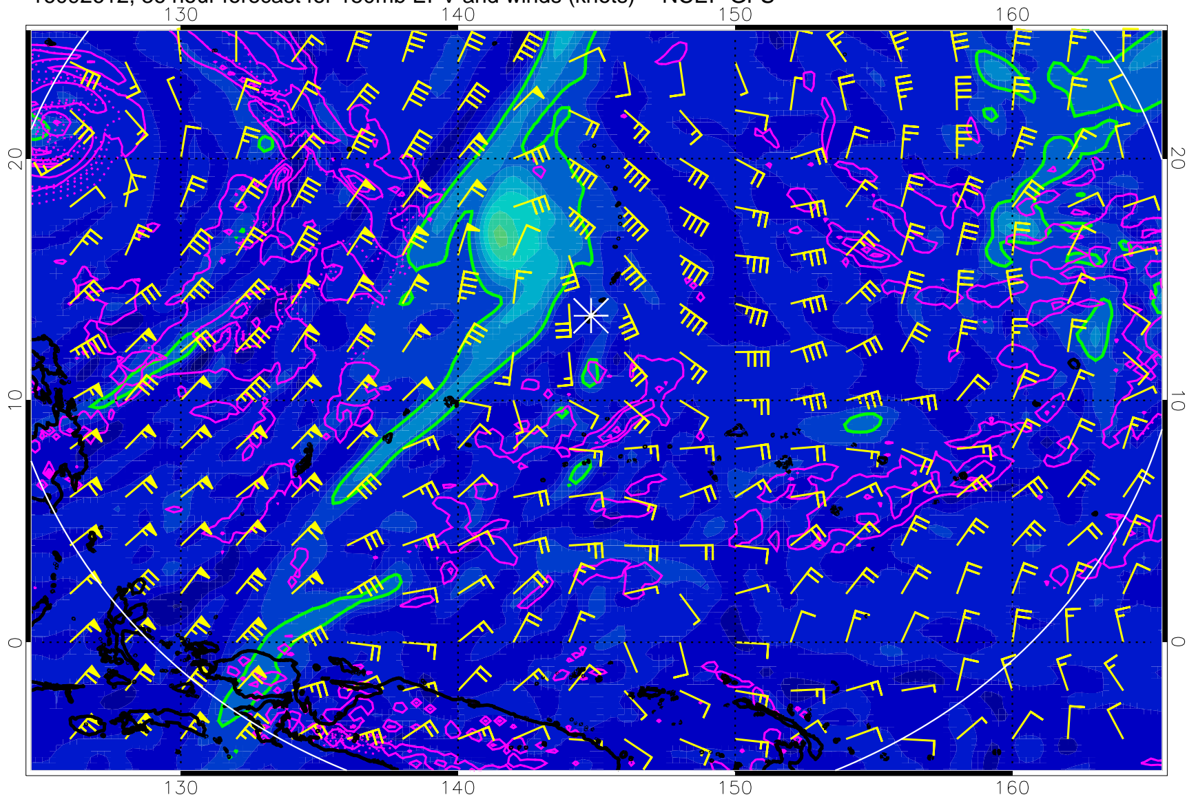
16092612, 36 hour forecast for 150mb EPV and winds (knots) -- NCEP GFS
