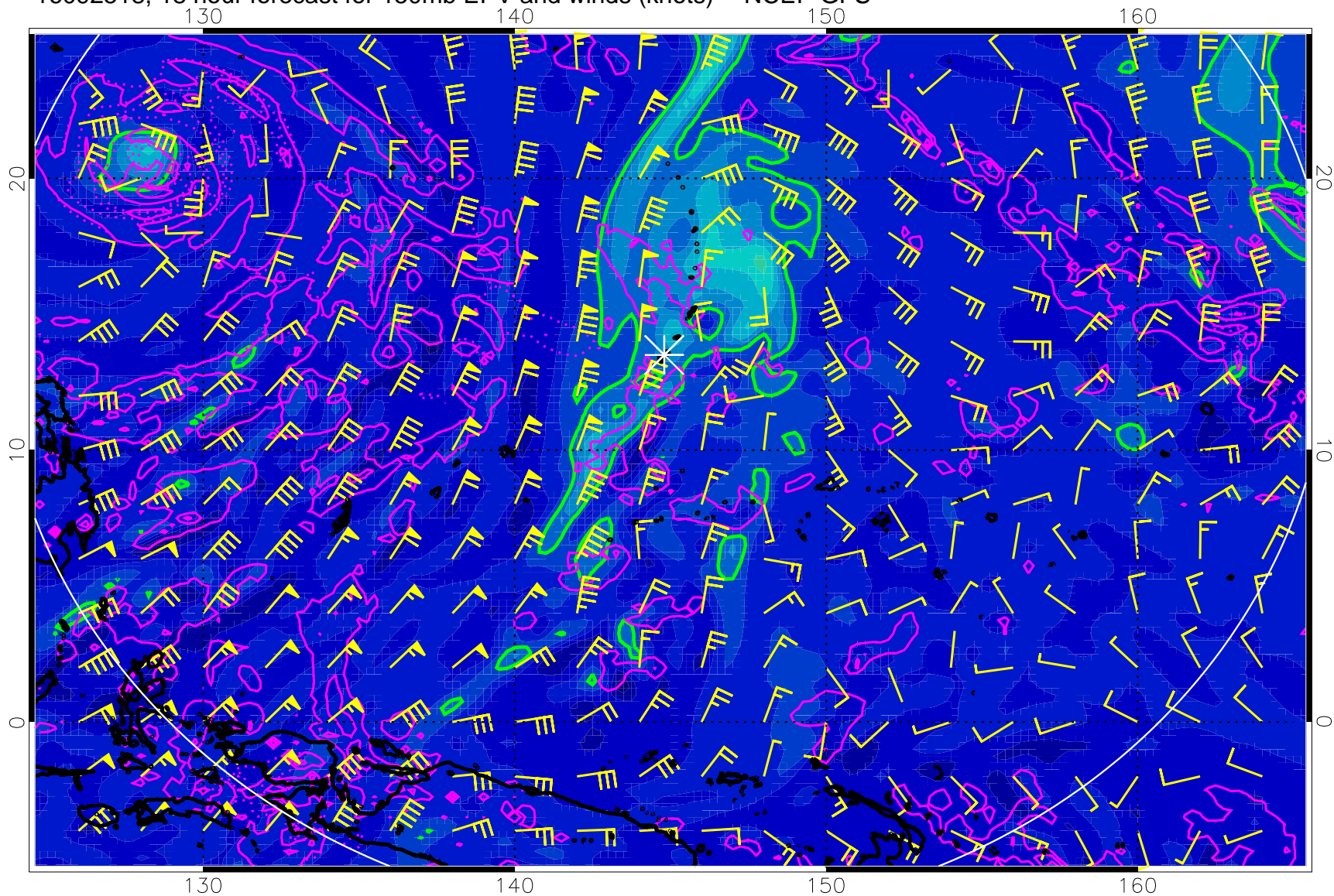
16092518, 18 hour forecast for 150mb EPV and winds (knots) -- NCEP GFS
