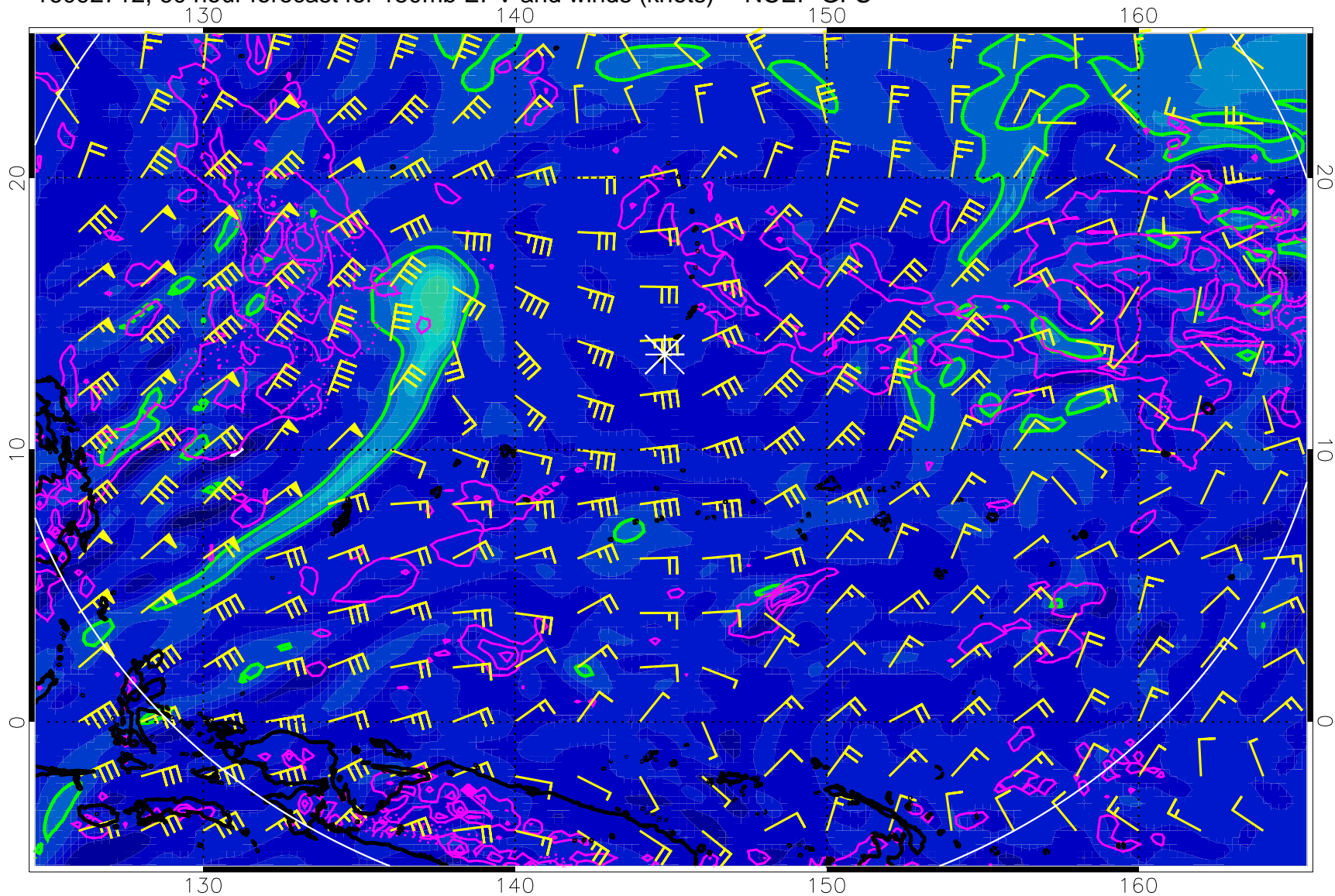
16092712, 60 hour forecast for 150mb EPV and winds (knots) -- NCEP GFS
