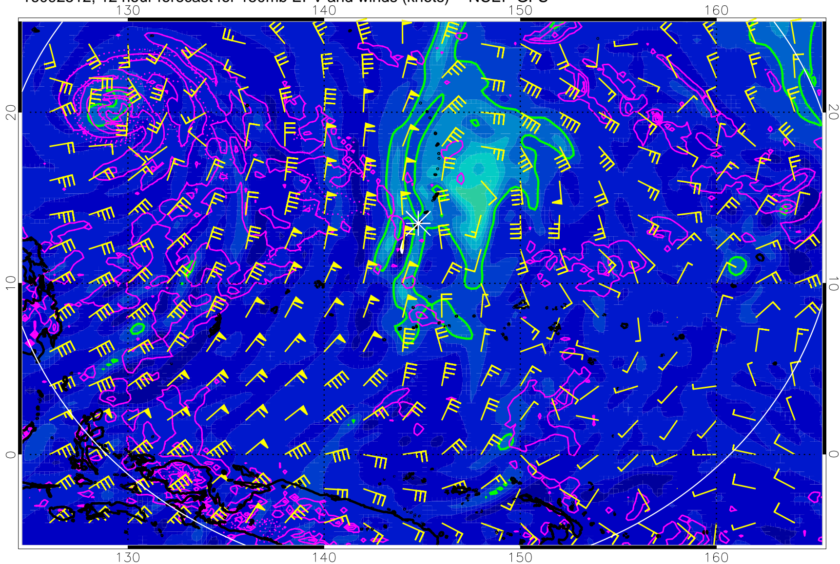
16092512, 12 hour forecast for 150mb EPV and winds (knots) -- NCEP GFS
