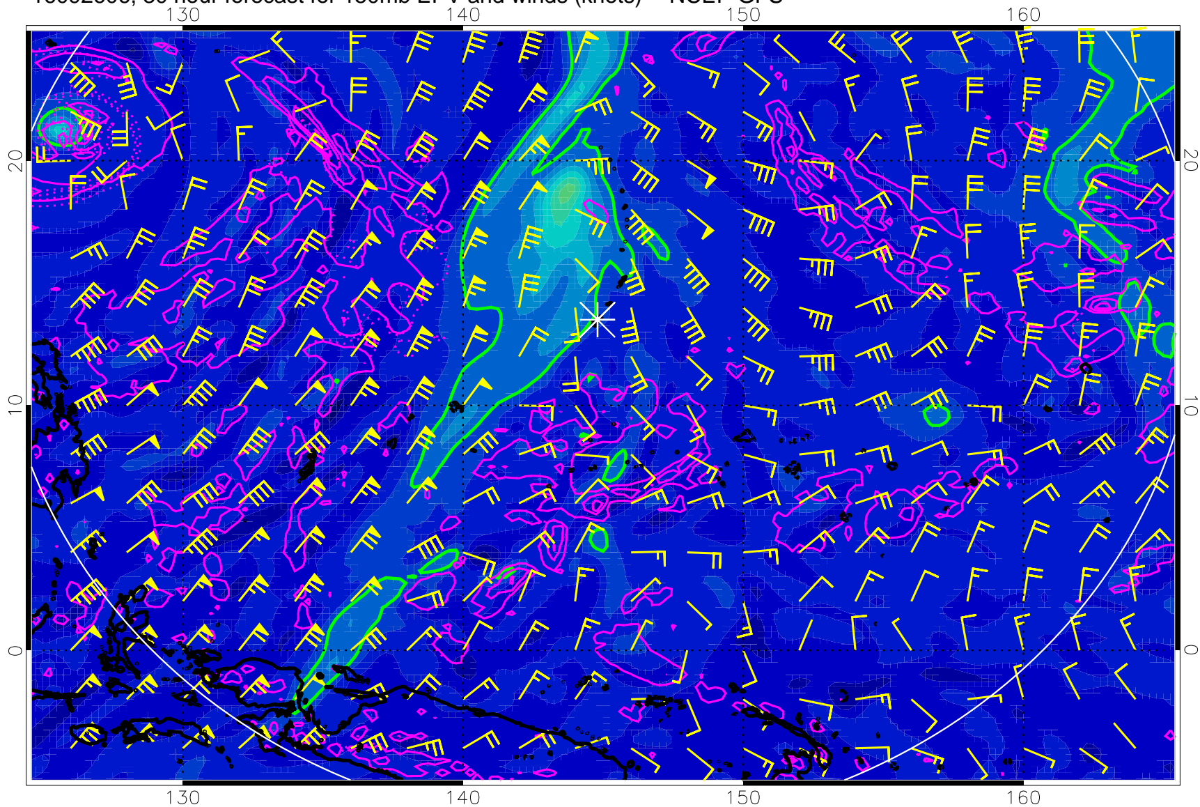
16092606, 30 hour forecast for 150mb EPV and winds (knots) -- NCEP GFS
