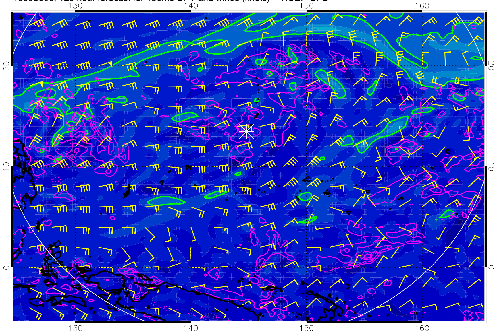
16093000, 120 hour forecast for 150mb EPV and winds (knots) -- NCEP GFS
