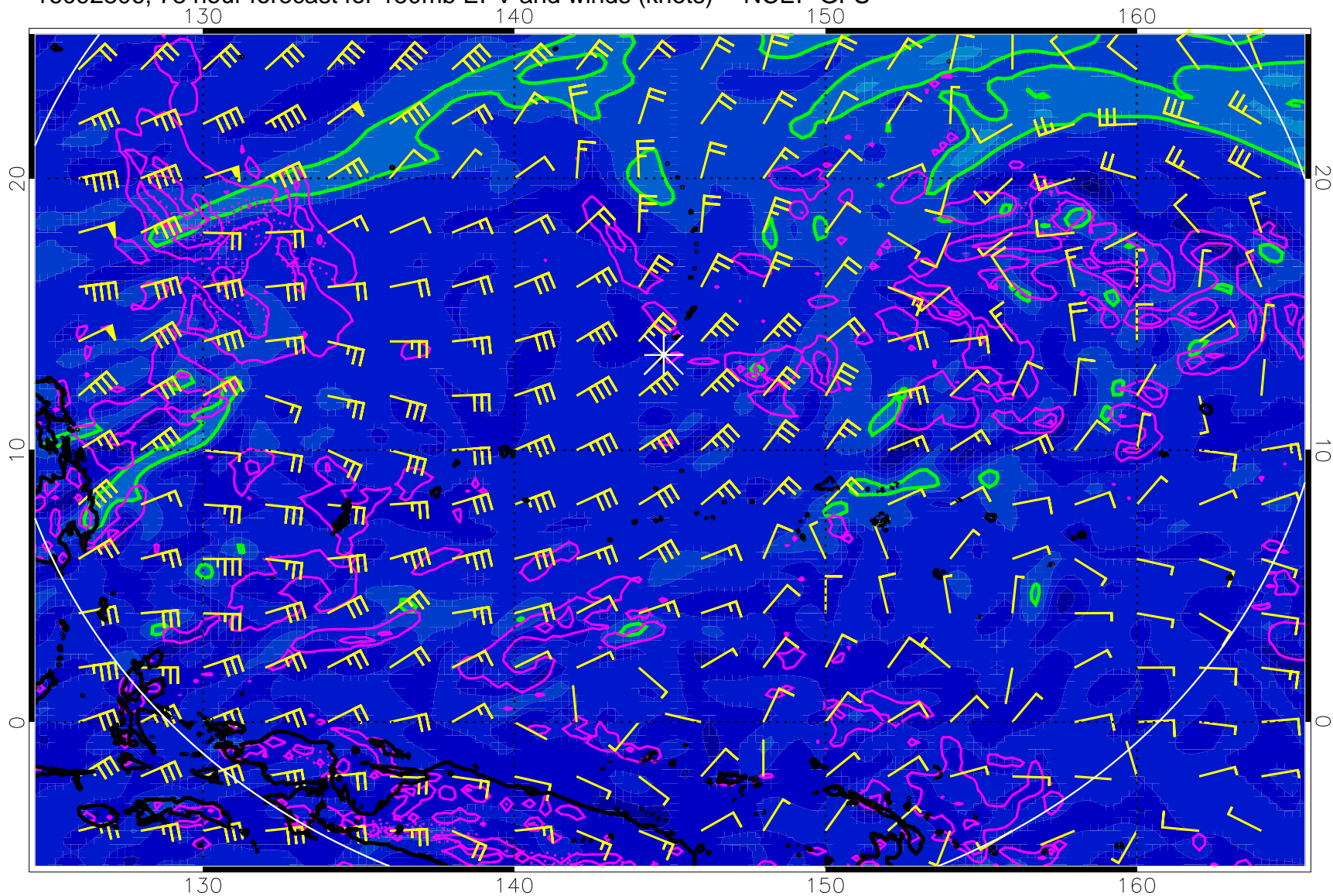
16092806, 78 hour forecast for 150mb EPV and winds (knots) -- NCEP GFS
