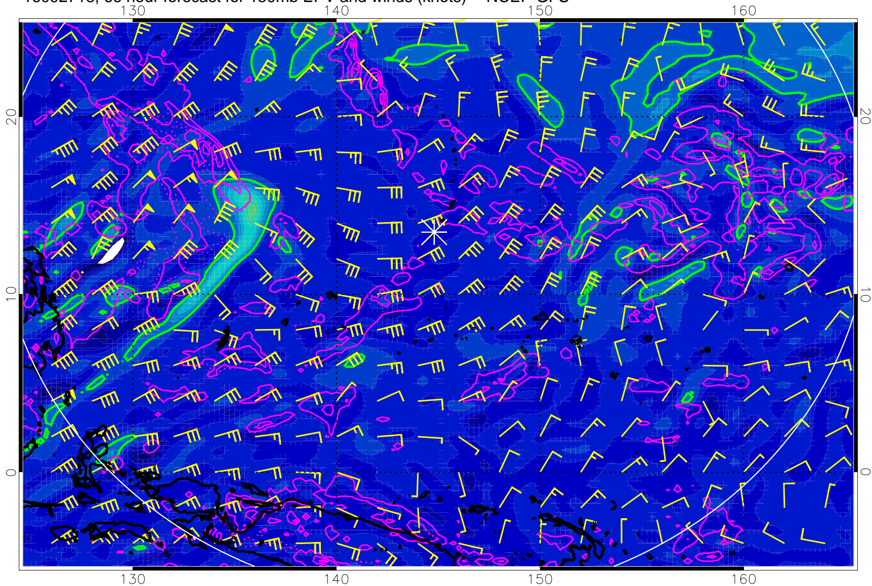
16092718, 66 hour forecast for 150mb EPV and winds (knots) -- NCEP GFS
