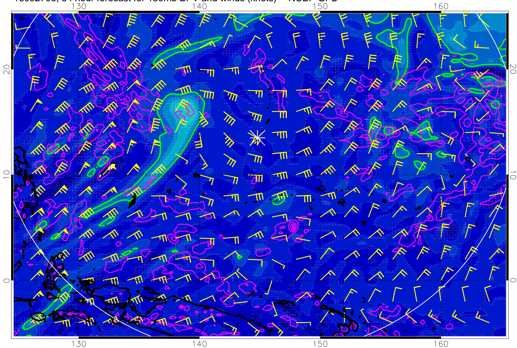
16092706, 54 hour forecast for 150mb EPV and winds (knots) -- NCEP GFS
