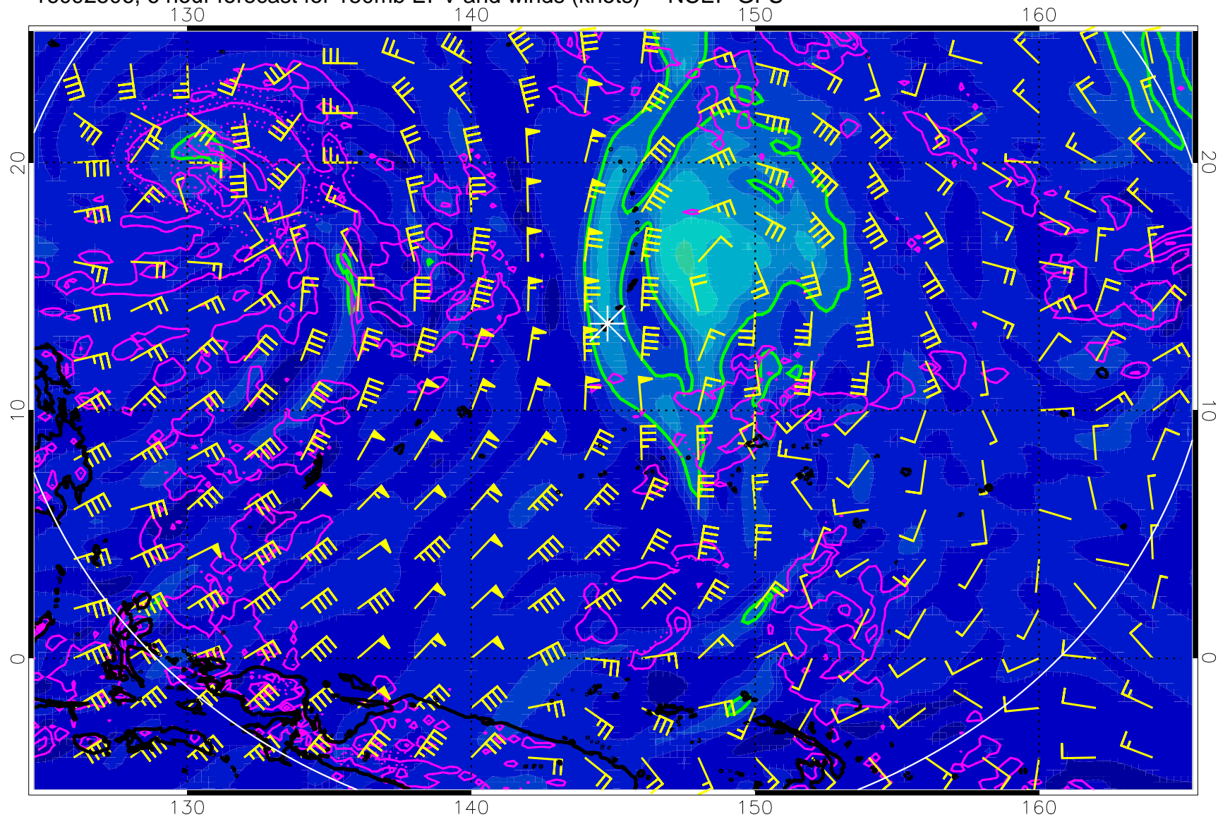
16092506, 6 hour forecast for 150mb EPV and winds (knots) -- NCEP GFS
