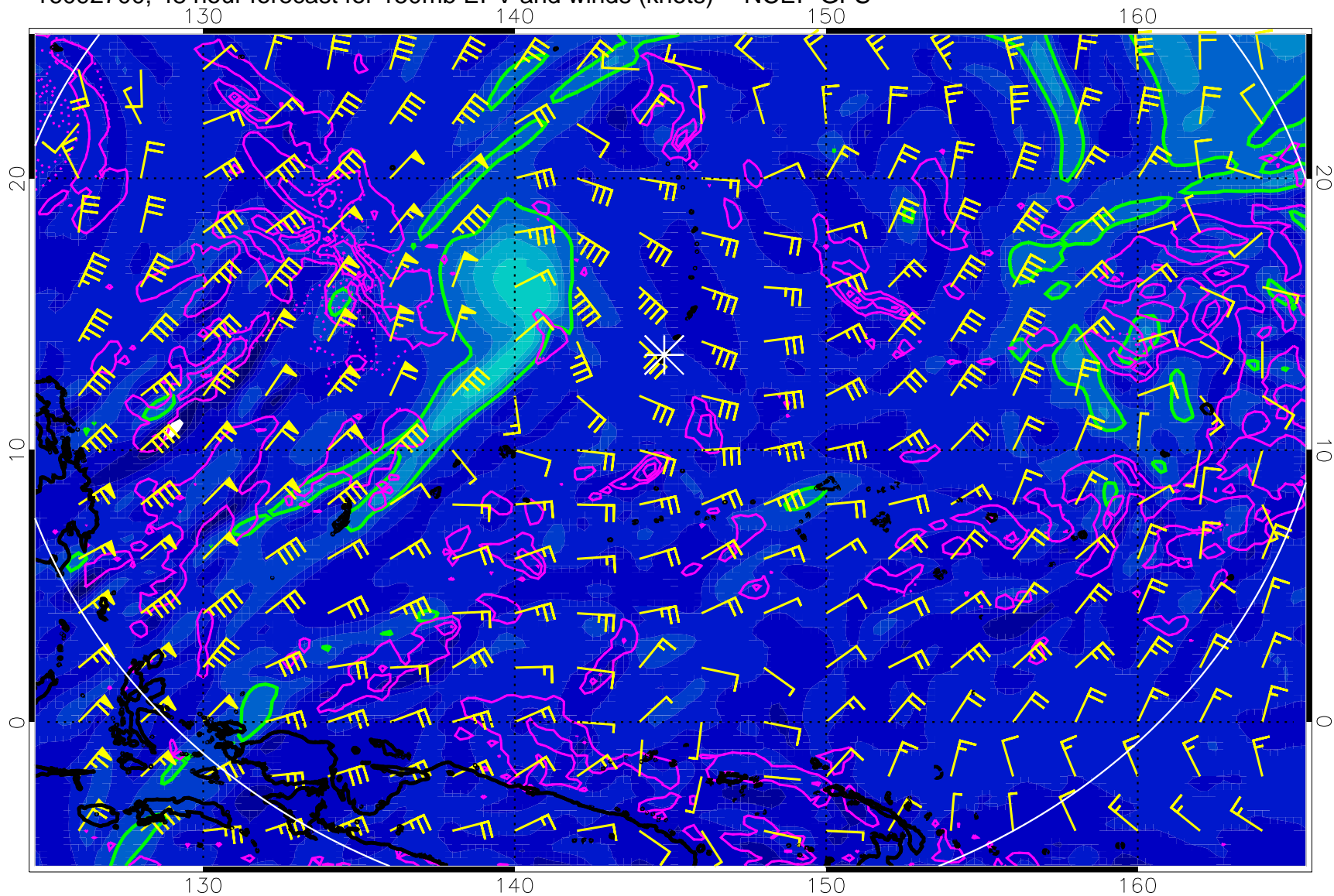
16092700, 48 hour forecast for 150mb EPV and winds (knots) -- NCEP GFS
