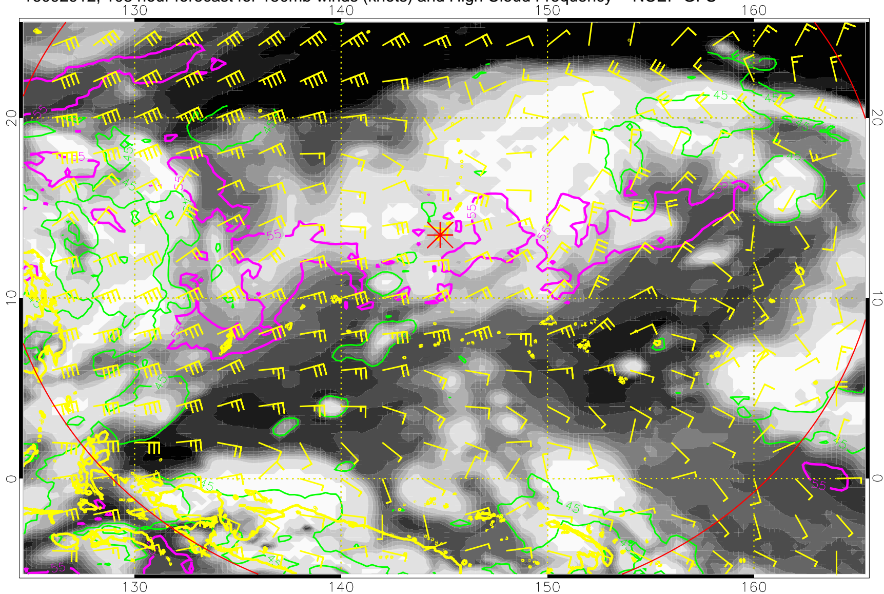
16092912, 108 hour forecast for 150mb winds (knots) and High Cloud Frequency -- NCEP GFS
