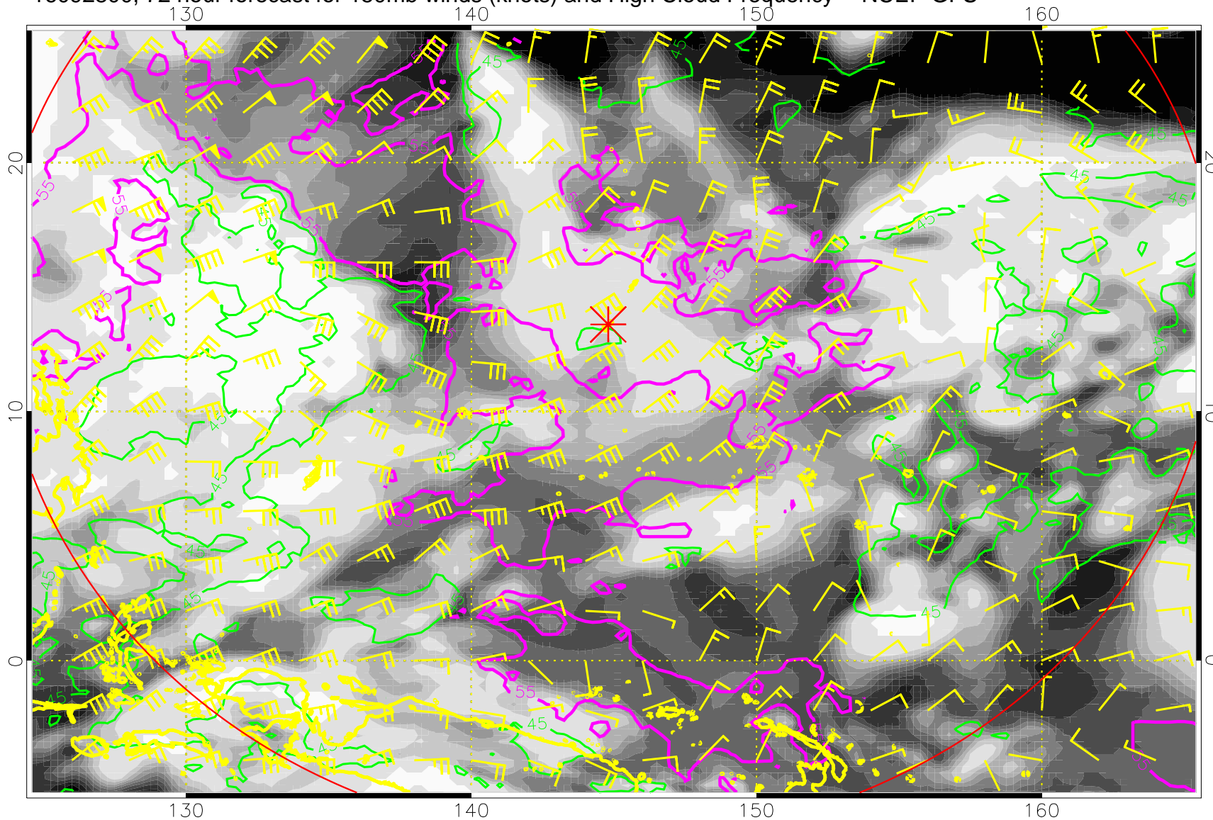
16092800, 72 hour forecast for 150mb winds (knots) and High Cloud Frequency -- NCEP GFS
