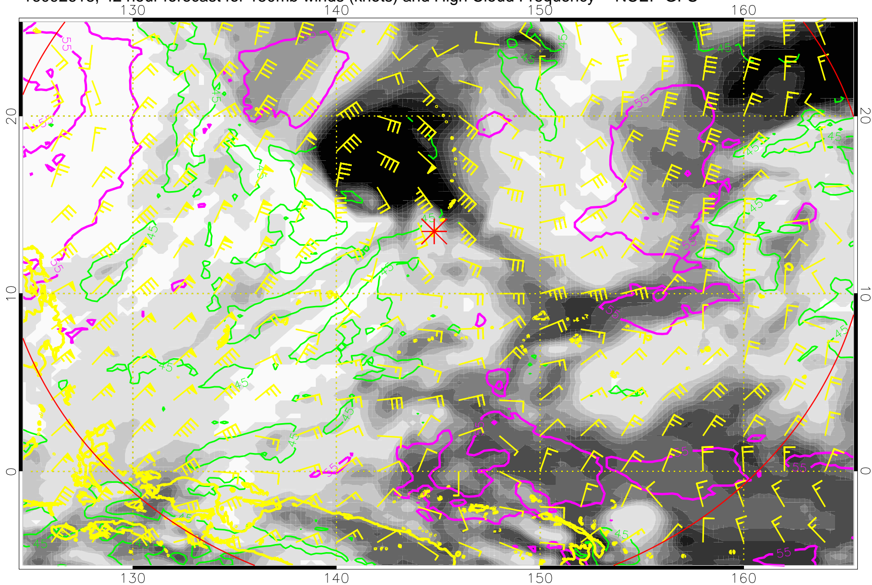
16092618, 42 hour forecast for 150mb winds (knots) and High Cloud Frequency -- NCEP GFS
