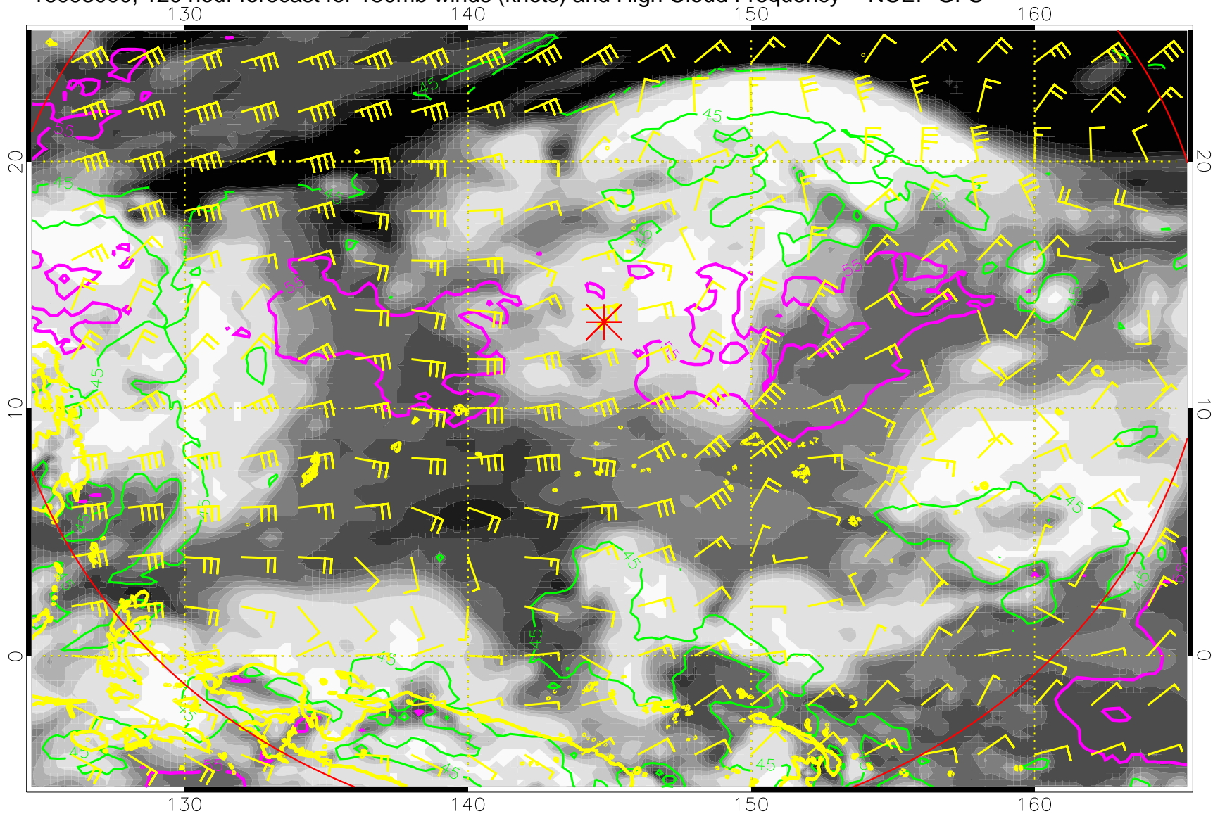
16093000, 120 hour forecast for 150mb winds (knots) and High Cloud Frequency -- NCEP GFS
