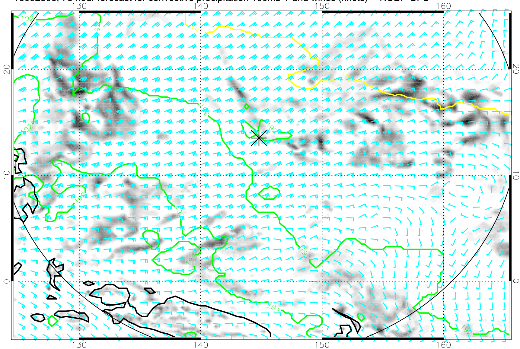
16092806, 78 hour forecast for convective precipitation 100mb T and winds (knots) -- NCEP GFS
