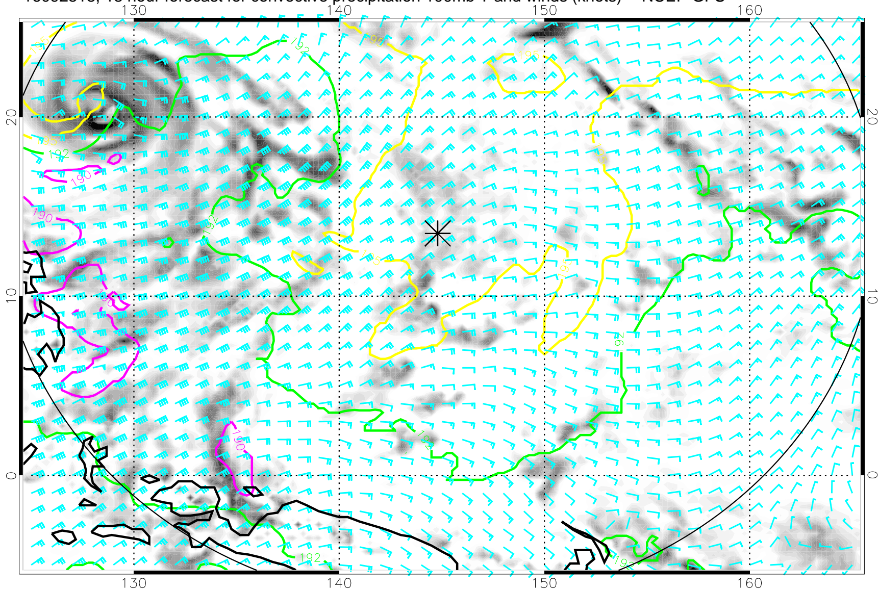
16092518, 18 hour forecast for convective precipitation 100mb T and winds (knots) -- NCEP GFS
