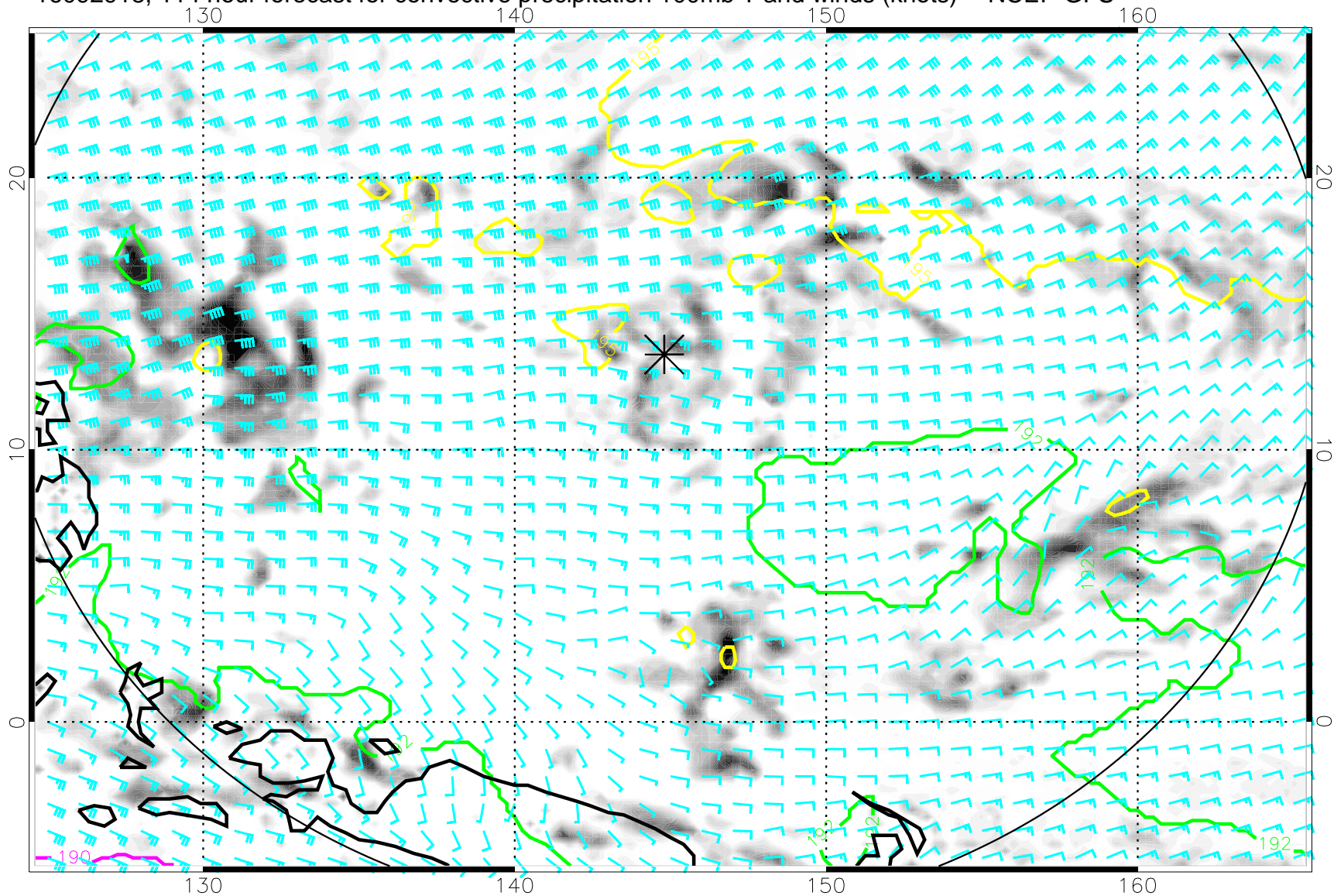
16092918, 114 hour forecast for convective precipitation 100mb T and winds (knots) -- NCEP GFS
