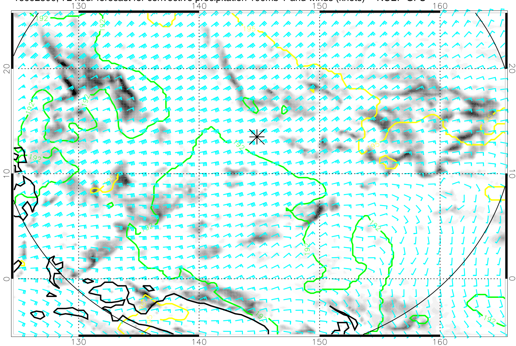
16092800, 72 hour forecast for convective precipitation 100mb T and winds (knots) -- NCEP GFS
