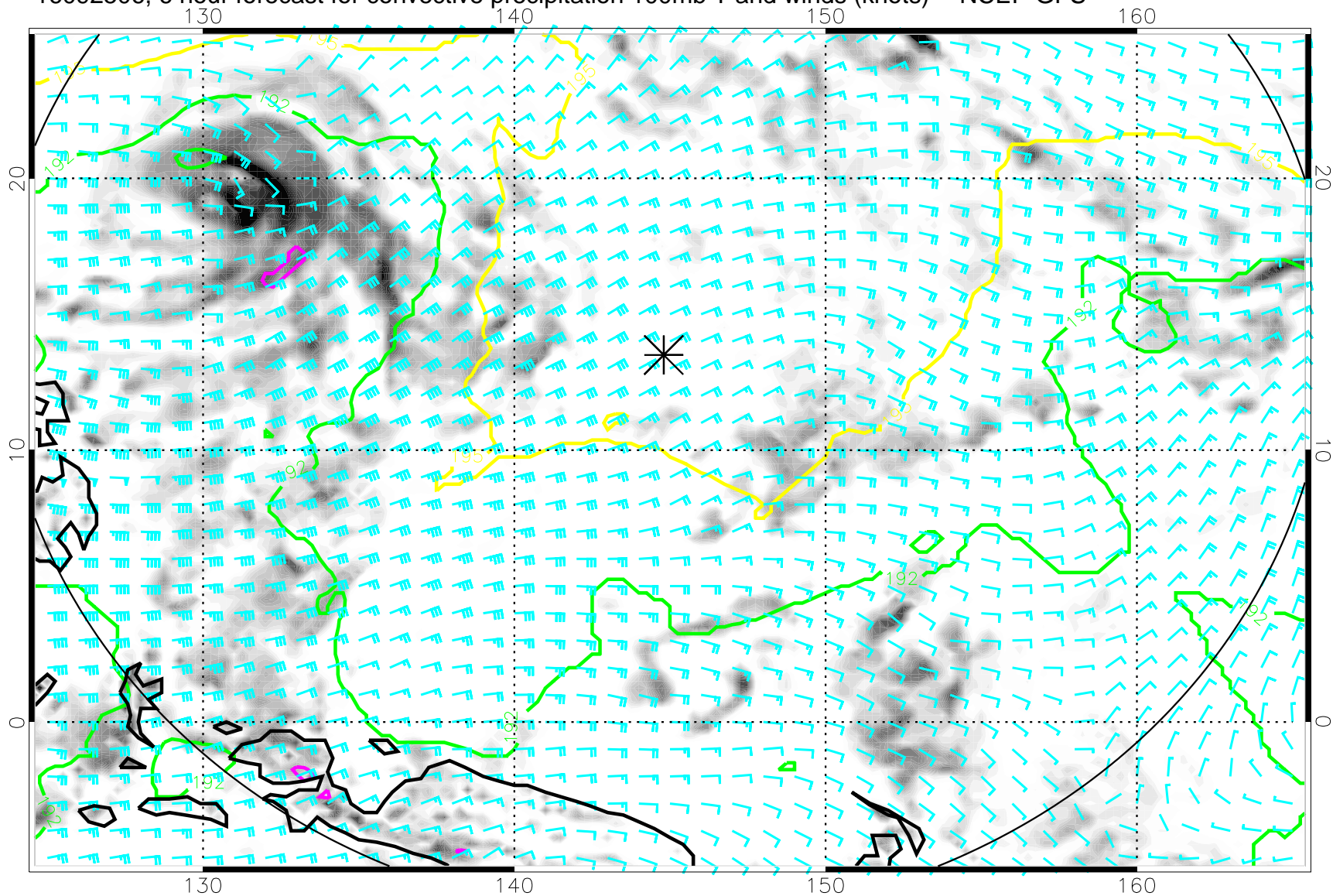
16092506, 6 hour forecast for convective precipitation 100mb T and winds (knots) -- NCEP GFS
