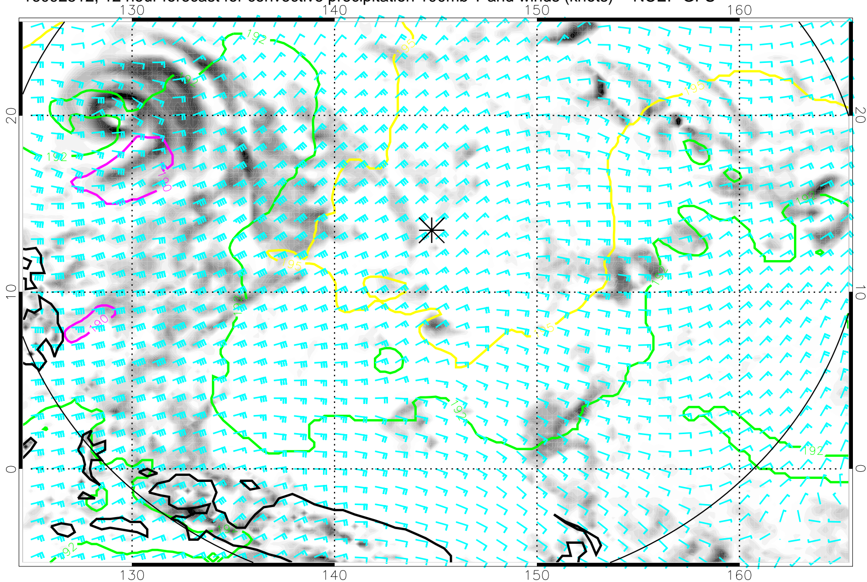
16092512, 12 hour forecast for convective precipitation 100mb T and winds (knots) -- NCEP GFS
