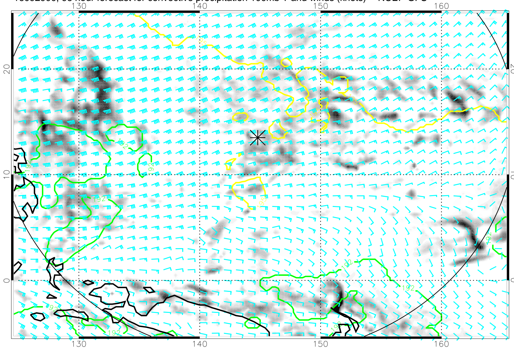
16092900, 96 hour forecast for convective precipitation 100mb T and winds (knots) -- NCEP GFS
