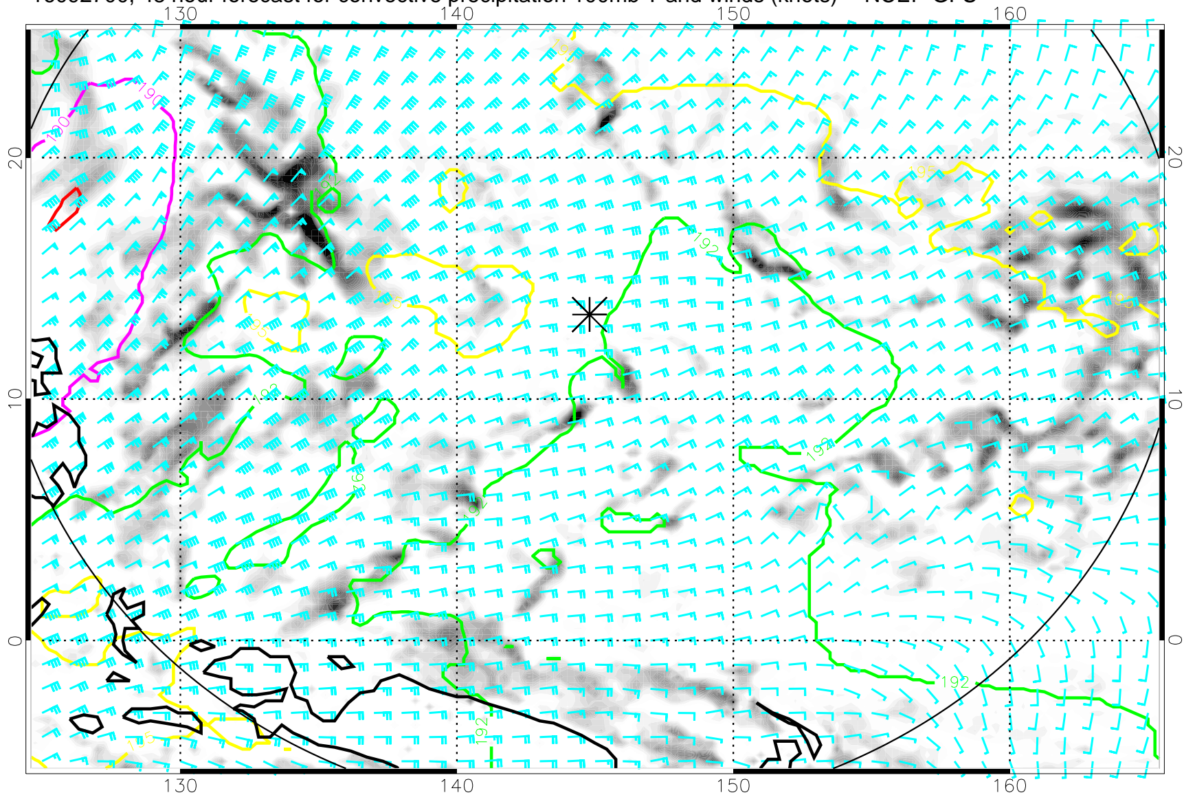
16092700, 48 hour forecast for convective precipitation 100mb T and winds (knots) -- NCEP GFS
