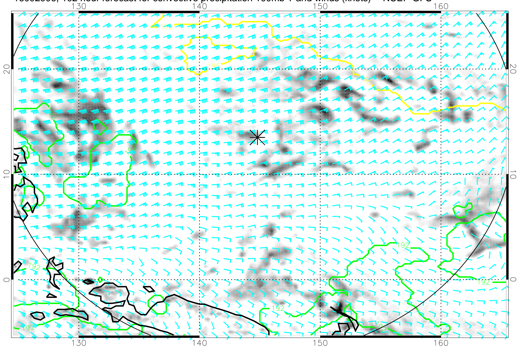
16092906, 102 hour forecast for convective precipitation 100mb T and winds (knots) -- NCEP GFS
