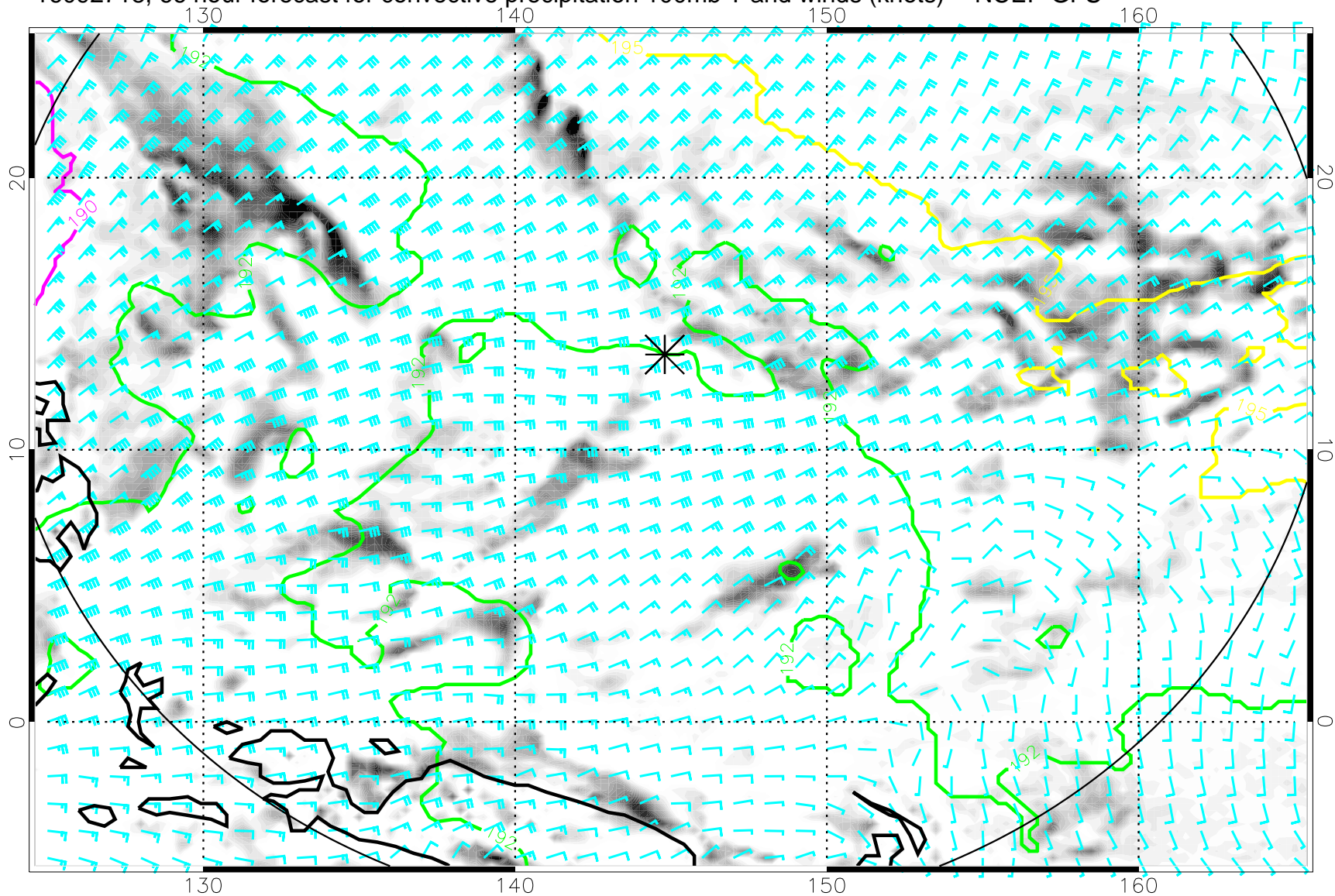
16092718, 66 hour forecast for convective precipitation 100mb T and winds (knots) -- NCEP GFS
