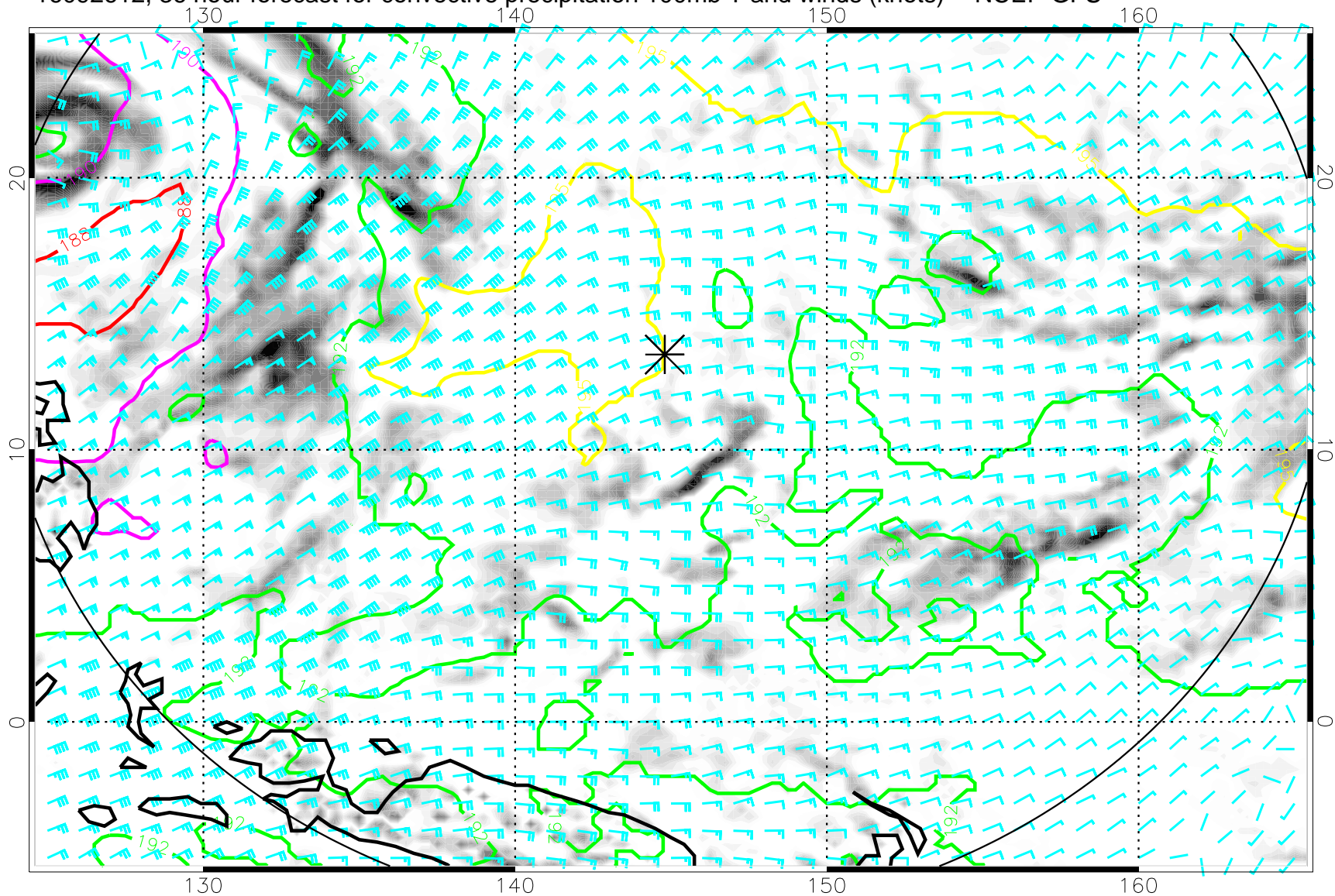
16092612, 36 hour forecast for convective precipitation 100mb T and winds (knots) -- NCEP GFS
