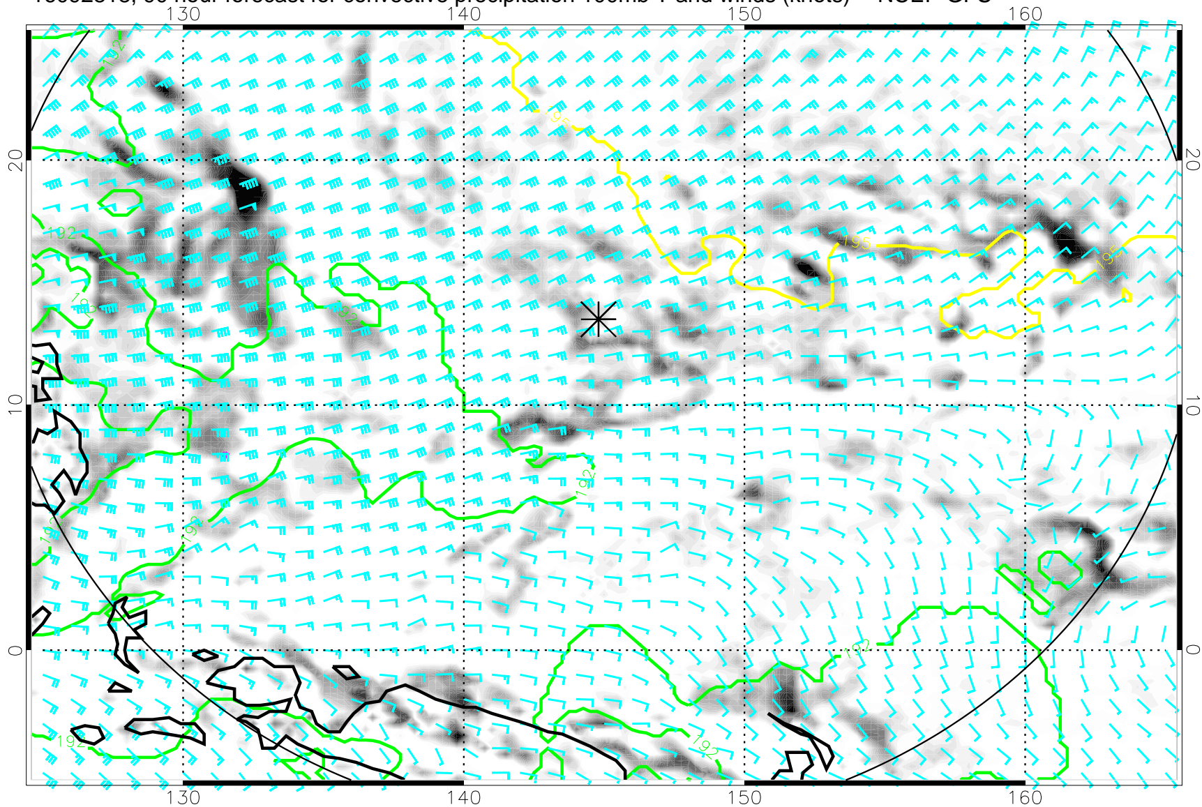
16092818, 90 hour forecast for convective precipitation 100mb T and winds (knots) -- NCEP GFS
