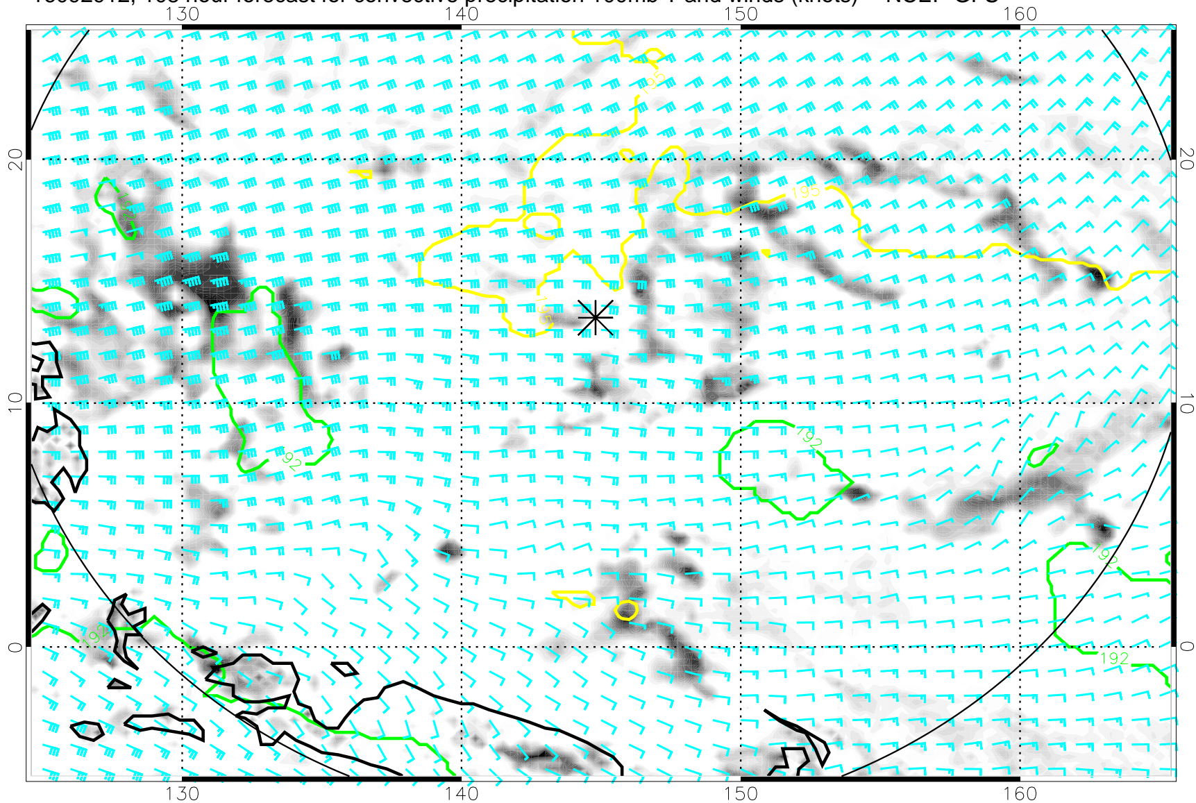
16092912, 108 hour forecast for convective precipitation 100mb T and winds (knots) -- NCEP GFS
