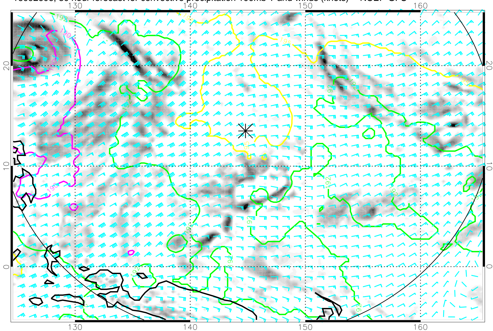
16092606, 30 hour forecast for convective precipitation 100mb T and winds (knots) -- NCEP GFS
