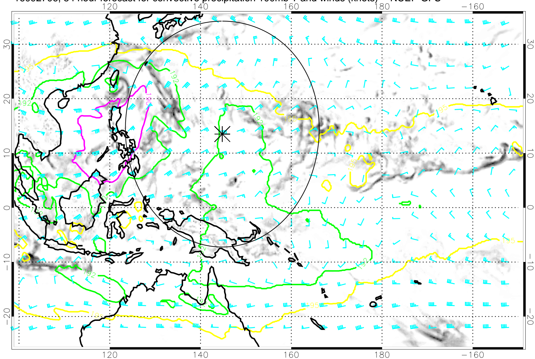
16092706, 54 hour forecast for convective precipitation 100mb T and winds (knots) -- NCEP GFS
