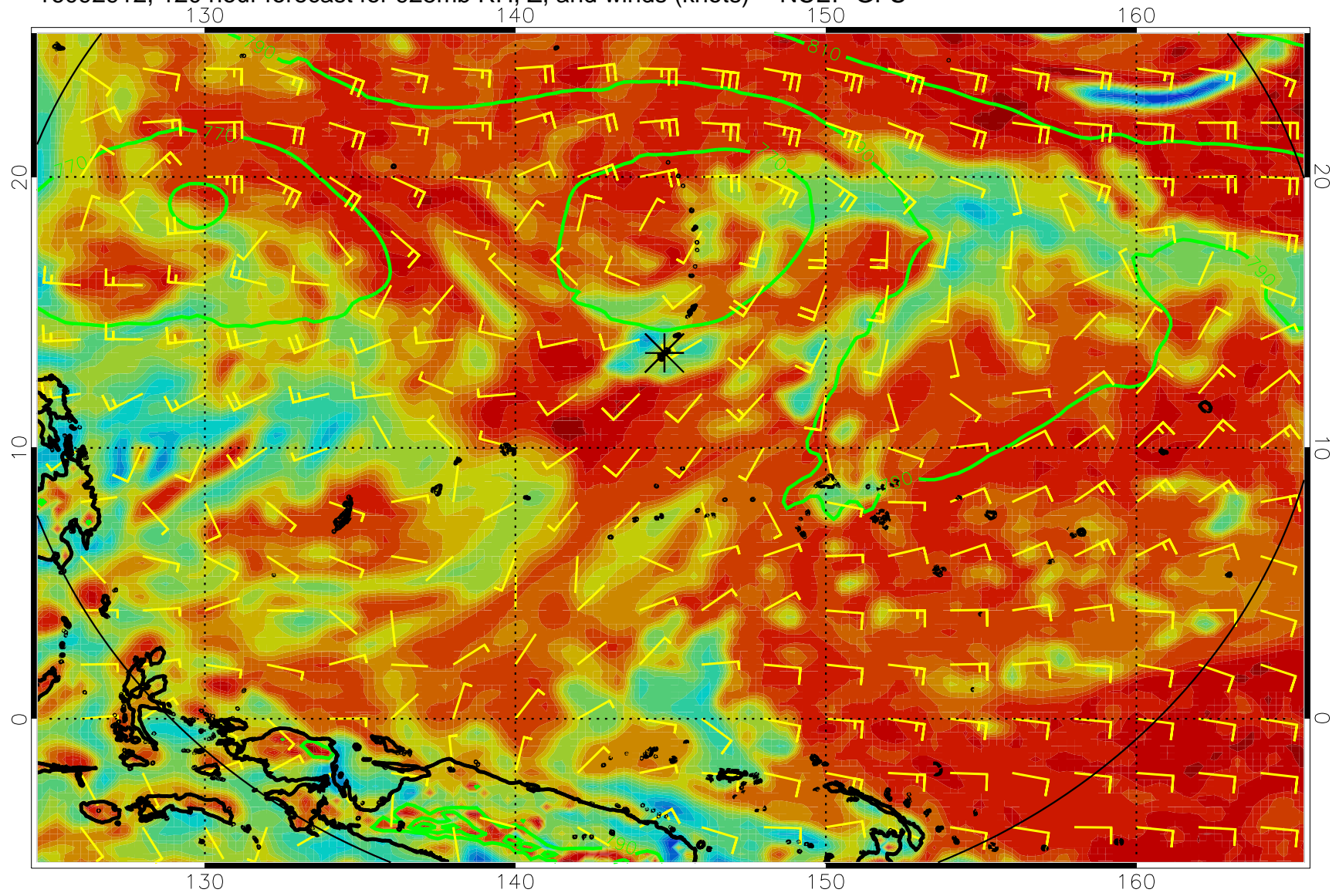
16092912, 120 hour forecast for 925mb RH, Z, and winds (knots) -- NCEP GFS
