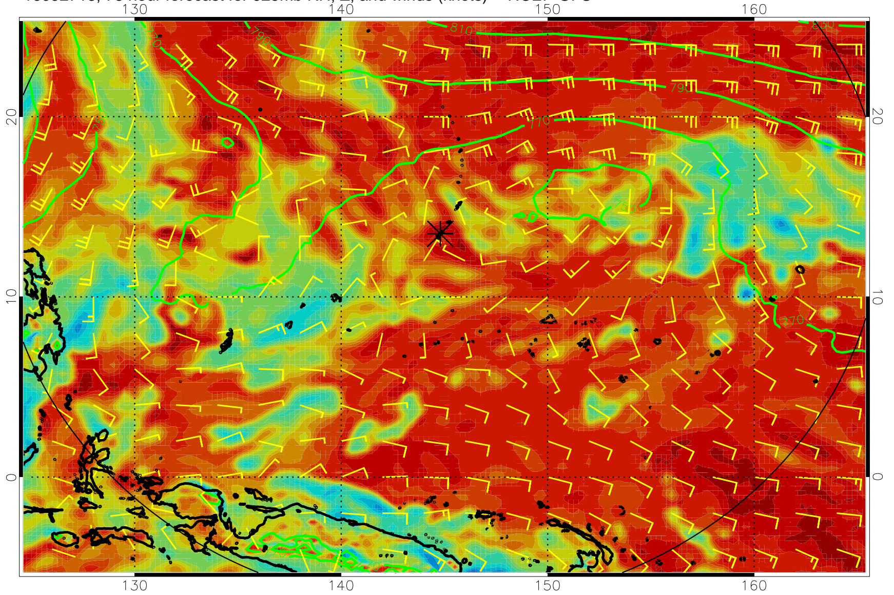
16092718, 78 hour forecast for 925mb RH, Z, and winds (knots) -- NCEP GFS
