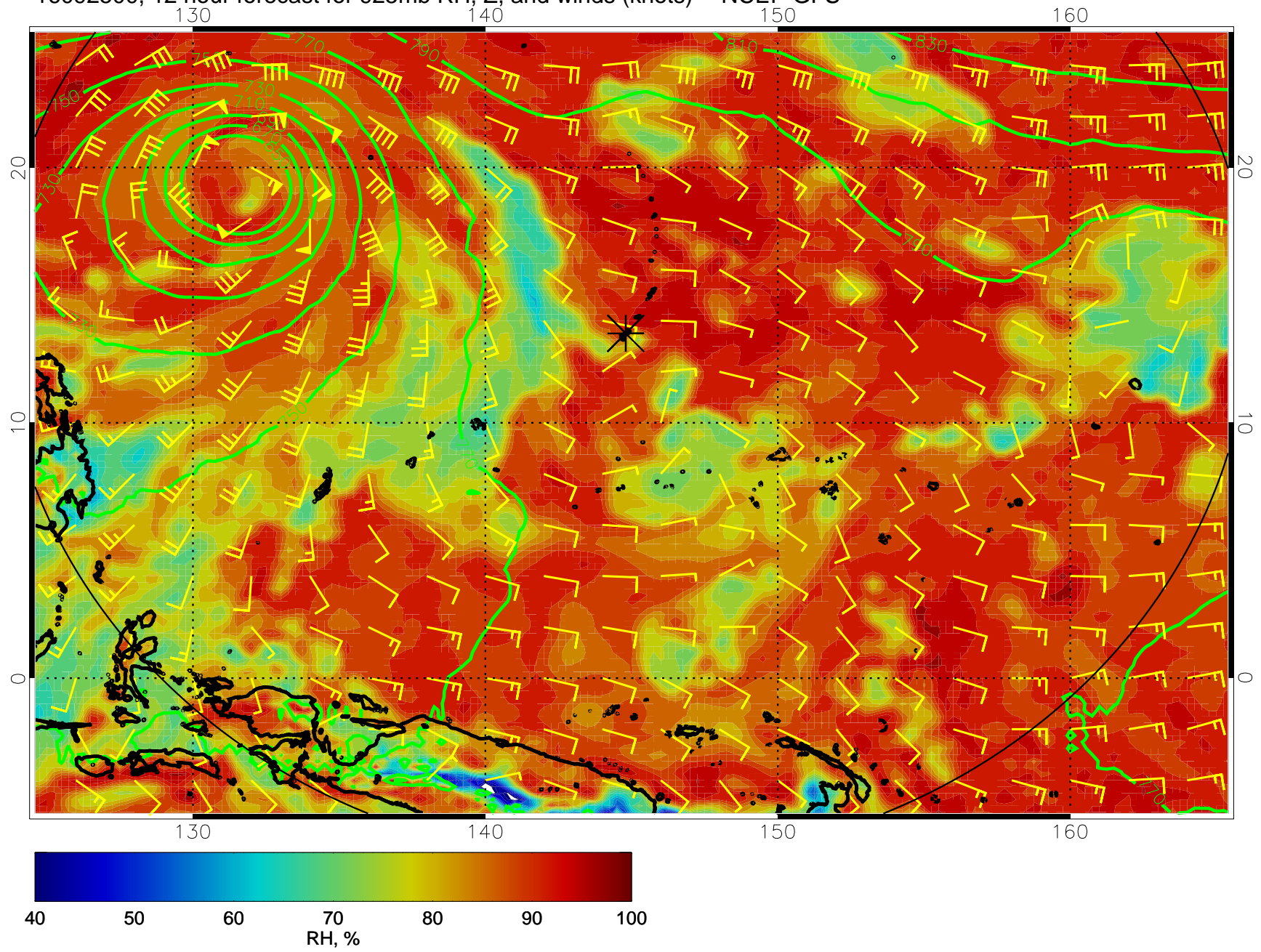
16092500, 12 hour forecast for 925mb RH, Z, and winds (knots) -- NCEP GFS
