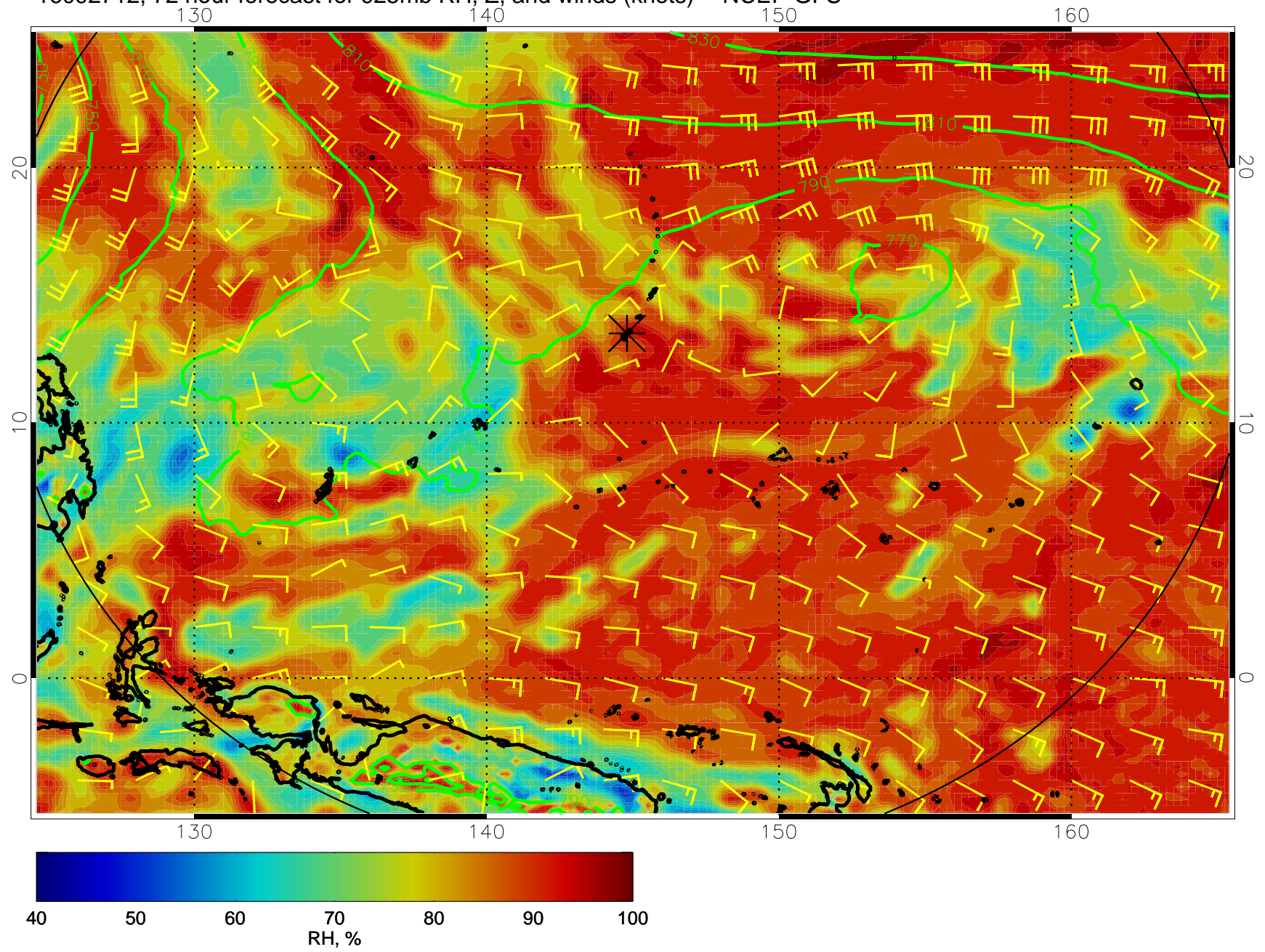
16092712, 72 hour forecast for 925mb RH, Z, and winds (knots) -- NCEP GFS
