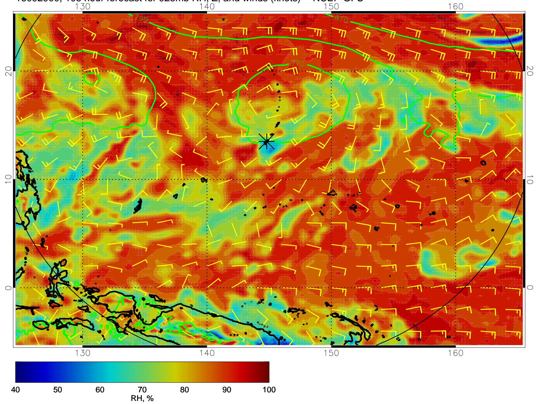
16092900, 108 hour forecast for 925mb RH, Z, and winds (knots) -- NCEP GFS
