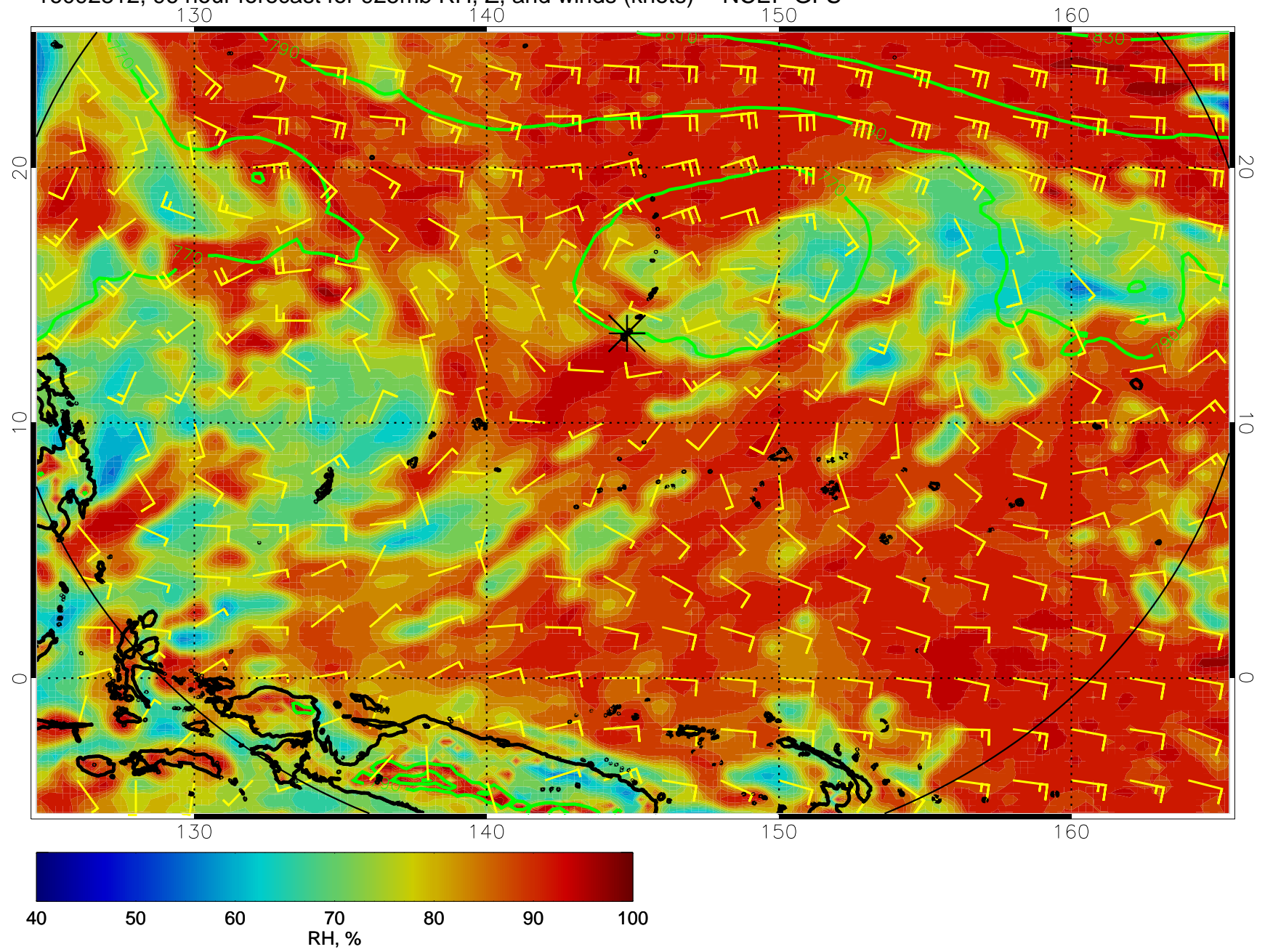
16092812, 96 hour forecast for 925mb RH, Z, and winds (knots) -- NCEP GFS
