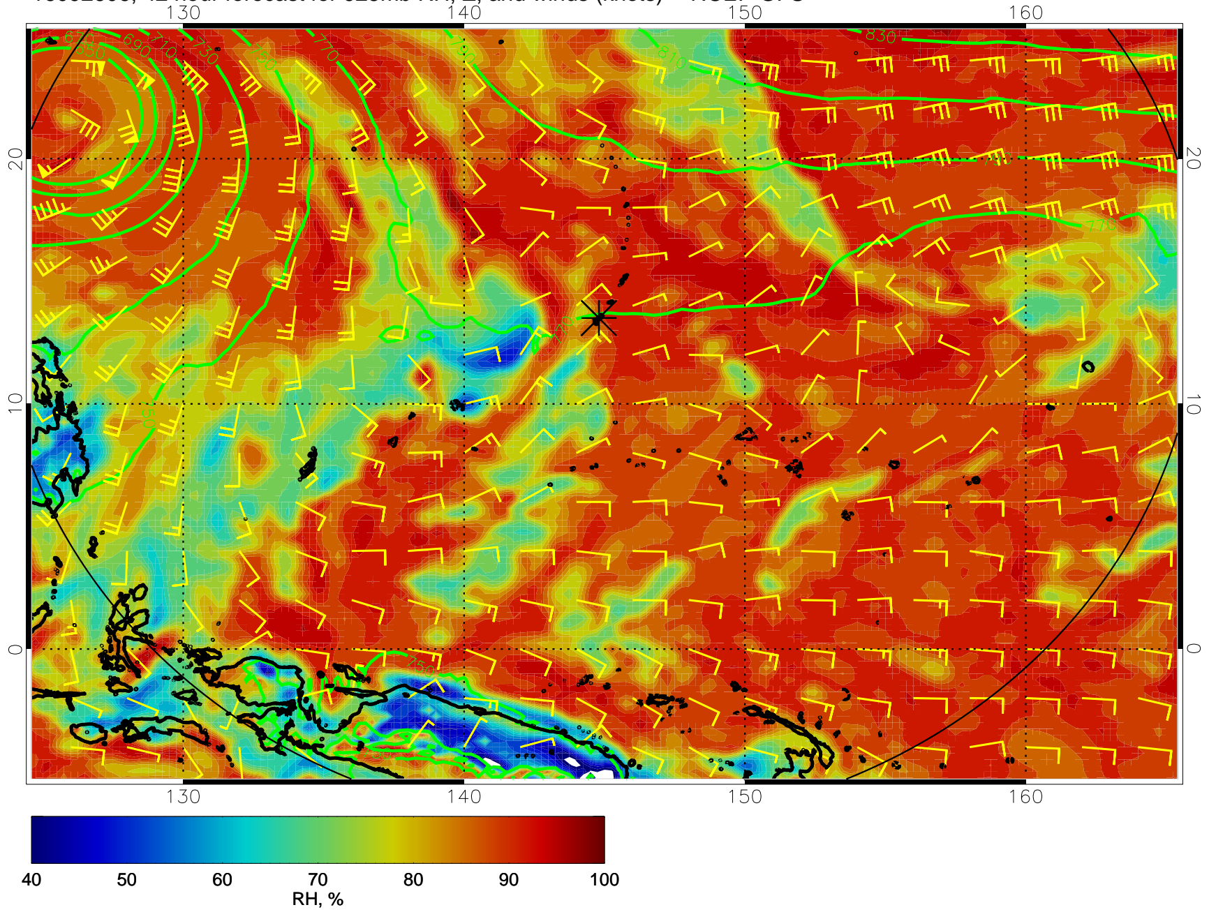
16092606, 42 hour forecast for 925mb RH, Z, and winds (knots) -- NCEP GFS
