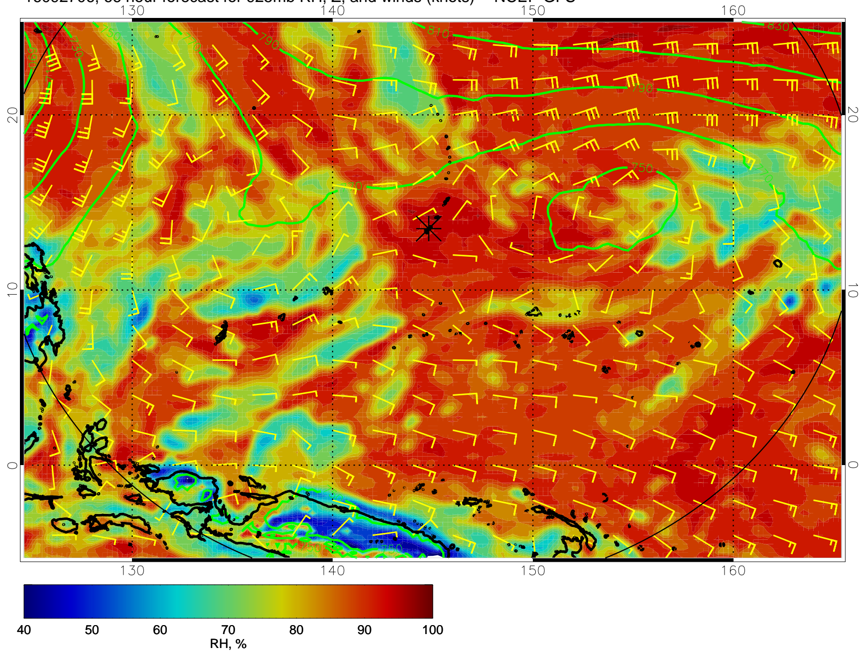
16092706, 66 hour forecast for 925mb RH, Z, and winds (knots) -- NCEP GFS
