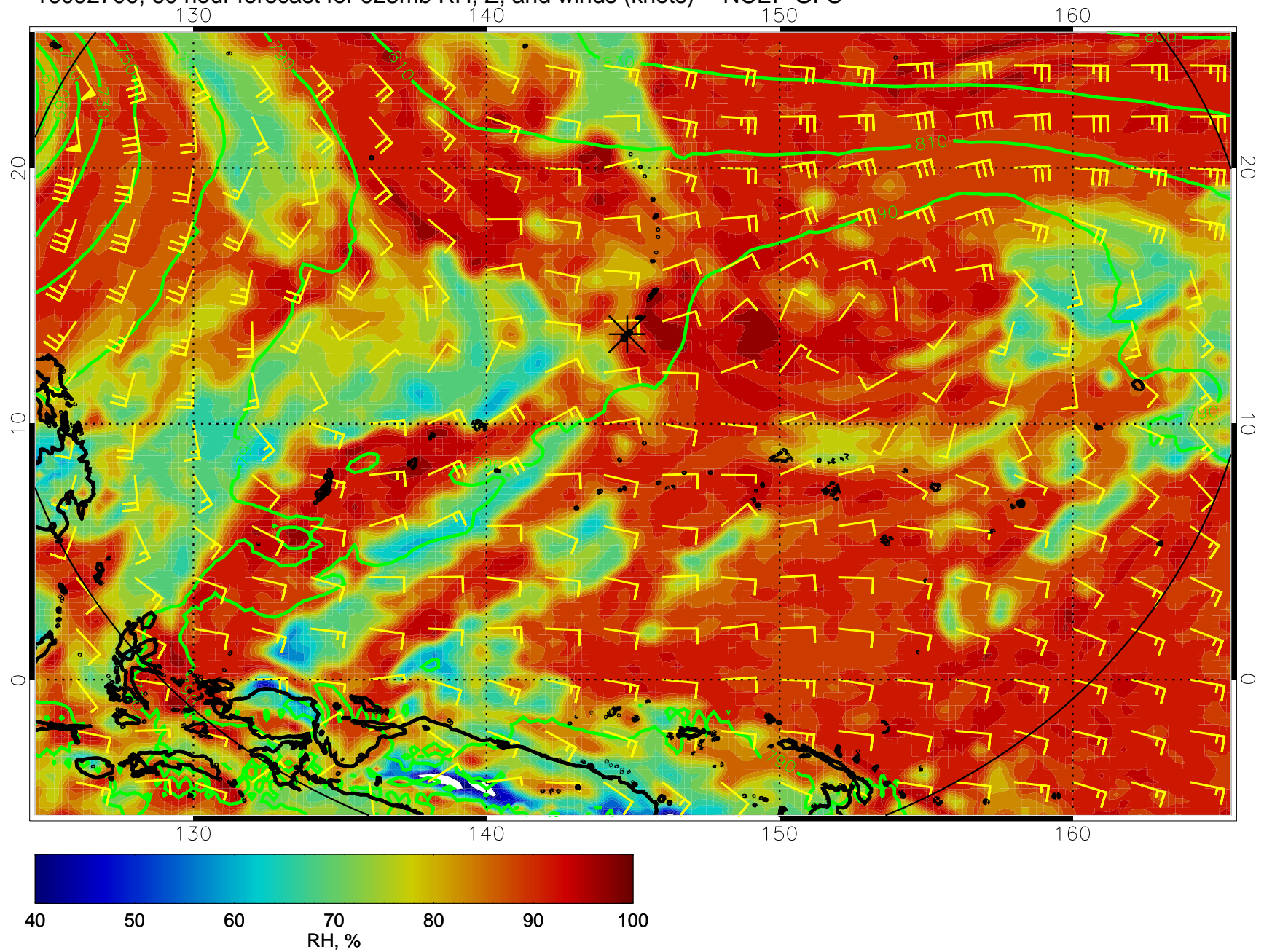
16092700, 60 hour forecast for 925mb RH, Z, and winds (knots) -- NCEP GFS
