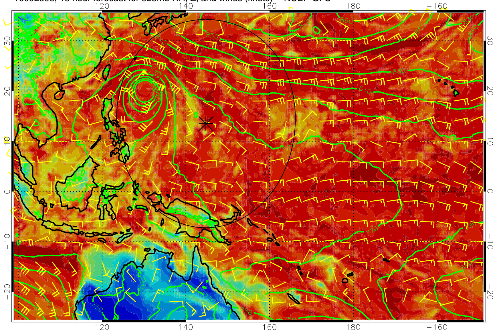
16092506, 18 hour forecast for 925mb RH, Z, and winds (knots) -- NCEP GFS
