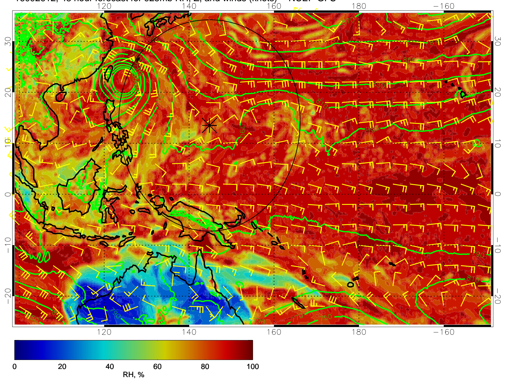
16092612, 48 hour forecast for 925mb RH, Z, and winds (knots) -- NCEP GFS
