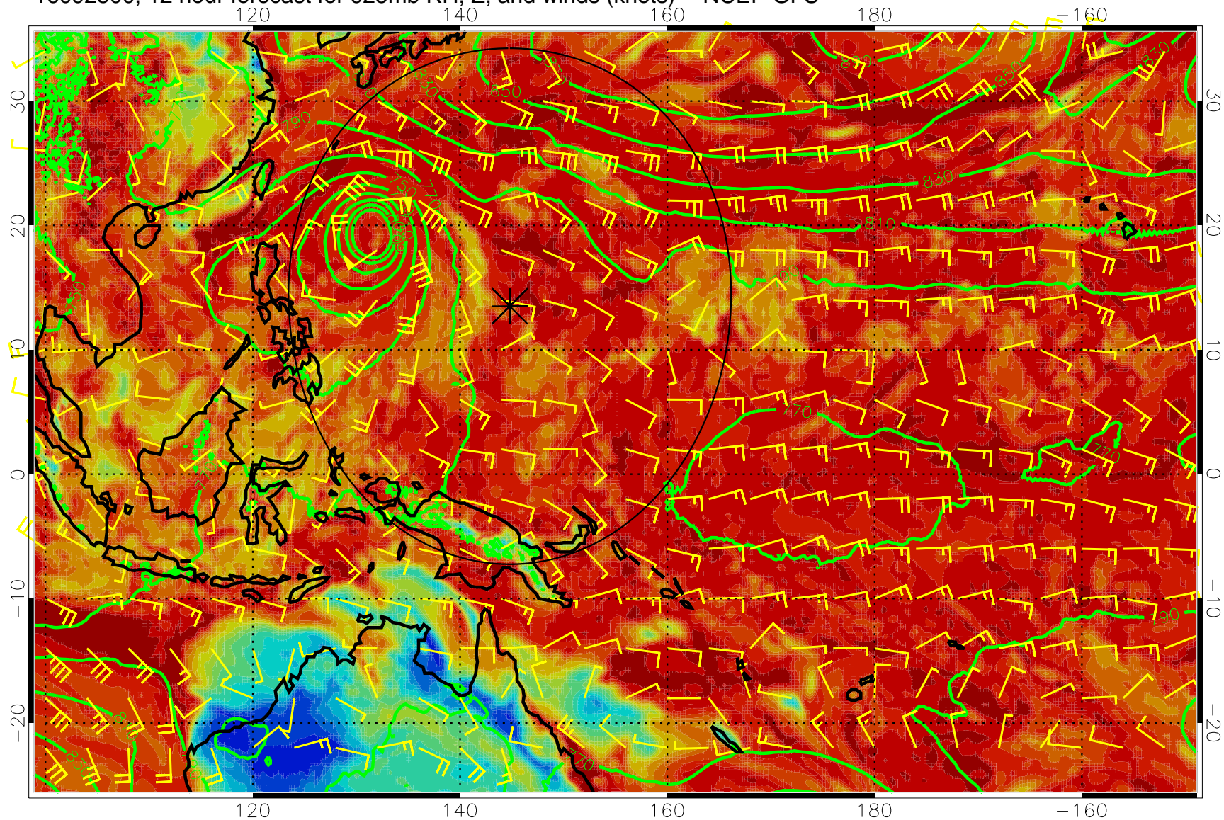
16092500, 12 hour forecast for 925mb RH, Z, and winds (knots) -- NCEP GFS
