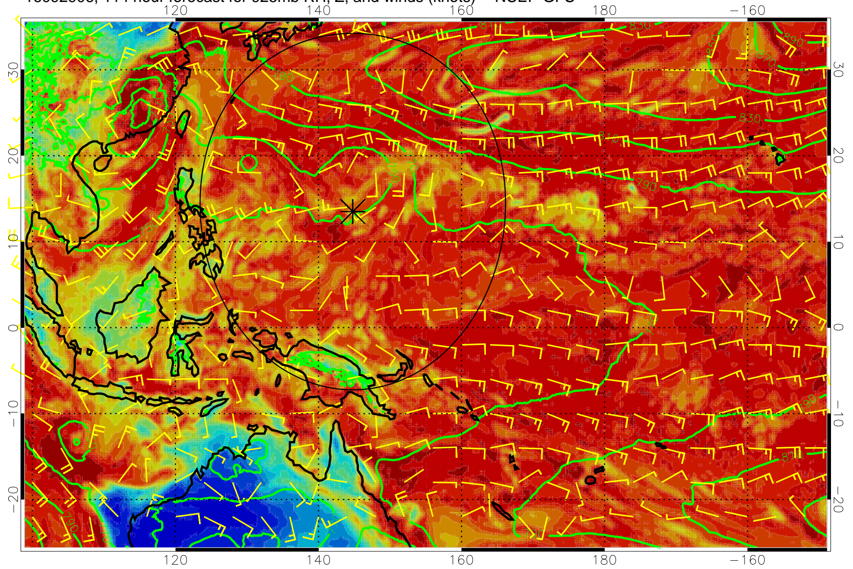
16092906, 114 hour forecast for 925mb RH, Z, and winds (knots) -- NCEP GFS
