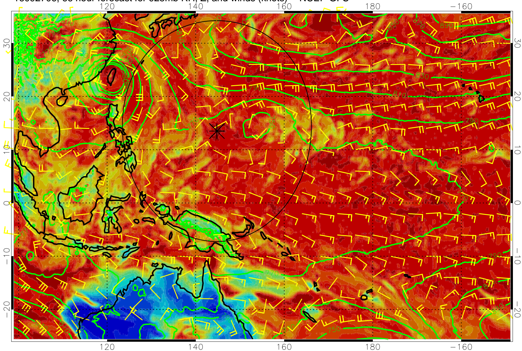
16092706, 66 hour forecast for 925mb RH, Z, and winds (knots) -- NCEP GFS
