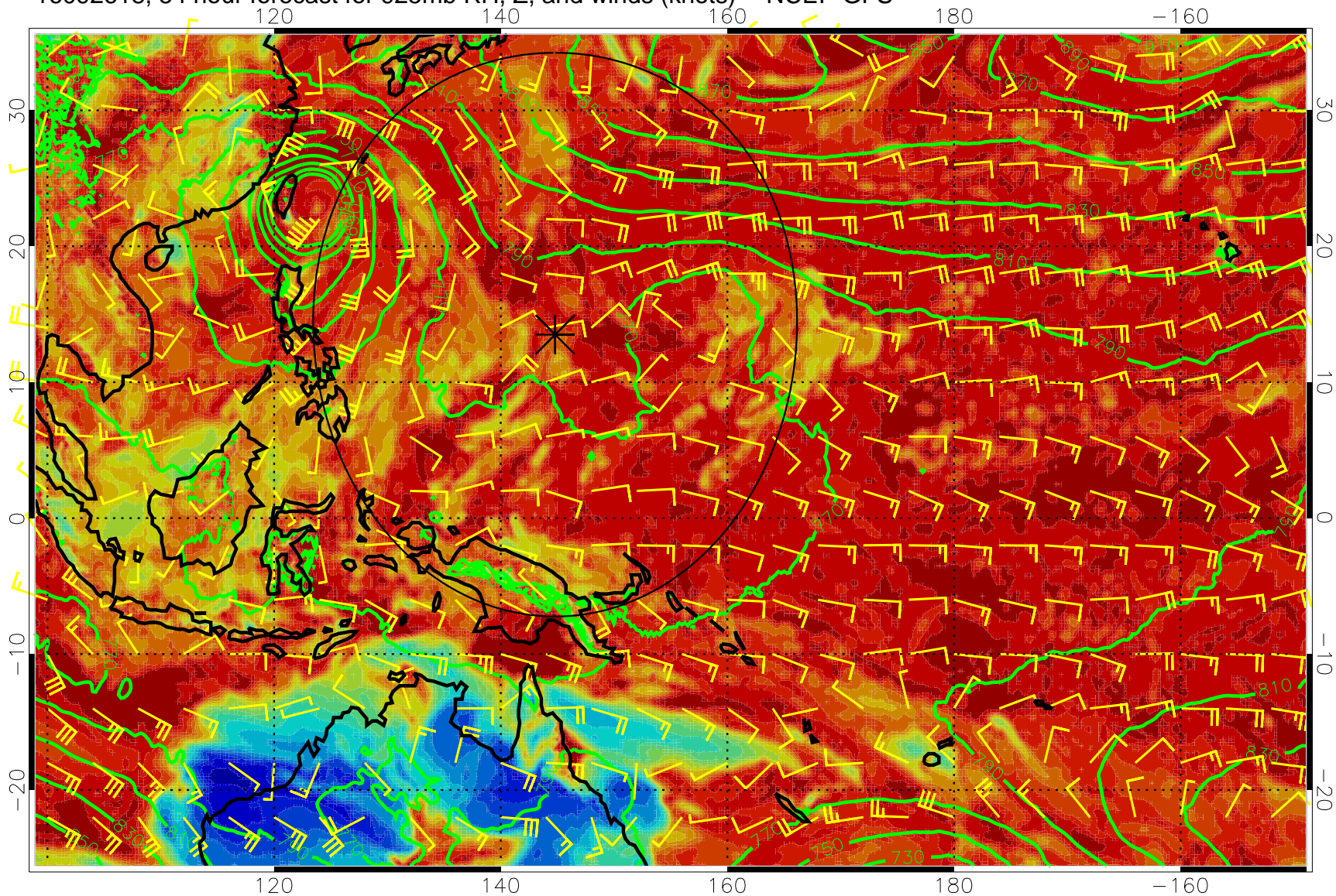
16092618, 54 hour forecast for 925mb RH, Z, and winds (knots) -- NCEP GFS
