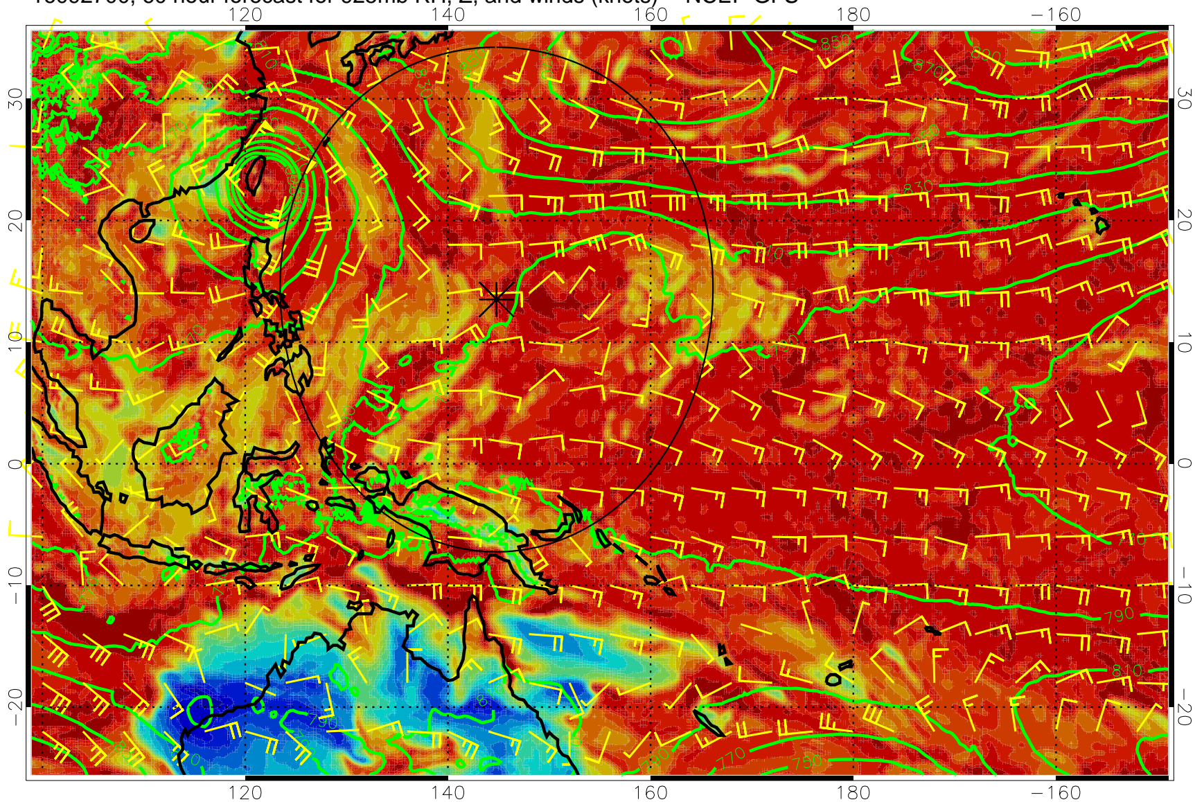
16092700, 60 hour forecast for 925mb RH, Z, and winds (knots) -- NCEP GFS
