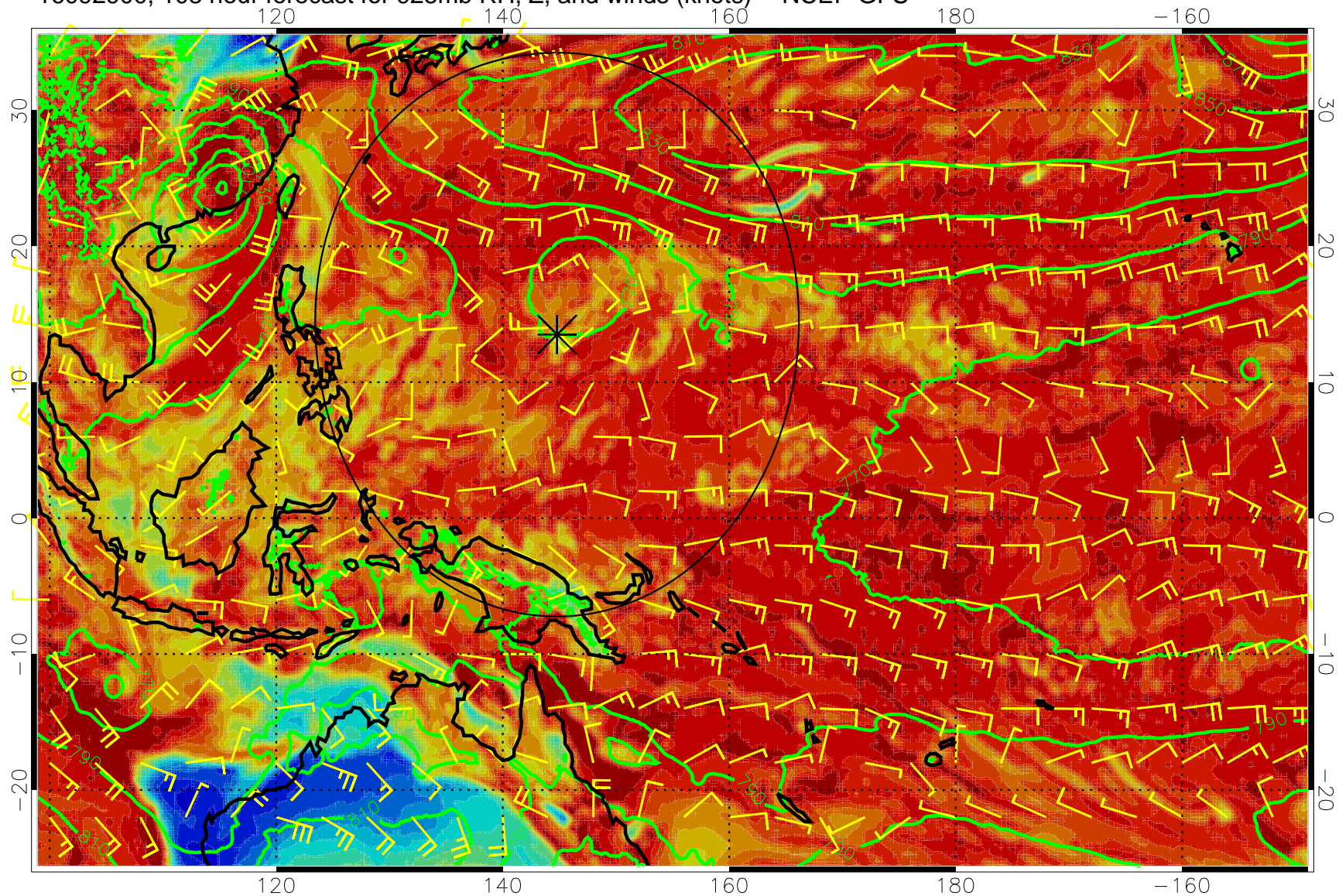
16092900, 108 hour forecast for 925mb RH, Z, and winds (knots) -- NCEP GFS
