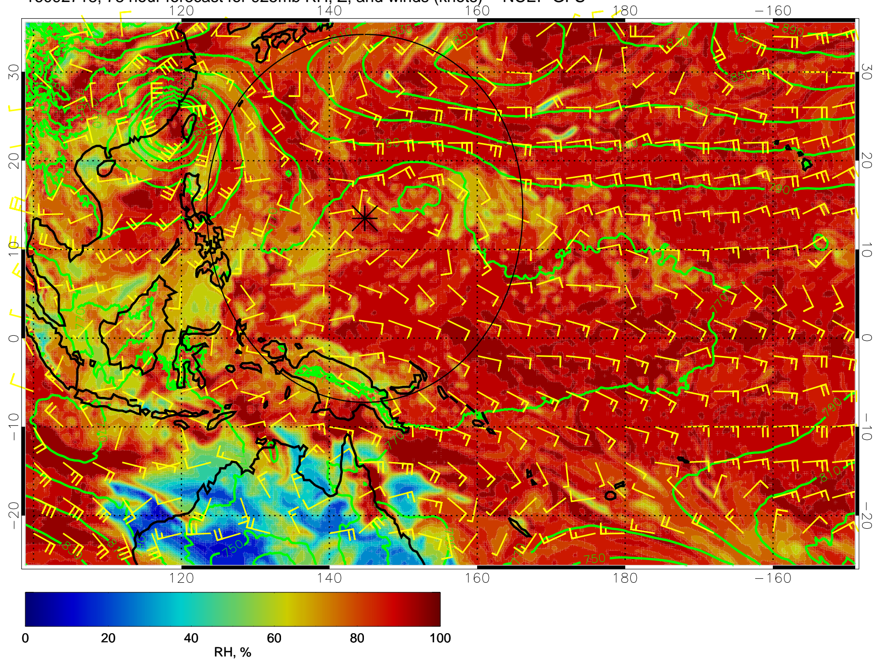
16092718, 78 hour forecast for 925mb RH, Z, and winds (knots) -- NCEP GFS
