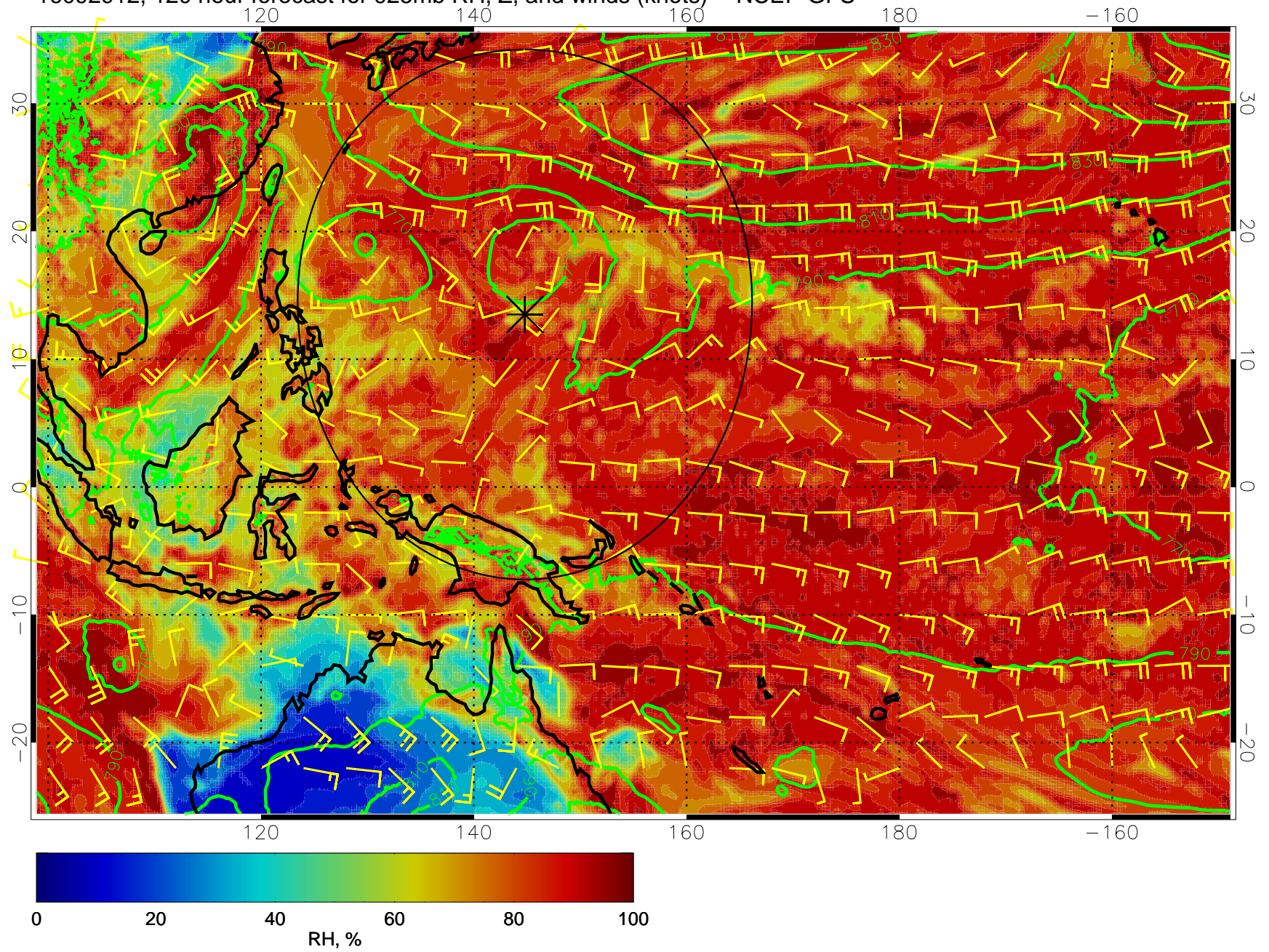
16092912, 120 hour forecast for 925mb RH, Z, and winds (knots) -- NCEP GFS
