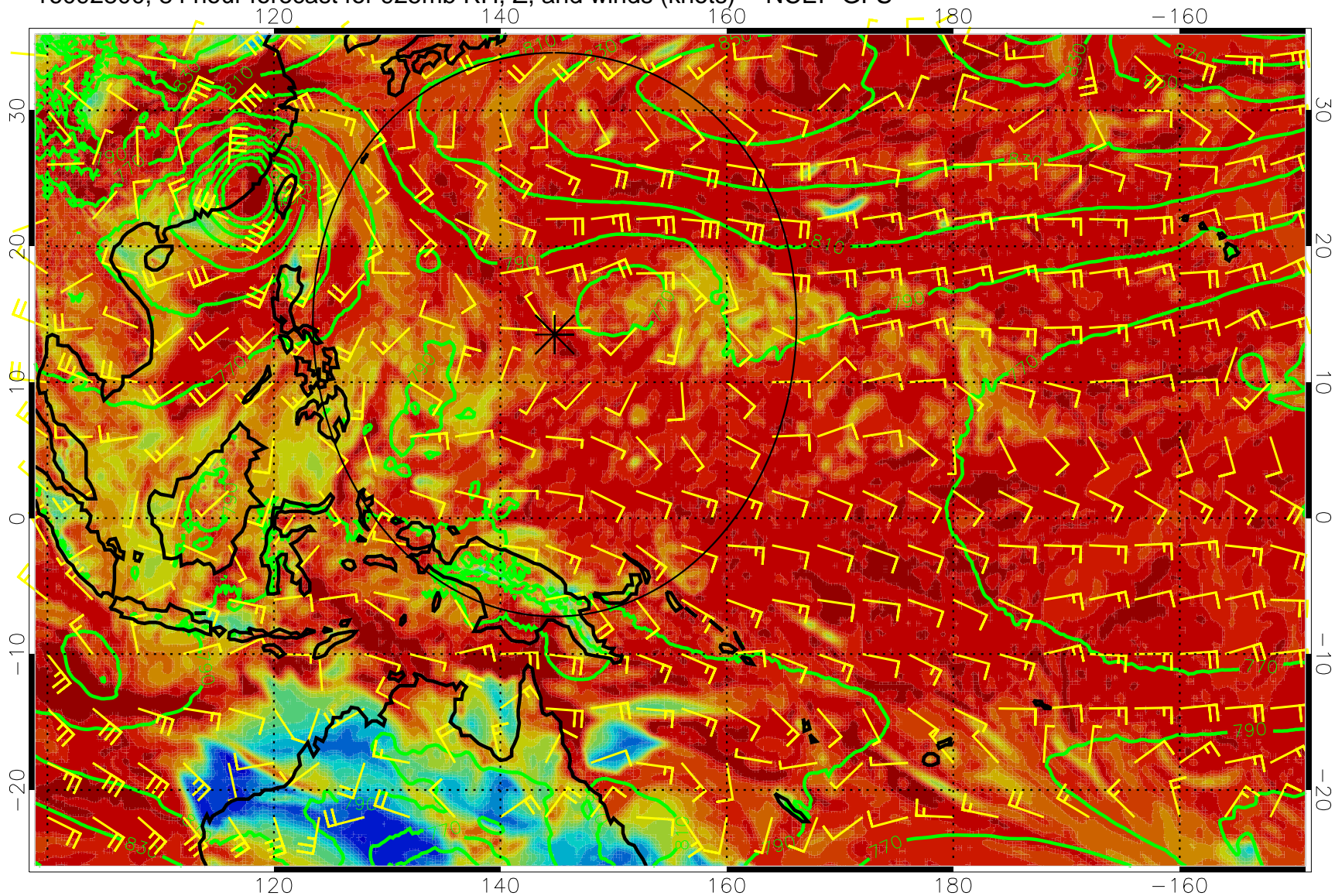
16092800, 84 hour forecast for 925mb RH, Z, and winds (knots) -- NCEP GFS
