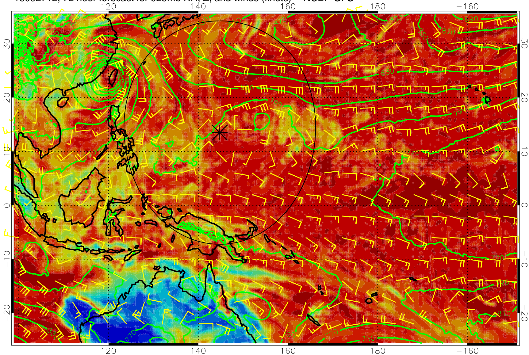
16092712, 72 hour forecast for 925mb RH, Z, and winds (knots) -- NCEP GFS
