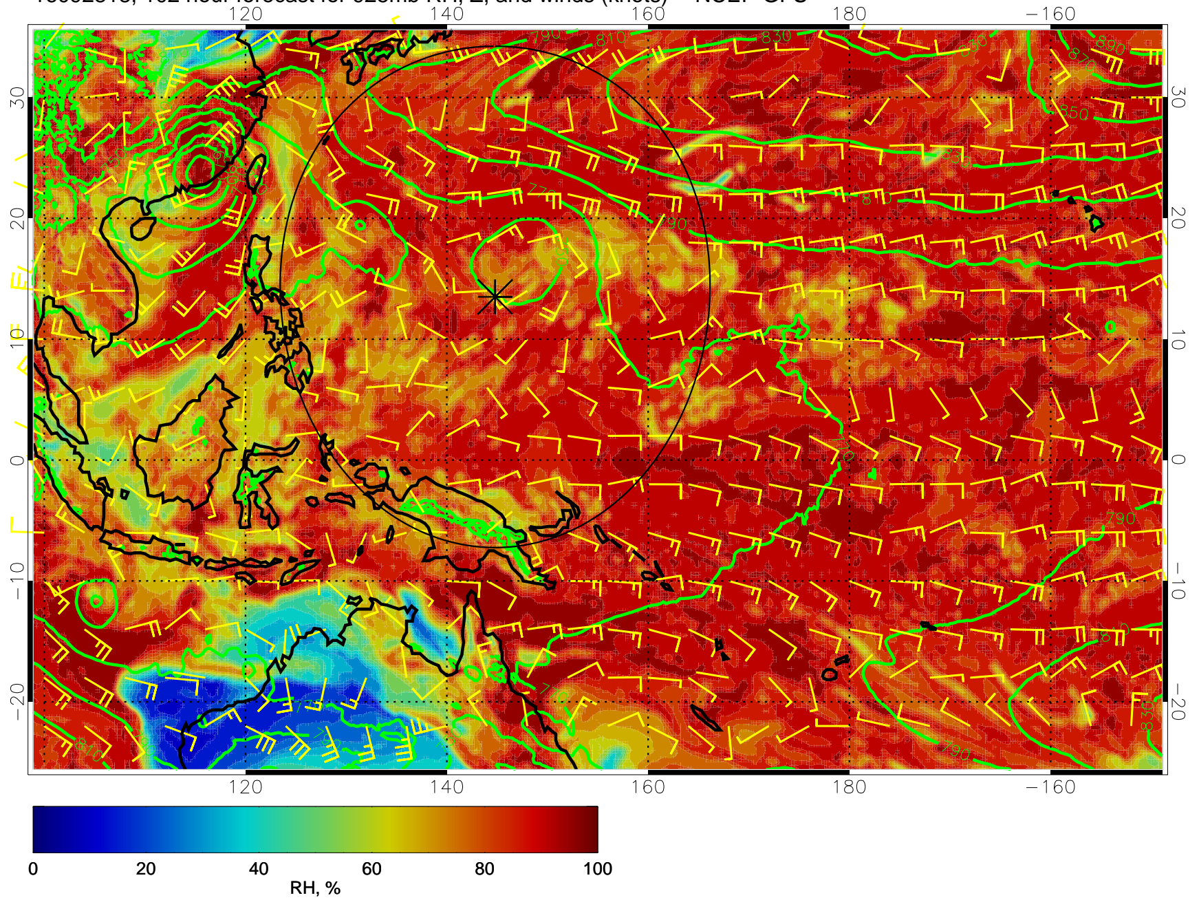
16092818, 102 hour forecast for 925mb RH, Z, and winds (knots) -- NCEP GFS
