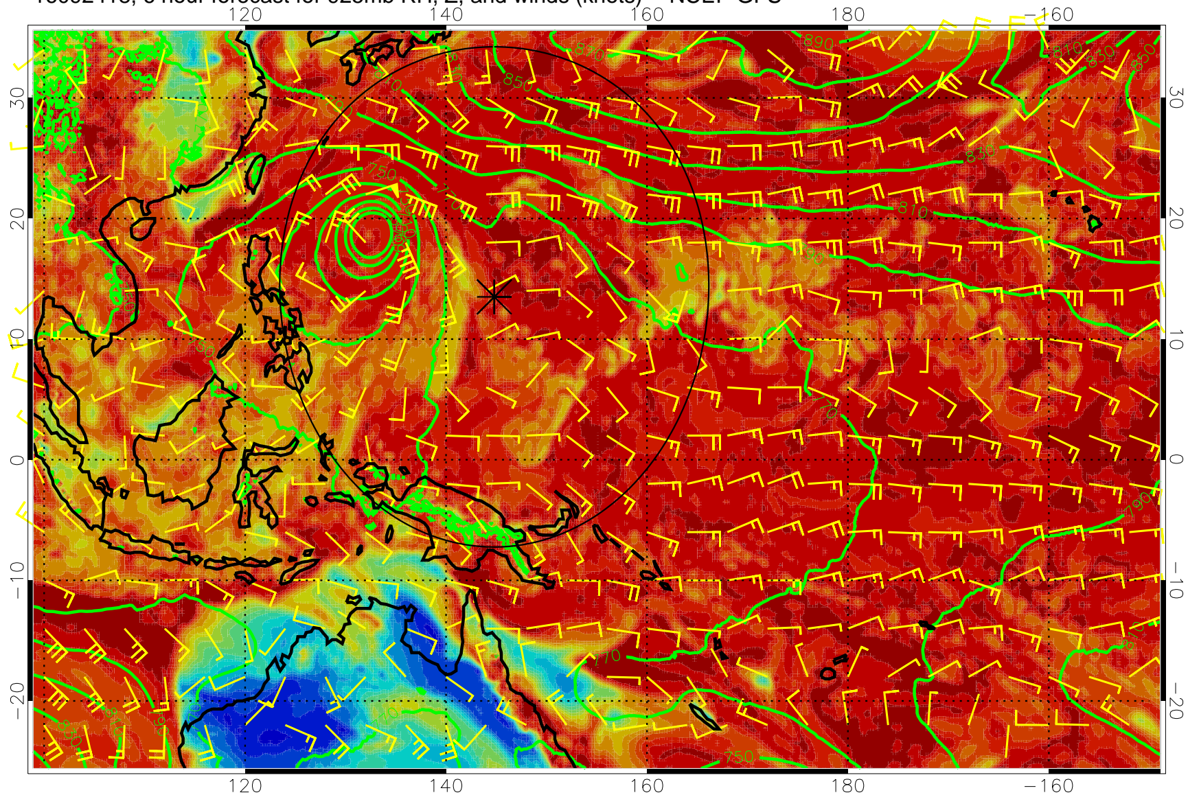
16092418, 6 hour forecast for 925mb RH, Z, and winds (knots) -- NCEP GFS
