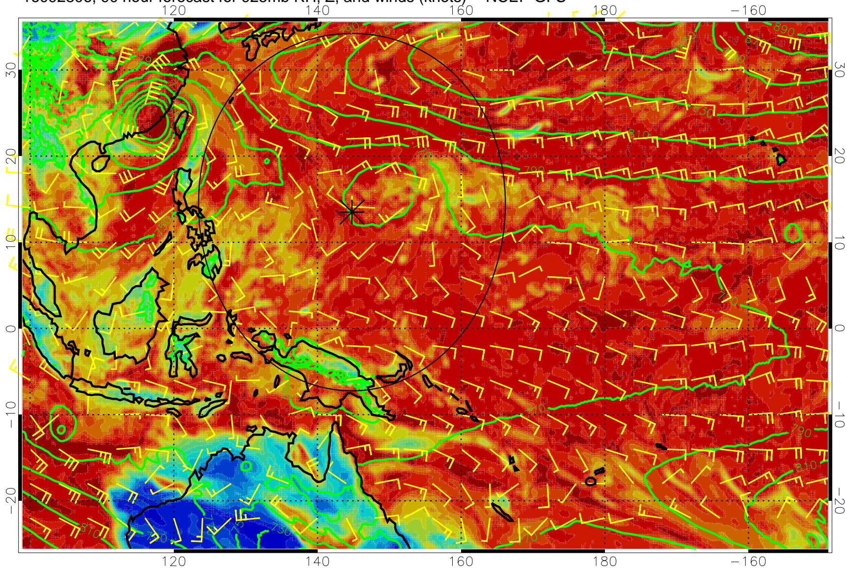
16092806, 90 hour forecast for 925mb RH, Z, and winds (knots) -- NCEP GFS
