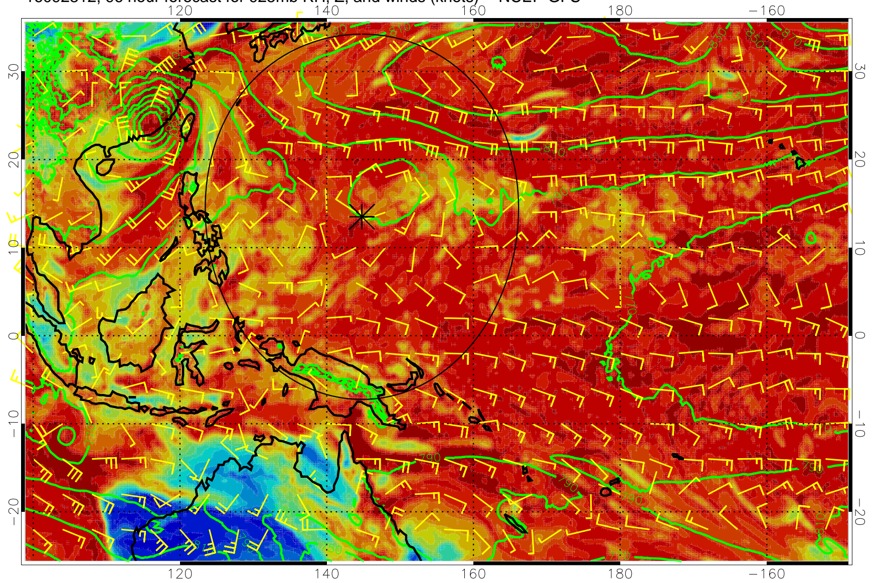
16092812, 96 hour forecast for 925mb RH, Z, and winds (knots) -- NCEP GFS
