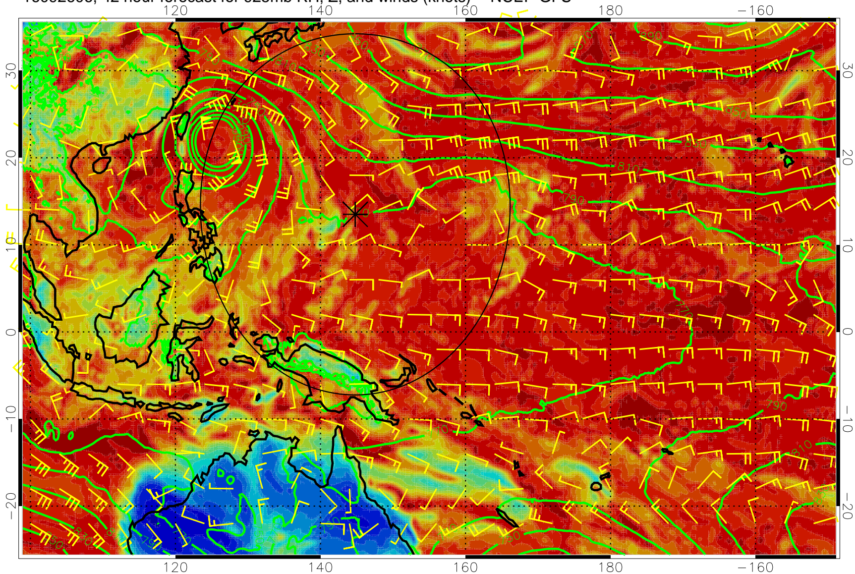
16092606, 42 hour forecast for 925mb RH, Z, and winds (knots) -- NCEP GFS
