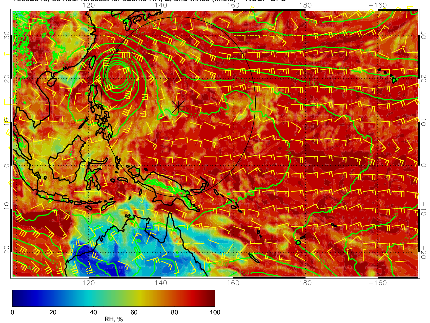
16092518, 30 hour forecast for 925mb RH, Z, and winds (knots) -- NCEP GFS
