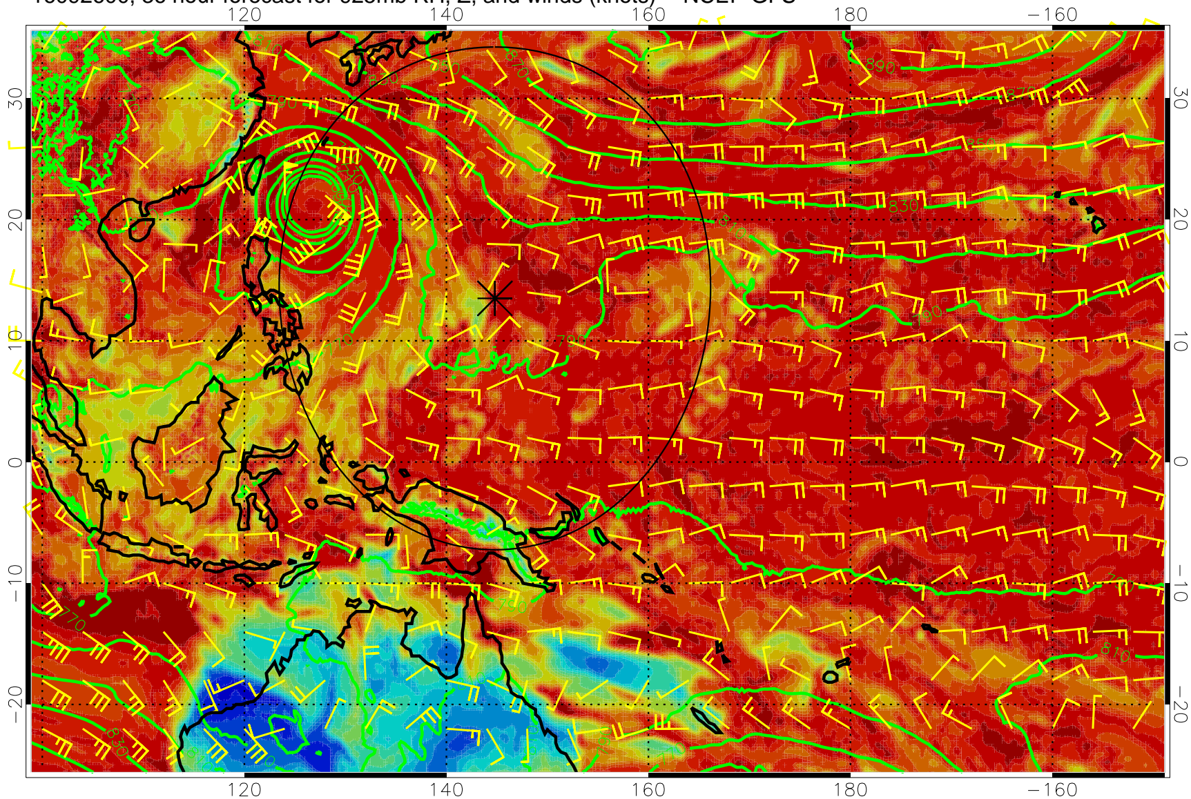
16092600, 36 hour forecast for 925mb RH, Z, and winds (knots) -- NCEP GFS
