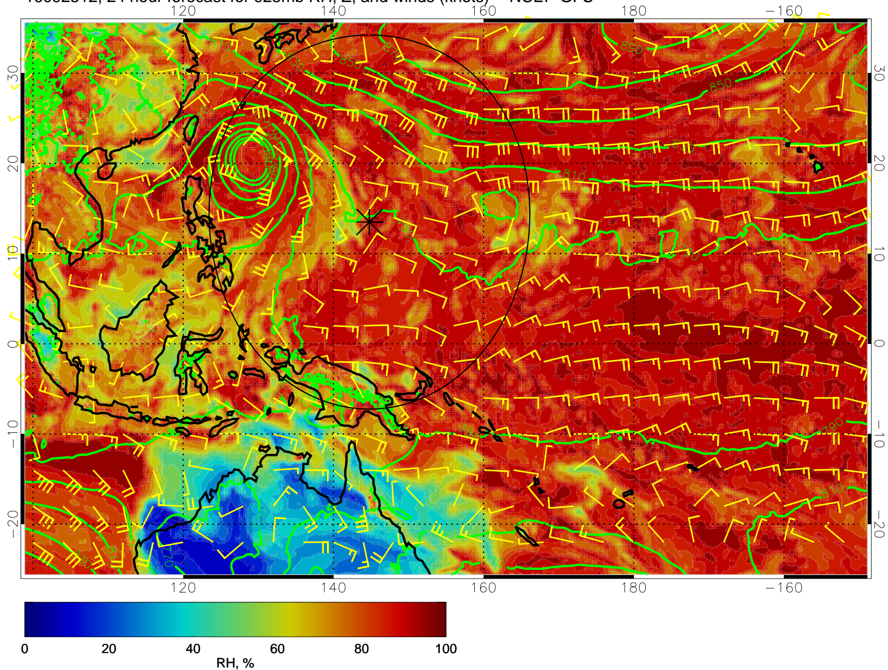
16092512, 24 hour forecast for 925mb RH, Z, and winds (knots) -- NCEP GFS
