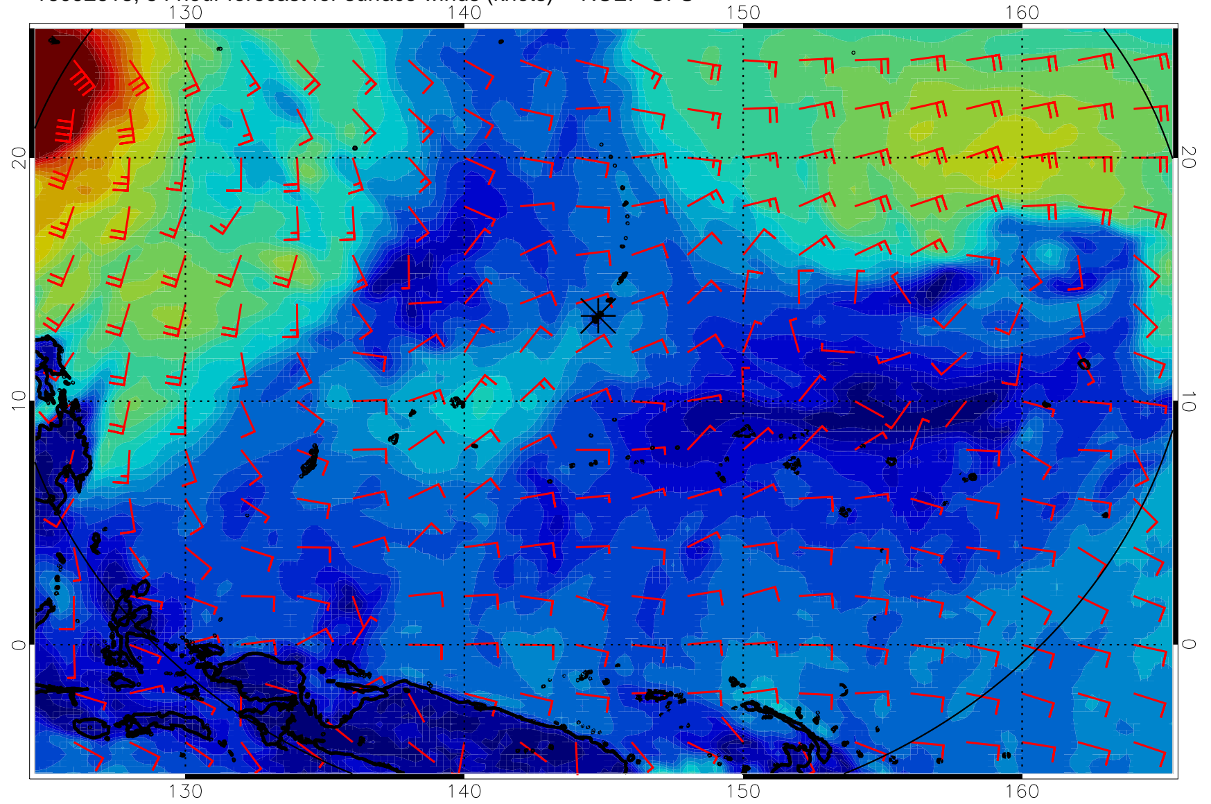
16092618, 54 hour forecast for surface winds (knots) -- NCEP GFS
