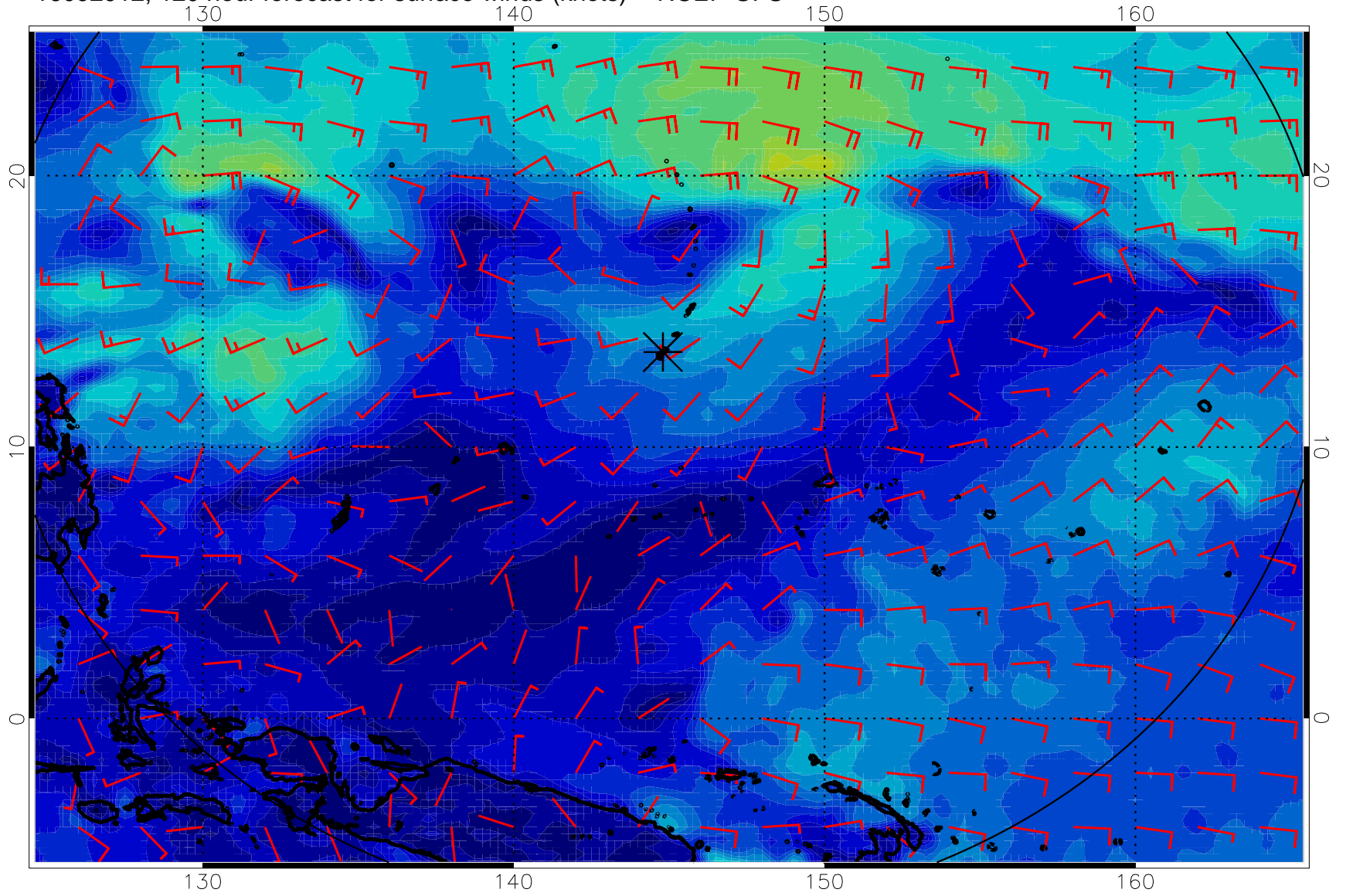
16092912, 120 hour forecast for surface winds (knots) -- NCEP GFS
