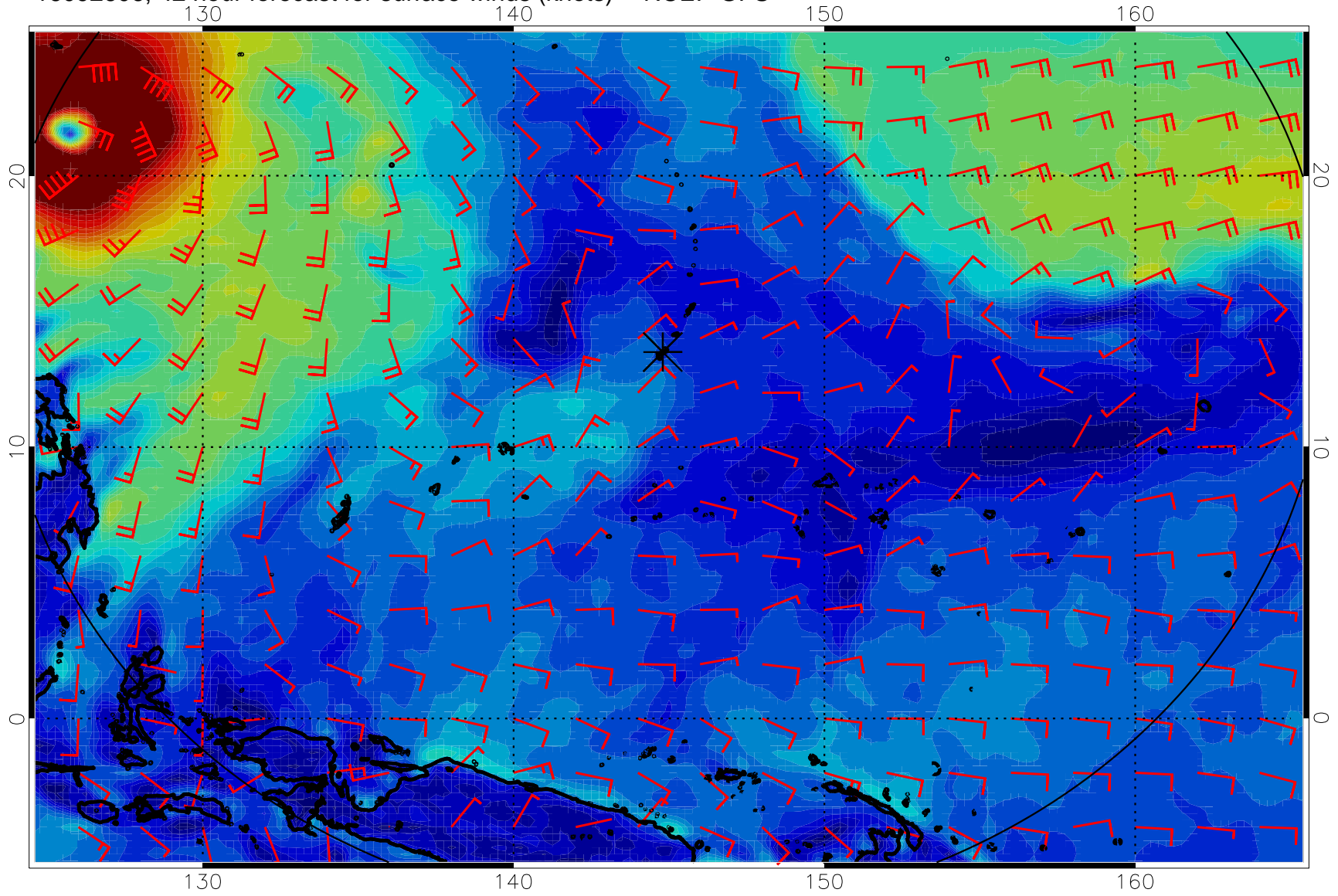
16092606, 42 hour forecast for surface winds (knots) -- NCEP GFS
