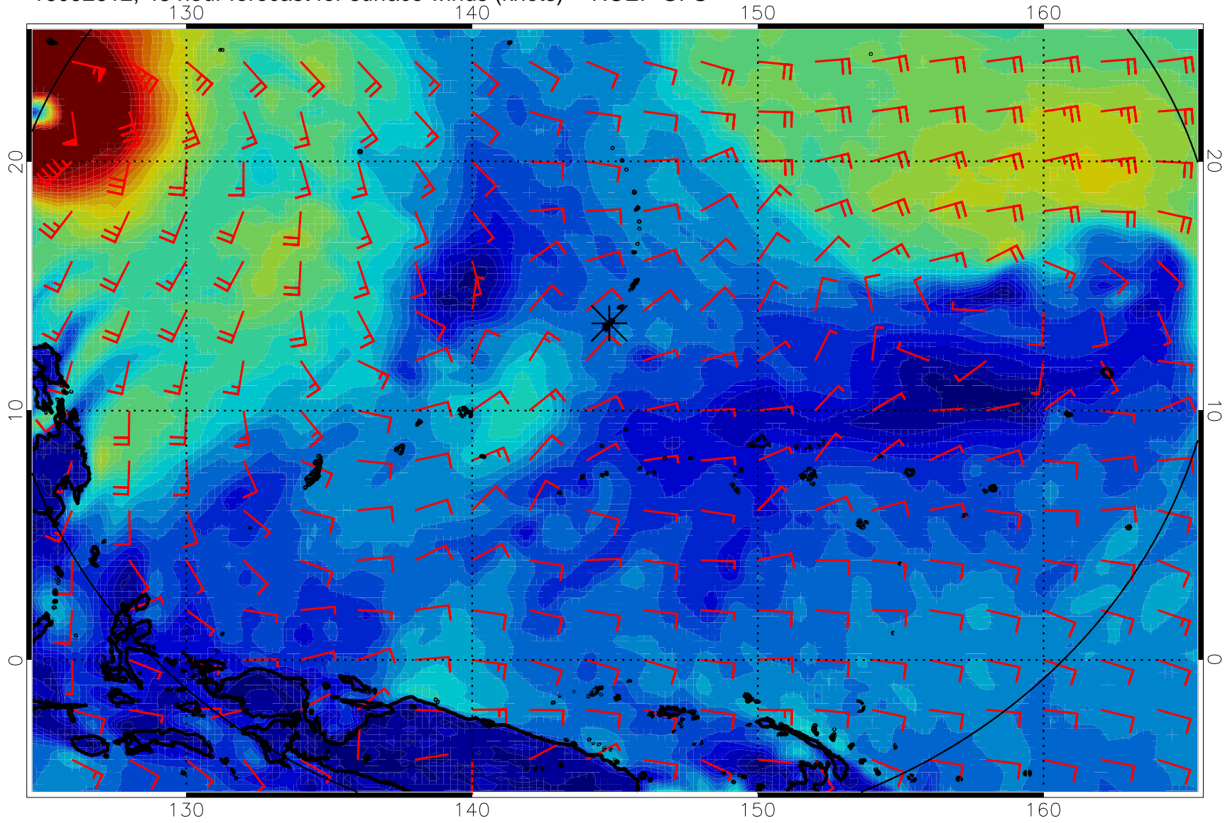
16092612, 48 hour forecast for surface winds (knots) -- NCEP GFS
