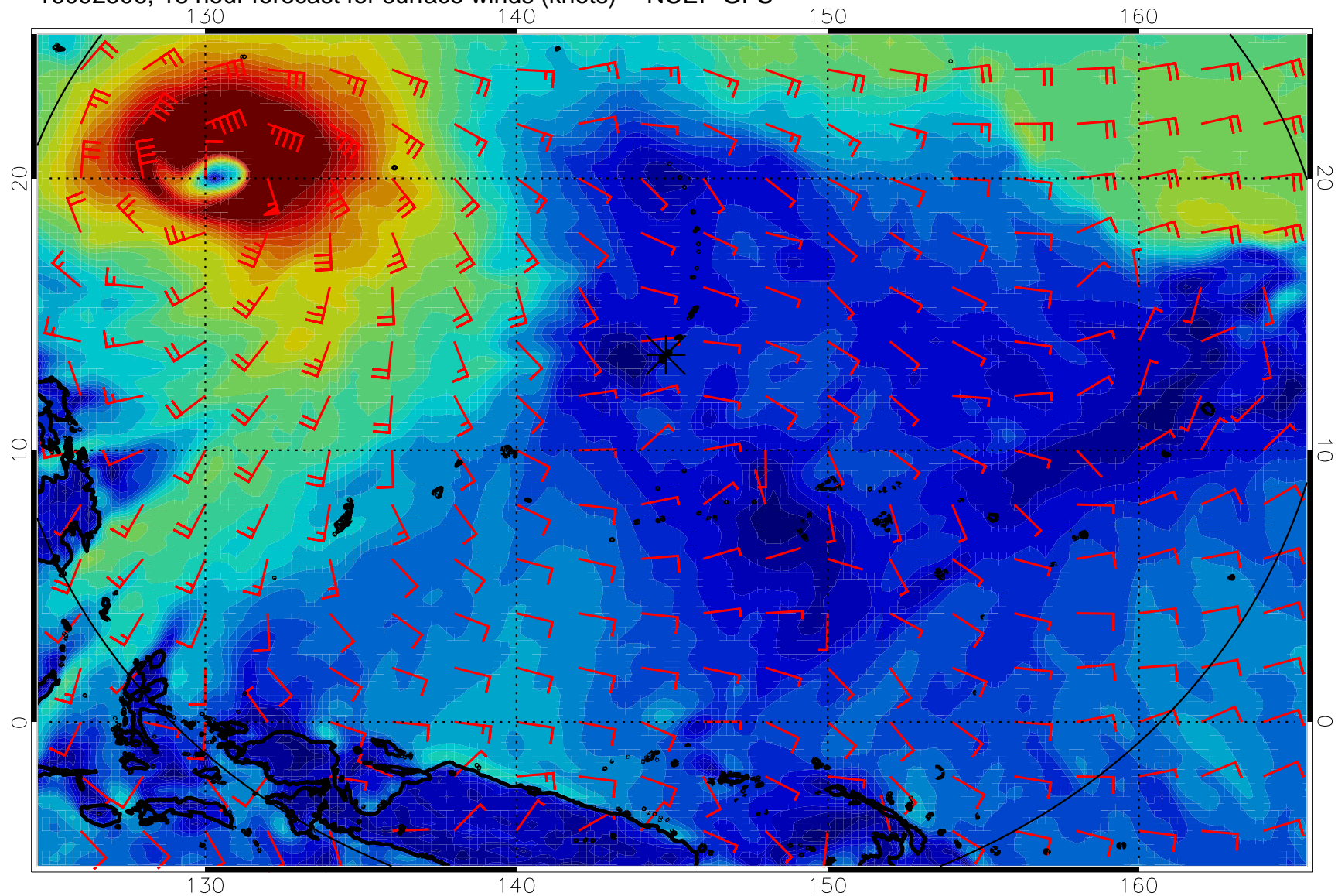
16092506, 18 hour forecast for surface winds (knots) -- NCEP GFS
