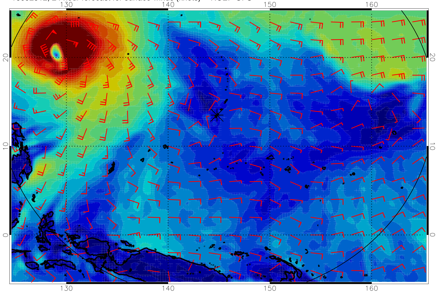
16092512, 24 hour forecast for surface winds (knots) -- NCEP GFS
