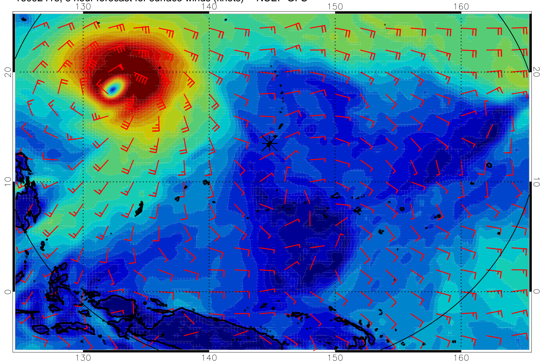
16092418, 6 hour forecast for surface winds (knots) -- NCEP GFS
