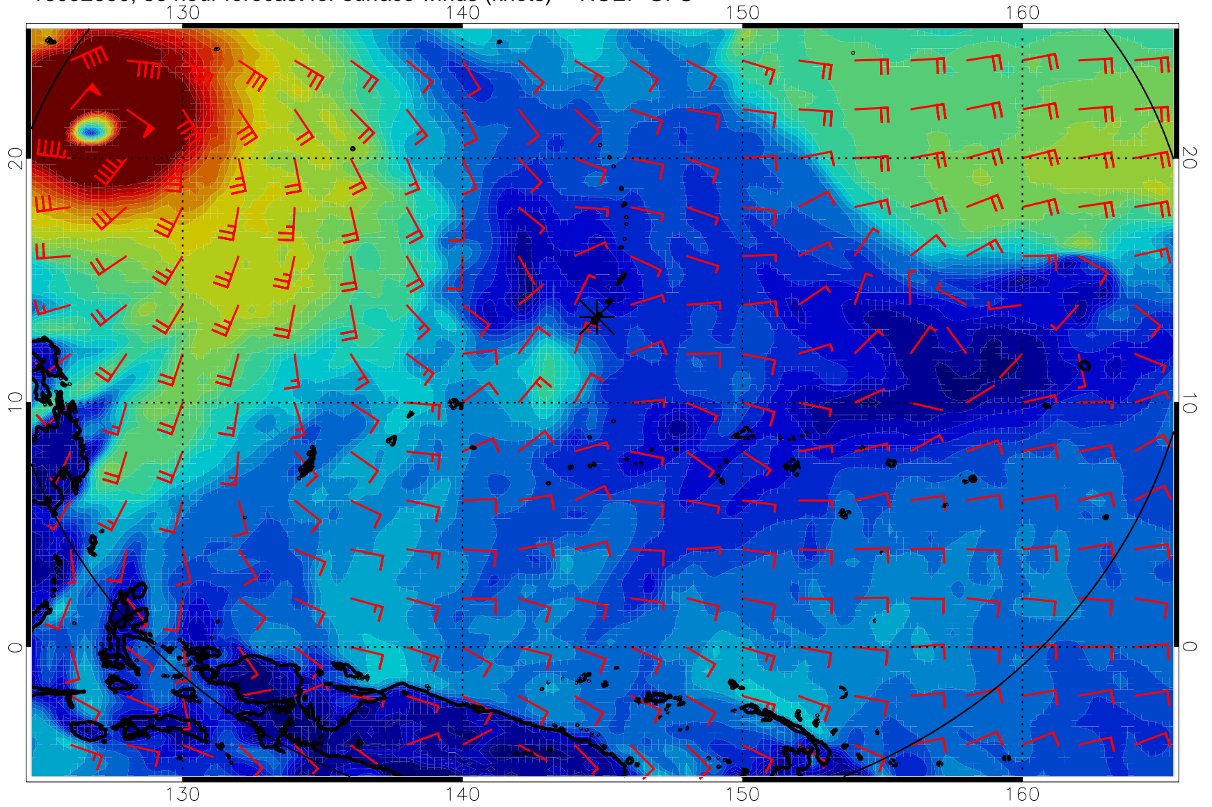
16092600, 36 hour forecast for surface winds (knots) -- NCEP GFS
