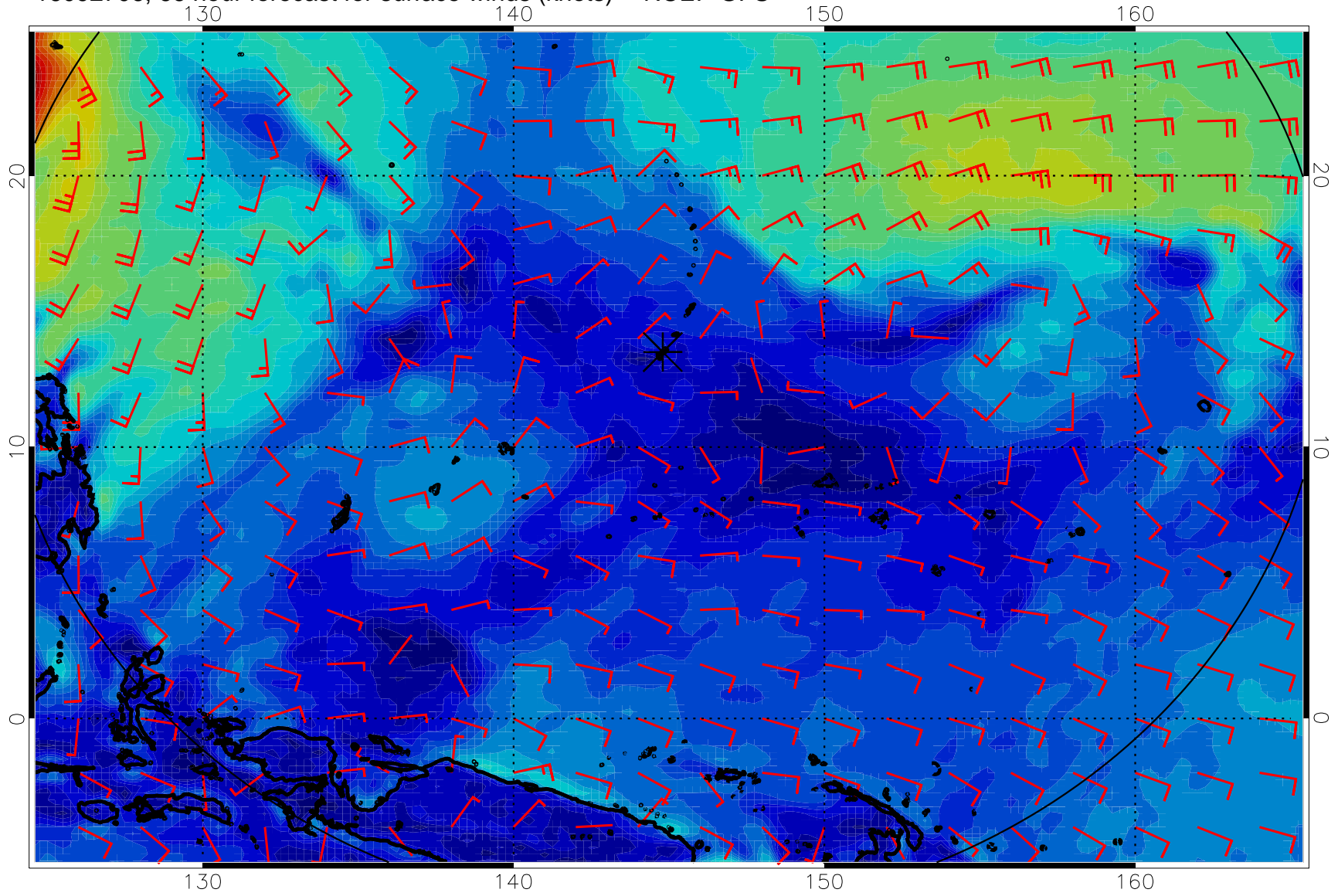
16092706, 66 hour forecast for surface winds (knots) -- NCEP GFS
