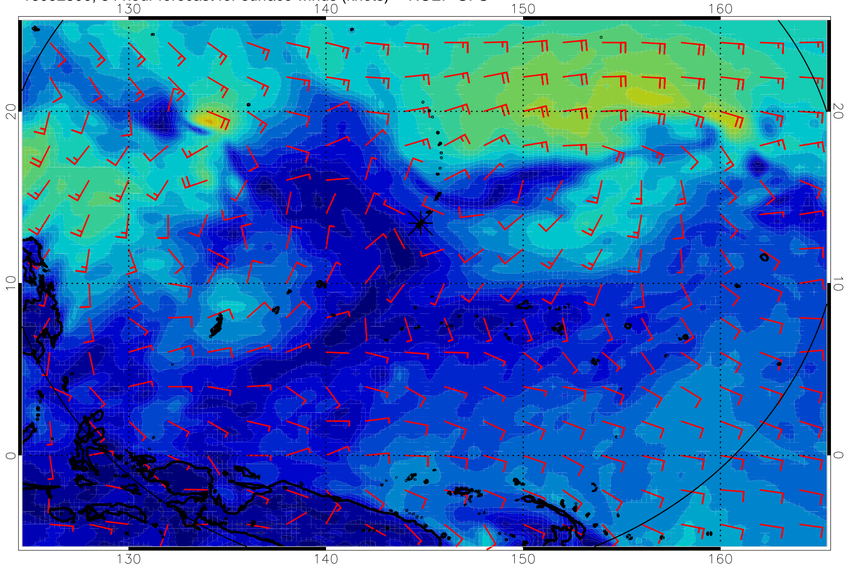
16092800, 84 hour forecast for surface winds (knots) -- NCEP GFS
