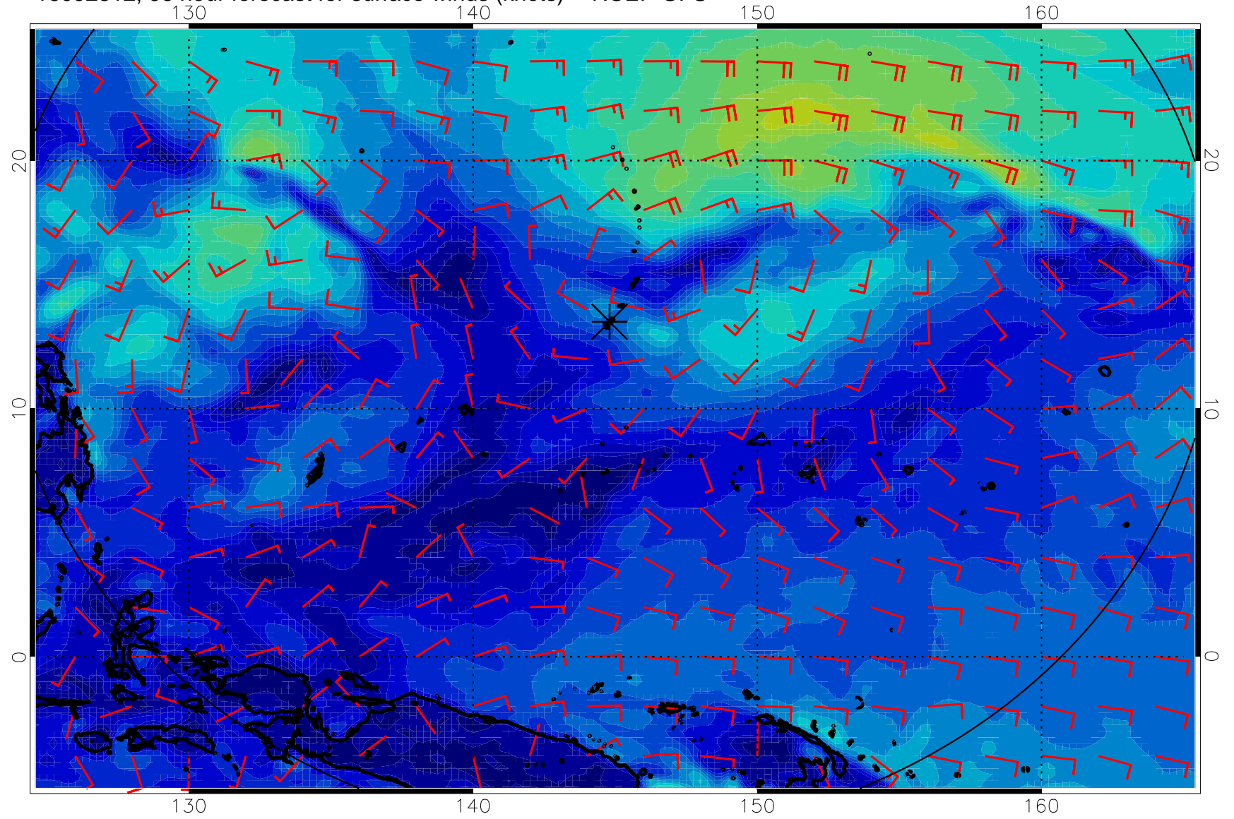
16092812, 96 hour forecast for surface winds (knots) -- NCEP GFS
