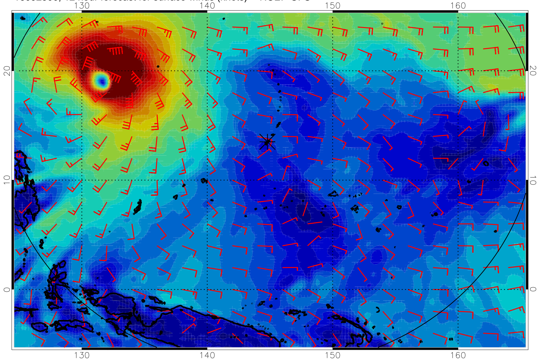
16092500, 12 hour forecast for surface winds (knots) -- NCEP GFS
