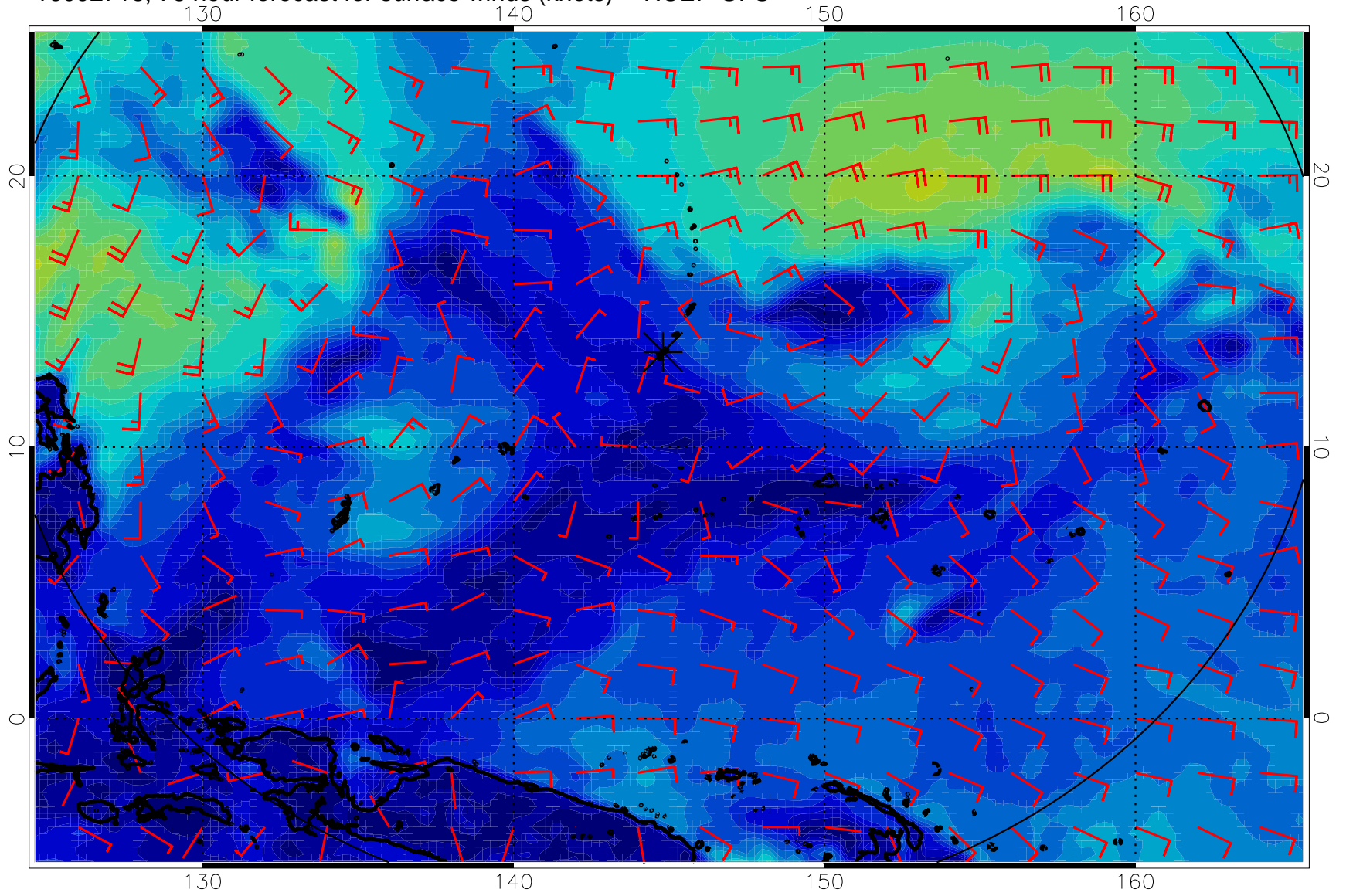
16092718, 78 hour forecast for surface winds (knots) -- NCEP GFS
