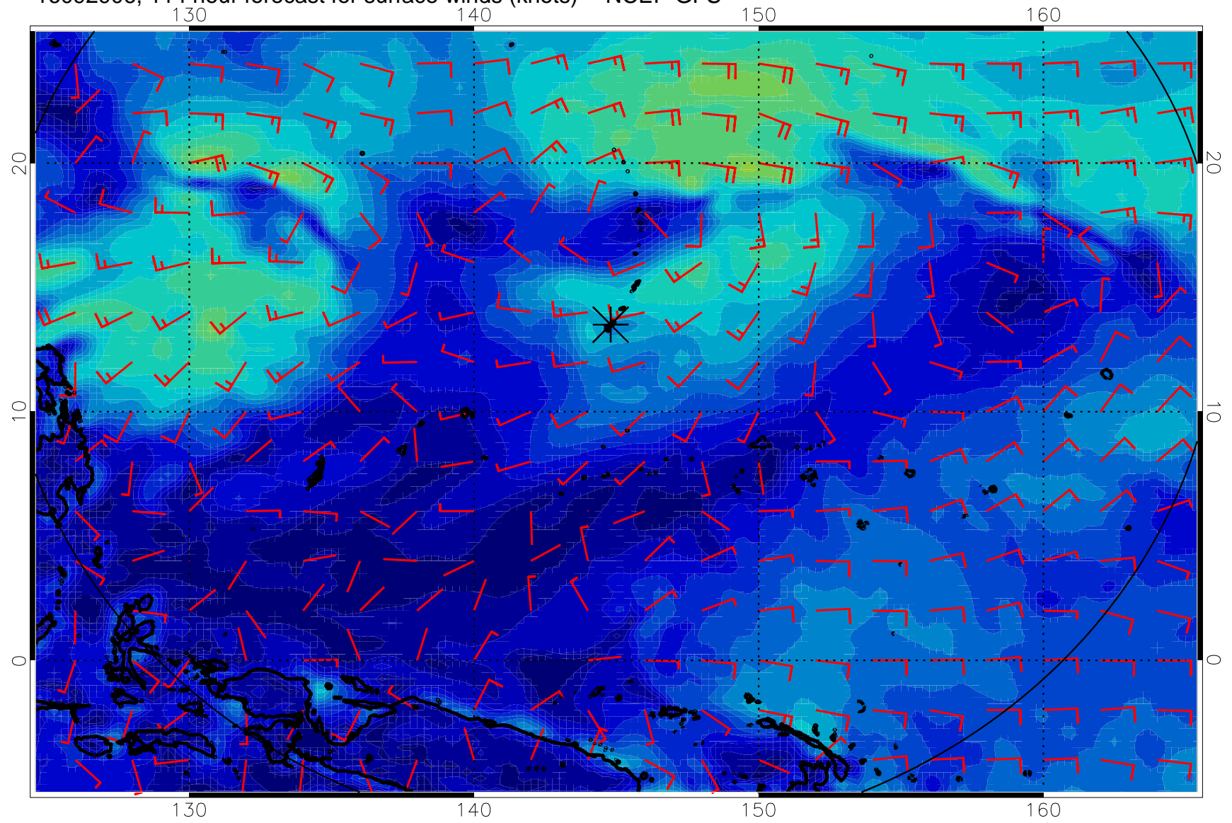
16092906, 114 hour forecast for surface winds (knots) -- NCEP GFS
