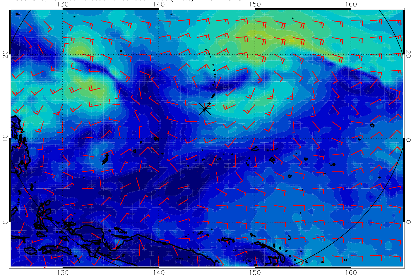
16092818, 102 hour forecast for surface winds (knots) -- NCEP GFS
