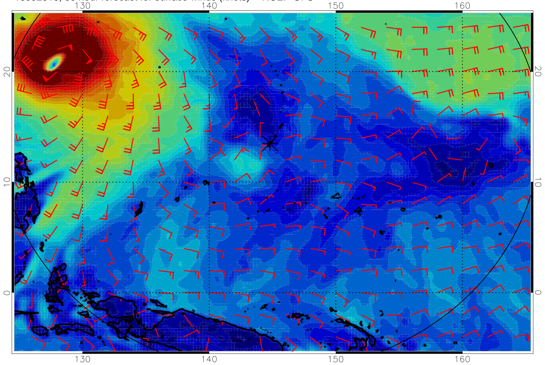
16092518, 30 hour forecast for surface winds (knots) -- NCEP GFS
