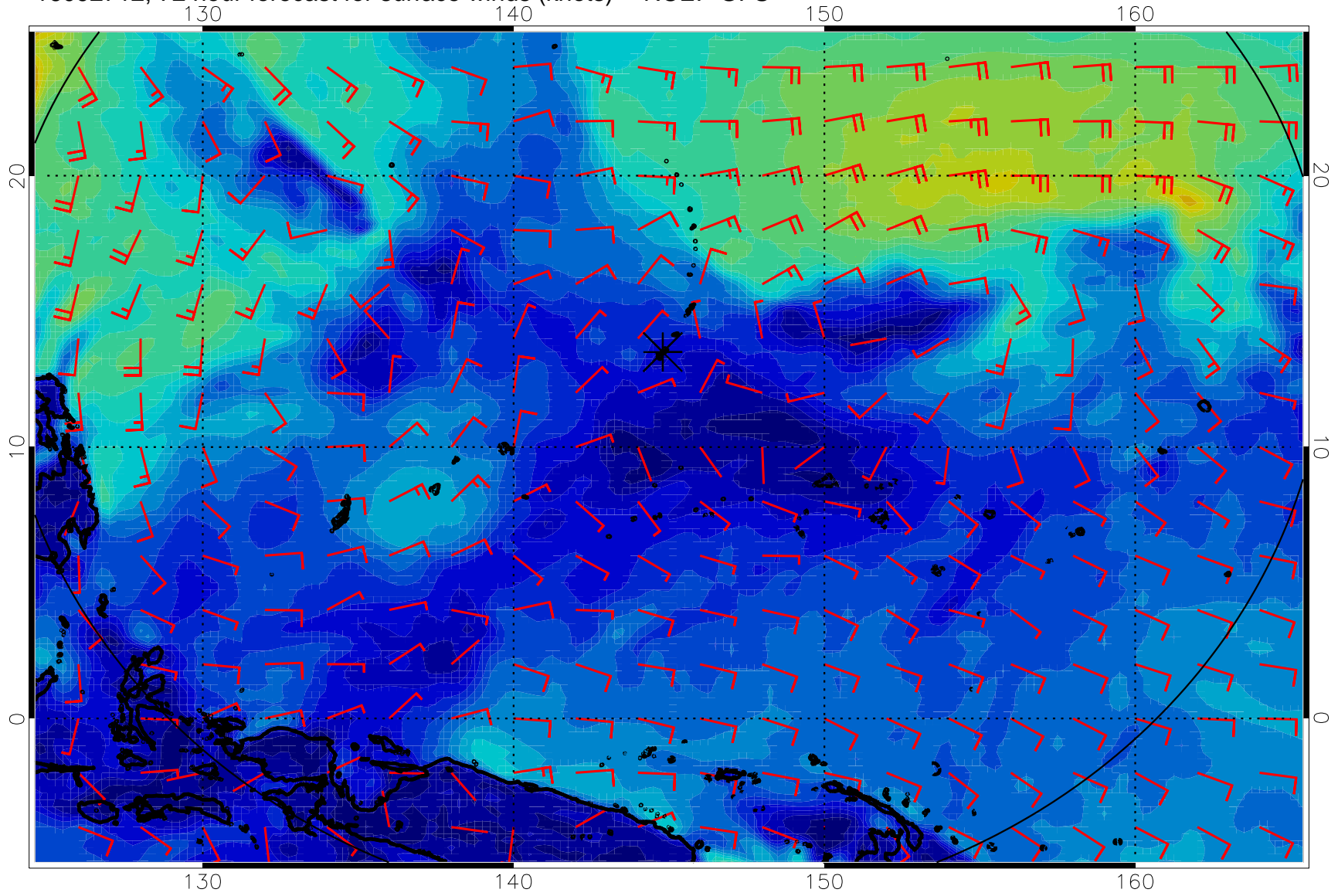
16092712, 72 hour forecast for surface winds (knots) -- NCEP GFS
