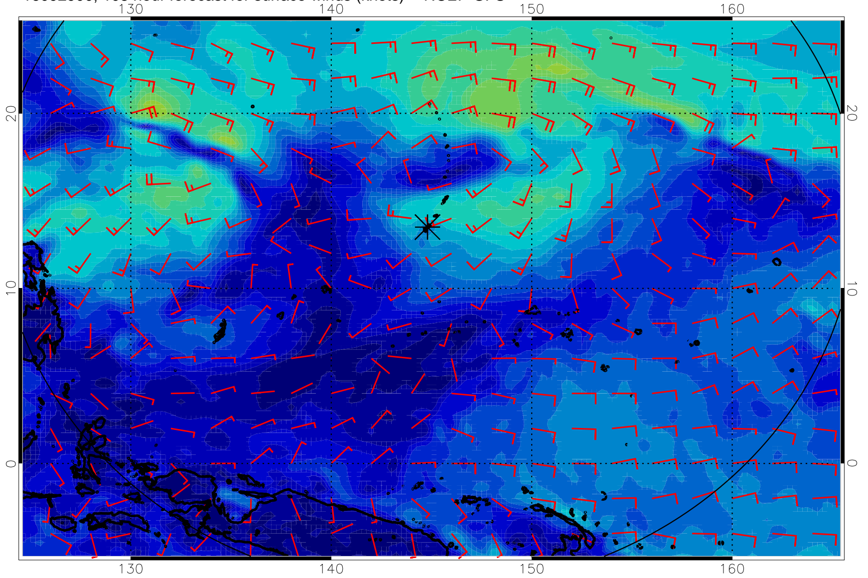
16092900, 108 hour forecast for surface winds (knots) -- NCEP GFS
