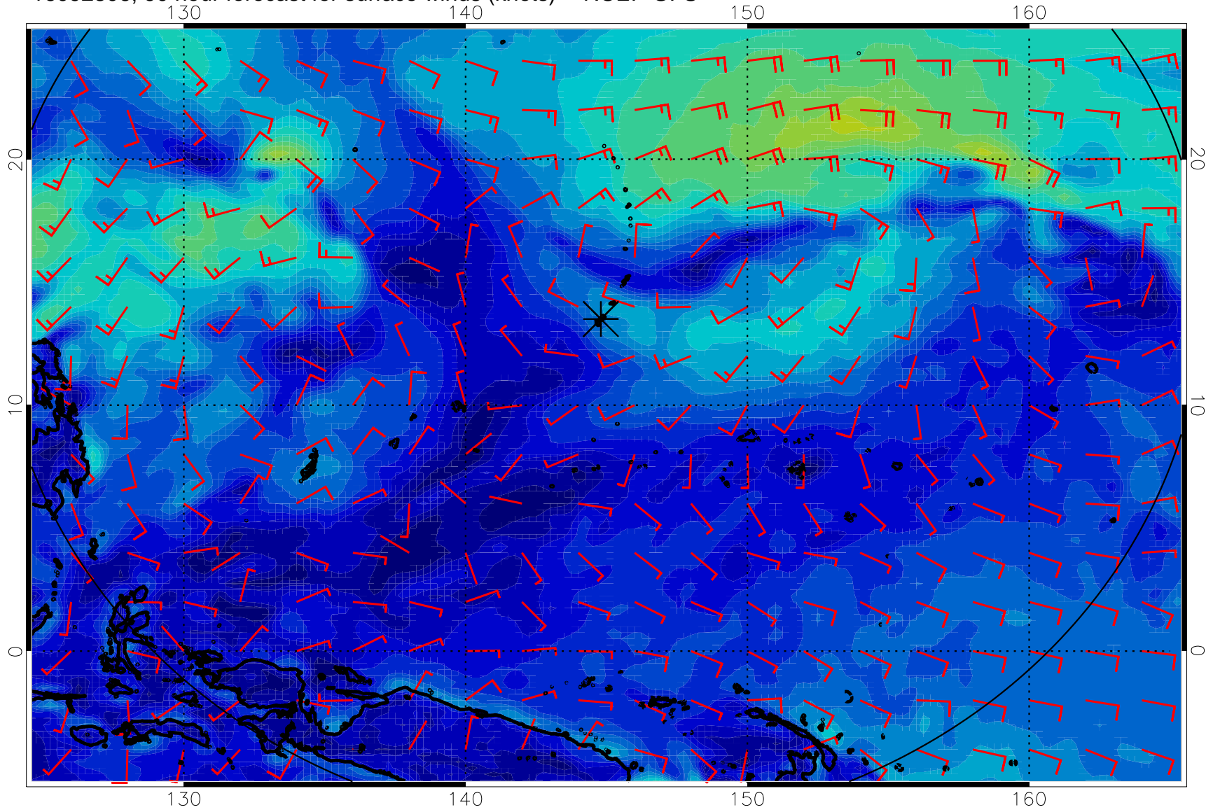
16092806, 90 hour forecast for surface winds (knots) -- NCEP GFS
