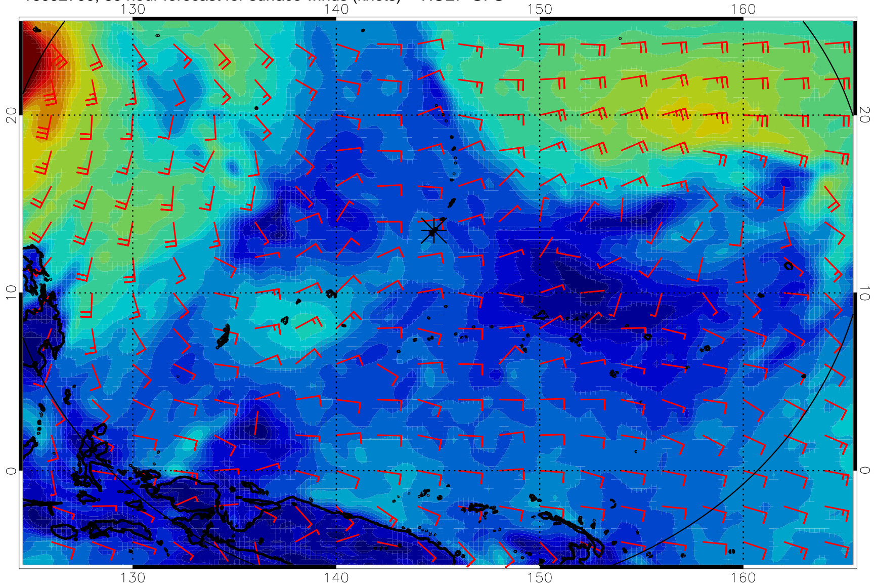
16092700, 60 hour forecast for surface winds (knots) -- NCEP GFS
