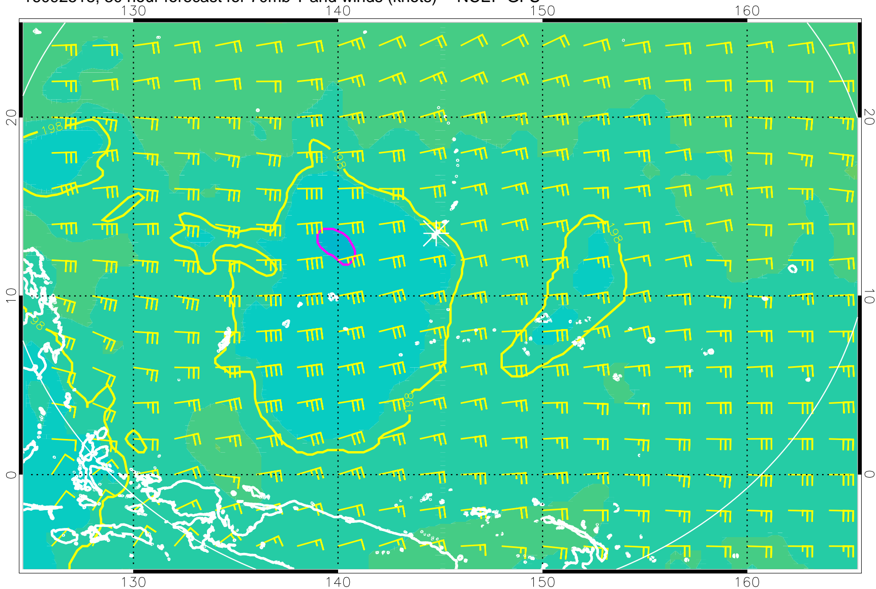
16092518, 30 hour forecast for 70mb T and winds (knots) -- NCEP GFS
