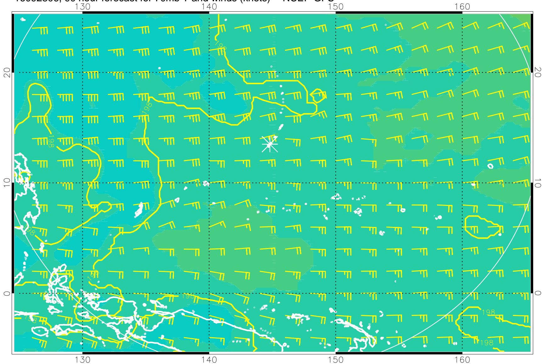
16092806, 90 hour forecast for 70mb T and winds (knots) -- NCEP GFS
