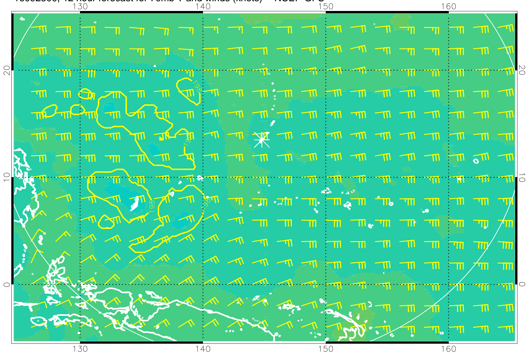
16092500, 12 hour forecast for 70mb T and winds (knots) -- NCEP GFS
