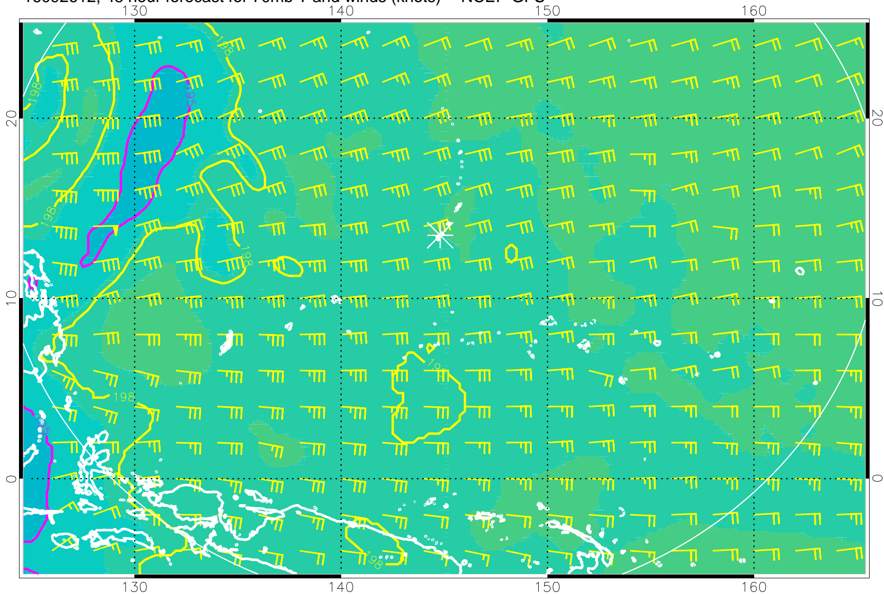
16092612, 48 hour forecast for 70mb T and winds (knots) -- NCEP GFS
