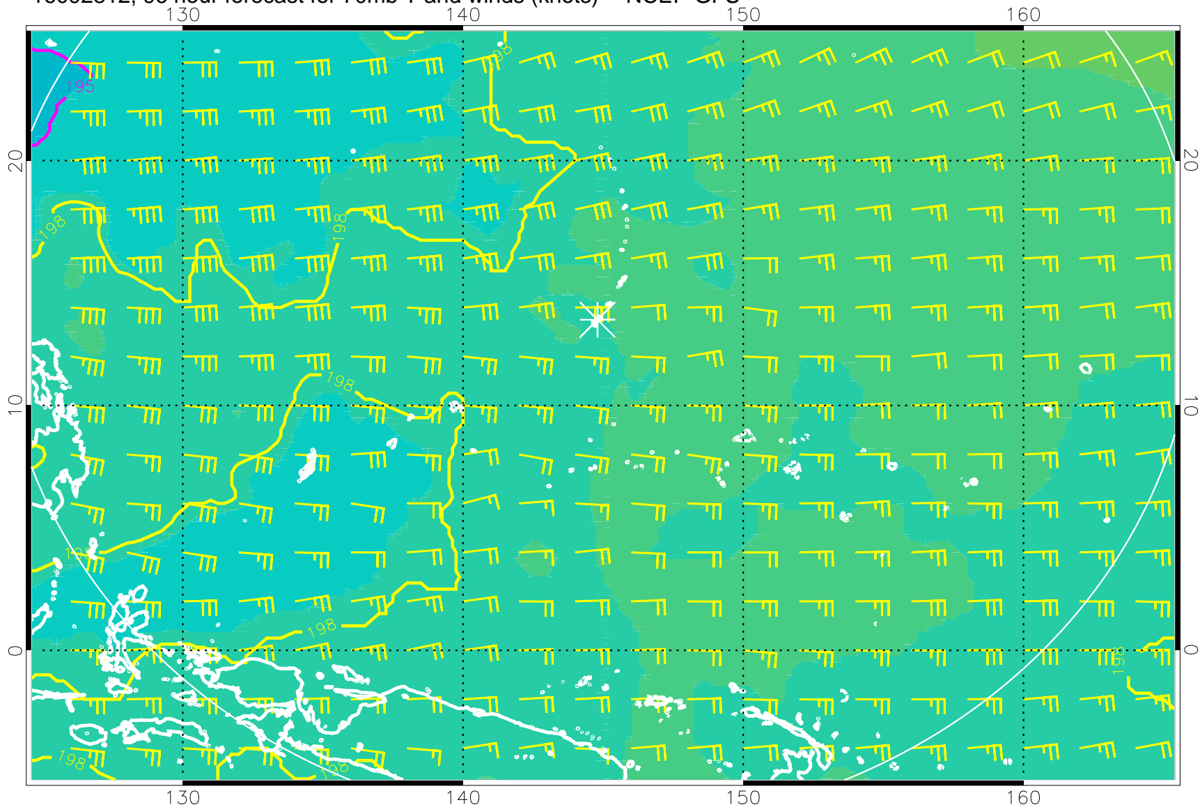
16092812, 96 hour forecast for 70mb T and winds (knots) -- NCEP GFS
