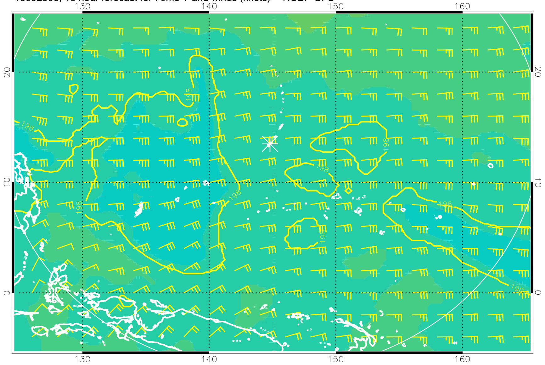
16092506, 18 hour forecast for 70mb T and winds (knots) -- NCEP GFS
