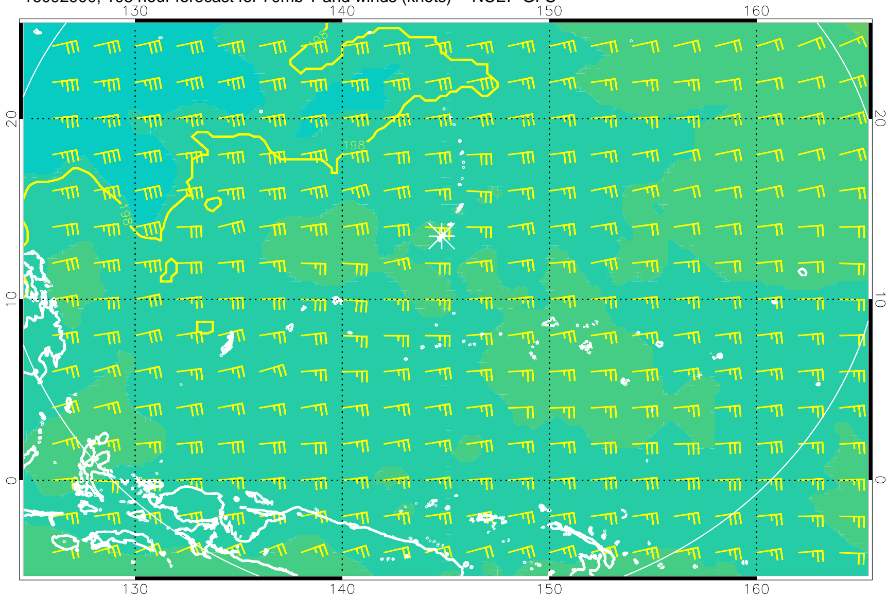
16092900, 108 hour forecast for 70mb T and winds (knots) -- NCEP GFS
