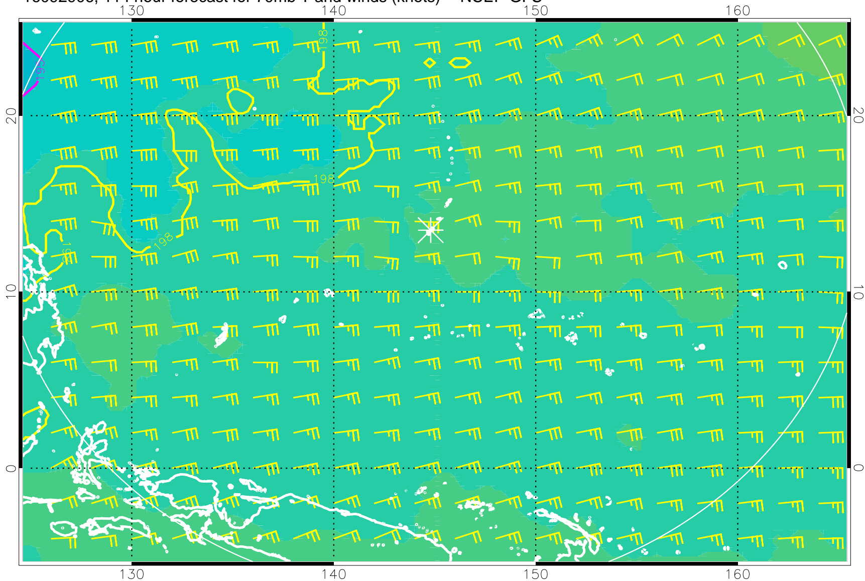
16092906, 114 hour forecast for 70mb T and winds (knots) -- NCEP GFS
