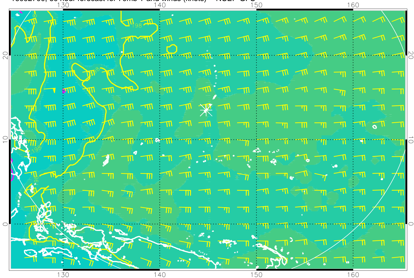
16092700, 60 hour forecast for 70mb T and winds (knots) -- NCEP GFS
