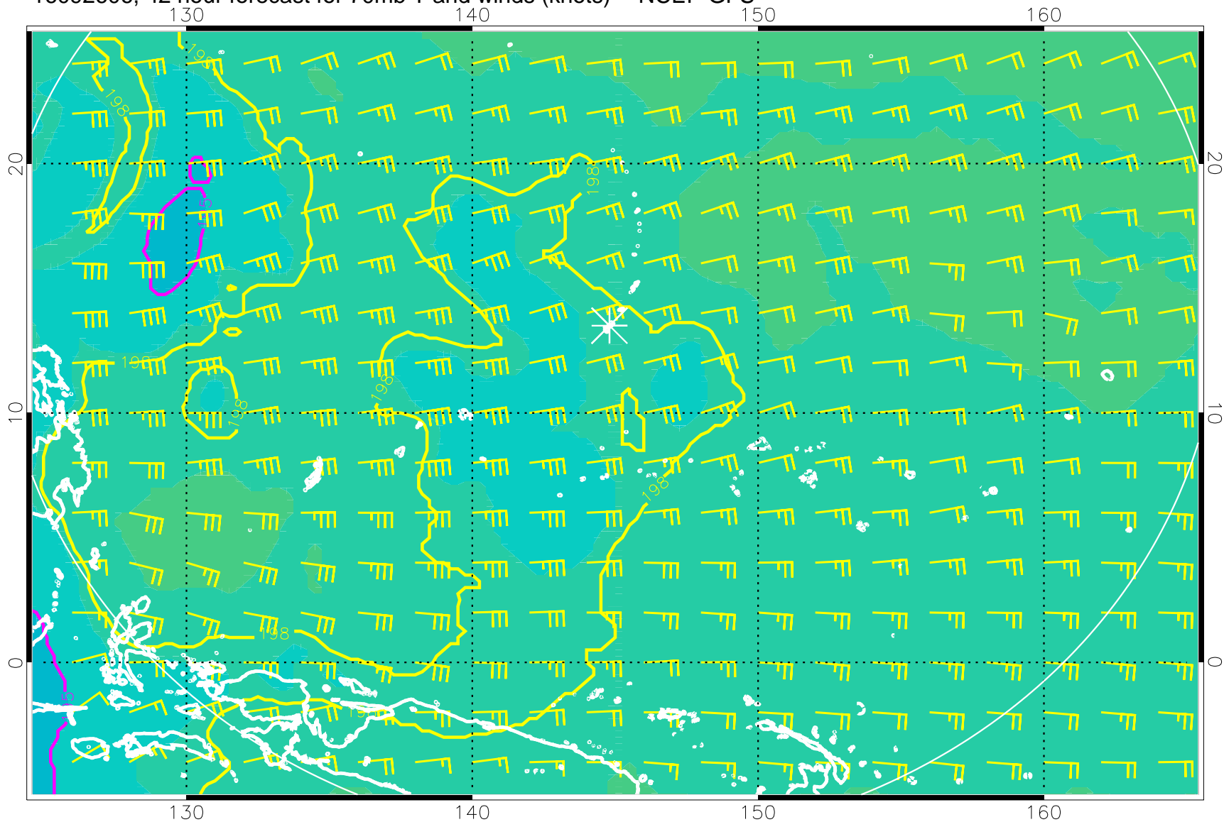
16092606, 42 hour forecast for 70mb T and winds (knots) -- NCEP GFS
