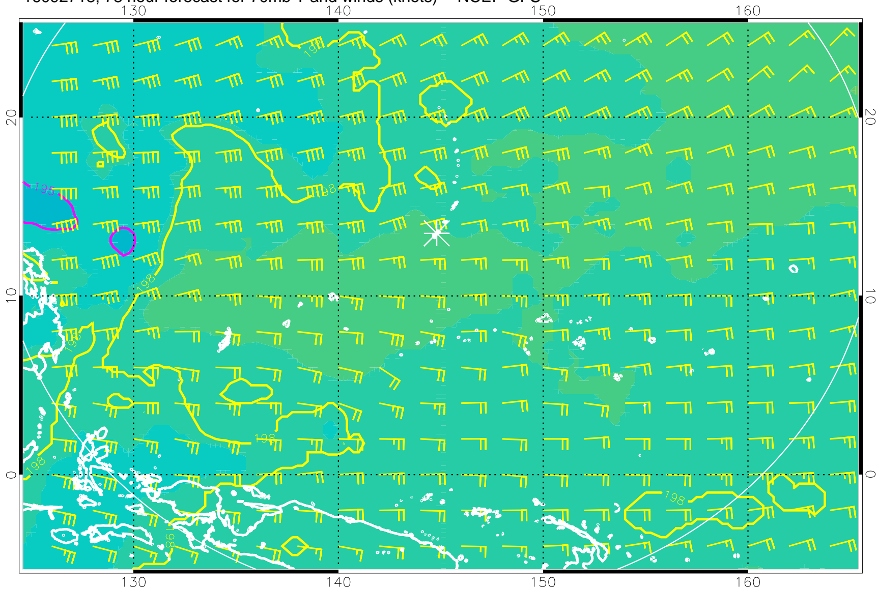
16092718, 78 hour forecast for 70mb T and winds (knots) -- NCEP GFS
