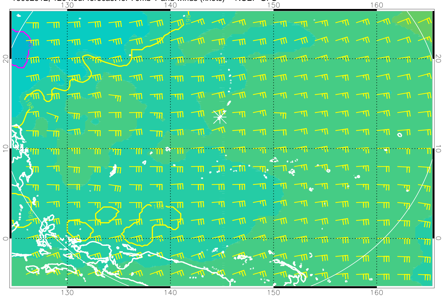
16092912, 120 hour forecast for 70mb T and winds (knots) -- NCEP GFS
