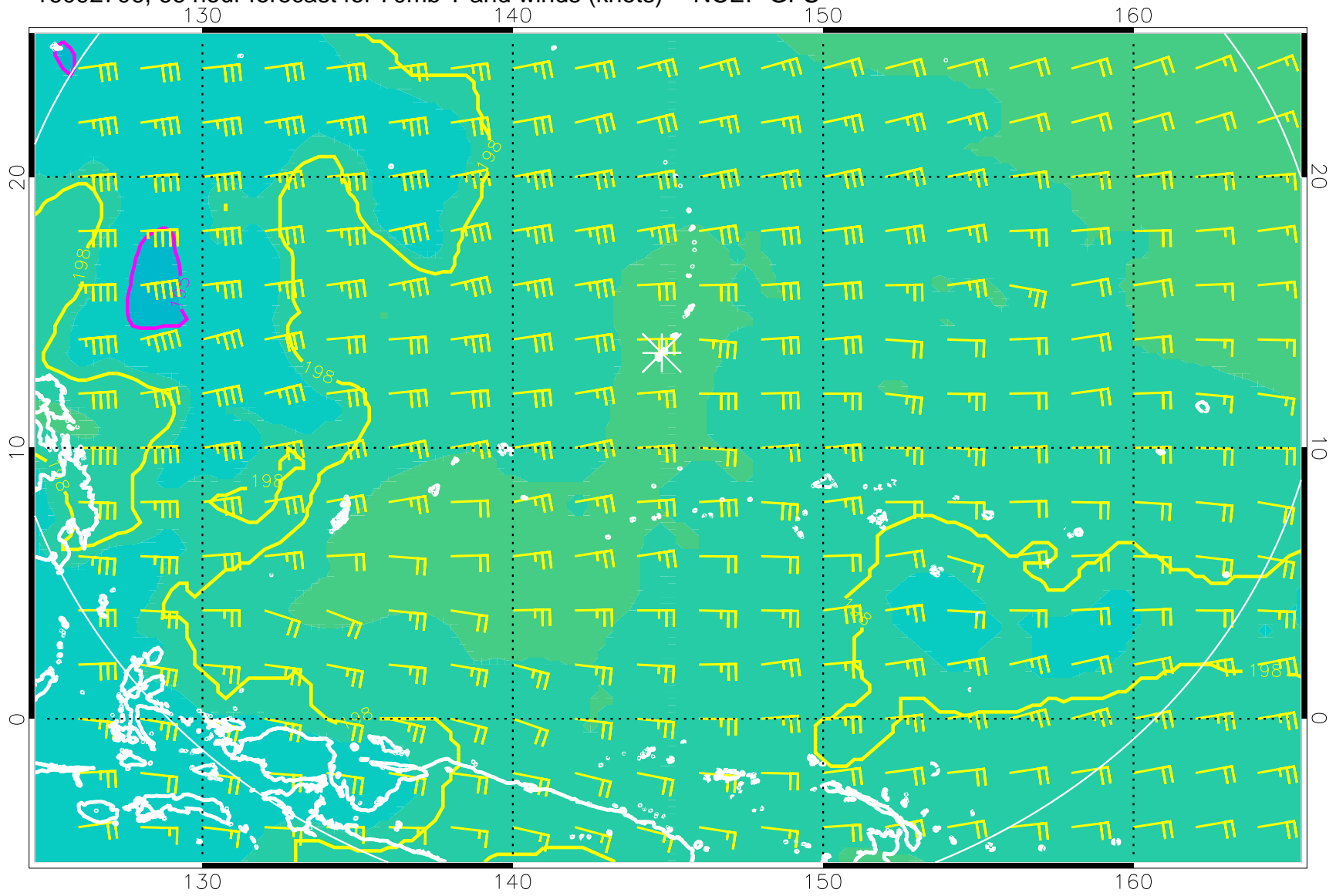
16092706, 66 hour forecast for 70mb T and winds (knots) -- NCEP GFS
