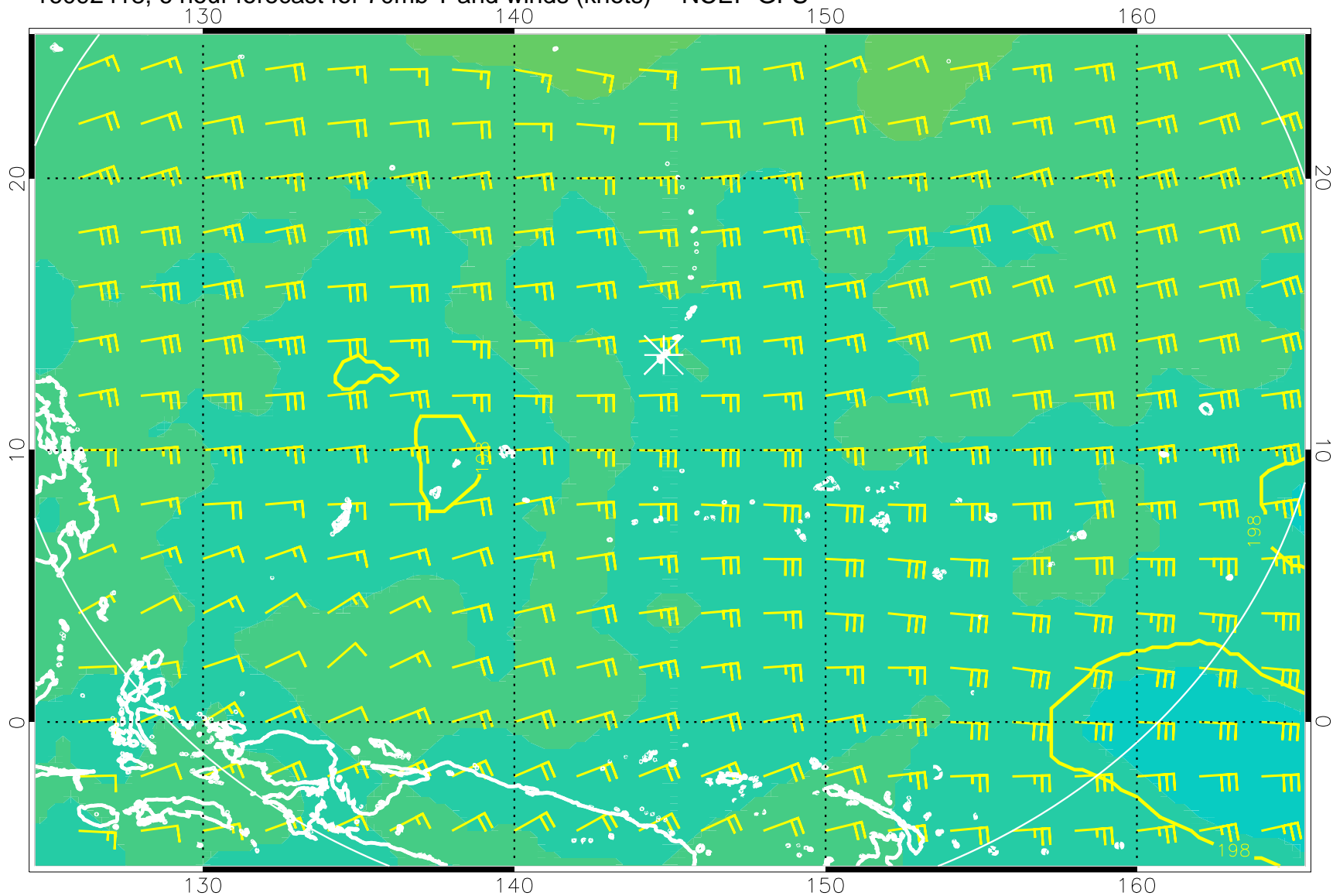
16092418, 6 hour forecast for 70mb T and winds (knots) -- NCEP GFS
