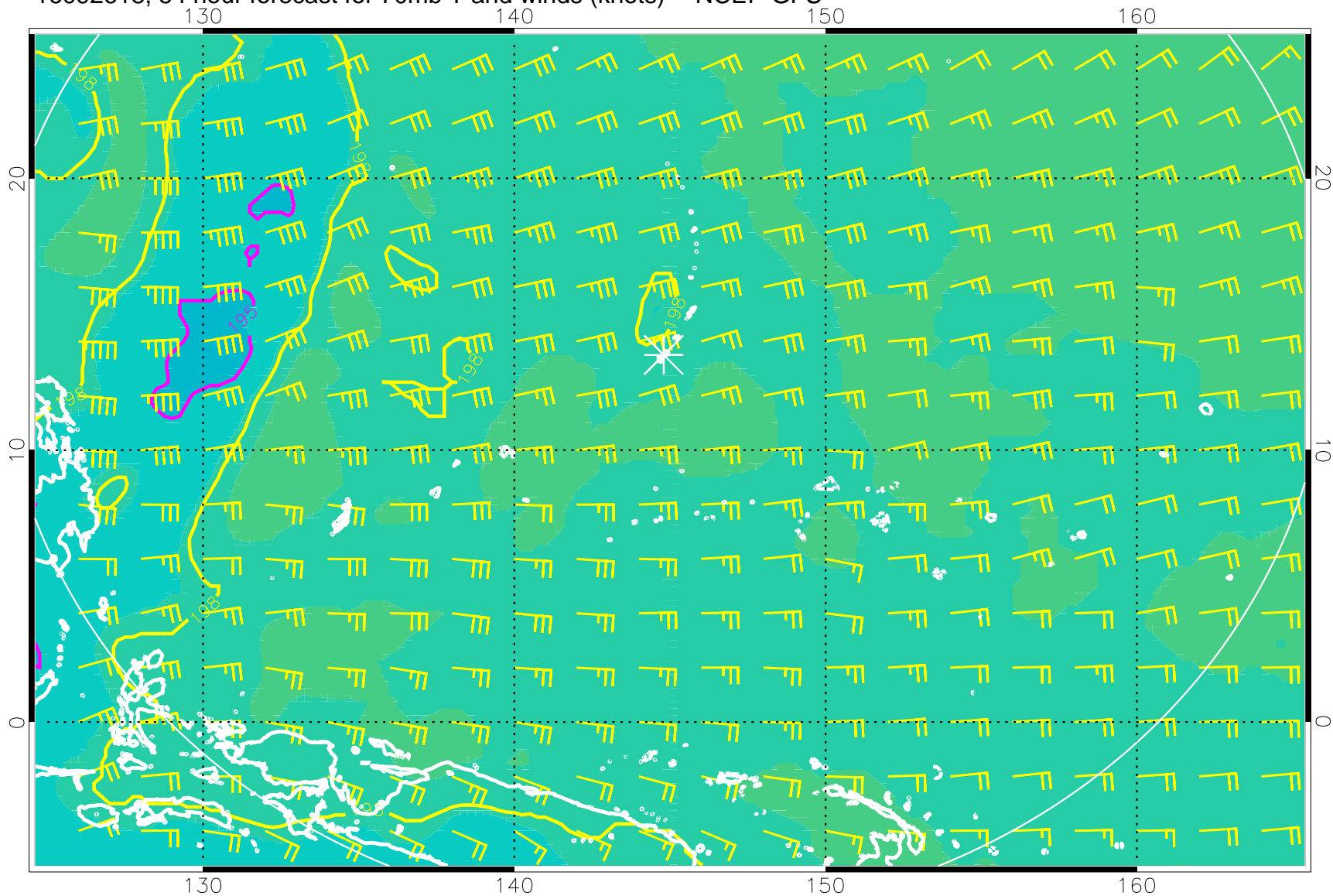
16092618, 54 hour forecast for 70mb T and winds (knots) -- NCEP GFS
