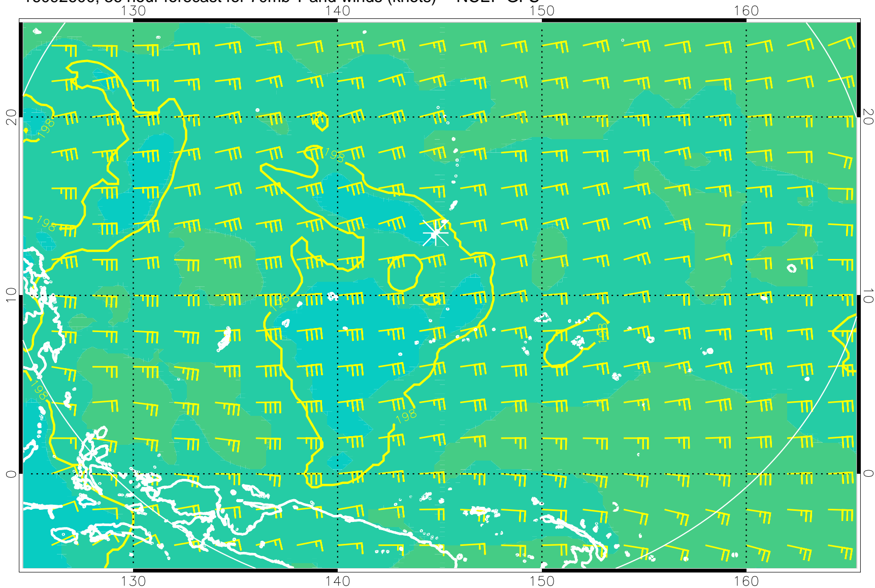
16092600, 36 hour forecast for 70mb T and winds (knots) -- NCEP GFS
