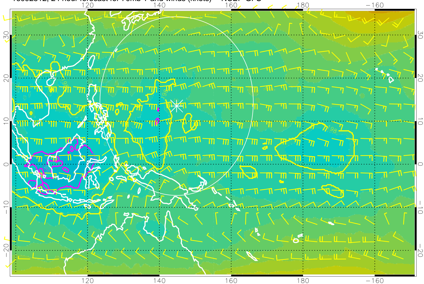
16092512, 24 hour forecast for 70mb T and winds (knots) -- NCEP GFS
