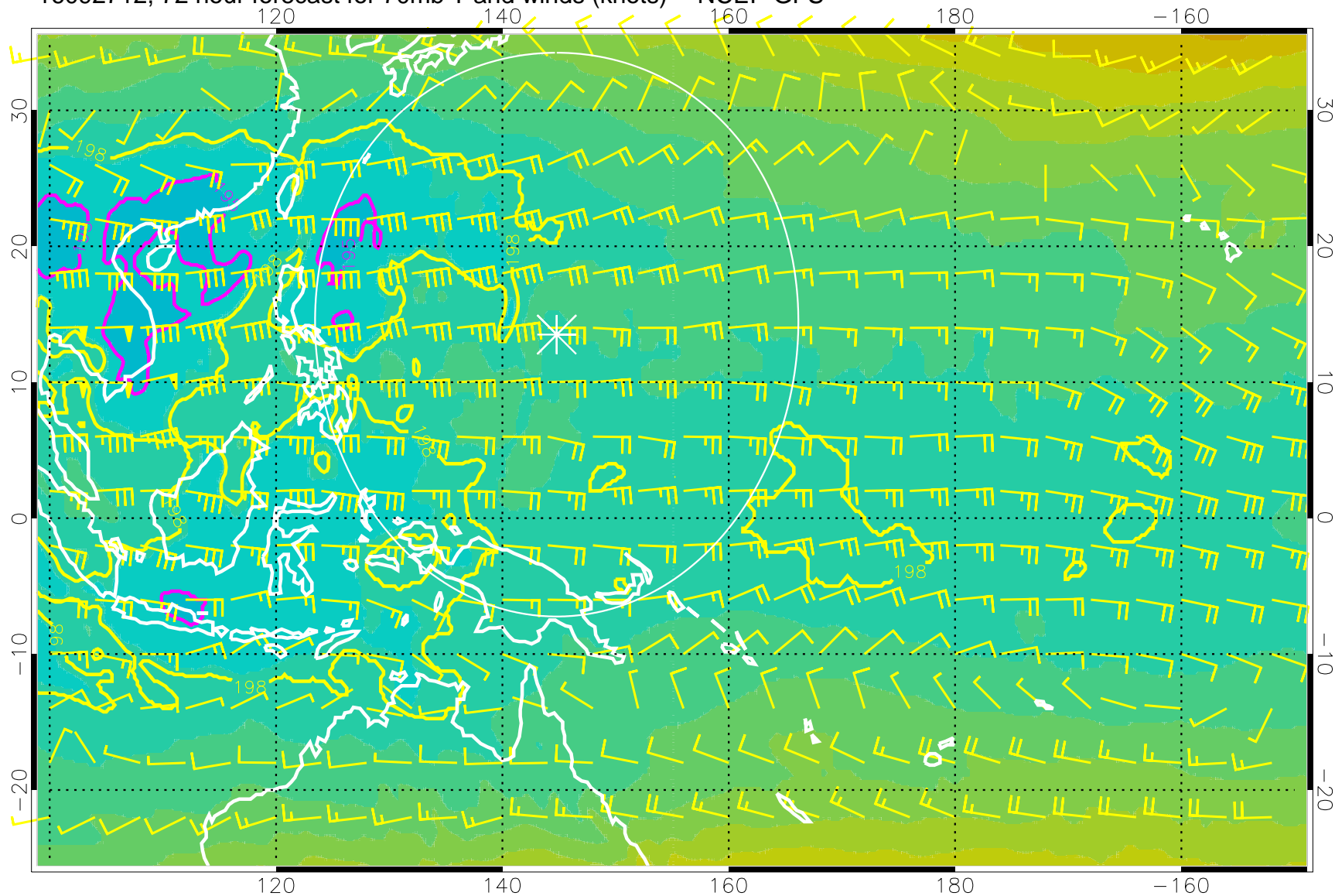
16092712, 72 hour forecast for 70mb T and winds (knots) -- NCEP GFS
