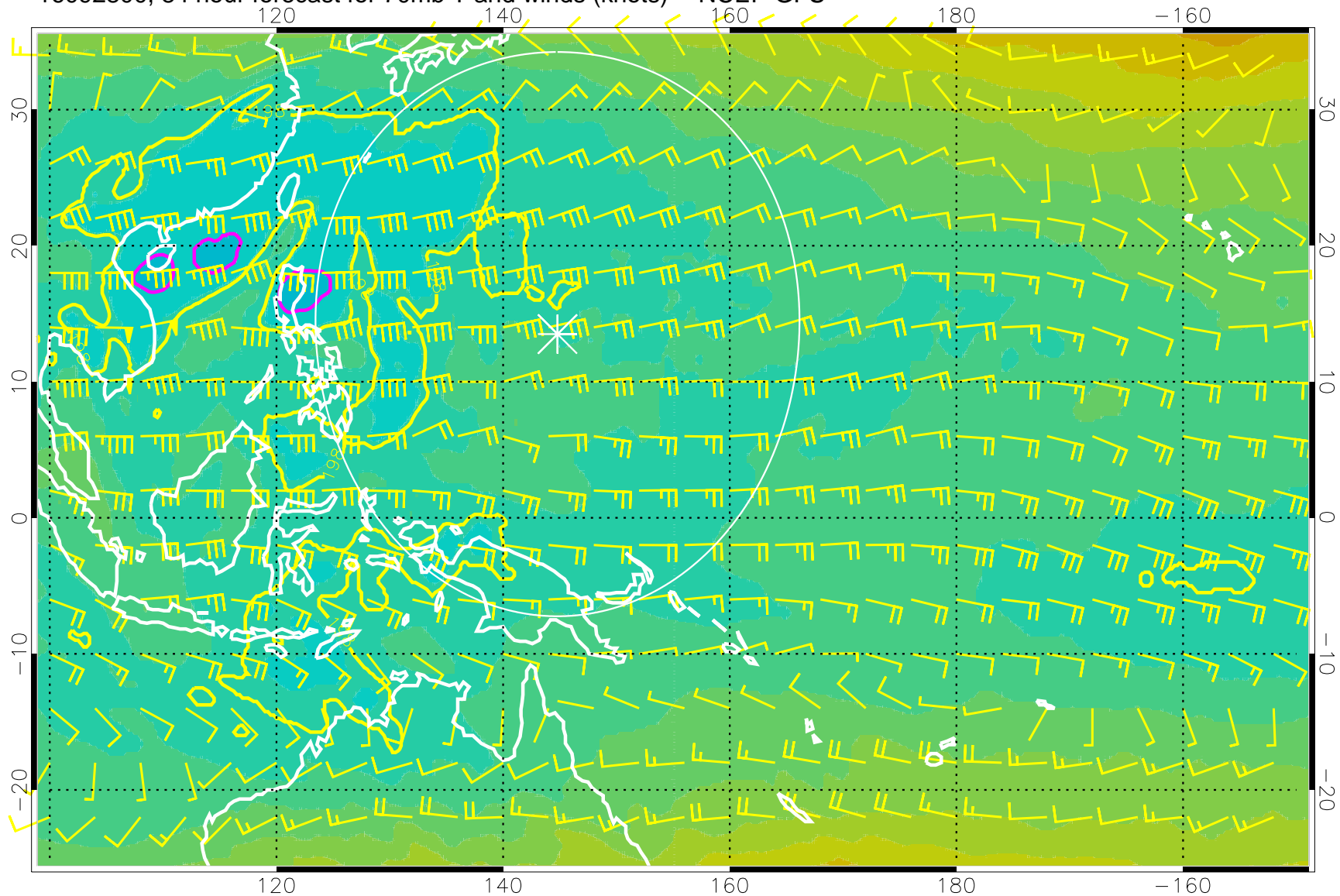
16092800, 84 hour forecast for 70mb T and winds (knots) -- NCEP GFS
