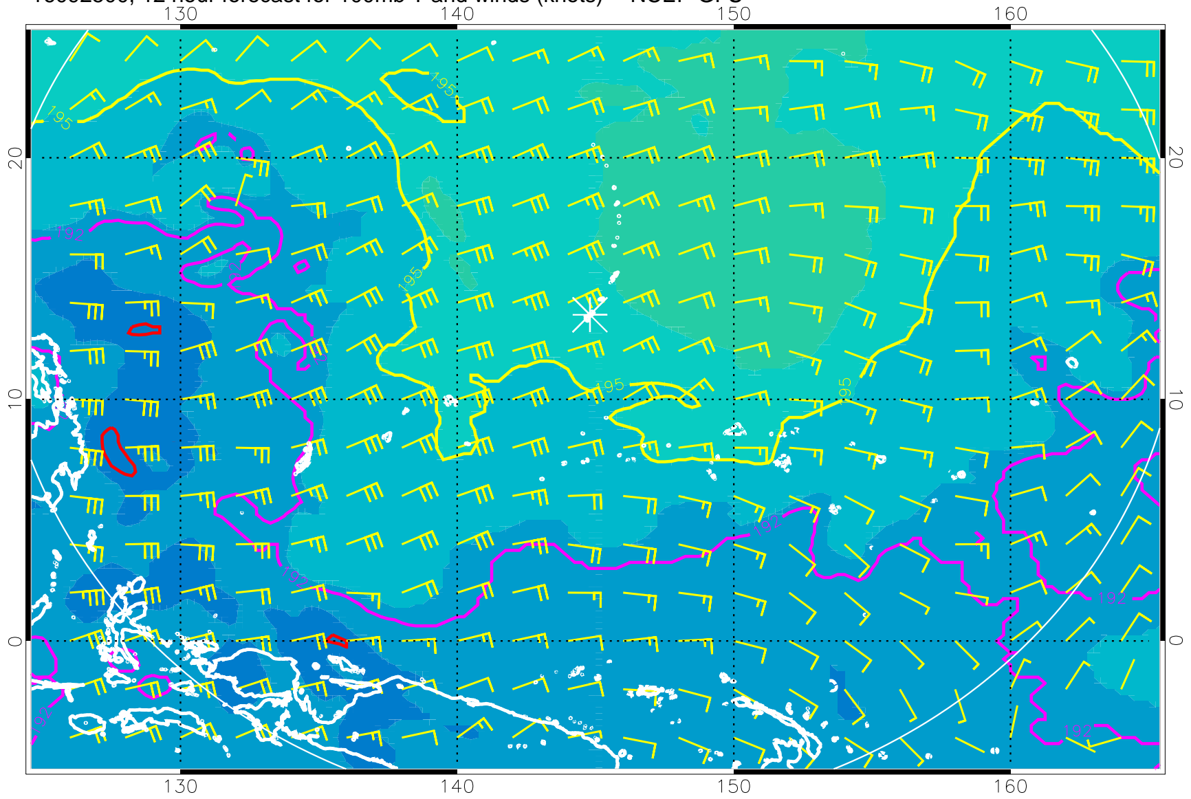
16092500, 12 hour forecast for 100mb T and winds (knots) -- NCEP GFS
