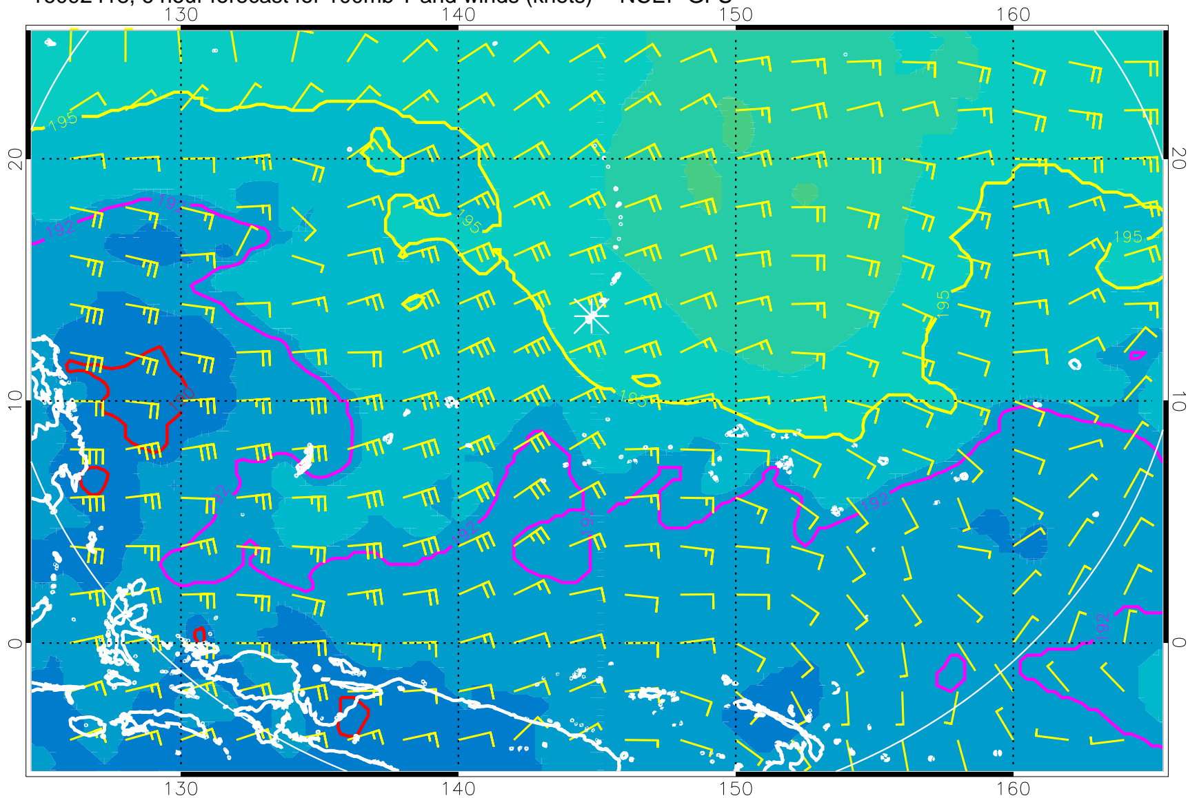
16092418, 6 hour forecast for 100mb T and winds (knots) -- NCEP GFS
