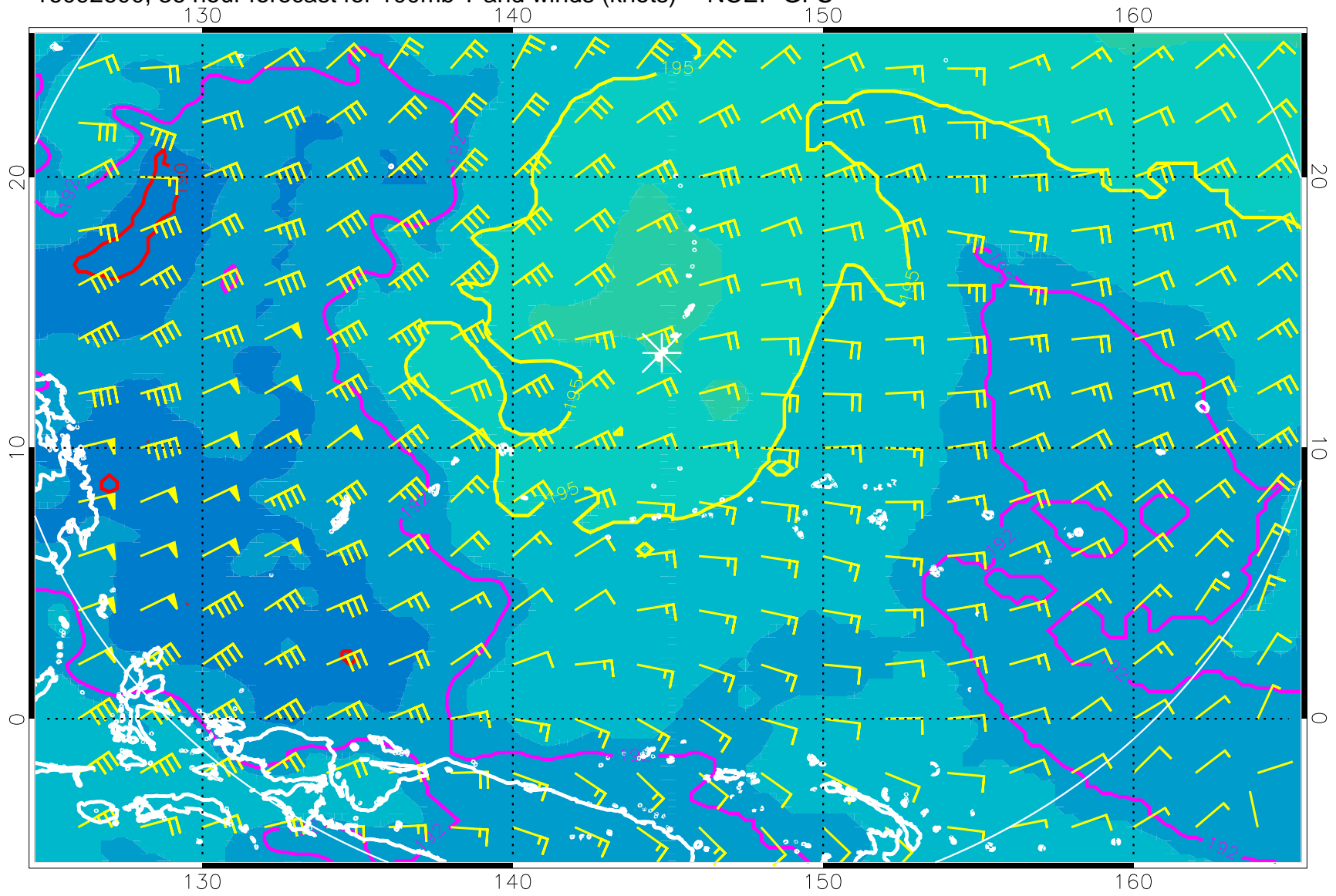
16092600, 36 hour forecast for 100mb T and winds (knots) -- NCEP GFS
