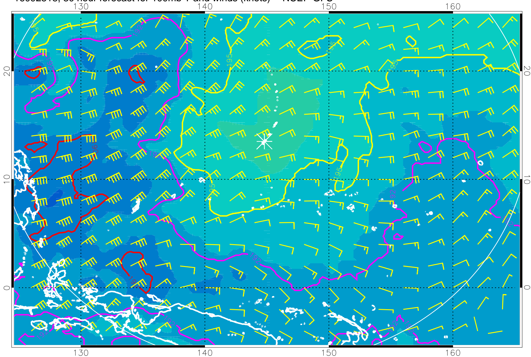
16092518, 30 hour forecast for 100mb T and winds (knots) -- NCEP GFS
