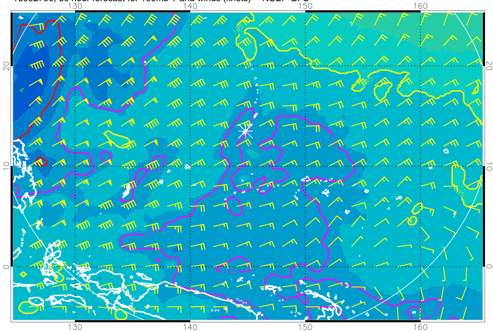
16092700, 60 hour forecast for 100mb T and winds (knots) -- NCEP GFS
