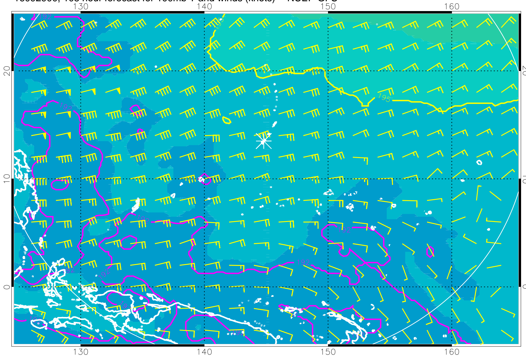
16092900, 108 hour forecast for 100mb T and winds (knots) -- NCEP GFS
