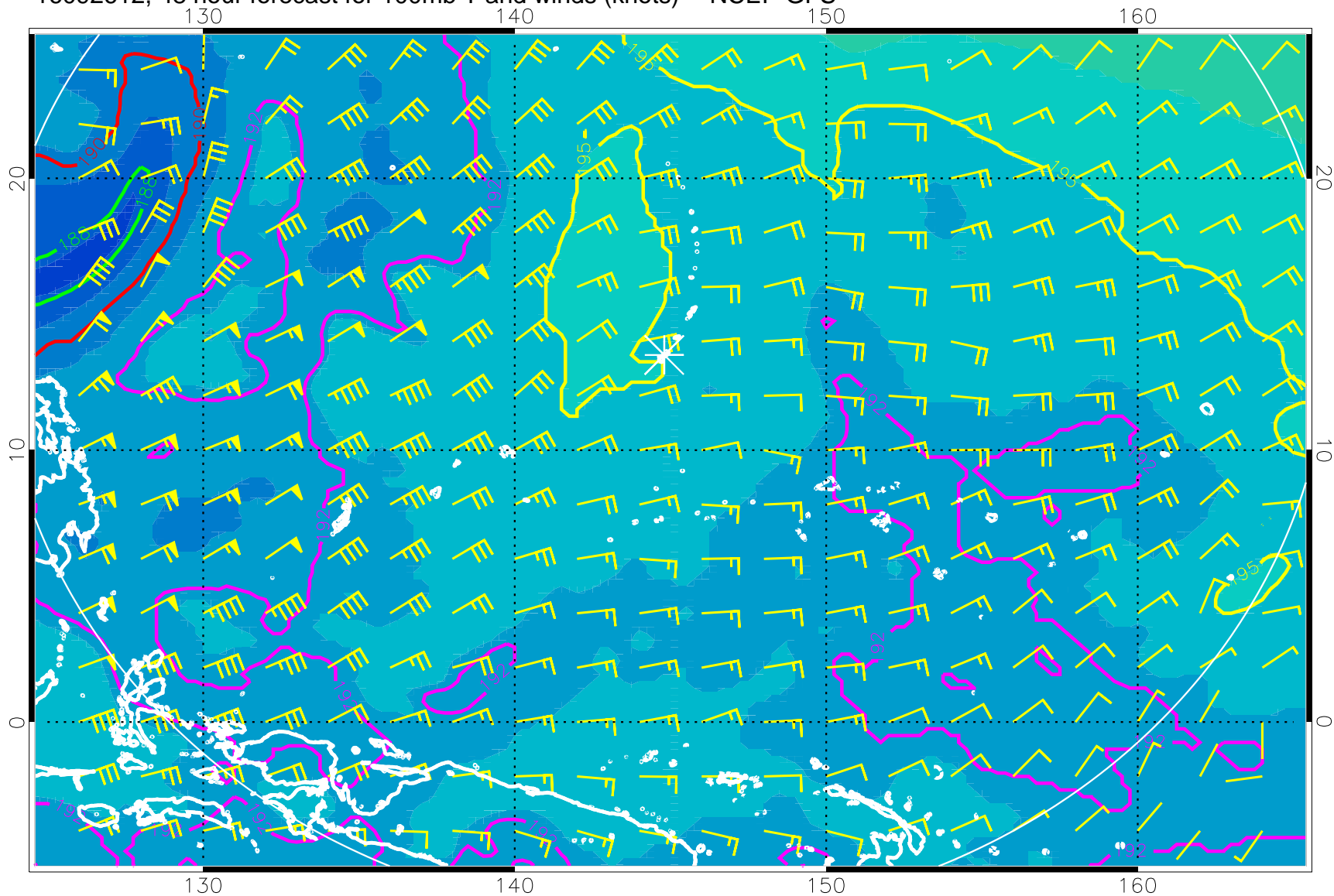
16092612, 48 hour forecast for 100mb T and winds (knots) -- NCEP GFS
