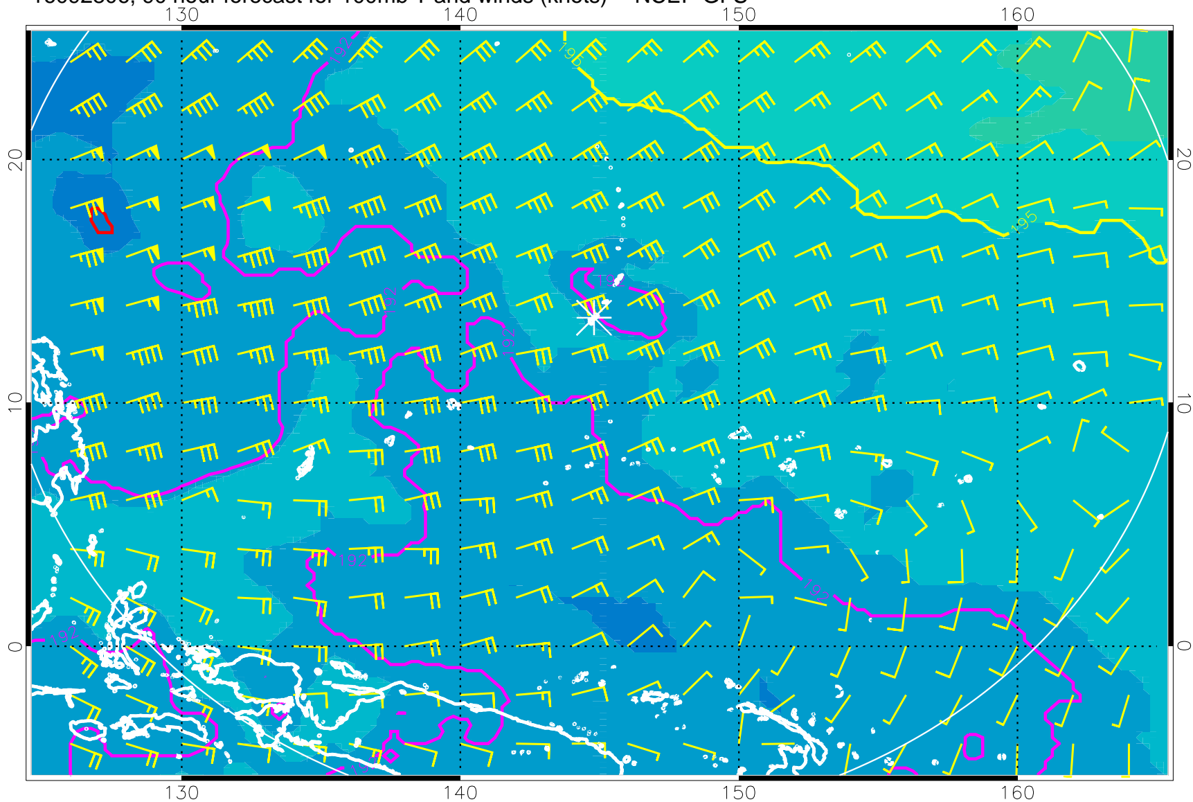
16092806, 90 hour forecast for 100mb T and winds (knots) -- NCEP GFS
