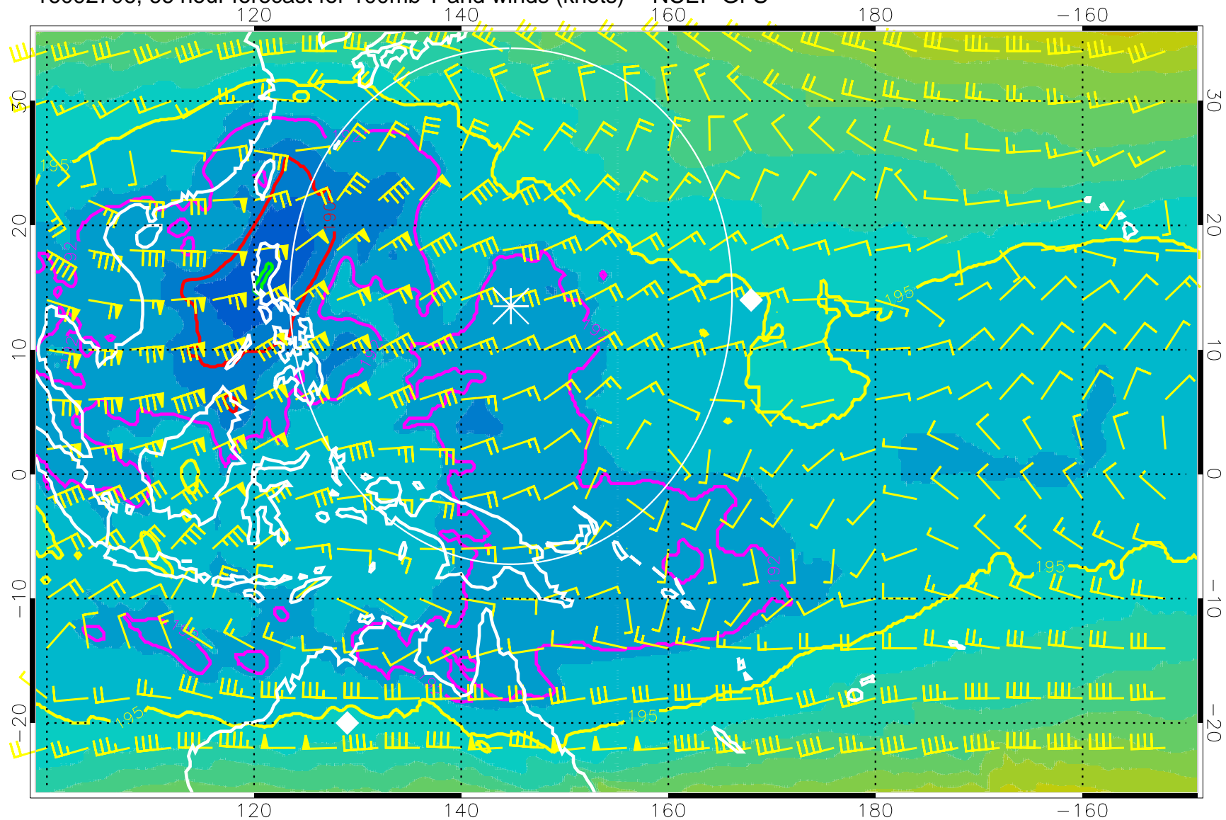
16092706, 66 hour forecast for 100mb T and winds (knots) -- NCEP GFS
