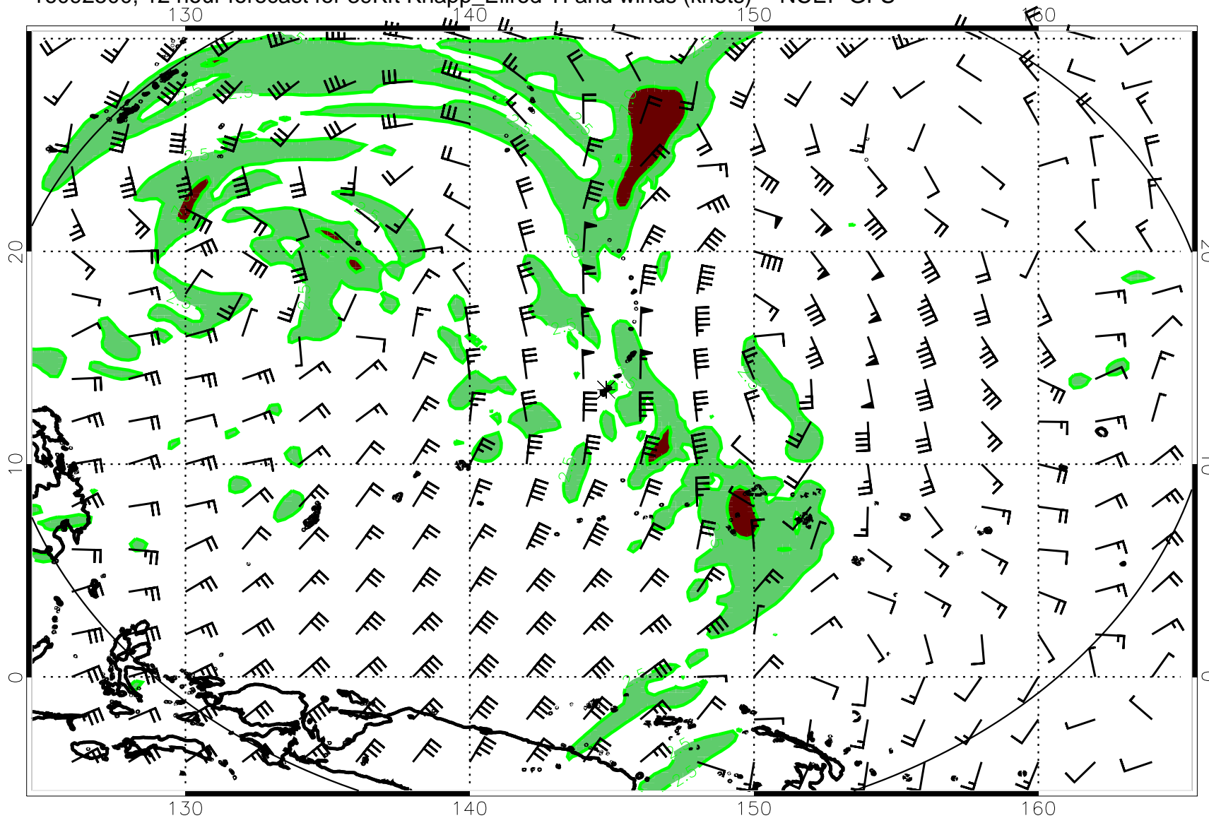
16092500, 12 hour forecast for 39Kft Knapp_Ellrod TI and winds (knots) -- NCEP GFS
