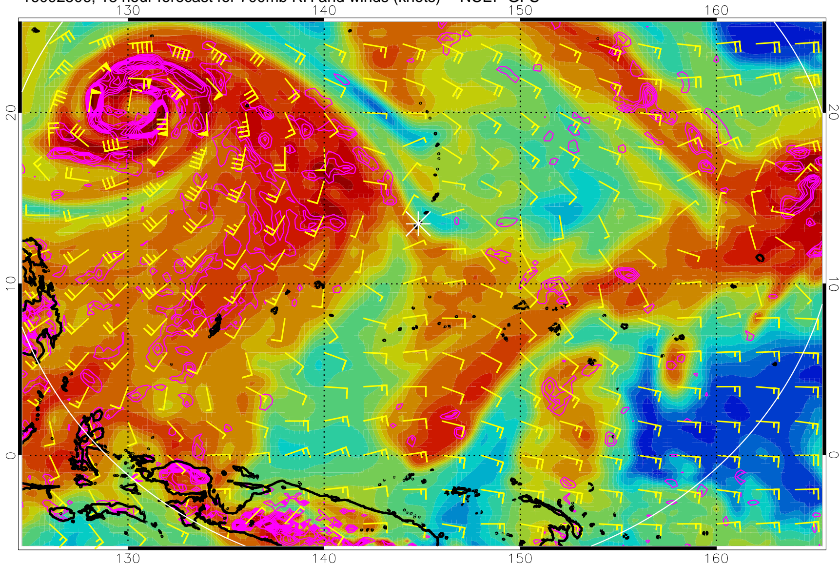
16092506, 18 hour forecast for 700mb RH and winds (knots) -- NCEP GFS
