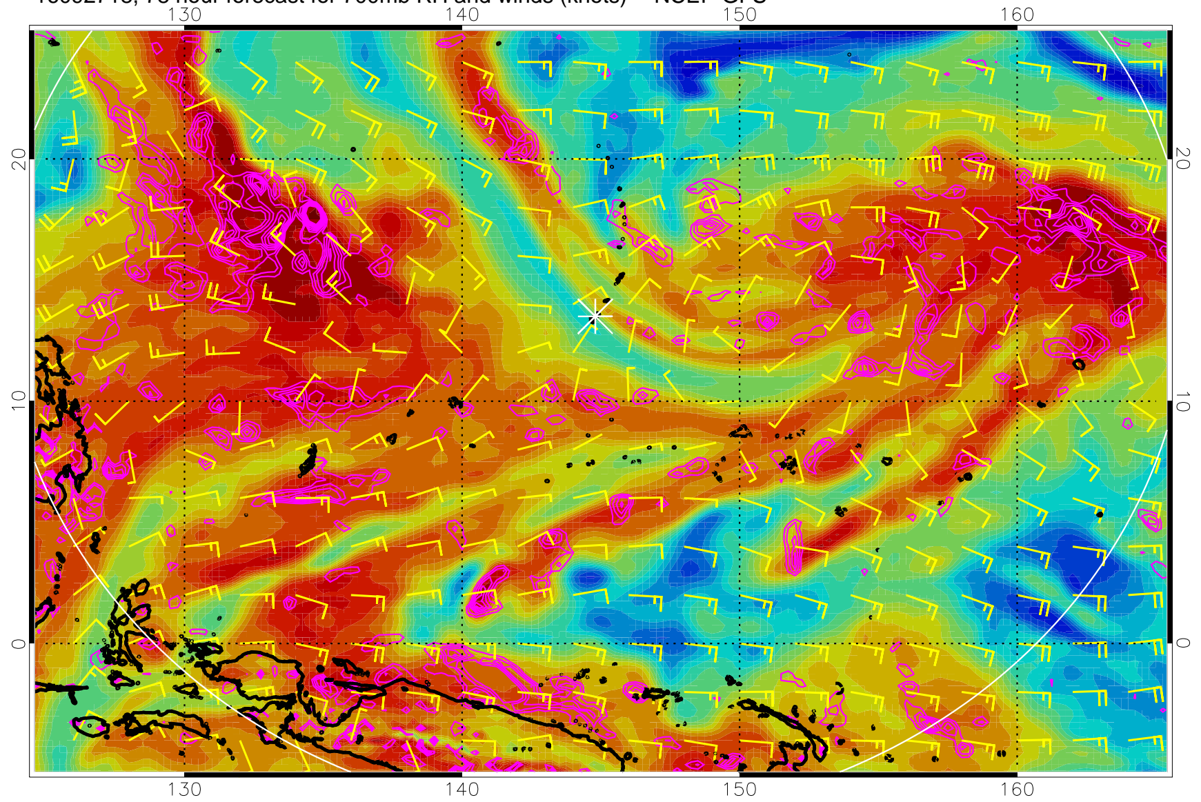
16092718, 78 hour forecast for 700mb RH and winds (knots) -- NCEP GFS
