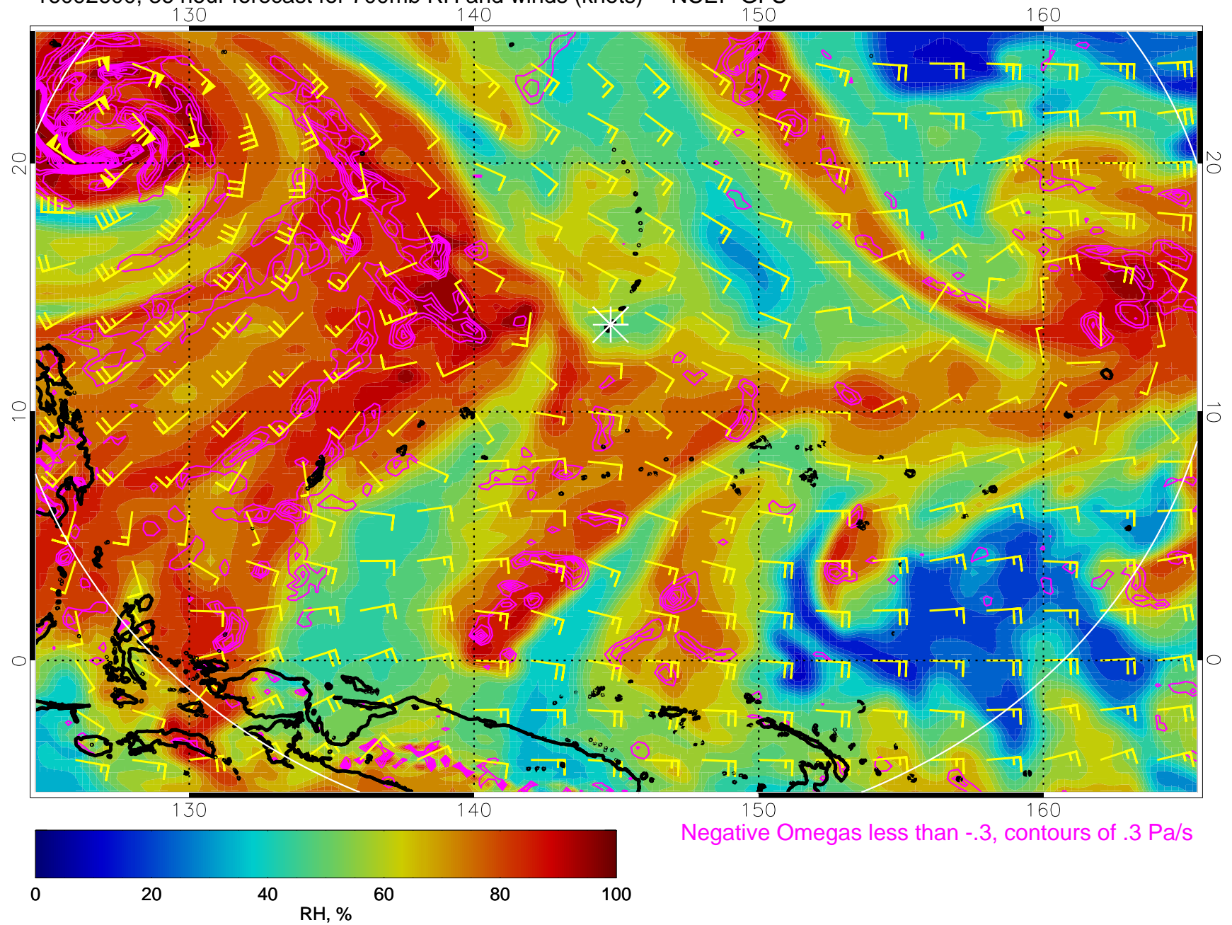
16092600, 36 hour forecast for 700mb RH and winds (knots) -- NCEP GFS
