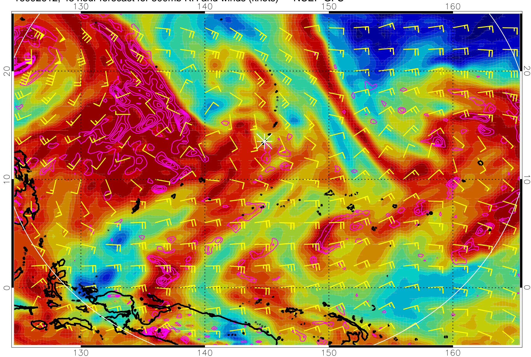
16092612, 48 hour forecast for 500mb RH and winds (knots) -- NCEP GFS
