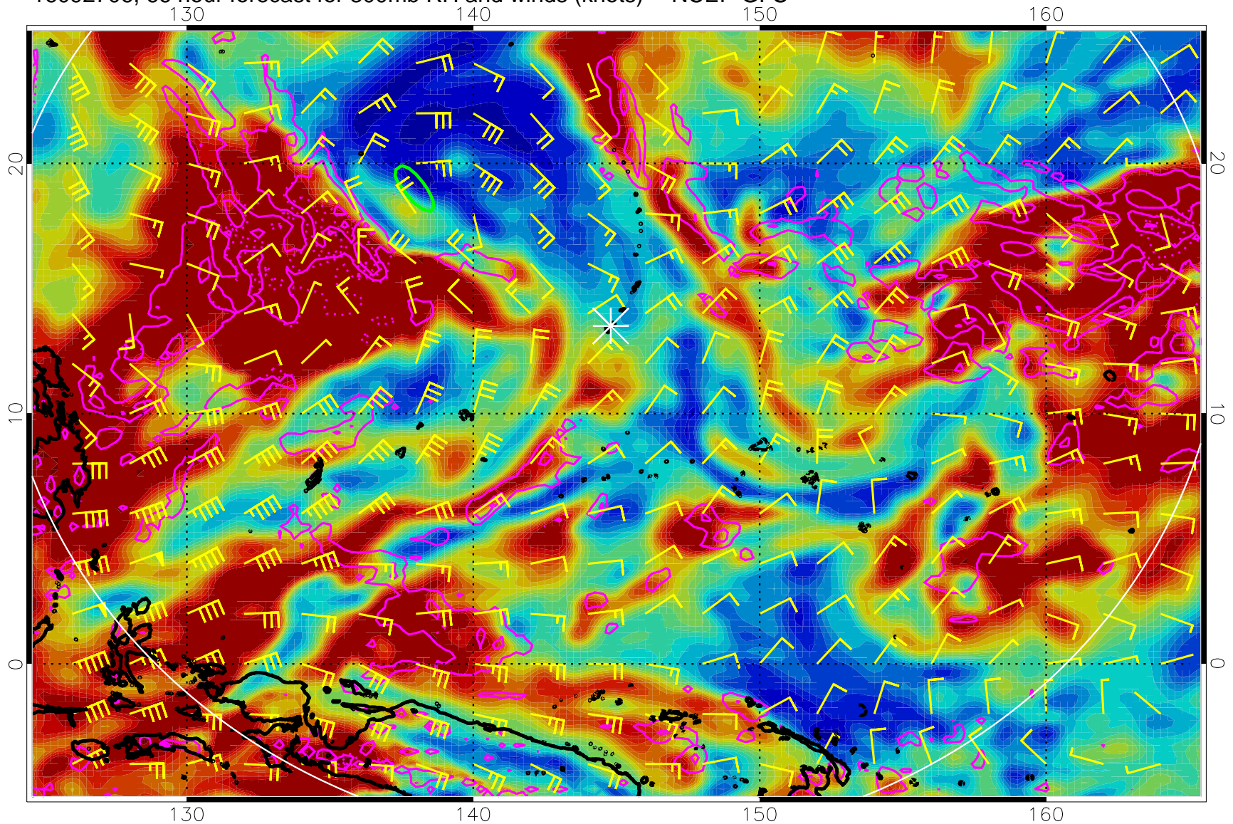
16092706, 66 hour forecast for 300mb RH and winds (knots) -- NCEP GFS
