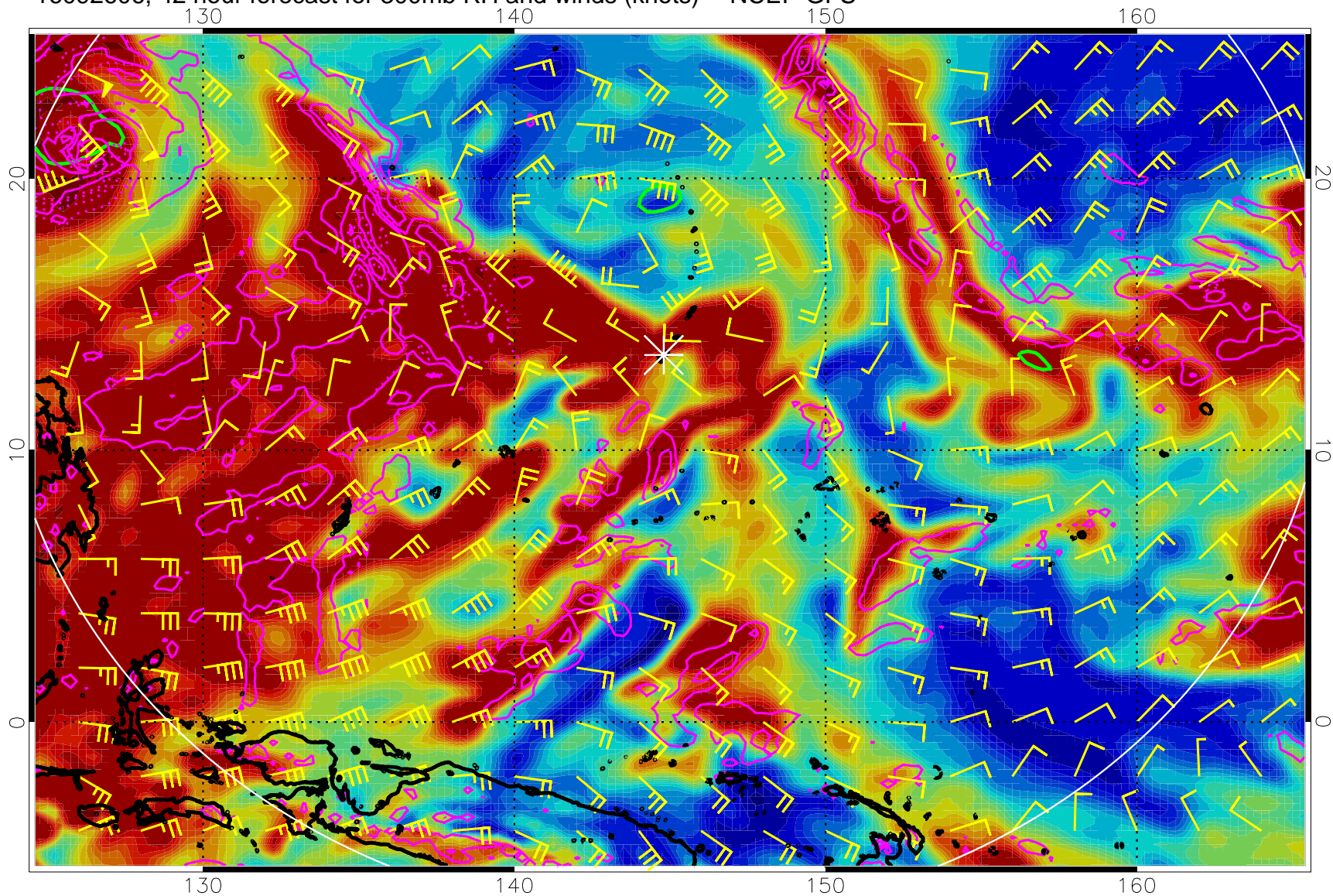
16092606, 42 hour forecast for 300mb RH and winds (knots) -- NCEP GFS
