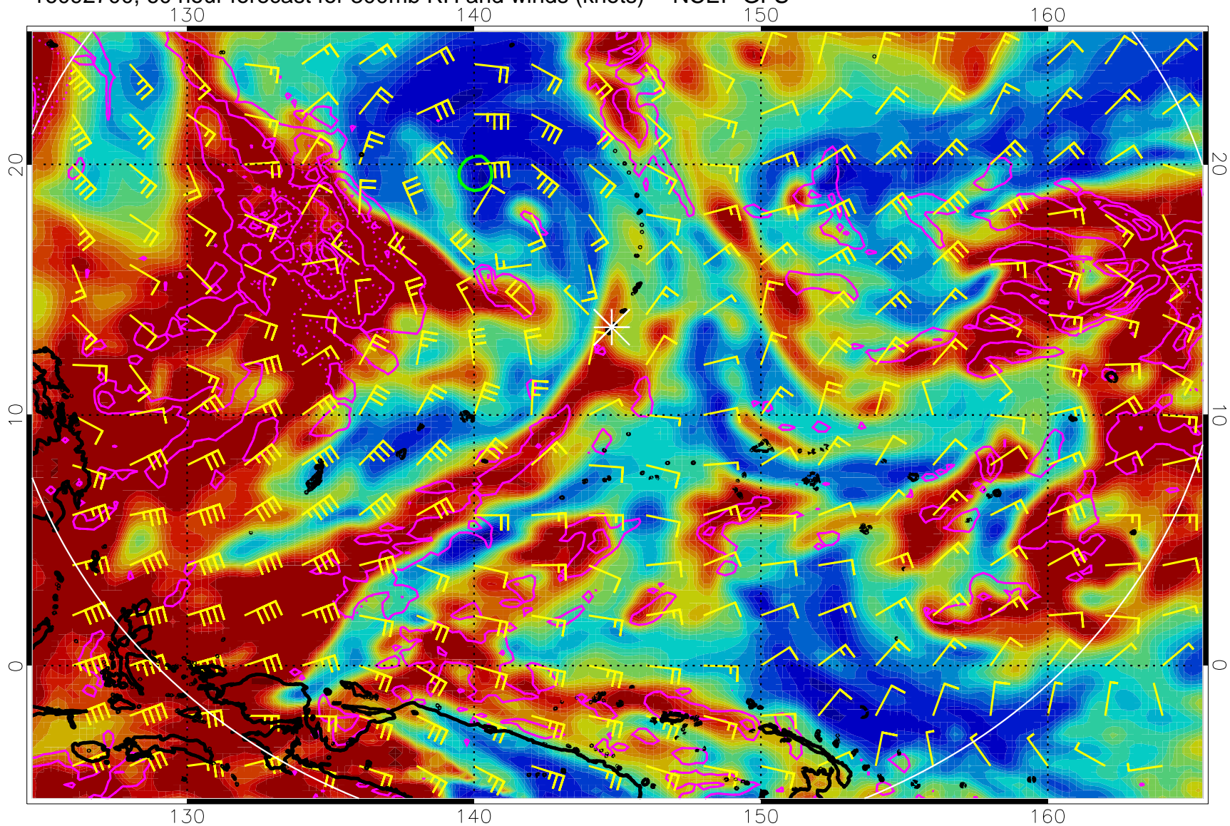
16092700, 60 hour forecast for 300mb RH and winds (knots) -- NCEP GFS
