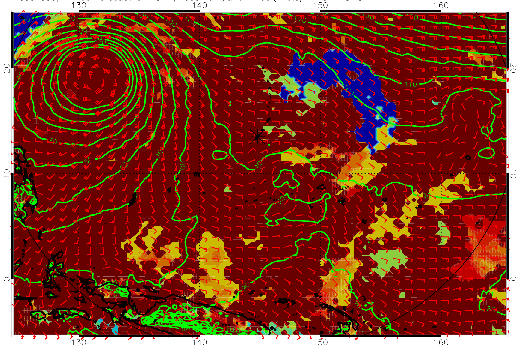
16092500, 12 hour forecast for HCAL, 1000mb Z, and winds (knots) -- NCEP GFS
