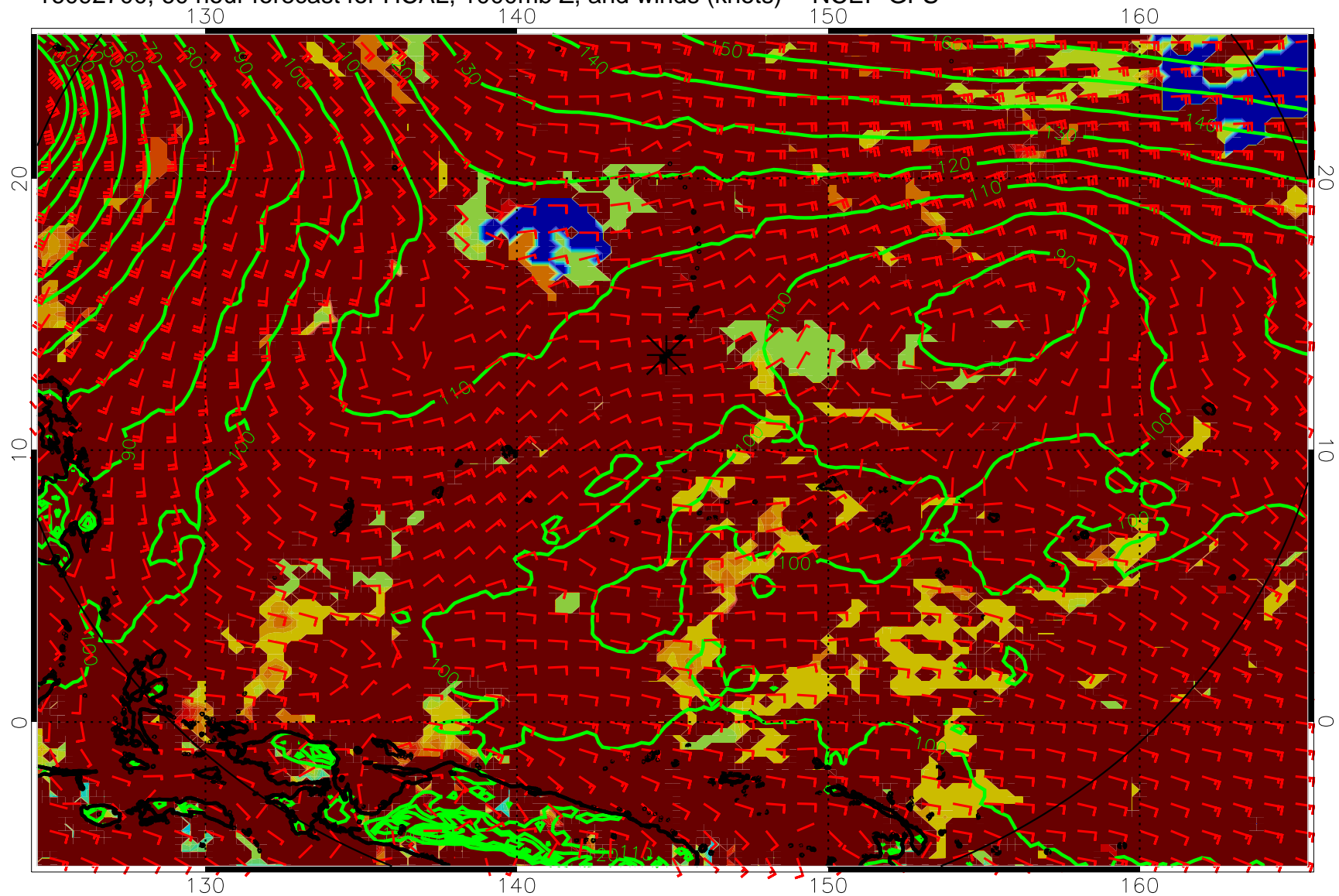
16092700, 60 hour forecast for HCAL, 1000mb Z, and winds (knots) -- NCEP GFS
