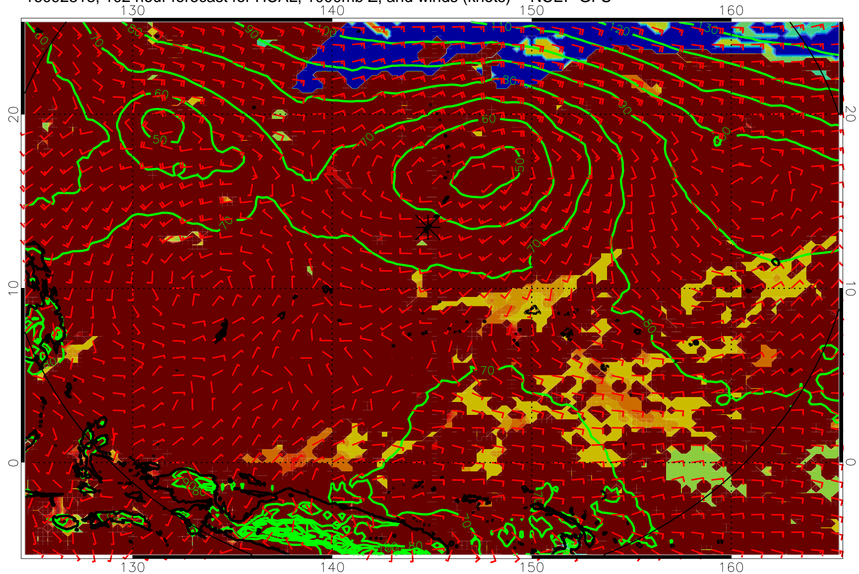
16092818, 102 hour forecast for HCAL, 1000mb Z, and winds (knots) -- NCEP GFS
