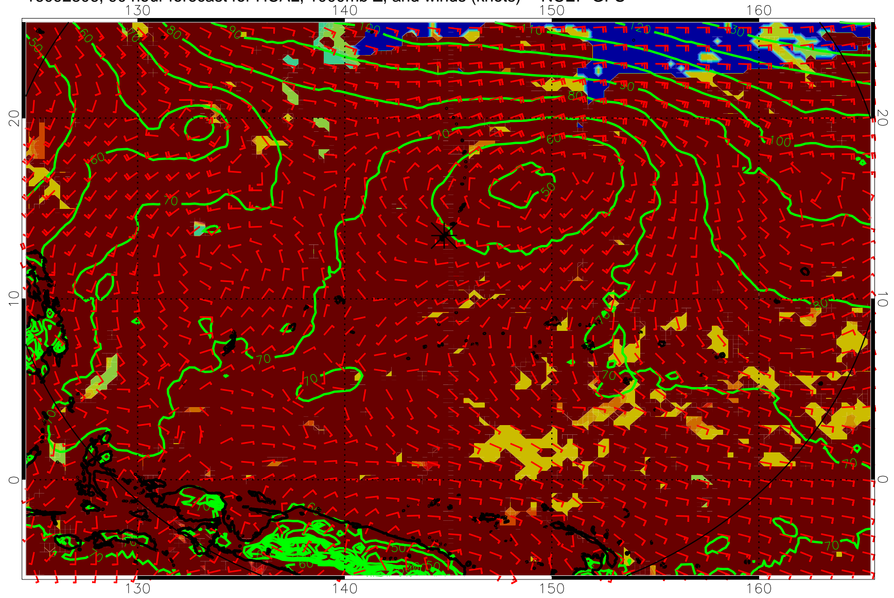
16092806, 90 hour forecast for HCAL, 1000mb Z, and winds (knots) -- NCEP GFS
