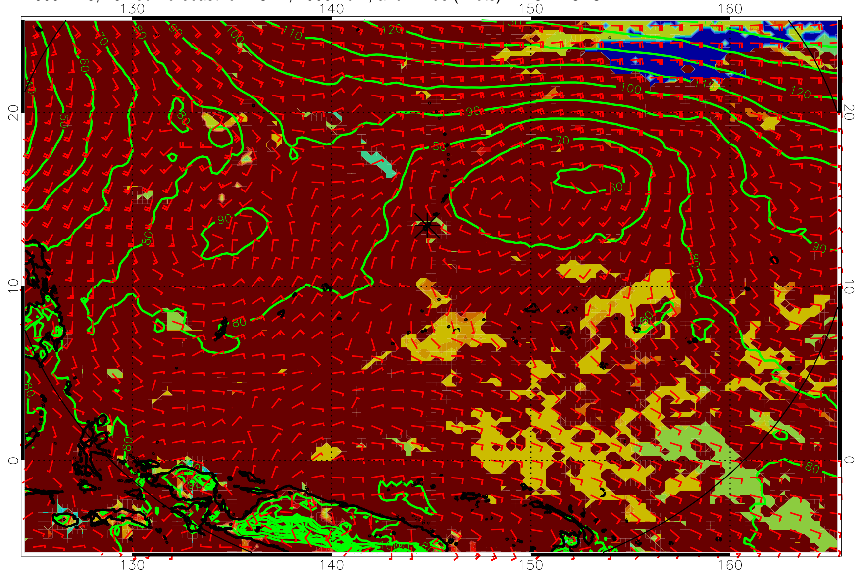
16092718, 78 hour forecast for HCAL, 1000mb Z, and winds (knots) -- NCEP GFS
