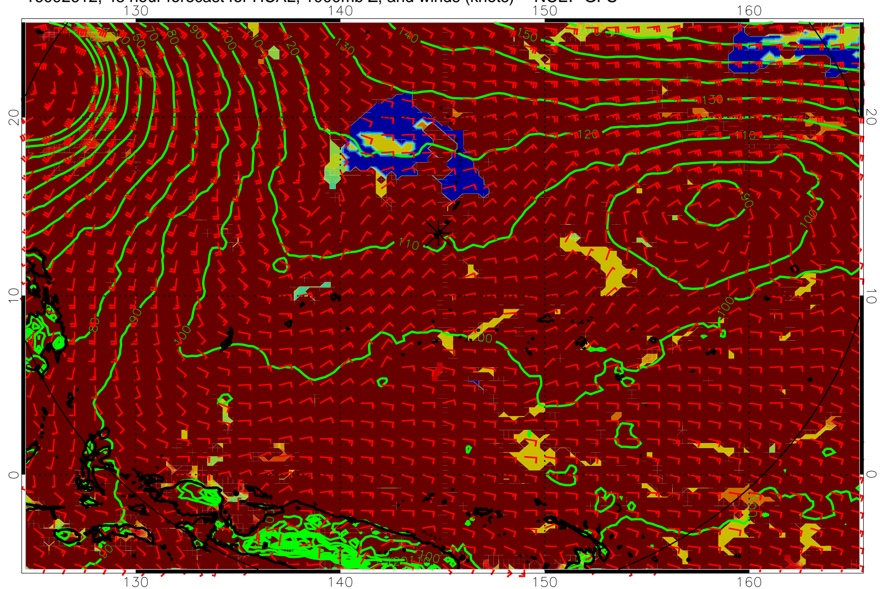
16092612, 48 hour forecast for HCAL, 1000mb Z, and winds (knots) -- NCEP GFS
