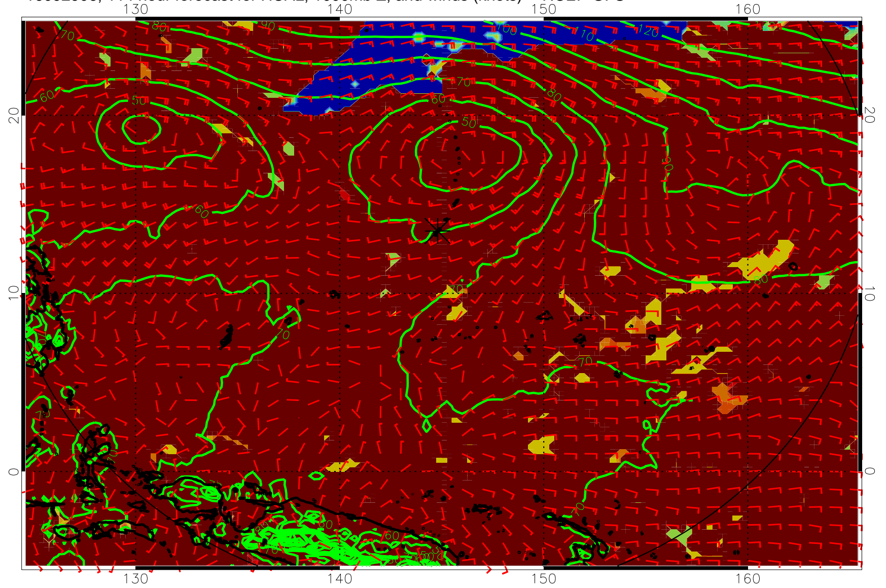
16092906, 114 hour forecast for HCAL, 1000mb Z, and winds (knots) -- NCEP GFS
