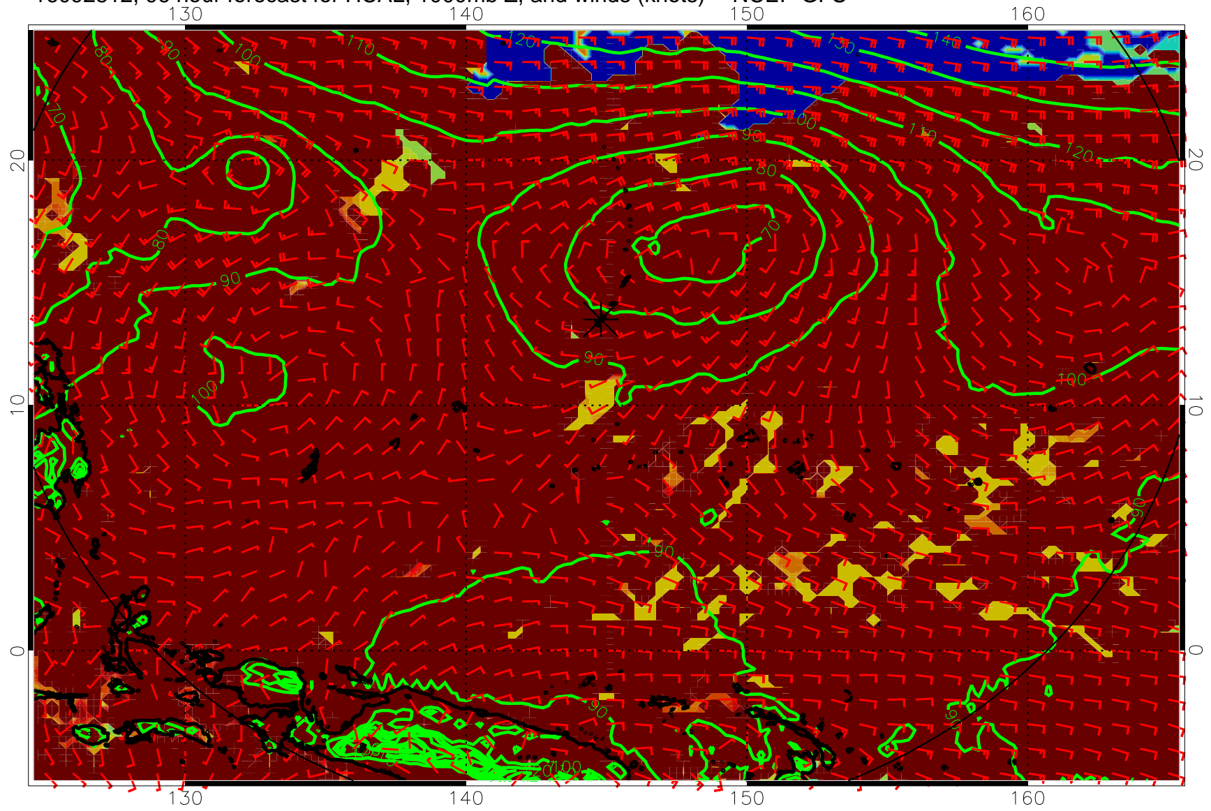
16092812, 96 hour forecast for HCAL, 1000mb Z, and winds (knots) -- NCEP GFS
