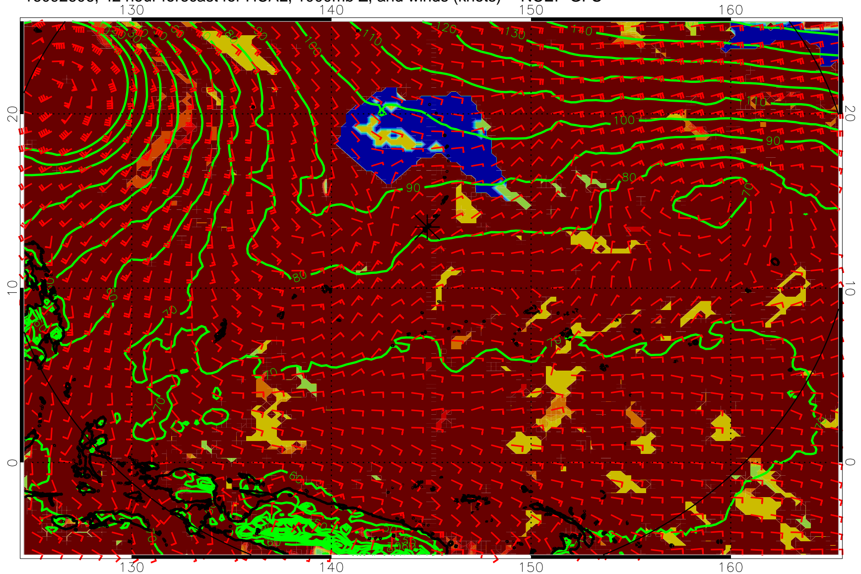
16092606, 42 hour forecast for HCAL, 1000mb Z, and winds (knots) -- NCEP GFS
