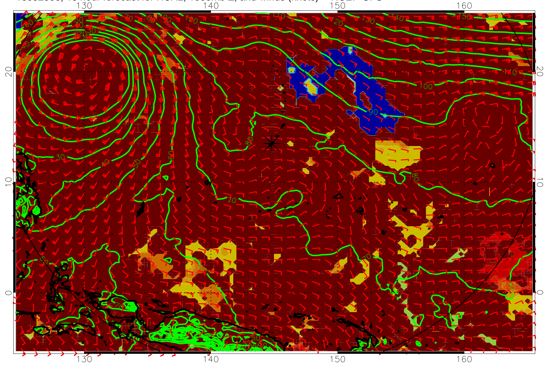
16092506, 18 hour forecast for HCAL, 1000mb Z, and winds (knots) -- NCEP GFS
