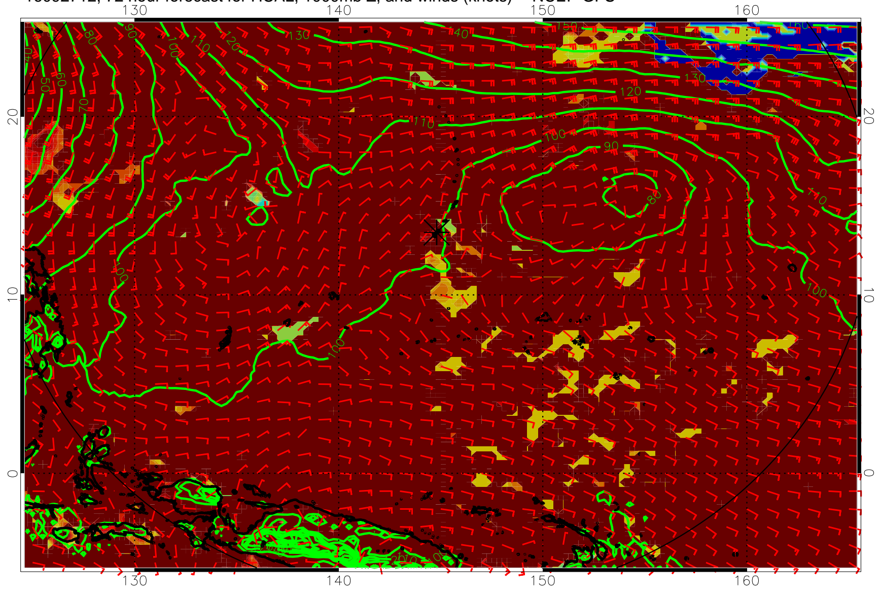
16092712, 72 hour forecast for HCAL, 1000mb Z, and winds (knots) -- NCEP GFS
