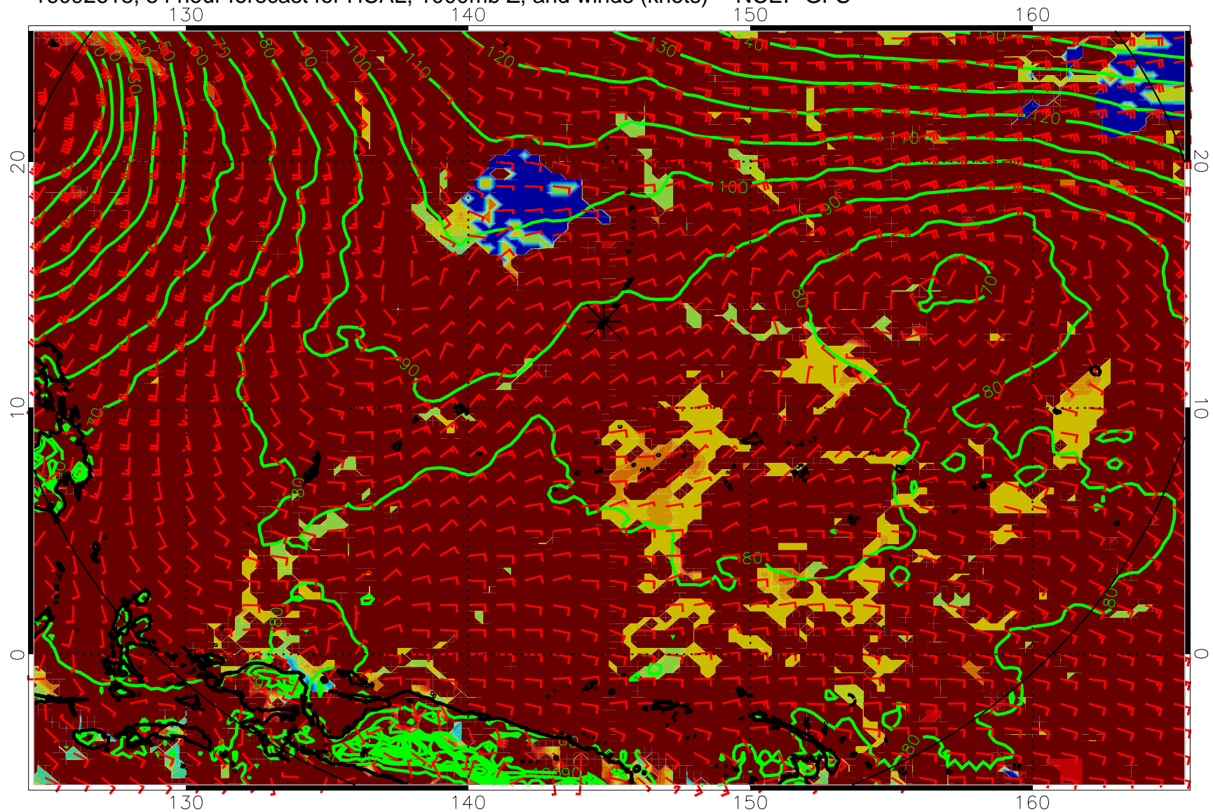
16092618, 54 hour forecast for HCAL, 1000mb Z, and winds (knots) -- NCEP GFS
