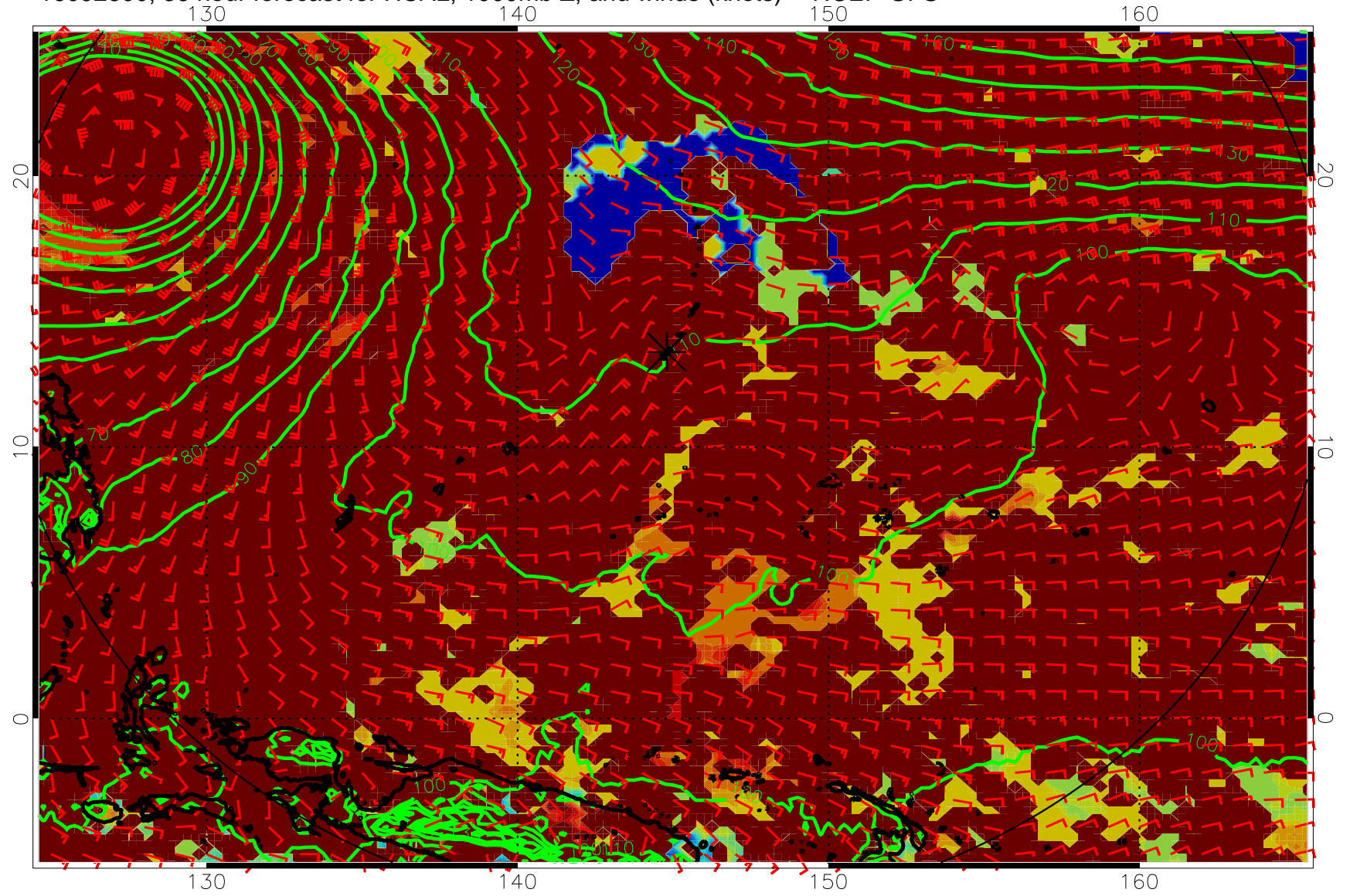
16092600, 36 hour forecast for HCAL, 1000mb Z, and winds (knots) -- NCEP GFS
