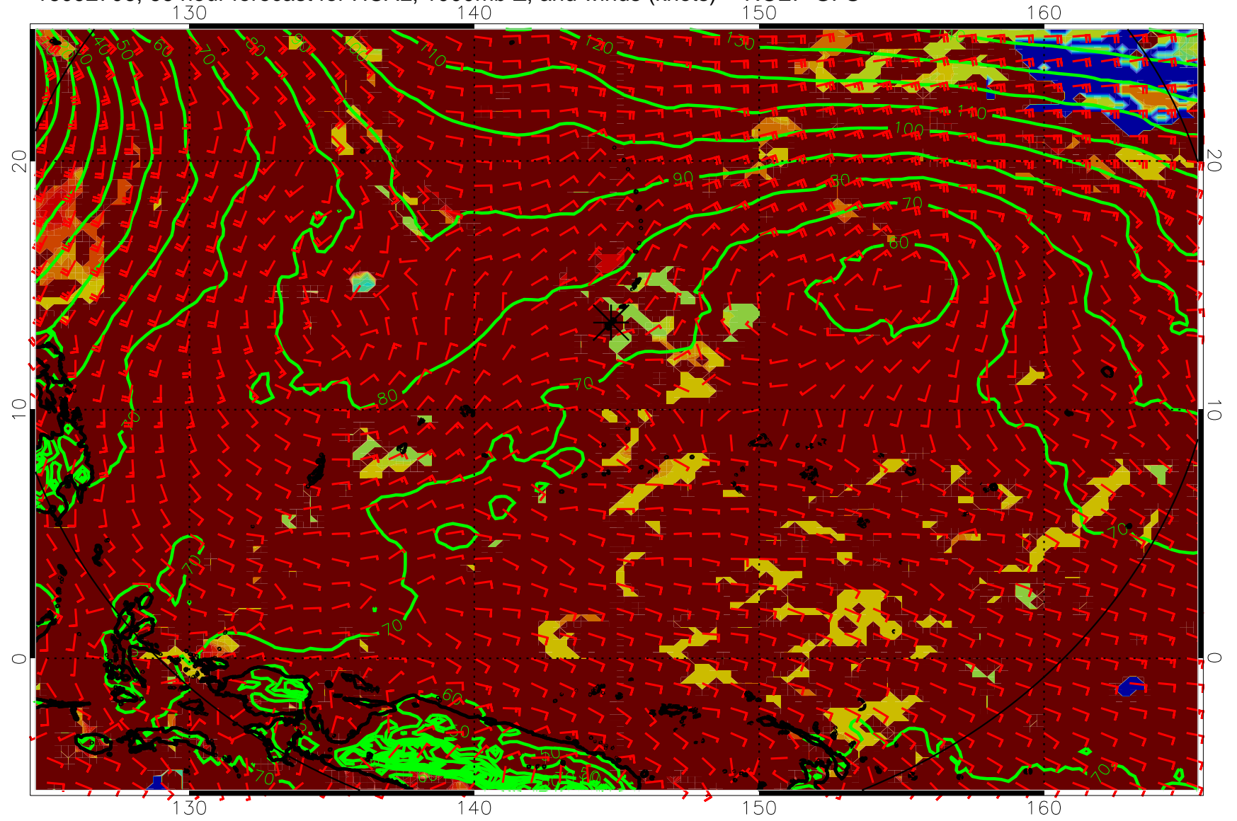
16092706, 66 hour forecast for HCAL, 1000mb Z, and winds (knots) -- NCEP GFS
