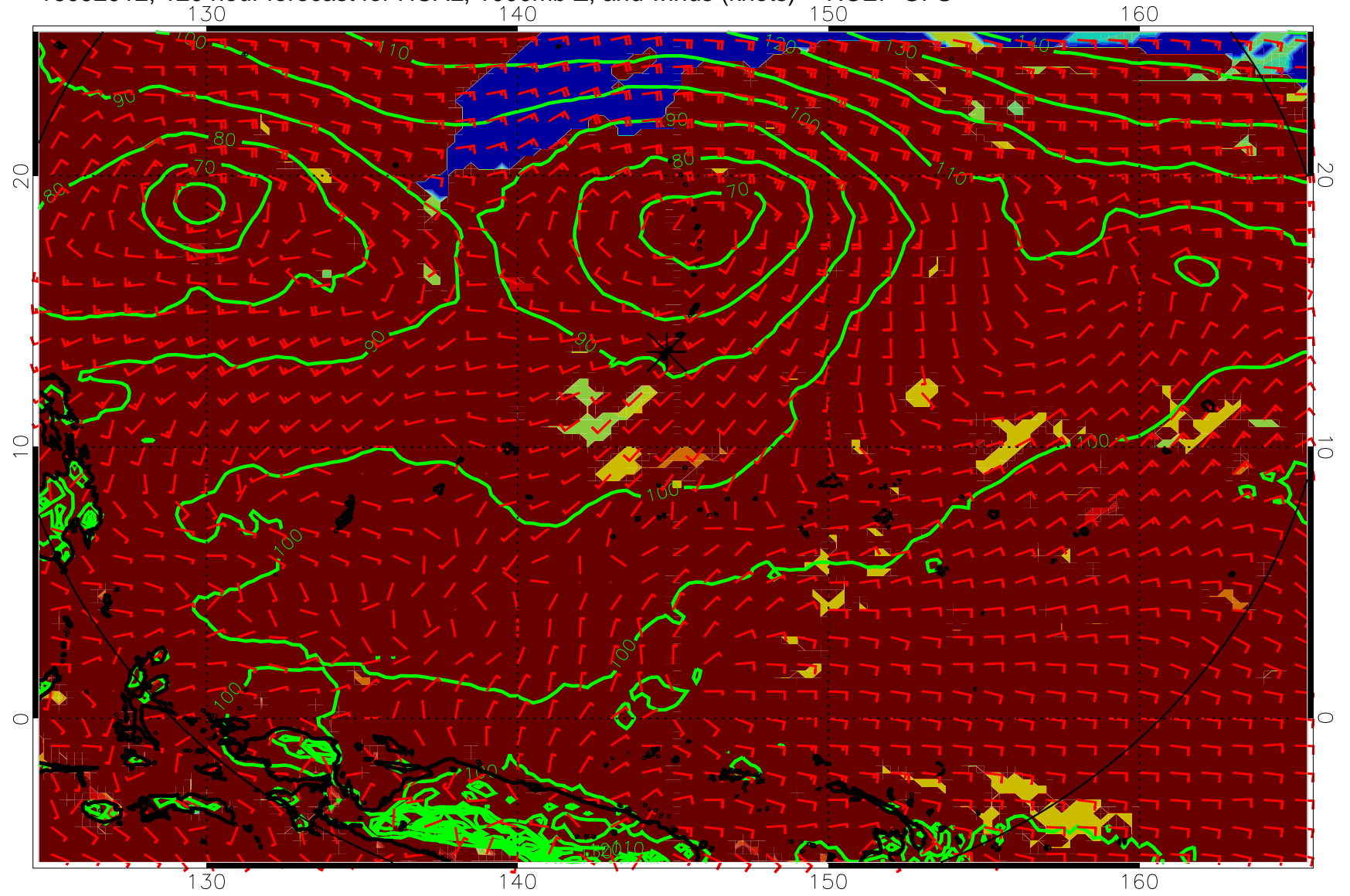
16092912, 120 hour forecast for HCAL, 1000mb Z, and winds (knots) -- NCEP GFS
