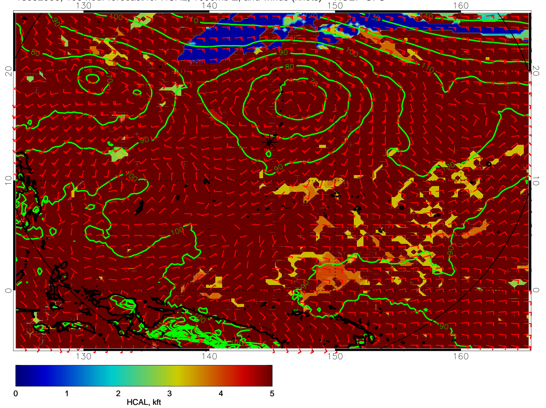
16092900, 108 hour forecast for HCAL, 1000mb Z, and winds (knots) -- NCEP GFS
