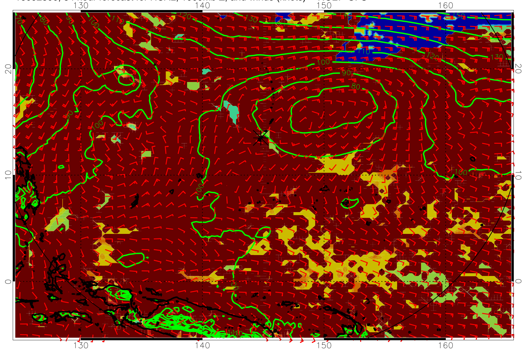
16092800, 84 hour forecast for HCAL, 1000mb Z, and winds (knots) -- NCEP GFS
