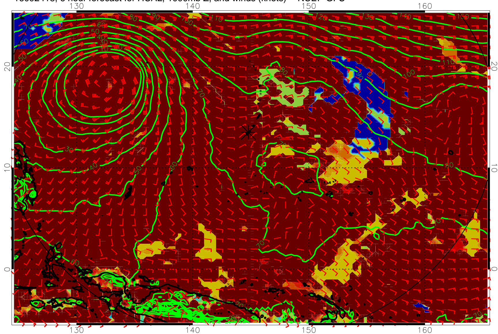
16092418, 6 hour forecast for HCAL, 1000mb Z, and winds (knots) -- NCEP GFS
