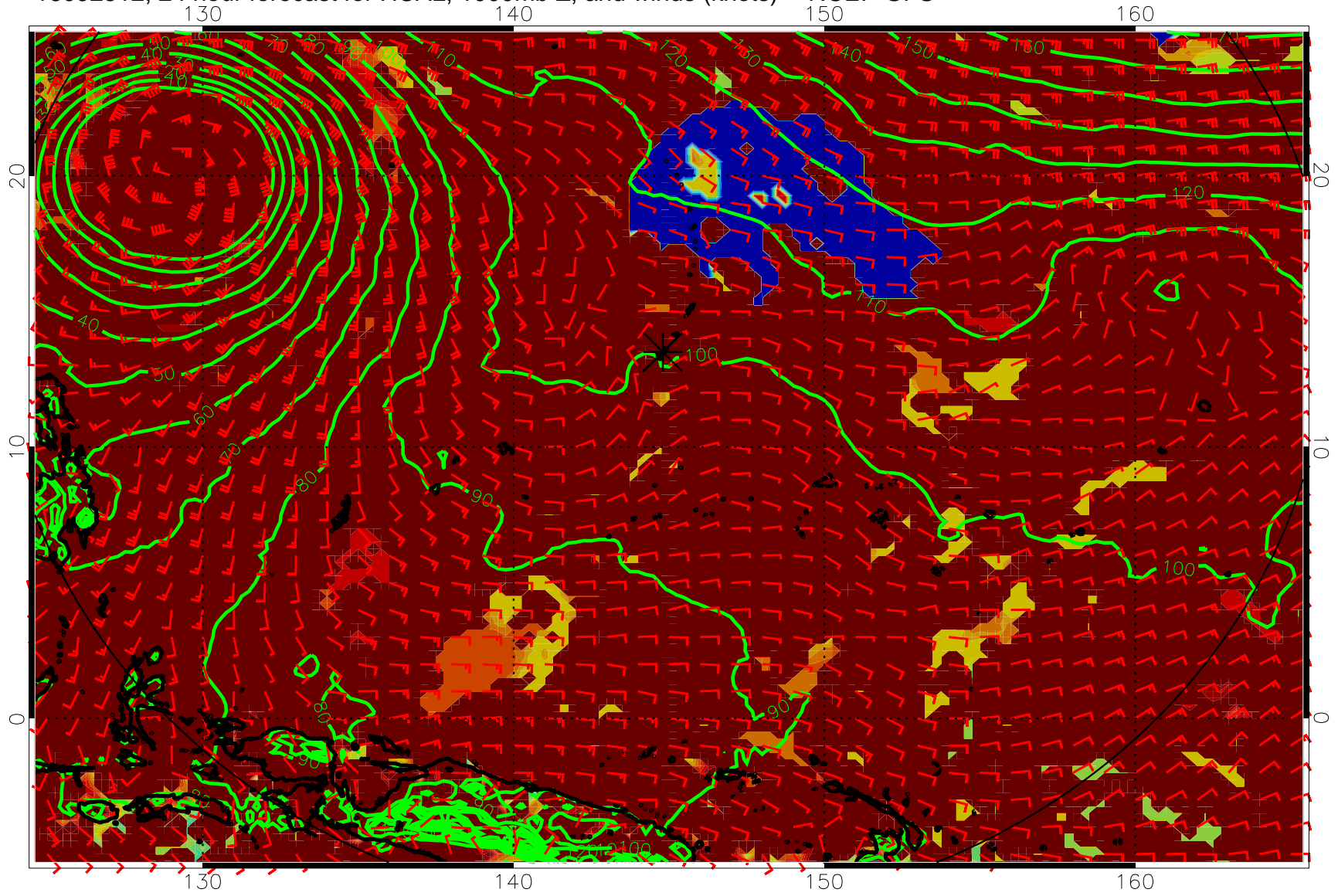
16092512, 24 hour forecast for HCAL, 1000mb Z, and winds (knots) -- NCEP GFS
