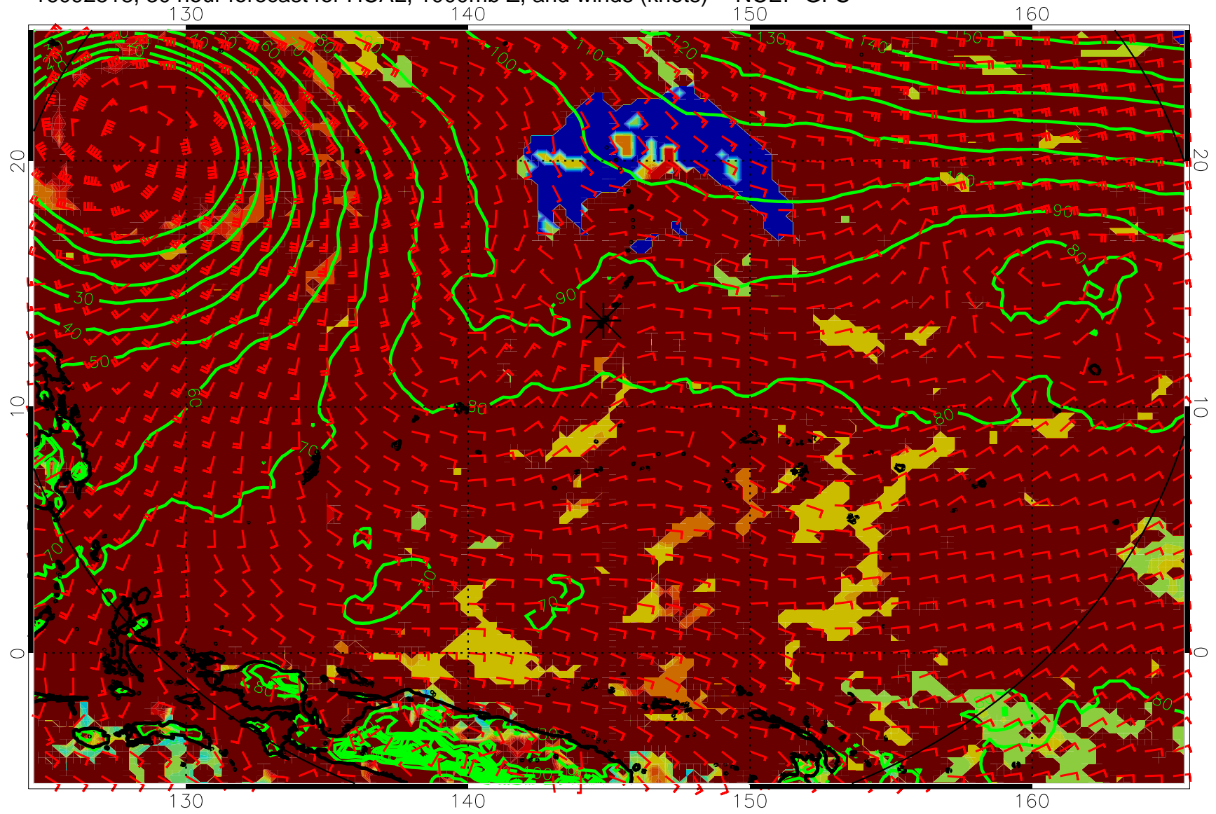
16092518, 30 hour forecast for HCAL, 1000mb Z, and winds (knots) -- NCEP GFS
