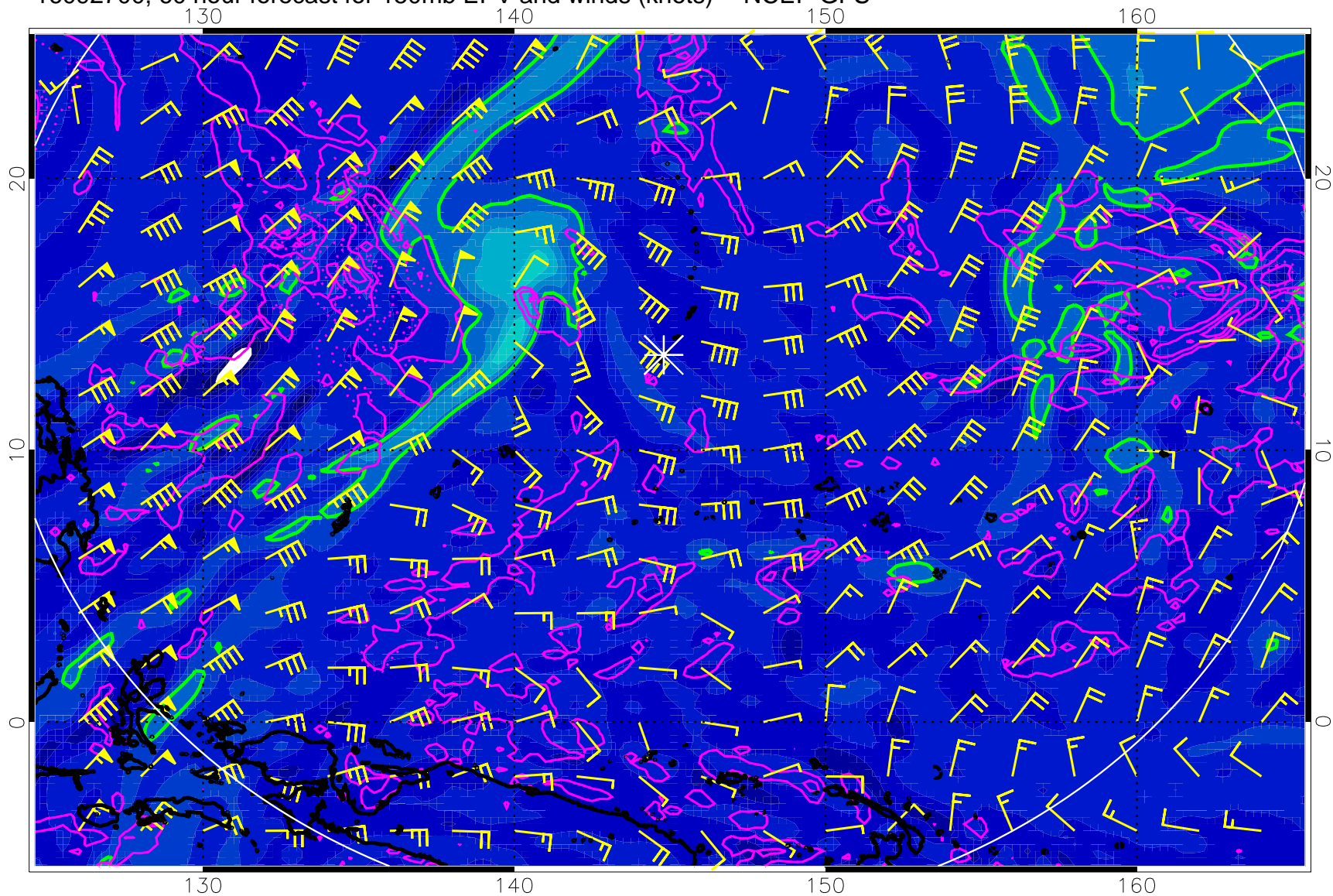
16092700, 60 hour forecast for 150mb EPV and winds (knots) -- NCEP GFS
