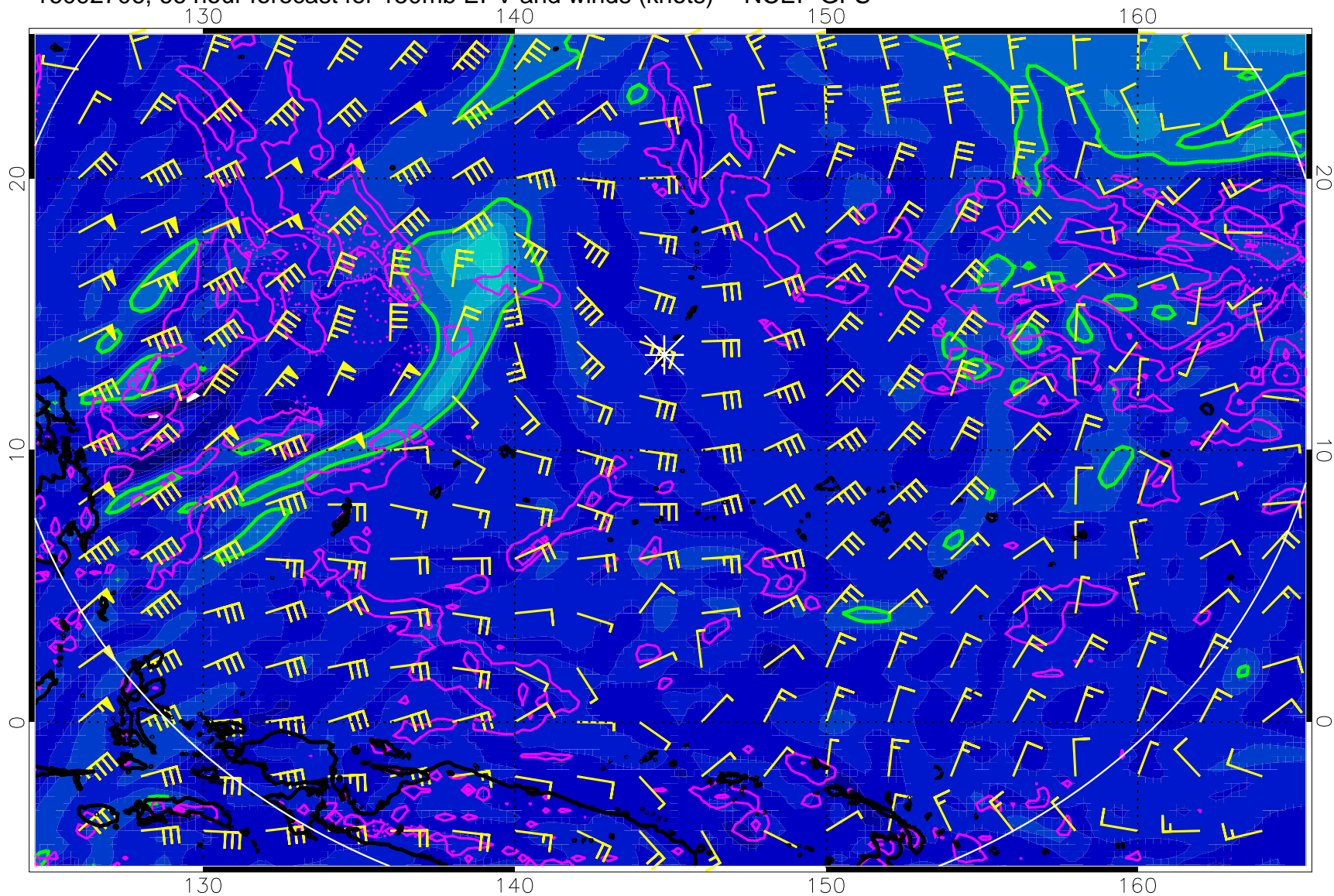
16092706, 66 hour forecast for 150mb EPV and winds (knots) -- NCEP GFS
