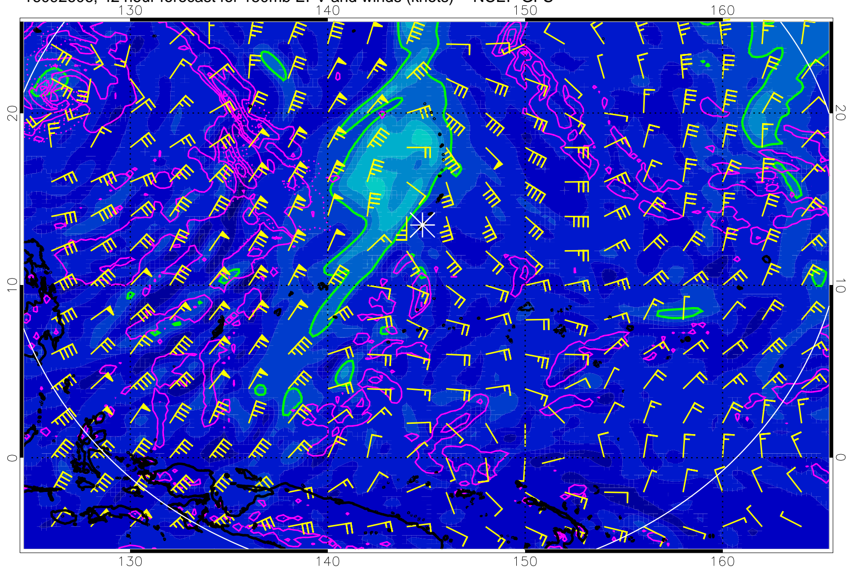
16092606, 42 hour forecast for 150mb EPV and winds (knots) -- NCEP GFS
