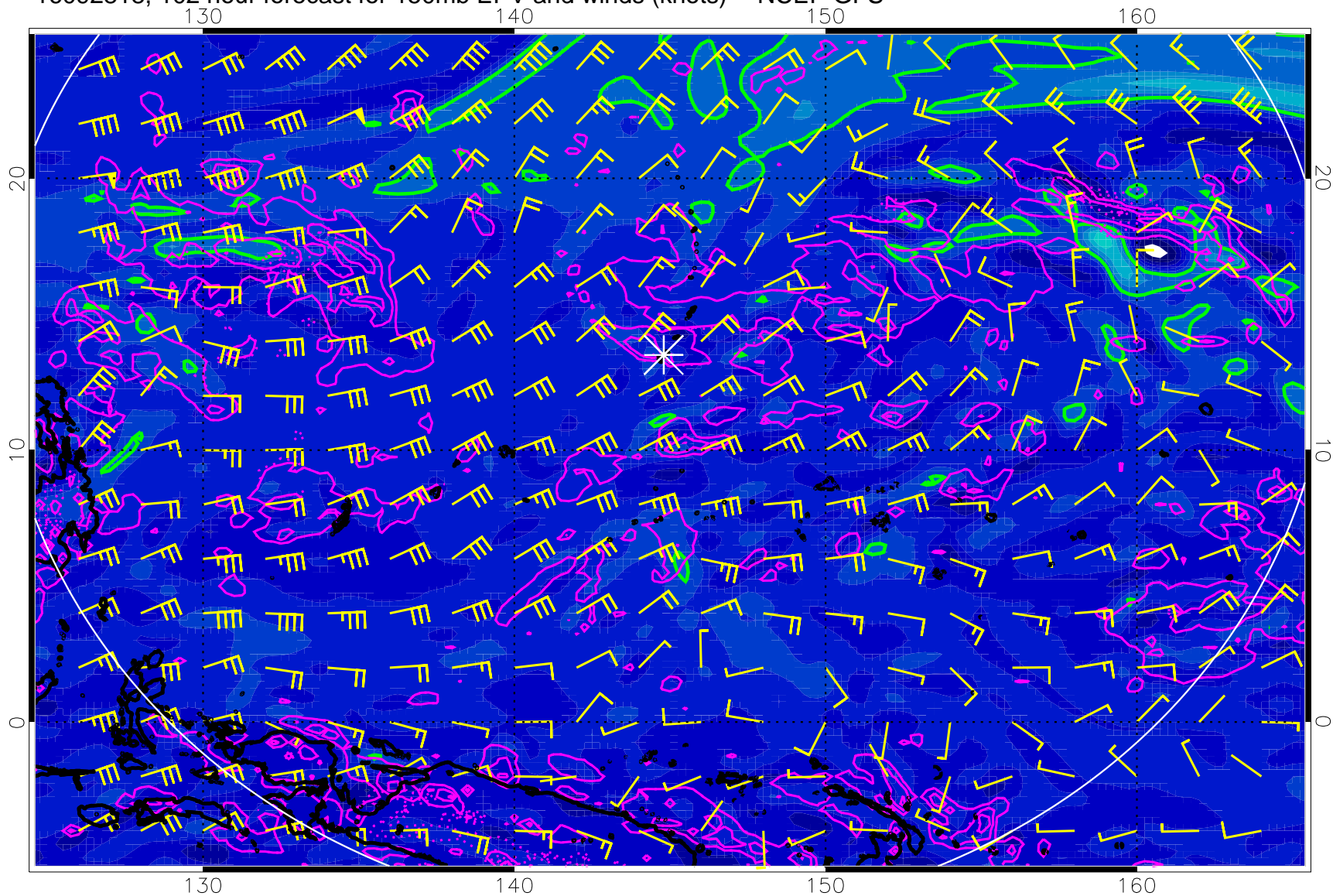
16092818, 102 hour forecast for 150mb EPV and winds (knots) -- NCEP GFS
