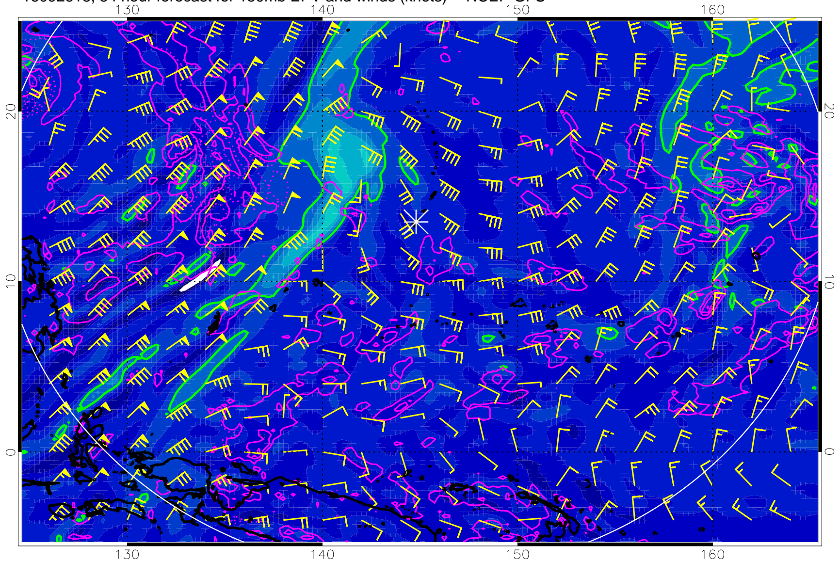
16092618, 54 hour forecast for 150mb EPV and winds (knots) -- NCEP GFS
