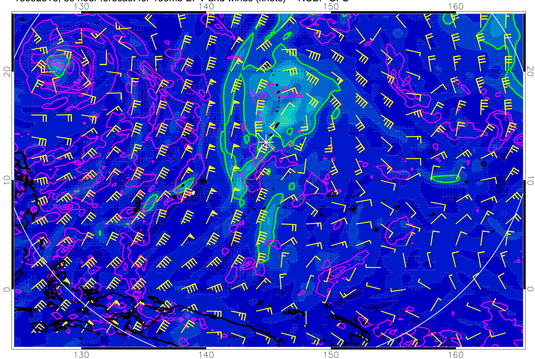
16092518, 30 hour forecast for 150mb EPV and winds (knots) -- NCEP GFS
