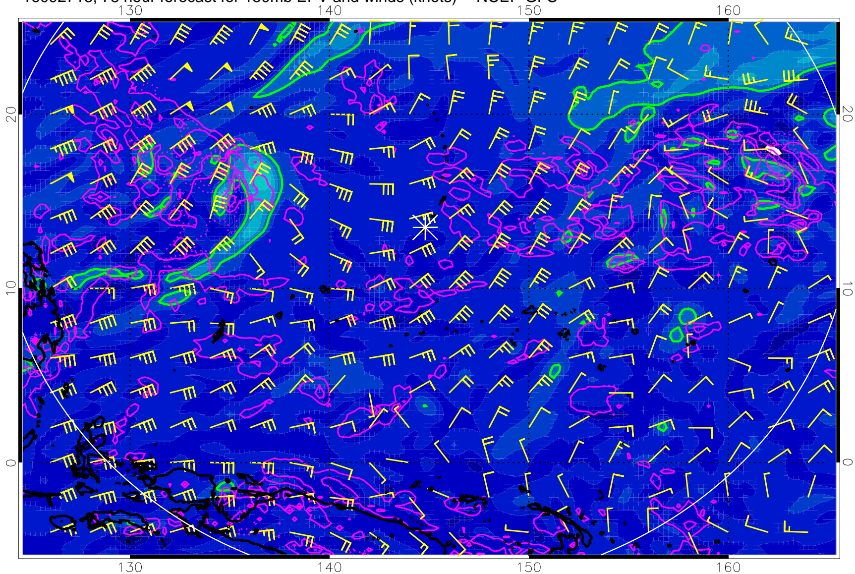
16092718, 78 hour forecast for 150mb EPV and winds (knots) -- NCEP GFS
