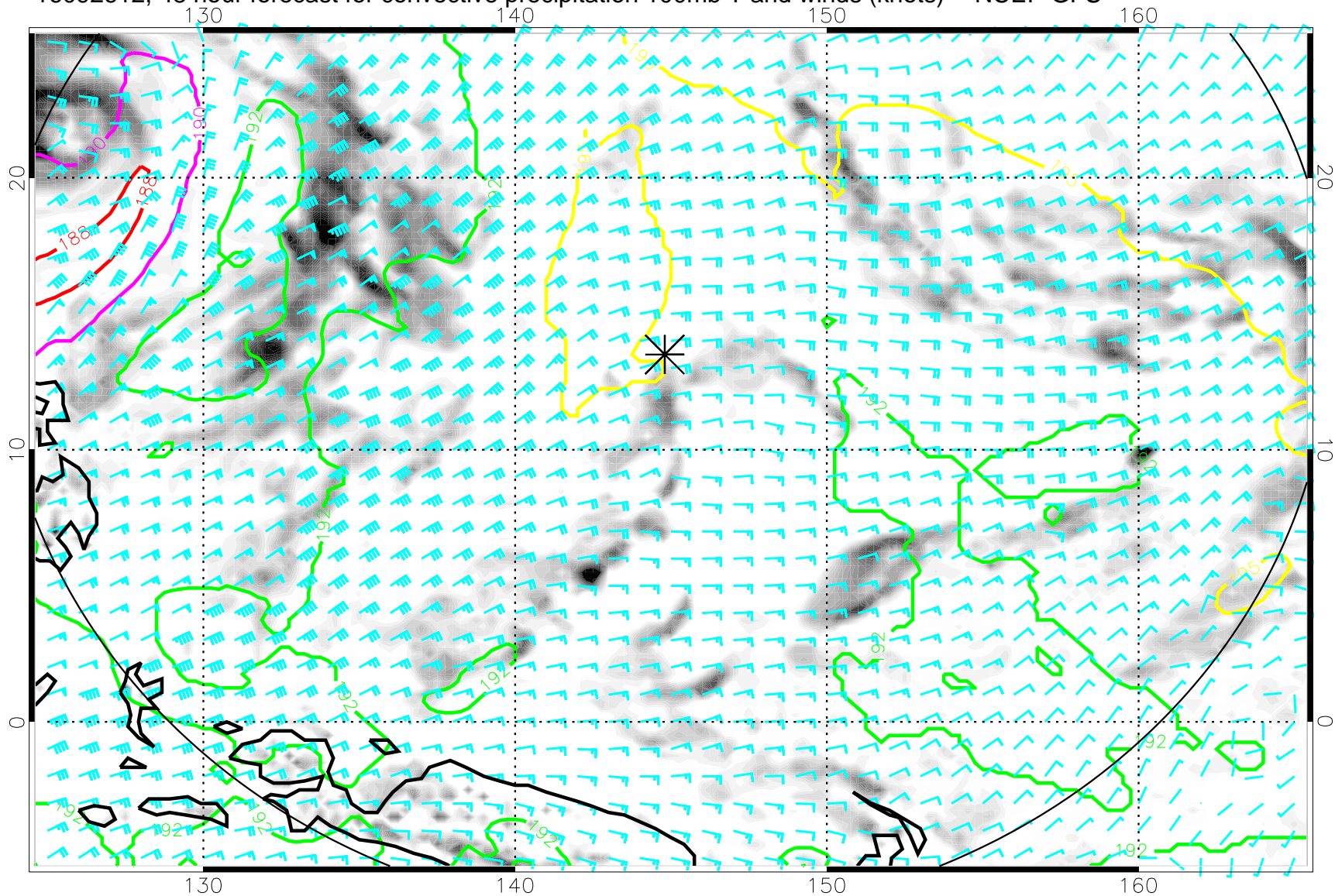
16092612, 48 hour forecast for convective precipitation 100mb T and winds (knots) -- NCEP GFS
