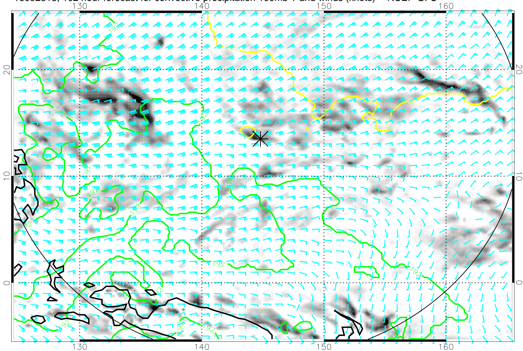
16092818, 102 hour forecast for convective precipitation 100mb T and winds (knots) -- NCEP GFS
