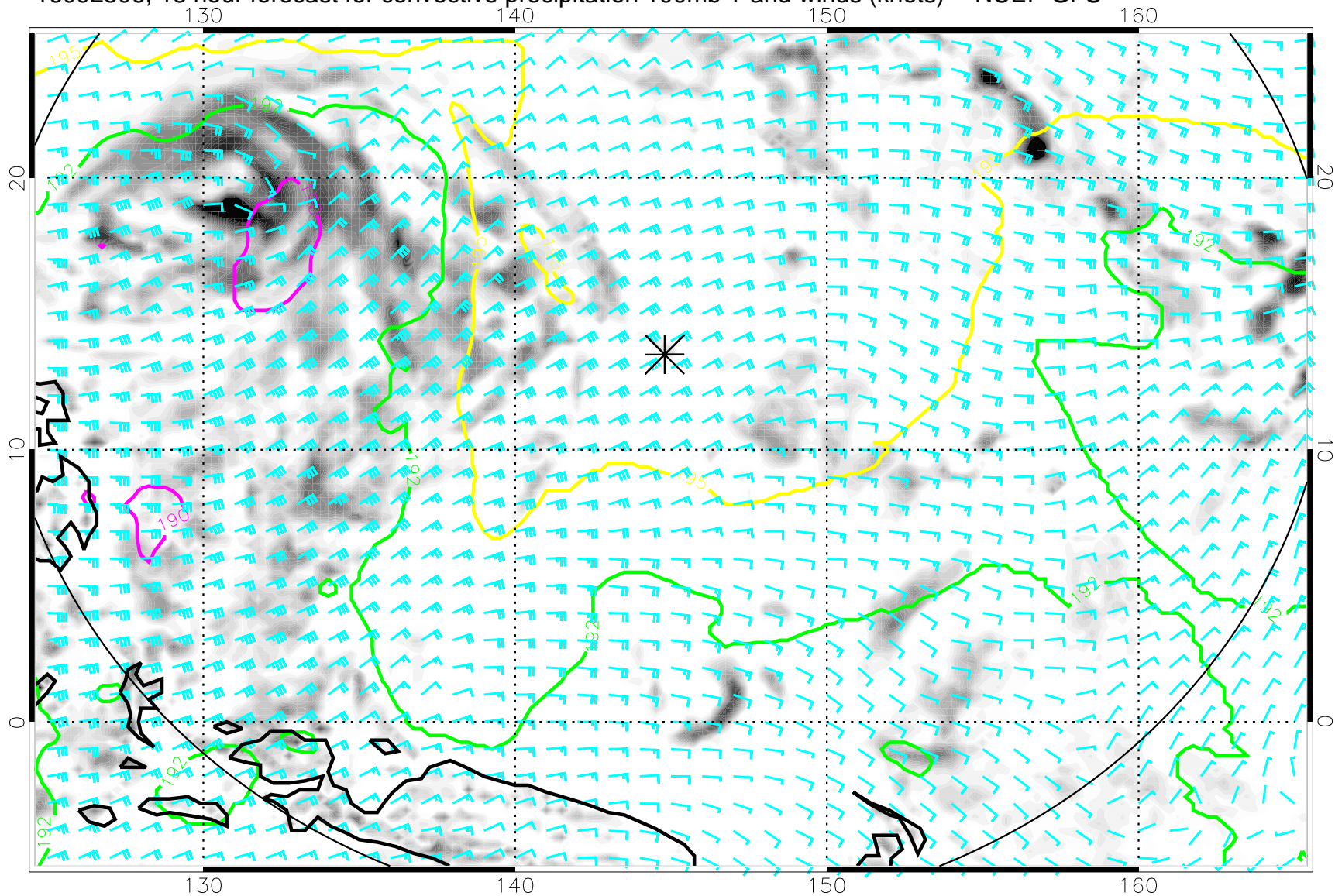
16092506, 18 hour forecast for convective precipitation 100mb T and winds (knots) -- NCEP GFS
