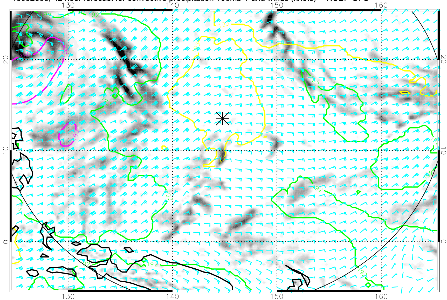
16092606, 42 hour forecast for convective precipitation 100mb T and winds (knots) -- NCEP GFS
