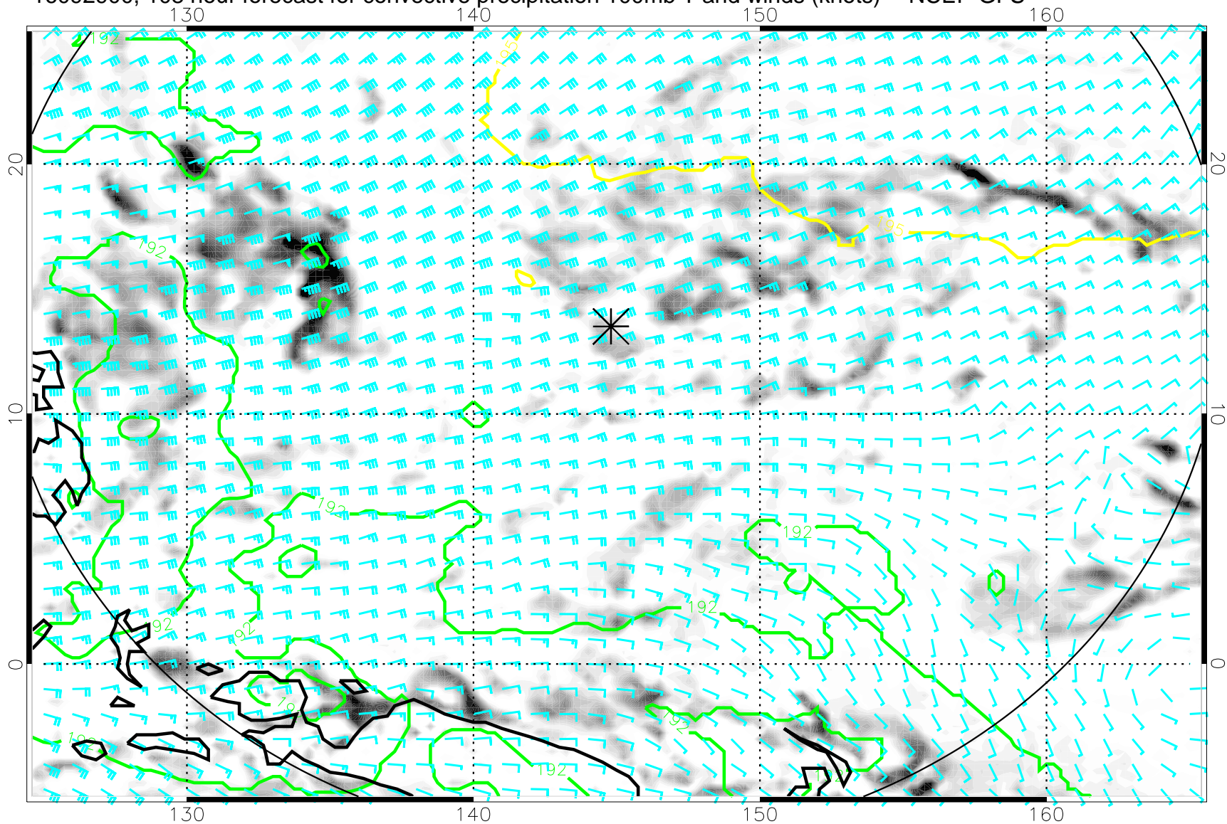
16092900, 108 hour forecast for convective precipitation 100mb T and winds (knots) -- NCEP GFS
