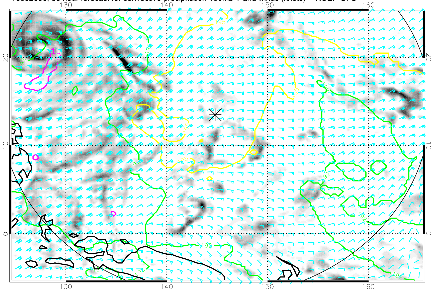
16092600, 36 hour forecast for convective precipitation 100mb T and winds (knots) -- NCEP GFS
