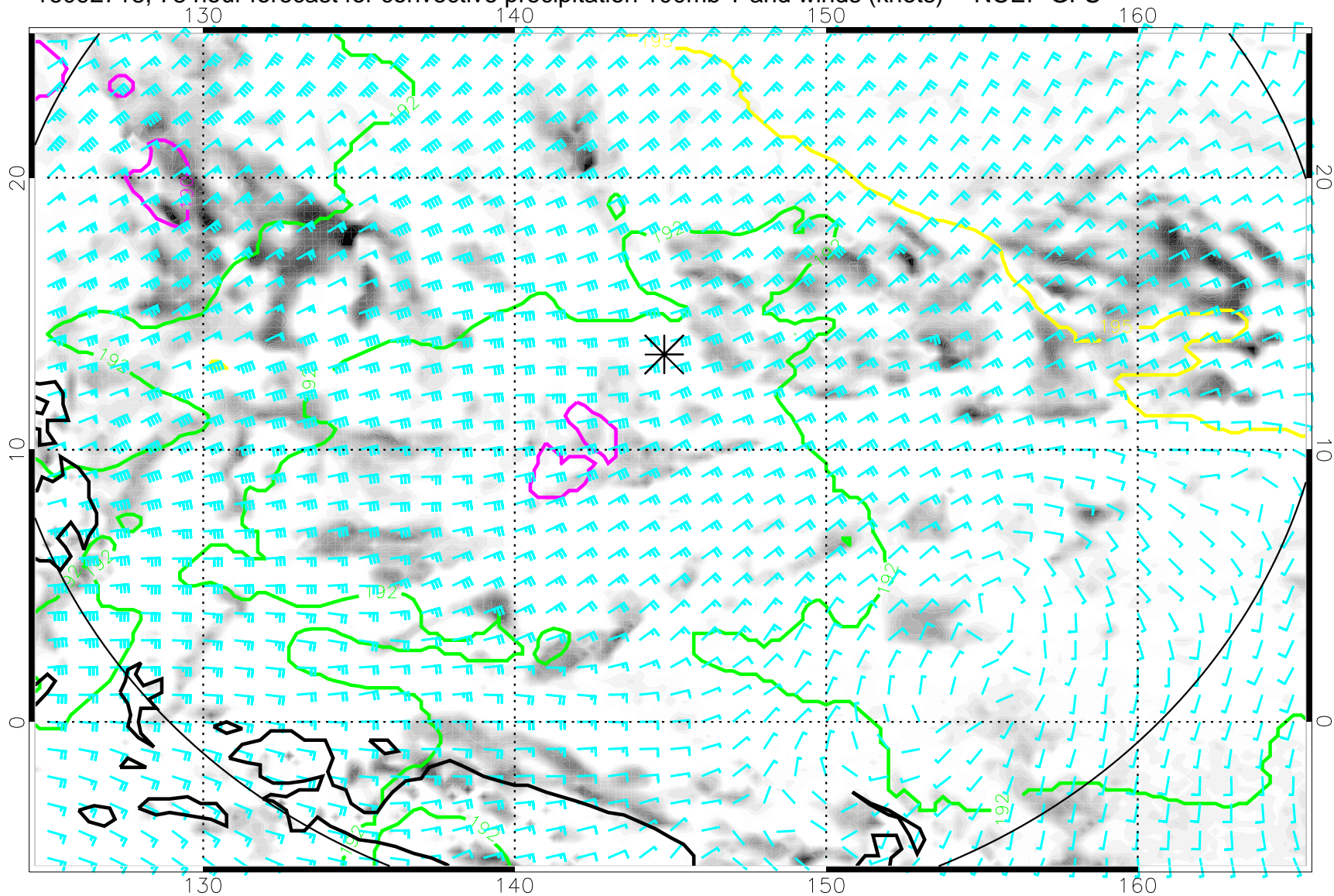
16092718, 78 hour forecast for convective precipitation 100mb T and winds (knots) -- NCEP GFS
