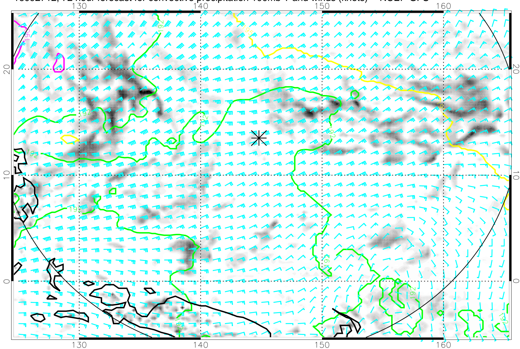
16092712, 72 hour forecast for convective precipitation 100mb T and winds (knots) -- NCEP GFS
