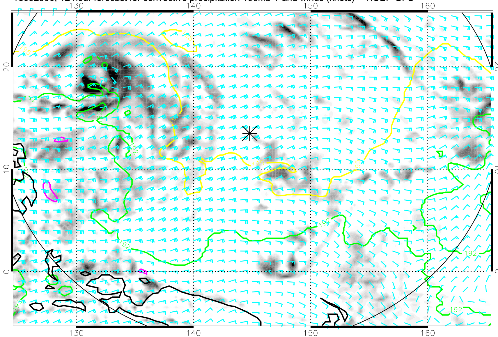
16092500, 12 hour forecast for convective precipitation 100mb T and winds (knots) -- NCEP GFS
