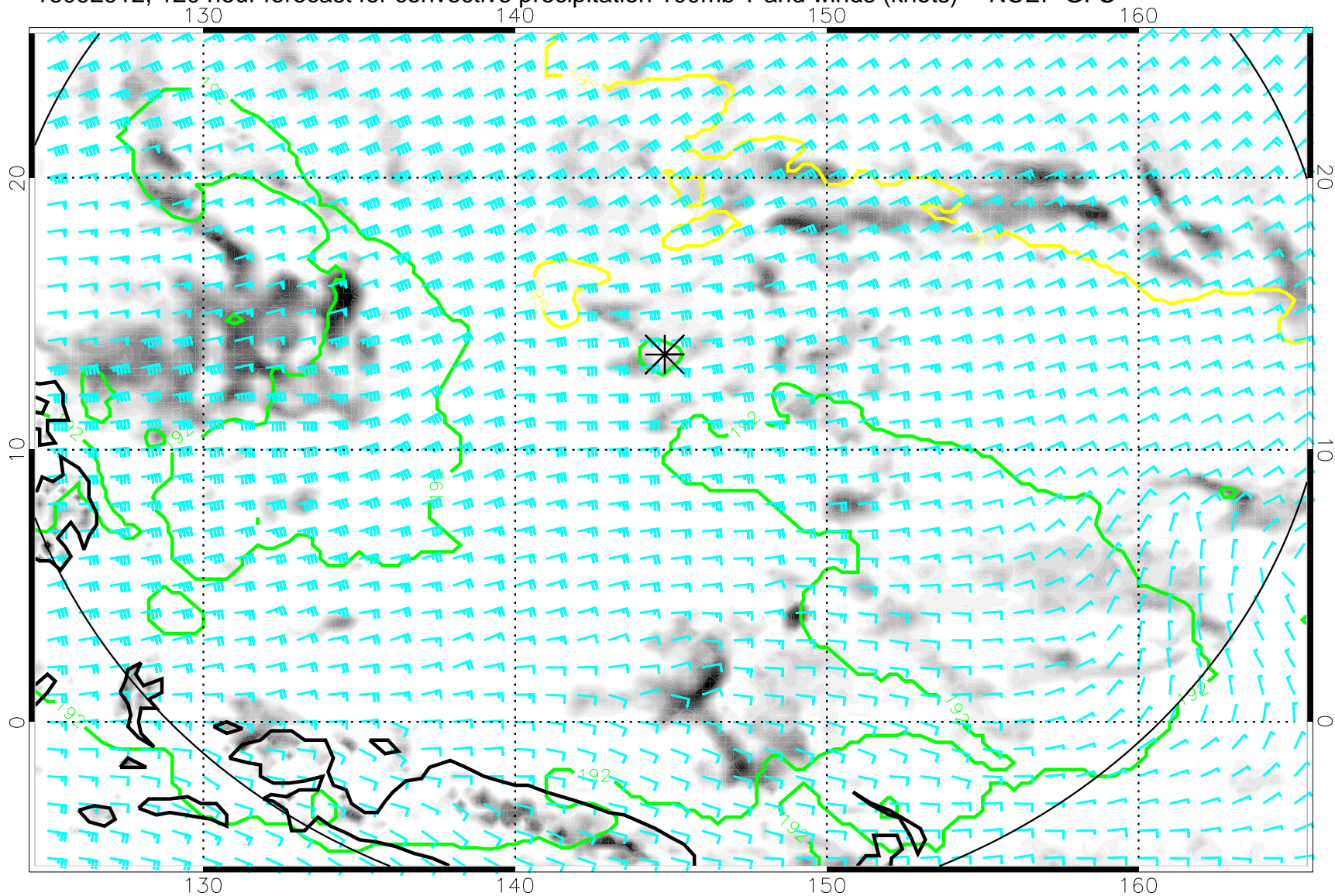
16092912, 120 hour forecast for convective precipitation 100mb T and winds (knots) -- NCEP GFS
