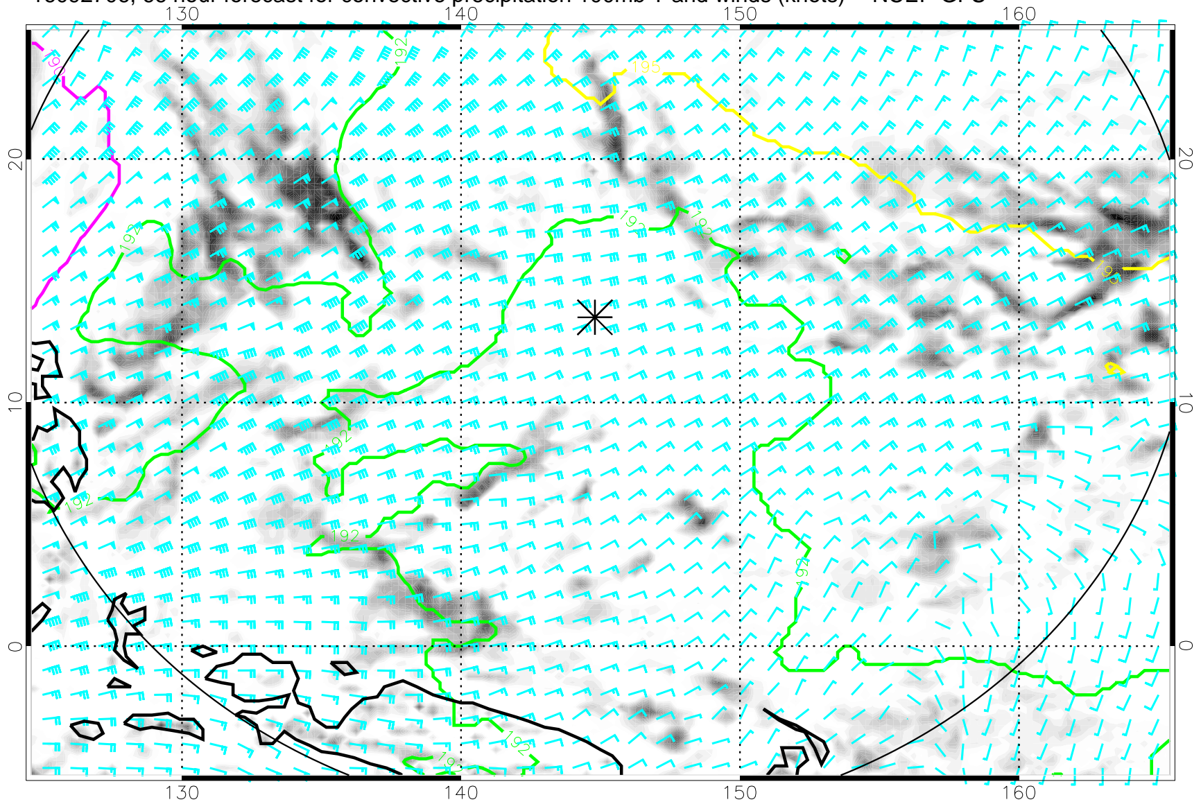
16092706, 66 hour forecast for convective precipitation 100mb T and winds (knots) -- NCEP GFS
