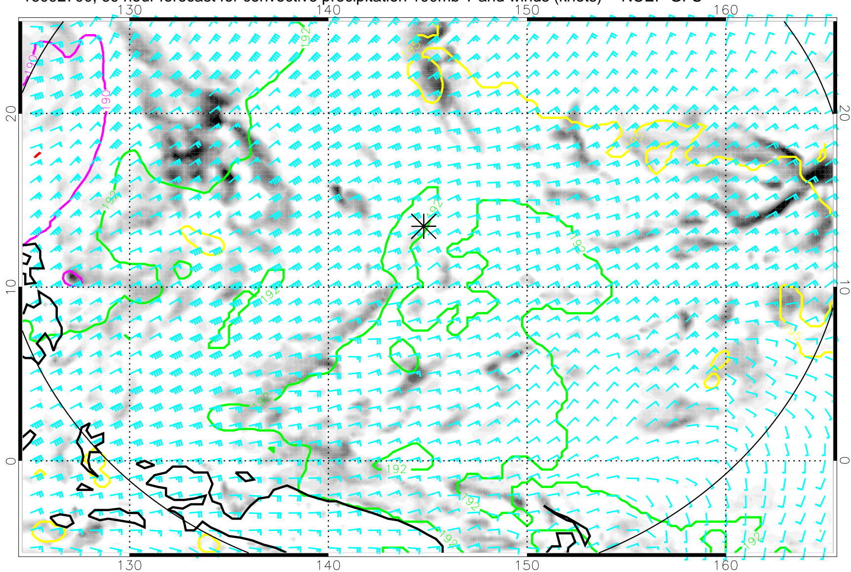
16092700, 60 hour forecast for convective precipitation 100mb T and winds (knots) -- NCEP GFS
