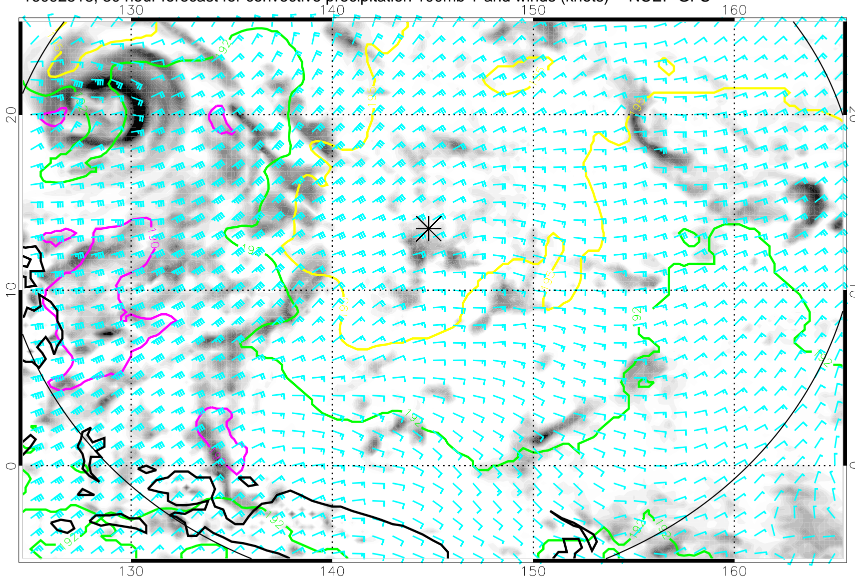
16092518, 30 hour forecast for convective precipitation 100mb T and winds (knots) -- NCEP GFS
