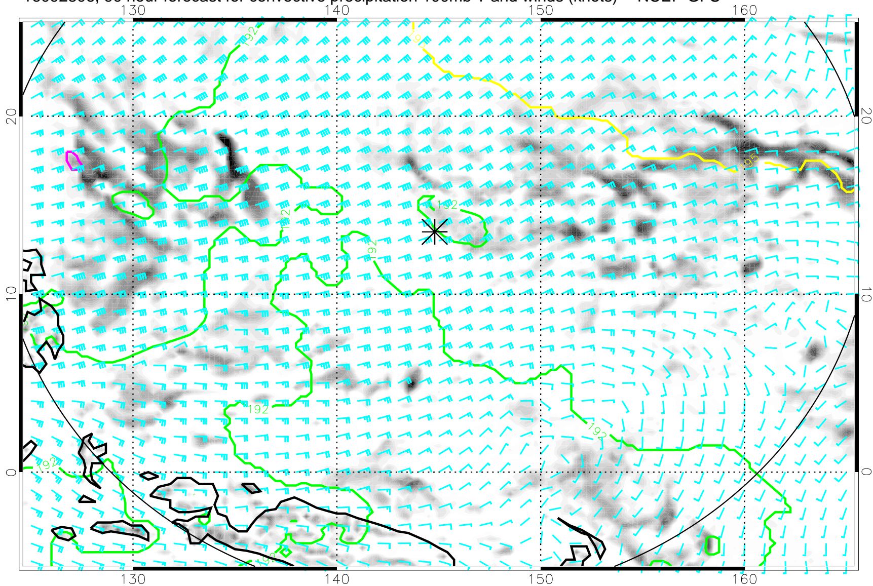
16092806, 90 hour forecast for convective precipitation 100mb T and winds (knots) -- NCEP GFS
