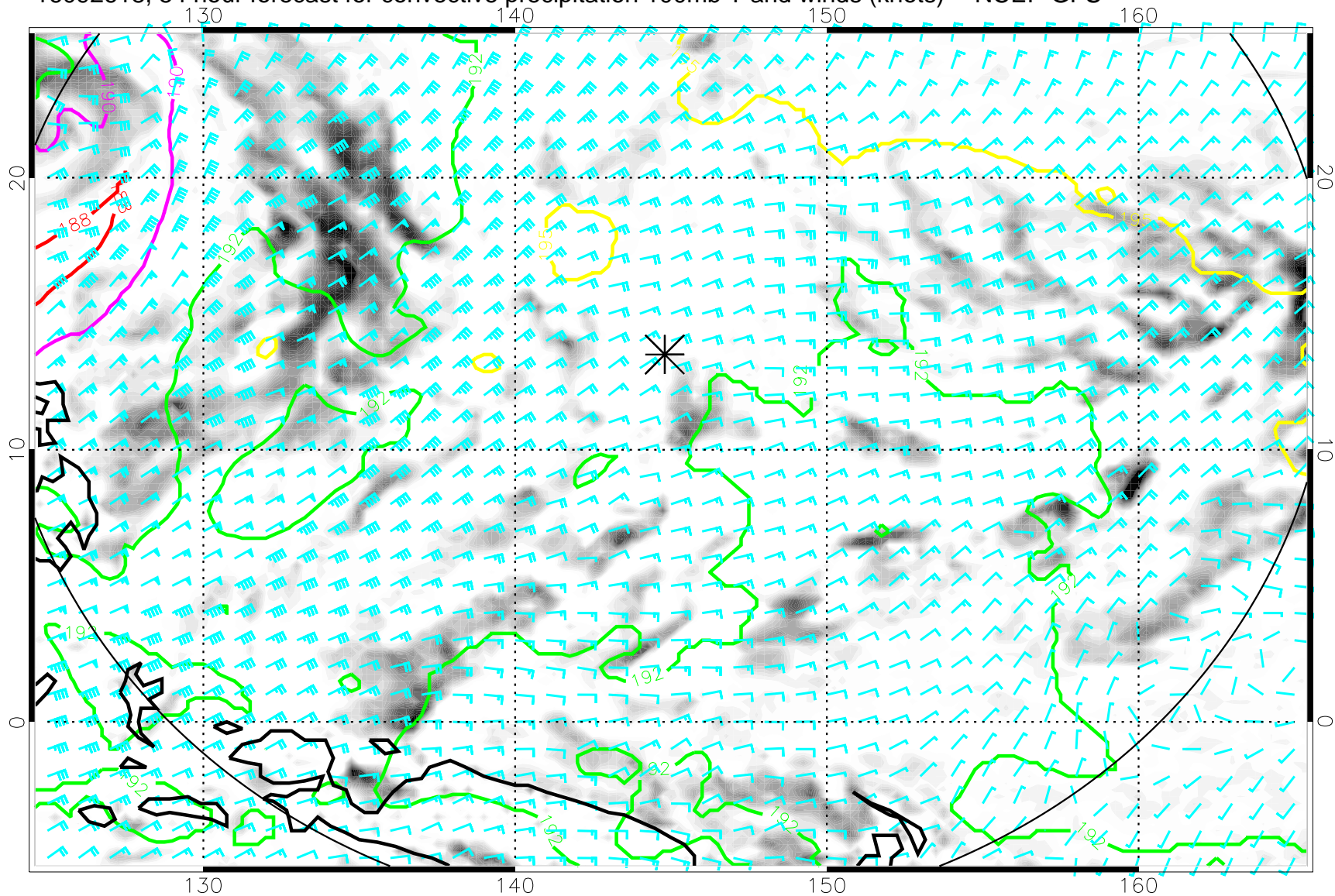
16092618, 54 hour forecast for convective precipitation 100mb T and winds (knots) -- NCEP GFS
