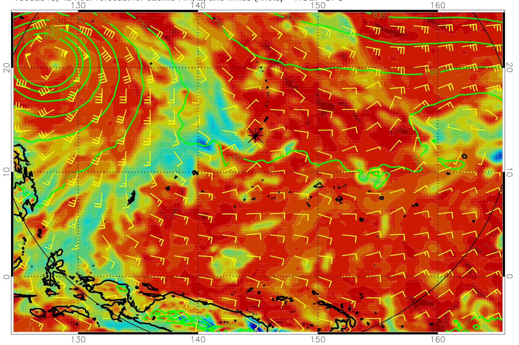
16092518, 42 hour forecast for 925mb RH, Z, and winds (knots) -- NCEP GFS
