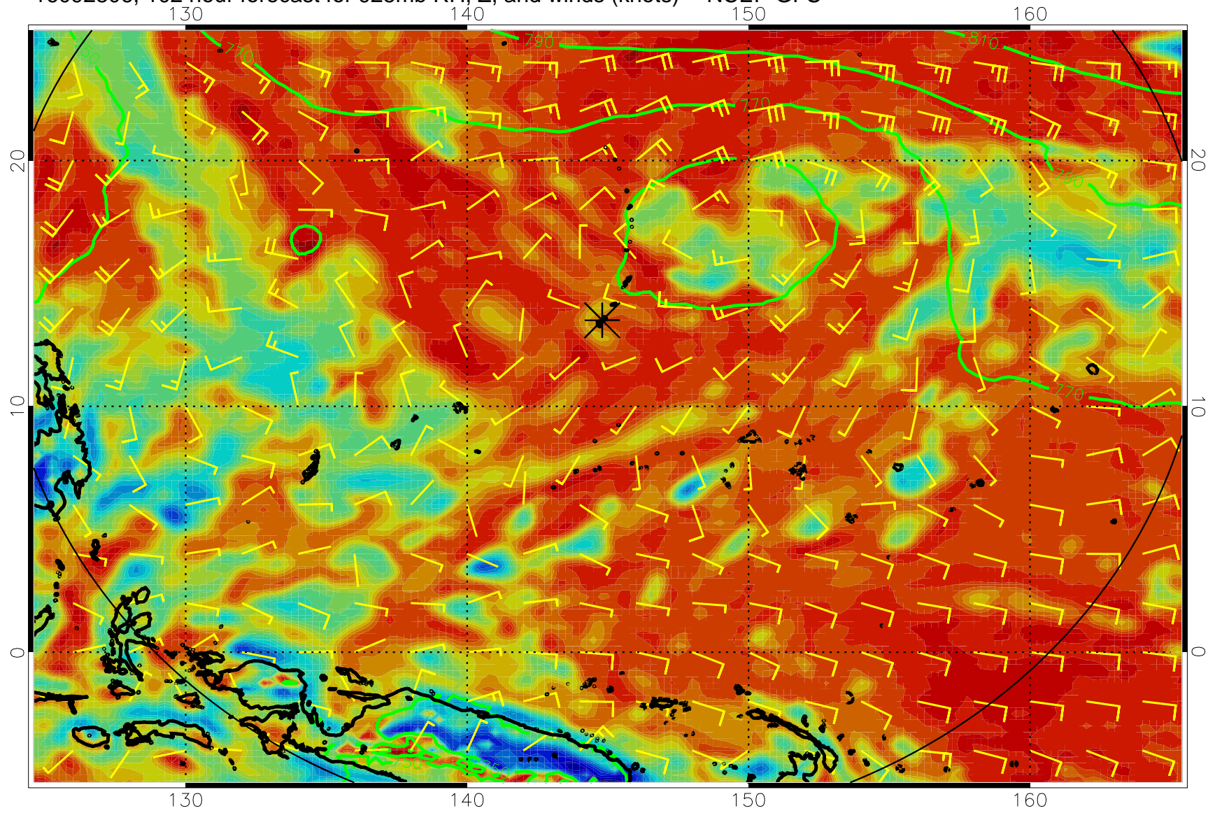
16092806, 102 hour forecast for 925mb RH, Z, and winds (knots) -- NCEP GFS
