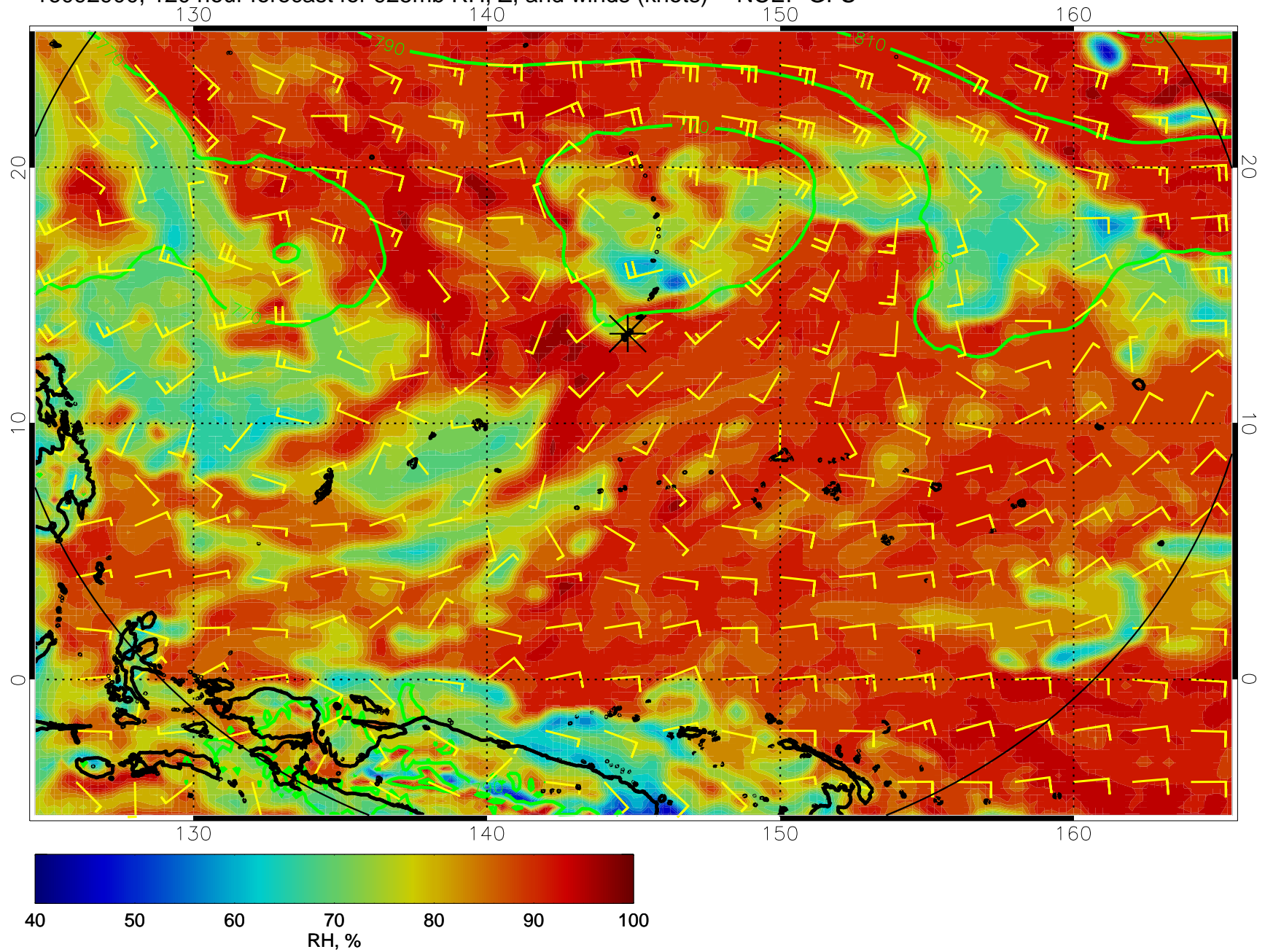
16092900, 120 hour forecast for 925mb RH, Z, and winds (knots) -- NCEP GFS
