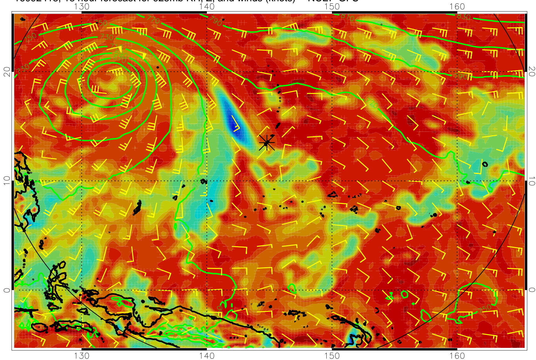
16092418, 18 hour forecast for 925mb RH, Z, and winds (knots) -- NCEP GFS
