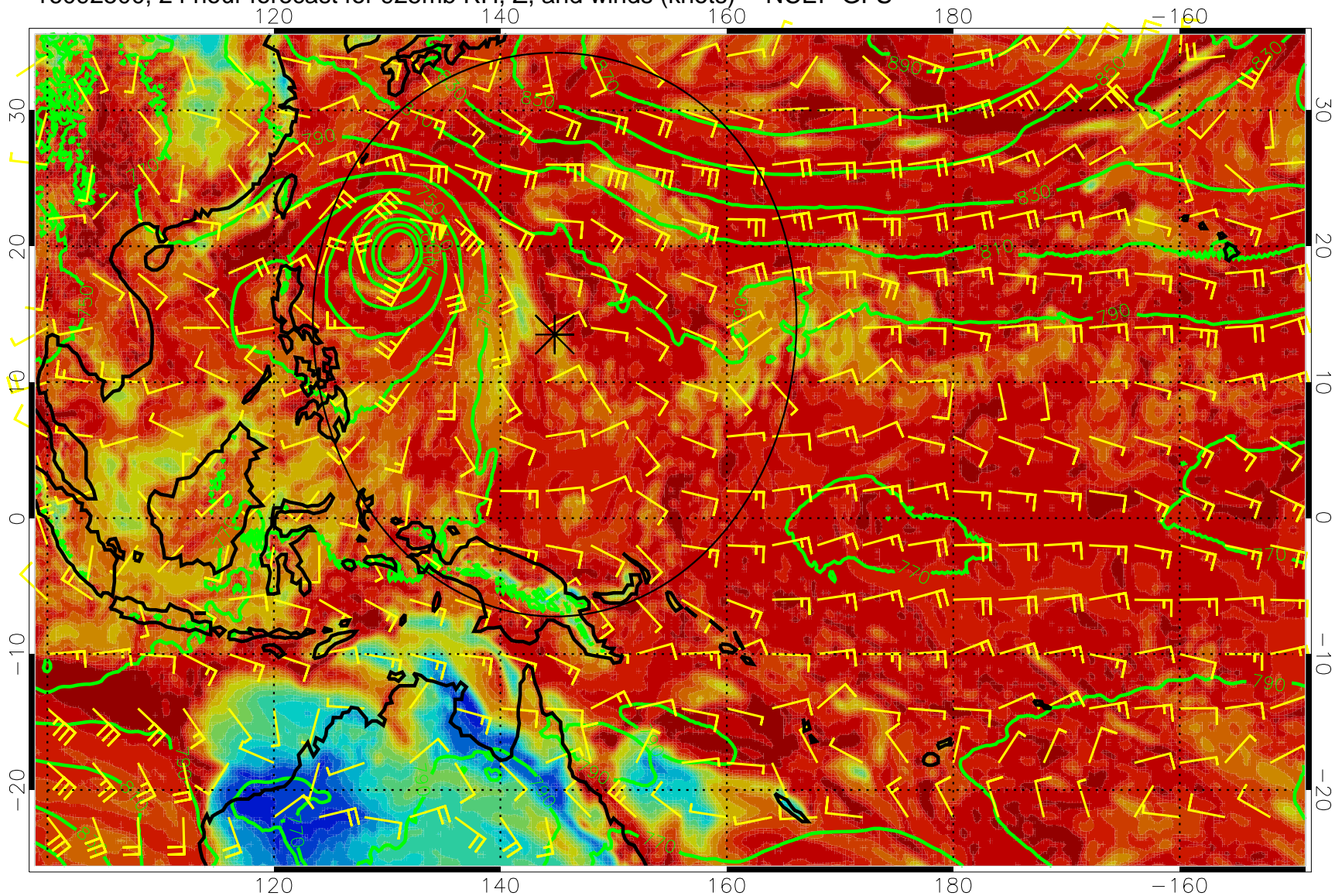
16092500, 24 hour forecast for 925mb RH, Z, and winds (knots) -- NCEP GFS
