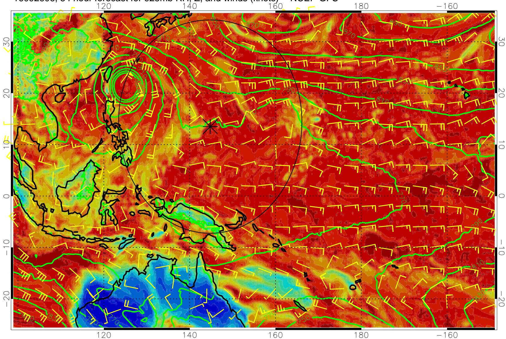
16092606, 54 hour forecast for 925mb RH, Z, and winds (knots) -- NCEP GFS
