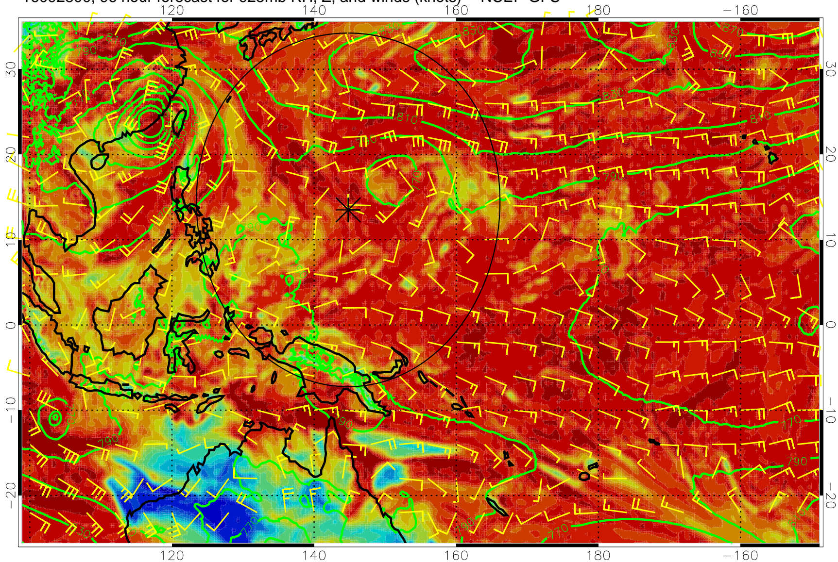
16092800, 96 hour forecast for 925mb RH, Z, and winds (knots) -- NCEP GFS
