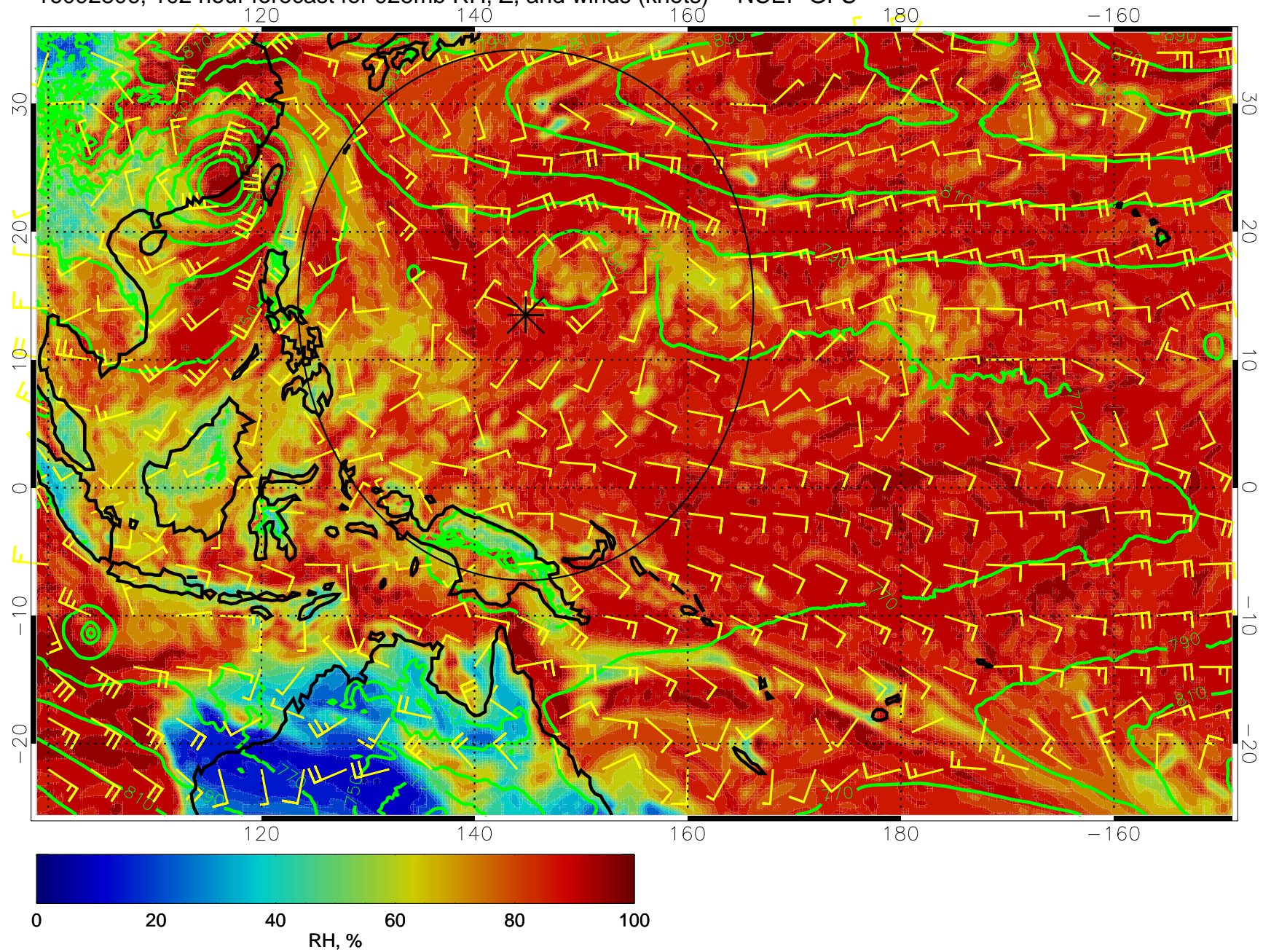
16092806, 102 hour forecast for 925mb RH, Z, and winds (knots) -- NCEP GFS
