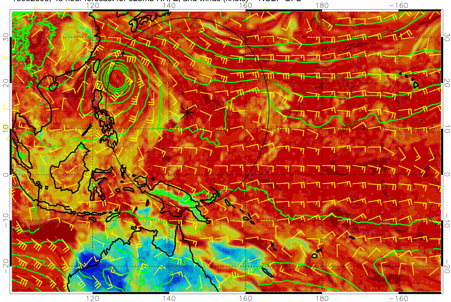
16092600, 48 hour forecast for 925mb RH, Z, and winds (knots) -- NCEP GFS
