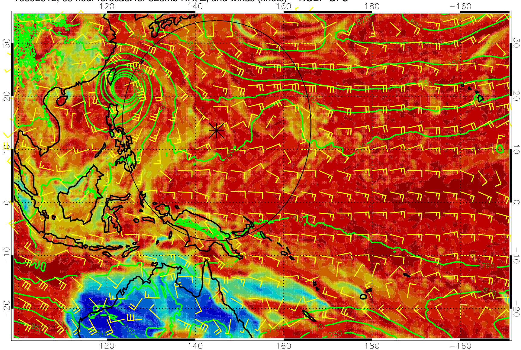
16092612, 60 hour forecast for 925mb RH, Z, and winds (knots) -- NCEP GFS
