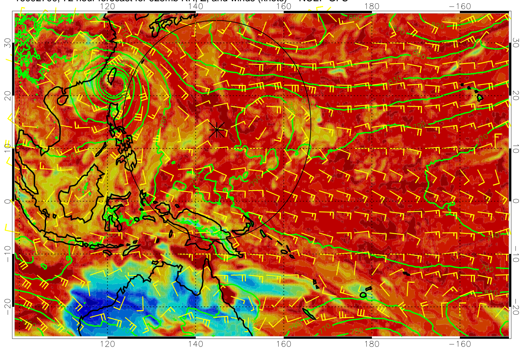
16092700, 72 hour forecast for 925mb RH, Z, and winds (knots) -- NCEP GFS
