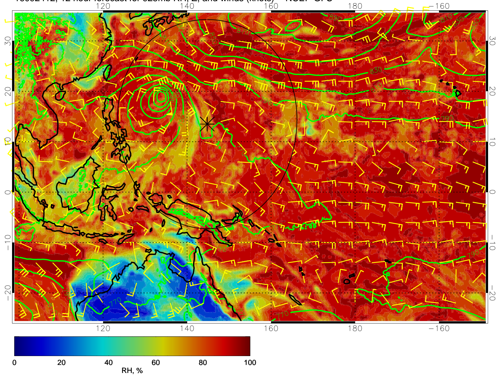
16092412, 12 hour forecast for 925mb RH, Z, and winds (knots) -- NCEP GFS
