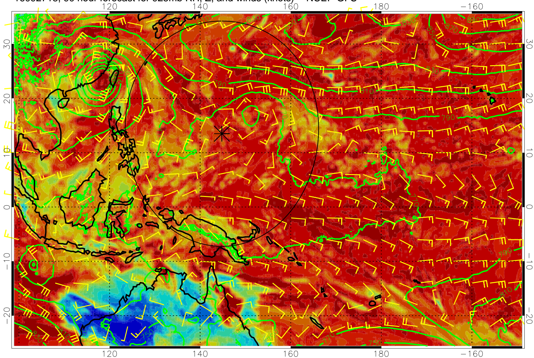
16092718, 90 hour forecast for 925mb RH, Z, and winds (knots) -- NCEP GFS
