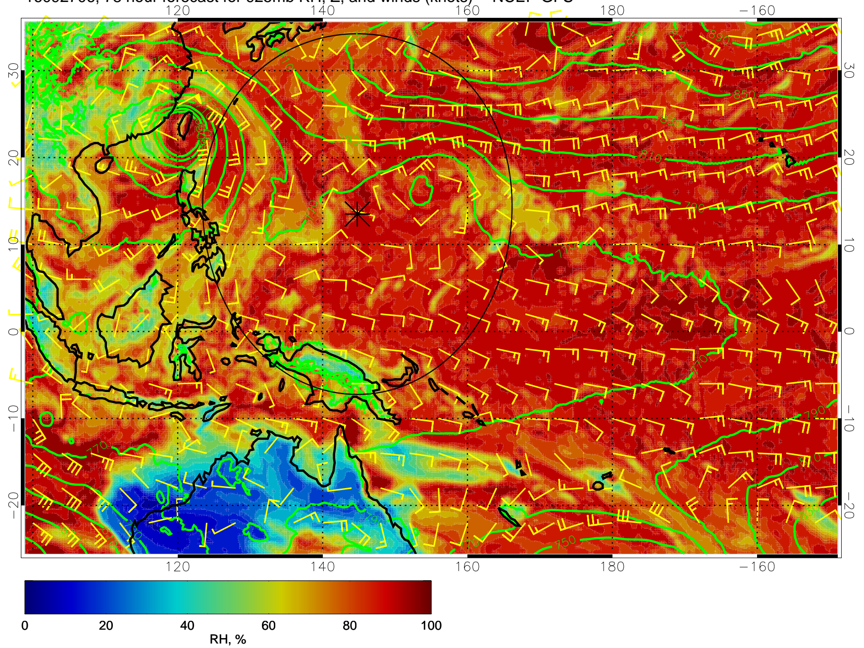
16092706, 78 hour forecast for 925mb RH, Z, and winds (knots) -- NCEP GFS
