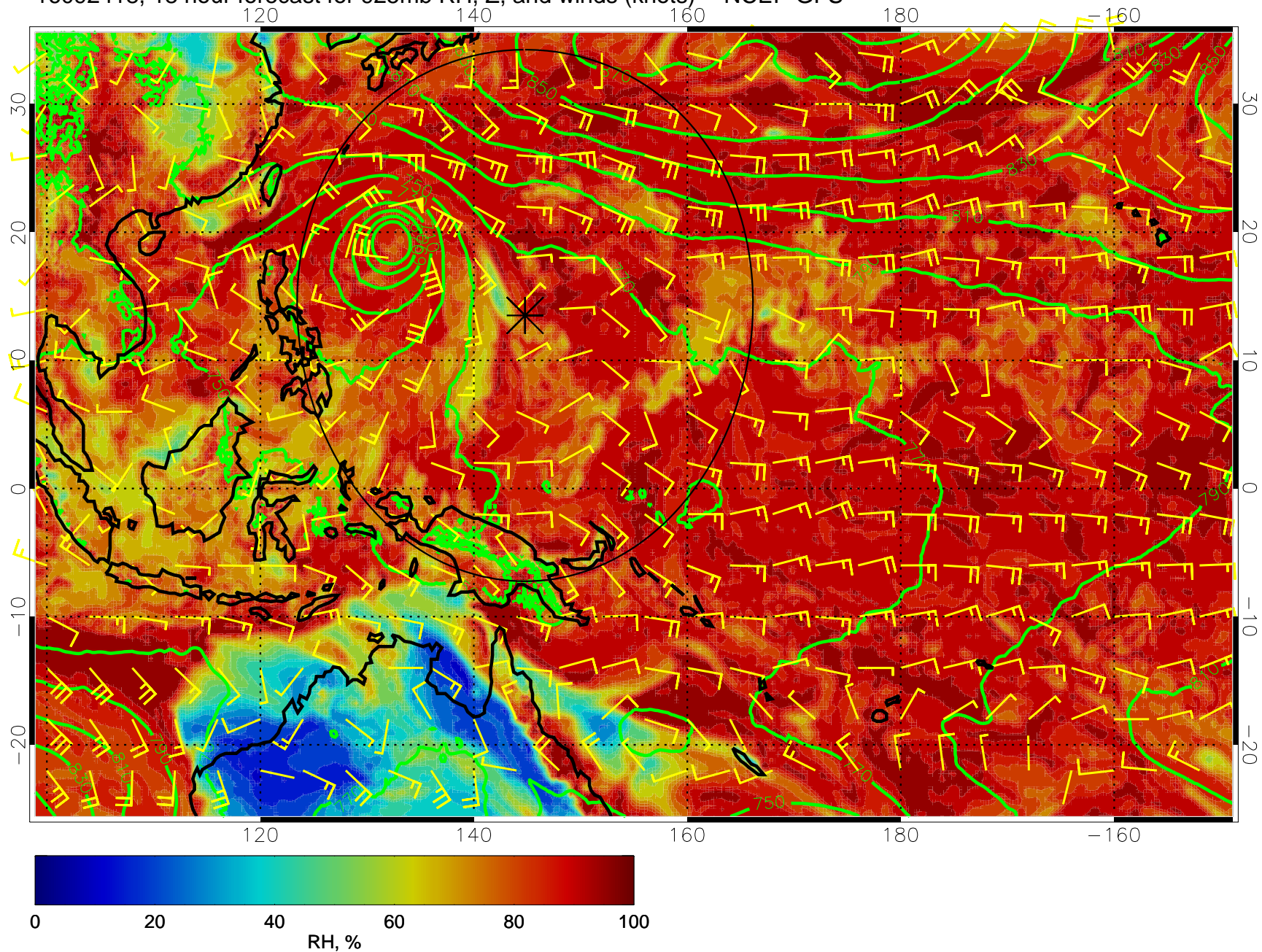
16092418, 18 hour forecast for 925mb RH, Z, and winds (knots) -- NCEP GFS
