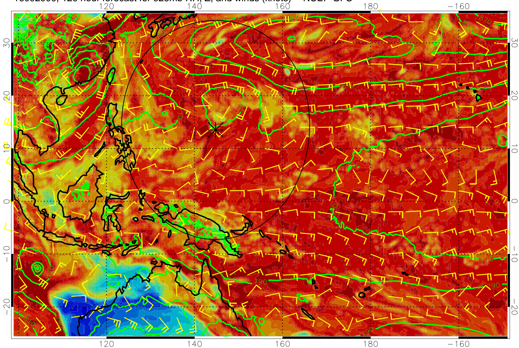
16092900, 120 hour forecast for 925mb RH, Z, and winds (knots) -- NCEP GFS
