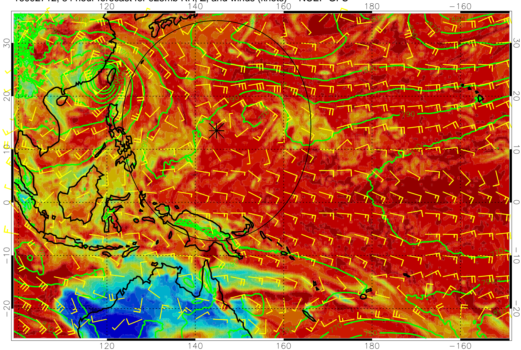
16092712, 84 hour forecast for 925mb RH, Z, and winds (knots) -- NCEP GFS
