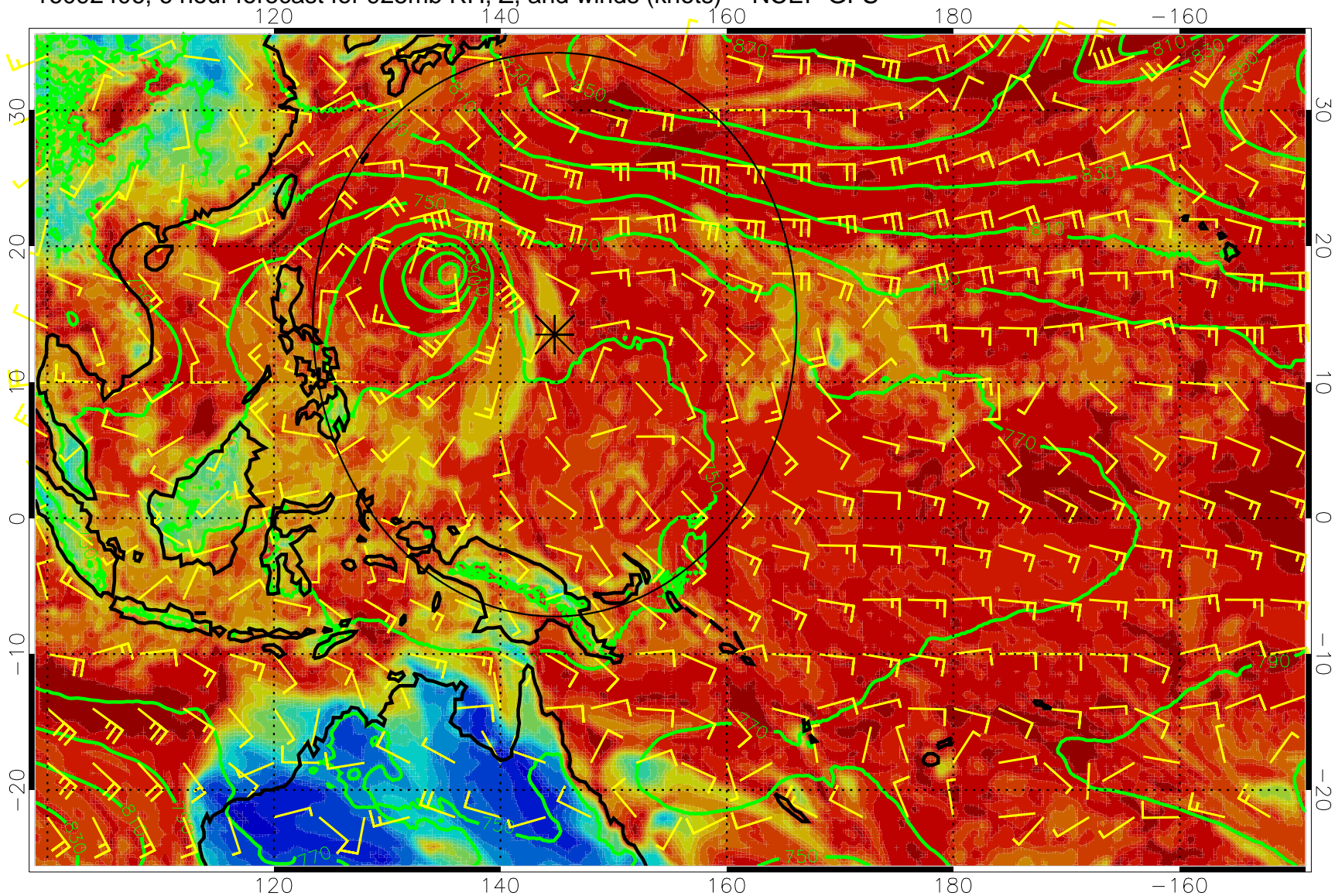
16092406, 6 hour forecast for 925mb RH, Z, and winds (knots) -- NCEP GFS
