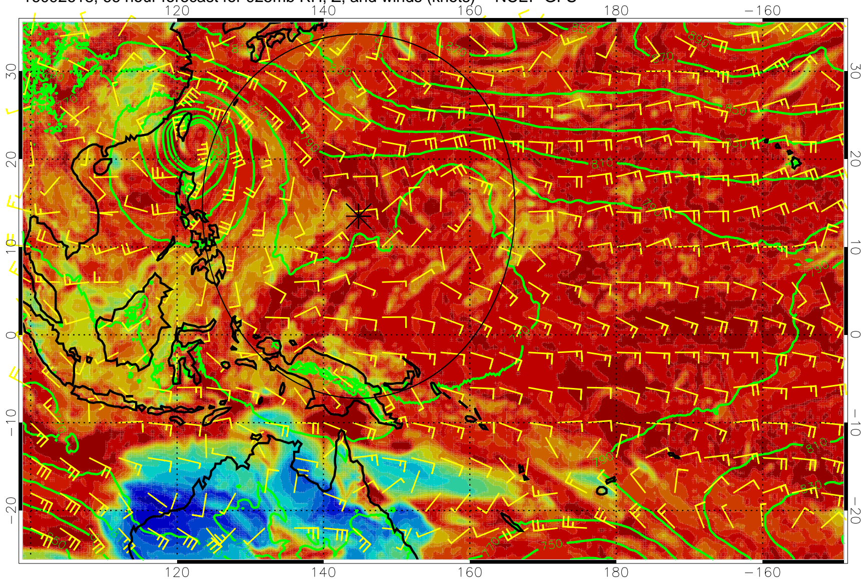
16092618, 66 hour forecast for 925mb RH, Z, and winds (knots) -- NCEP GFS
