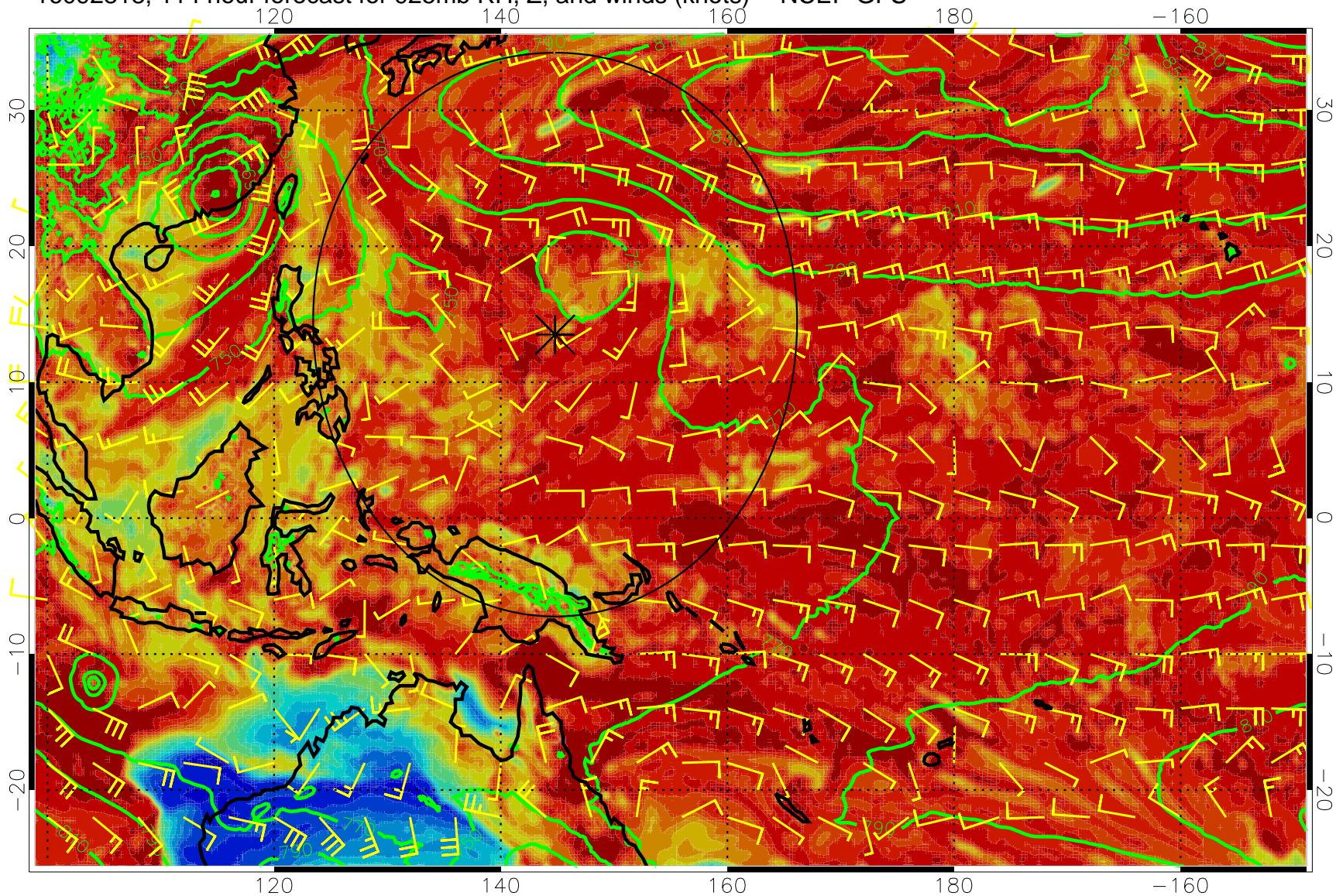
16092818, 114 hour forecast for 925mb RH, Z, and winds (knots) -- NCEP GFS
