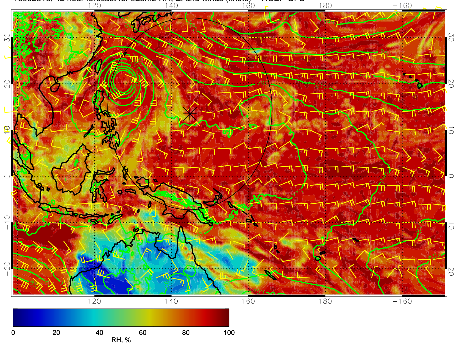
16092518, 42 hour forecast for 925mb RH, Z, and winds (knots) -- NCEP GFS
