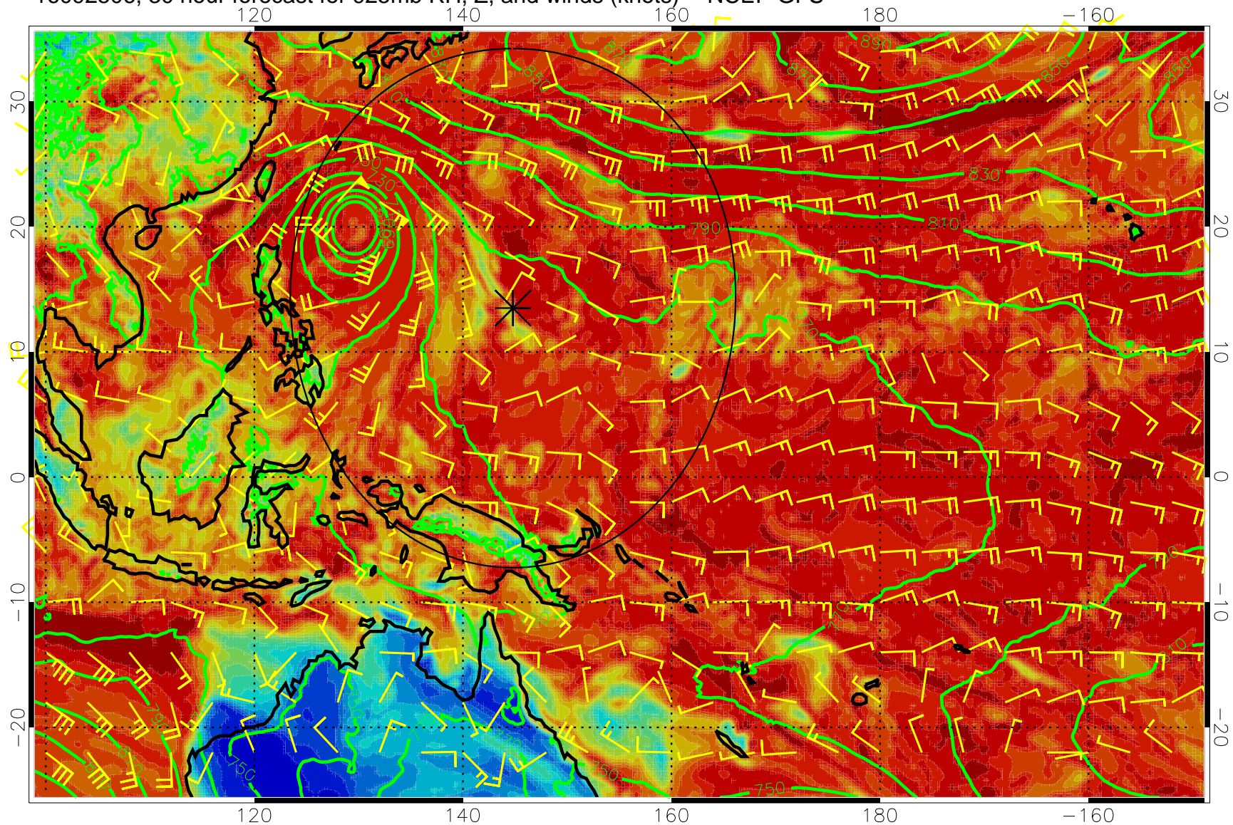
16092506, 30 hour forecast for 925mb RH, Z, and winds (knots) -- NCEP GFS
