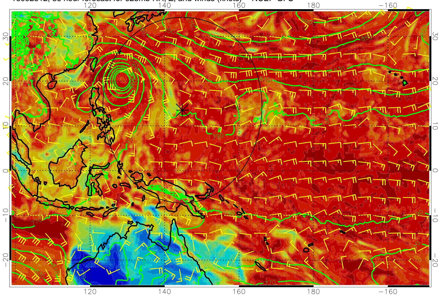
16092512, 36 hour forecast for 925mb RH, Z, and winds (knots) -- NCEP GFS
