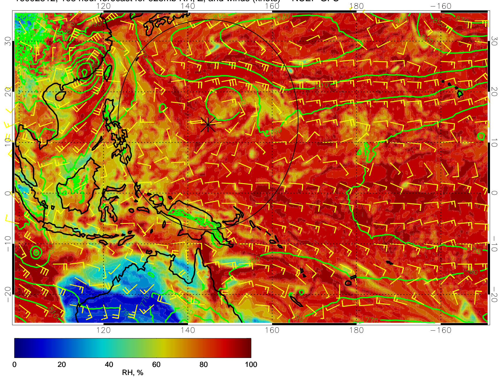
16092812, 108 hour forecast for 925mb RH, Z, and winds (knots) -- NCEP GFS
