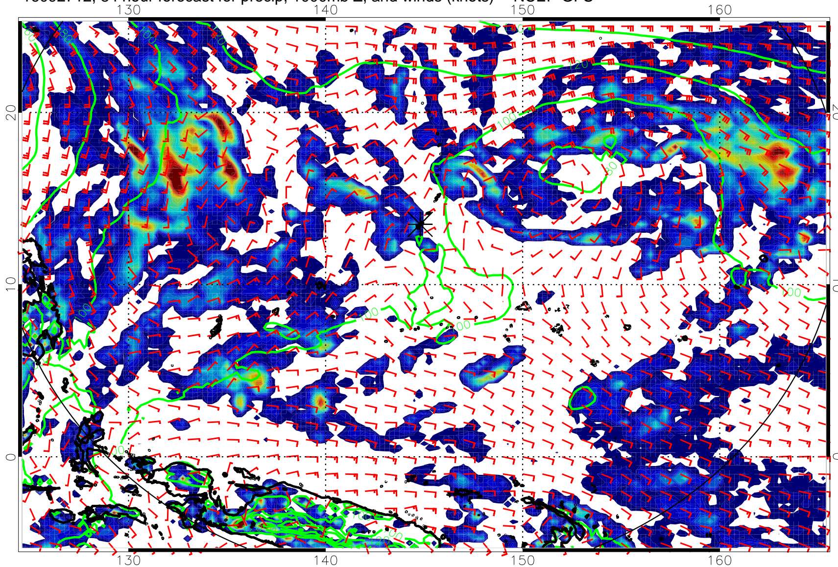
16092712, 84 hour forecast for precip, 1000mb Z, and winds (knots) -- NCEP GFS
