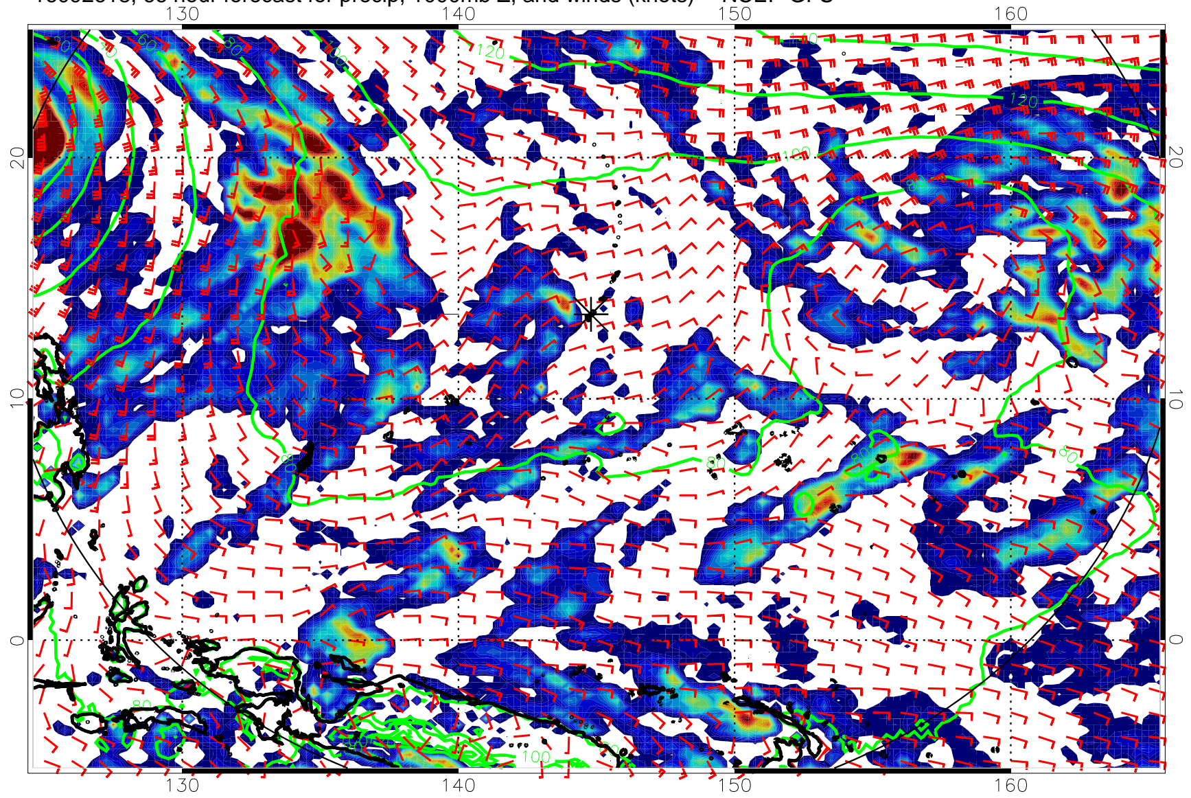
16092618, 66 hour forecast for precip, 1000mb Z, and winds (knots) -- NCEP GFS
