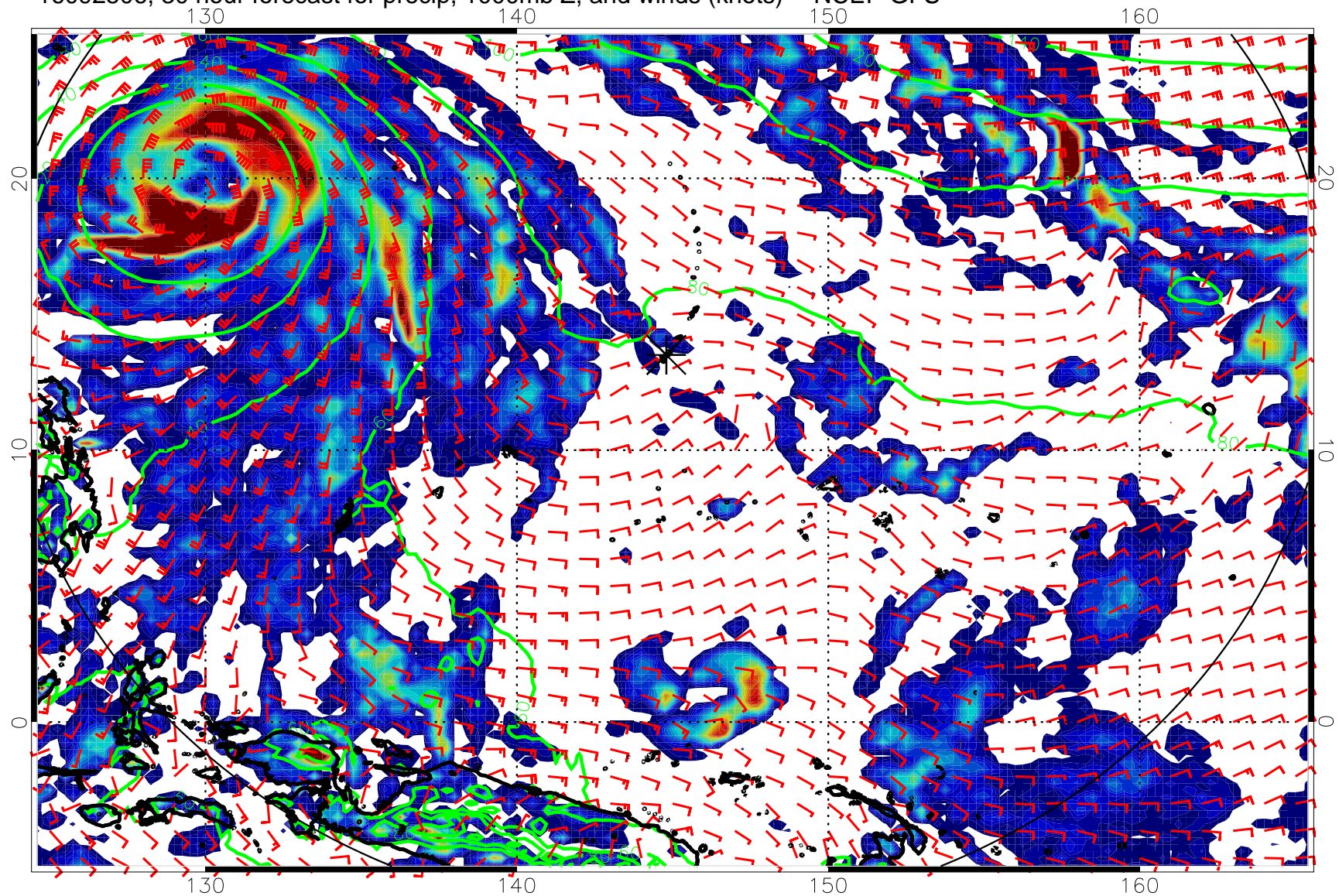
16092506, 30 hour forecast for precip, 1000mb Z, and winds (knots) -- NCEP GFS
