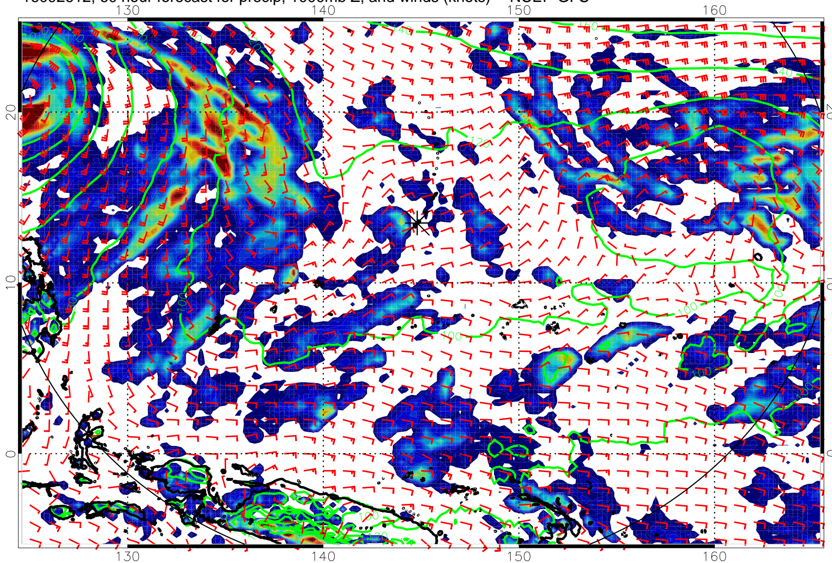
16092612, 60 hour forecast for precip, 1000mb Z, and winds (knots) -- NCEP GFS
