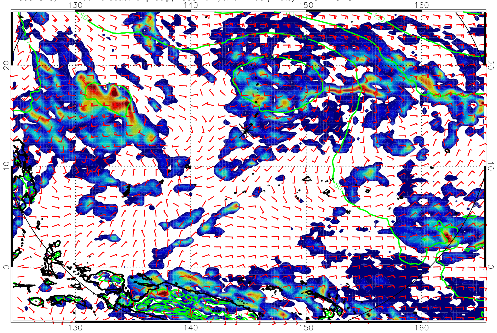
16092818, 114 hour forecast for precip, 1000mb Z, and winds (knots) -- NCEP GFS
