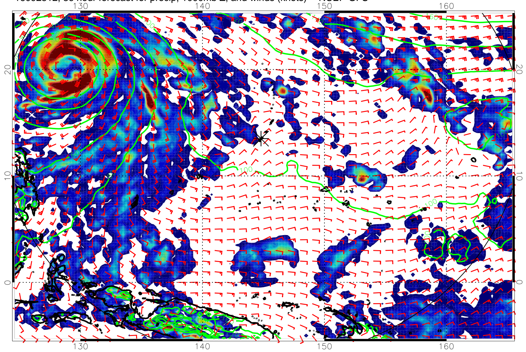
16092512, 36 hour forecast for precip, 1000mb Z, and winds (knots) -- NCEP GFS
