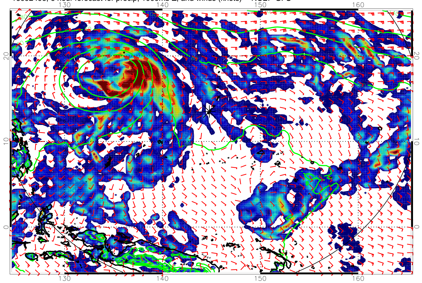
16092406, 6 hour forecast for precip, 1000mb Z, and winds (knots) -- NCEP GFS
