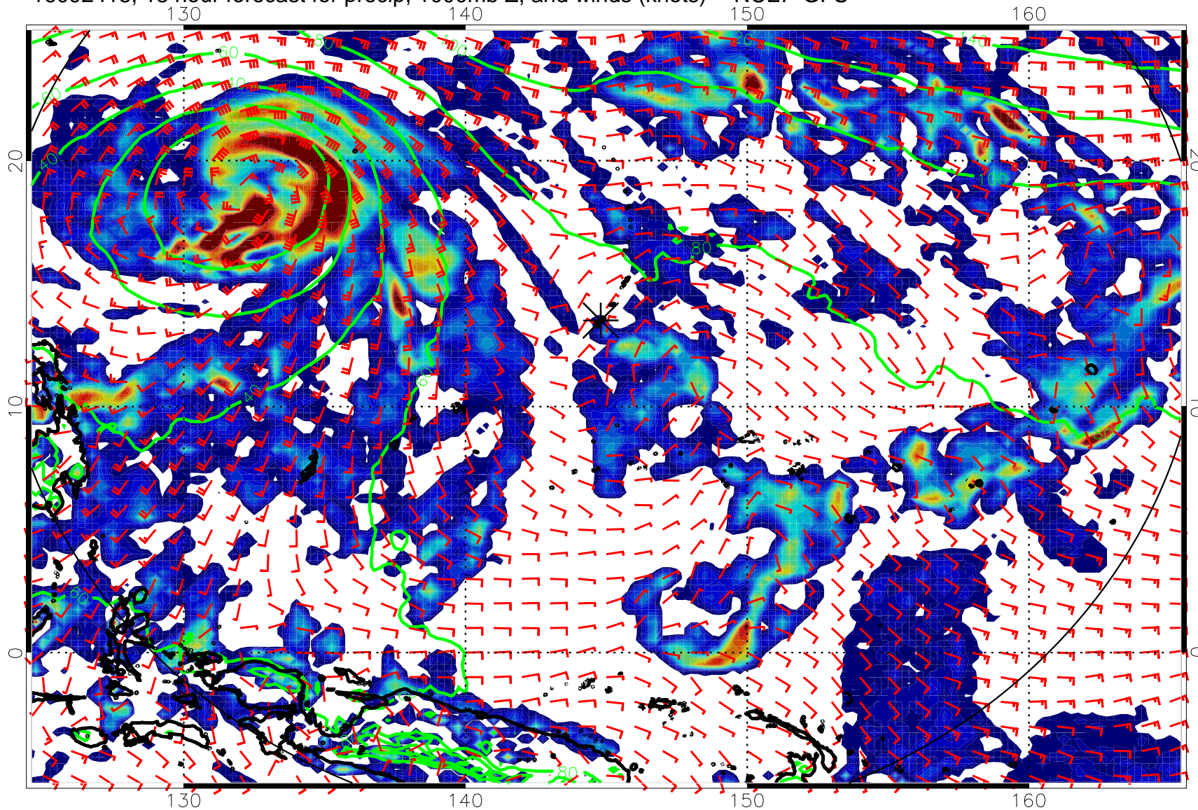
16092418, 18 hour forecast for precip, 1000mb Z, and winds (knots) -- NCEP GFS
