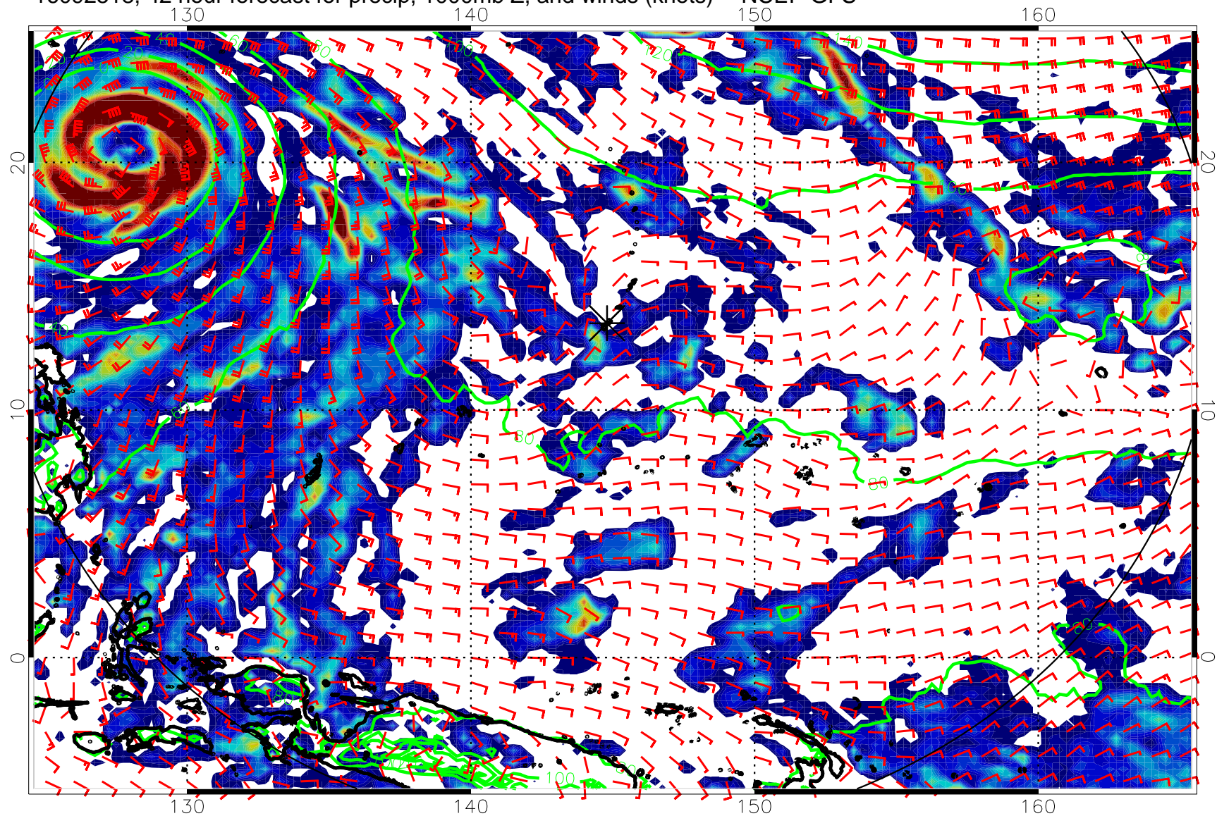
16092518, 42 hour forecast for precip, 1000mb Z, and winds (knots) -- NCEP GFS
