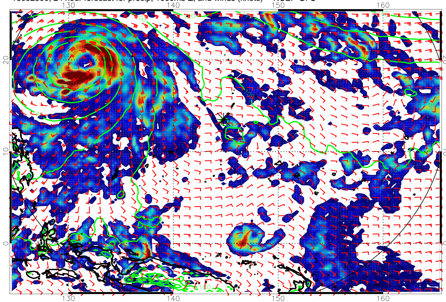
16092500, 24 hour forecast for precip, 1000mb Z, and winds (knots) -- NCEP GFS
