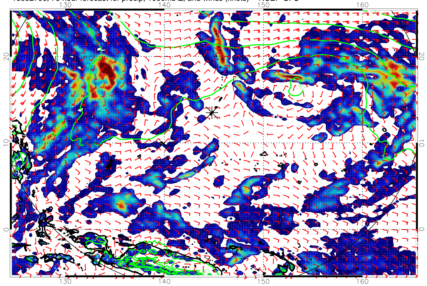
16092706, 78 hour forecast for precip, 1000mb Z, and winds (knots) -- NCEP GFS
