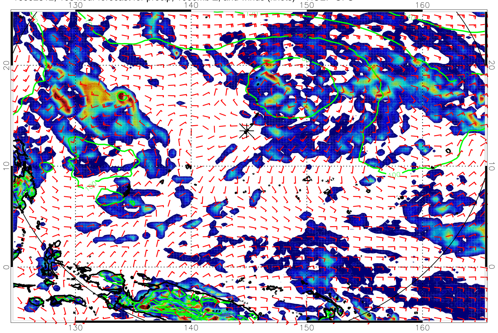
16092812, 108 hour forecast for precip, 1000mb Z, and winds (knots) -- NCEP GFS
