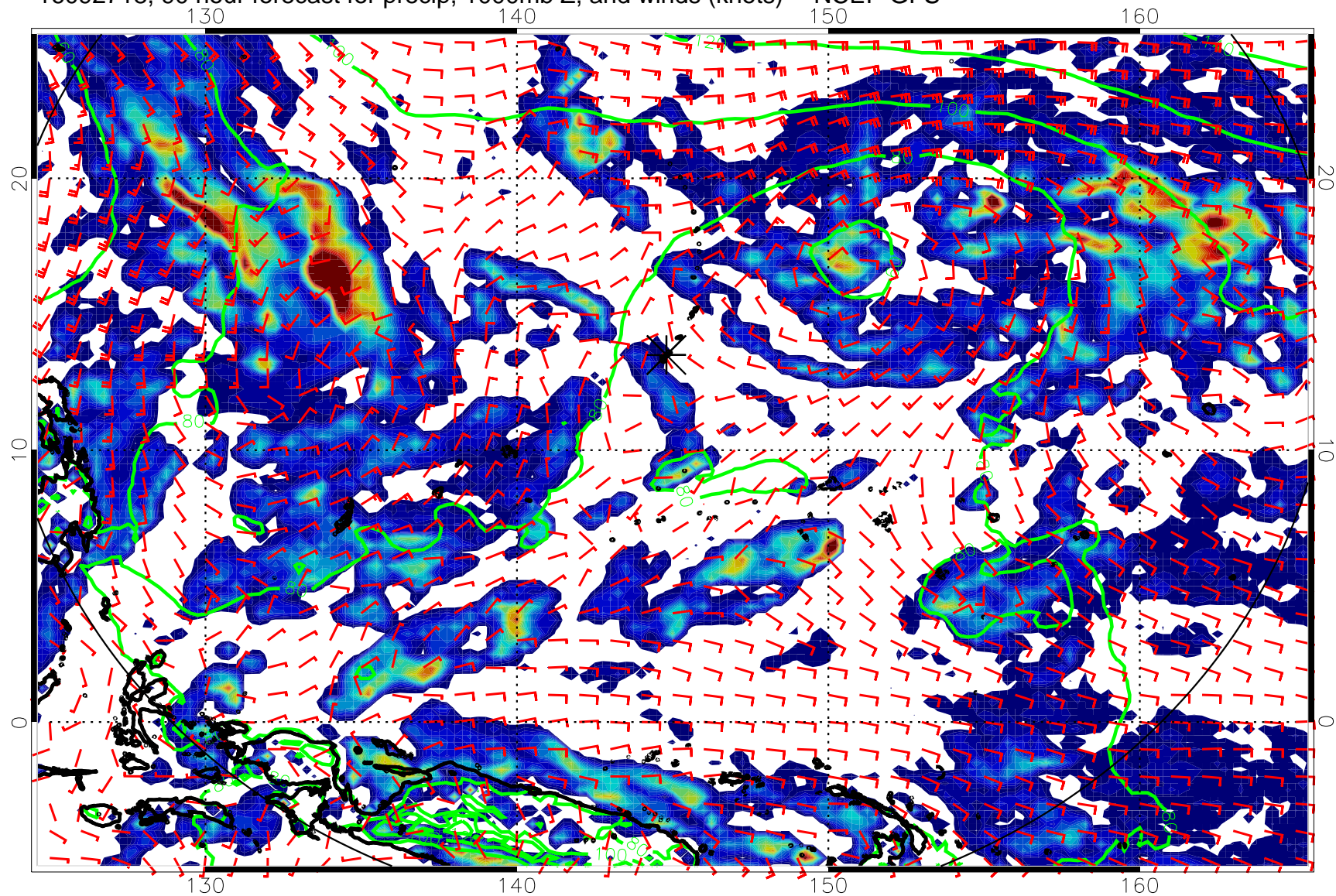
16092718, 90 hour forecast for precip, 1000mb Z, and winds (knots) -- NCEP GFS
