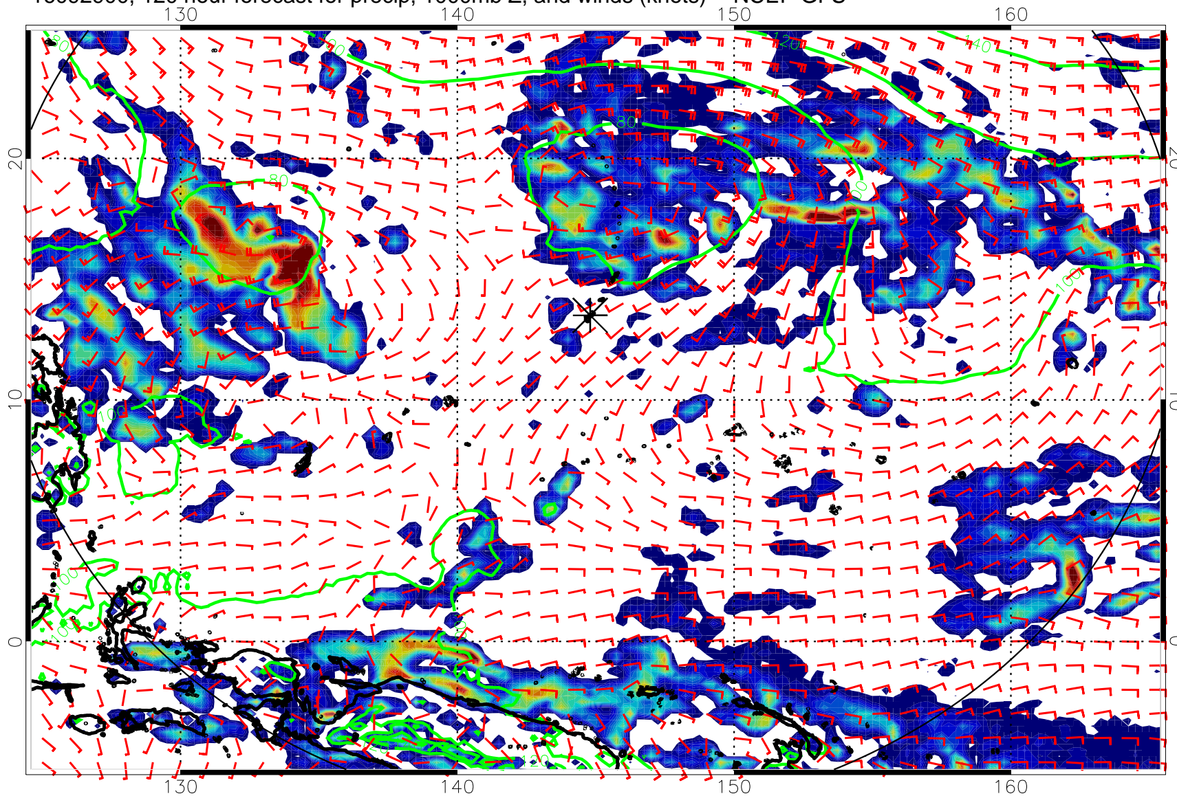
16092900, 120 hour forecast for precip, 1000mb Z, and winds (knots) -- NCEP GFS
