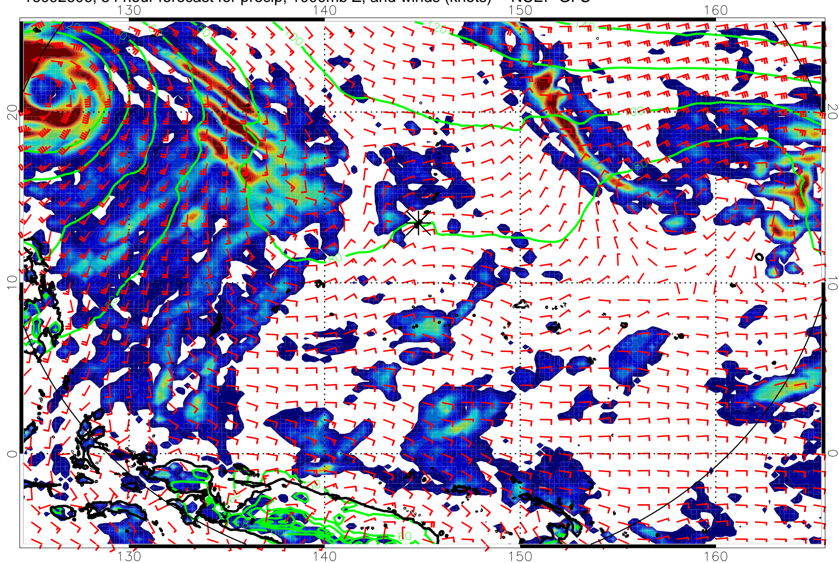
16092606, 54 hour forecast for precip, 1000mb Z, and winds (knots) -- NCEP GFS
