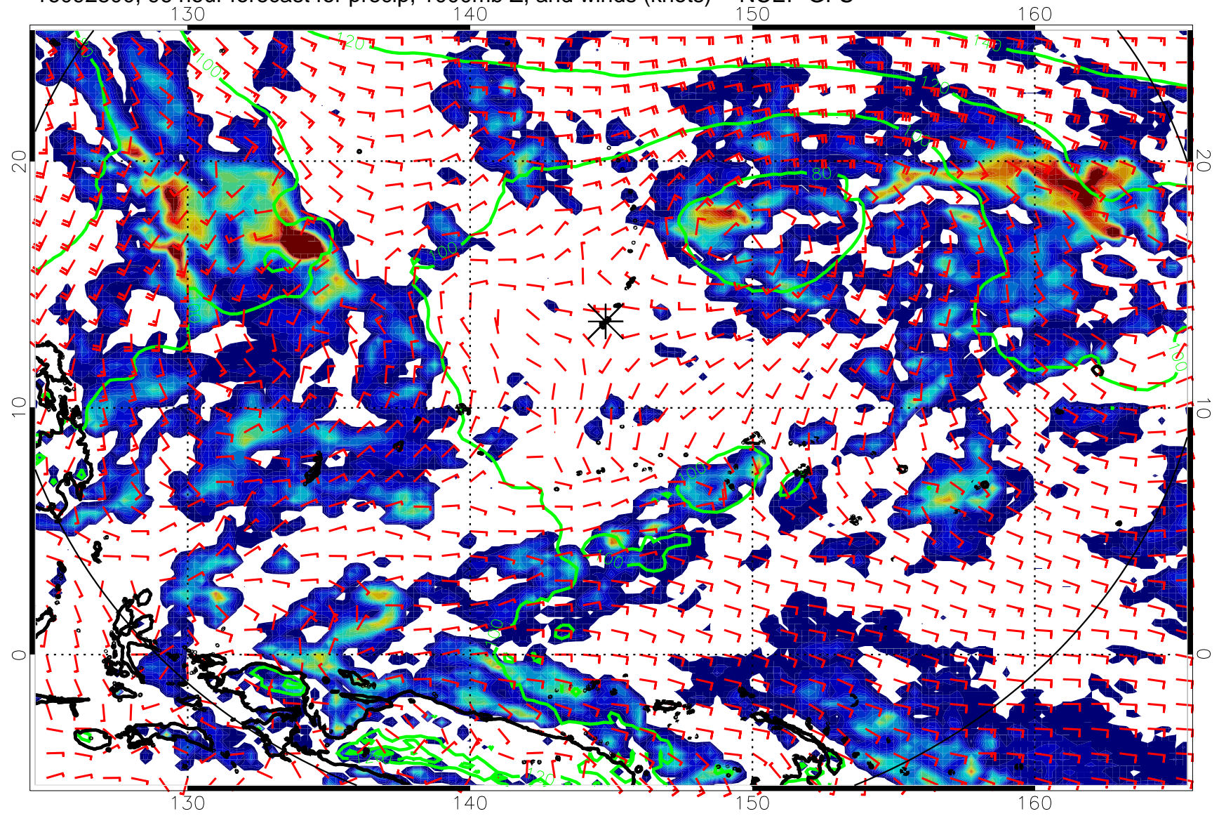
16092800, 96 hour forecast for precip, 1000mb Z, and winds (knots) -- NCEP GFS
