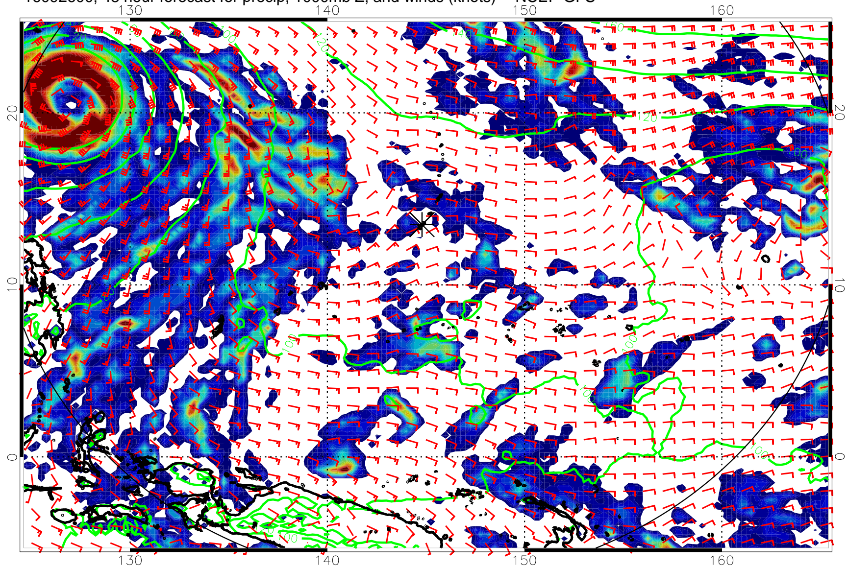
16092600, 48 hour forecast for precip, 1000mb Z, and winds (knots) -- NCEP GFS
