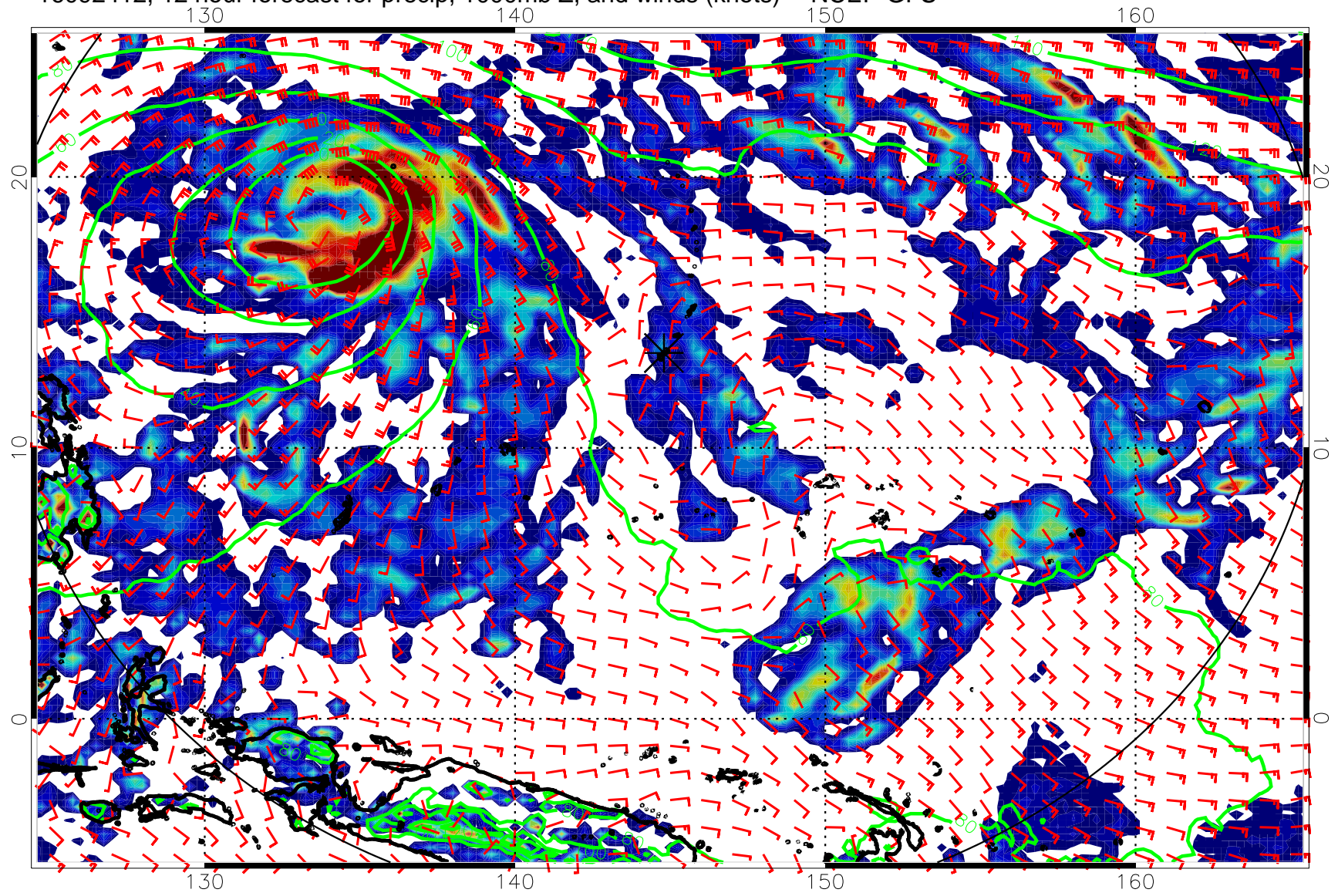
16092412, 12 hour forecast for precip, 1000mb Z, and winds (knots) -- NCEP GFS
