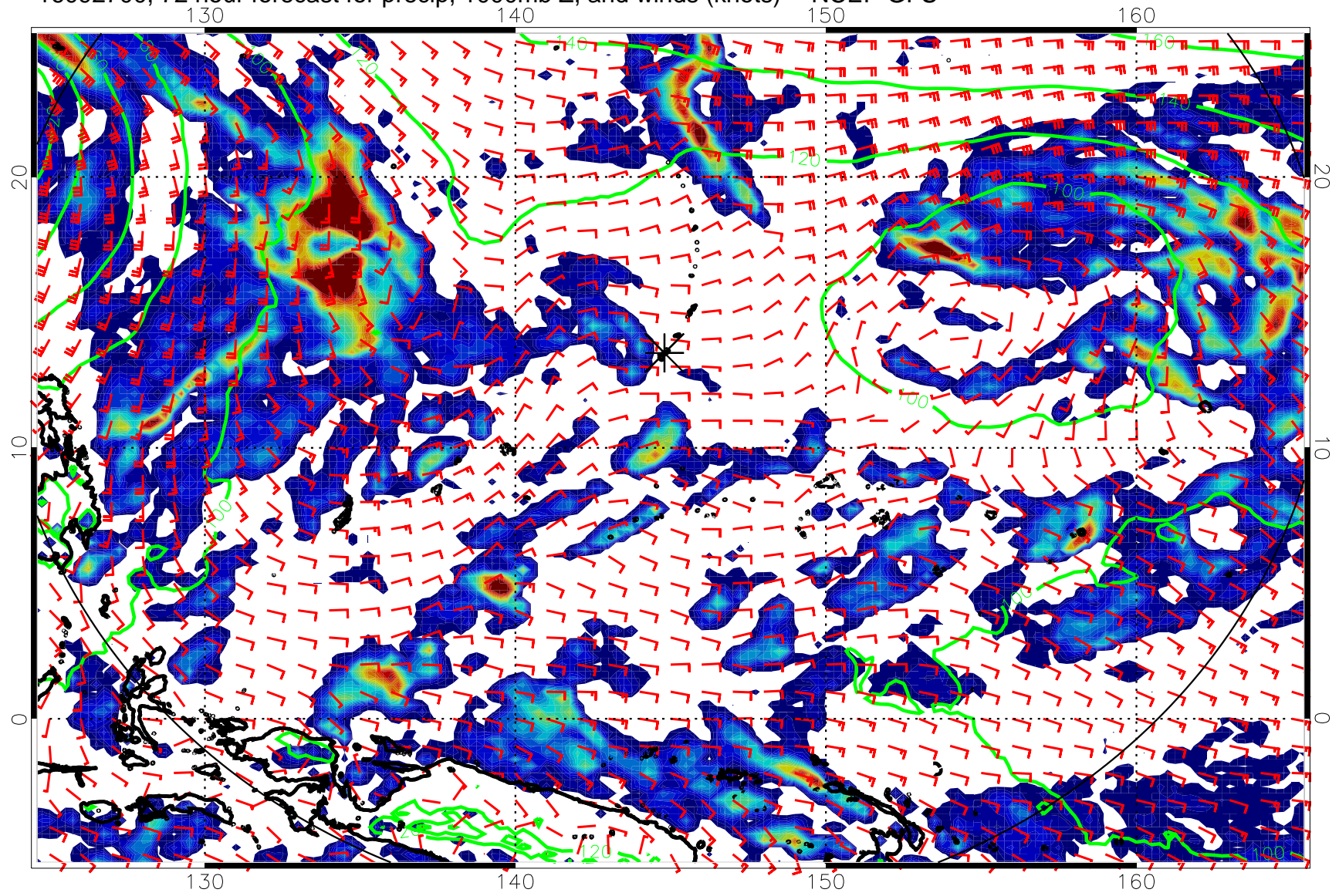
16092700, 72 hour forecast for precip, 1000mb Z, and winds (knots) -- NCEP GFS
