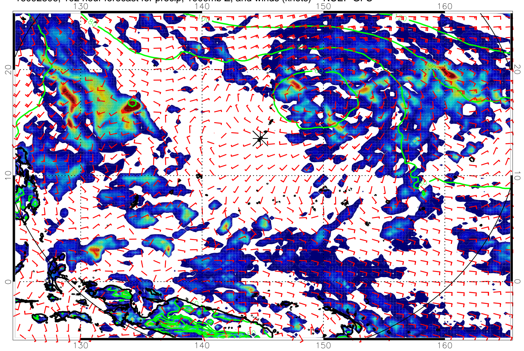
16092806, 102 hour forecast for precip, 1000mb Z, and winds (knots) -- NCEP GFS
