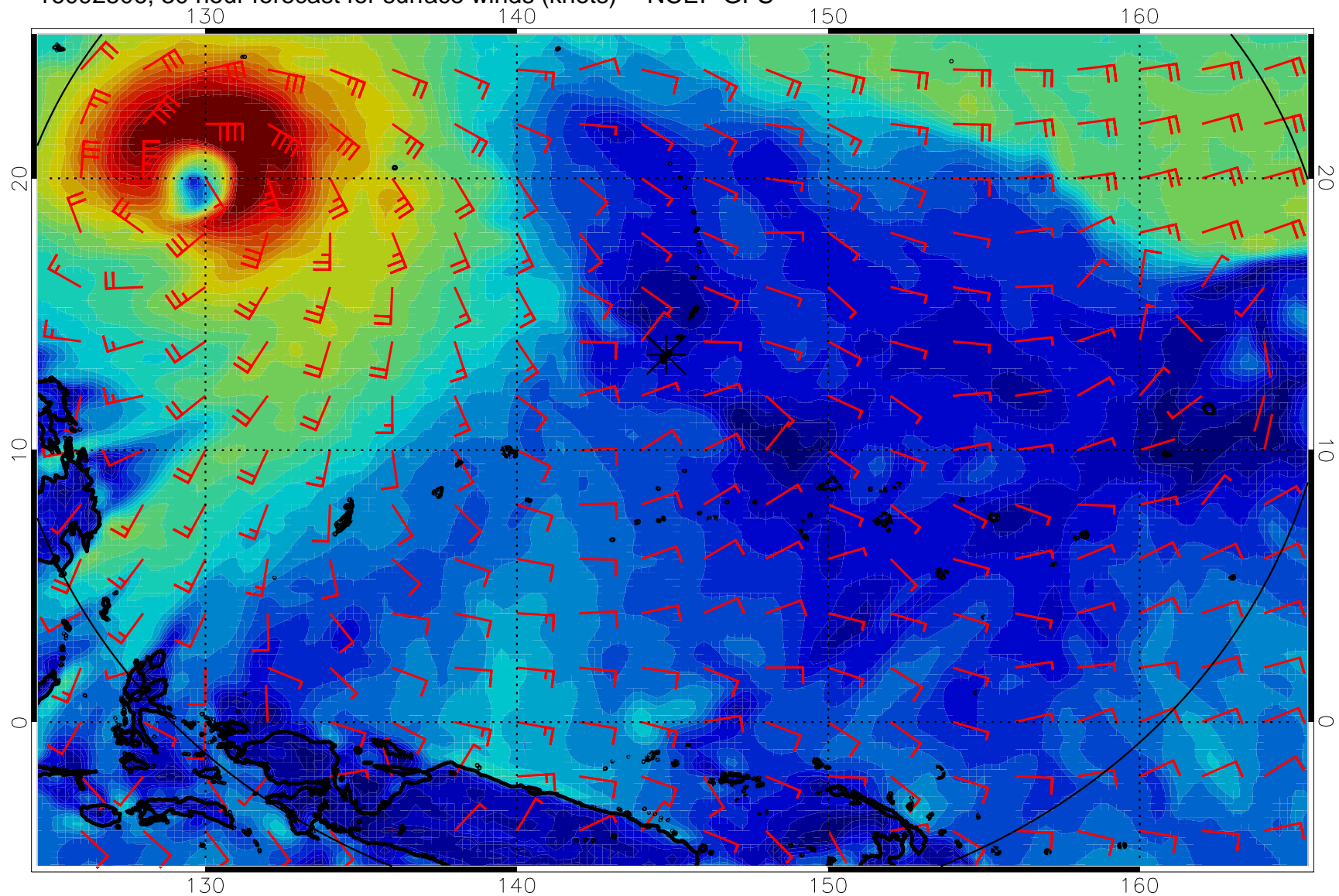
16092506, 30 hour forecast for surface winds (knots) -- NCEP GFS
