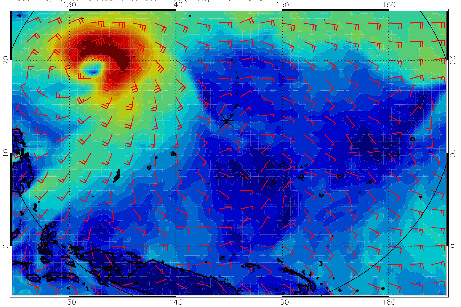
16092418, 18 hour forecast for surface winds (knots) -- NCEP GFS
