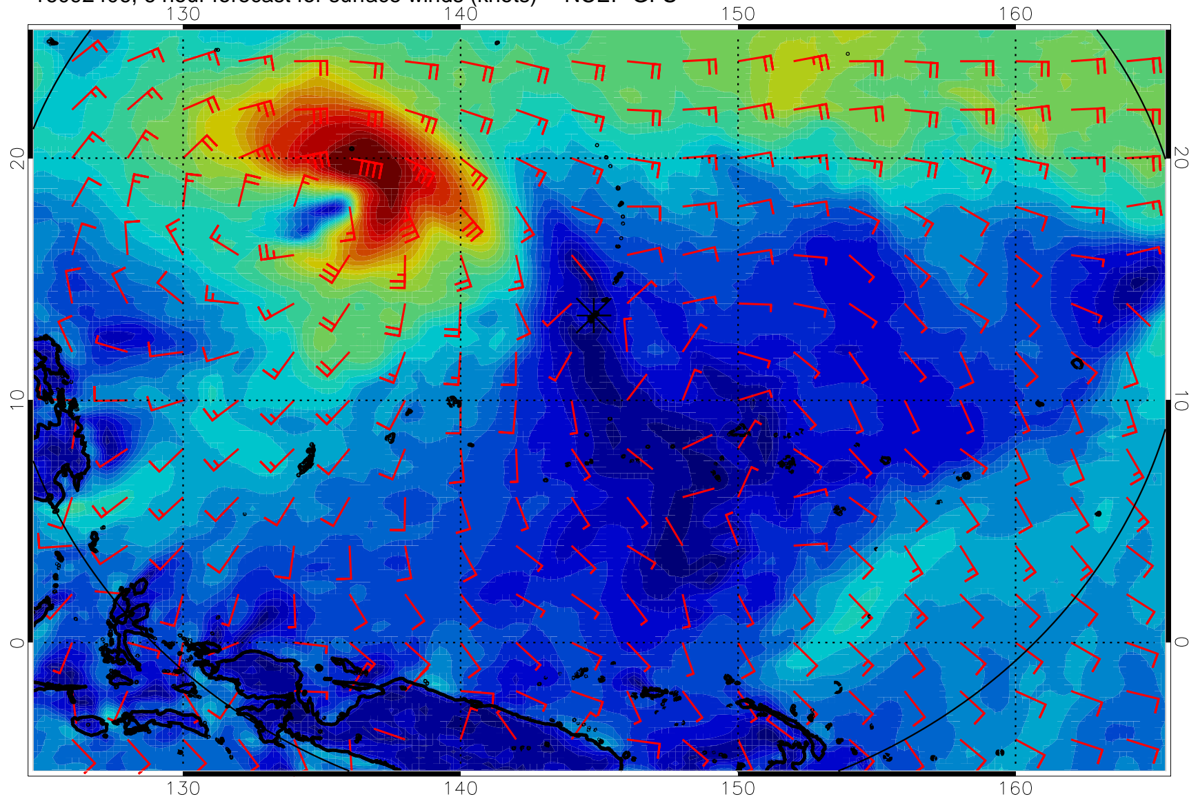
16092406, 6 hour forecast for surface winds (knots) -- NCEP GFS
