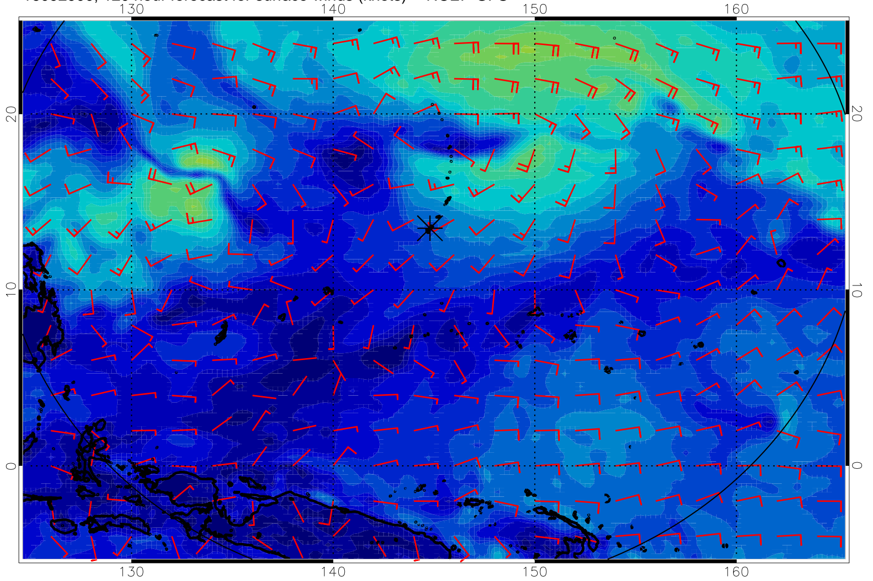
16092900, 120 hour forecast for surface winds (knots) -- NCEP GFS
