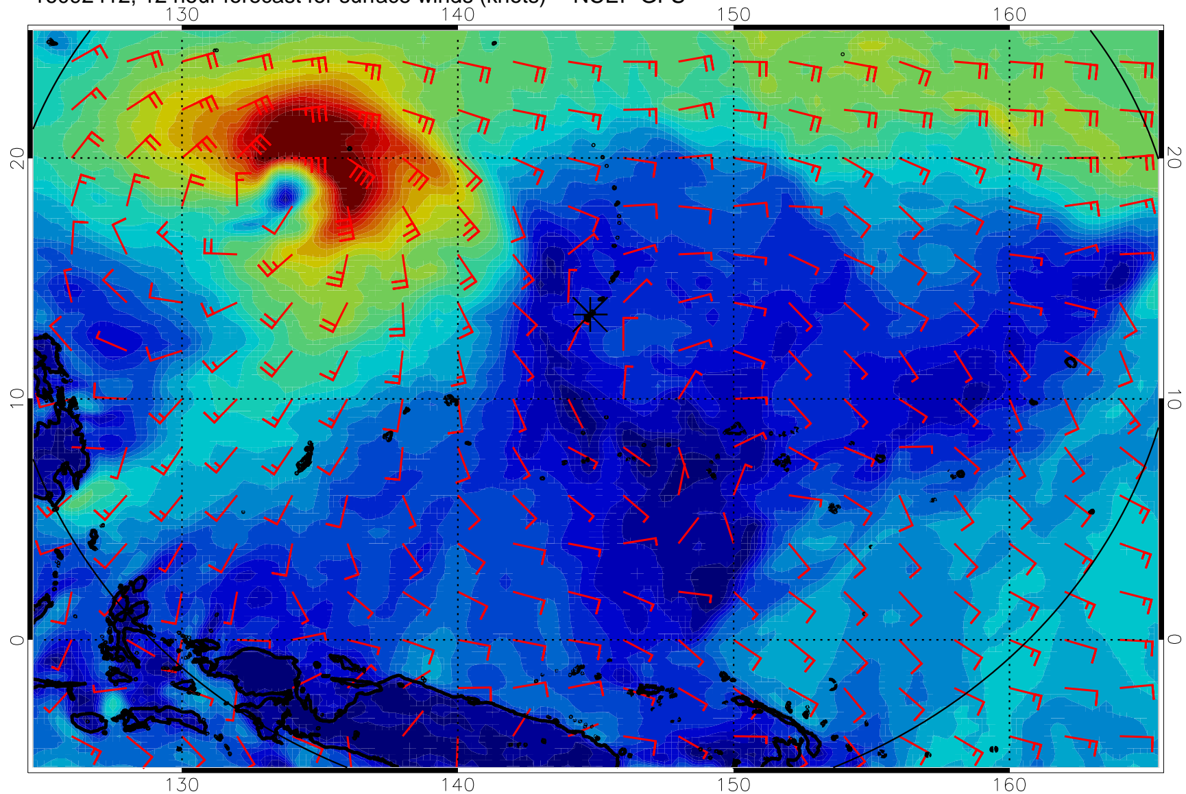
16092412, 12 hour forecast for surface winds (knots) -- NCEP GFS
