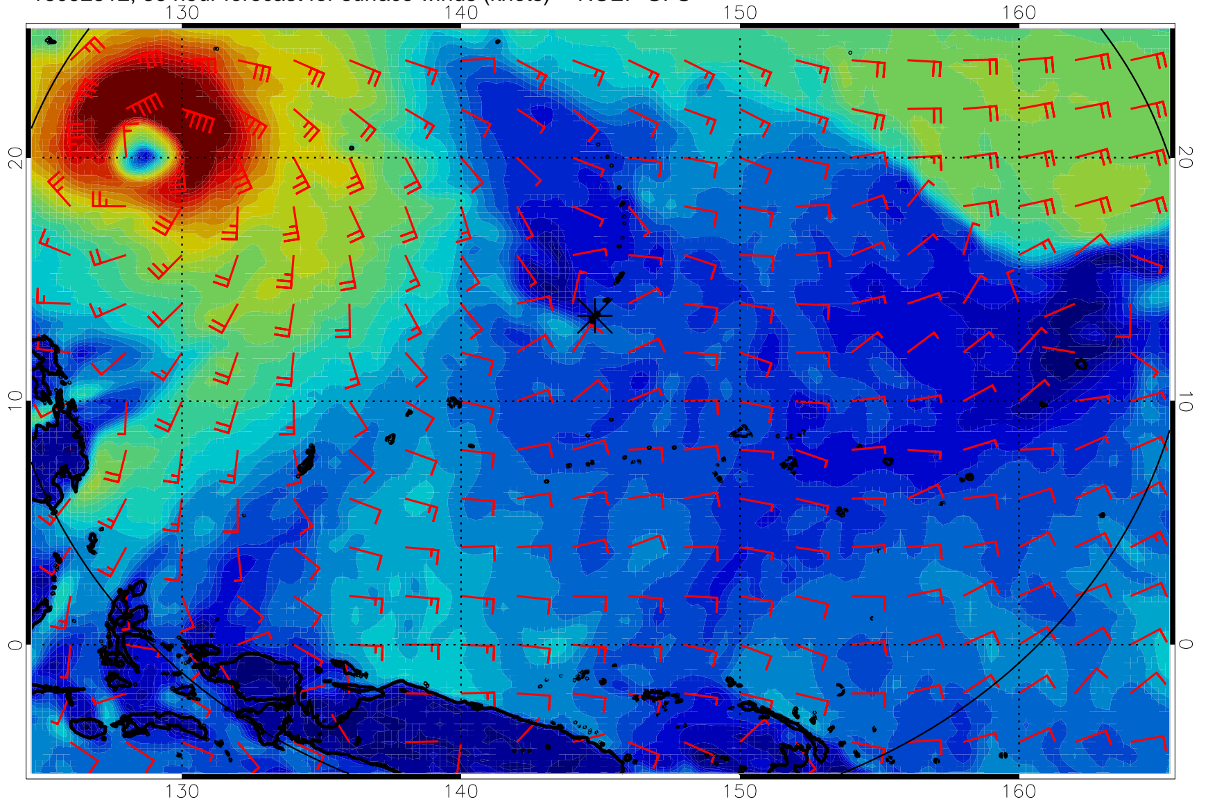
16092512, 36 hour forecast for surface winds (knots) -- NCEP GFS
