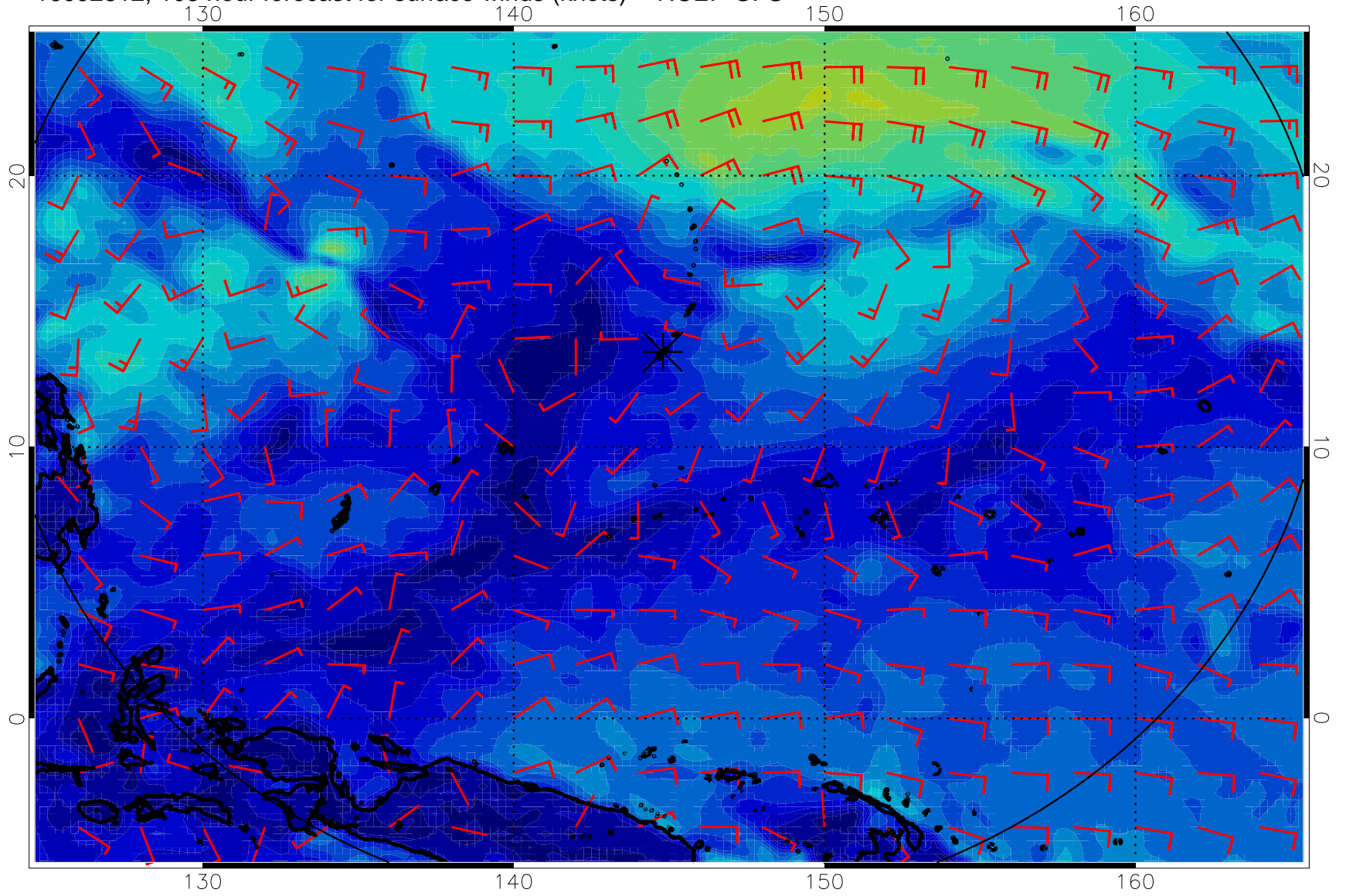
16092812, 108 hour forecast for surface winds (knots) -- NCEP GFS
