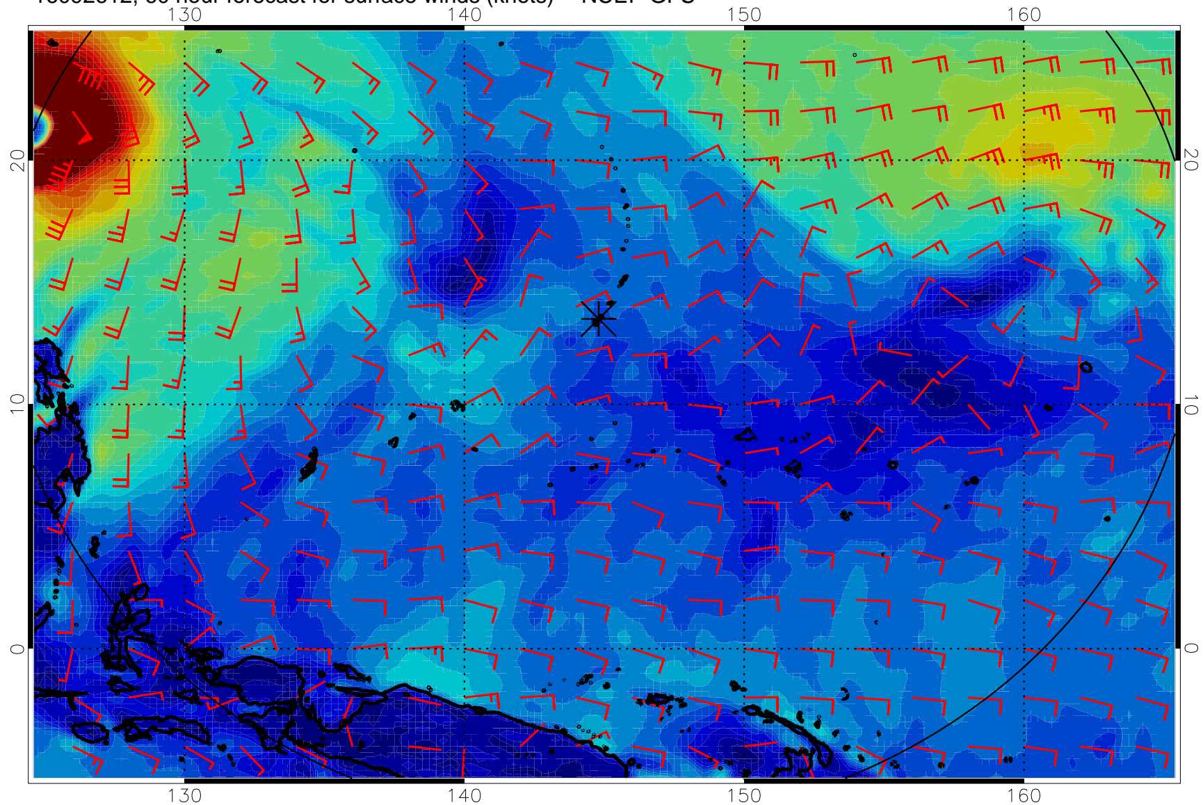
16092612, 60 hour forecast for surface winds (knots) -- NCEP GFS
