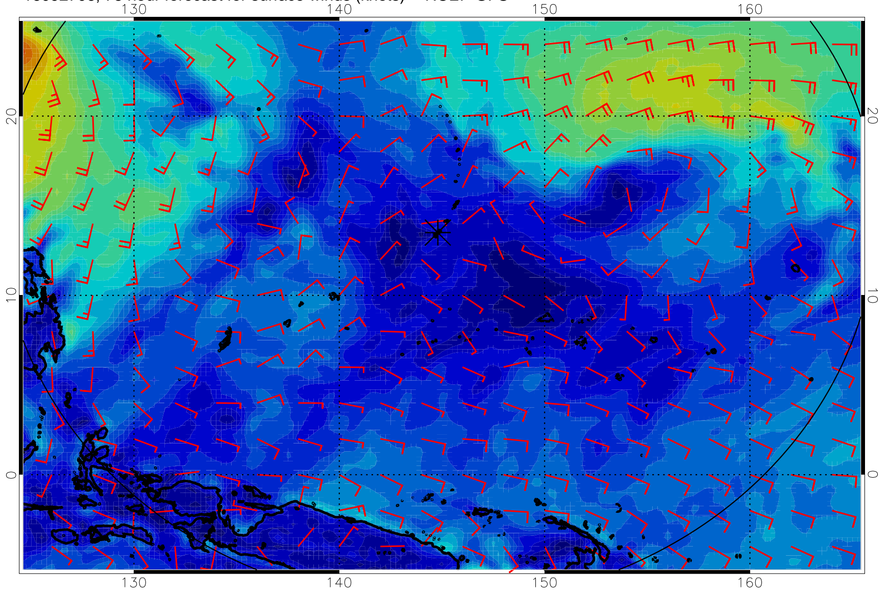
16092706, 78 hour forecast for surface winds (knots) -- NCEP GFS
