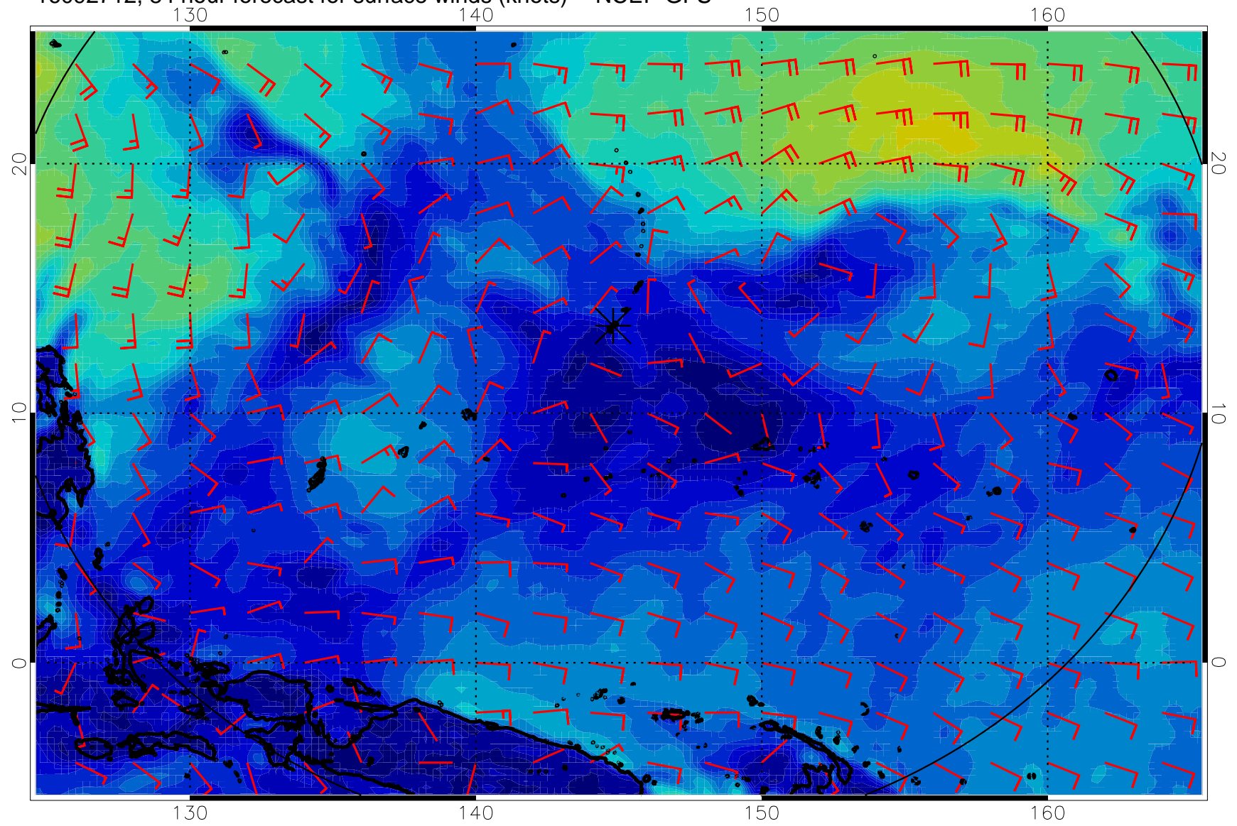
16092712, 84 hour forecast for surface winds (knots) -- NCEP GFS
