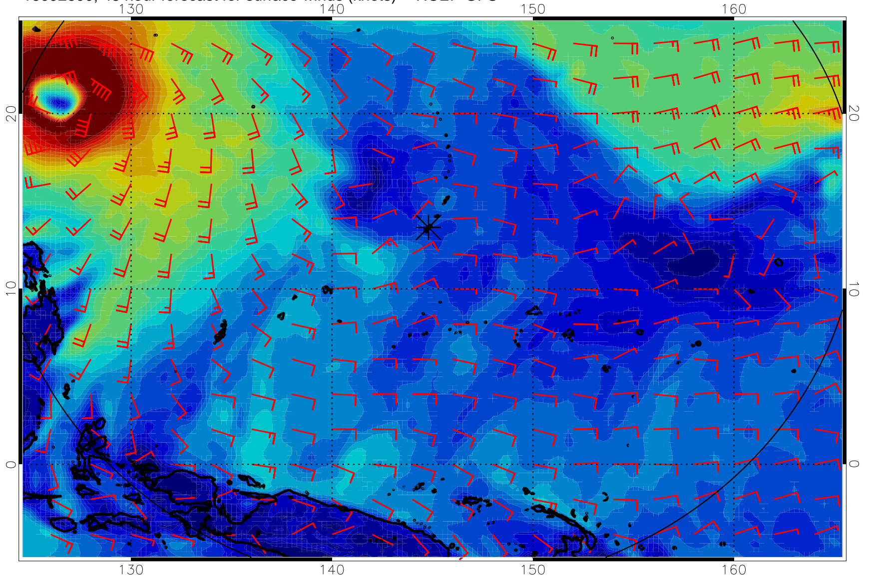
16092600, 48 hour forecast for surface winds (knots) -- NCEP GFS
