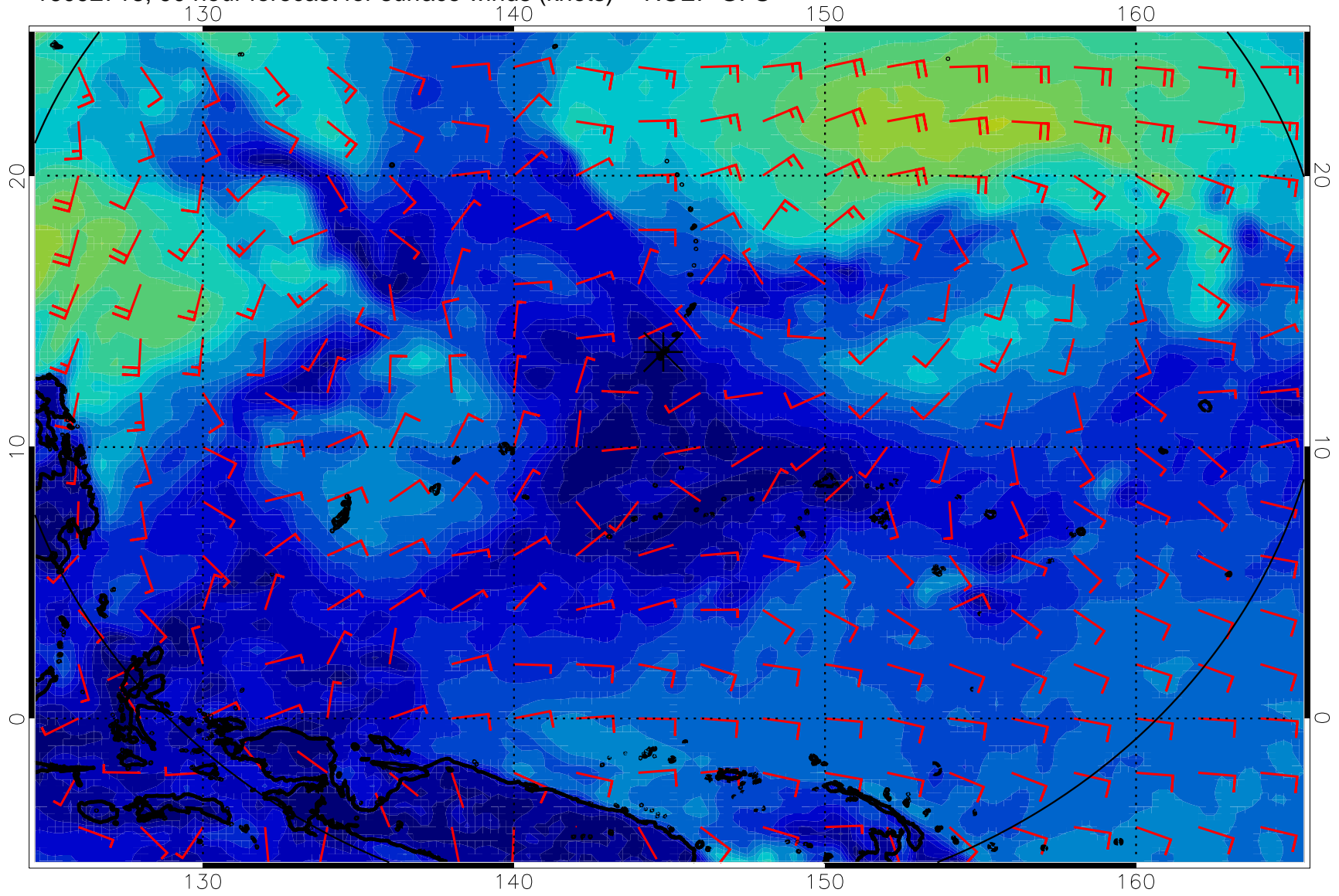
16092718, 90 hour forecast for surface winds (knots) -- NCEP GFS
