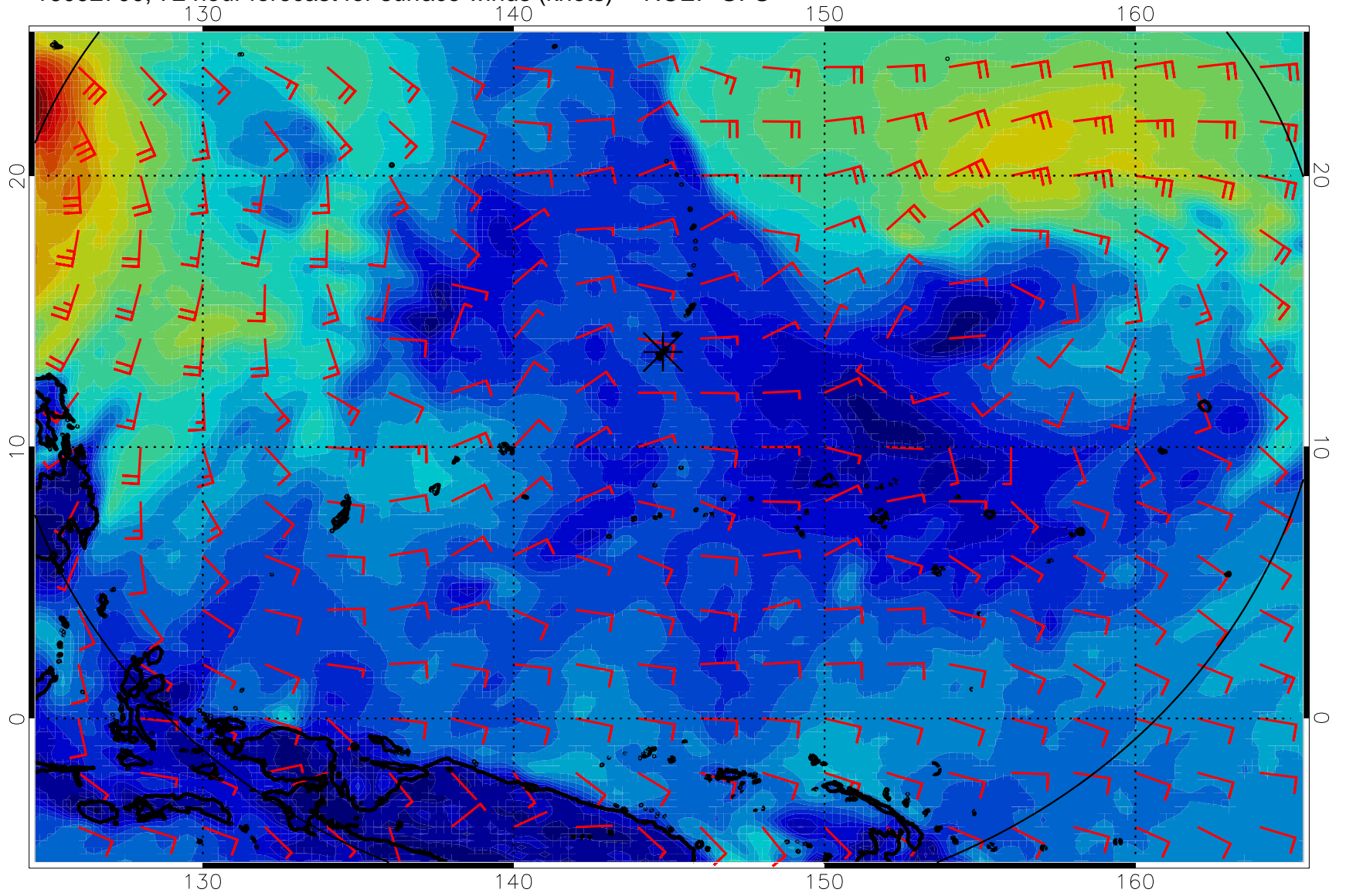
16092700, 72 hour forecast for surface winds (knots) -- NCEP GFS
