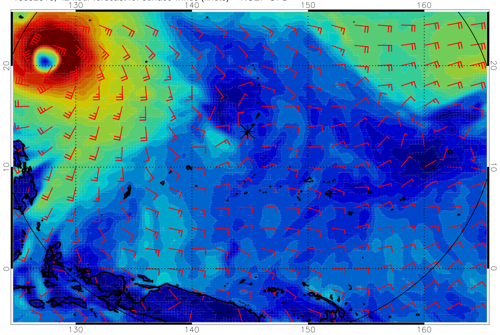
16092518, 42 hour forecast for surface winds (knots) -- NCEP GFS
