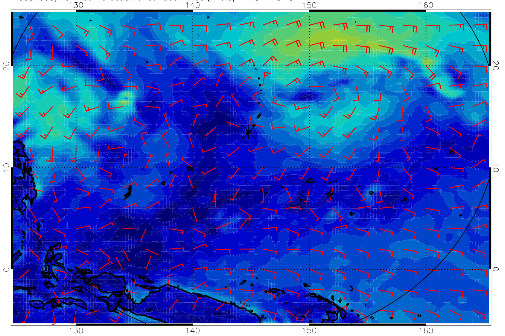
16092806, 102 hour forecast for surface winds (knots) -- NCEP GFS
