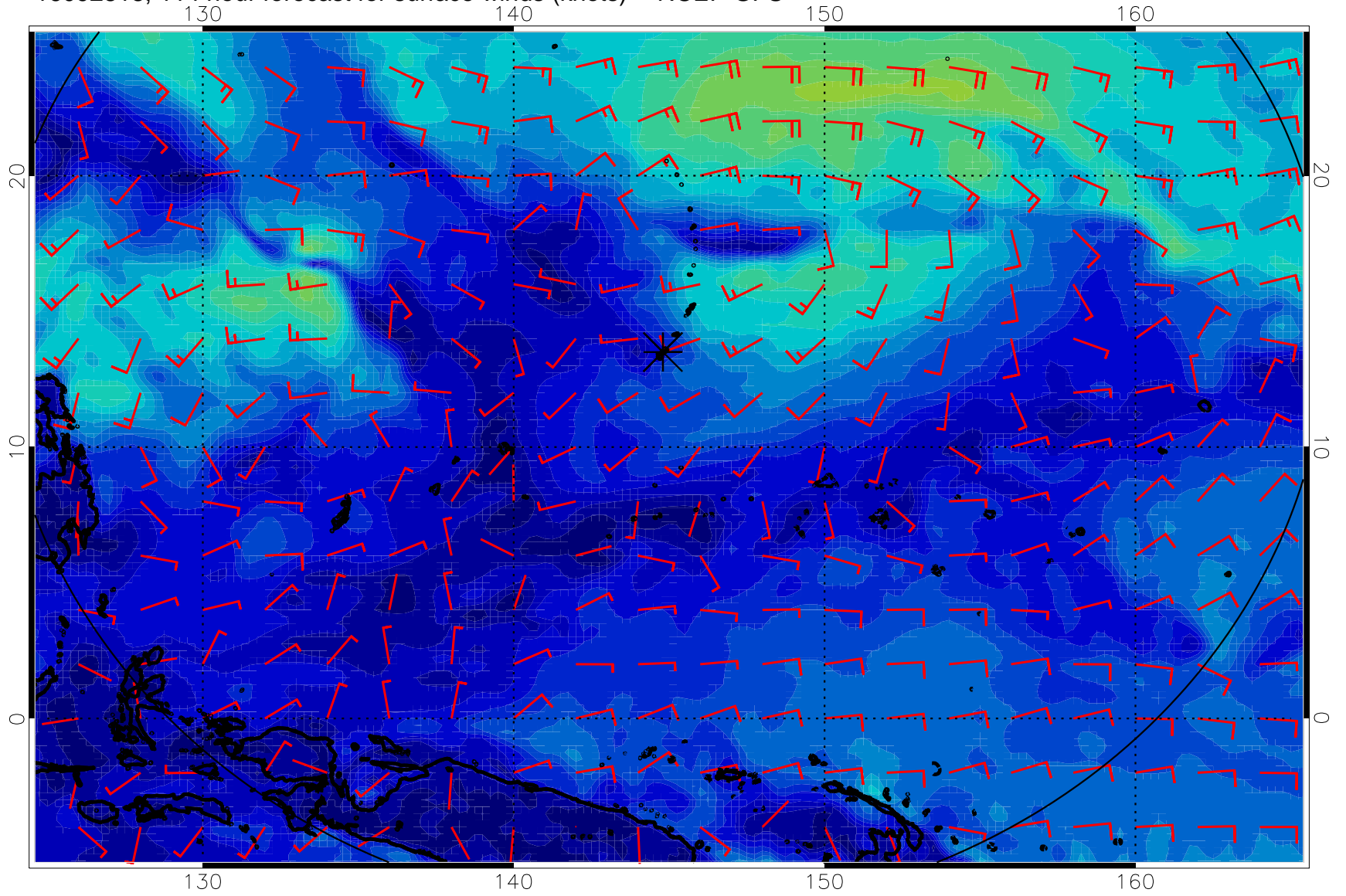
16092818, 114 hour forecast for surface winds (knots) -- NCEP GFS
