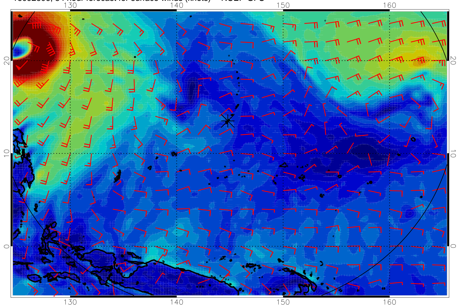
16092606, 54 hour forecast for surface winds (knots) -- NCEP GFS
