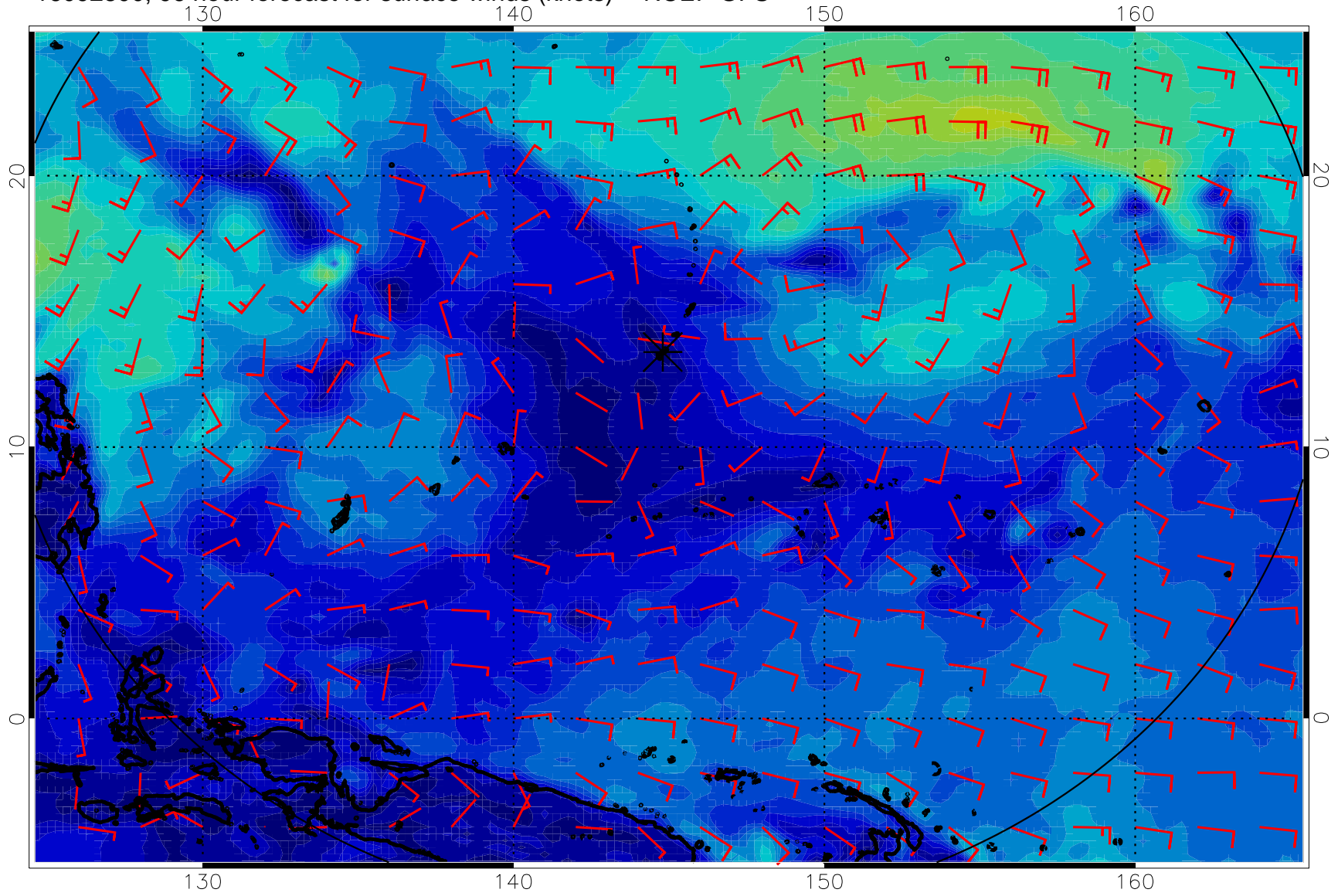
16092800, 96 hour forecast for surface winds (knots) -- NCEP GFS
