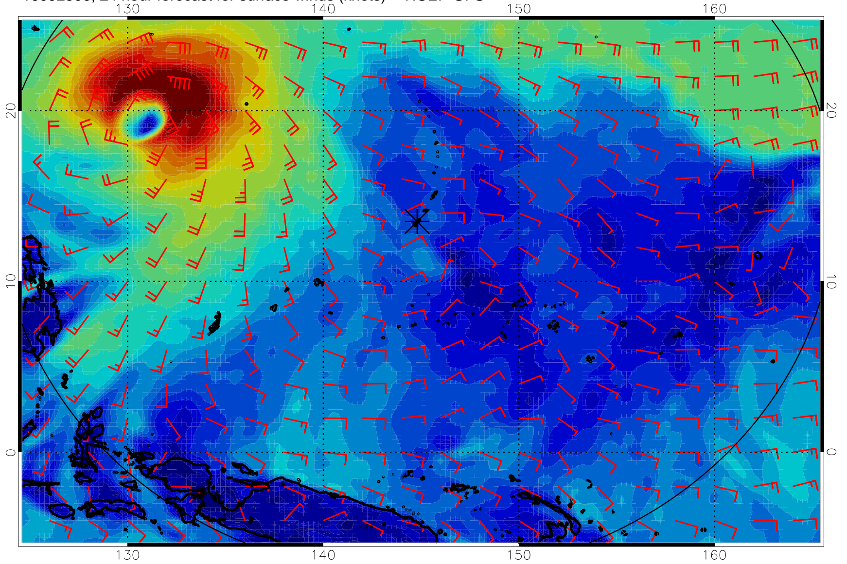
16092500, 24 hour forecast for surface winds (knots) -- NCEP GFS
