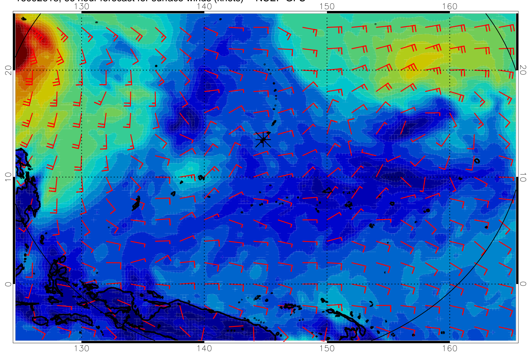
16092618, 66 hour forecast for surface winds (knots) -- NCEP GFS
