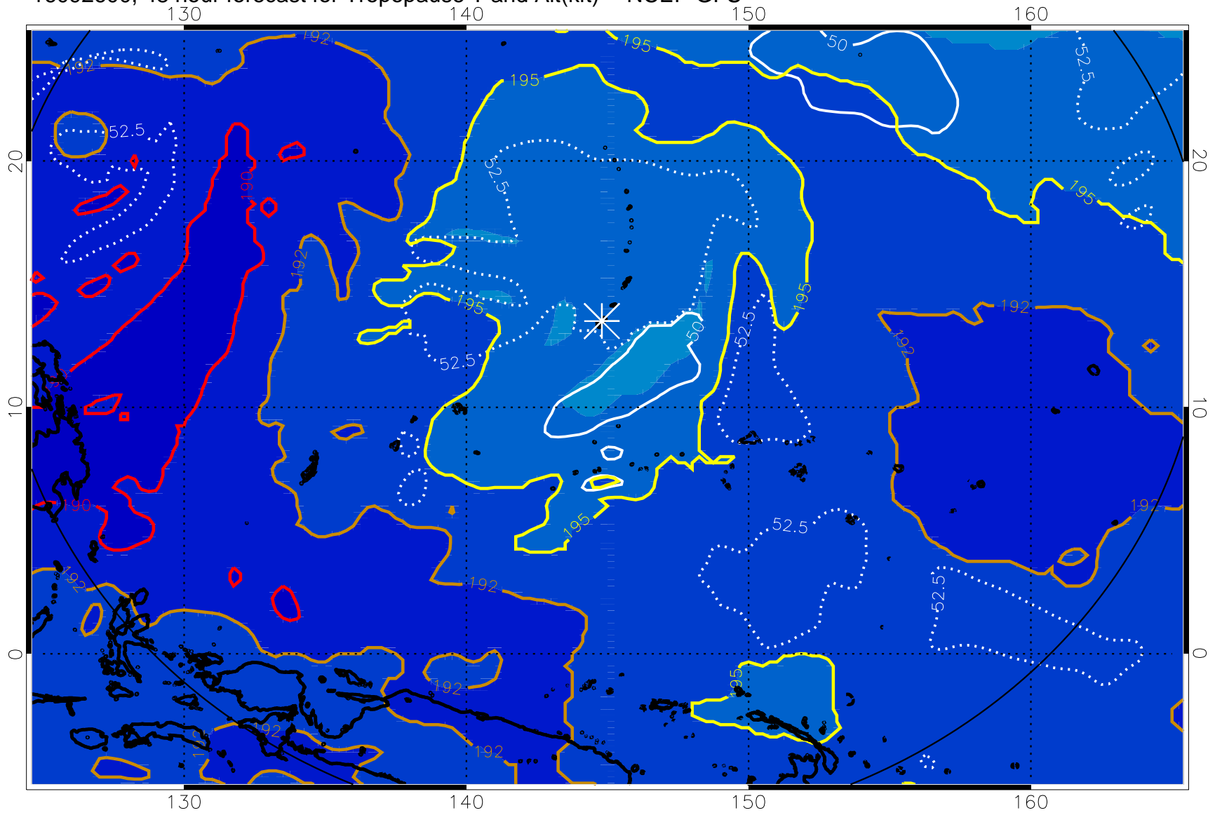
16092600, 48 hour forecast for Tropopause T and Alt(kft) -- NCEP GFS
