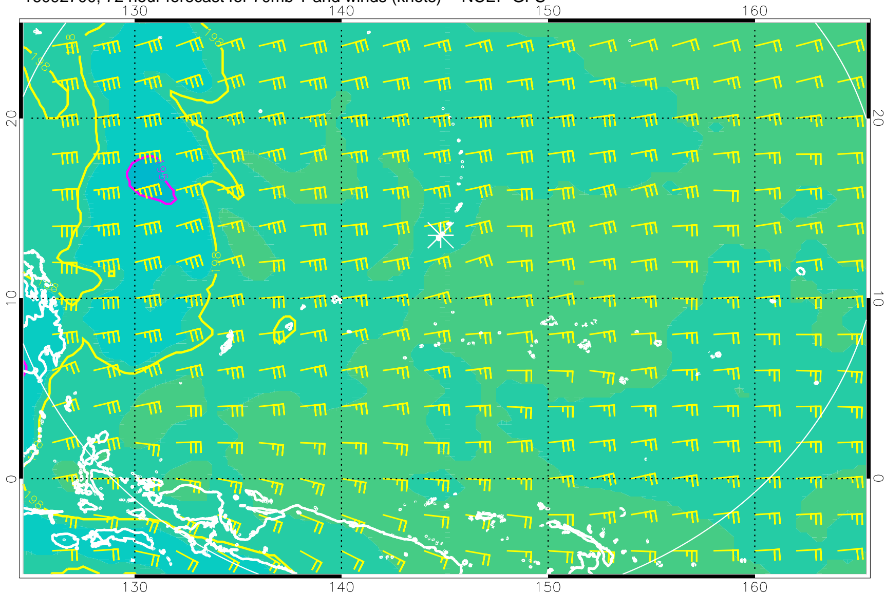
16092700, 72 hour forecast for 70mb T and winds (knots) -- NCEP GFS
