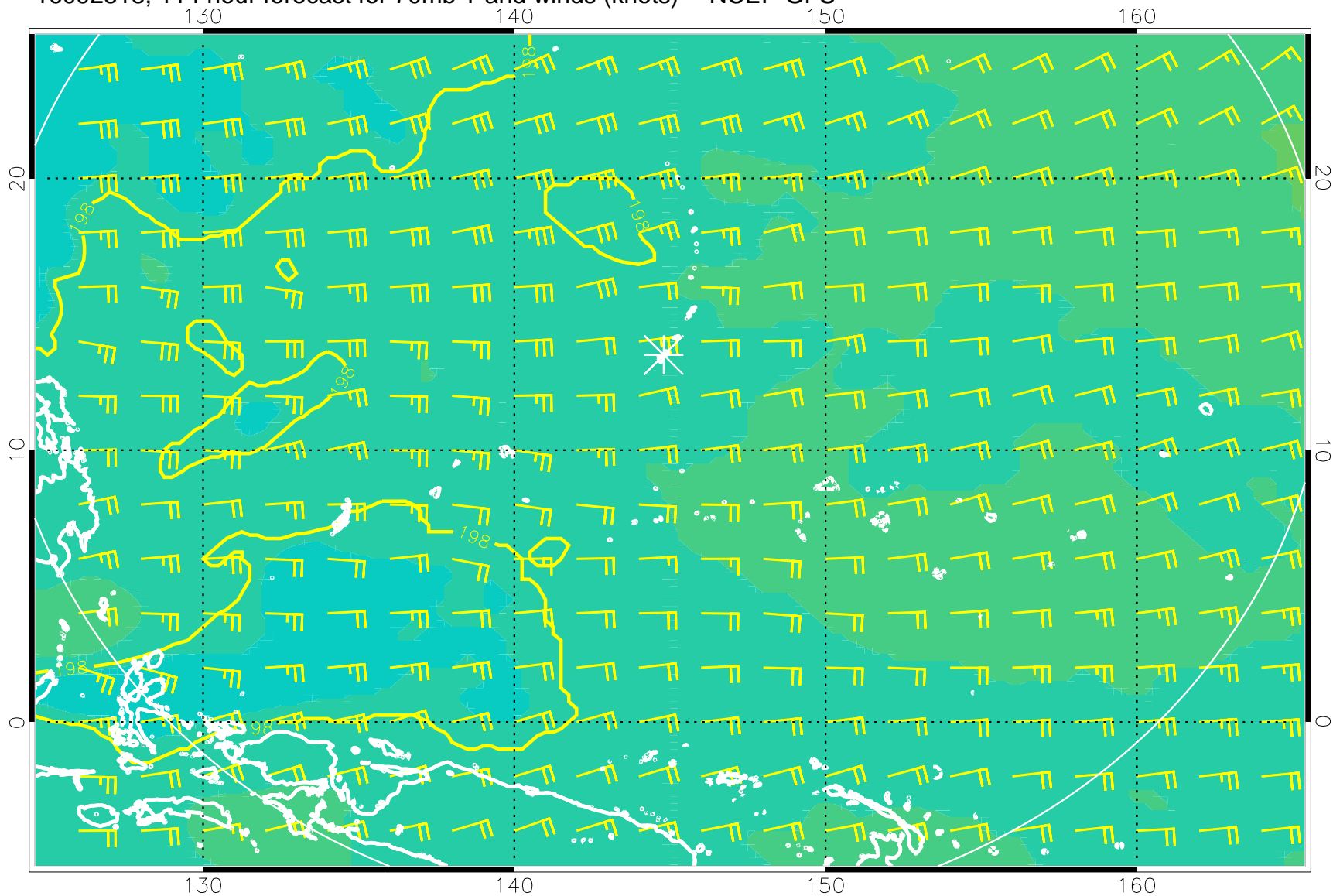
16092818, 114 hour forecast for 70mb T and winds (knots) -- NCEP GFS
