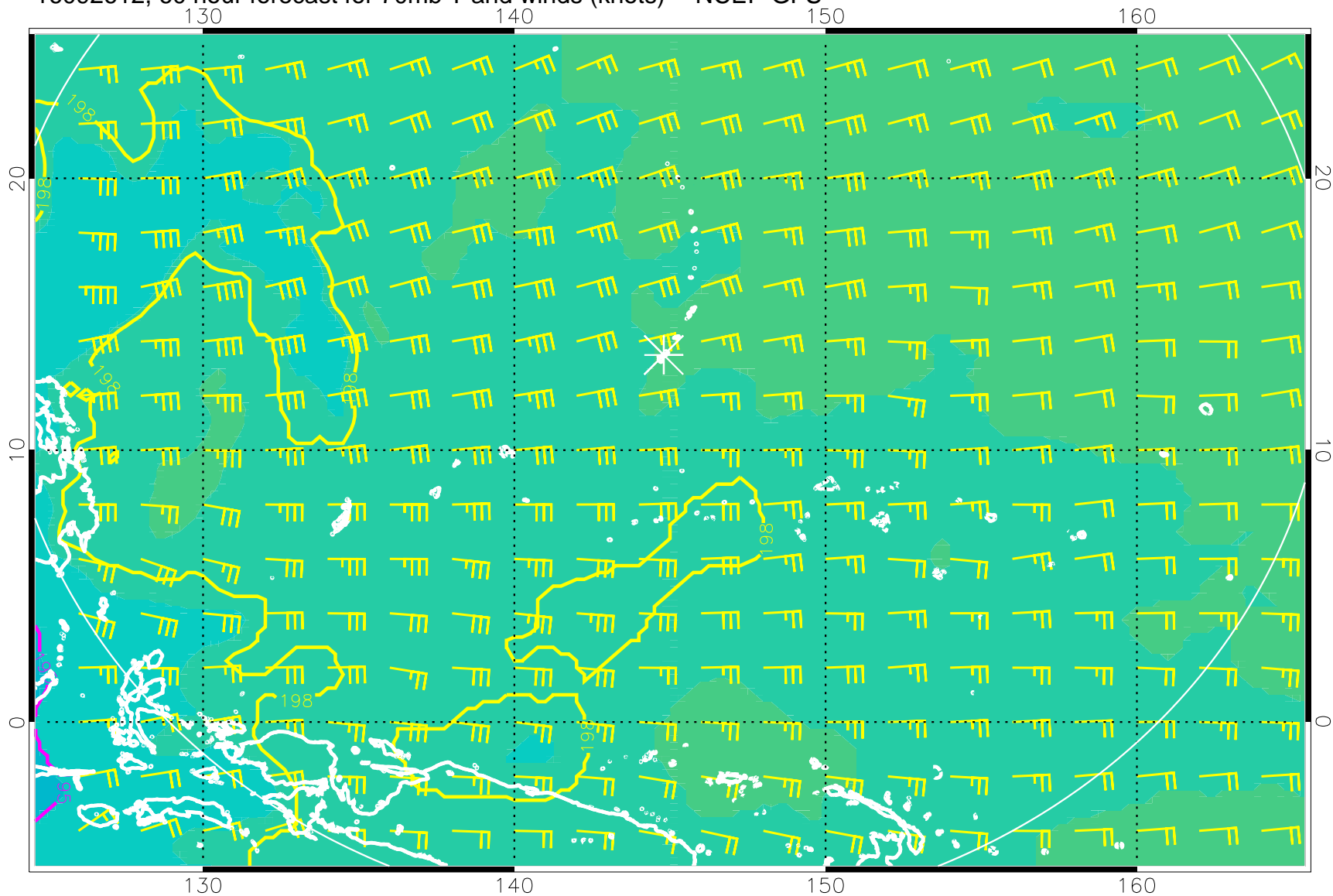
16092612, 60 hour forecast for 70mb T and winds (knots) -- NCEP GFS
