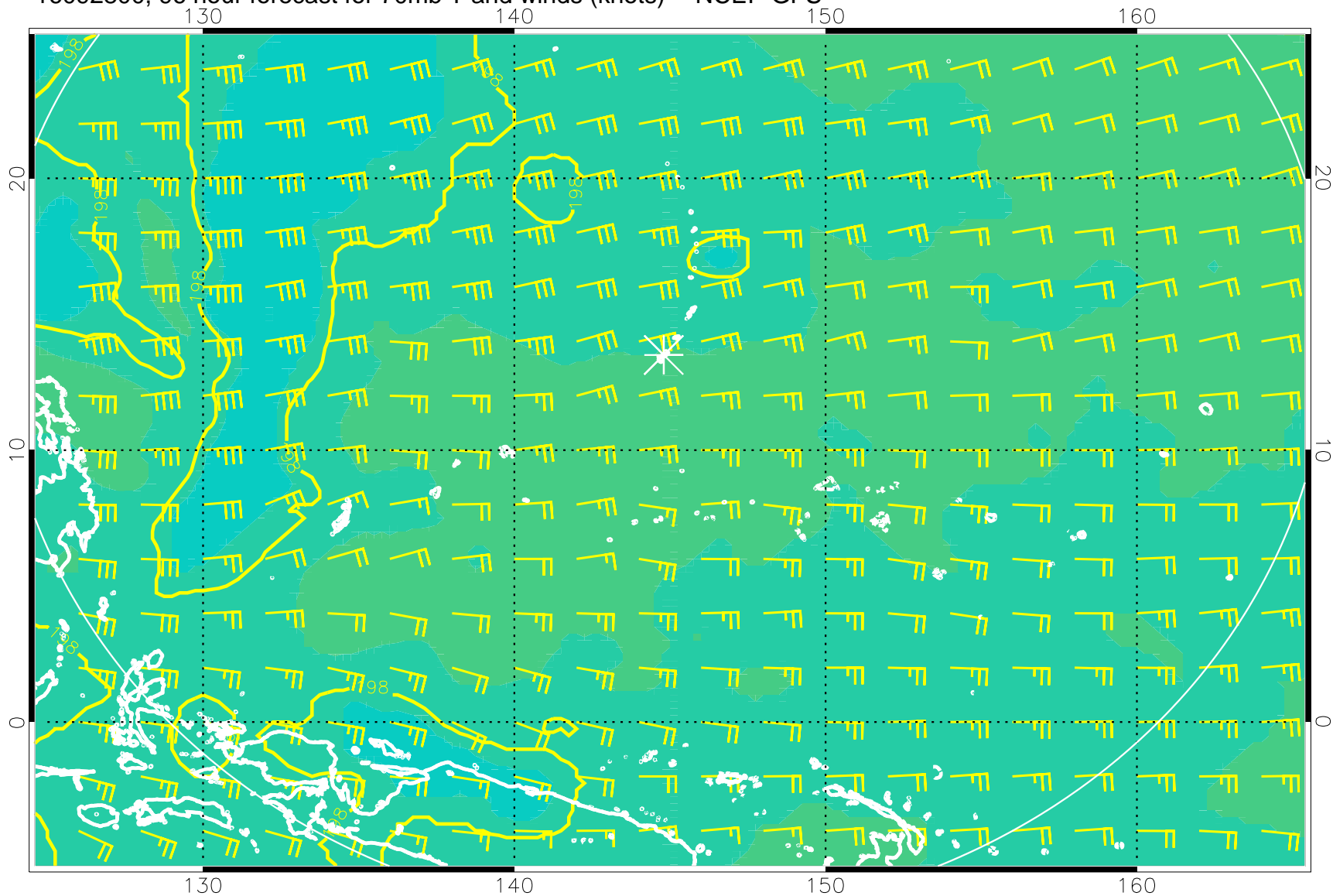
16092800, 96 hour forecast for 70mb T and winds (knots) -- NCEP GFS
