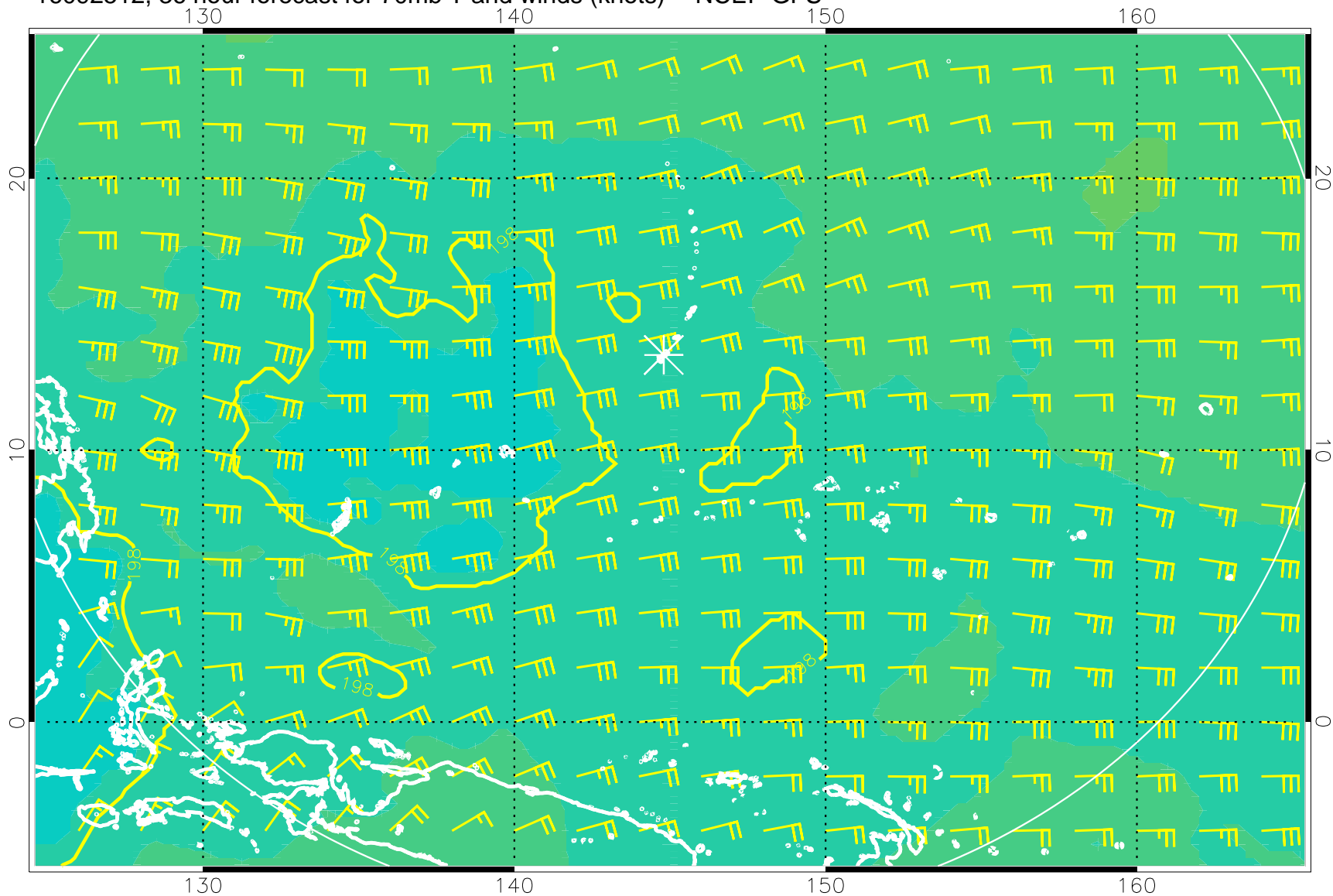
16092512, 36 hour forecast for 70mb T and winds (knots) -- NCEP GFS
