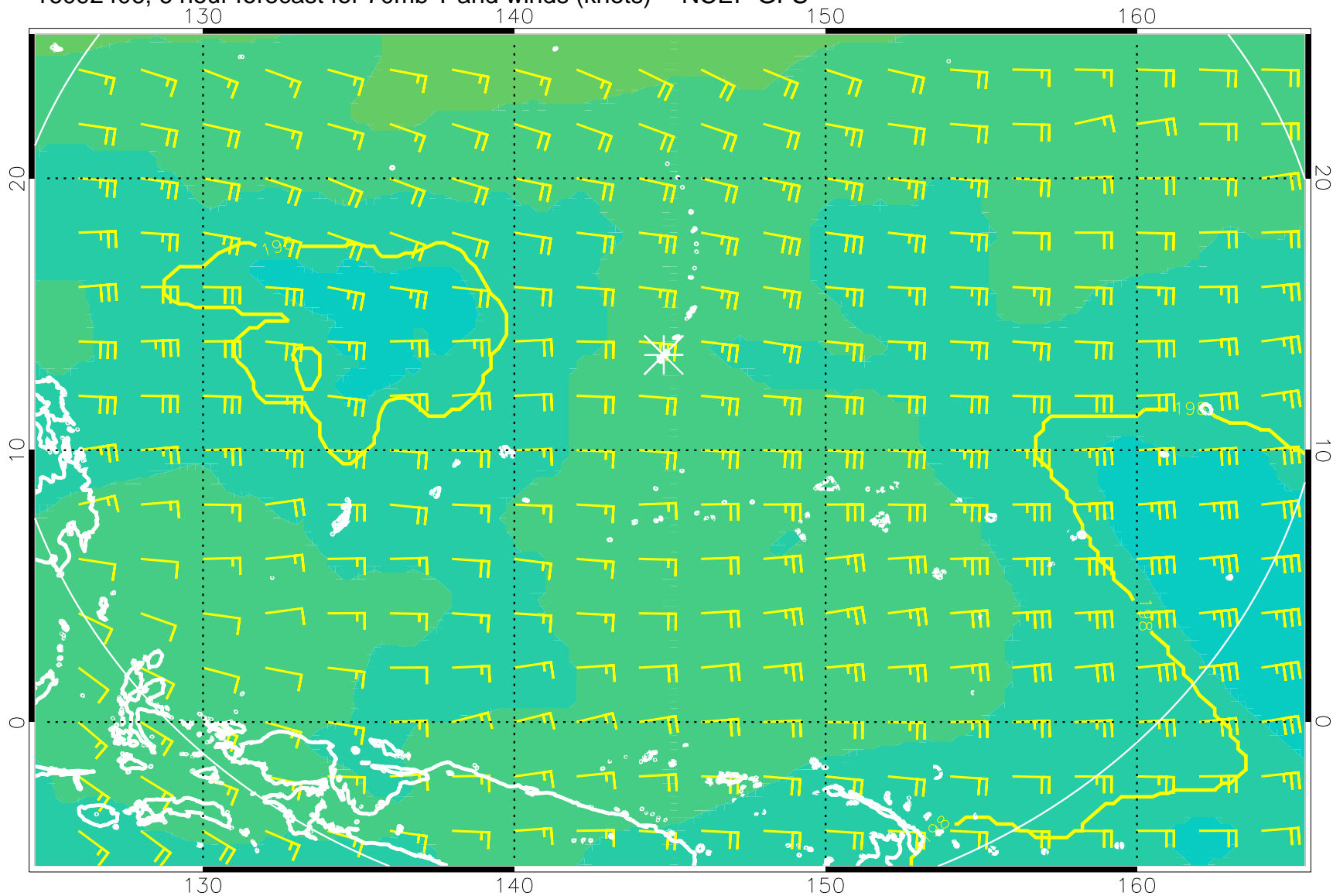
16092406, 6 hour forecast for 70mb T and winds (knots) -- NCEP GFS
