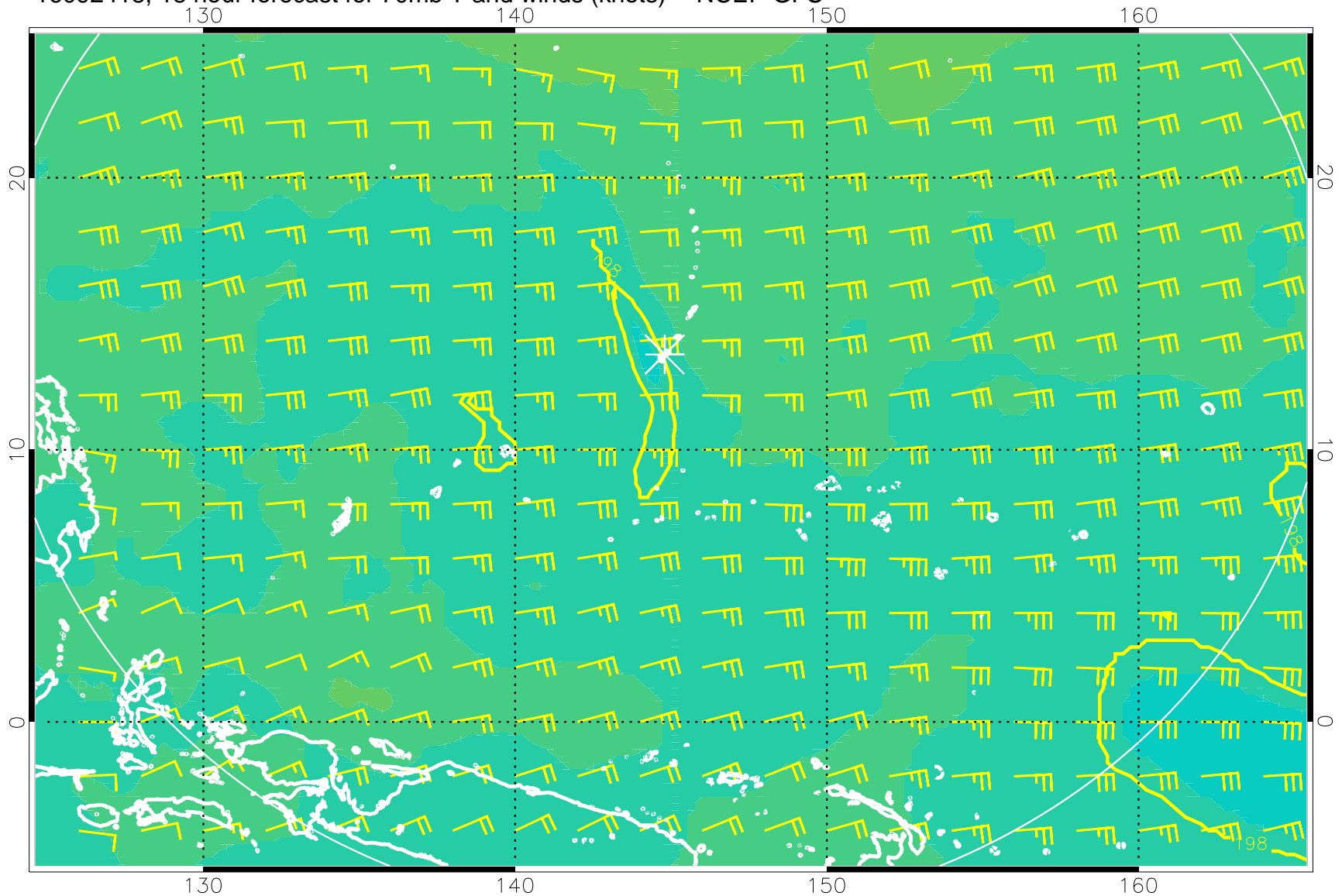
16092418, 18 hour forecast for 70mb T and winds (knots) -- NCEP GFS
