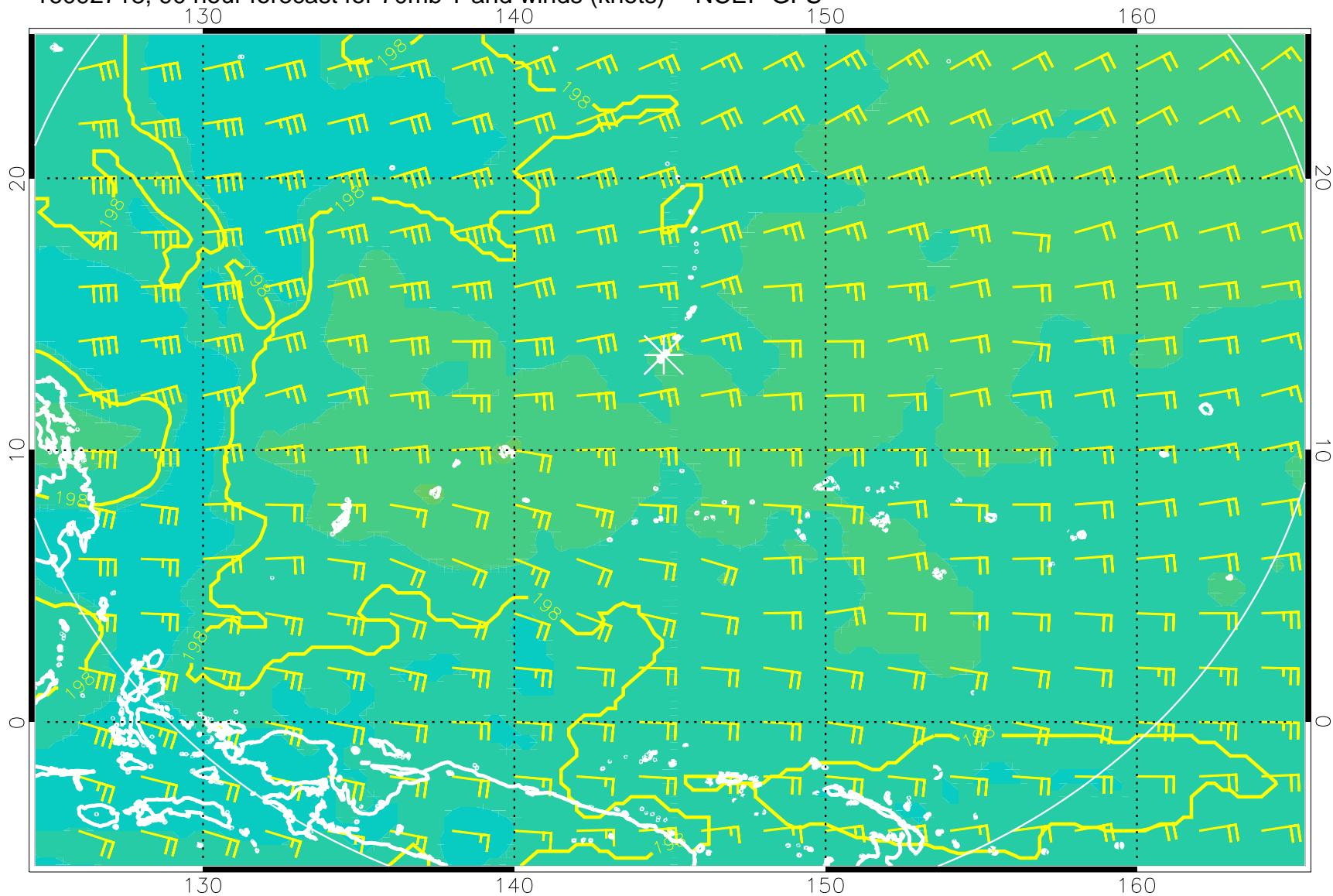
16092718, 90 hour forecast for 70mb T and winds (knots) -- NCEP GFS
