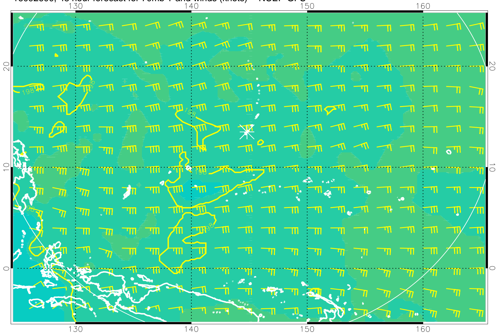
16092600, 48 hour forecast for 70mb T and winds (knots) -- NCEP GFS
