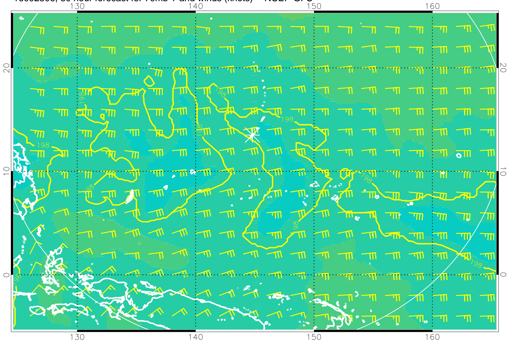
16092506, 30 hour forecast for 70mb T and winds (knots) -- NCEP GFS
