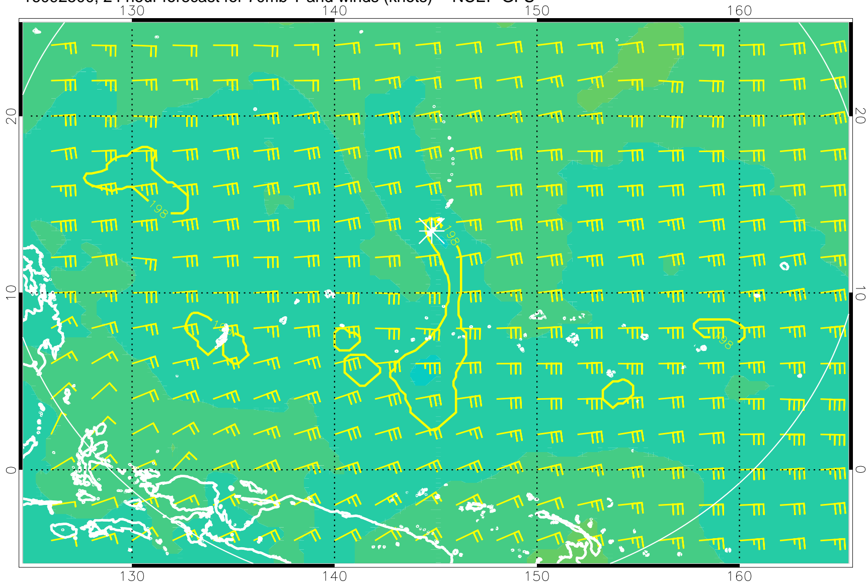
16092500, 24 hour forecast for 70mb T and winds (knots) -- NCEP GFS
