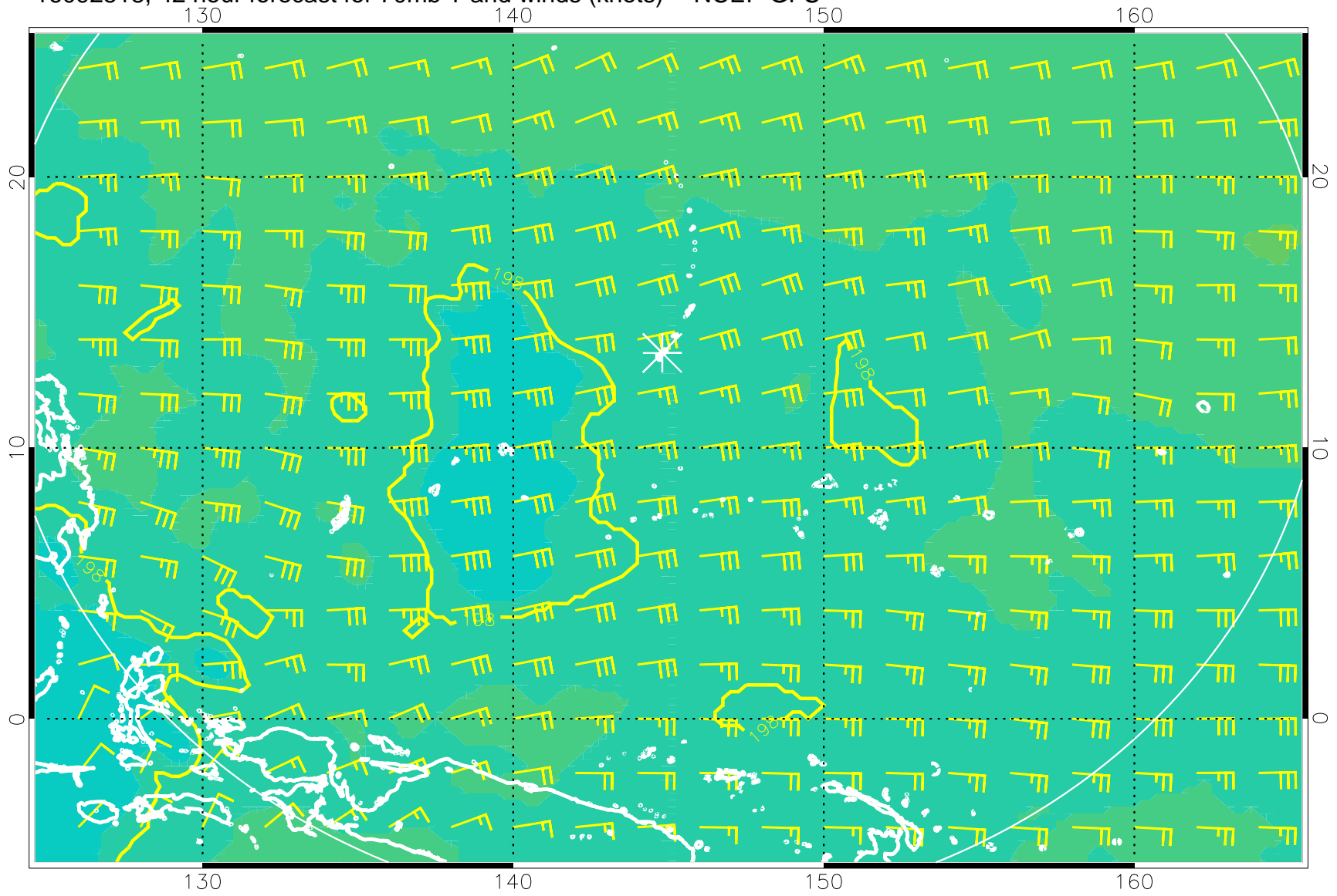
16092518, 42 hour forecast for 70mb T and winds (knots) -- NCEP GFS
