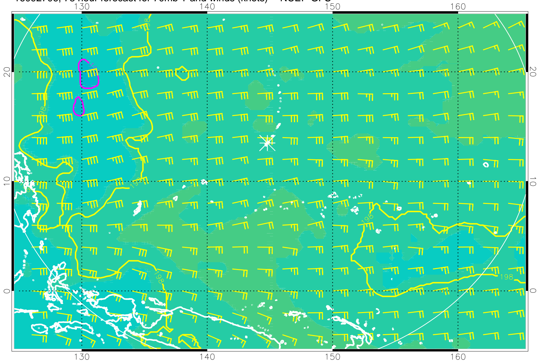
16092706, 78 hour forecast for 70mb T and winds (knots) -- NCEP GFS
