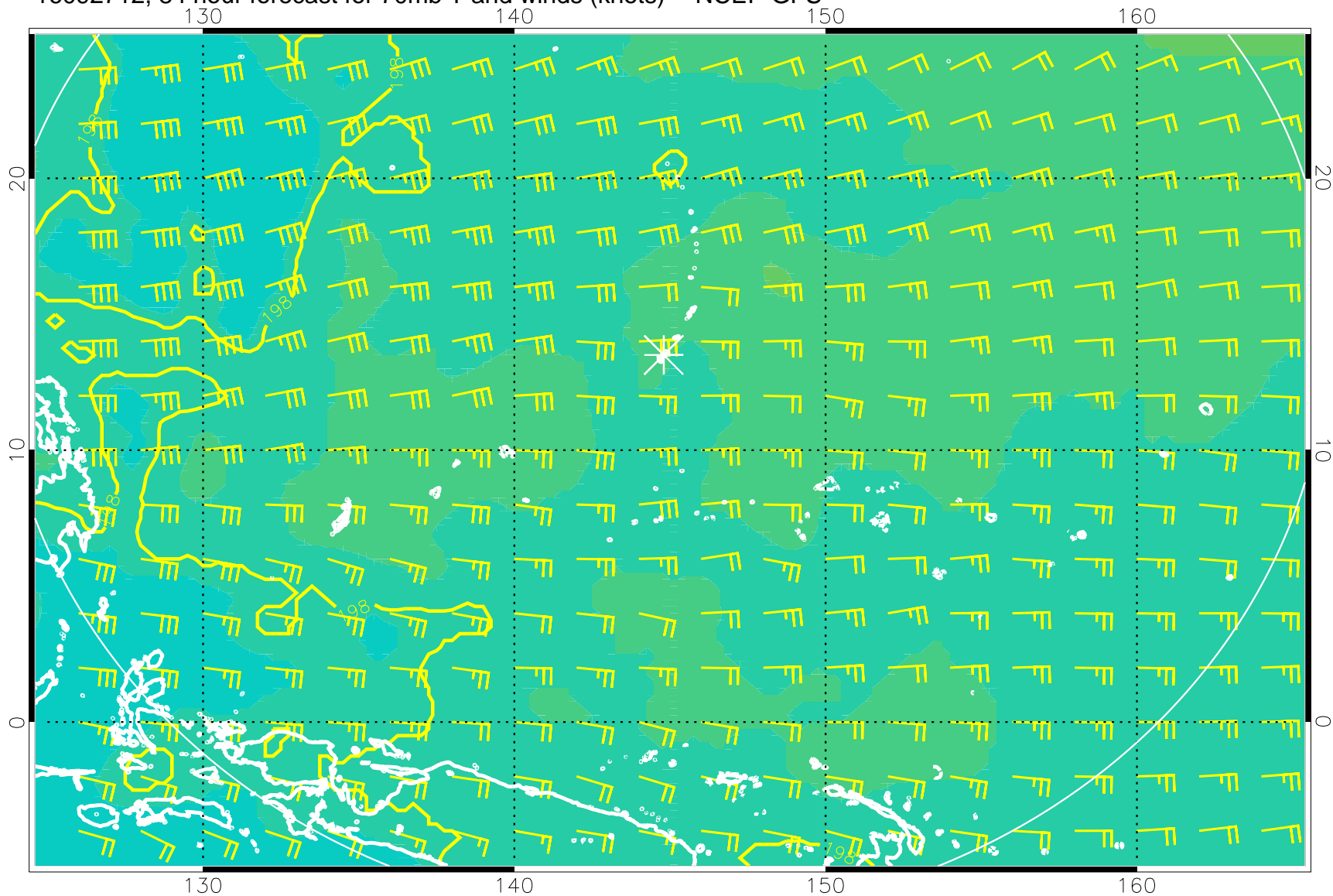
16092712, 84 hour forecast for 70mb T and winds (knots) -- NCEP GFS
