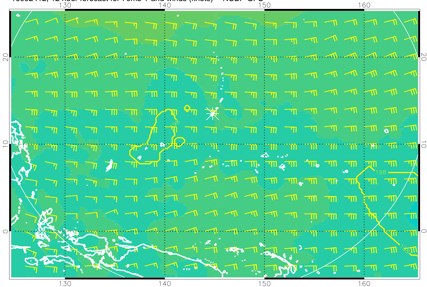
16092412, 12 hour forecast for 70mb T and winds (knots) -- NCEP GFS
