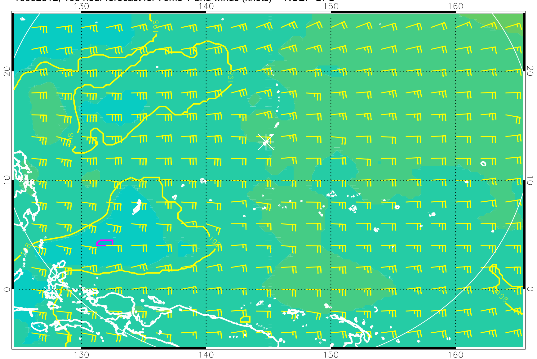
16092812, 108 hour forecast for 70mb T and winds (knots) -- NCEP GFS
