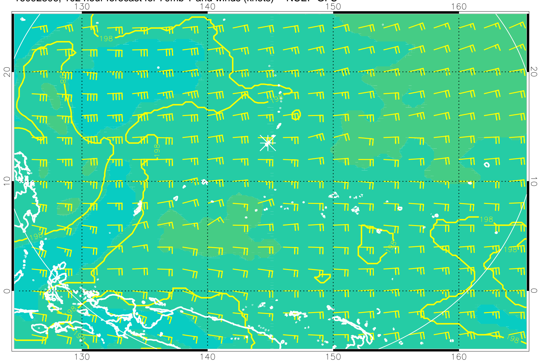
16092806, 102 hour forecast for 70mb T and winds (knots) -- NCEP GFS
