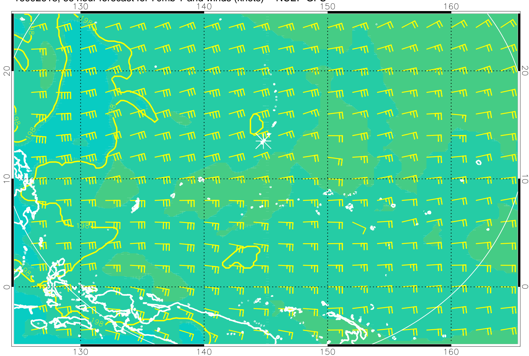
16092618, 66 hour forecast for 70mb T and winds (knots) -- NCEP GFS
