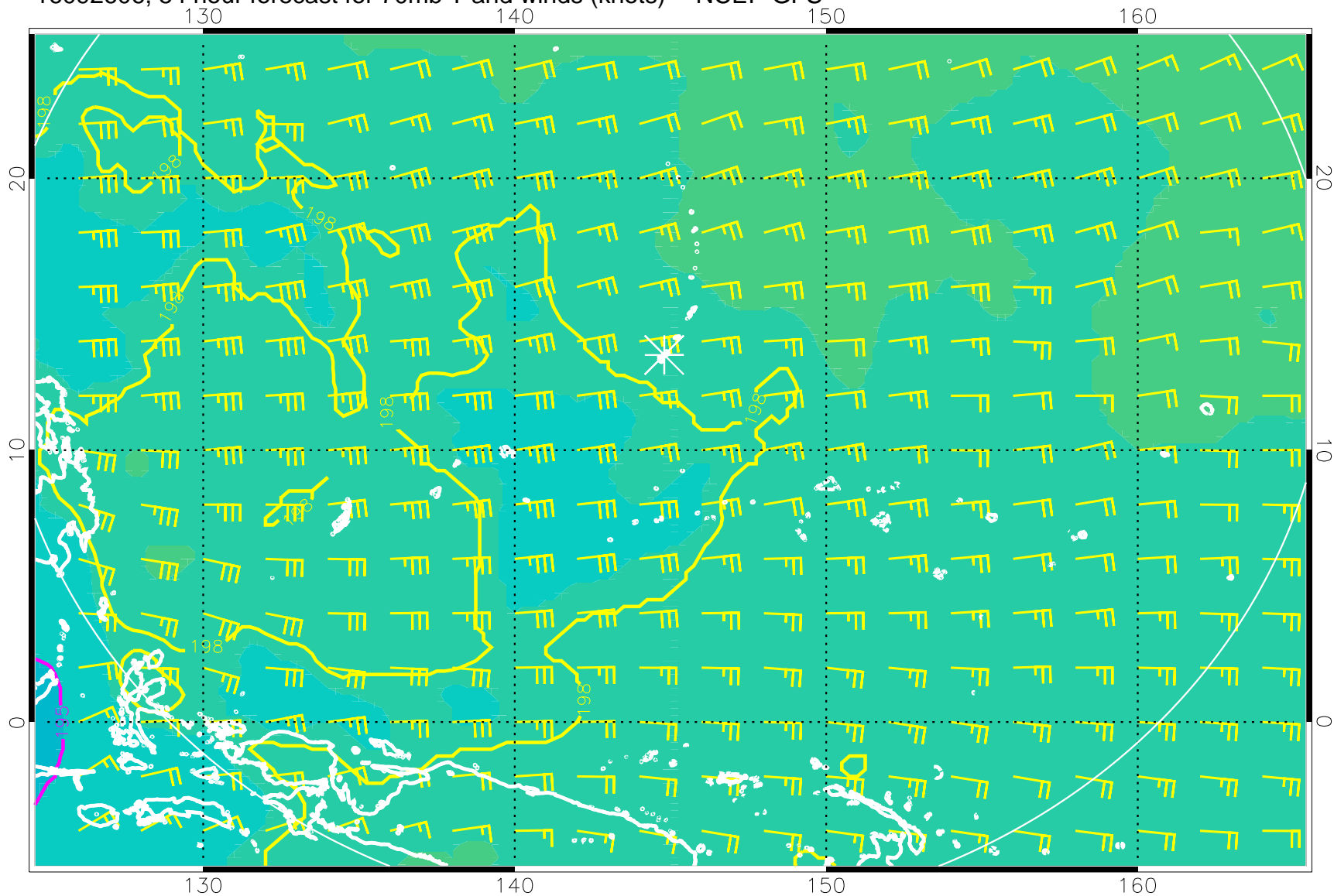
16092606, 54 hour forecast for 70mb T and winds (knots) -- NCEP GFS
