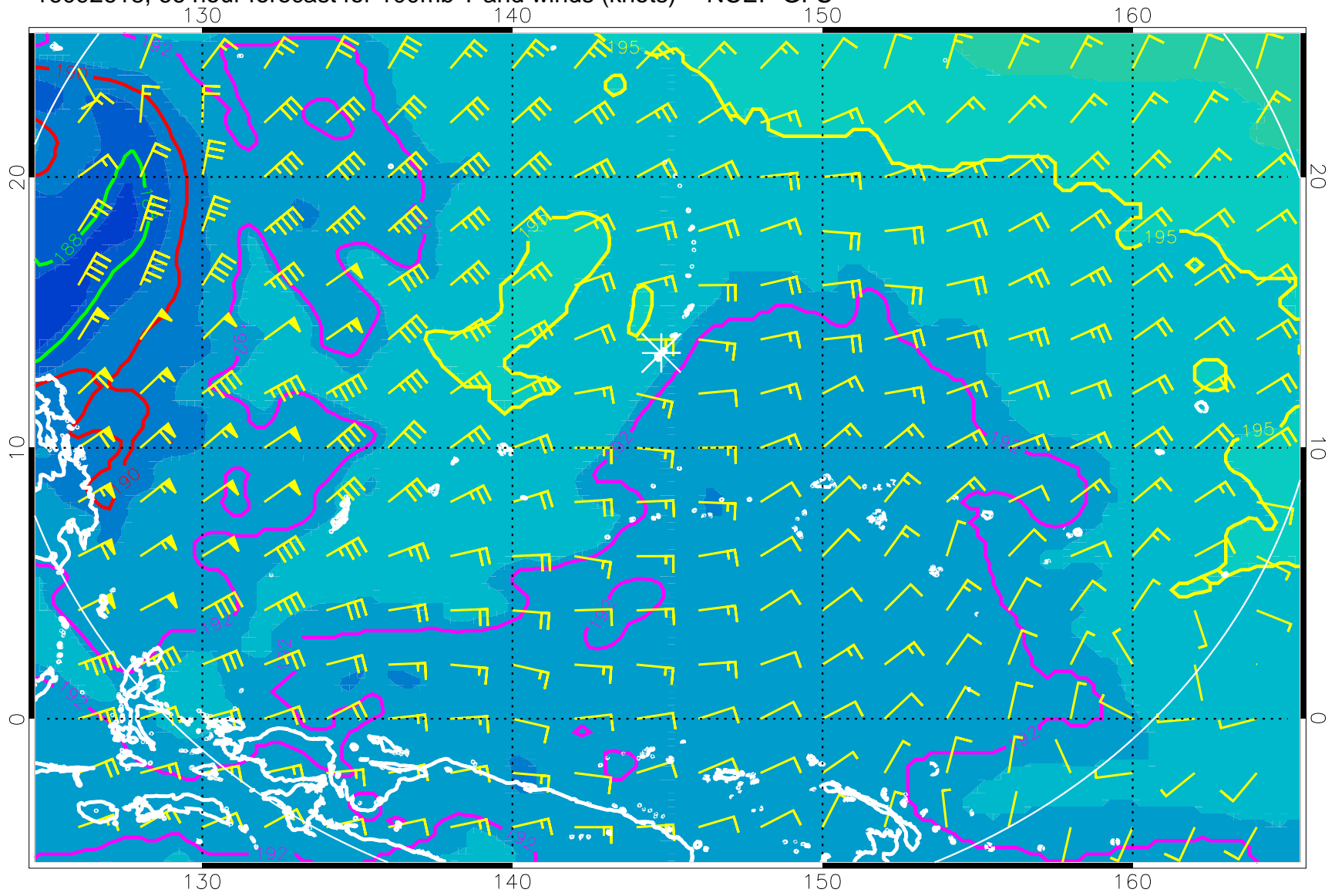
16092618, 66 hour forecast for 100mb T and winds (knots) -- NCEP GFS
