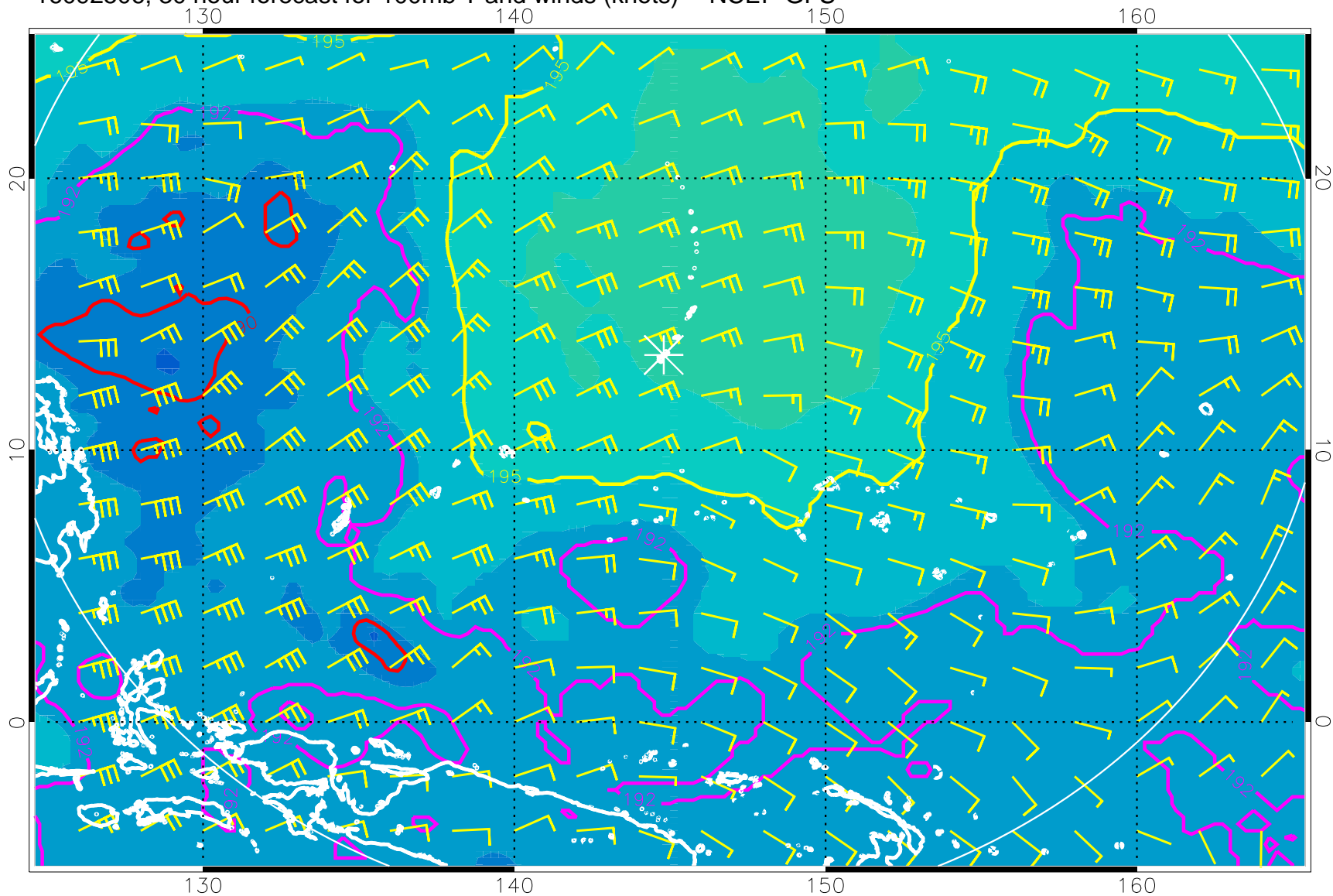
16092506, 30 hour forecast for 100mb T and winds (knots) -- NCEP GFS
