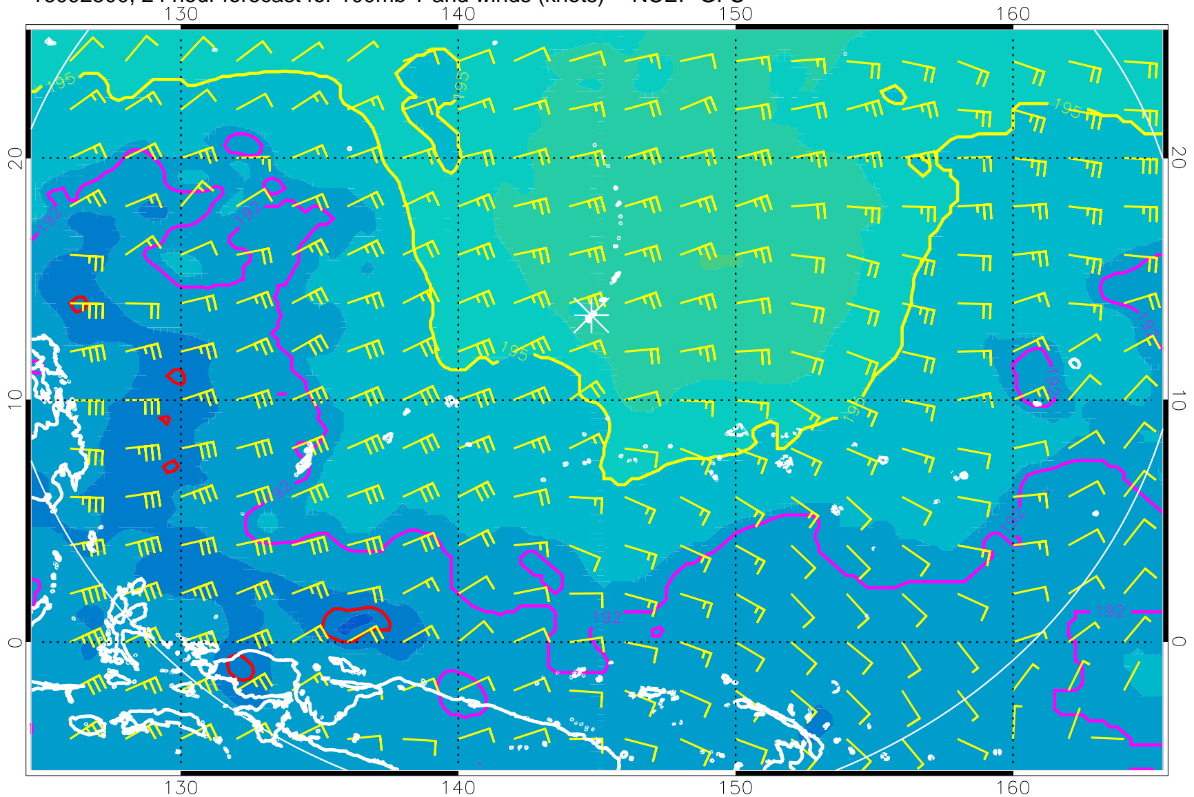
16092500, 24 hour forecast for 100mb T and winds (knots) -- NCEP GFS
