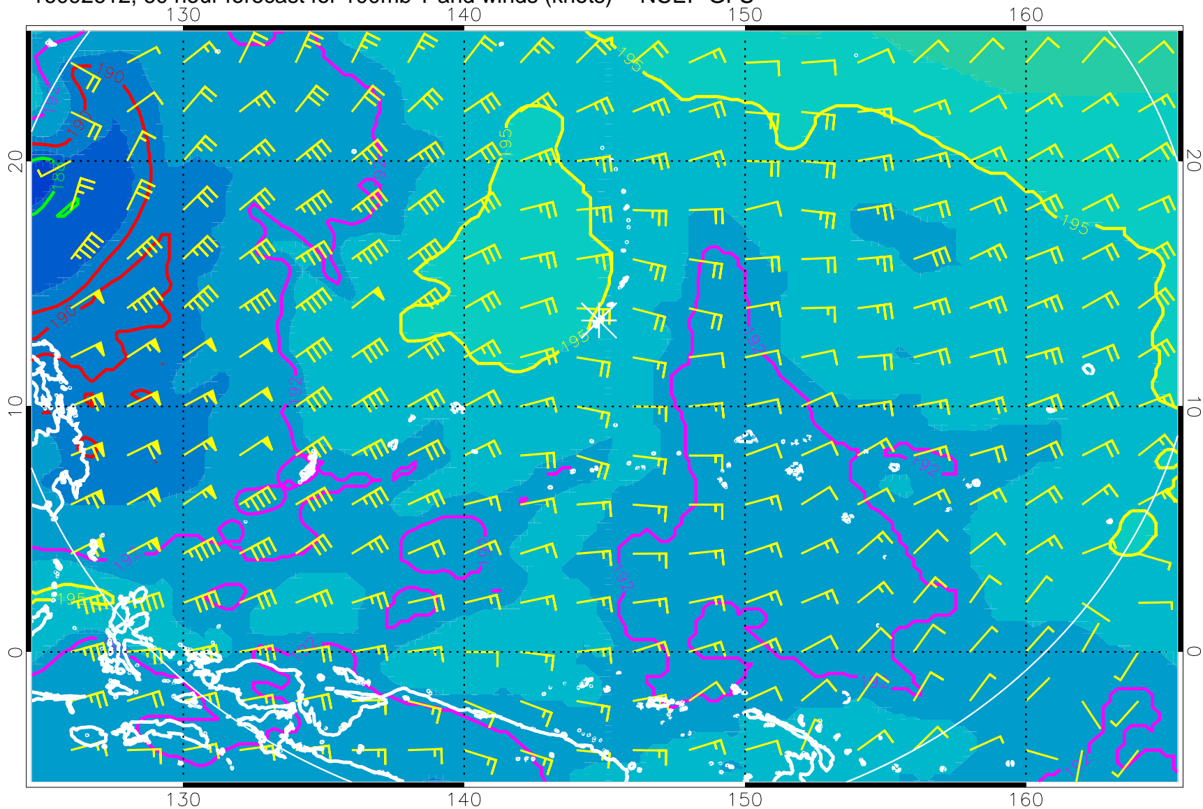
16092612, 60 hour forecast for 100mb T and winds (knots) -- NCEP GFS
