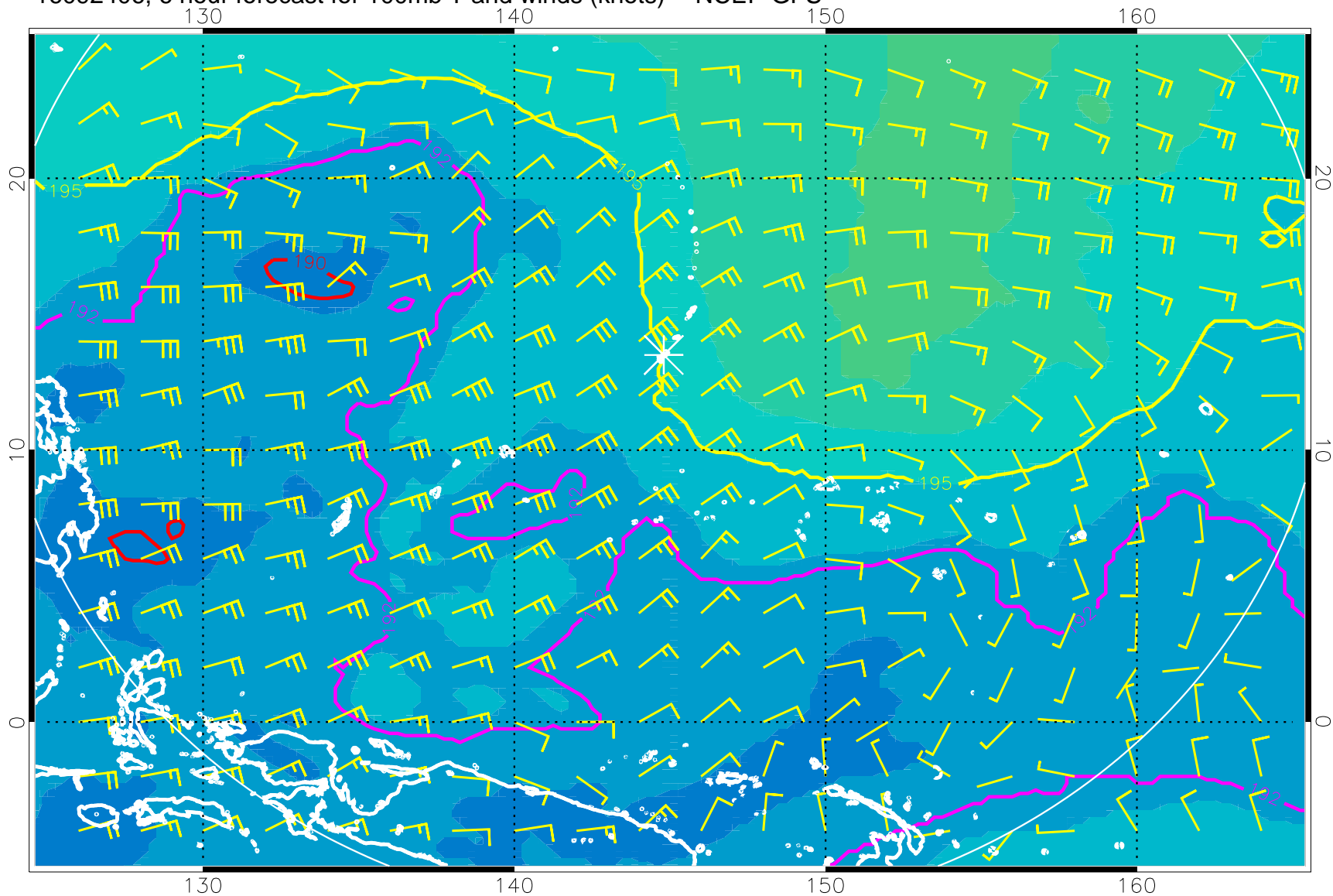
16092406, 6 hour forecast for 100mb T and winds (knots) -- NCEP GFS
