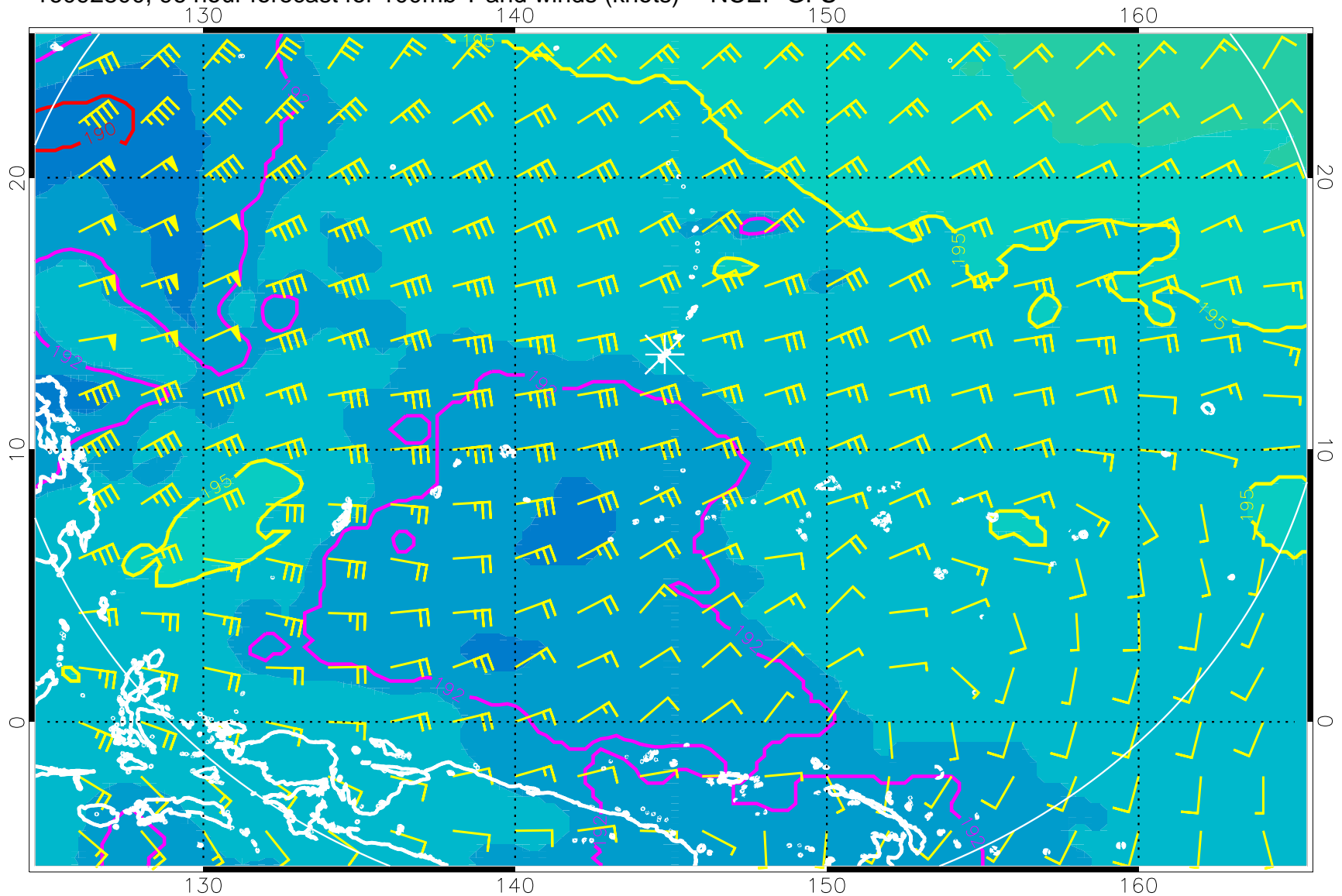
16092800, 96 hour forecast for 100mb T and winds (knots) -- NCEP GFS
