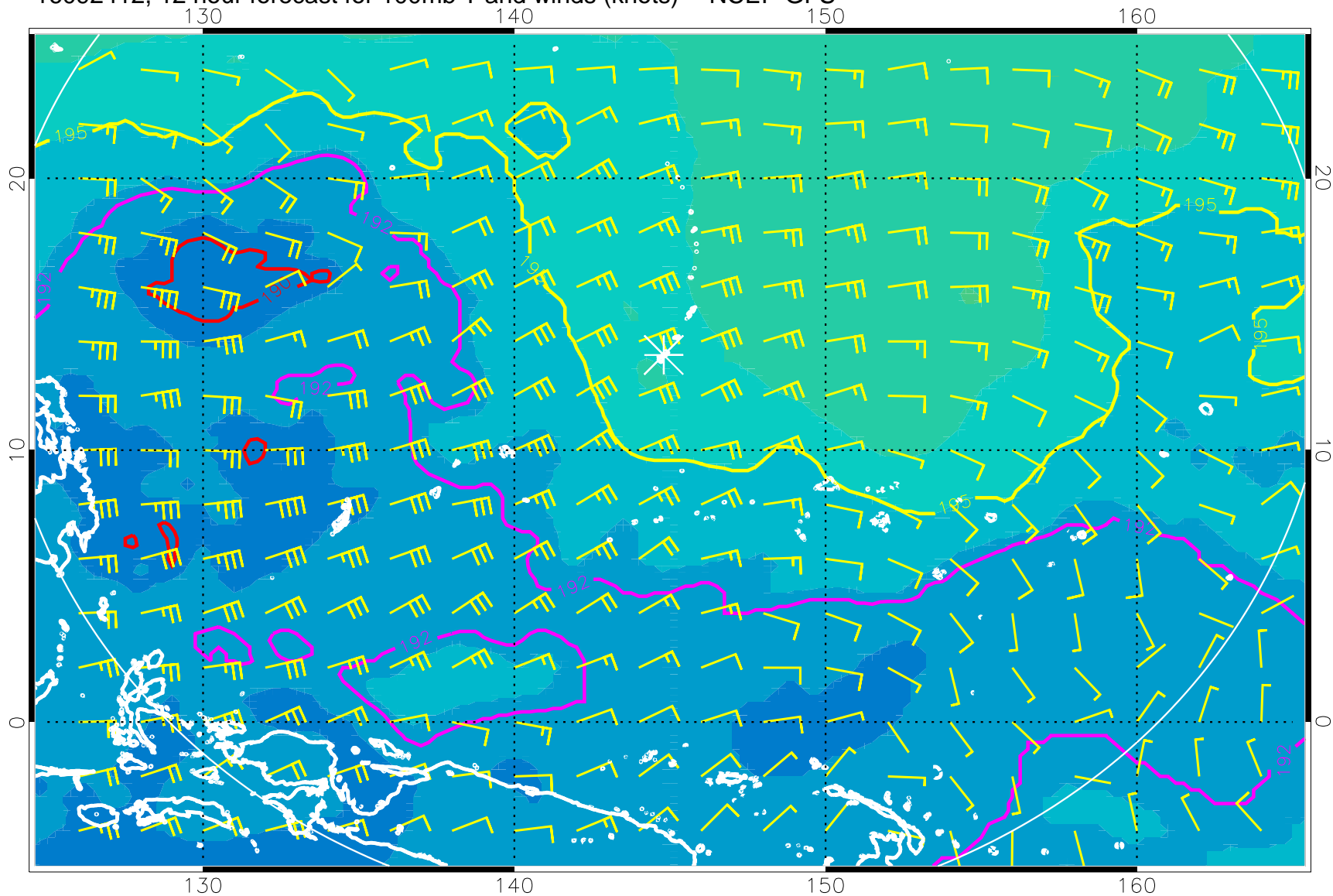
16092412, 12 hour forecast for 100mb T and winds (knots) -- NCEP GFS
