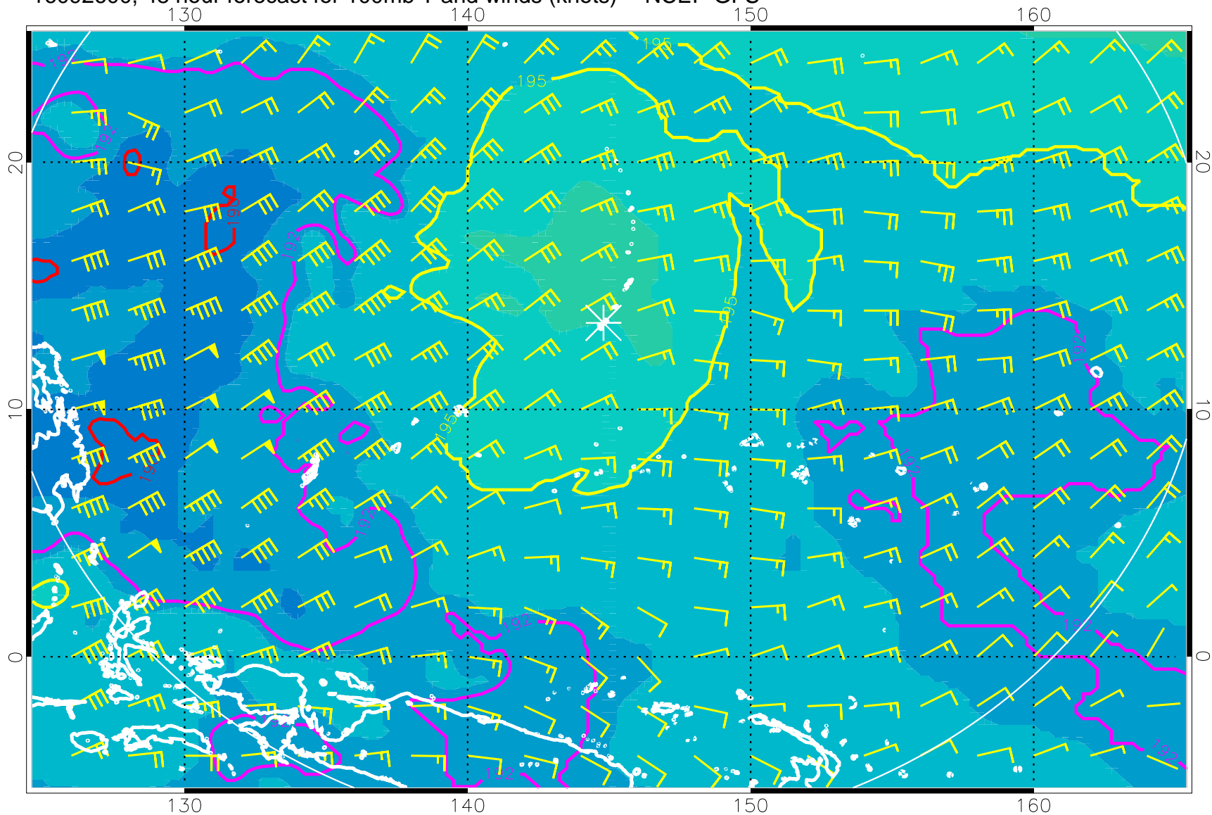
16092600, 48 hour forecast for 100mb T and winds (knots) -- NCEP GFS
