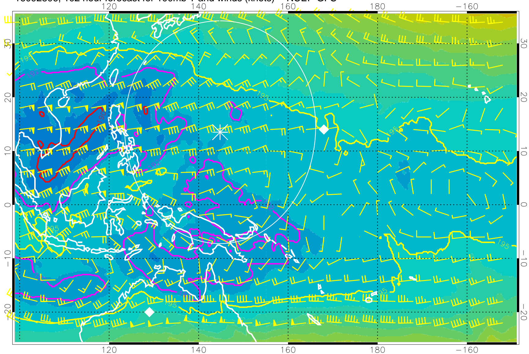
16092806, 102 hour forecast for 100mb T and winds (knots) -- NCEP GFS
