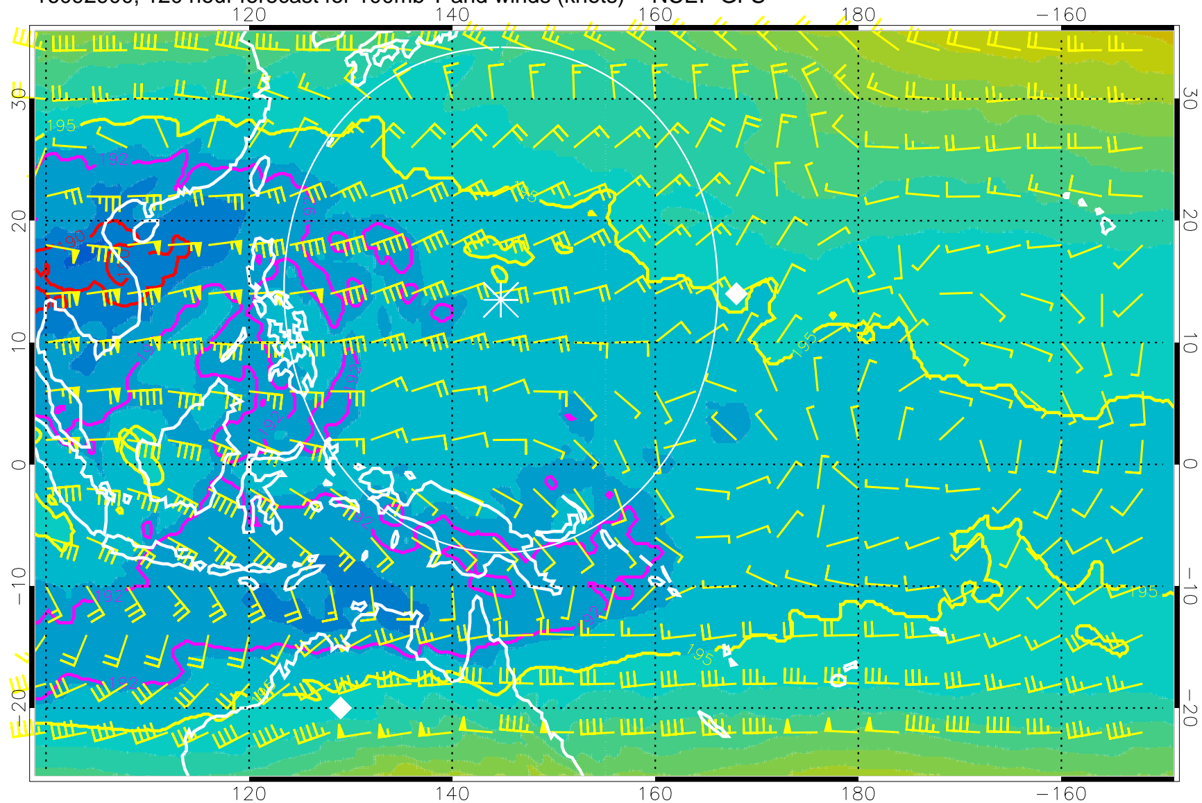
16092900, 120 hour forecast for 100mb T and winds (knots) -- NCEP GFS
