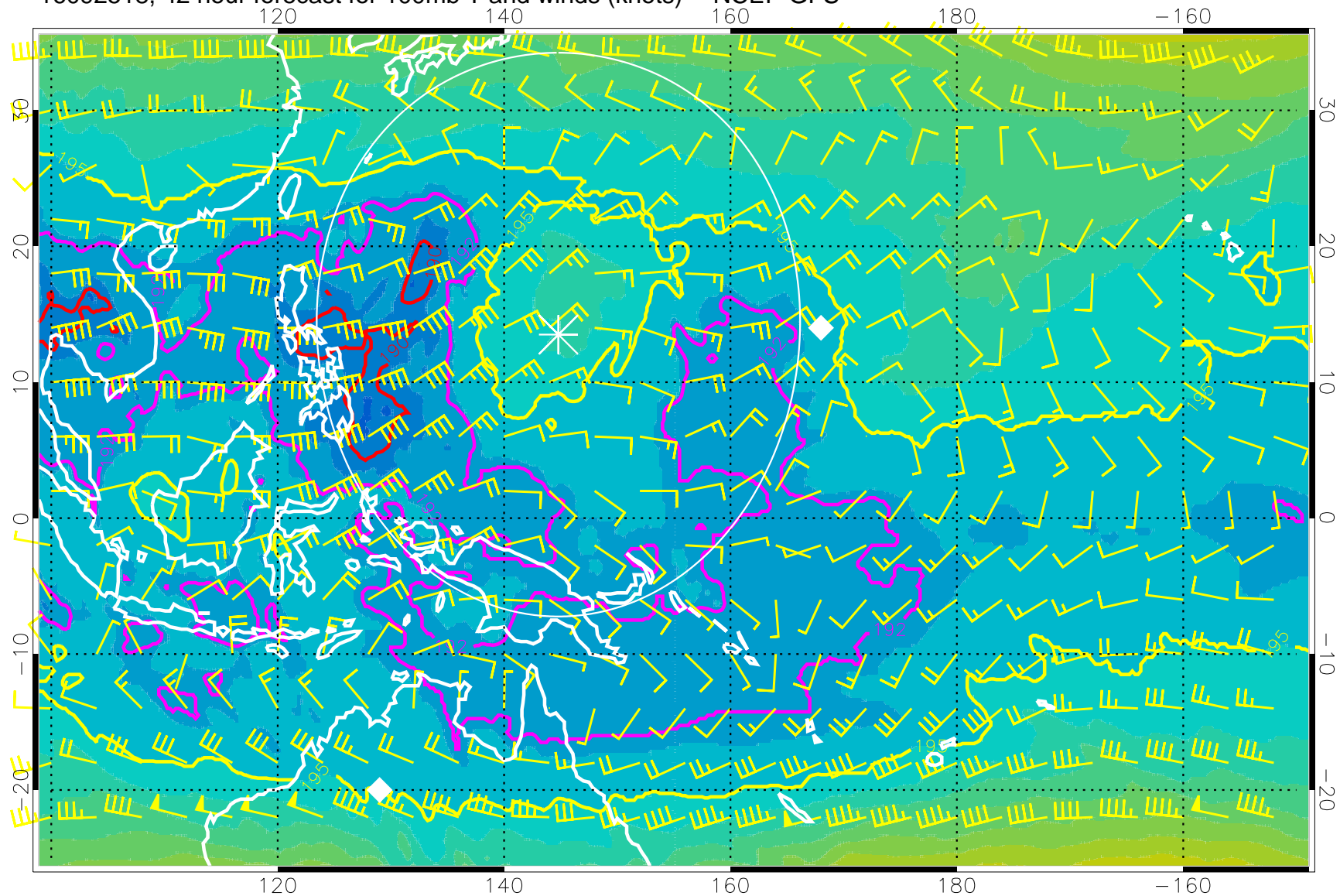
16092518, 42 hour forecast for 100mb T and winds (knots) -- NCEP GFS
