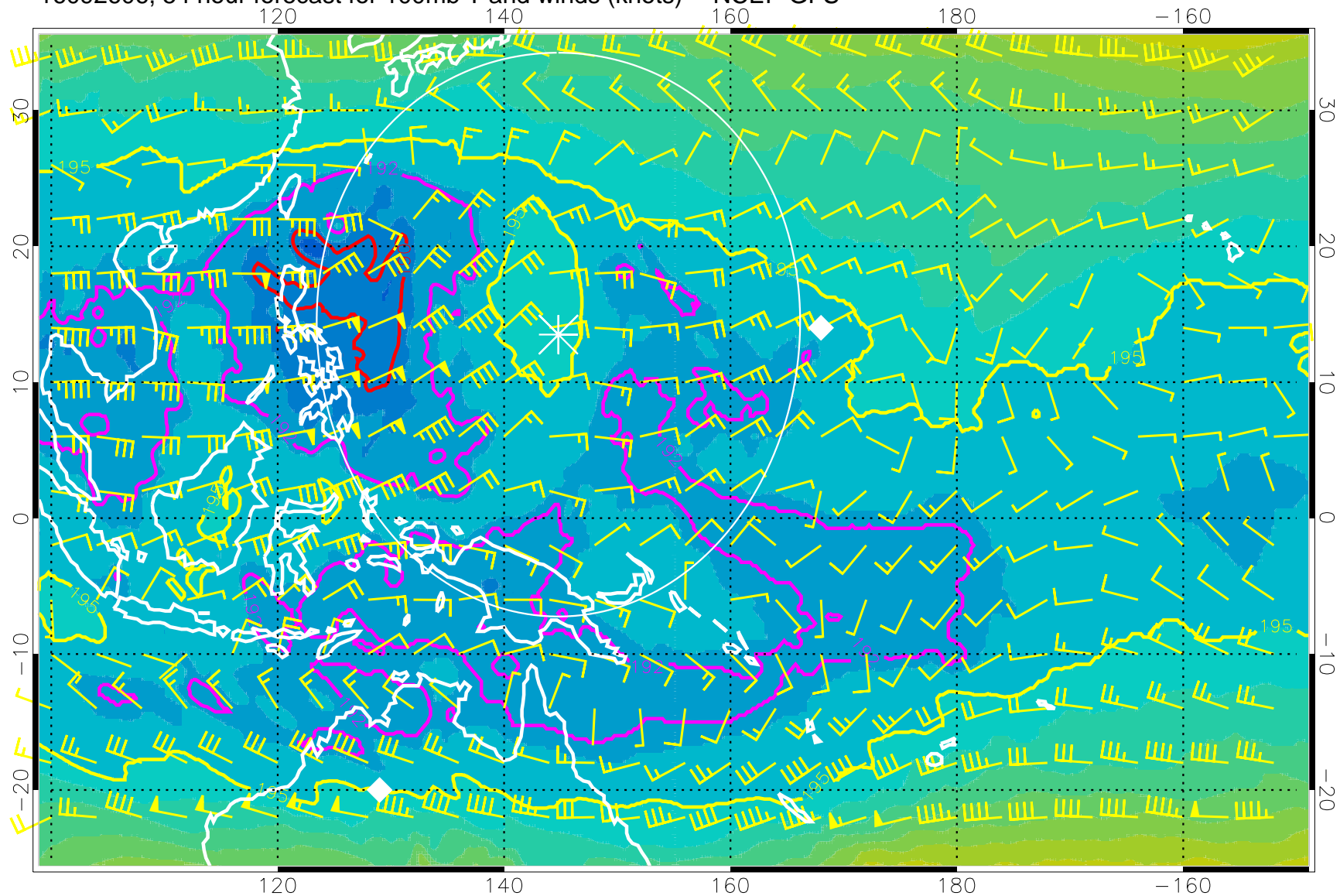
16092606, 54 hour forecast for 100mb T and winds (knots) -- NCEP GFS
