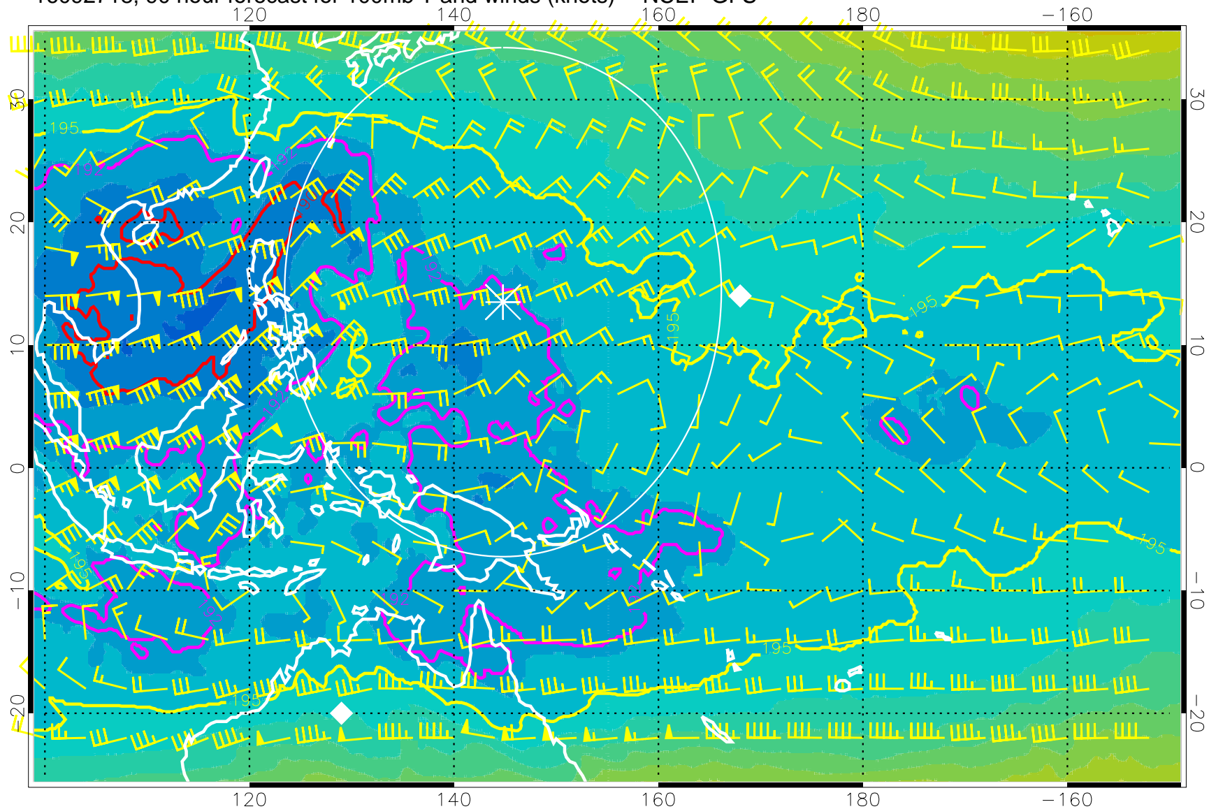
16092718, 90 hour forecast for 100mb T and winds (knots) -- NCEP GFS
