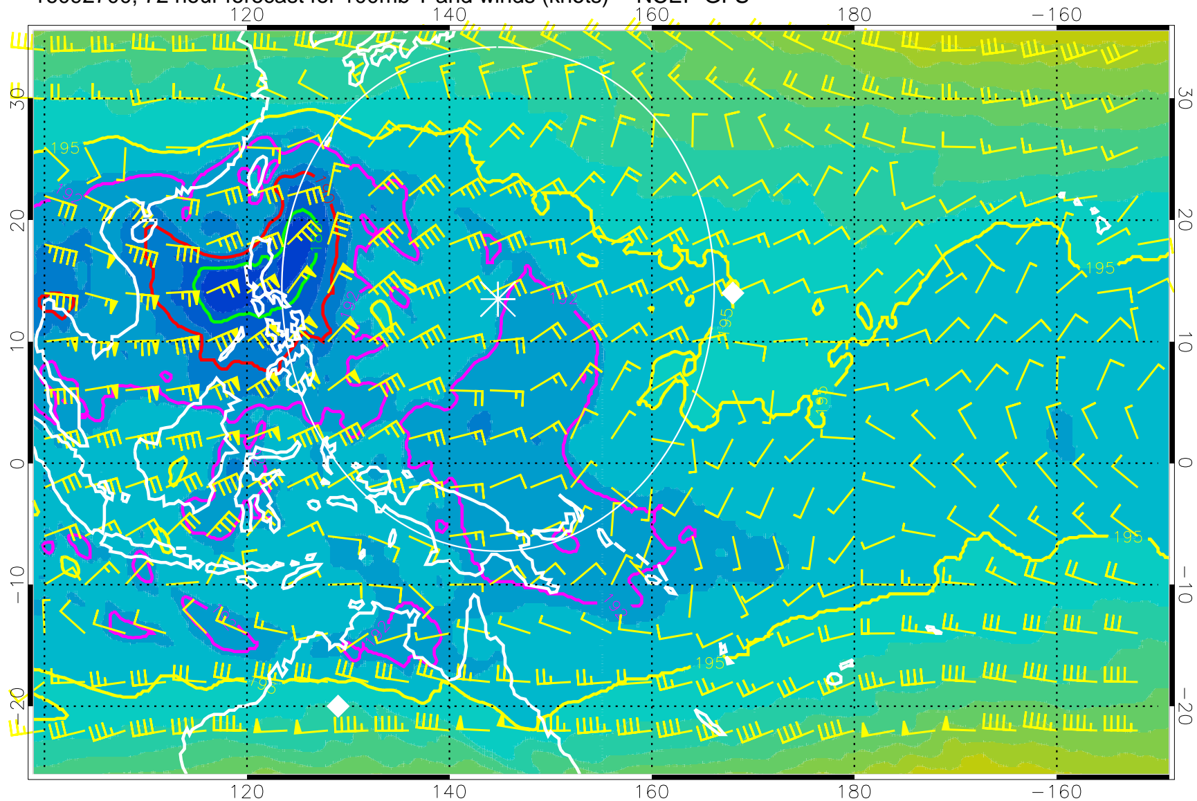
16092700, 72 hour forecast for 100mb T and winds (knots) -- NCEP GFS
