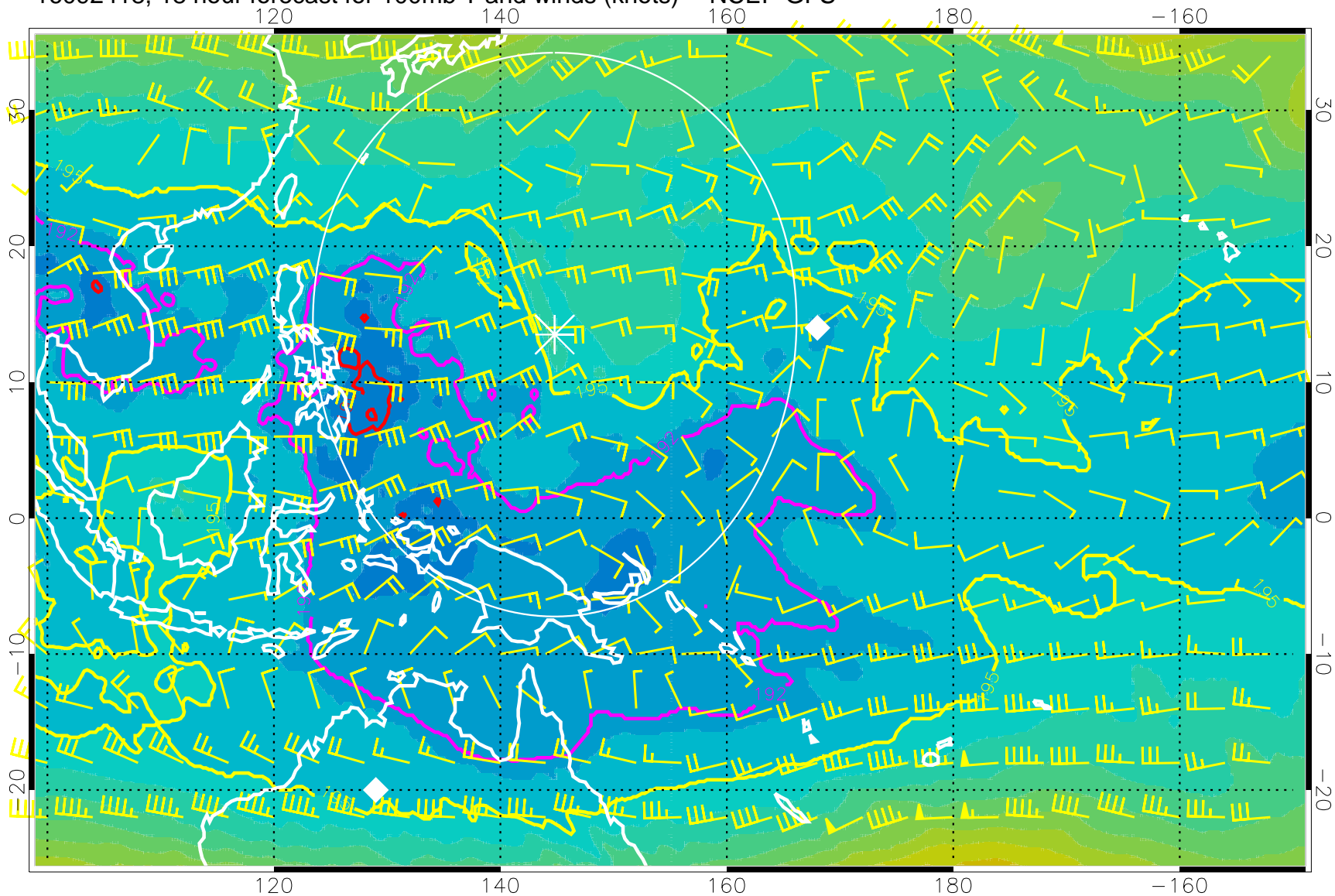
16092418, 18 hour forecast for 100mb T and winds (knots) -- NCEP GFS
