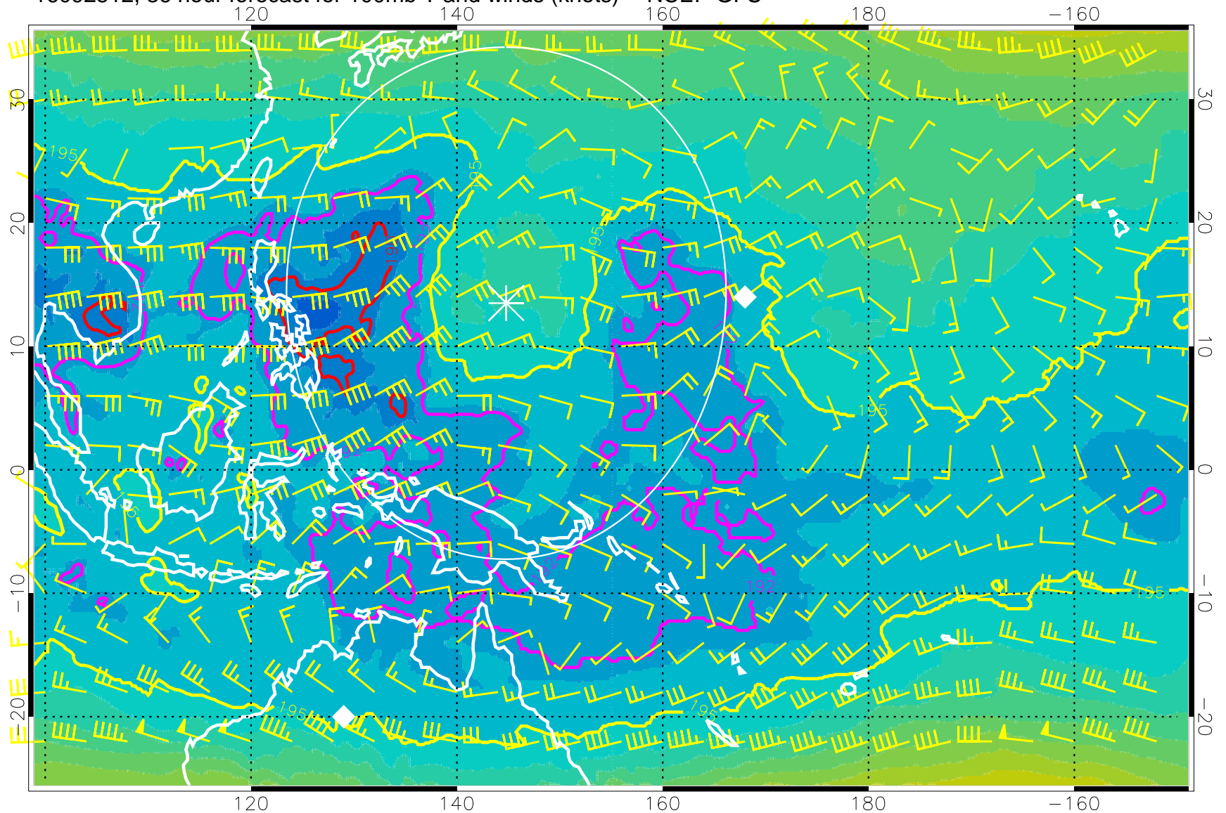
16092512, 36 hour forecast for 100mb T and winds (knots) -- NCEP GFS
