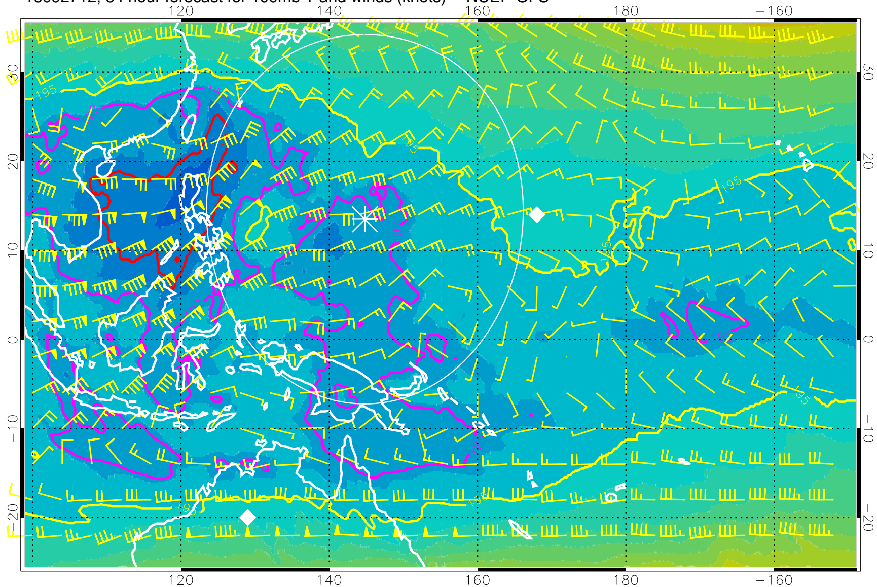
16092712, 84 hour forecast for 100mb T and winds (knots) -- NCEP GFS
