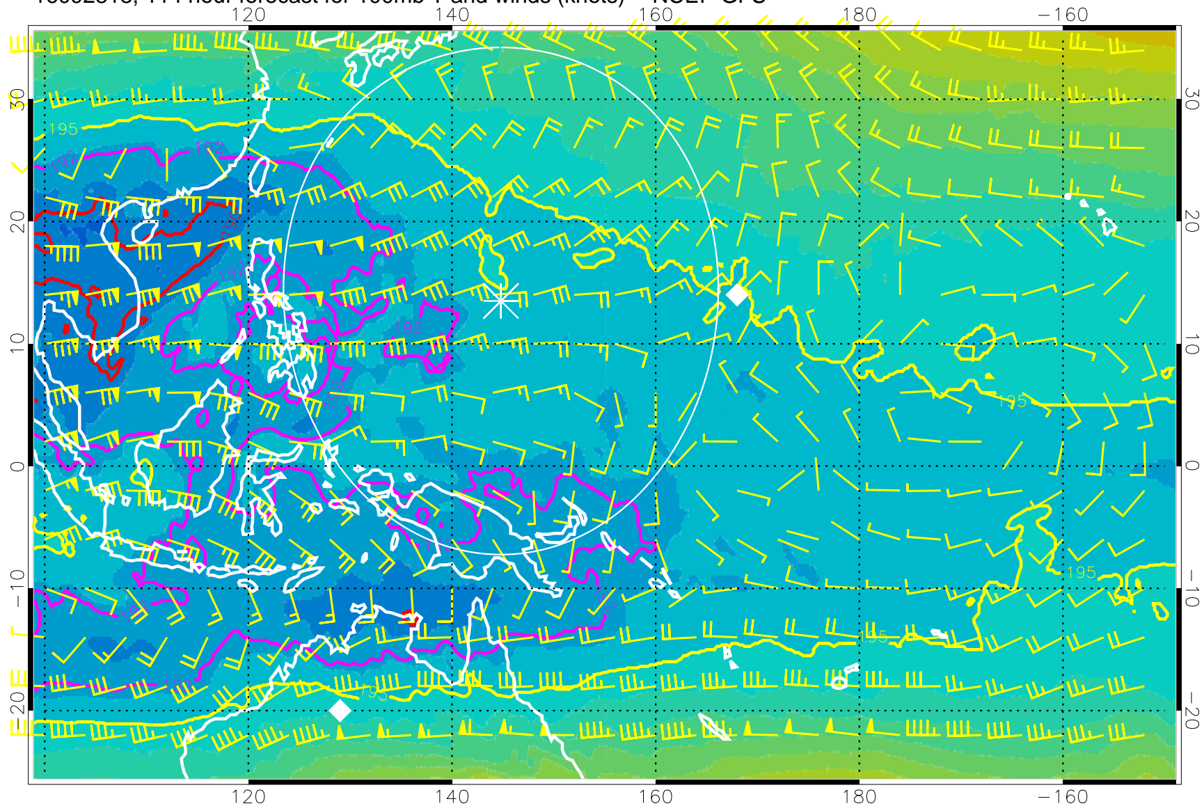
16092818, 114 hour forecast for 100mb T and winds (knots) -- NCEP GFS
