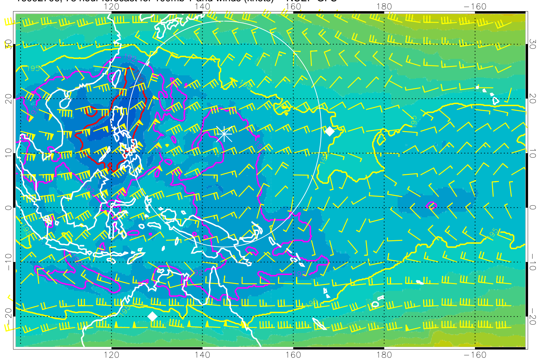
16092706, 78 hour forecast for 100mb T and winds (knots) -- NCEP GFS
