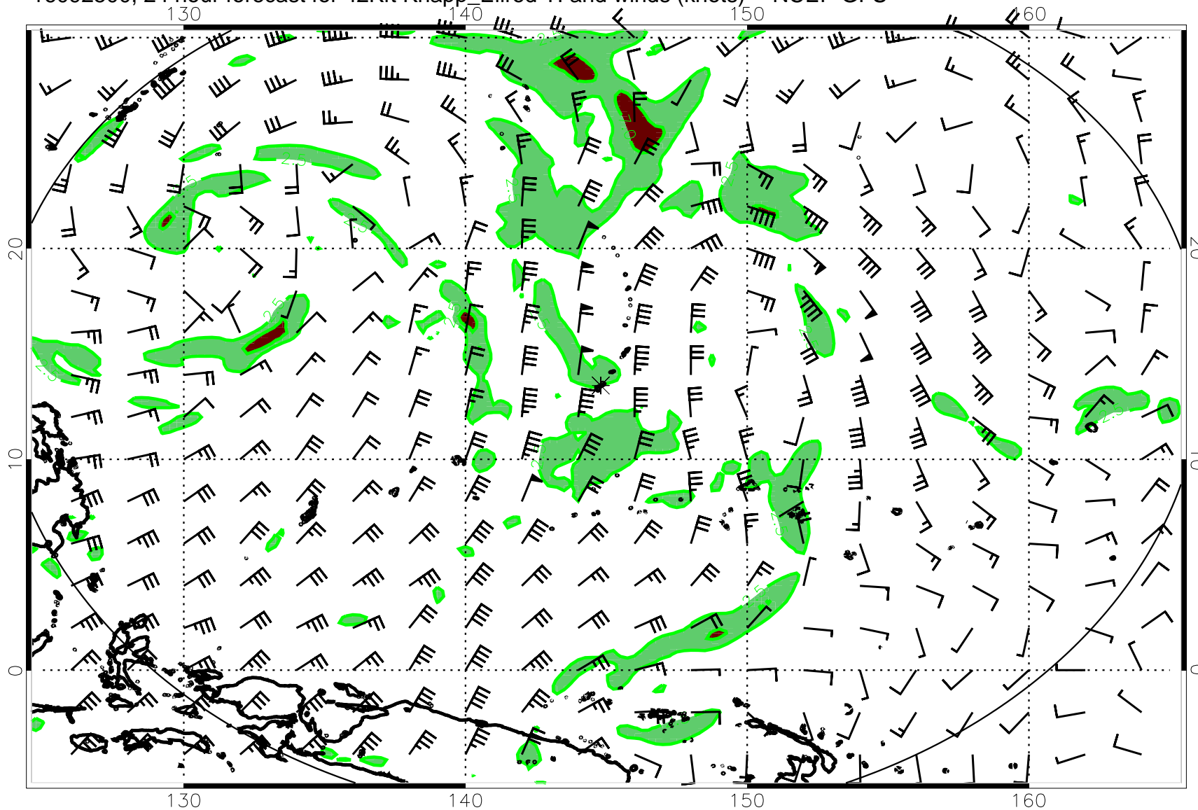
16092500, 24 hour forecast for 42Kft Knapp_Ellrod TI and winds (knots) -- NCEP GFS
