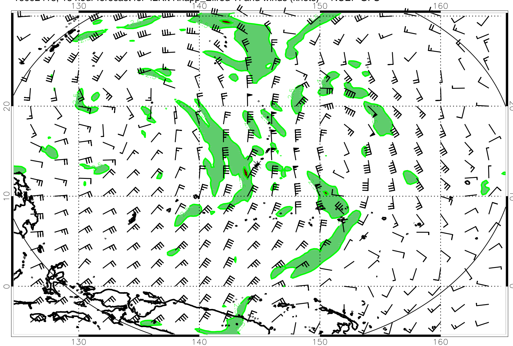
16092418, 18 hour forecast for 42Kft Knapp_Ellrod TI and winds (knots) -- NCEP GFS
