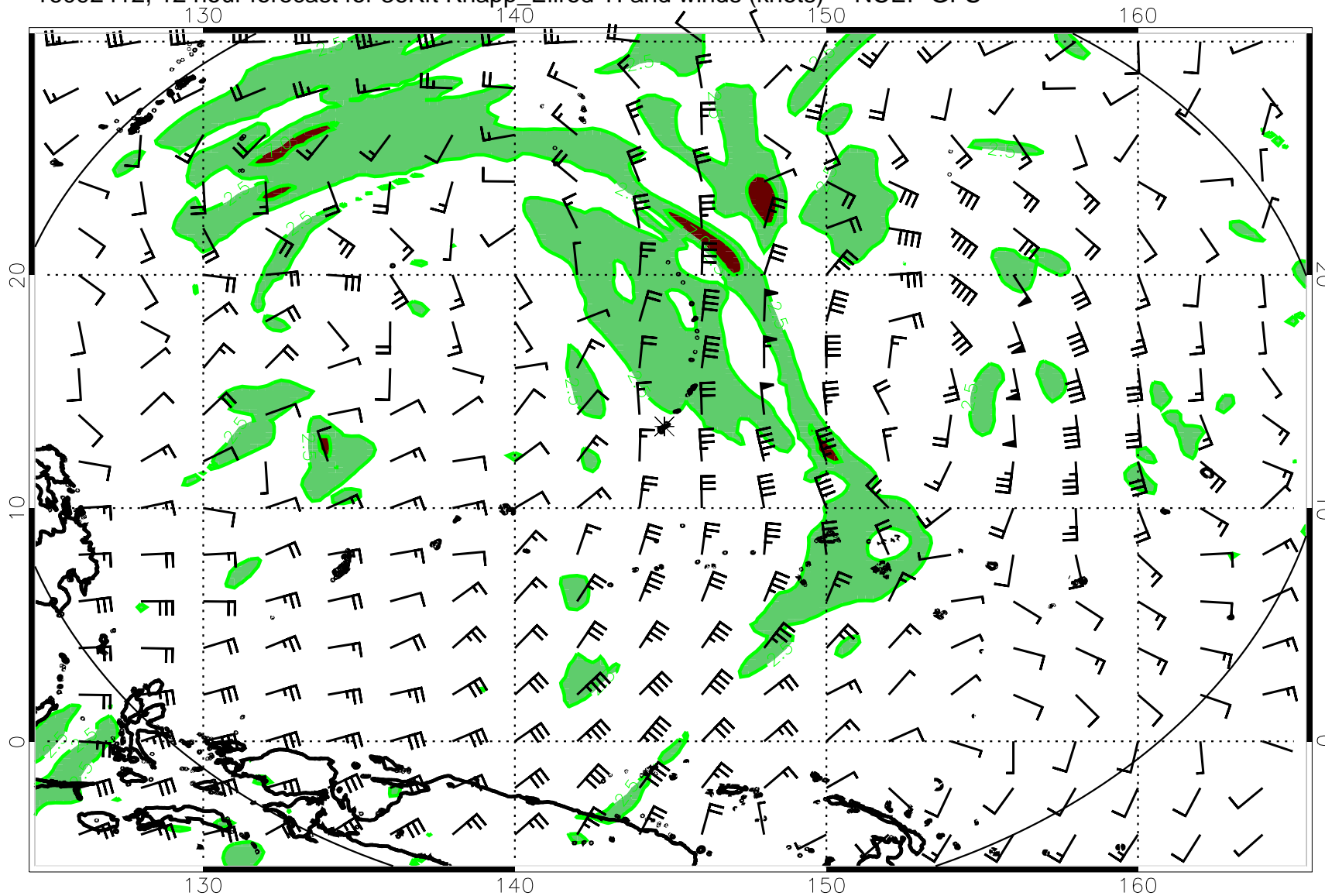
16092412, 12 hour forecast for 36Kft Knapp_Ellrod TI and winds (knots) -- NCEP GFS
