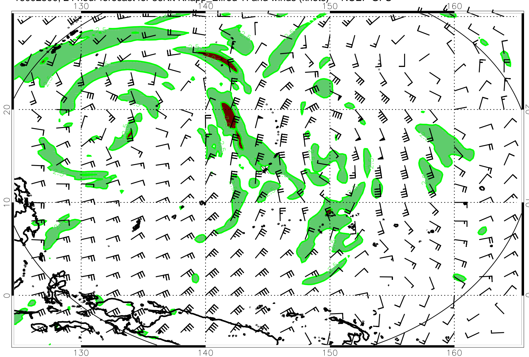
16092500, 24 hour forecast for 36Kft Knapp_Ellrod TI and winds (knots) -- NCEP GFS
