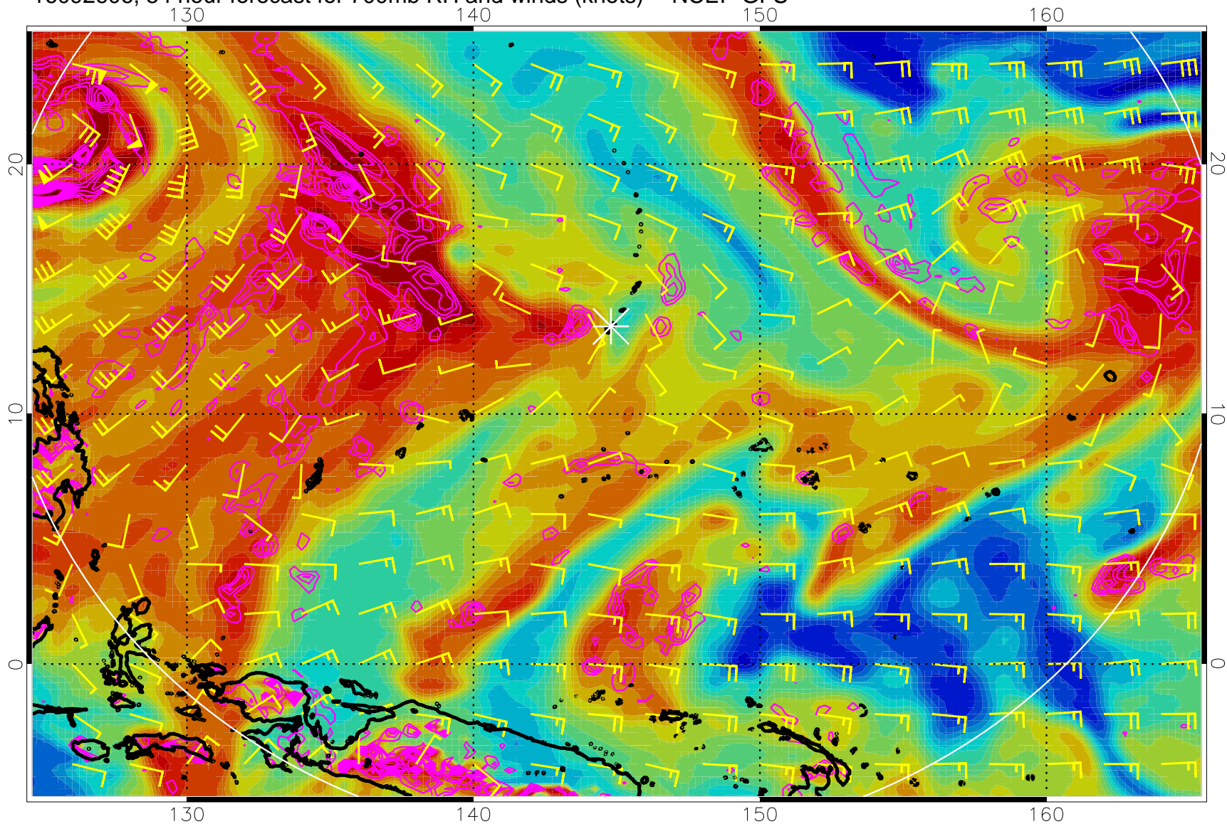
16092606, 54 hour forecast for 700mb RH and winds (knots) -- NCEP GFS
