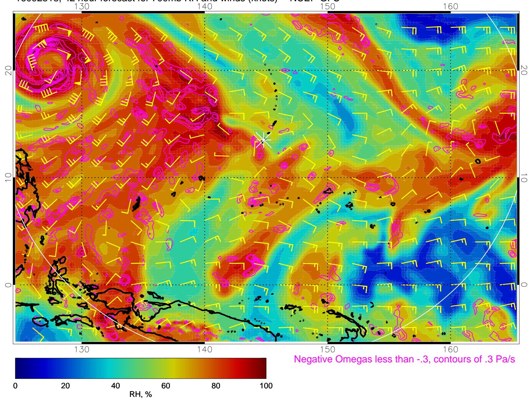
16092518, 42 hour forecast for 700mb RH and winds (knots) -- NCEP GFS
