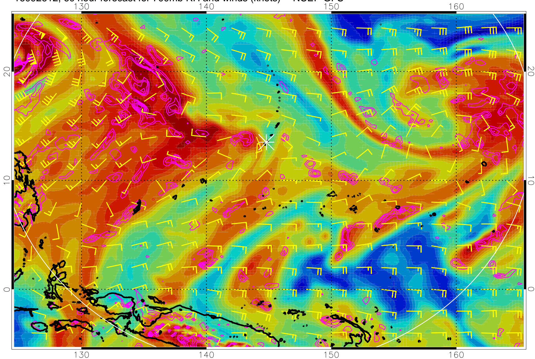
16092612, 60 hour forecast for 700mb RH and winds (knots) -- NCEP GFS
