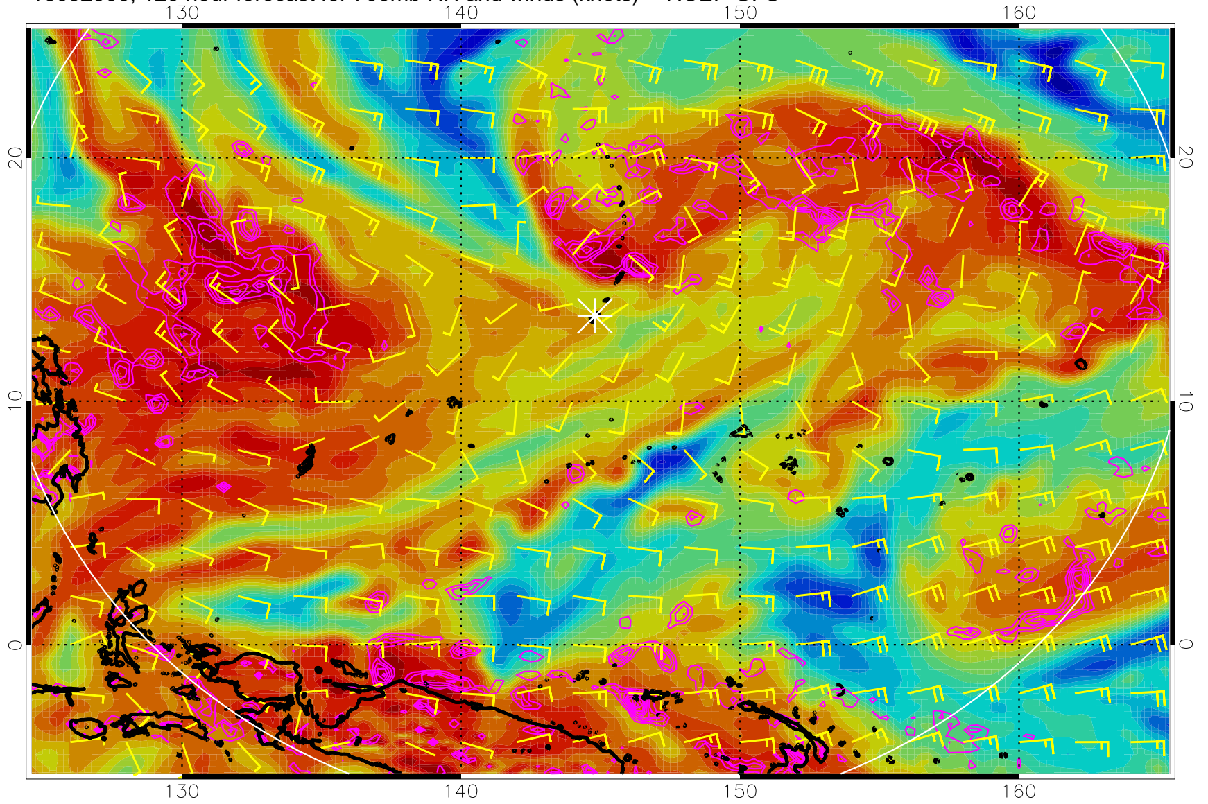
16092900, 120 hour forecast for 700mb RH and winds (knots) -- NCEP GFS
