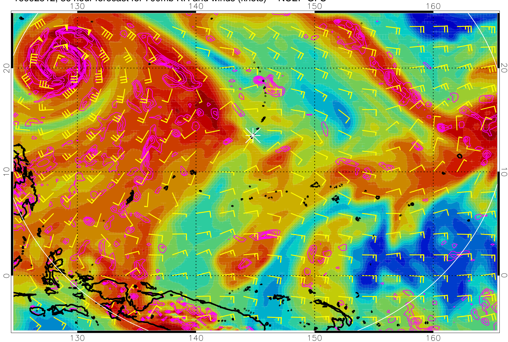
16092512, 36 hour forecast for 700mb RH and winds (knots) -- NCEP GFS
