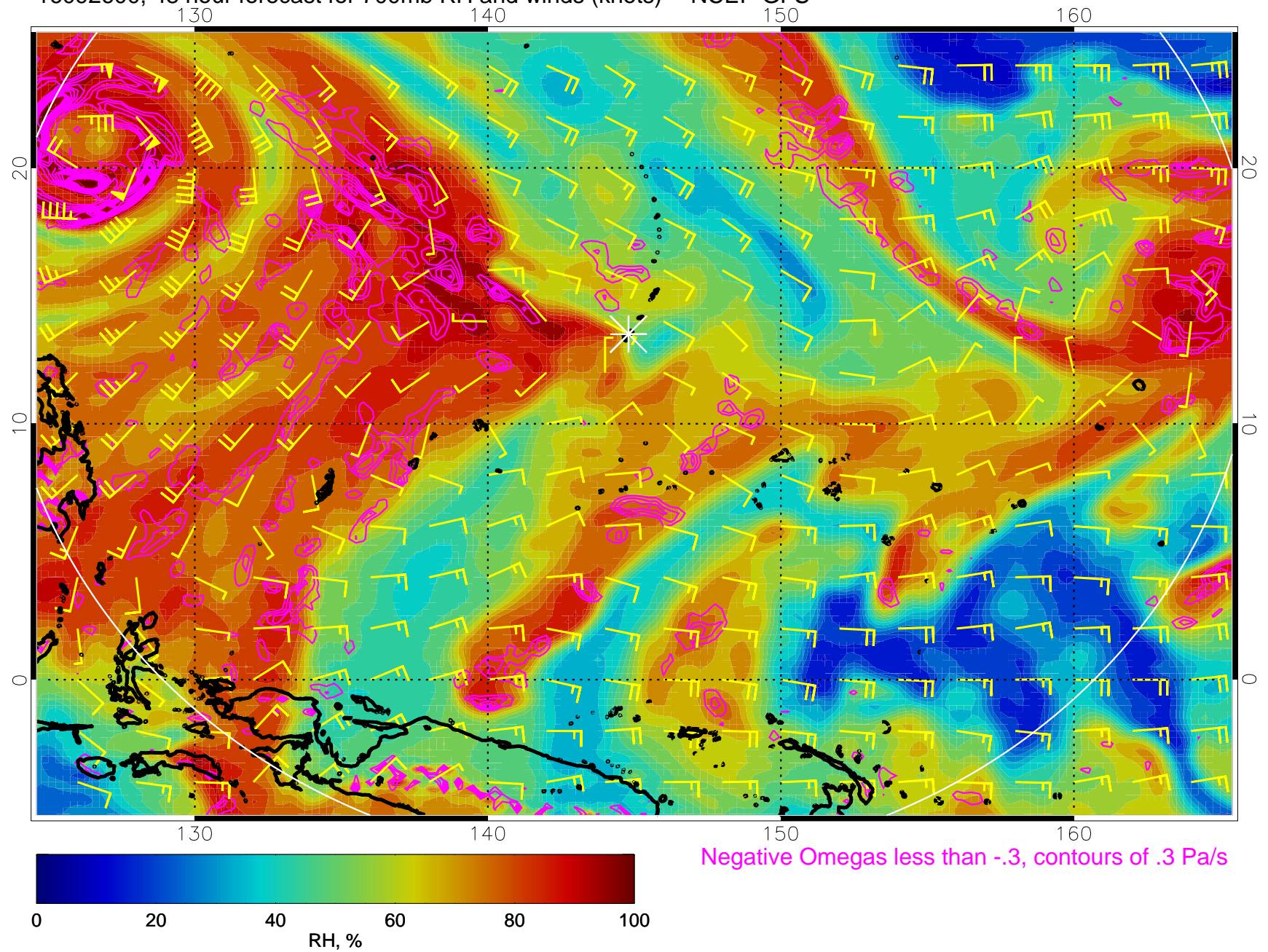
16092600, 48 hour forecast for 700mb RH and winds (knots) -- NCEP GFS
