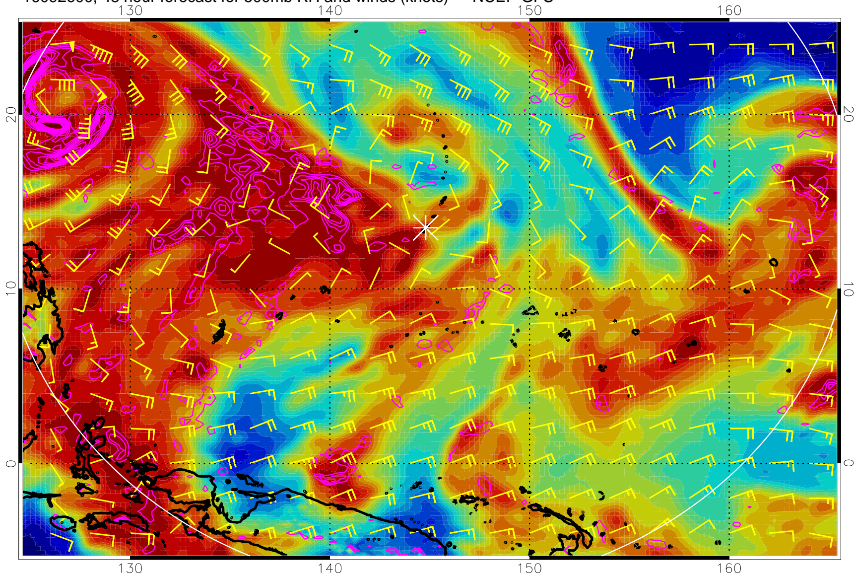
16092600, 48 hour forecast for 500mb RH and winds (knots) -- NCEP GFS
