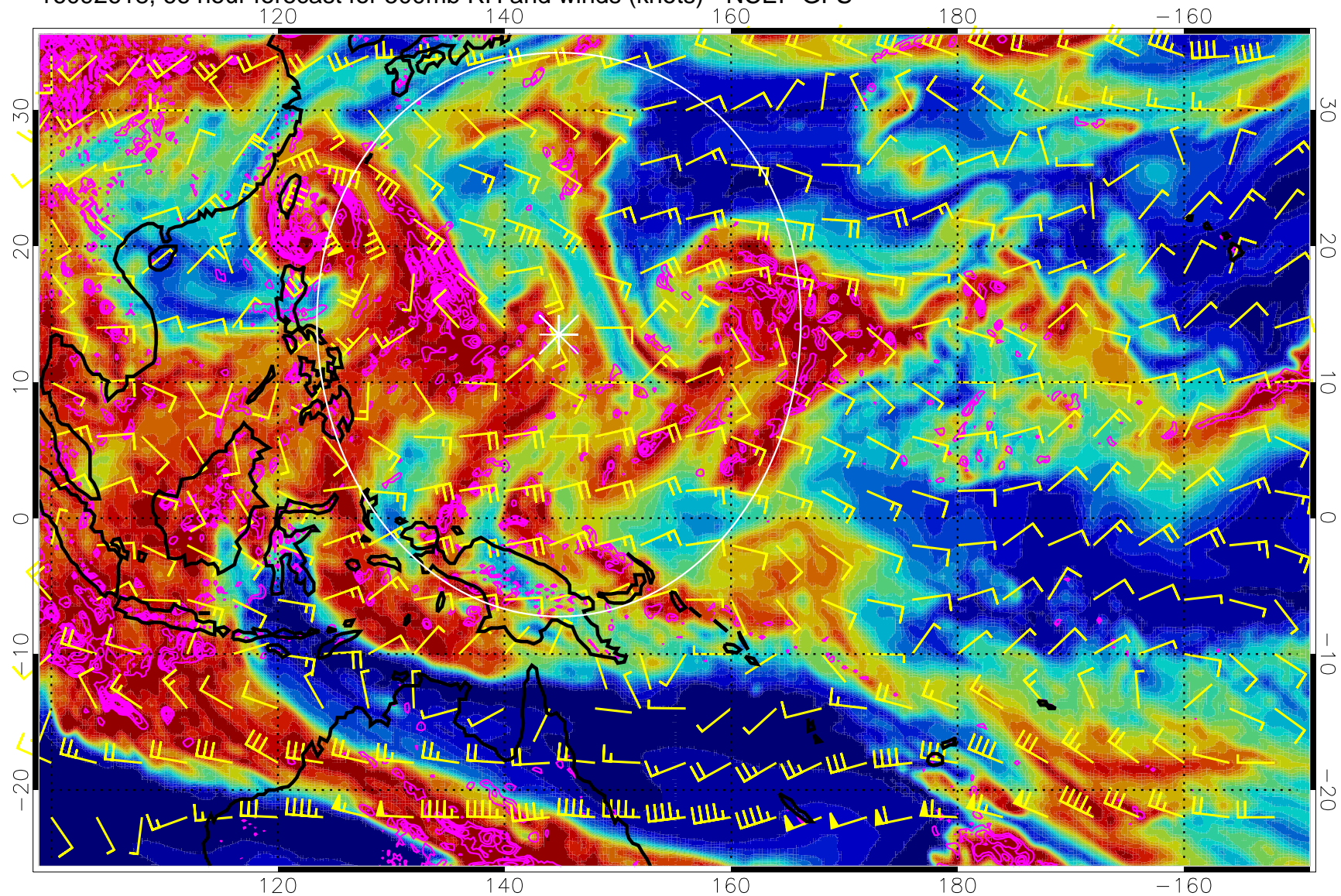
16092618, 66 hour forecast for 500mb RH and winds (knots) - NCEP GFS
