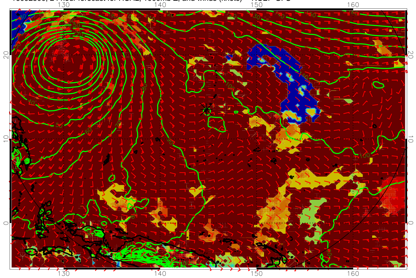
16092500, 24 hour forecast for HCAL, 1000mb Z, and winds (knots) -- NCEP GFS
