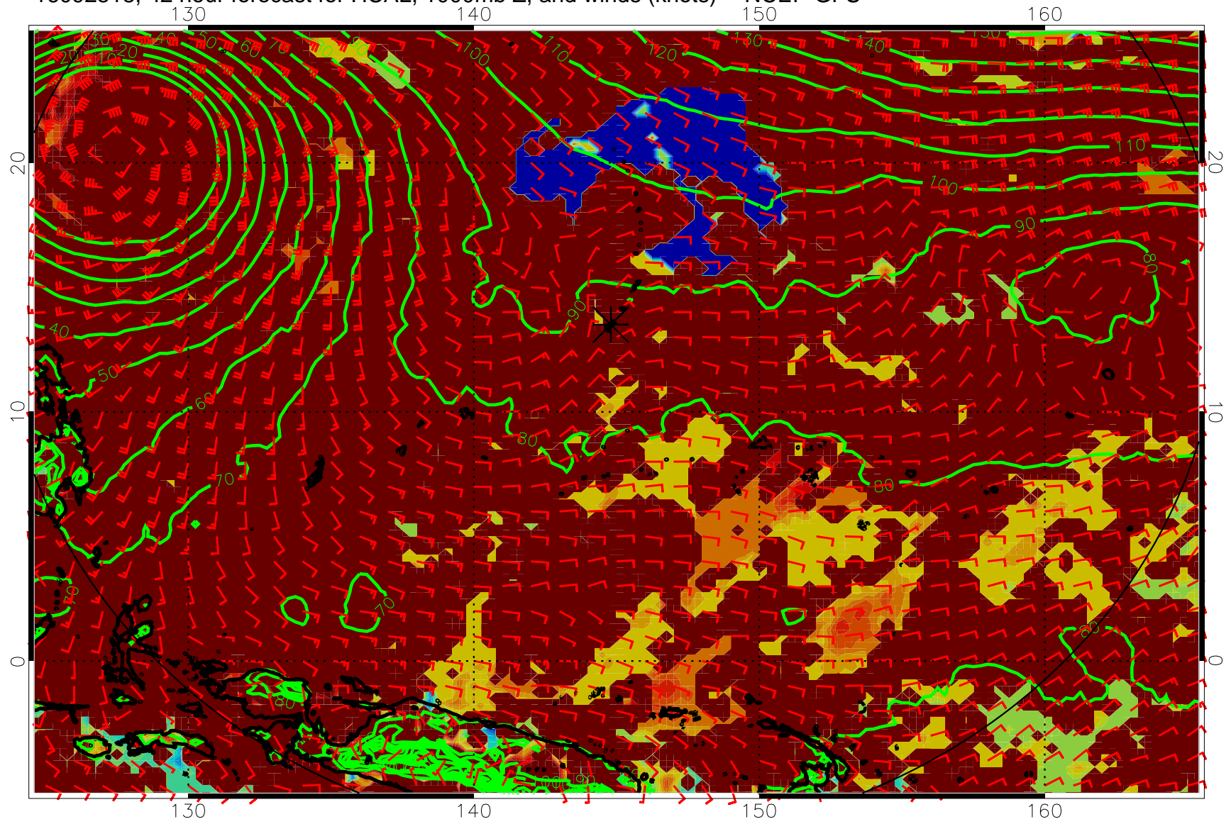
16092518, 42 hour forecast for HCAL, 1000mb Z, and winds (knots) -- NCEP GFS
