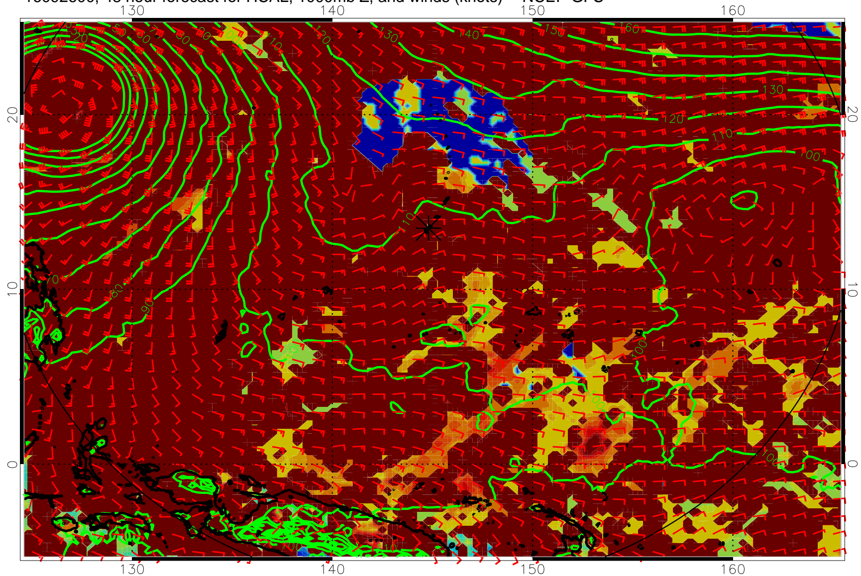
16092600, 48 hour forecast for HCAL, 1000mb Z, and winds (knots) -- NCEP GFS
