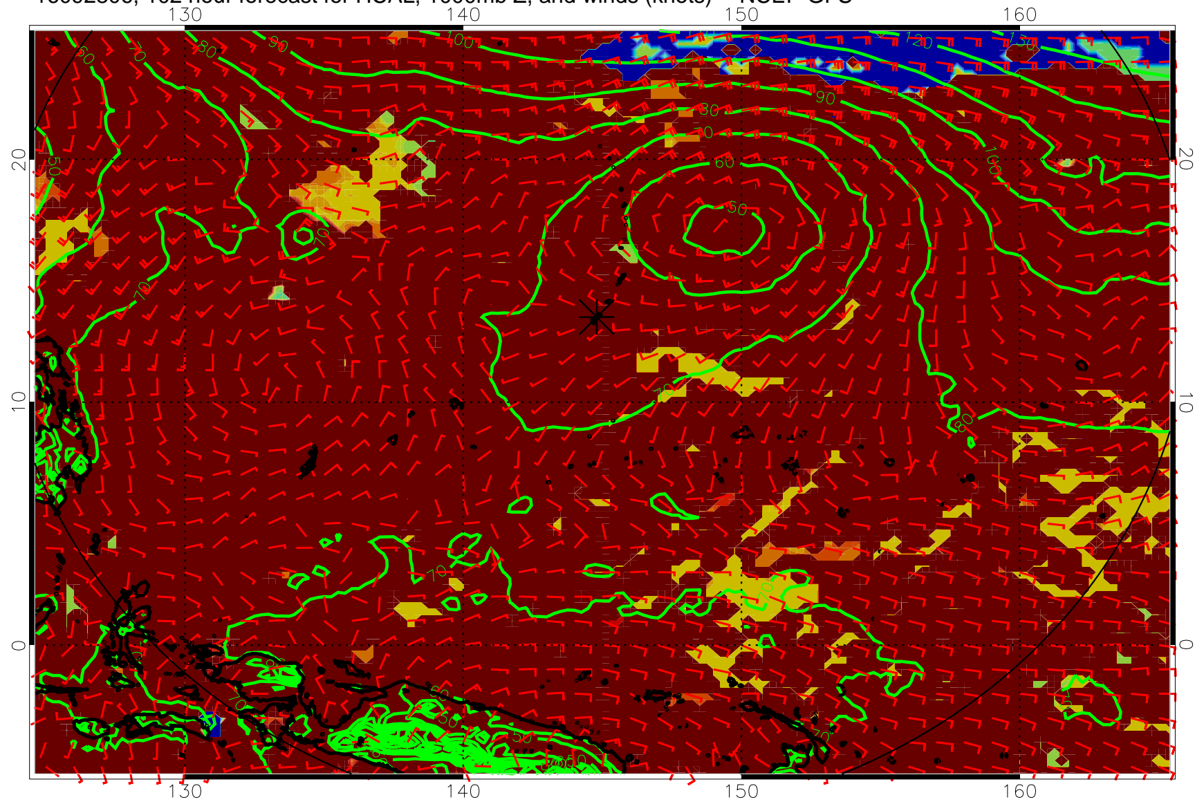
16092806, 102 hour forecast for HCAL, 1000mb Z, and winds (knots) -- NCEP GFS
