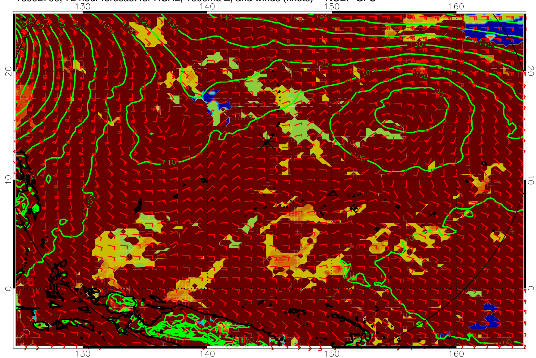
16092700, 72 hour forecast for HCAL, 1000mb Z, and winds (knots) -- NCEP GFS
