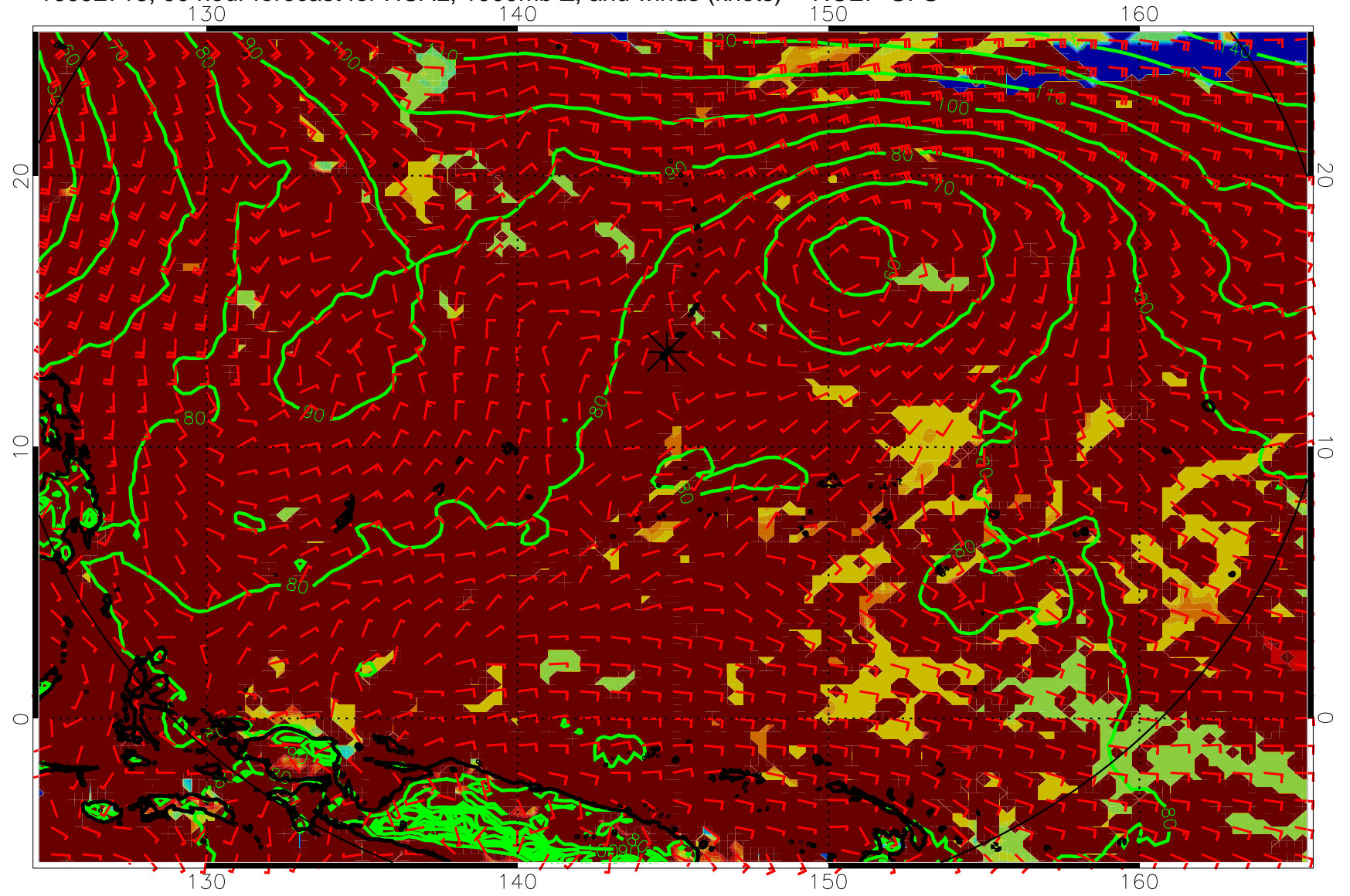
16092718, 90 hour forecast for HCAL, 1000mb Z, and winds (knots) -- NCEP GFS
