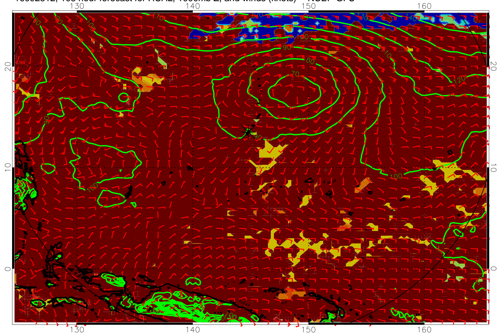
16092812, 108 hour forecast for HCAL, 1000mb Z, and winds (knots) -- NCEP GFS
