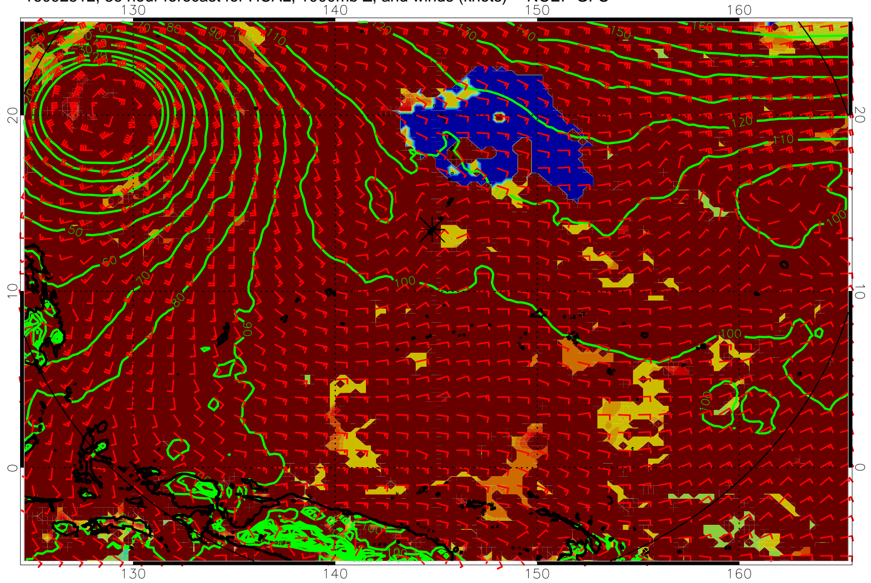
16092512, 36 hour forecast for HCAL, 1000mb Z, and winds (knots) -- NCEP GFS
