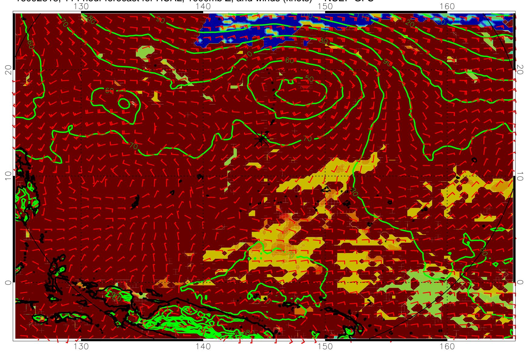
16092818, 114 hour forecast for HCAL, 1000mb Z, and winds (knots) -- NCEP GFS
