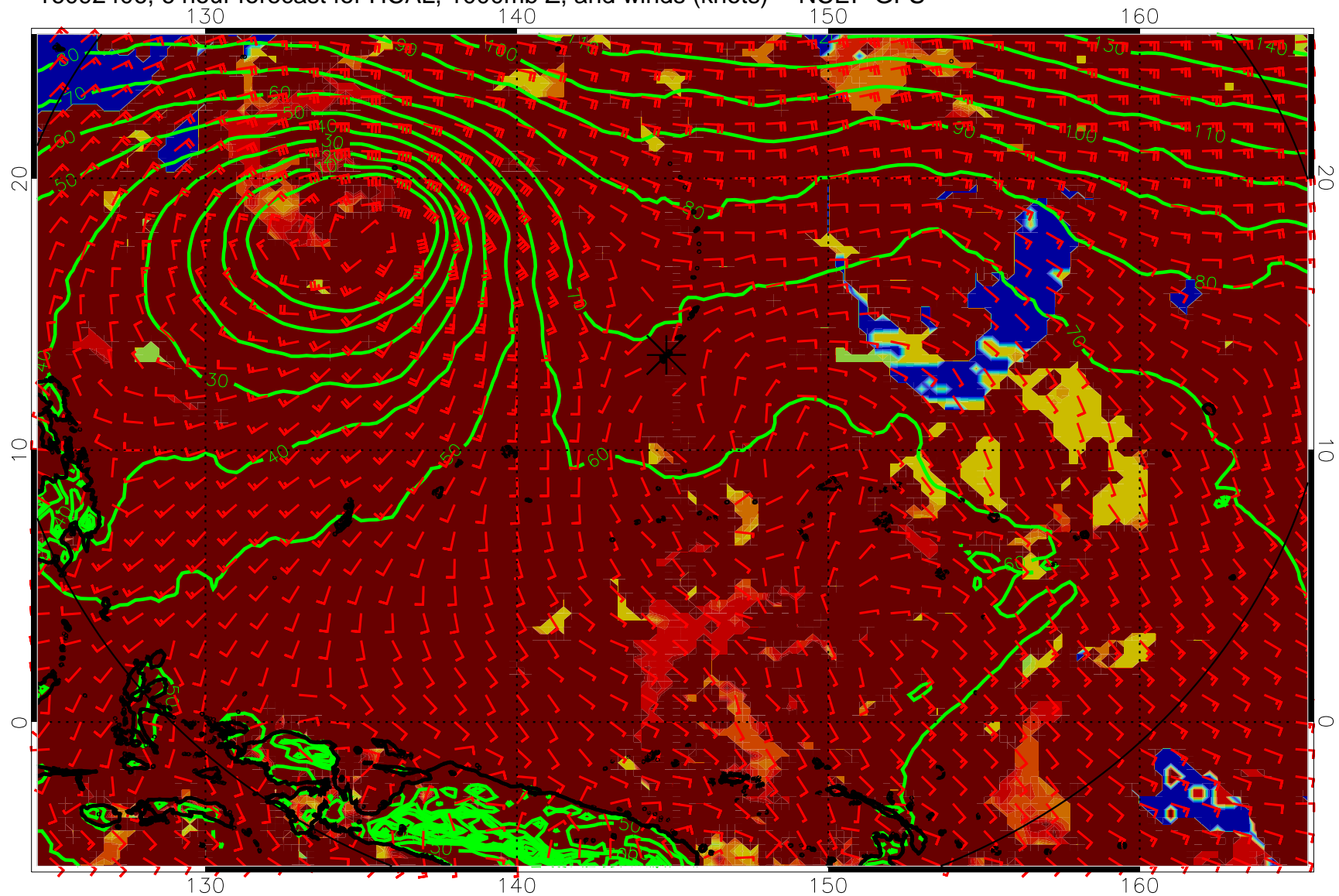
16092406, 6 hour forecast for HCAL, 1000mb Z, and winds (knots) -- NCEP GFS
