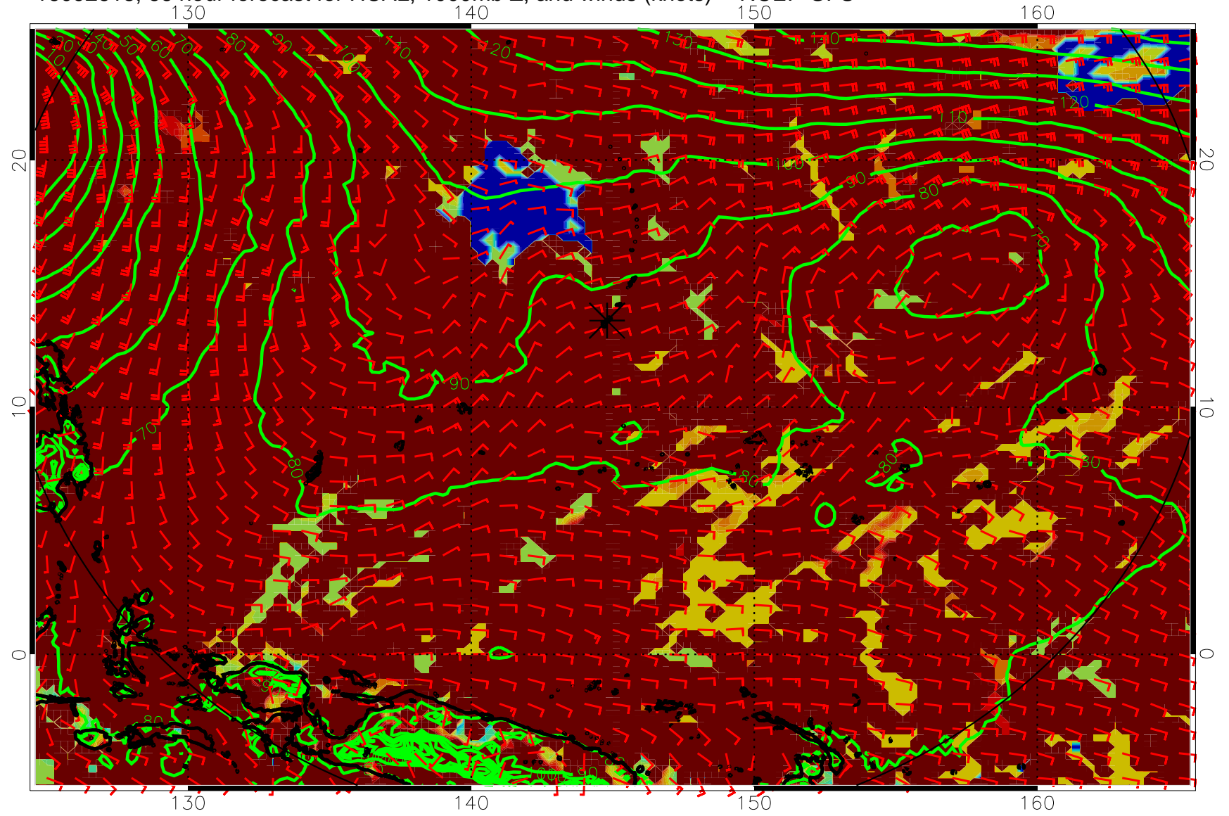
16092618, 66 hour forecast for HCAL, 1000mb Z, and winds (knots) -- NCEP GFS
