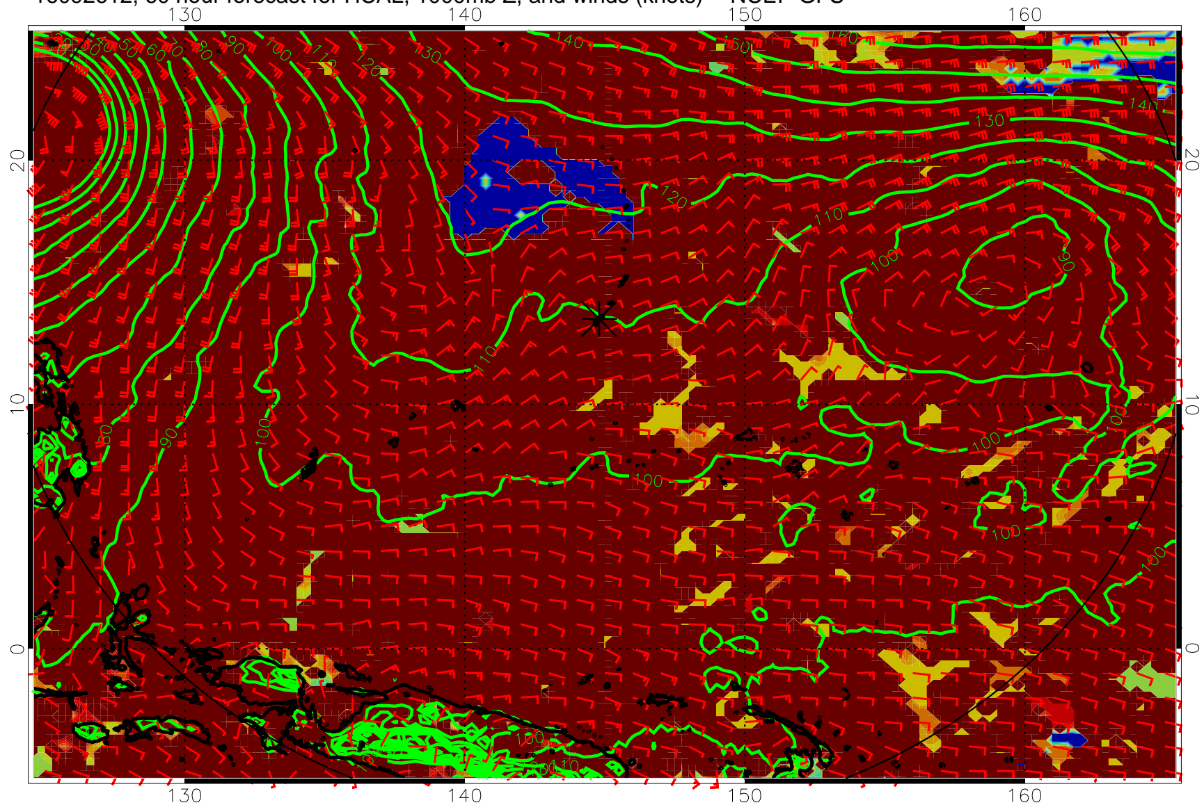
16092612, 60 hour forecast for HCAL, 1000mb Z, and winds (knots) -- NCEP GFS
