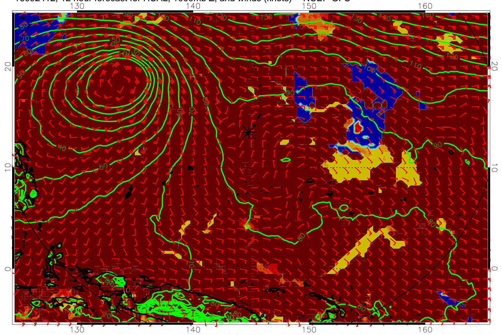
16092412, 12 hour forecast for HCAL, 1000mb Z, and winds (knots) -- NCEP GFS
