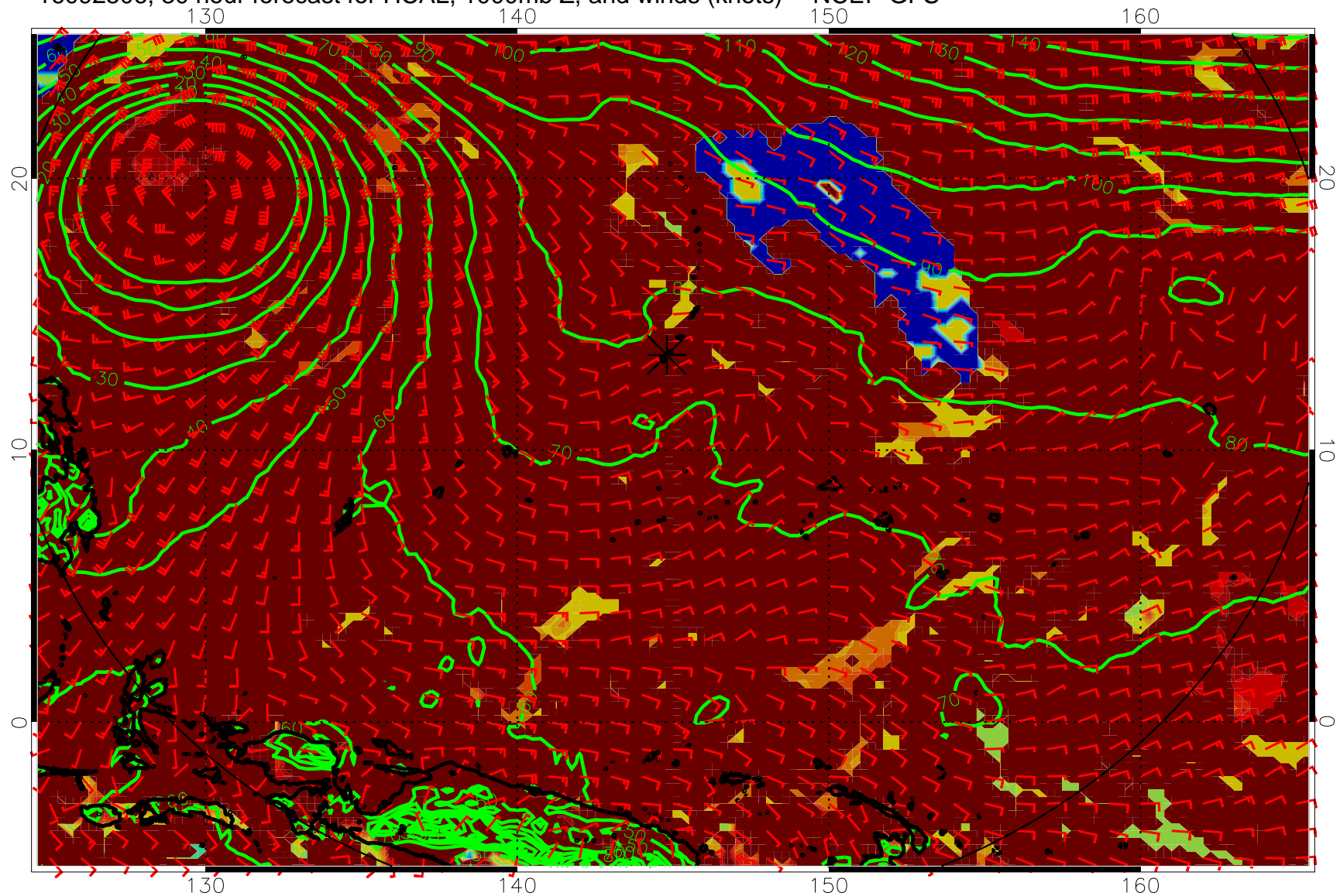
16092506, 30 hour forecast for HCAL, 1000mb Z, and winds (knots) -- NCEP GFS
