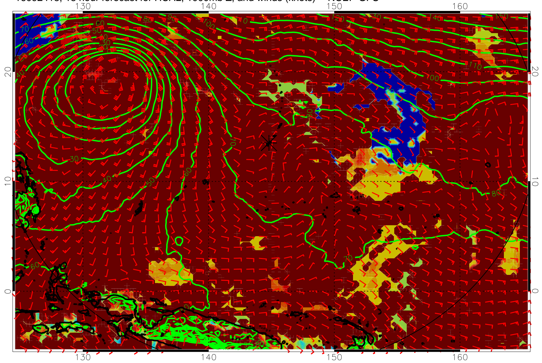
16092418, 18 hour forecast for HCAL, 1000mb Z, and winds (knots) -- NCEP GFS
