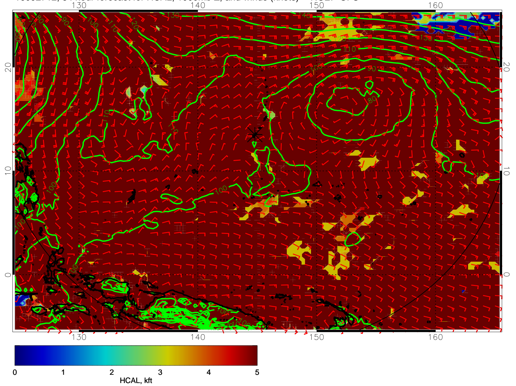
16092712, 84 hour forecast for HCAL, 1000mb Z, and winds (knots) -- NCEP GFS
