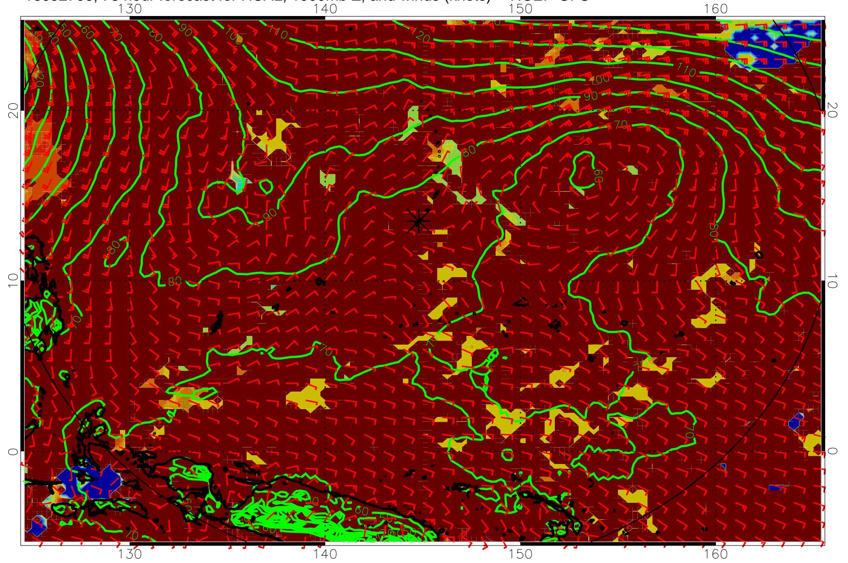
16092706, 78 hour forecast for HCAL, 1000mb Z, and winds (knots) -- NCEP GFS
