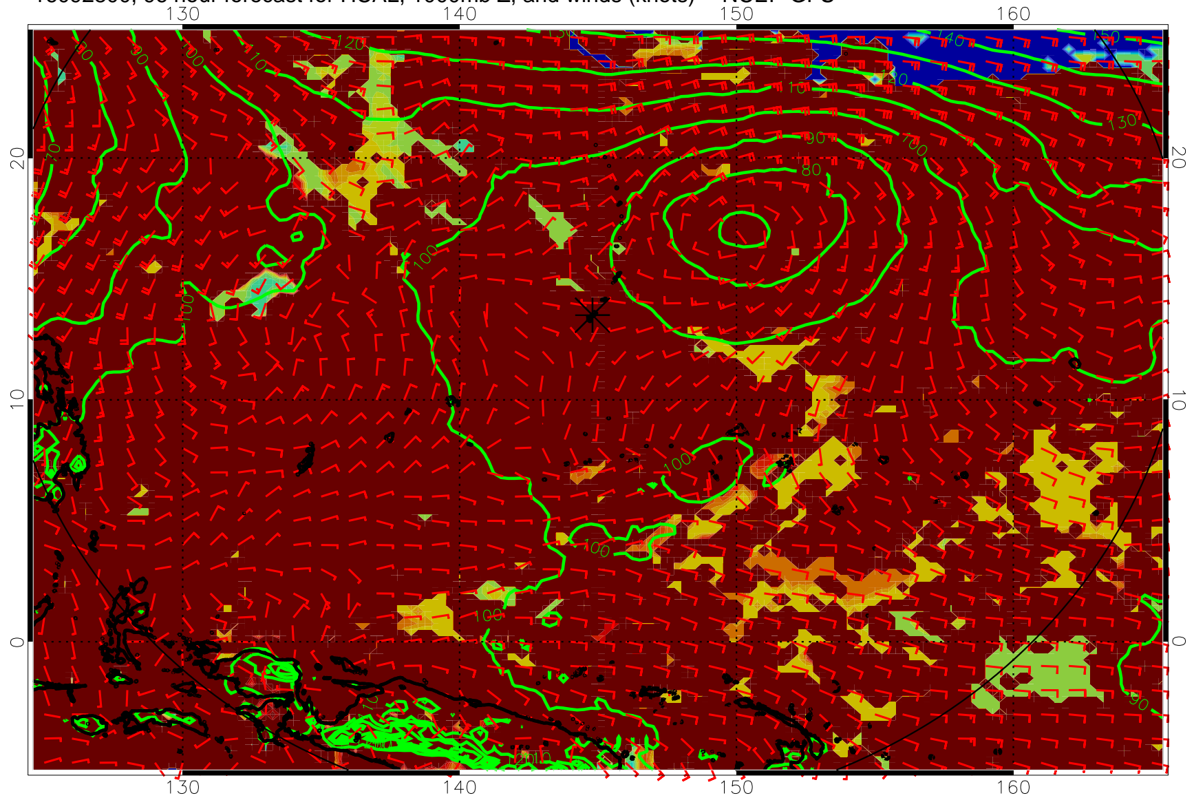
16092800, 96 hour forecast for HCAL, 1000mb Z, and winds (knots) -- NCEP GFS
