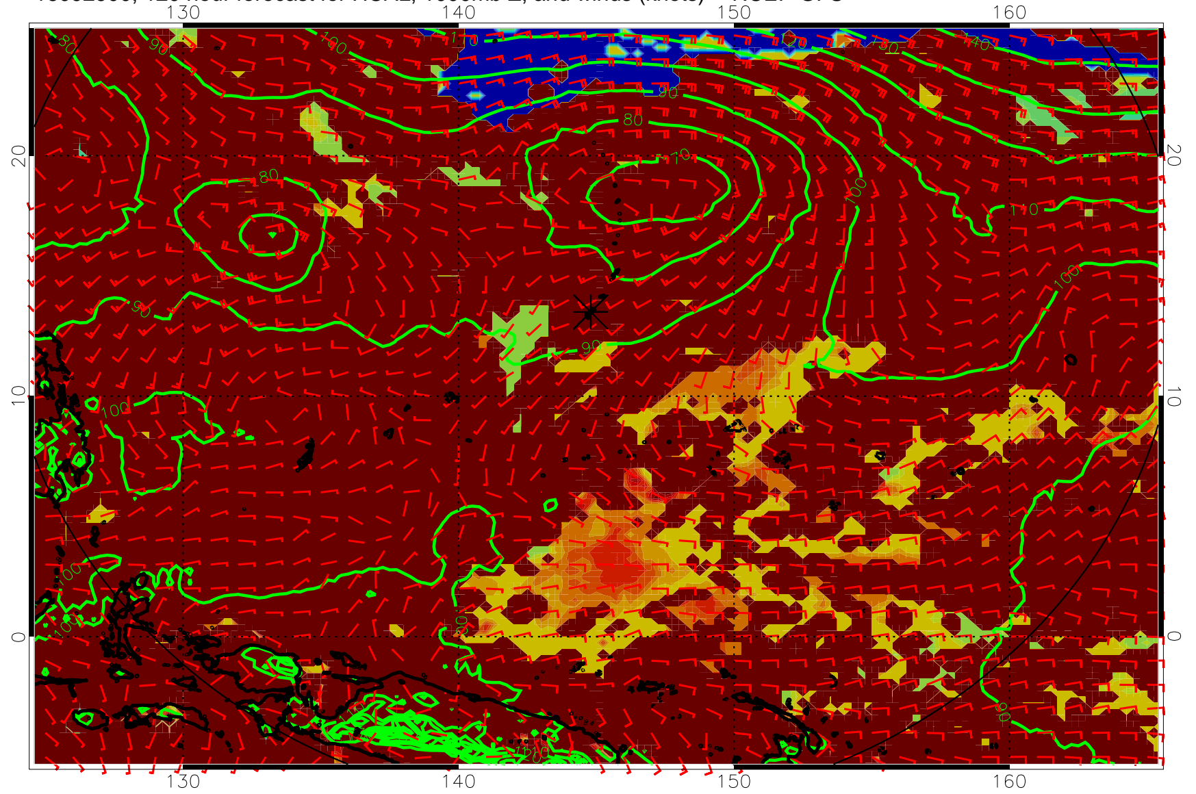
16092900, 120 hour forecast for HCAL, 1000mb Z, and winds (knots) -- NCEP GFS
