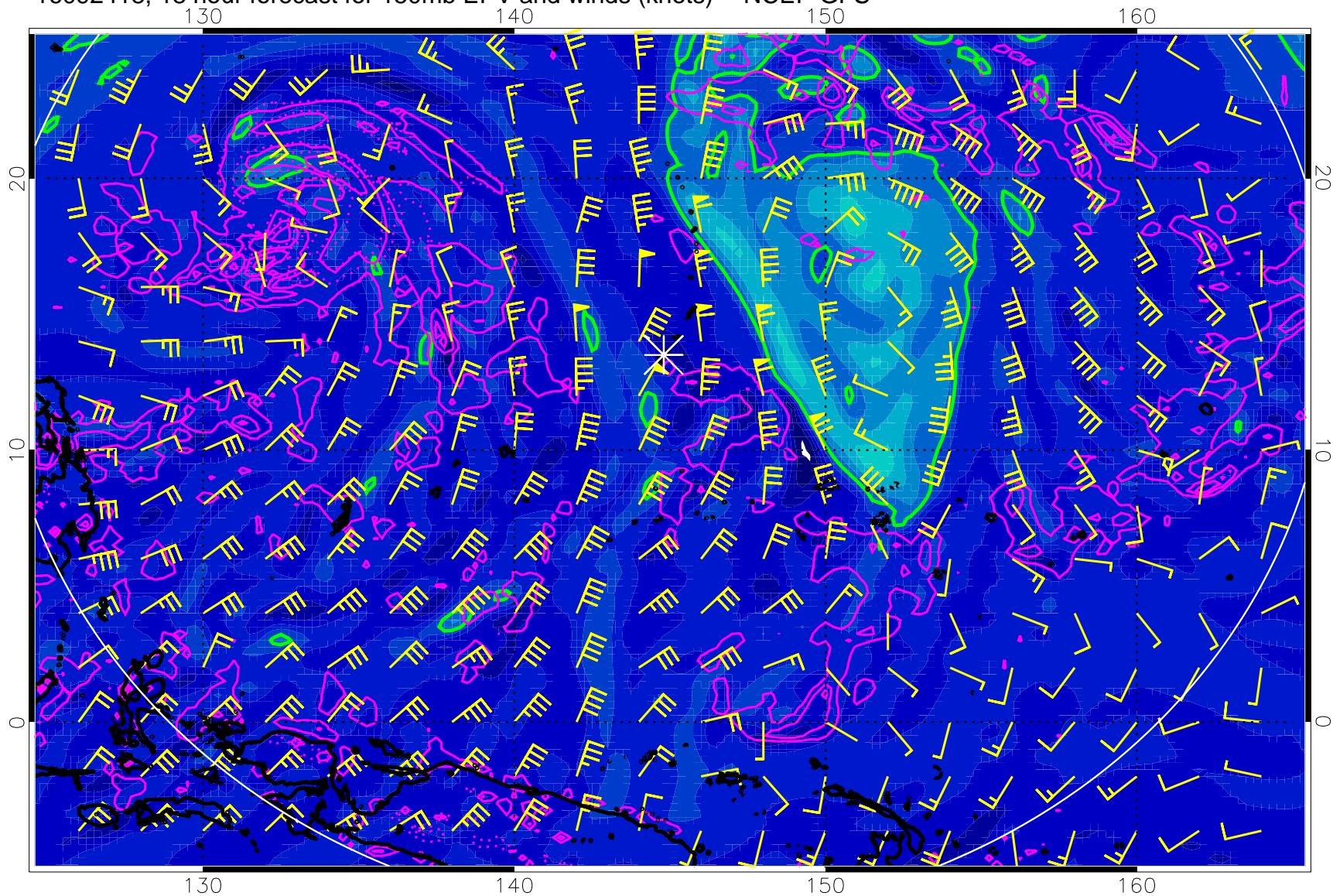
16092418, 18 hour forecast for 150mb EPV and winds (knots) -- NCEP GFS
